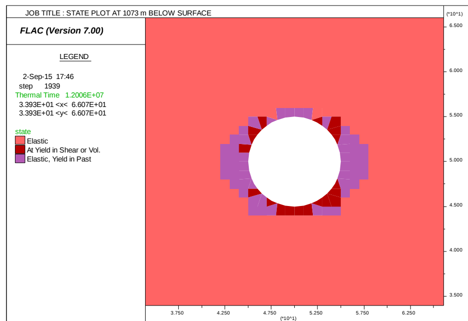
Figure 5.54: State plot at 1073 m below surface
