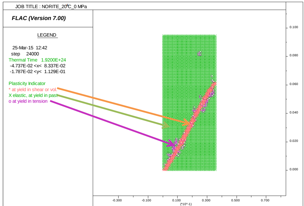
Figure 5.13: Plasticity indicator plot for norite at ambient temperature under no confinement.
