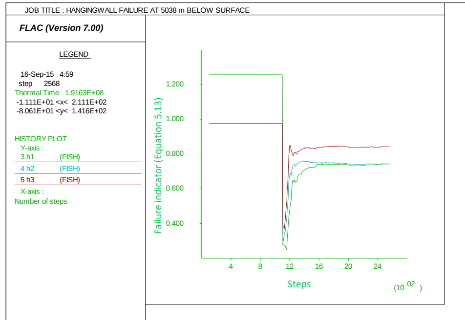
Figure 5.43: Hangingwall failure indicator at 5038 m below surface
