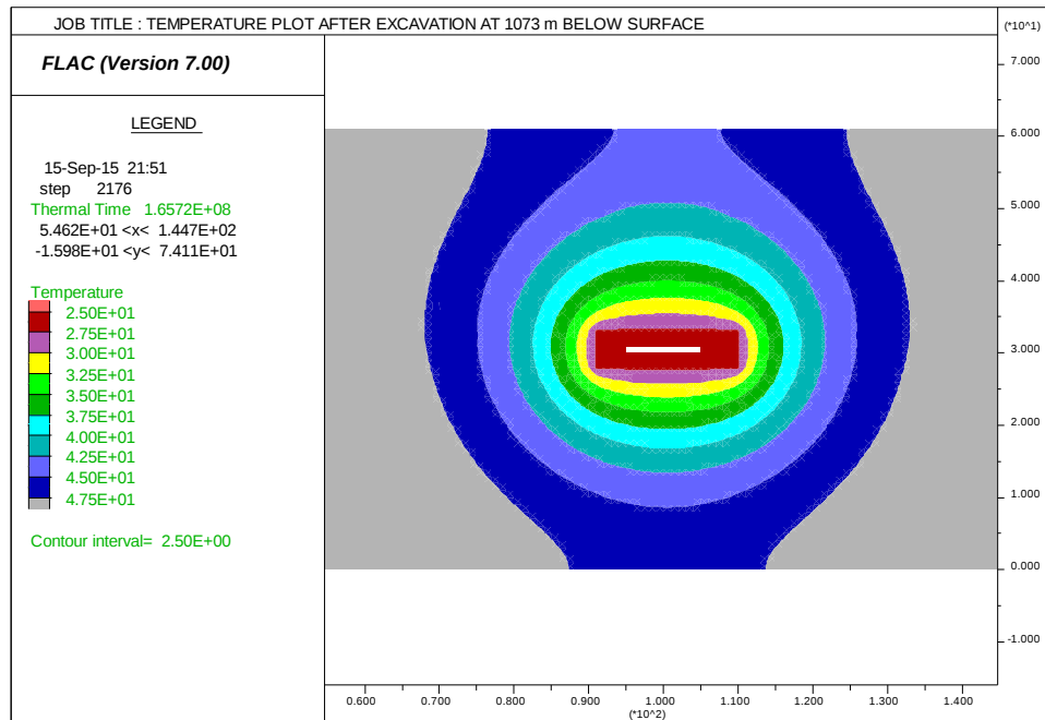
Figure 5.26: Temperature plot for the stope at 1073 m below surface.
