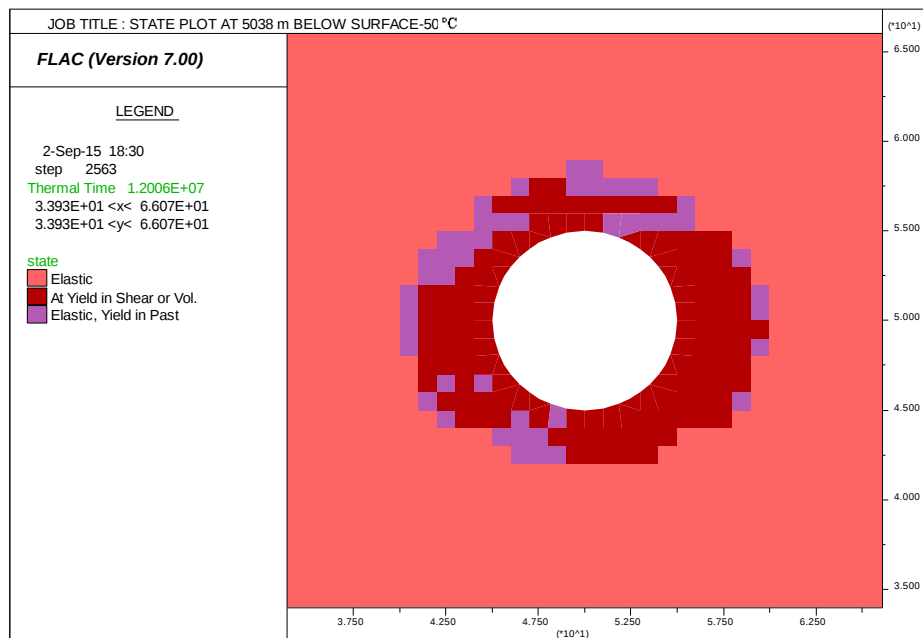
Figure 5.59: State plot for temperature 50°C at 5038 m below surface
