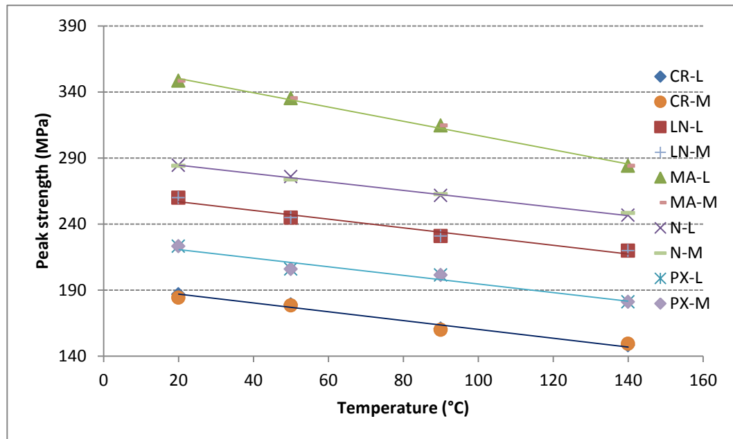
Figure 5.12: Plot of laboratory numerical modelling peak strengths
