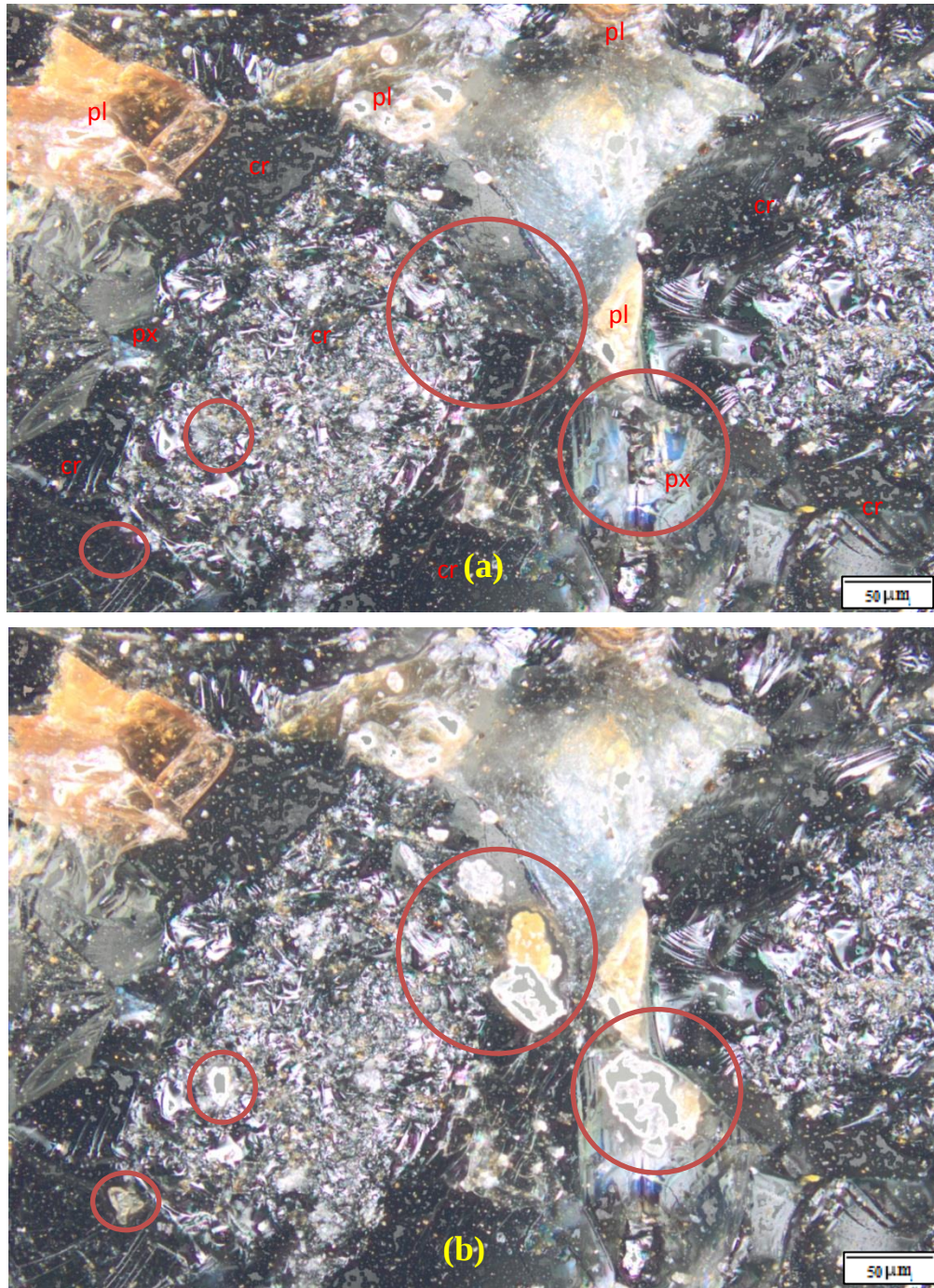
Figure 4.6: Micrograph of CR (a) before and (b) after heat treatment to 140°C
