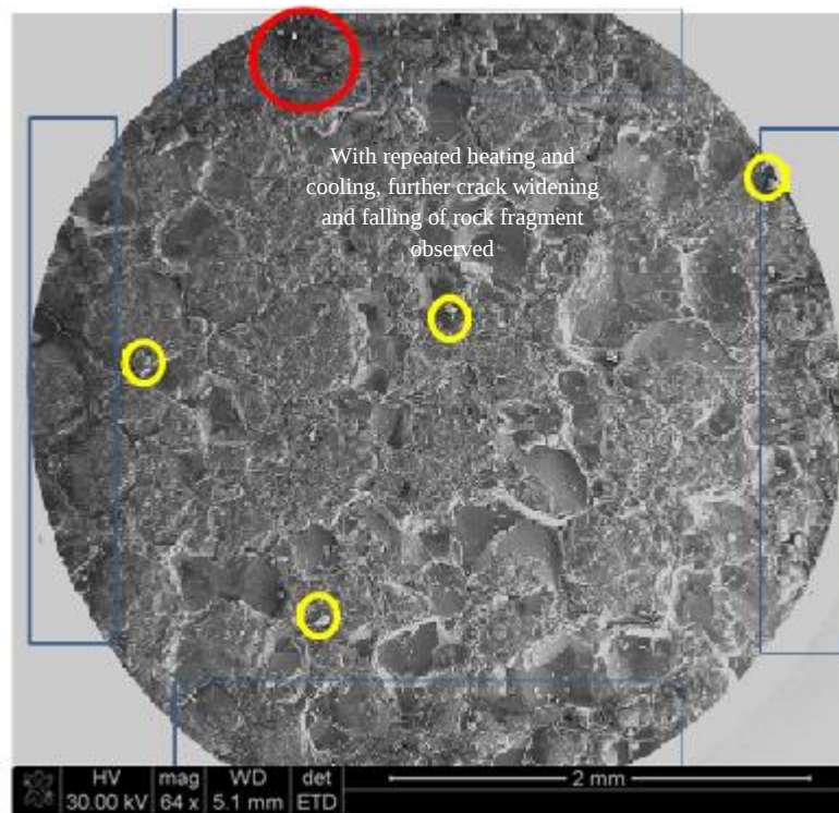
Figure 4.9: Chromitite after heat treatment to 140°C with repeated heating and cooling.
