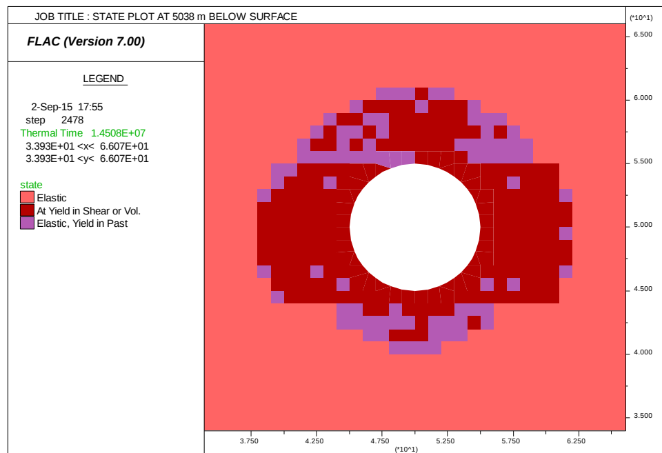
Figure 5.56: State plot at 5038 m below surface
