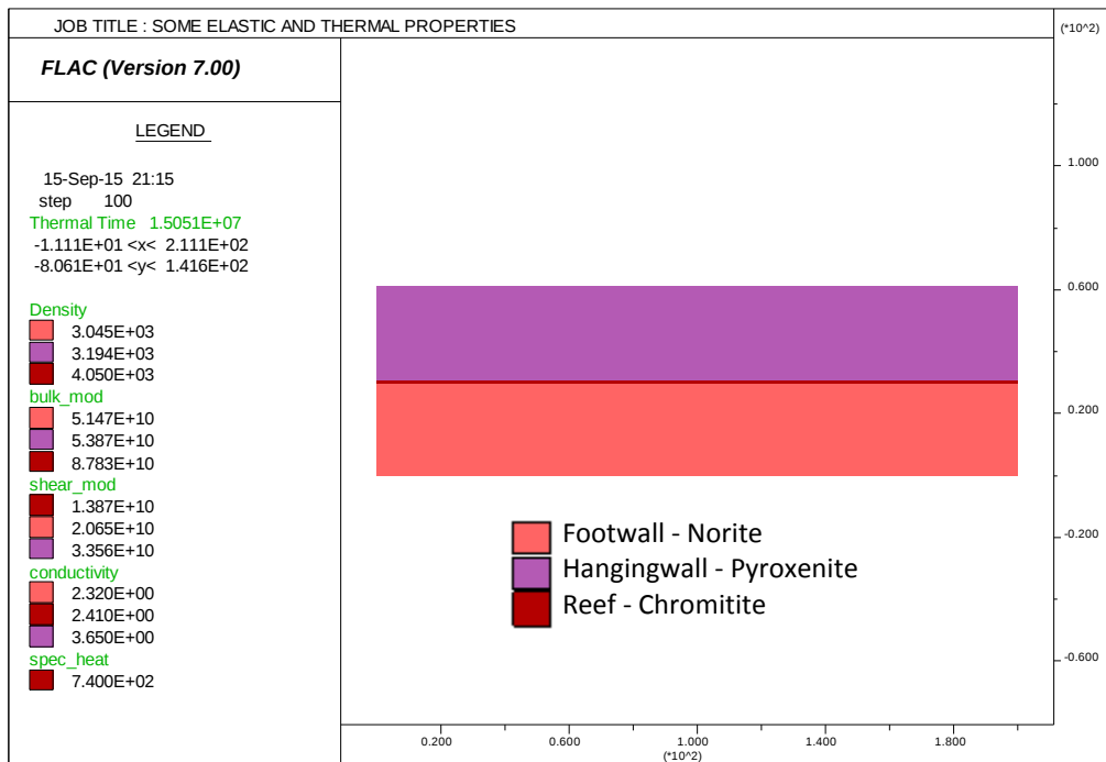
Figure 5.25: Some of the model properties for excavation at a depth of 1073 m.
