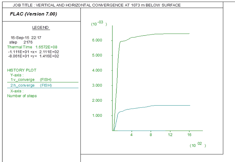
Figure 5.34: Plot of vertical and horizontal displacements at 1073 m below surface
