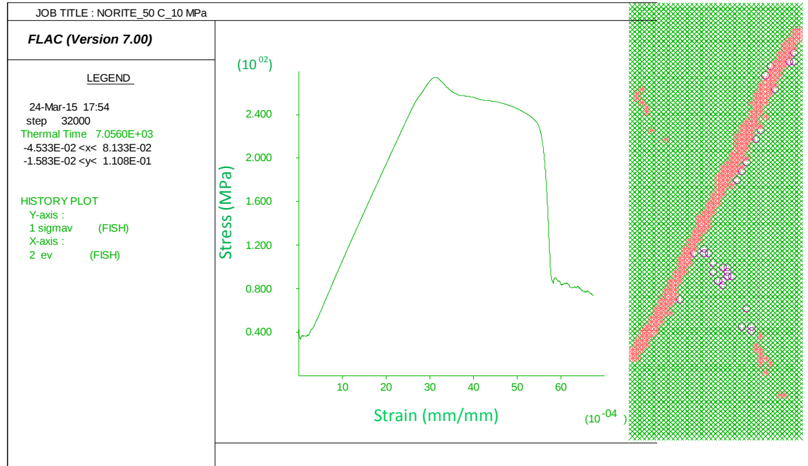
Figure 5.6: FLAC plot of norite tested at 50°C and confining pressure of 10 MPa
