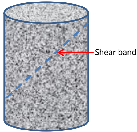
Figure 5.3: Illustration of shear band on a failed triaxial test specimen.
