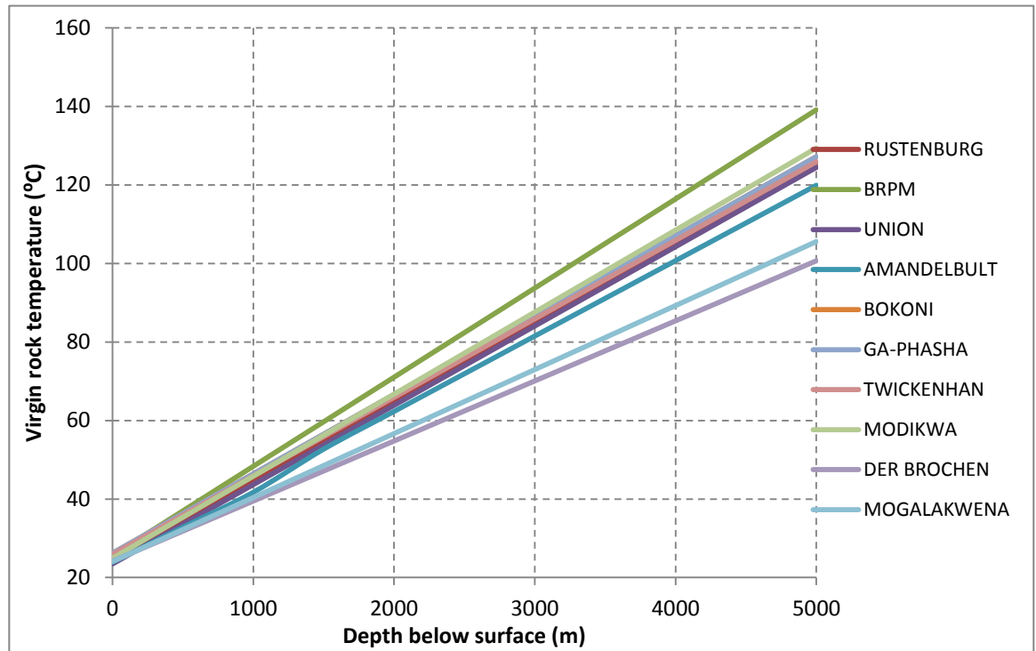
Figure 5.1: Graph of virgin rock temperature against depth for platinum mines (Erasmus, 2012)
