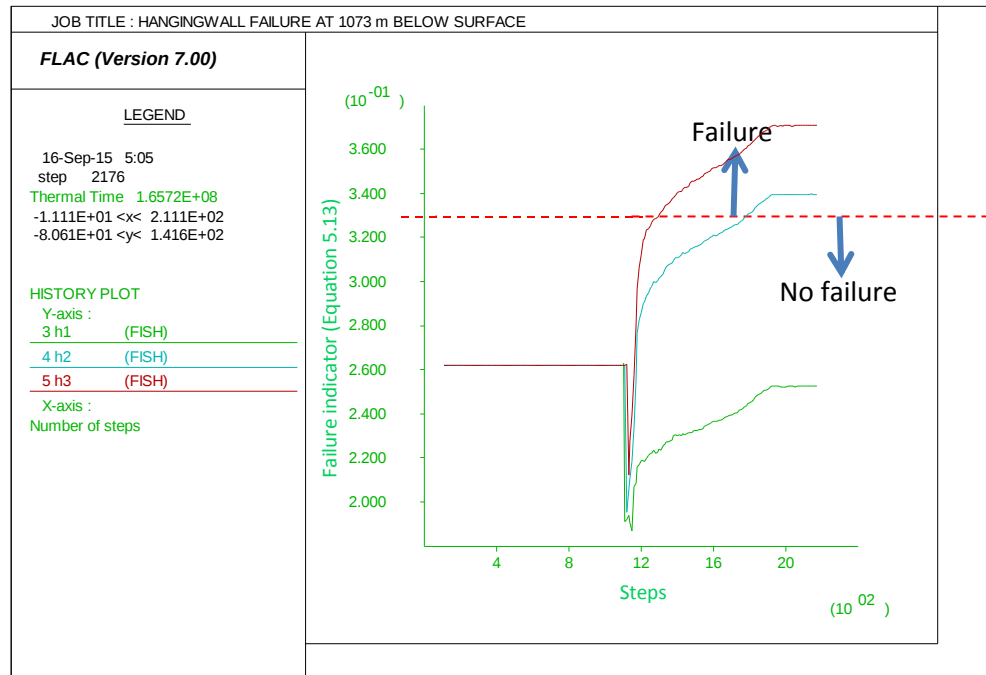
Figure 5.41: Hangingwall failure indicator at 1073 m below surface
