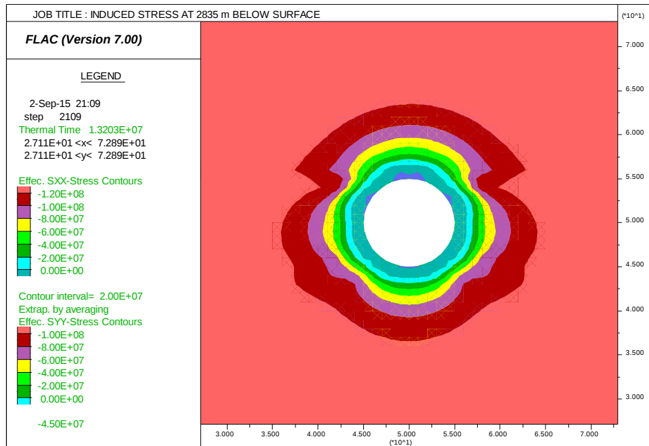
Figure 5.52: Plot of induced stresses at 2835 m below surface
