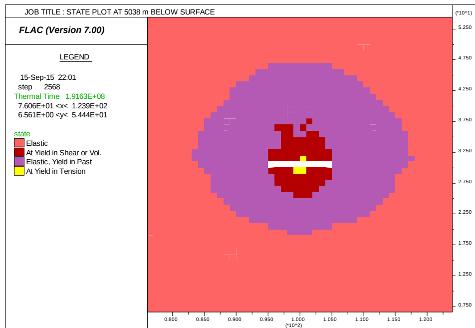
Figure 5.30: State plot at 5038 m below surface
