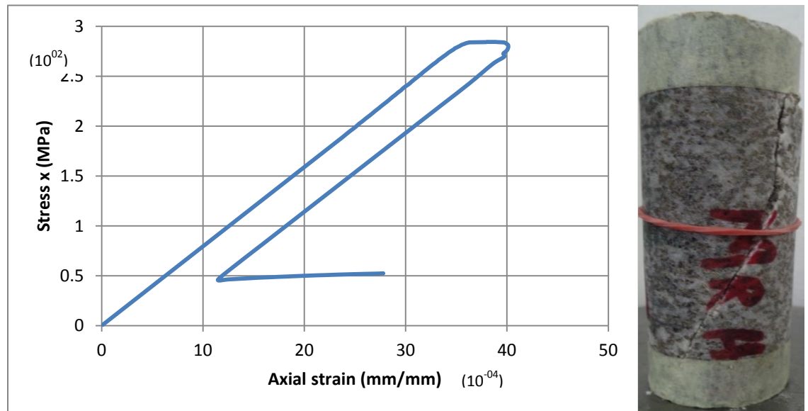
Figure 5.5: Laboratory plot of norite tested at 20°C and confining pressure of 10 MPa
