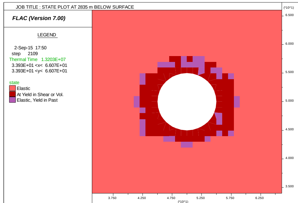
Figure 5.55: State plot at 2835 m below surface
