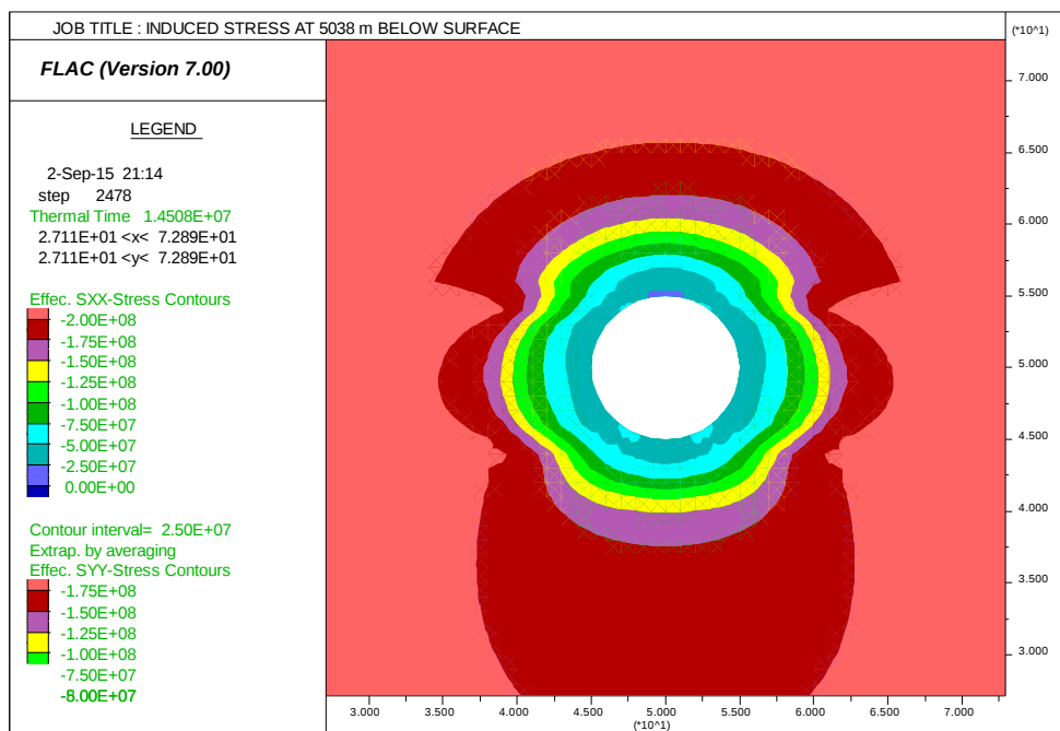
Figure 5.53: Plot of induced stresses at 5038 m below surface
