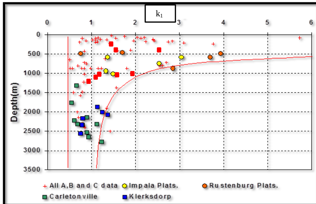
Figure 5.18: Major horizontal to vertical stress ratio as a function of depth (Stacey and Wesseloo, 1998)
