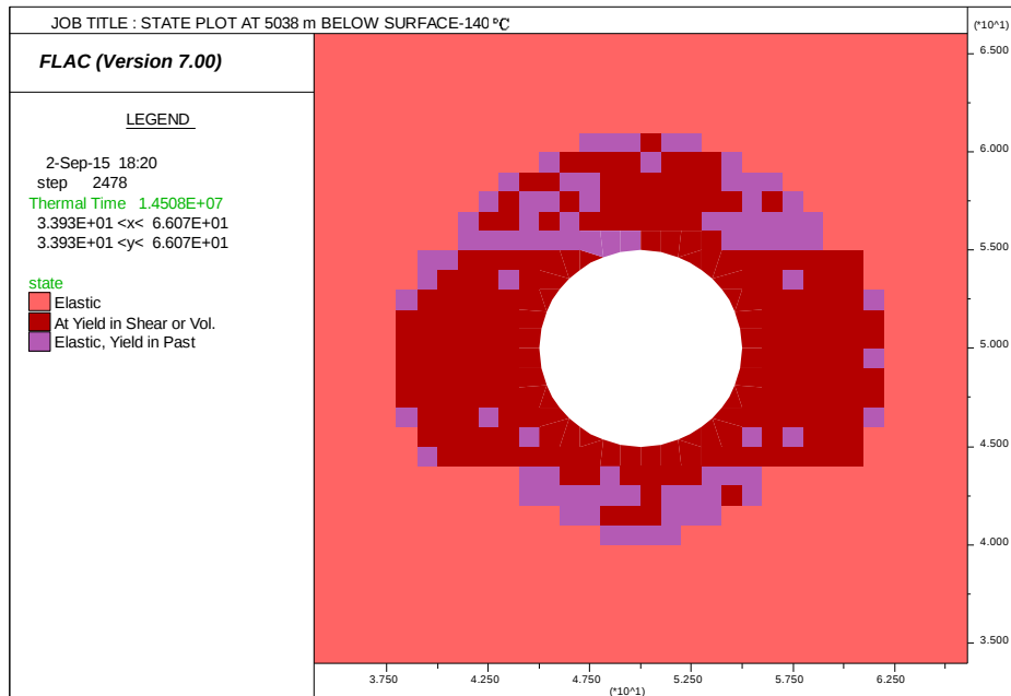
Figure 5.58: State plot for temperature 140°C at 5038 m below surface
