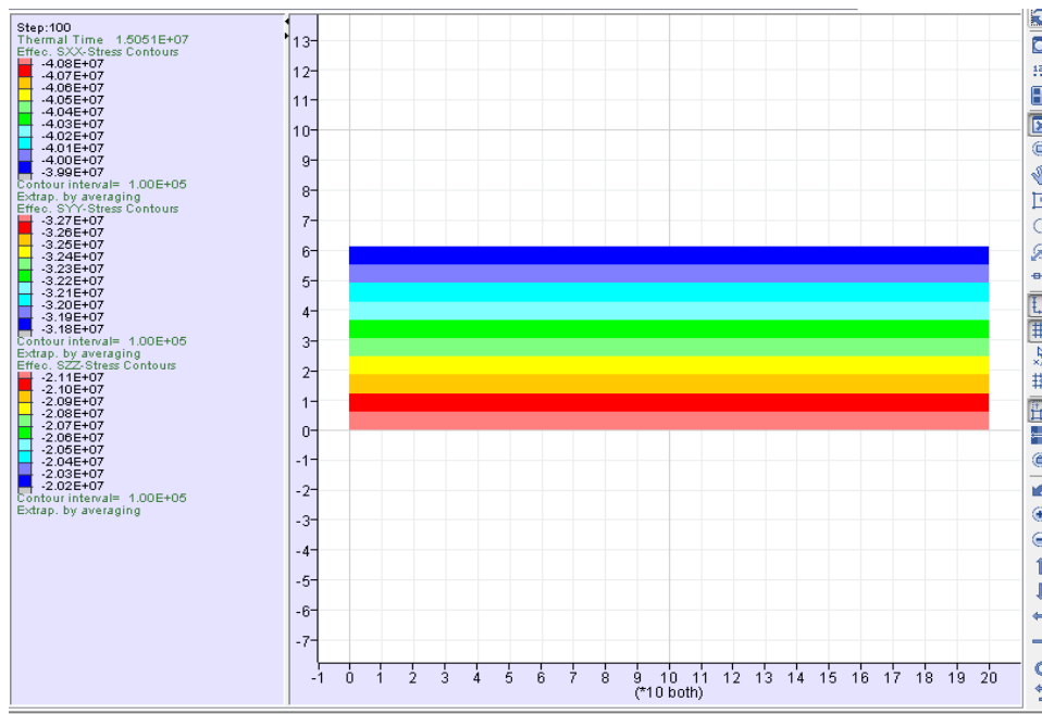
Figure 5.27: Plot of the pre-mining in-situ stresses at 1073 m below surface
