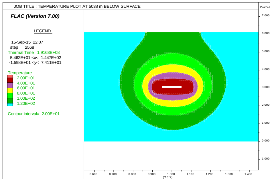
Figure 5.31: Post-excavation temperature at 5038 m below surface
