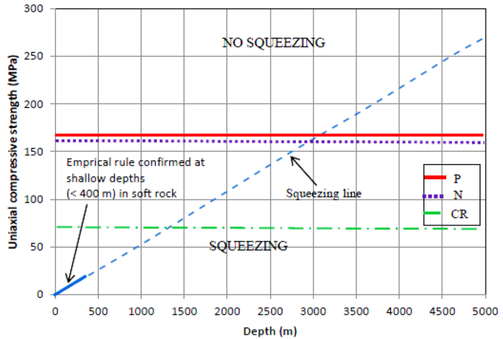
Figure 5.32: Hypothetical squeezing conditions of ultra-deep mining excavations in hard rocks (Malan and Basson, 1998)
