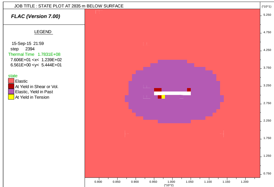
Figure 5.29: State plot at 2835 m below surface
