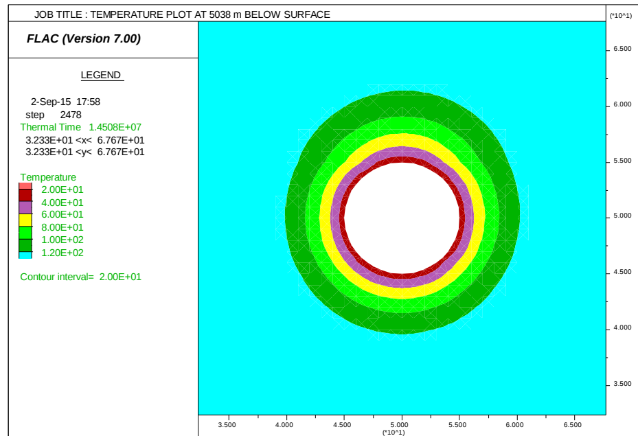
Figure 5.57: Post-excavation temperature at 5038 m below surface
