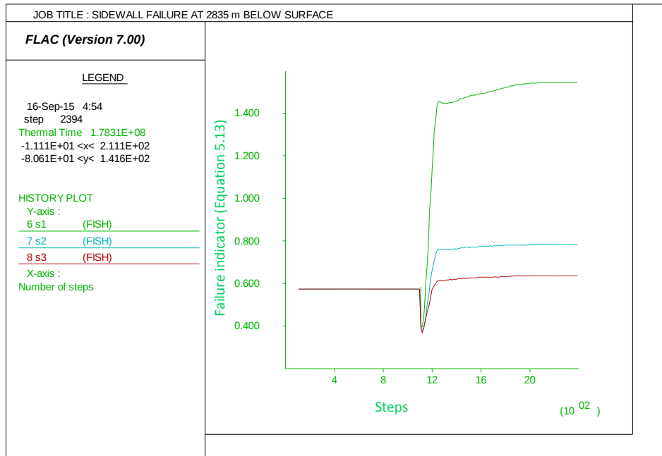
Figure 5.39: Sidewall failure indicator at 2835 m below surface
