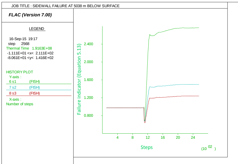
Figure 5.40: Sidewall failure indicator at 5038 m below surface
