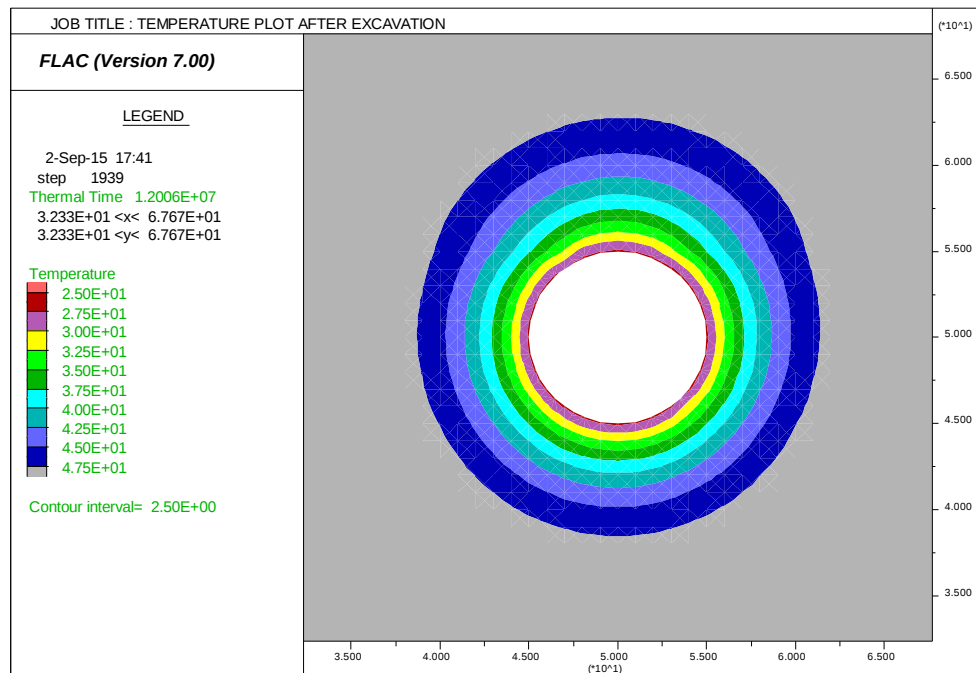
Figure 5.50: Temperature plot for the slope at 1073 m below surface.
