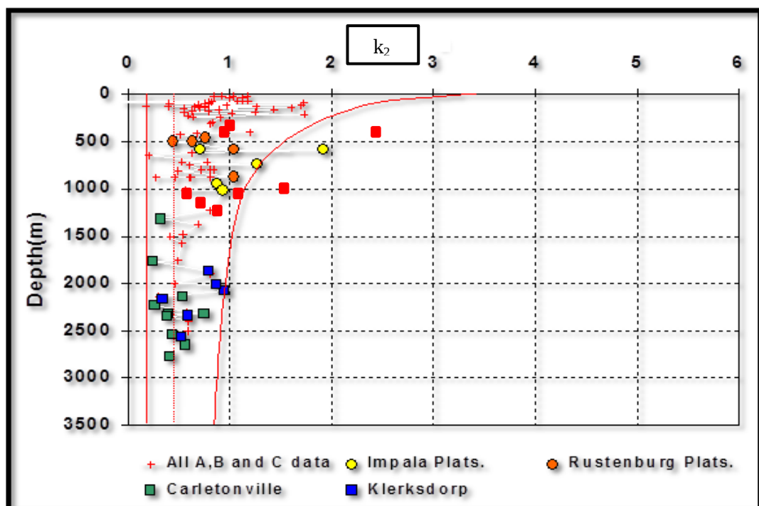
Figure 5.19: Minor horizontal to vertical stress ratio as a function of depth (Stacey and Wesseloo, 1998)
