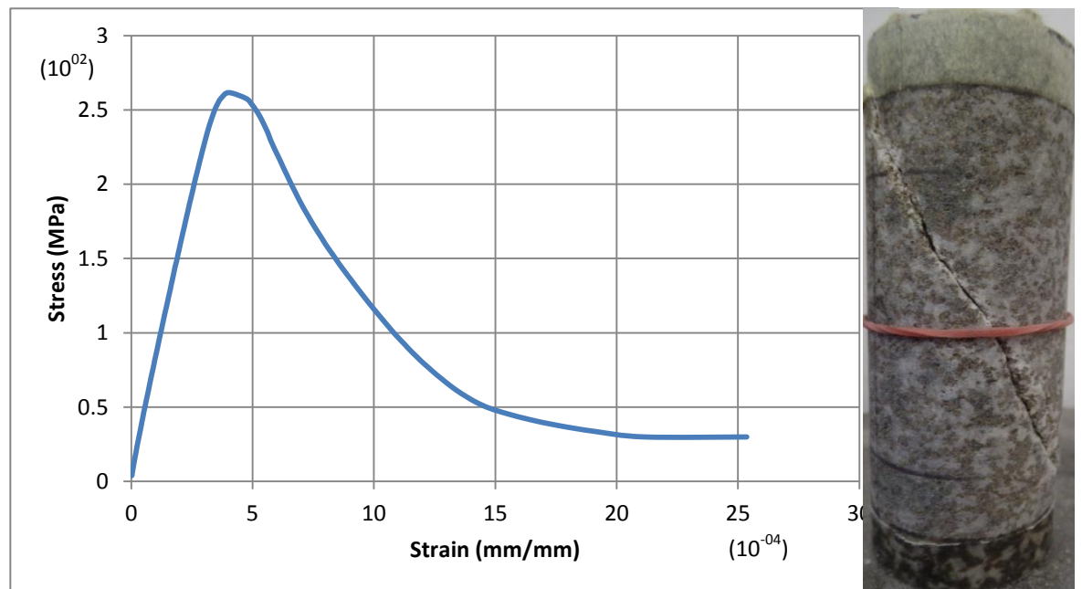
Figure 5.9: Laboratory plot of norite tested at 90°C and confining pressure of 10 MPa
