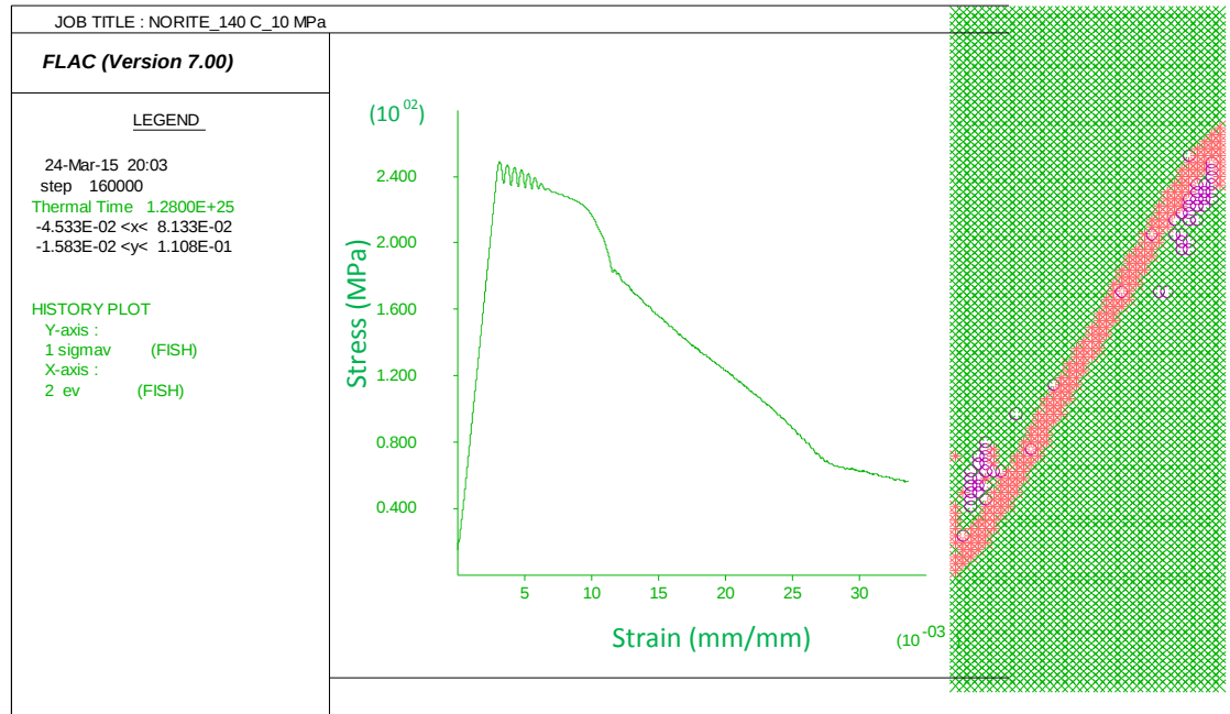
Figure 5.10: FLAC plot of norite tested at 140°C and confining pressure of 10 MPa
