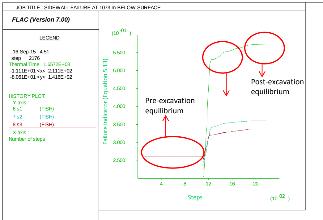
Figure 5.38: Sidewall failure indicator at 1073 m below surface
