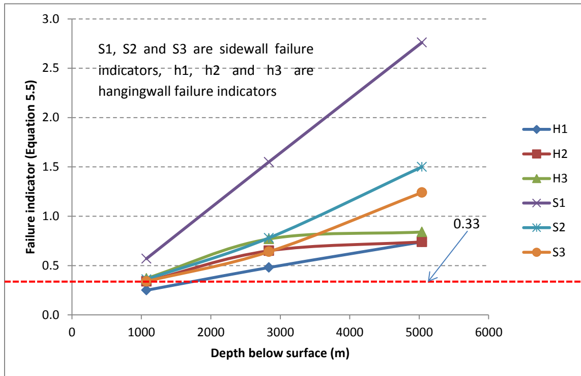
Figure 5.44: Comparison of sidewall and hangingwall failure indicators at different depths
