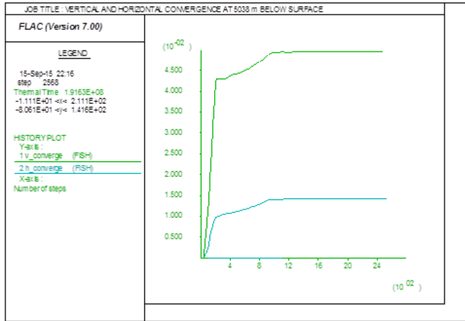
Figure 5.36: Plot of vertical and horizontal displacements at 5038 m below surface
