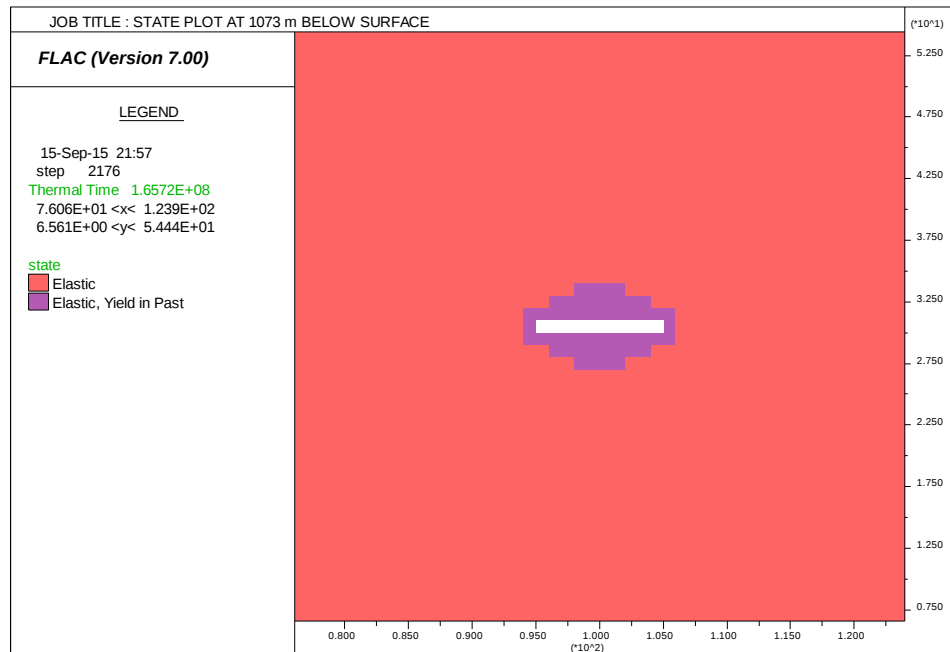
Figure 5.28: State plot at 1073 m below surface
