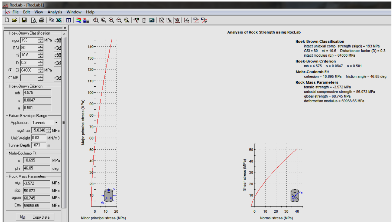
Figure 5.21: Screen shot of RocLab software used for the determination of rock mass parameters
