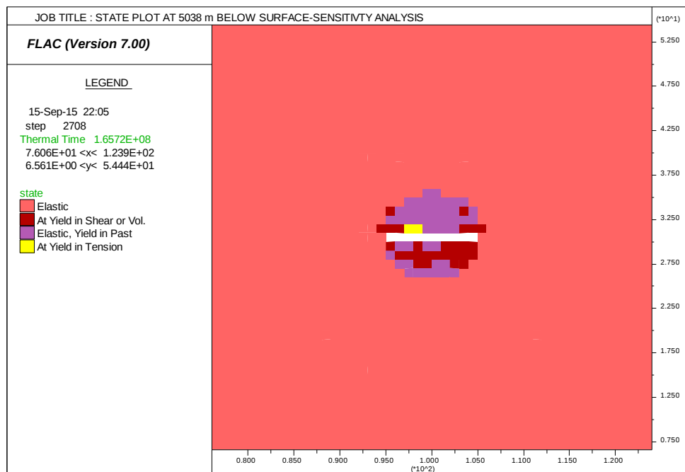
Figure 5.47: State plot for temperature 50°C at 5038 m below surface
