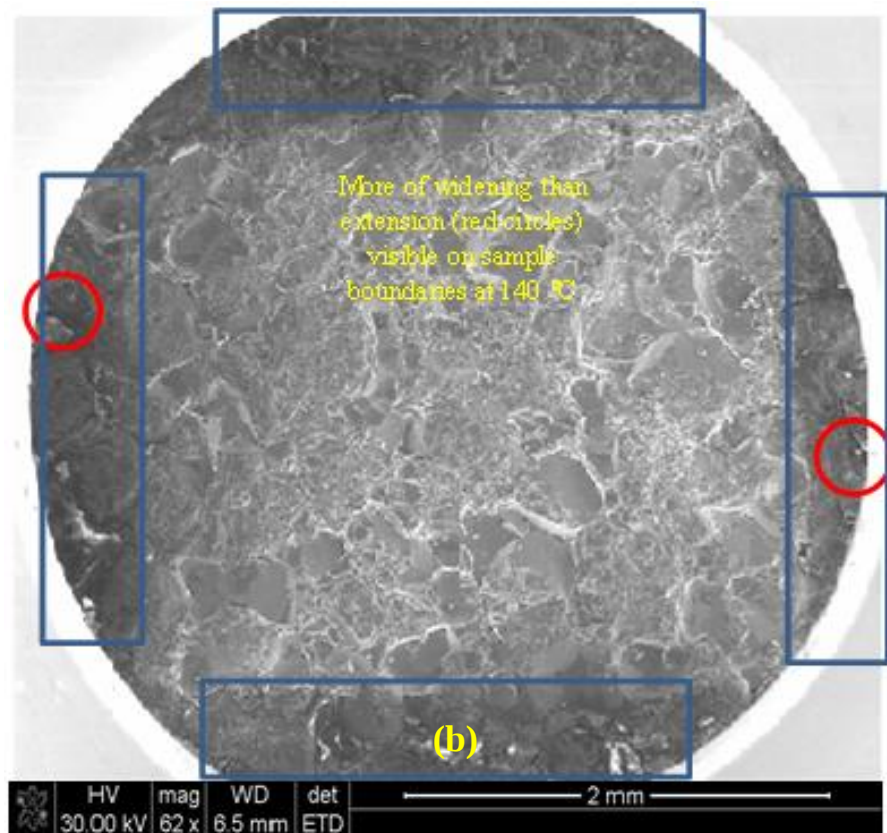
Figure 4.8: Chromitite after heat treatment to (a) 100°C (b) 140°C
