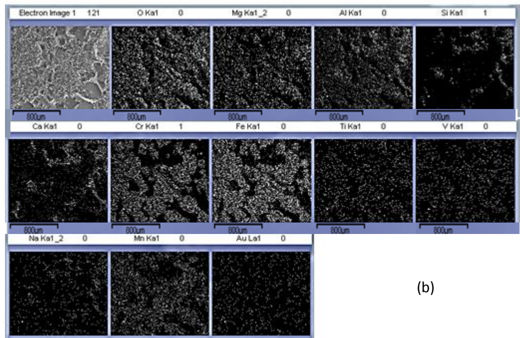
Figure 4.12: Element map of chromitite (a) before and (b) after heat treatment to 50°C
