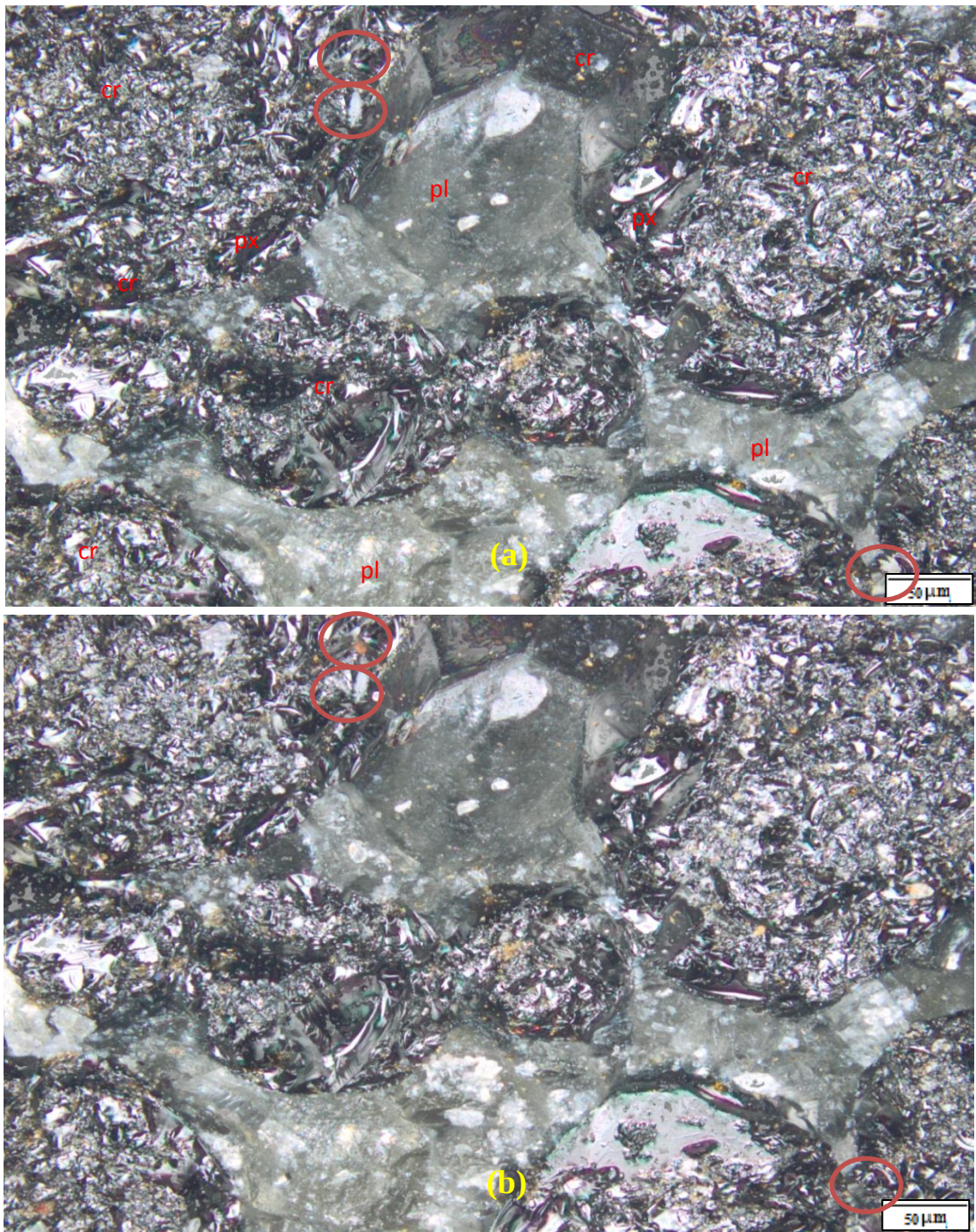
Figure 4.4: Micrograph of CR (a) before and (b) after heat treatment to 50°C
