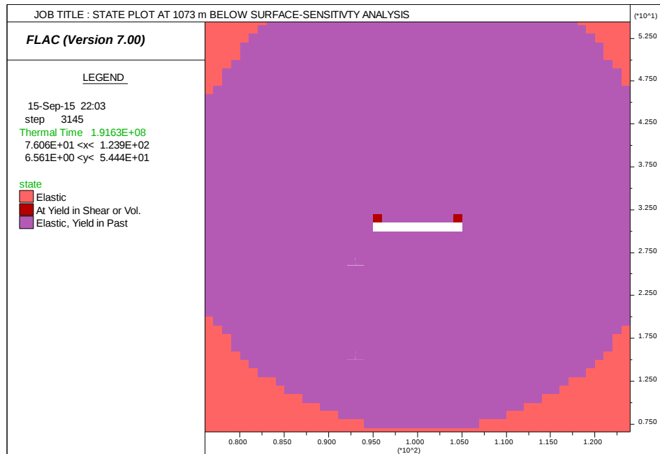
Figure 5.48: State plot for temperature 140°C at 1073 m below surface
