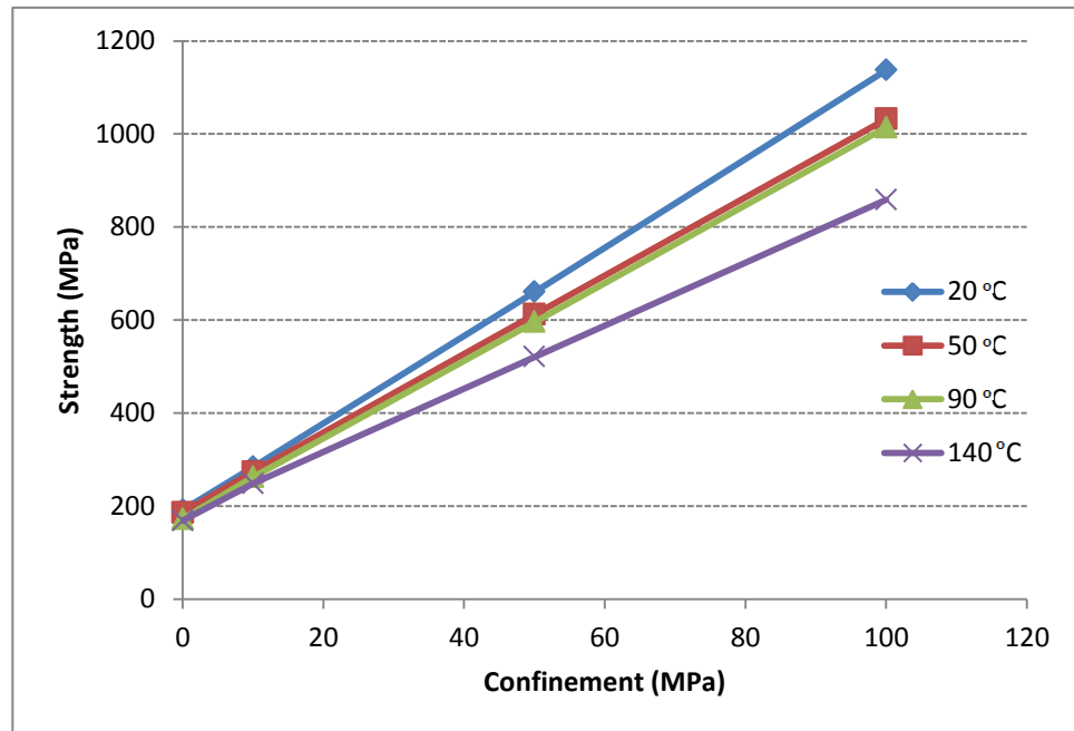
Figure 5.16: Peak strength of norite at various temperatures and confining pressure
