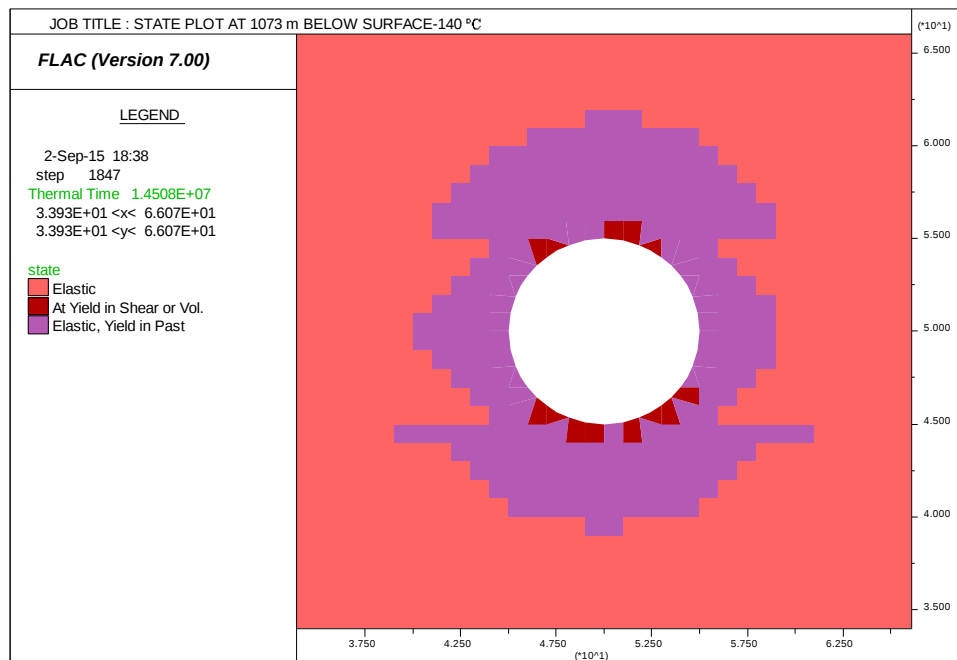
Figure 5.60: State plot for temperature 140°C at 1073 m below surface
