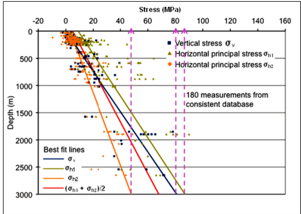
Figure 5.20: Plot of consistent stress measurement database (Handley, 2013).
