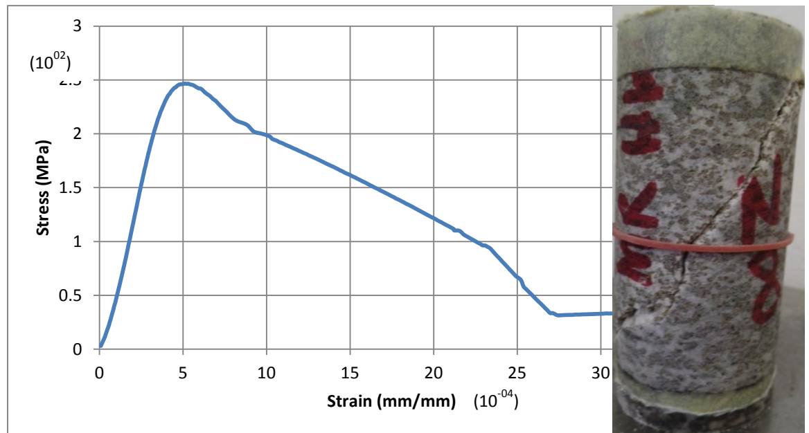
Figure 5.11: Laboratory plot of norite tested at 140°C and confining pressure of 10 MPa
