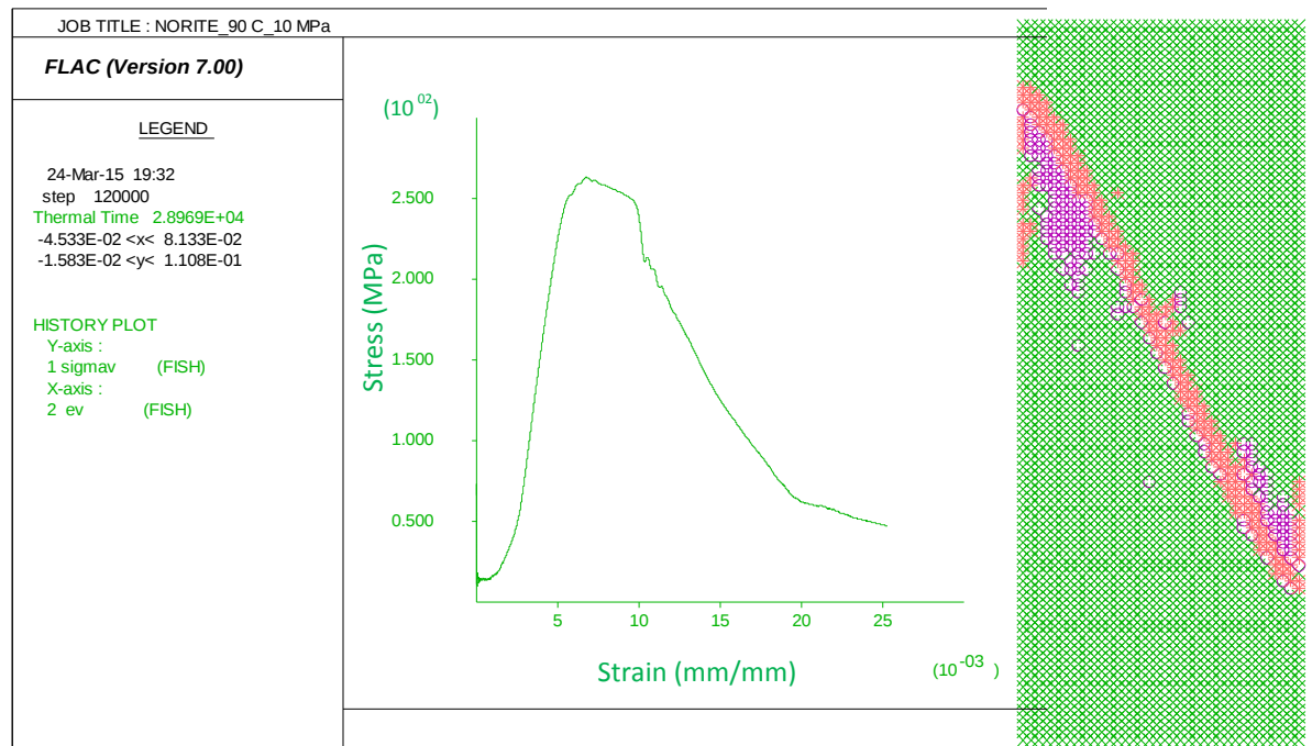
Figure 5.8: FLAC plot of norite tested at 90°C and confining pressure of 10 MPa
