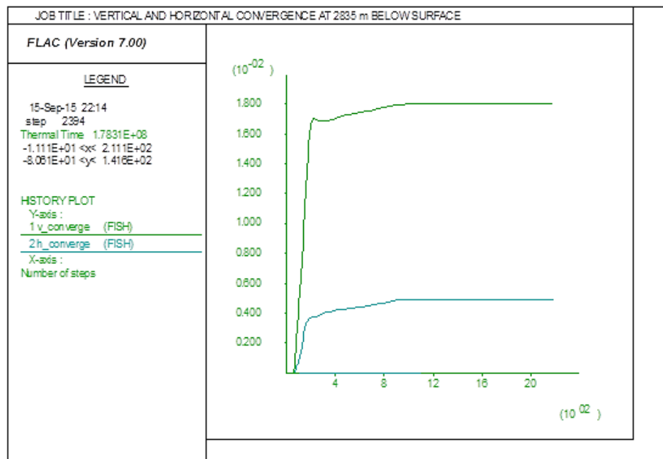
Figure 5.35: Plot of vertical and horizontal displacements at 2835 m below surface
