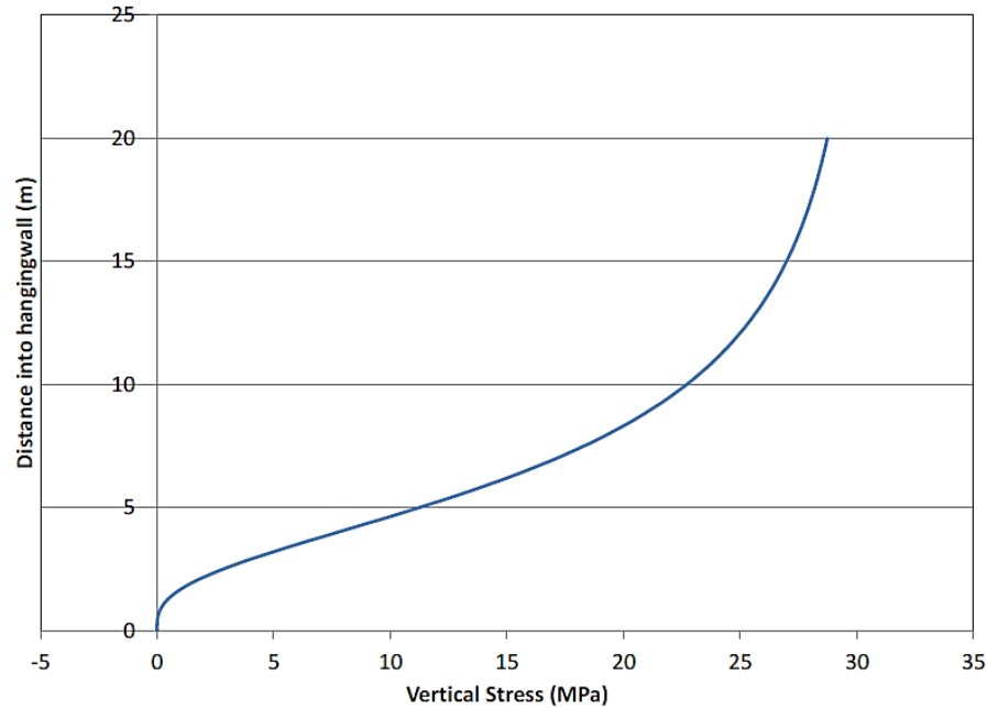
Figure 5.23: Plot of equation 5.5 (Malan (2015), personal communication.)
