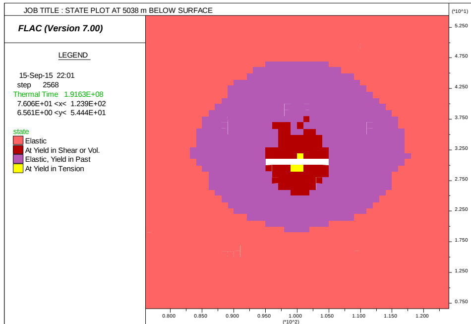
Figure 5.46: State plot for temperature 140°C at 5038 m below surface
