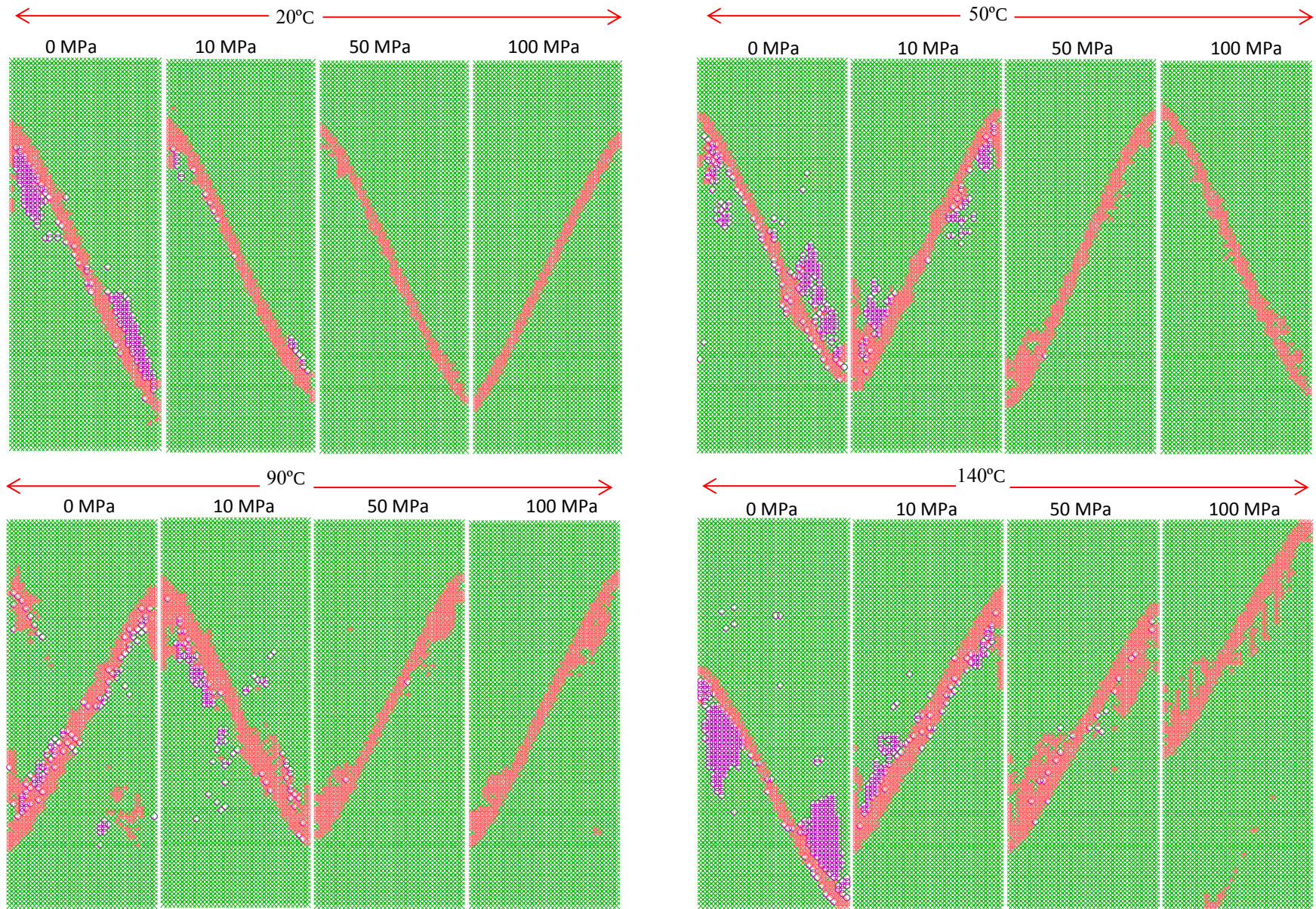
Figure 5.15: Plasticity indicator of chromitite sample at different temperature and confining pressure
