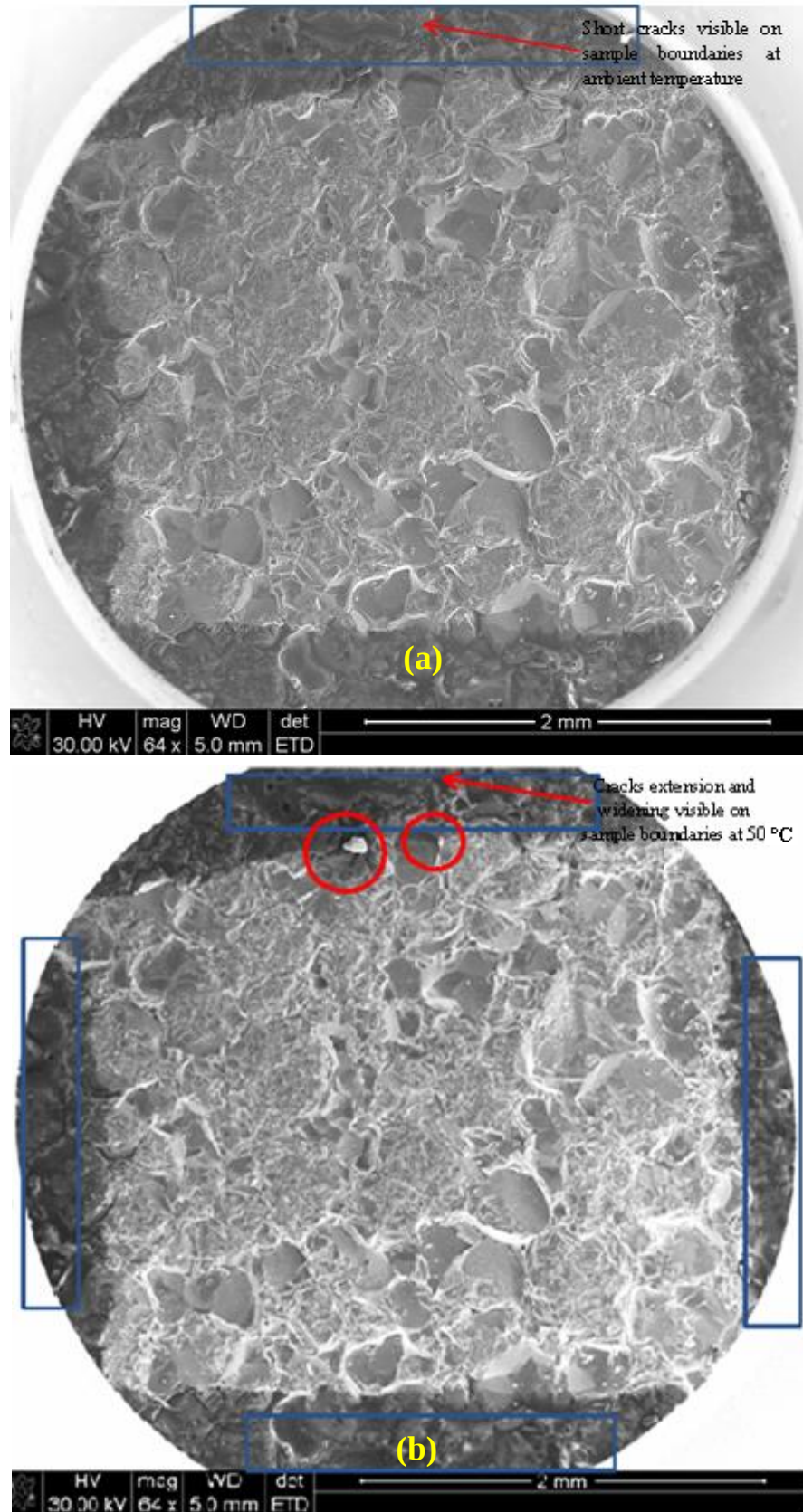
Figure 4.7: Chromitite (a) before and (b) after heat treatment to 50°C
