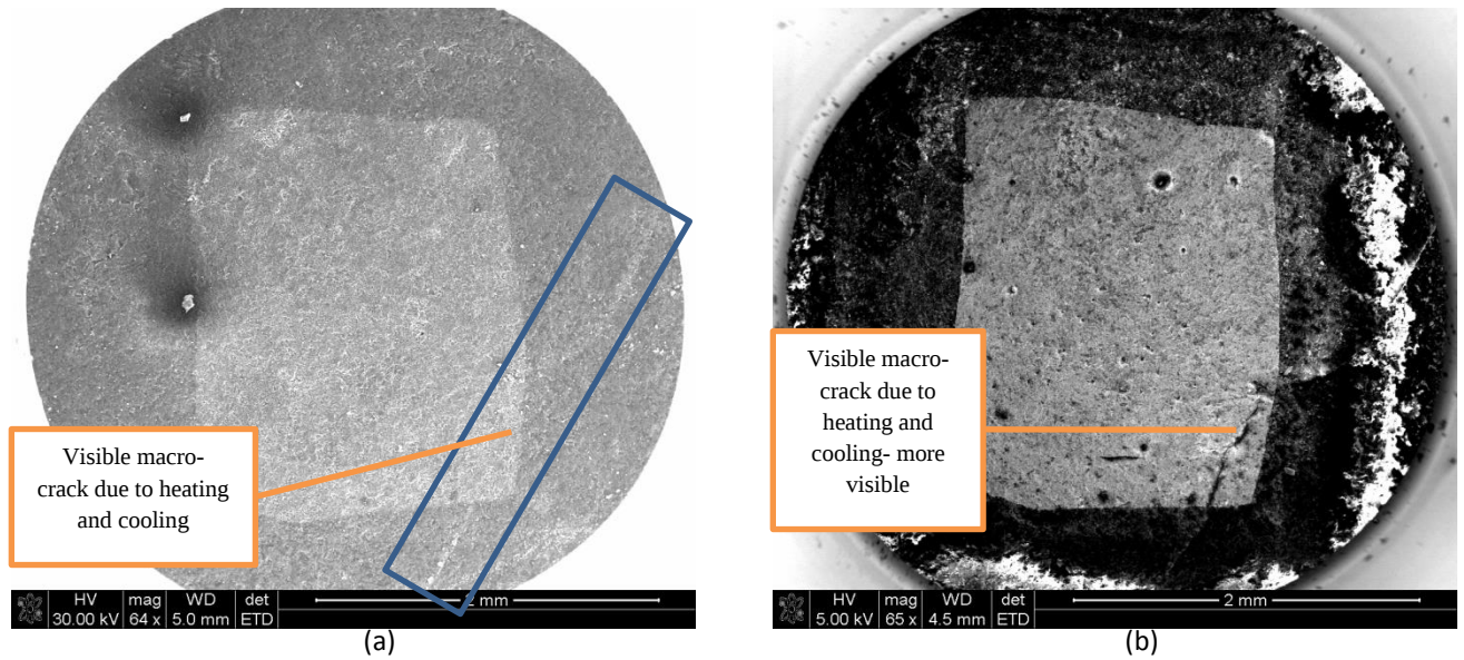
Figure 4.11: Granite subjected to repeated heating and cooling (a) after sputter coating, (b) before sputter coating
