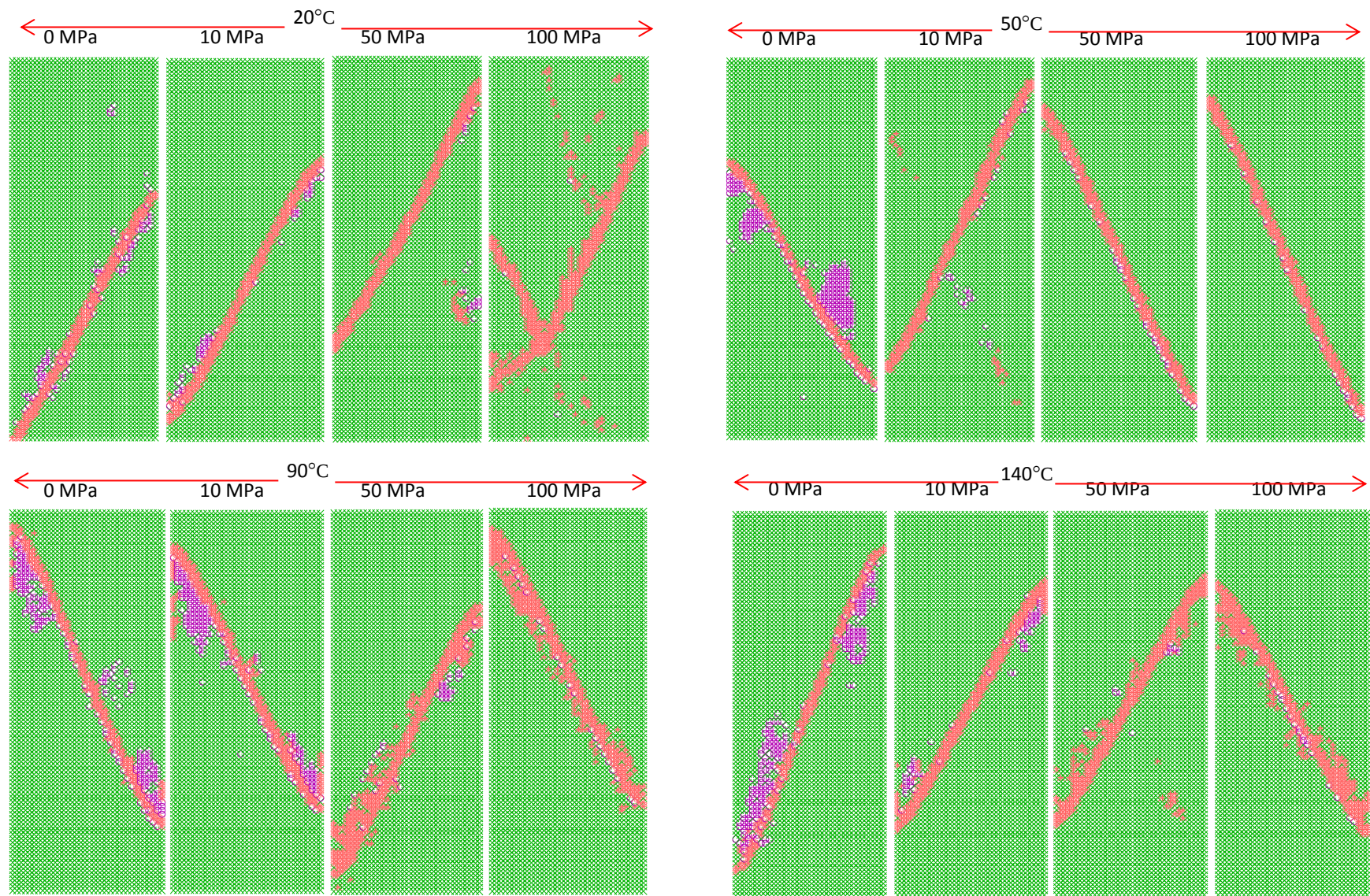
Figure 5.14: Plasticity indicator of norite sample at different temperature and confining pressure
