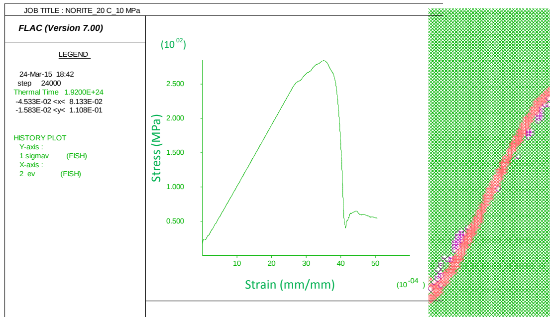
Figure 5.4: FLAC plot of norite tested at 20°C and confining pressure of 10 MPa
