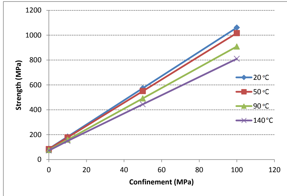
Figure 5.17: Peak strength of chromitite at various temperatures and confining pressure
