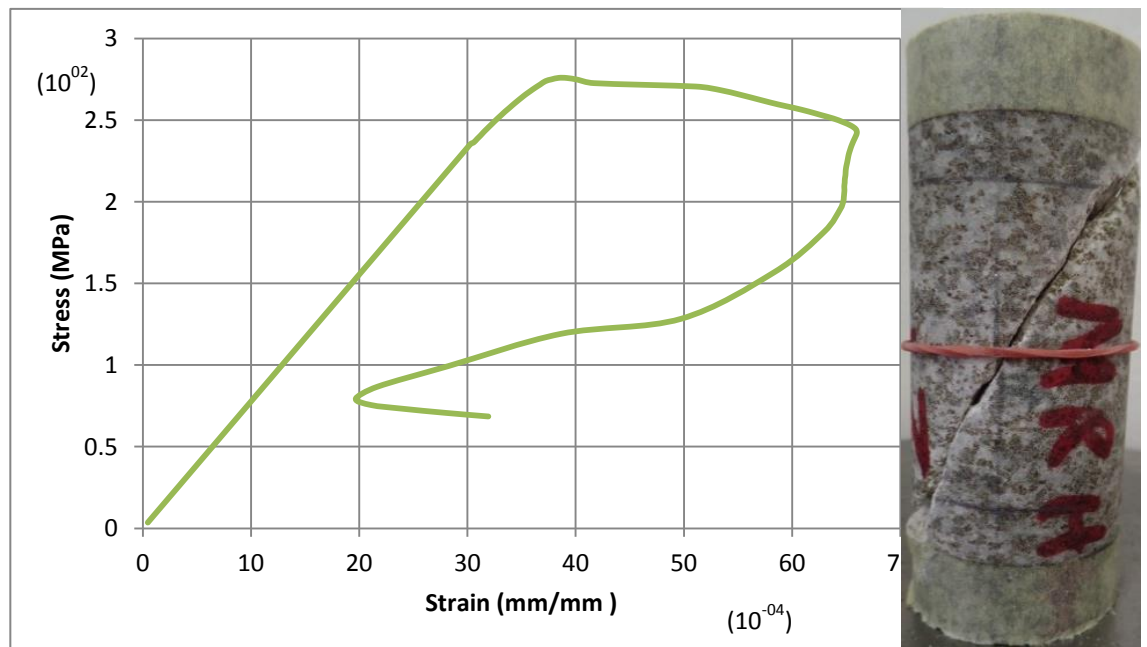
Figure 5.7: Laboratory plot of norite tested at 50°C and confining pressure of 10 MPa
