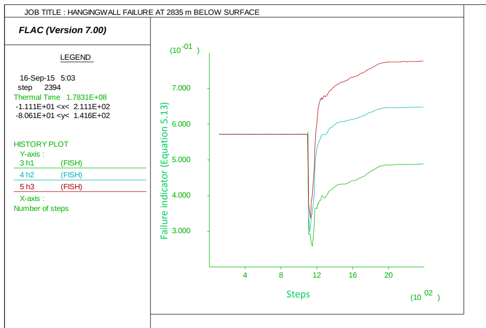
Figure 5.42: Hangingwall failure indicator at 2835 m below surface
