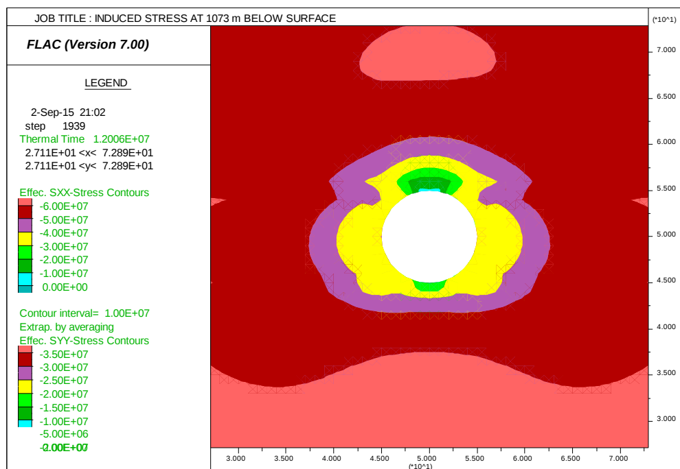
Figure 5.51: Plot of induced stresses at 1073 m below surface
