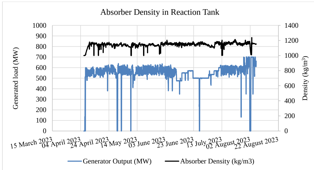
Figure 4.2.1.3-2: Actual absorber density
