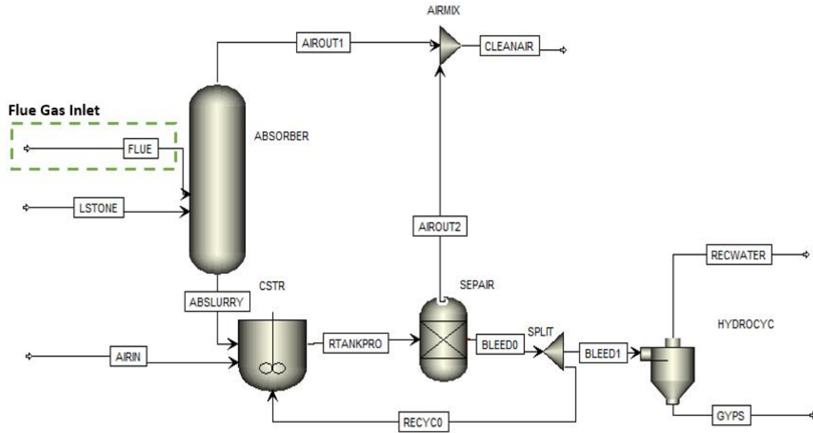
Figure 5.2-2: WFGD Absorber with variable flue gas flow volume
