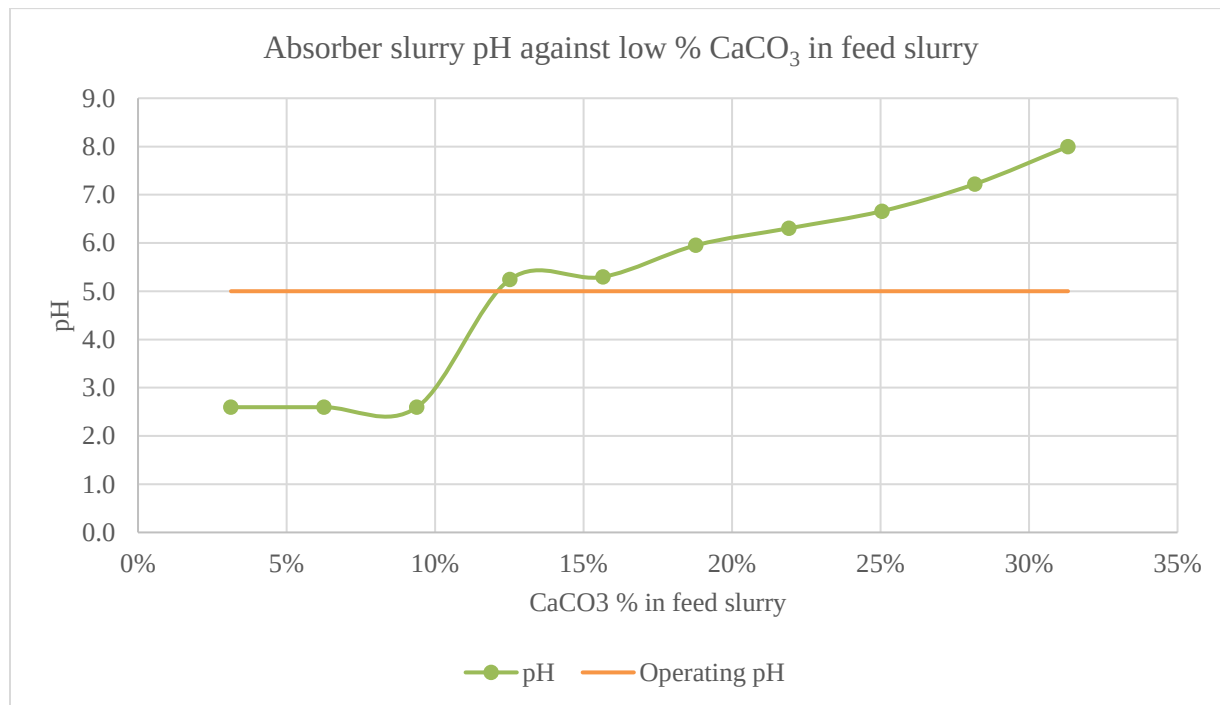
Figure 5.1-5: Absorber slurry pH vs \text{CaCO}_3 % in feed slurry
