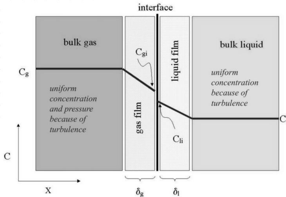
Figure 3.5.1-3: Two film theory (Liu, 2023)
