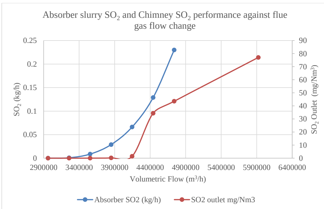
Figure 5.2-5: Absorber outlet SO 2 emissions
