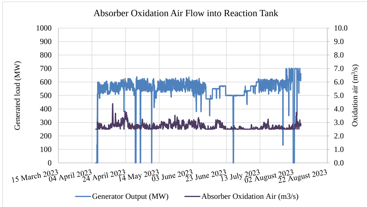
Figure 4.2.1.4-1: Actual oxidation air
