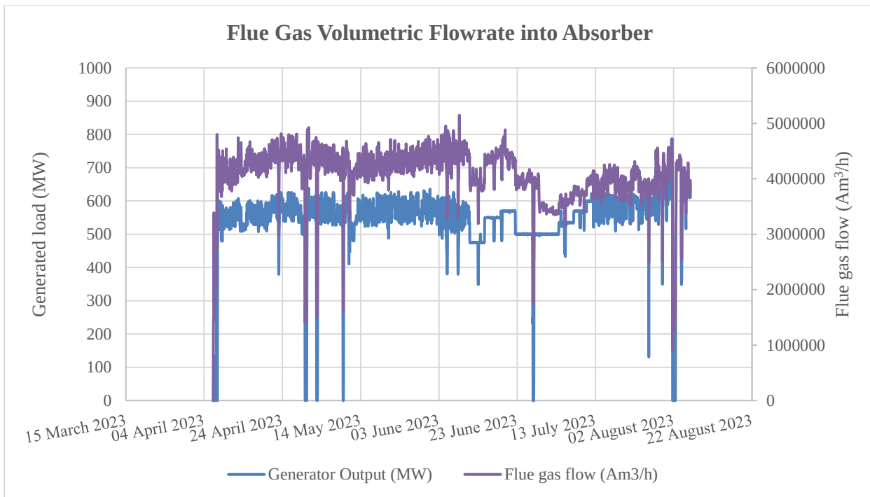
Figure 4.2.1.1-1: Actual Volumetric Flue Gas Flowrates
