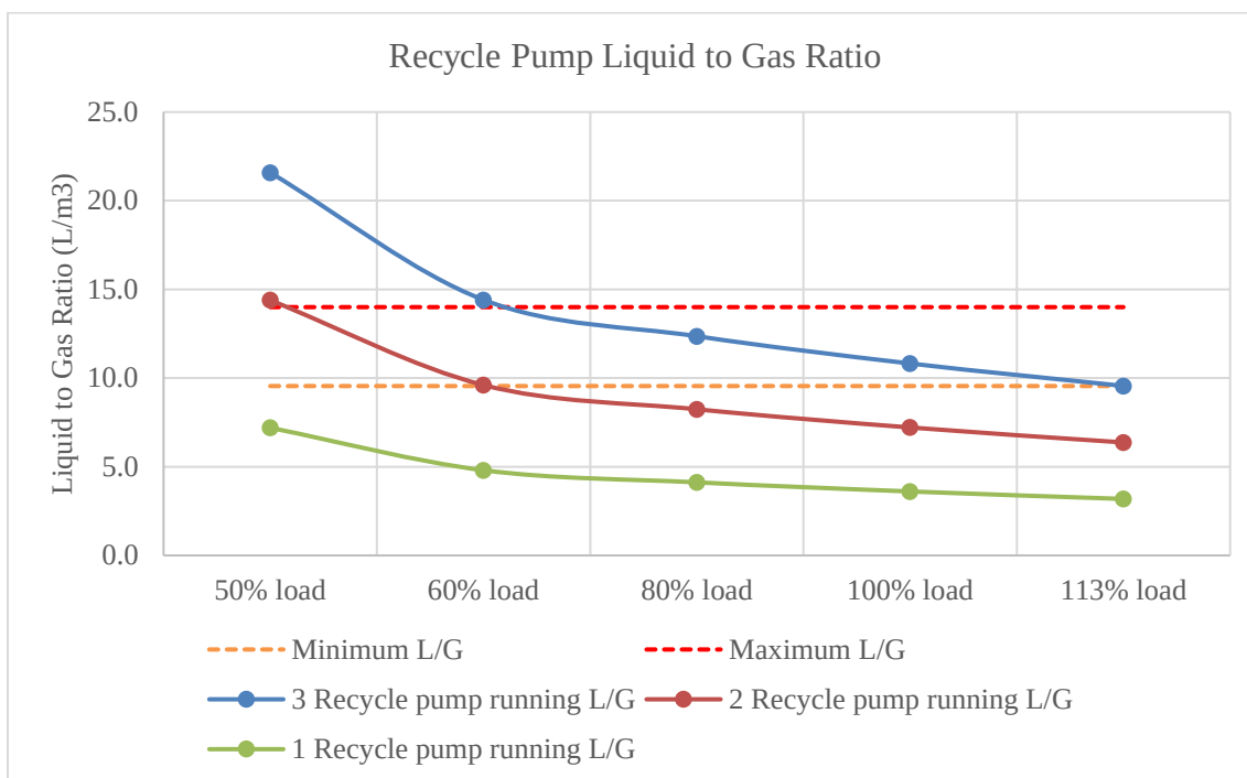
Figure 5.2-1: L/G ratio against Boiler load
