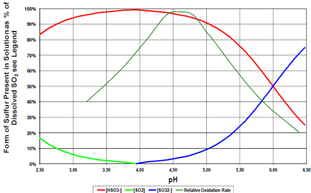
Figure 3.4.4-1: Form of \text{SO}_2 present in reaction tank solution (Steinmuller Engineering, 2013)
