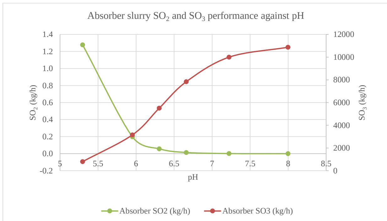
Figure 5.1-4: Absorber SO 2 and SO 3 performance against pH
