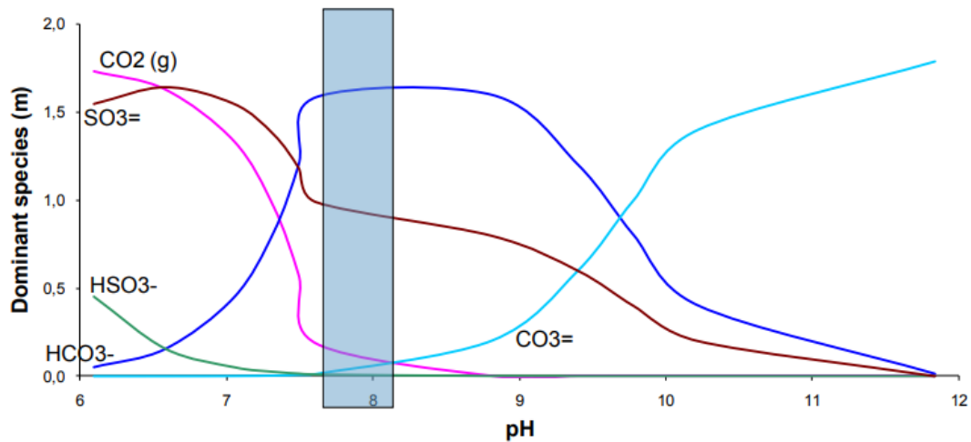
Figure 5.1-3: Sulphite-carbonate equilibrium (TNO,EnBW, CSIRO, 2011)
