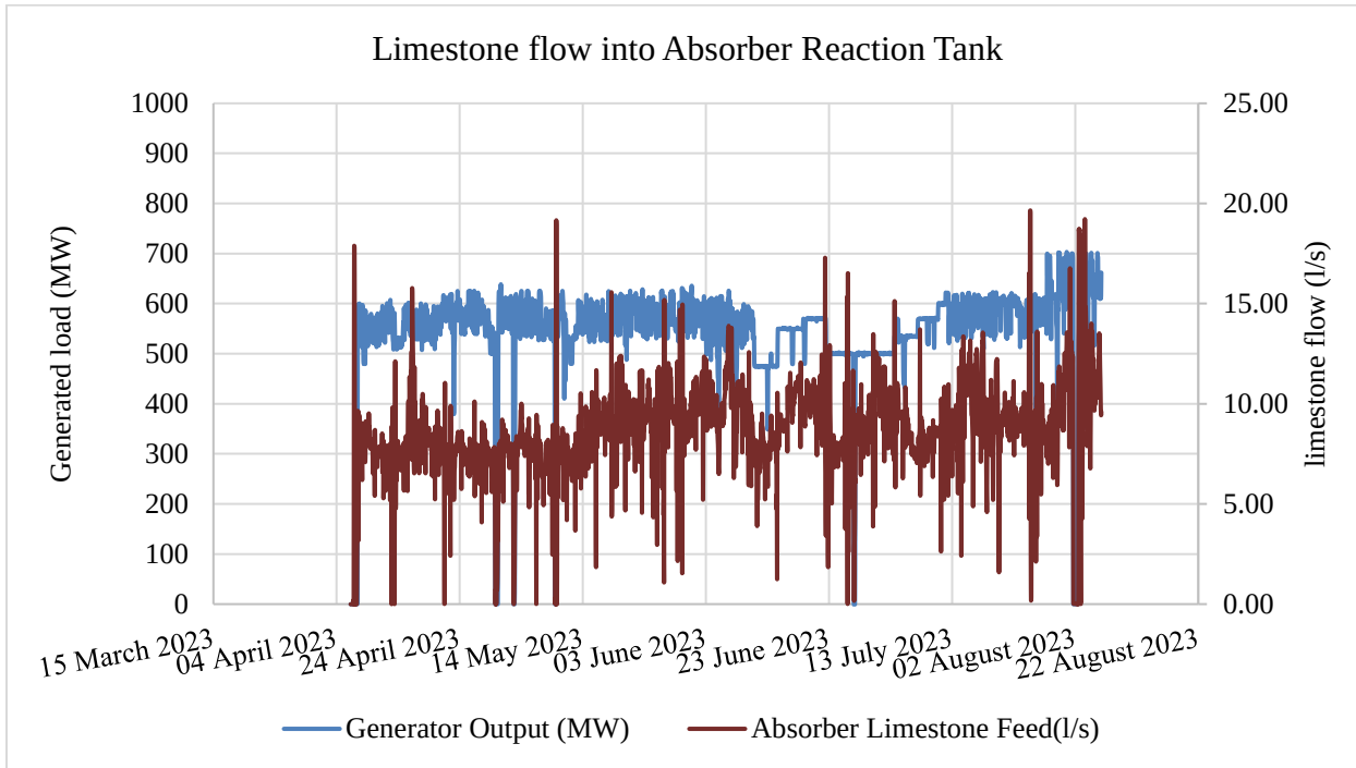
Figure 4.2.1.5-1: Actual Limestone feed to absorber
