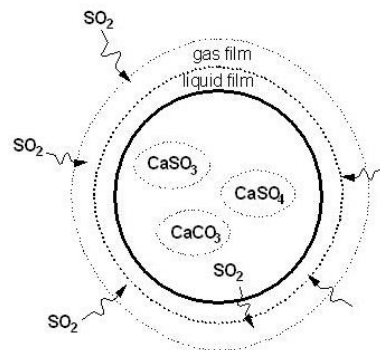
Figure 3.5.1-1 Mass transfer across phase boundary (Alstom Thermal Systems, 2014)
