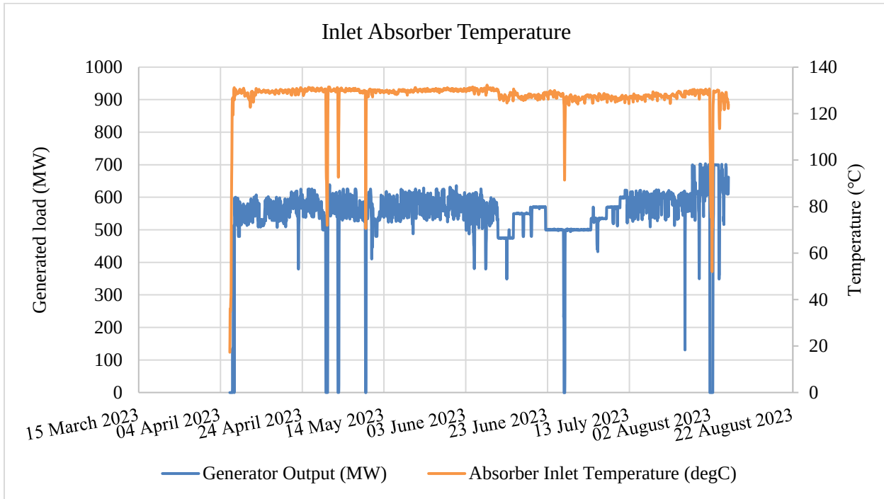
Figure 4.2.1.2-1: Actual Inlet absorber temperature
