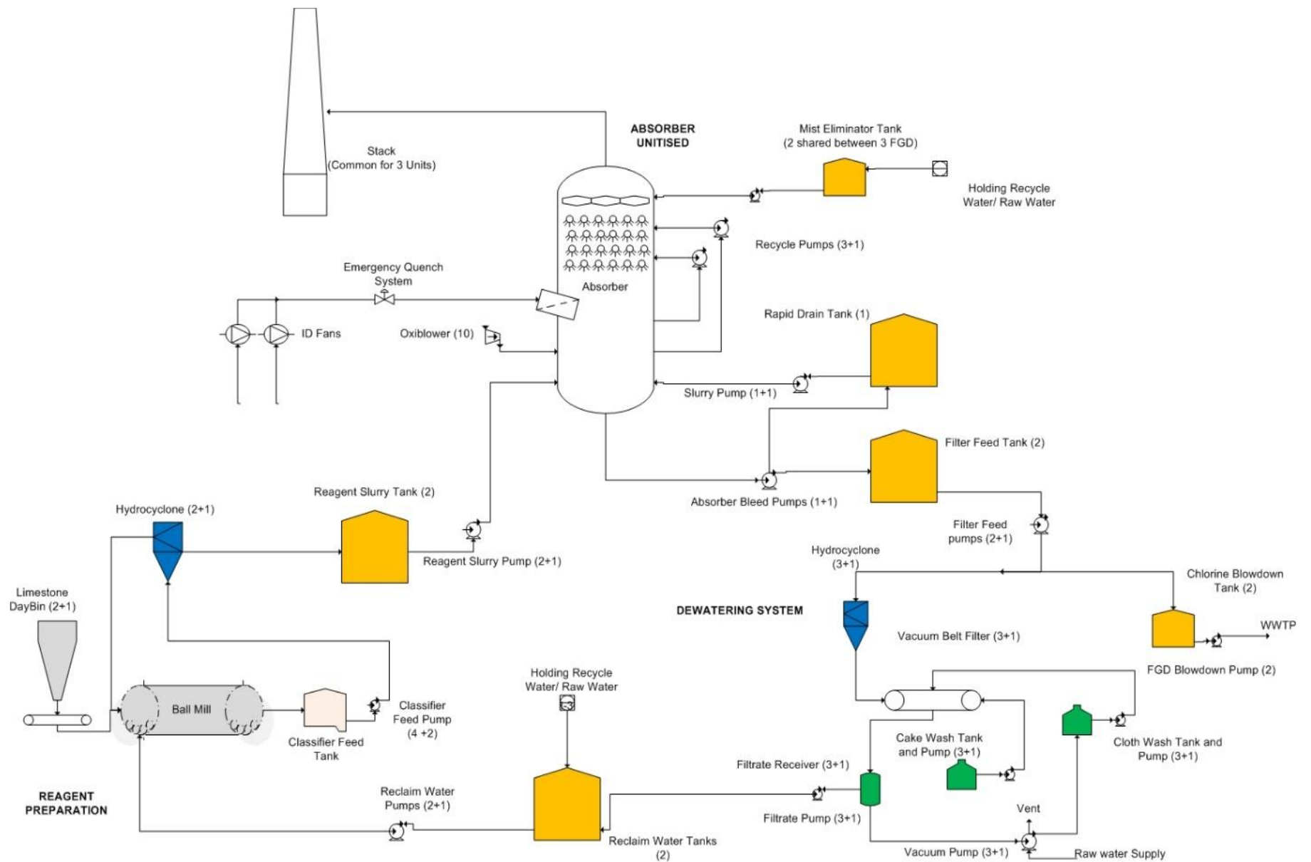
Figure 2.1-1: WFGD Plant Process Flow
