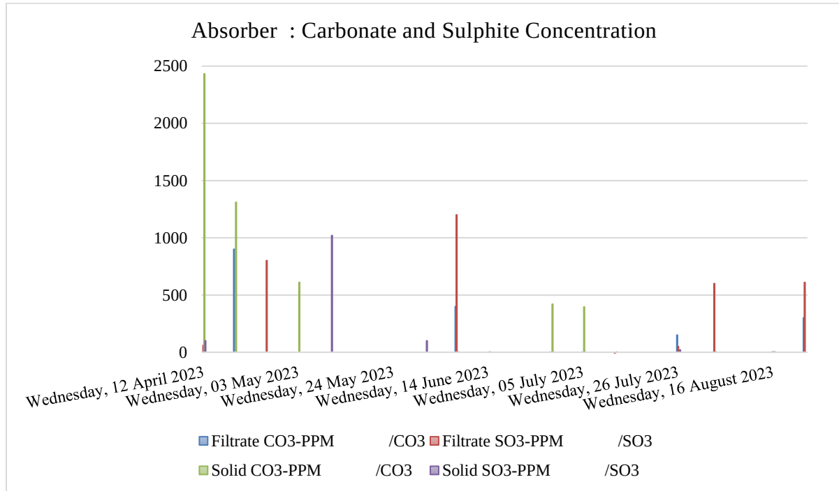
Figure 4.2.1.7-1: Actual absorber carbonate and sulphite concentrations in the reaction
