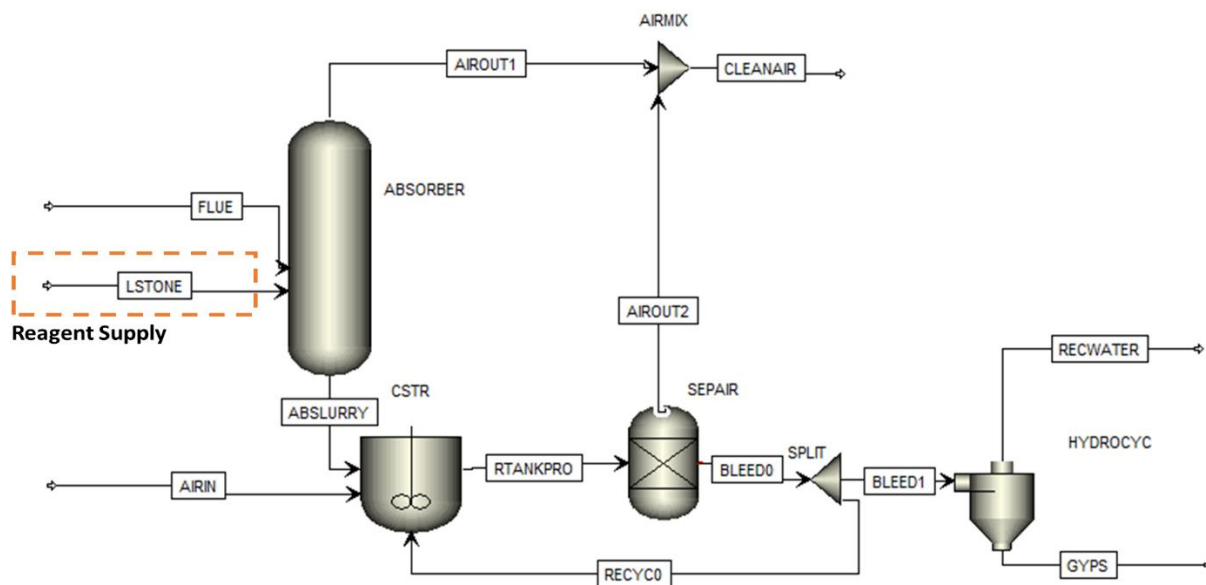
Figure 5.1-1: WFGD Absorber with variable slurry feed
