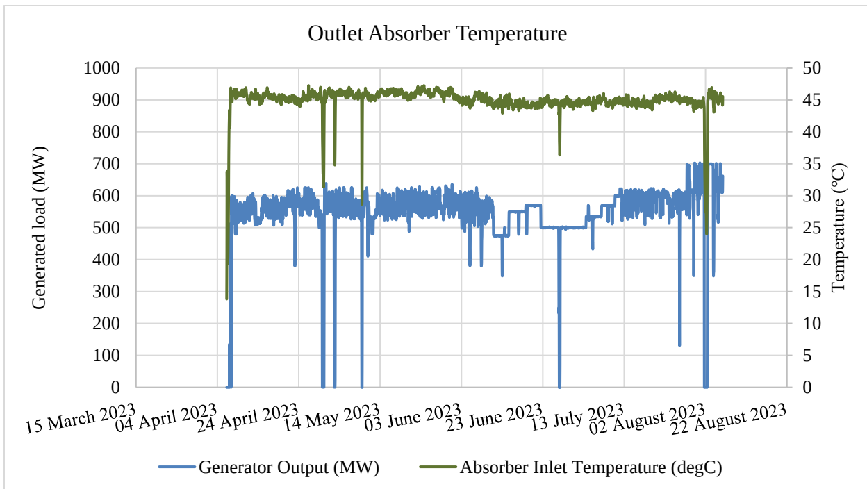
Figure 4.2.1.2-2: Actual Inlet and Outlet absorber temperature
