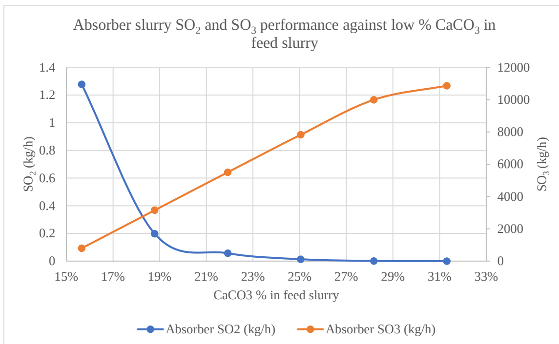
Figure 5.1-2: Absorber slurry SO 2 /SO 3 vs CaCO 3 feed
