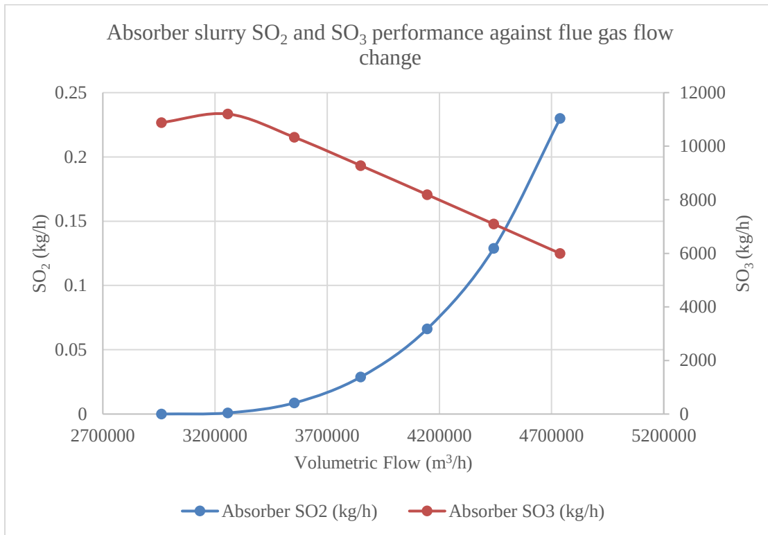
Figure 5.2-3: Absorber SO 2 /SO 3 vs flue gas volumetric flowrate
