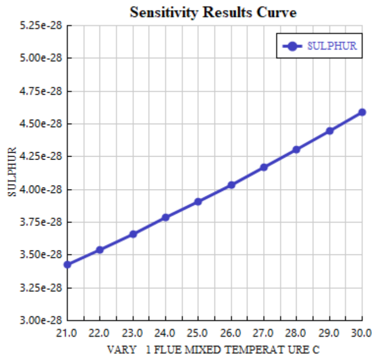
Figure 4.2.8.4-1 RADFRAC Outlet Sulphur vs Flue Gas inlet temperature
