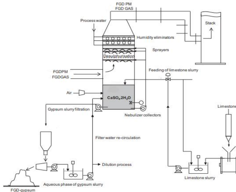
Figure 3.3-2 Typical FGD plant process flow diagram (Córdoba, 2015)
