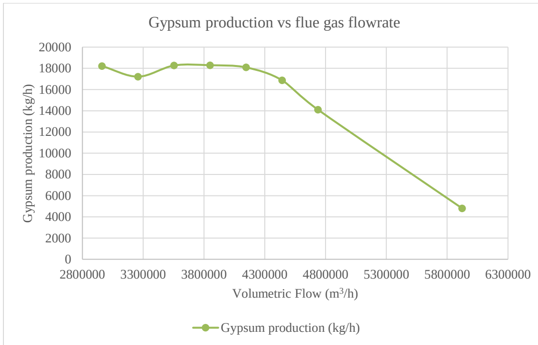
Figure 5.2-6: Gypsum production with increasing flue gas flow
