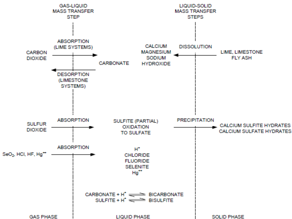
Figure 3.3.1-1: Mass transfer and Chemical reactions for WFGD system
