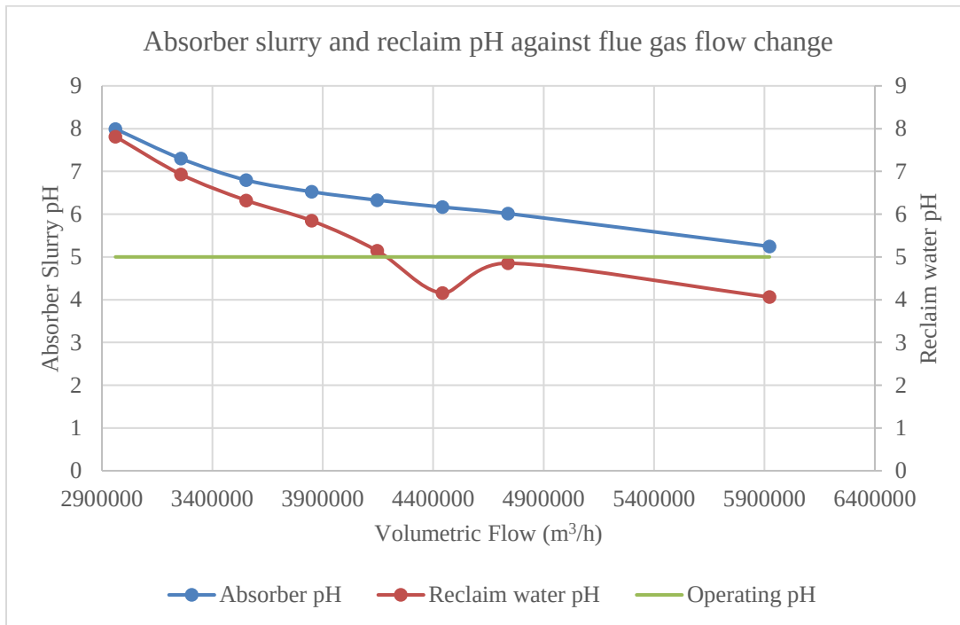
Figure 5.2-4: Absorber and reclaim water pH
