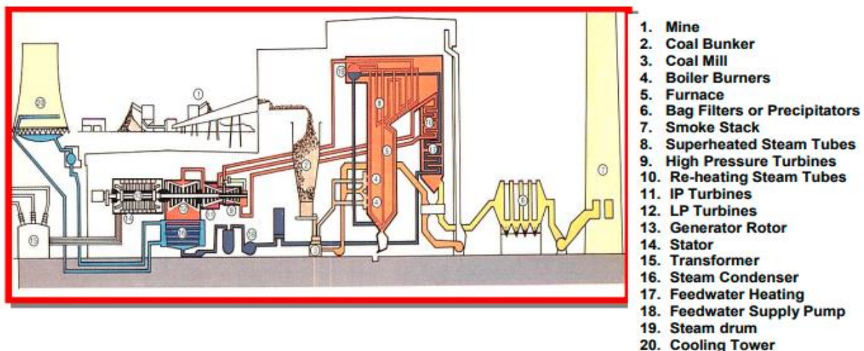
Figure 3.1-1: Typical coal-fired power station (Eskom Holdings SOC Ltd, 2021)
