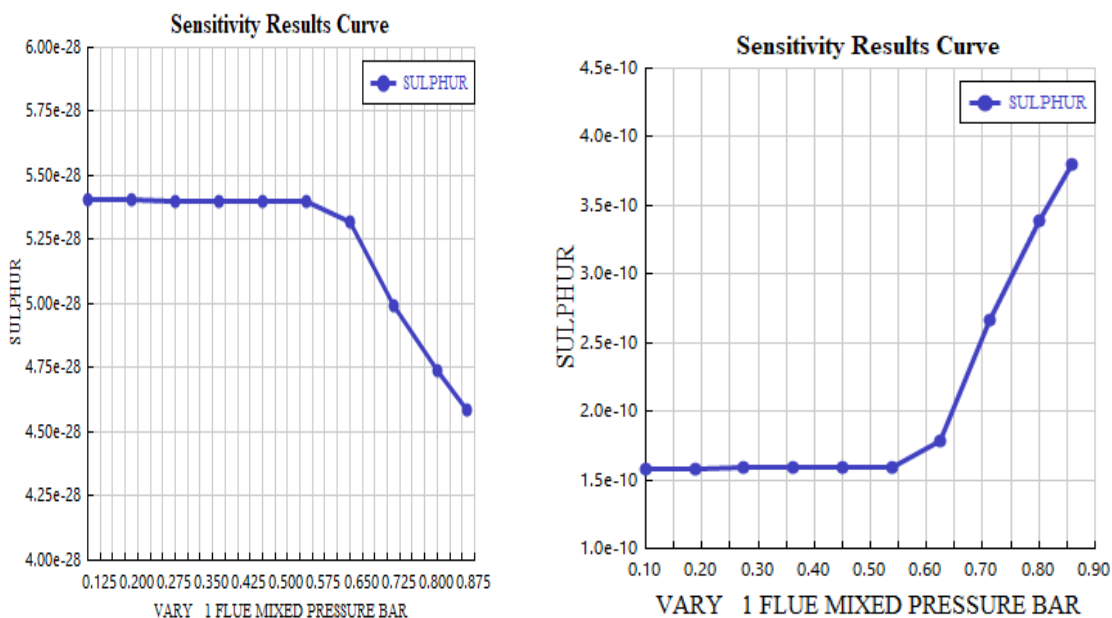
Figure 4.2.8.4-2 RADFRAC Absorber slurry SO 2 concentration (left) vs flue gas pressure & RADFRAC Outlet SO 2 (right) vs Flue Gas Pressure
