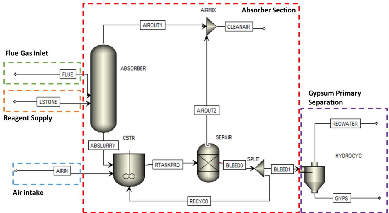
Figure 4.2.8.1-1: WFGD Absorber Base Model
