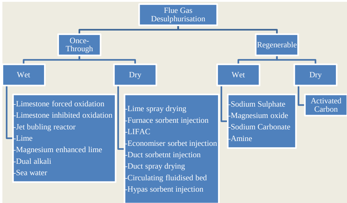
Figure 3.3-1 Classification of FGD technologies (Srivastava & Jozewicz, 2001)
