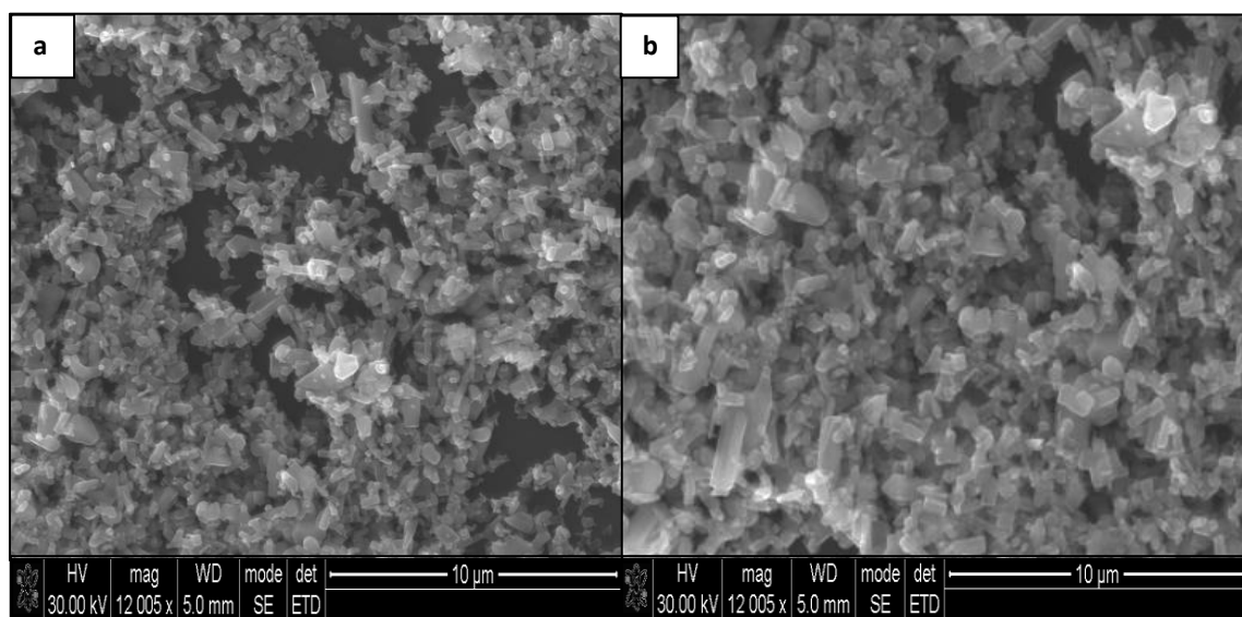
Figure 6.7: SEM images of the HDA capped \text{CuIn}_{0.25}\text{Ga}_{0.75}\text{Te}_2 synthesized using precursor 2 and EDT treated \text{CuIn}_{0.25}\text{Ga}_{0.75}\text{Te}_2 solar cells.
