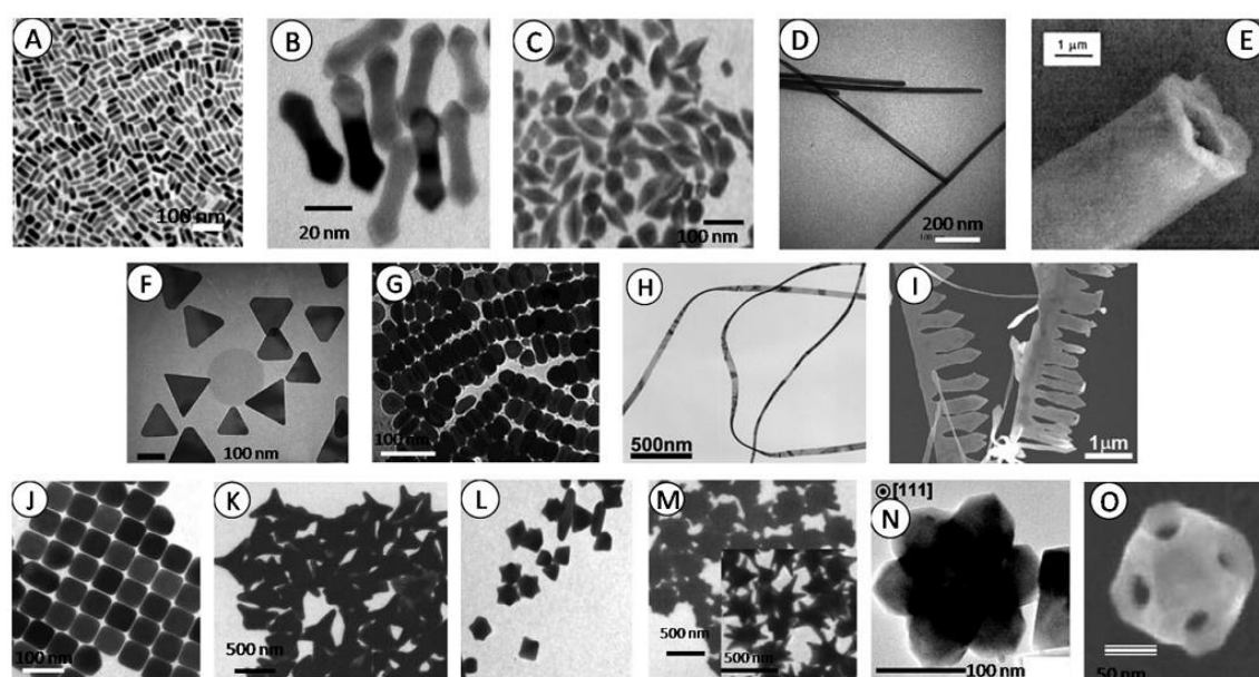
Figure 2.5: 1D: A) nanorods [39], B) nanoshuttles [40], and C) nanobipyramids [41] D) nanowires [42] E) nanotubule [43] 2D nanoparticles: F) triangular nanoplate [44], G) nanodisk [45], and H) ribbons [46]; I) belts [46]. 3D nanoparticles: J) nanocubes [47], K) tetrapods [47], L–M) star-shaped [47] N) nanoheptapods [48], and O) nanocage [49].
