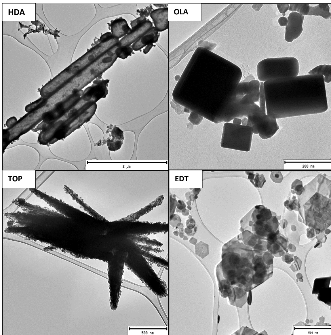
Figure 4.5: TEM micrographs of \text{CuInTe}_2 synthesized at 250 °C using various capping agents.
