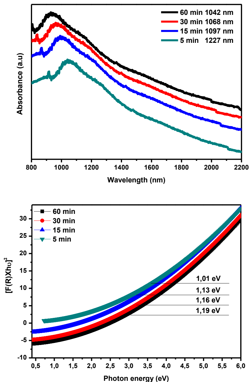
Figure 4.12: UV-Vis-NIR absorption spectra (top) and optical band gap (bottom) of CuInTe 2 crystallites synthesized at temperature 250 °C at various reaction times.
