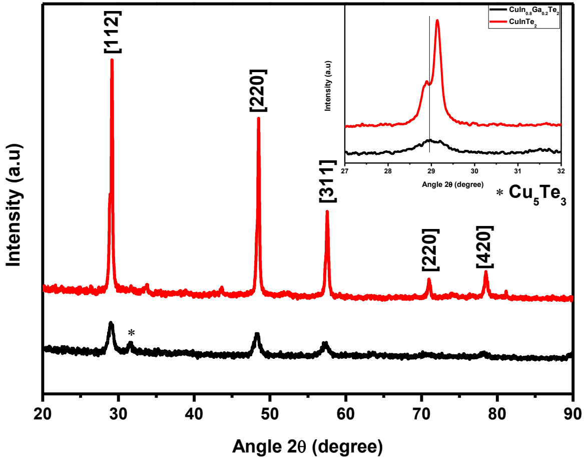
Figure 5.3: (a) XRD patterns of \text{CuInTe}_2 and \text{CuIn}_{1-x}\text{Ga}_x\text{Te}_2 at 250 °C with inset of an expanded view of (111) peak.
