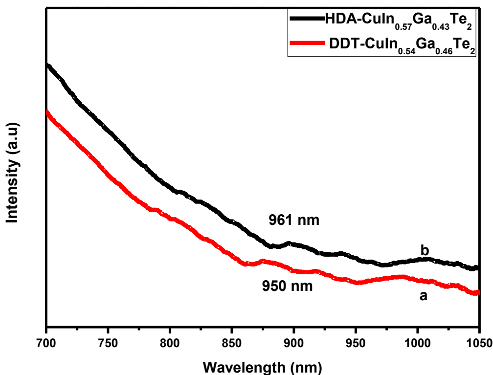
Figure 5.24: UV-Vis absorption spectra of \text{CuIn}_{1-x}\text{Ga}_x\text{Te}_2 with In:Ga actual ratios of (a) 0.57:0.43 in HDA and (b) 0.54:0.48 in DDT.
