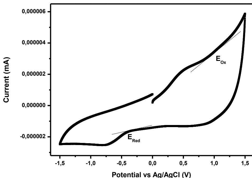
Figure 6.3: Cyclic voltammogram of HDA capped \text{CuIn}_{0.25}\text{Ga}_{0.75}\text{Te}_2 synthesized using precursor 2.
