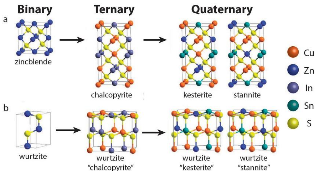
Figure 2.1: Crystal structures of ternary and quaternary Cu chalcogenide NCs. a) If the binary NCs have a zinc-blende-like crystal structure, the resulting ternary NCs have the chalcopyrite crystal structure, whereas the quaternary NCs will have either stannite or kesterite structures. b) If cation-exchange reactions are deployed on wurtzite-like Cu chalcogenides, the resulting ternary and quaternary NCs also have a wurtzite structure [11].
