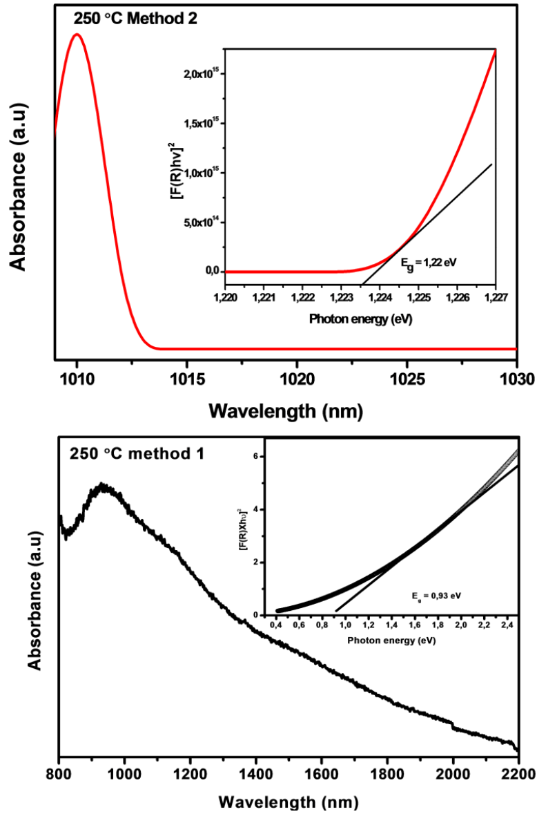
Figure 3.6: UV–Vis–NIR absorbance spectra and optical bands (insets) gaps of \text{CuInTe}_2 crystallites synthesized at 250 °C using method 1 and 2.
