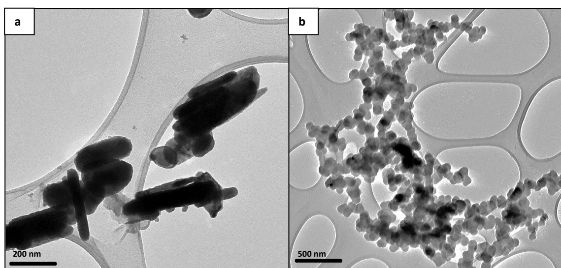
Figure 5.10: TEM micrographs of (a) \text{CuIn}_{0.84}\text{Ga}_{0.16}\text{Te}_2 and (b) \text{CuIn}_{0.25}\text{Ga}_{0.75}\text{Te}_2 synthesized with Precursor 1 and with Precursor 2 respectively.
