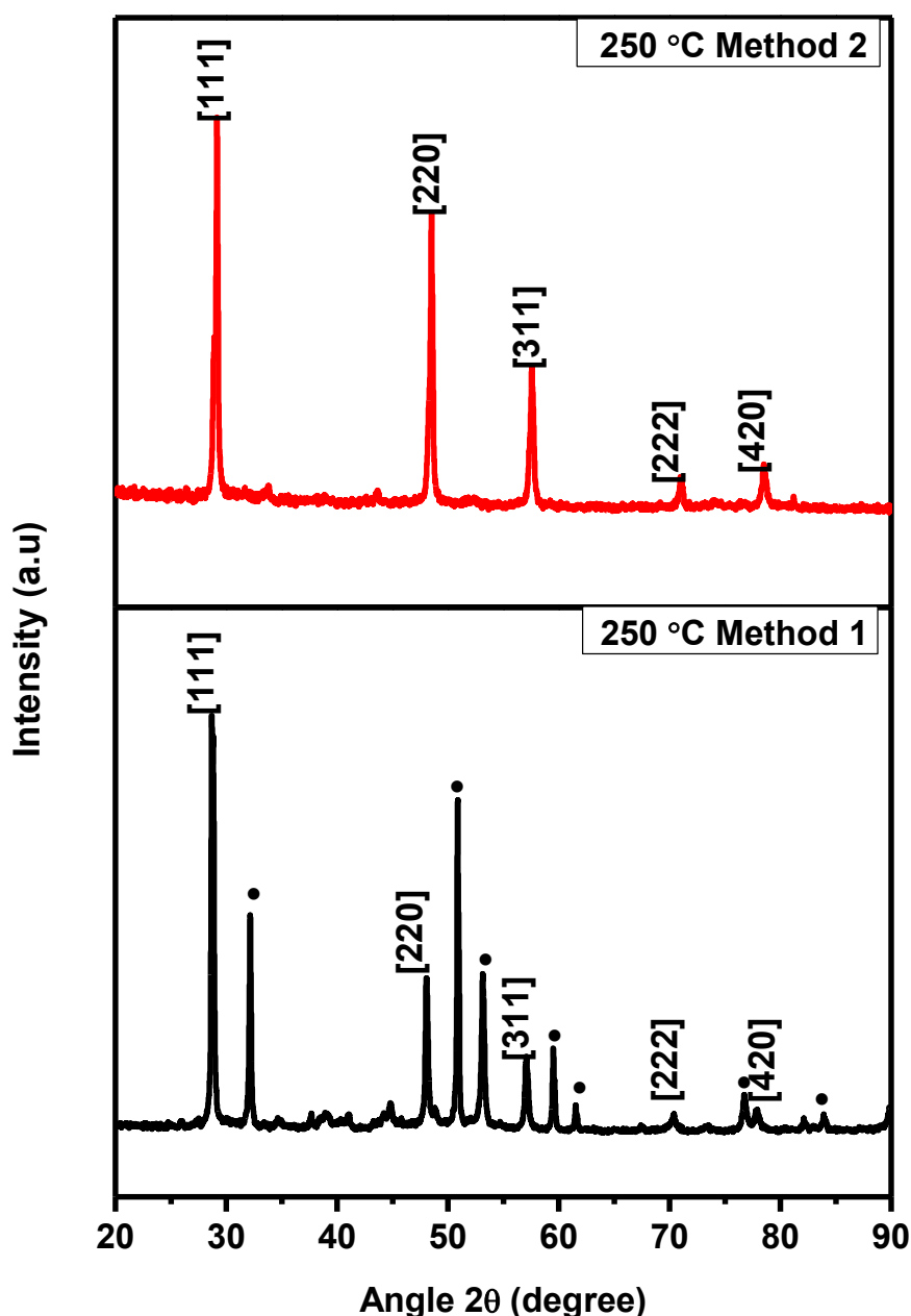
Figure 3.4: XRD patterns of \text{CuInTe}_2 crystallites synthesized at 250 °C using method 1 and 2, where • = \text{Cu}_5\text{Te}_3 .
