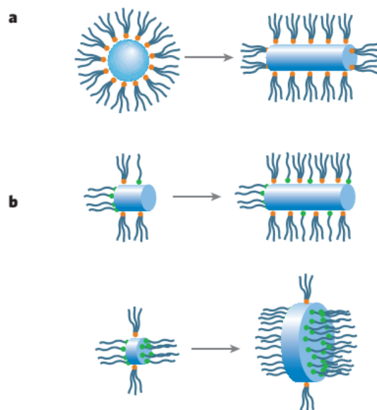
Figure 4.3: shape control of colloidal nanocrystals a) Kinetic shape control at high growth rate. The high-energy facets grow more quickly than low energy facets in a kinetic regime. b) Kinetic shape control through selective adhesion [1].
