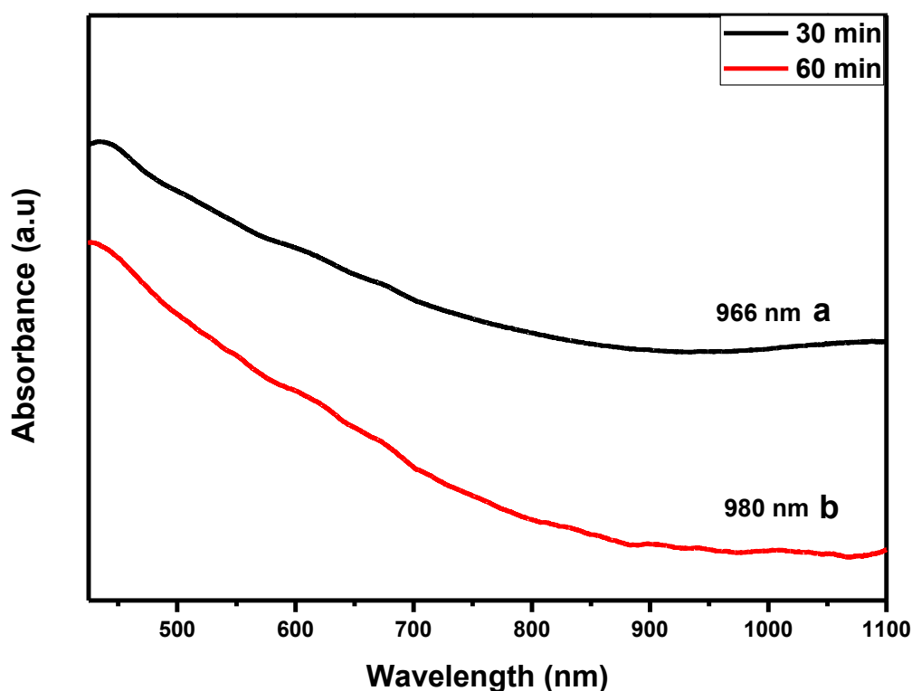
Figure 5.12: UV-Vis absorption spectra of CuIn 1-x Ga x Te 2 synthesized at reaction time (a) 30 min and (b) 60 min.
