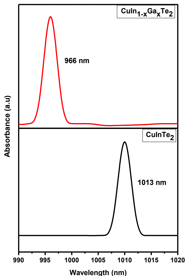
Figure 5.6: Absorbance spectra of \text{CuInTe}_2 and \text{CuIn}_{0.8}\text{Ga}_{0.2}\text{Te}_2 materials synthesized at 250 °C.
