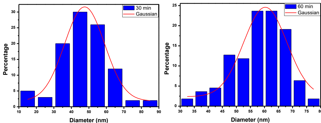
Figure 5.15: Particle size distribution measured from TEM of \text{CuIn}_{1-x}\text{Ga}_x\text{Te}_2 synthesized at reaction time 30 min and 60 min.
