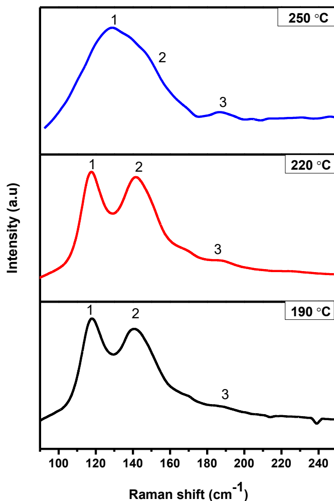
Figure 3.2: Raman spectra of crystallites synthesized using method 1 at various temperatures.
