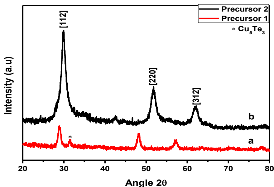
Figure 5.7: XRD patterns of \text{CuIn}_{1-x}\text{Ga}_x\text{Te}_2 synthesized with (a) Precursor 1 and (b) Precursor 2.
