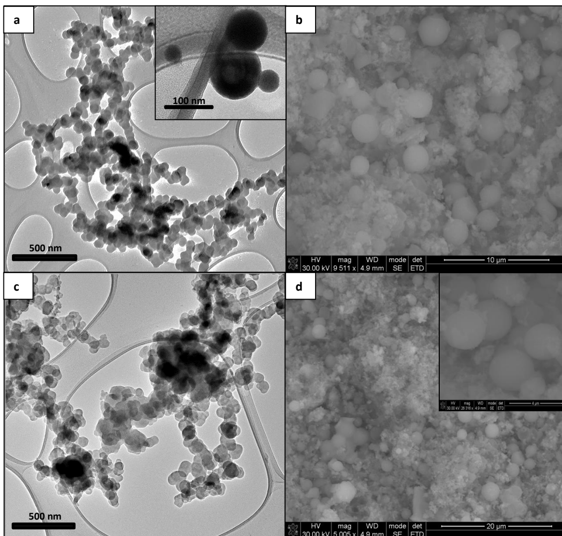
Figure 5.14: TEM and SEM micrographs of \text{CuIn}_{1-x}\text{Ga}_x\text{Te}_2 synthesized at reaction time 30 min (a-b) and 60 min (c-d).
