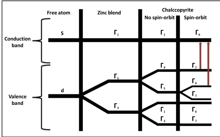
Figure 4.7: Schematic diagram of the band structure of chalcopyrite with modified d-levels to fit the ordering levels in \text{CuInTe}_2 [29].
