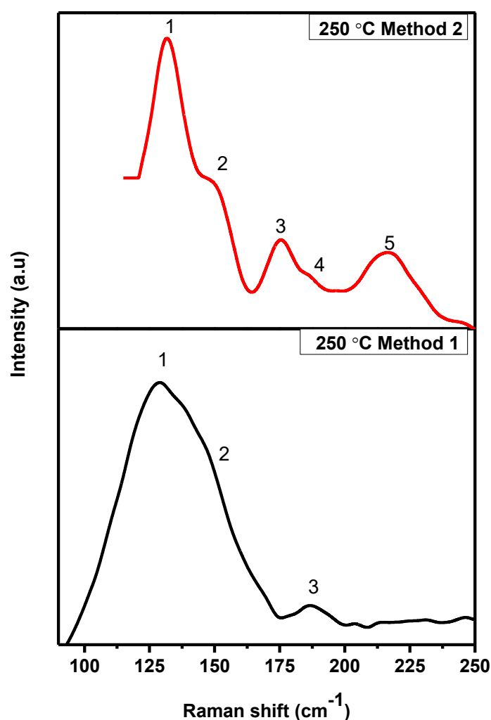
Figure 3.5: Raman spectra of \text{CuInTe}_2 crystallites synthesized at 250 °C using method 1 and 2.
