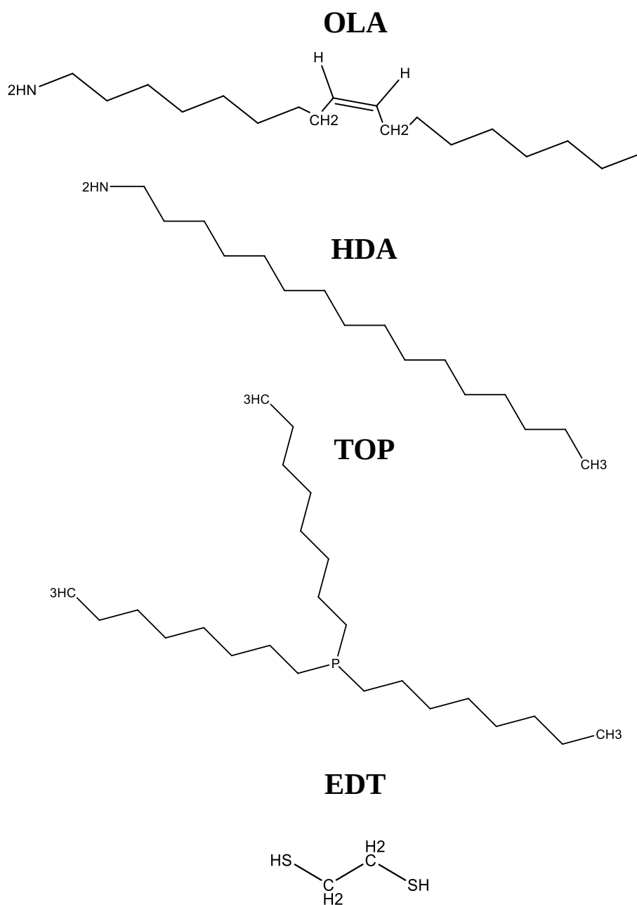
Figure 4.4 Scheme of the different capping agent molecules and their functionalities.
