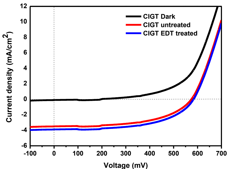
Figure 6.8: I-V curves of HDA capped \text{CuIn}_{0.25}\text{Ga}_{0.75}\text{Te}_2 synthesized using precursor 2 and EDT treated \text{CuIn}_{0.25}\text{Ga}_{0.75}\text{Te}_2 solar cells.
