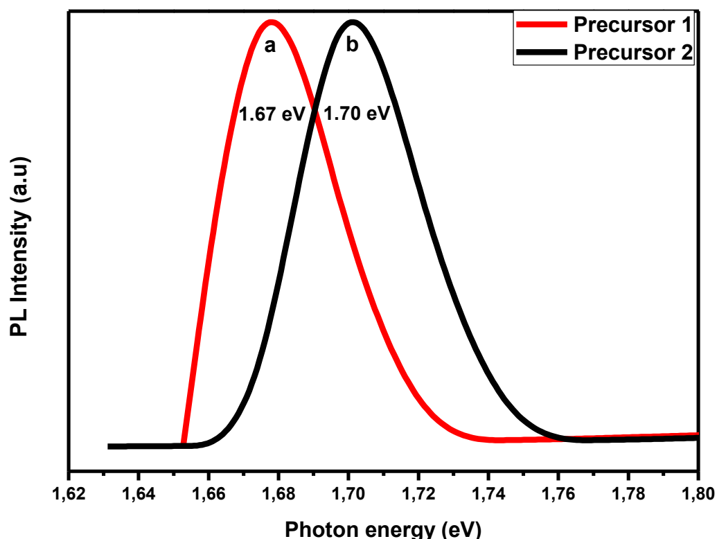
Figure 5.9: PL emission spectra of (a) \text{CuIn}_{0.84}\text{Ga}_{0.16}\text{Te}_2 synthesized with Precursor 1 and (b) \text{CuIn}_{0.25}\text{Ga}_{0.75}\text{Te}_2 with Precursor 2.
