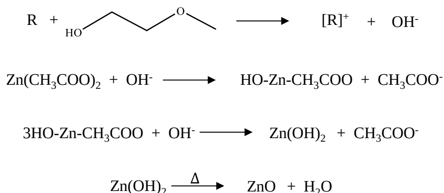
Figure 6.1: Scheme of Synthesis of ZnO via the sol-gel method.
