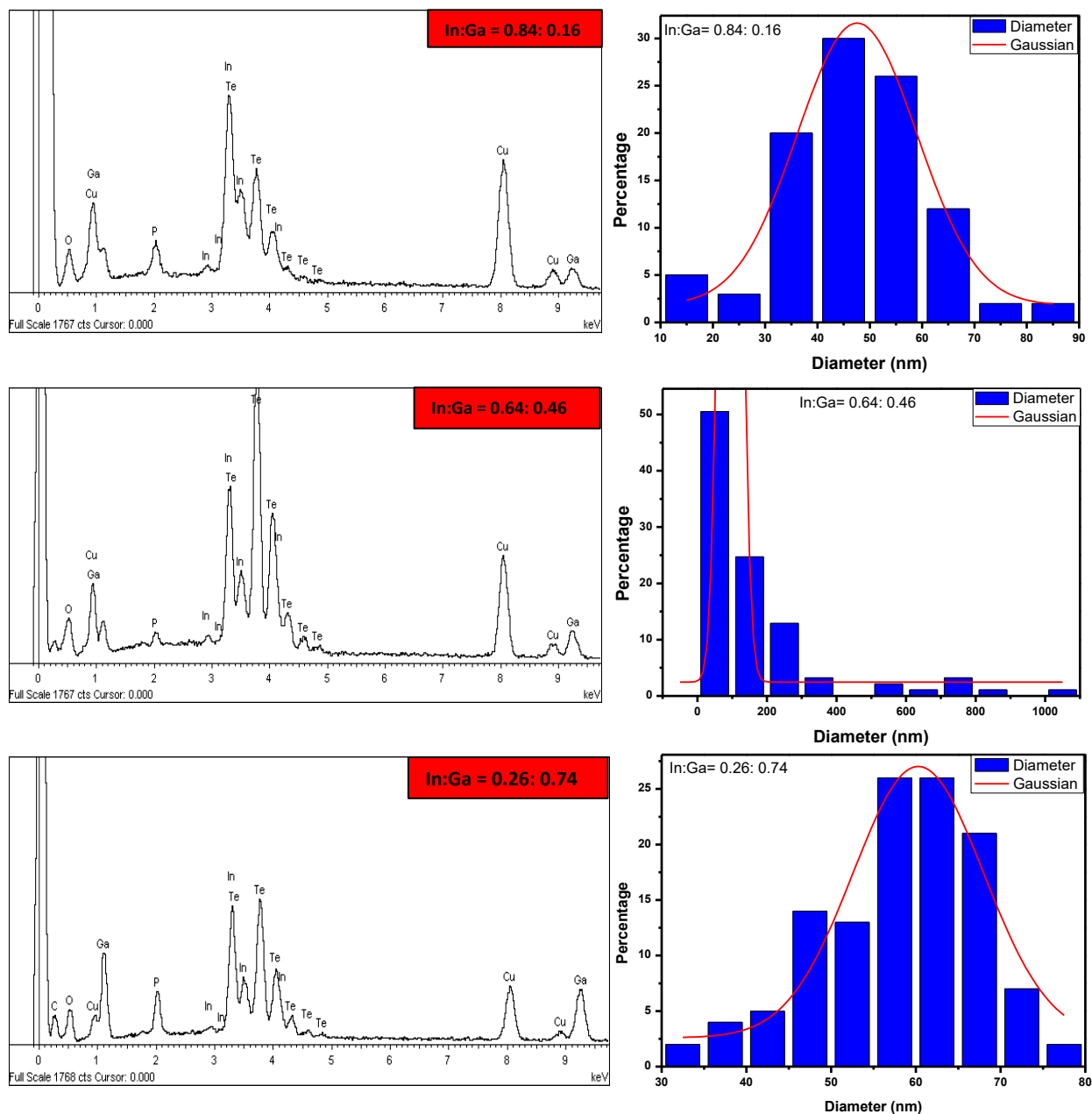
Figure 5.22: EDS spectra of TEM and particle size distribution of \text{CuIn}_{1-x}\text{Ga}_x\text{Te}_2 with various concentrations of In: Ga ratios.
