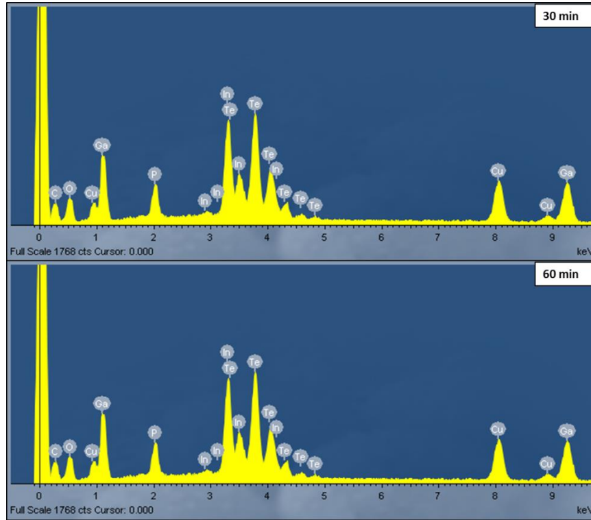
Figure 5.16: EDS spectra of TEM and SEM micrographs of \text{CuIn}_{1-x}\text{Ga}_x\text{Te}_2 synthesized at reaction time 30 min and 60 min.
