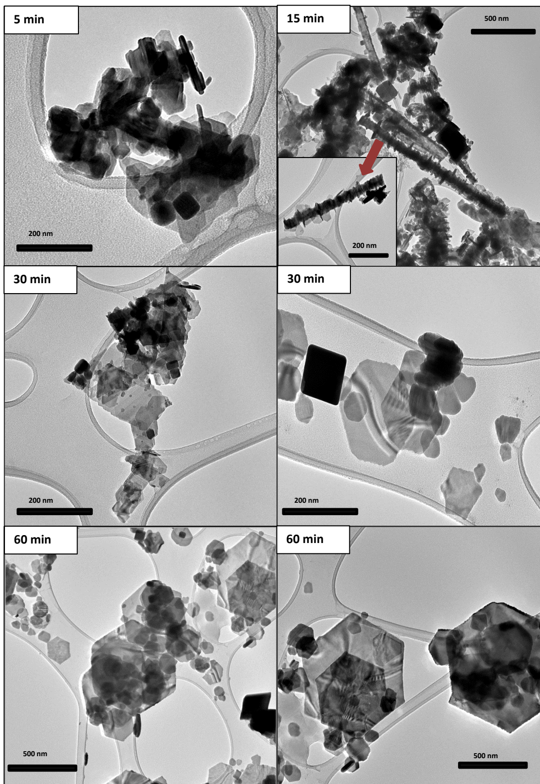
Figure 4.9: Morphology transition from 1D to 2D Shape of \text{CuInTe}_2 with increasing reaction time.
