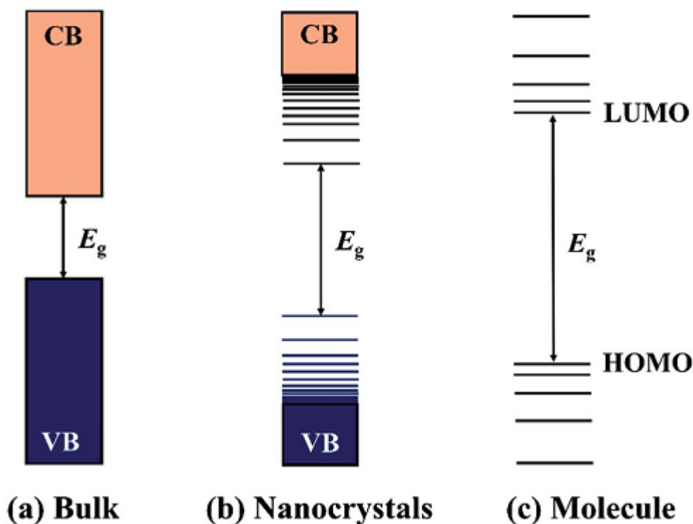
Figure 2.6: A comparison of the electronic energy states of different types of semiconductor materials: (a) bulk semiconductors, (b) semiconductor nanocrystals, and (c) molecular semiconductors [17].
