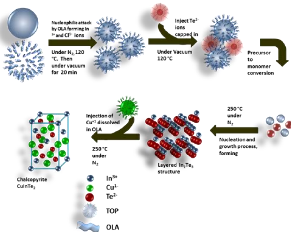
Figure 3.10: Proposed reaction path for the formation of phase pure \text{CuInTe}_2 .
