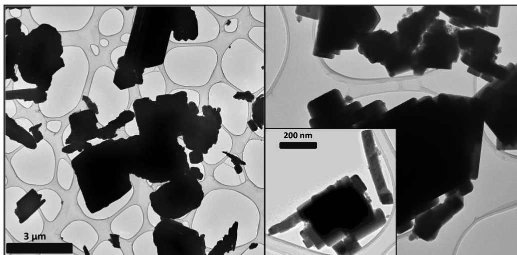
Figure 3.3: TEM micrographs of crystallites synthesized using method 1 at 250 °C.
