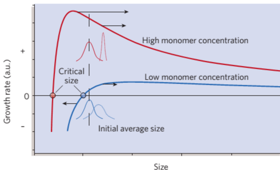
Figure 2.3: Growth rate dependency on the nanoparticle size for low and high monomer concentration [27].
