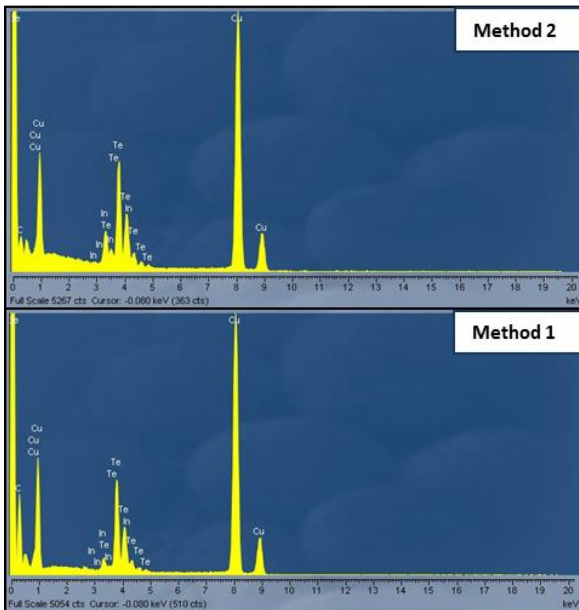
Figure 3.9: EDS spectra of TEM and HRTEM micrographs of \text{CuInTe}_2 crystallites synthesized at 250 °C using method 2 and method 1.
