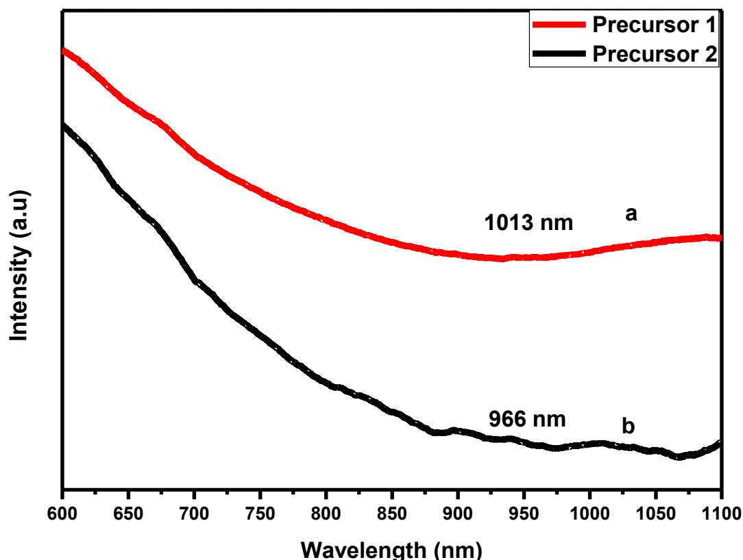
Figure 5.8: UV-Vis absorption spectra of (a) \text{CuIn}_{0.84}\text{Ga}_{0.16}\text{Te}_2 synthesized with Precursor 1 and (b) \text{CuIn}_{0.25}\text{Ga}_{0.75}\text{Te}_2 with Precursor 2.
