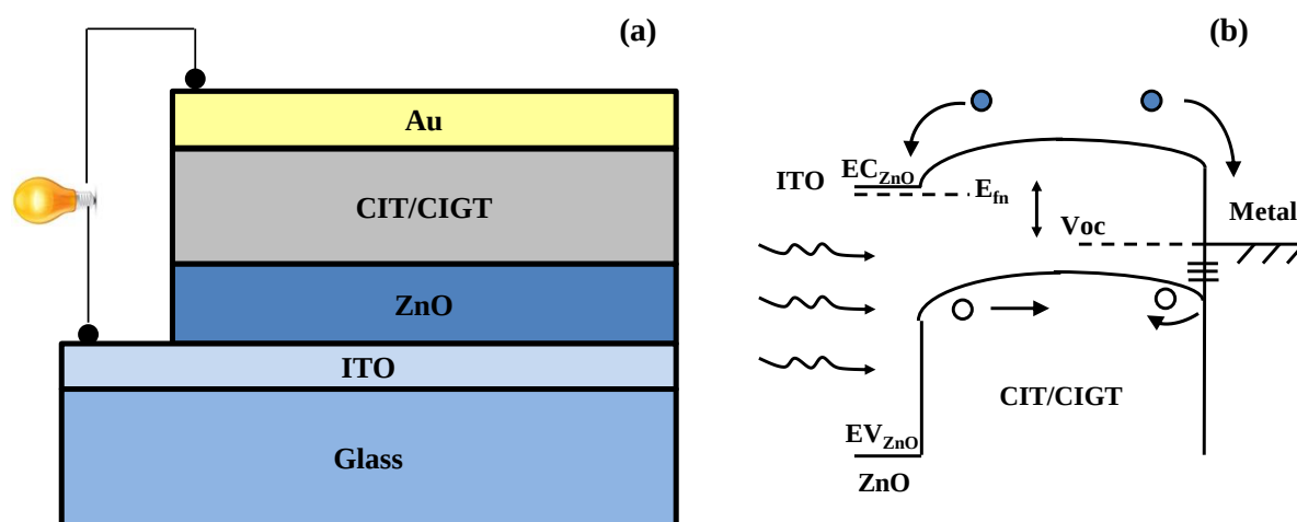
Figure 6.5: (a) Schematic of the solar cell structure ITO/ZnO/CIT or CIGT/Au and (b) device band structure under illumination. Holes meet the barrier height at the Au electrode, and electrons can flow in either of two opposite directions to electrodes.
