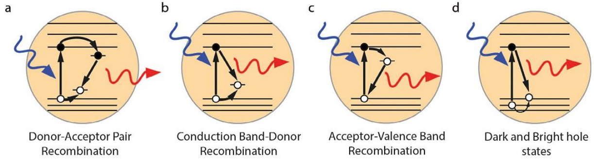
Figure 2.7: Possible recombination pathways in \text{CuInS}_2 nanocrystals. The origins of the intriguing optical properties of \text{CuInS}_2 NCs are not yet understood and are still under debate. a) PL of CIS NCs is due to a donor–acceptor pair recombination due to point defects such as \text{Cu}_{\text{In}} , \text{V}_{\text{In}} , or \text{V}_{\text{Cu}} . b) PL due to recombination of quantized CB electron states with localized holes. c) PL of CIS NCs is due to radiative recombination of quantized VB hole states with electrons localized at native point defects. d) PL of CIS NCs is intrinsic and originates from the 1\text{S}(\text{e}) - 1\text{S}(\text{h}) exciton transition [8a] .
