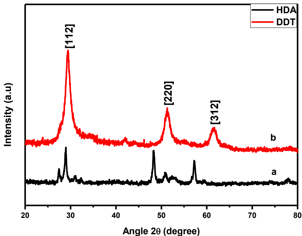
Figure 5.23: (a) XRD patterns of \text{CuIn}_{1-x}\text{Ga}_x\text{Te}_2 synthesized from In: Ga ratios of 1:1 in (a) HDA and (b) DDT.
