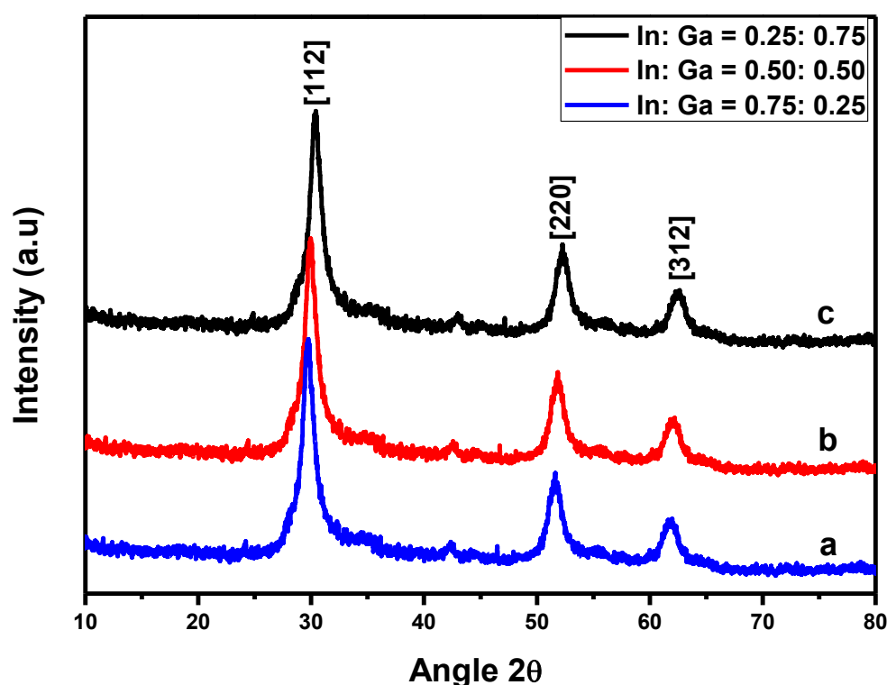
Figure 5.17: XRD patterns of \text{CuIn}_{1-x}\text{Ga}_x\text{Te}_2 synthesized from precursor concentrations of In: Ga ratios of (a) 0.75:0.25, (b) 0.50:0.50 and (c) 0.25: 0.75.
