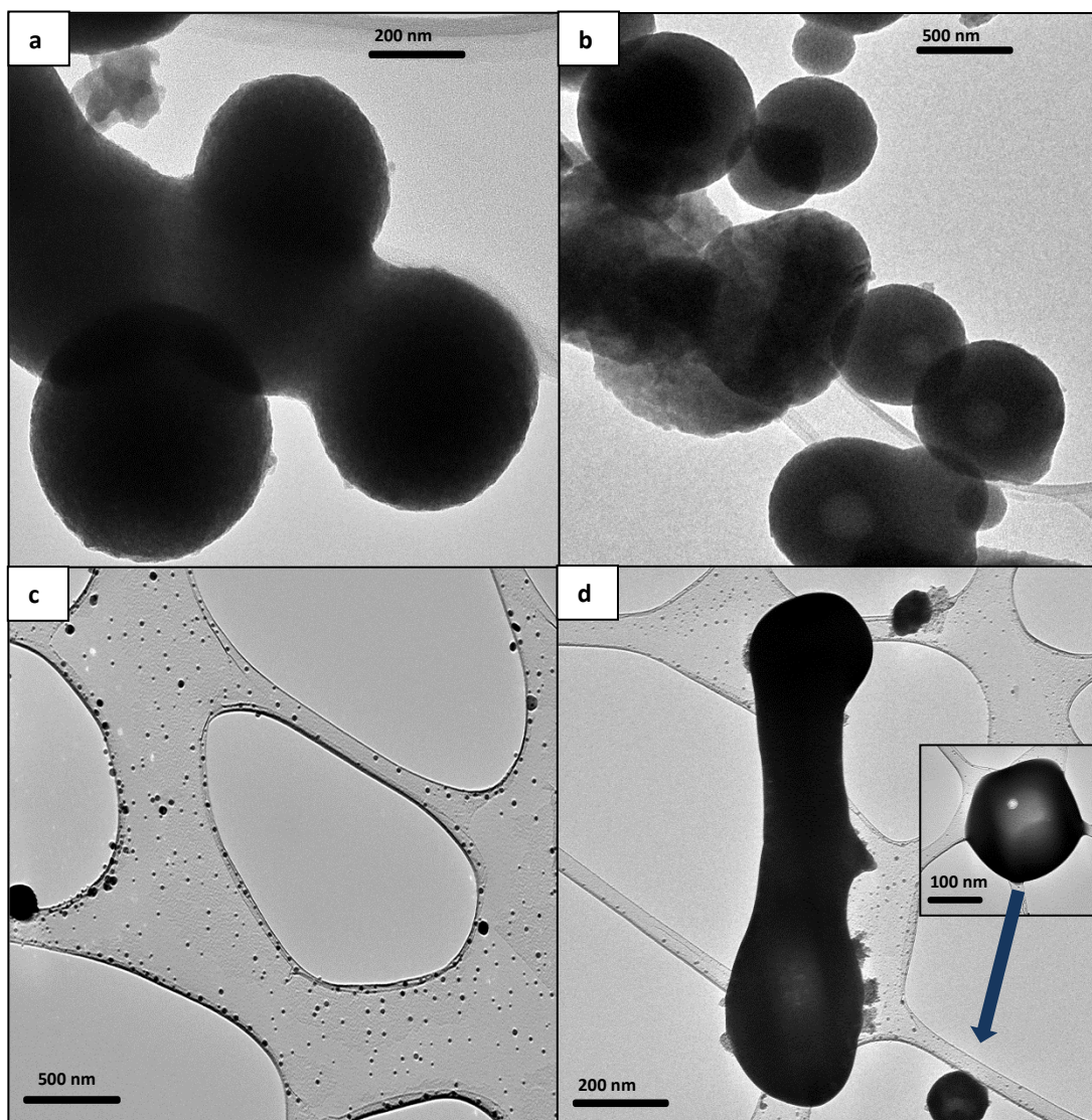
Figure 5.26: TEM micrographs of \text{CuIn}_{1-x}\text{Ga}_x\text{Te}_2 with In:Ga actual ratios of (a-b) 0.57:0.43 in HDA and (c-d) 0.54:0.48 in DDT.
