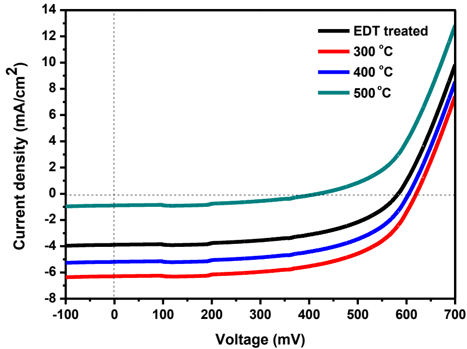
Figure 6.10: I-V curves of EDT treated \text{CuIn}_{0.25}\text{Ga}_{0.75}\text{Te}_2 and annealed films at 300, 400 and 500 °C.
