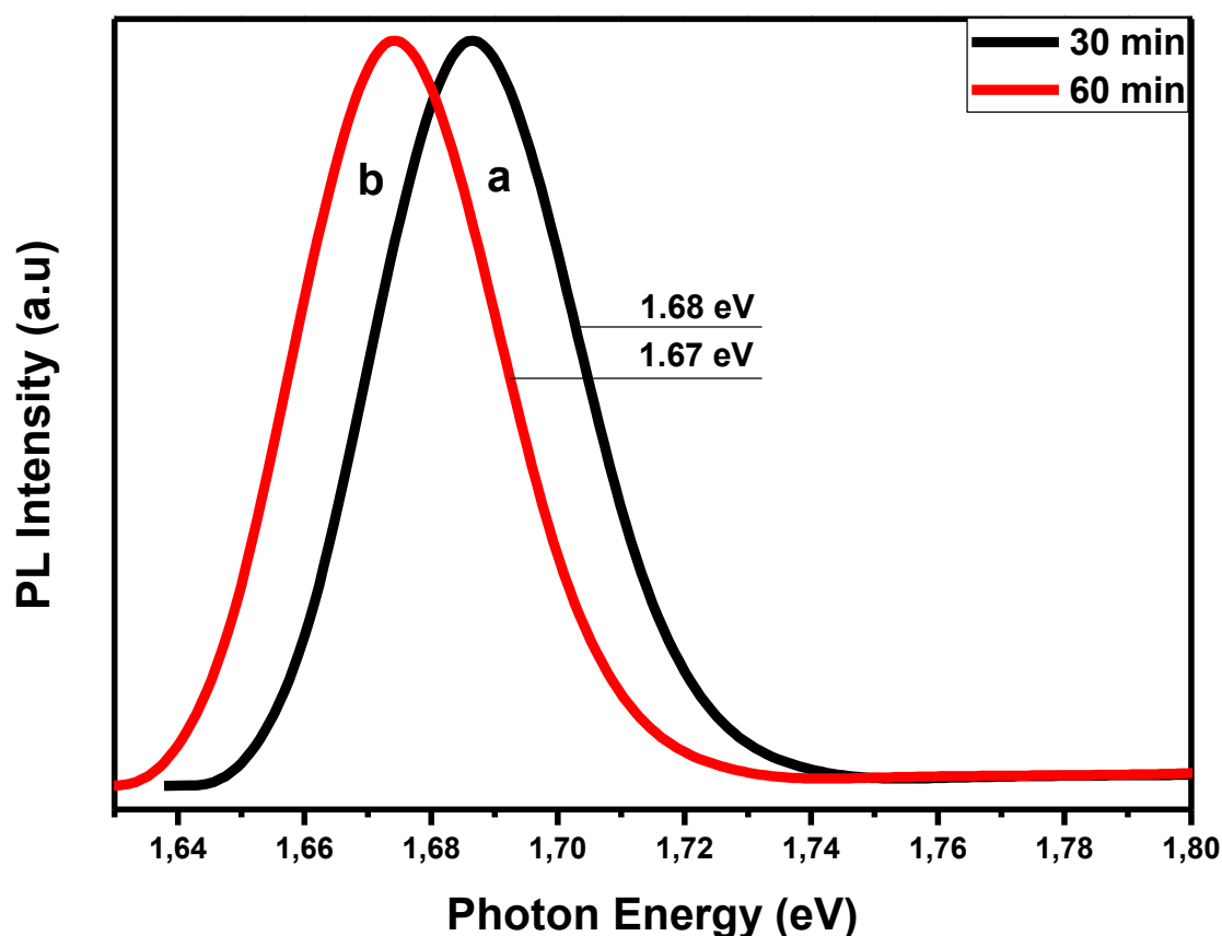
Figure 5.13: PL emission spectra of \text{CuIn}_{1-x}\text{Ga}_x\text{Te}_2 synthesized at reaction time (a) 30 min and (b) 60 min.
