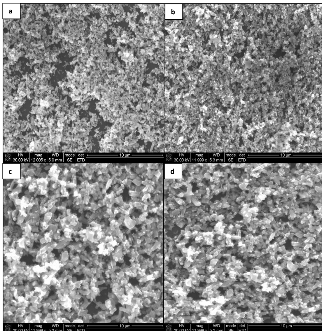
Figure 6.9: SEM micrographs of (a) EDT treated \text{CuIn}_{0.25}\text{Ga}_{0.75}\text{Te}_2 and annealed films at (b) 300, (c) 400 and (d) 500 °C.
