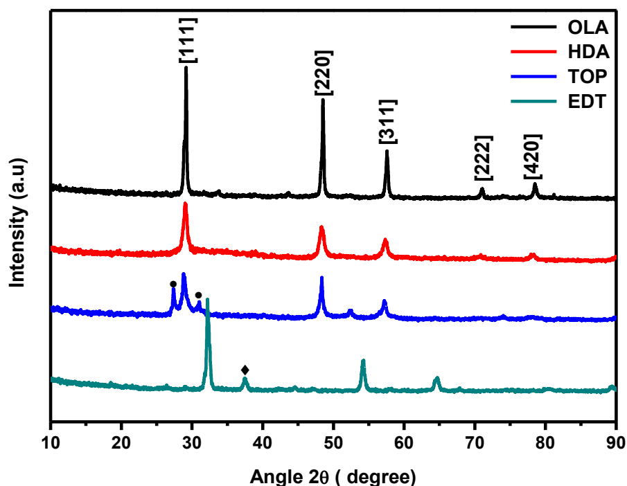
Figure 4.6: XRD patterns of \text{CuInTe}_2 synthesized at 250 °C using various capping agents ♦ = Te phase and • = \text{Cu}_5\text{Te}_3 .
