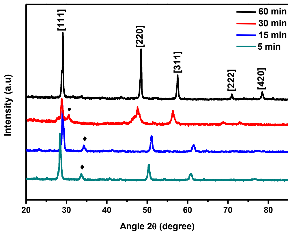
Figure 4.11: XRD patterns of CuInTe 2 synthesized at temperature 250 °C and various reaction time where ♦ = Te phase and • = Cu 5 Te 3 .
