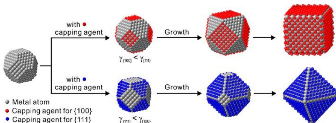
Figure 2.4: Schematic illustrations showing the role of capping agents in directing the growth of a single-crystal seed made of an fcc metal. Introduction of a capping agent (represented by red or blue dots) that can selectively bind to a specific type of facet, altering the order of surface free energies and eventually leading to the formation of a nanocube enclosed by \{100\} facets and an octahedron enclosed by \{111\} facets, respectively [35].
