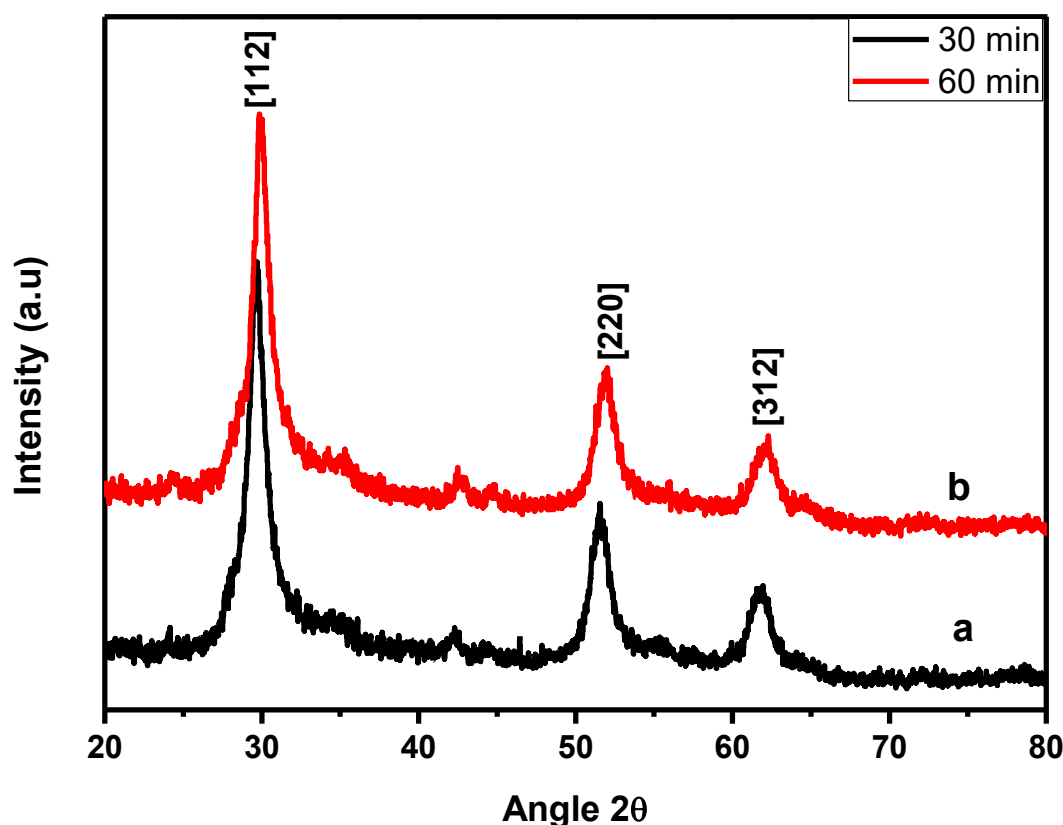
Figure 5.11: XRD patterns of \text{CuIn}_{1-x}\text{Ga}_x\text{Te}_2 synthesized at reaction time (a) 30 min and (b) 60 min.
