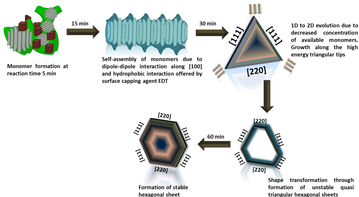
Figure 4.13: The proposed self-ripening mechanism of 1D to 2D morphology transformation.
