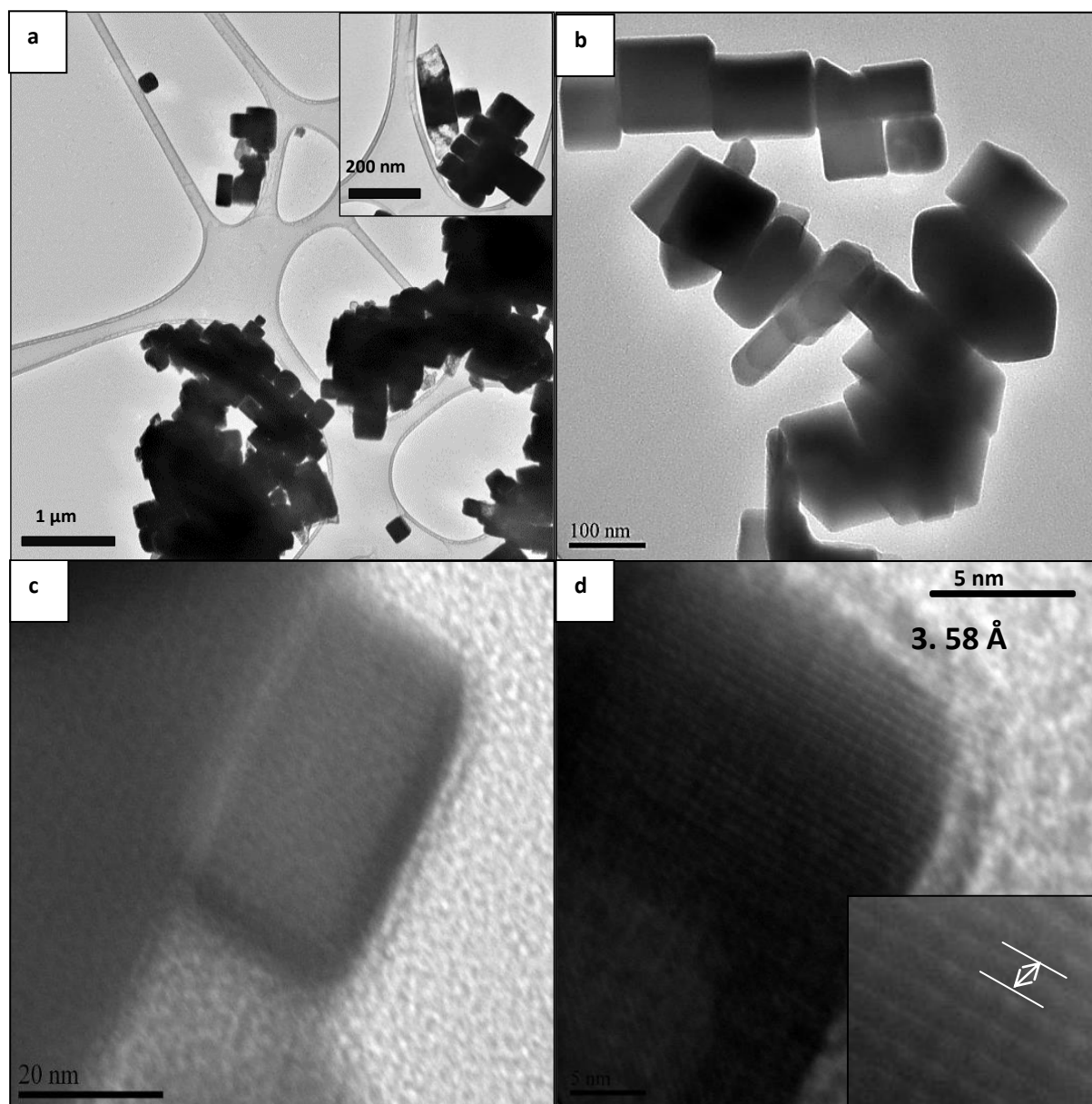
Figure 3.7: TEM and HRTEM micrographs of CuInTe 2 crystallites synthesized at 250 °C using method 2.
