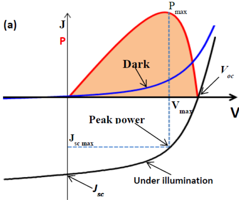
Figure 6.4: I-V curve showing the important parameters.
