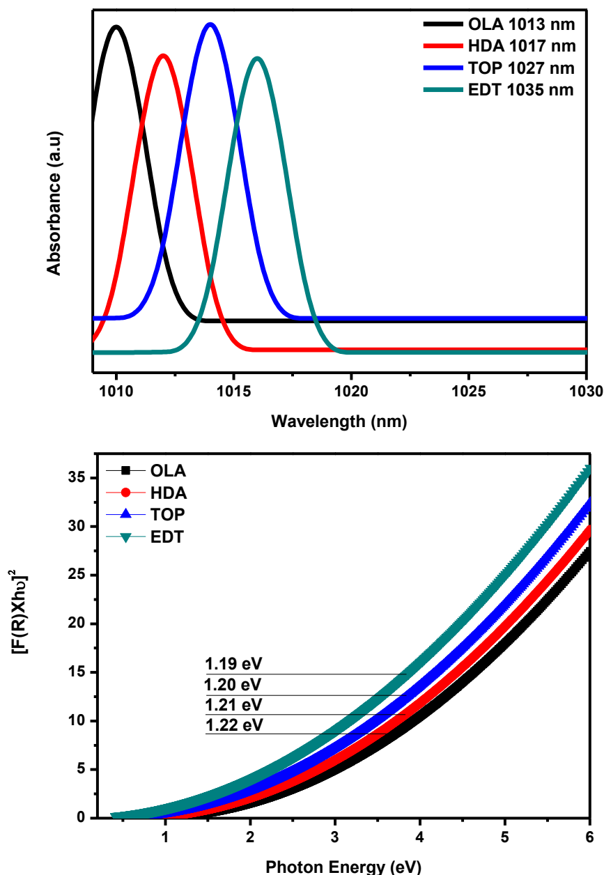
Figure 4.8: UV–Vis–NIR absorbance spectrum (top) and optical band gap (bottom) of \text{CuInTe}_2 crystallites synthesized at 250 °C using various capping agents.
