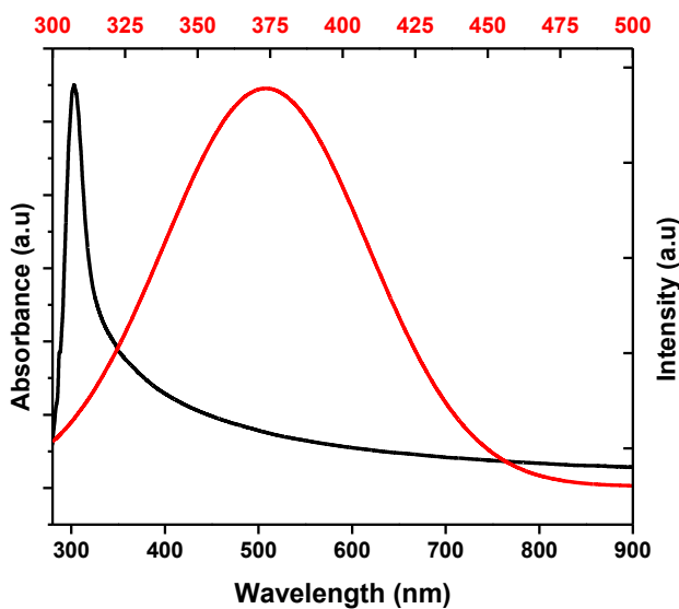
Figure 6.2: UV-Vis absorption and photoluminescence spectra of ZnO.
