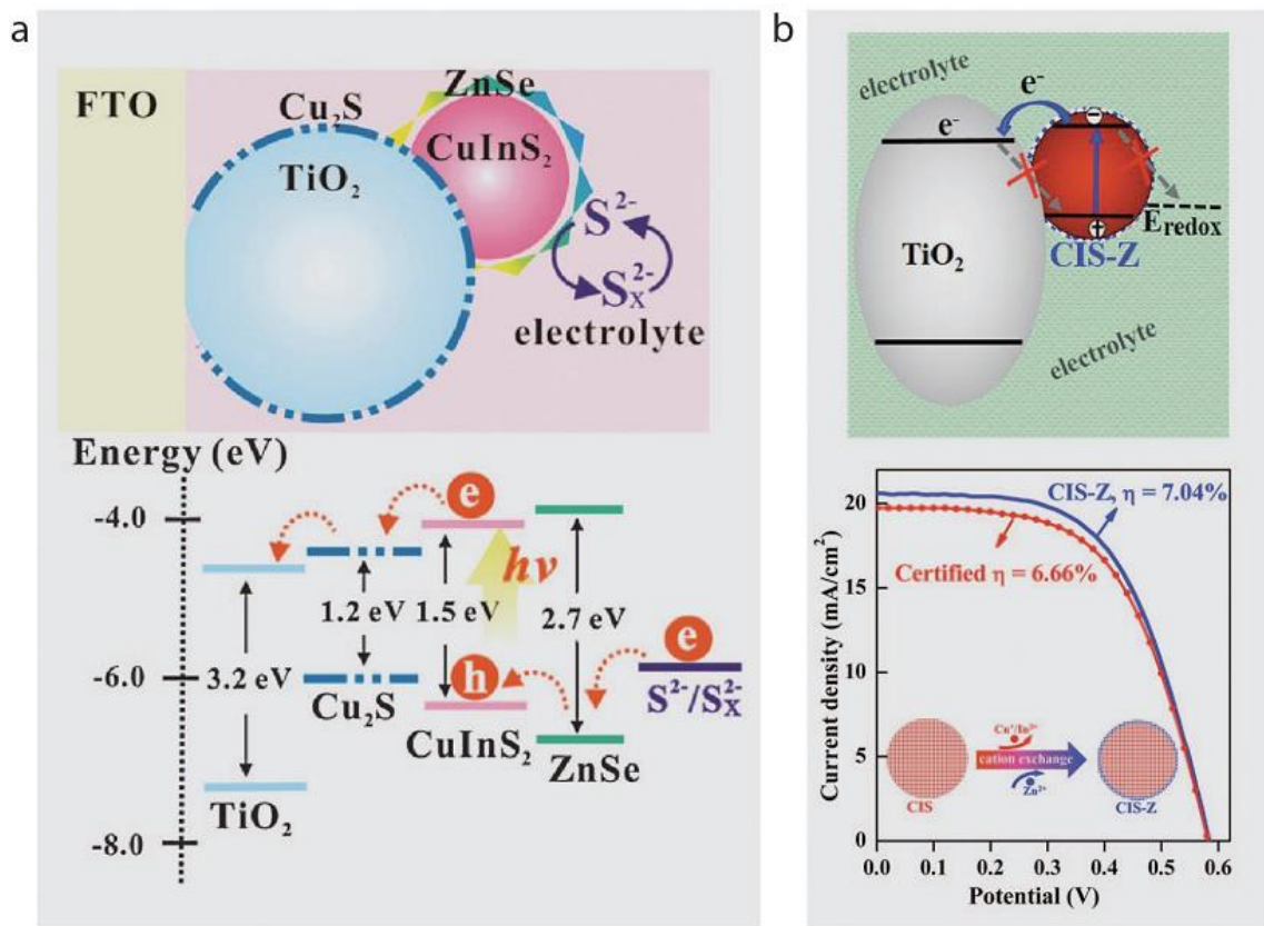
Figure 2.9: Quantum-dot-sensitized solar cells with CIS NCs as sensitizers. (a) The electrons are effectively injected into the TiO 2 particles, whereas the hole is captured by
