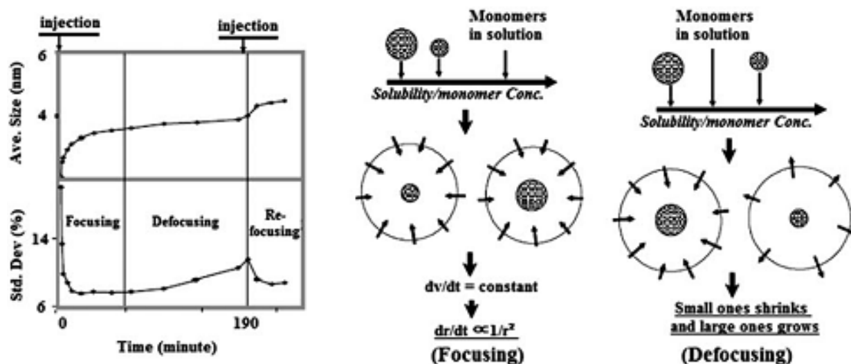
Figure 4.2: (a) Temporal evolution of the size distribution of CdSe NCs prepared by a hot injection method, including a secondary injection during the reaction. (b) Illustration of the focusing and defocusing of size distribution observed in (a) (reproduced with permission from ref. 52, copyright 1998, American Chemical Society, and ref. 53, copyright 2005, Springer) [2].
