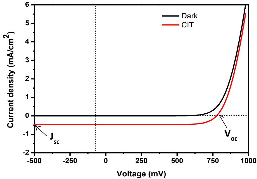
Figure 6.6: I-V curve of the EDT capped CuInTe 2 nanosheets.
