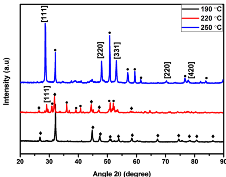
Figure 3.1: XRD patterns of crystallites synthesized using method 1 at various temperatures where ♦ = Te phase and • = \text{Cu}_5\text{Te}_3 .
