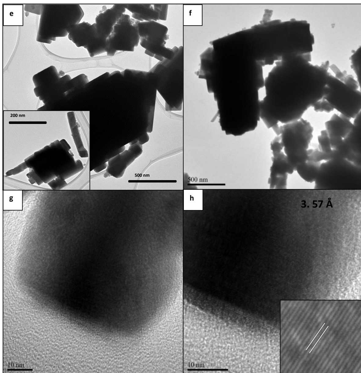
Figure 3.8: TEM and HRTEM micrographs of CuInTe 2 crystallites synthesized at 250 °C using method 1.
