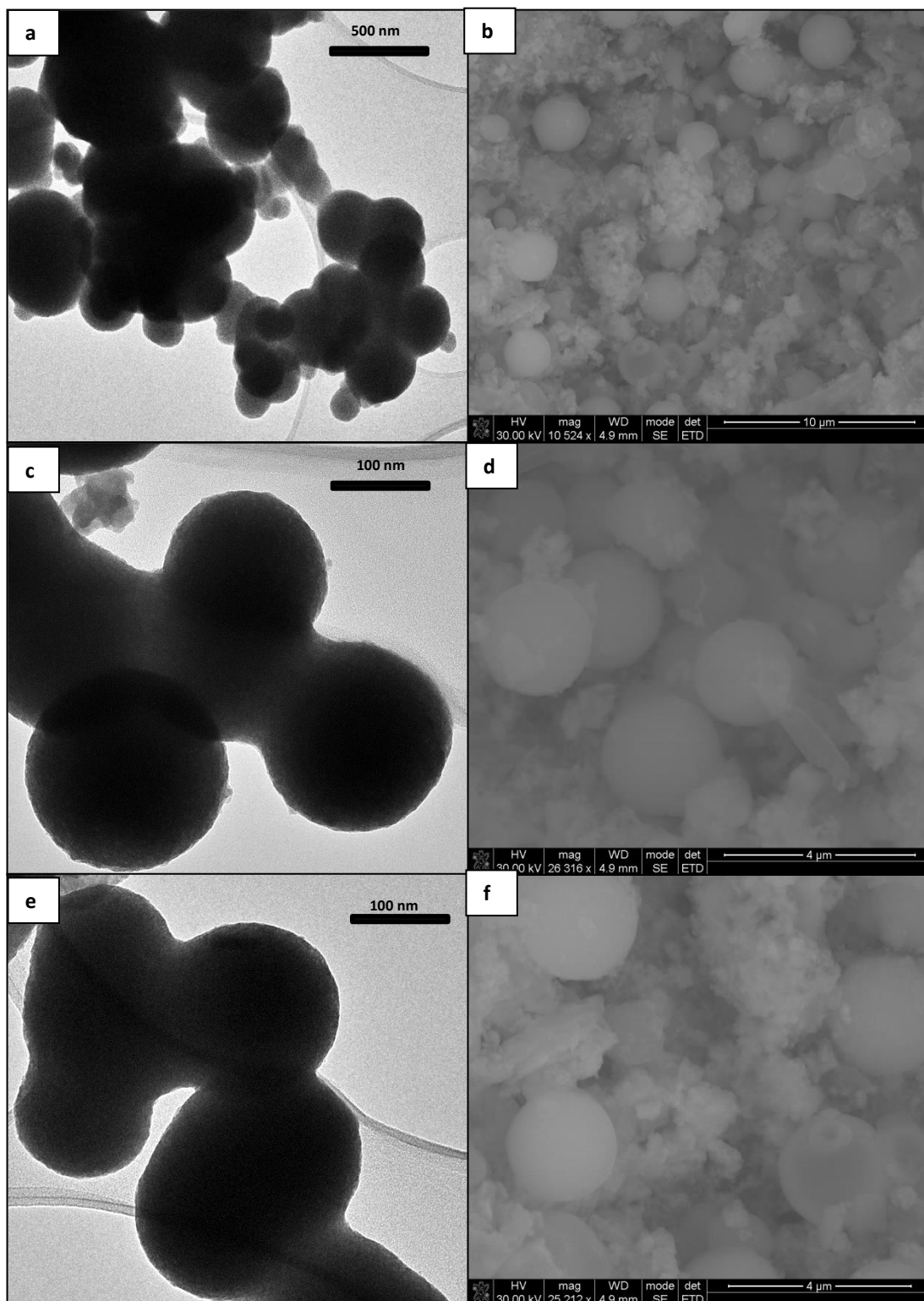
Figure 5.21: TEM and SEM micrographs of \text{CuIn}_{1-x}\text{Ga}_x\text{Te}_2 with precursor concentrations of In: Ga ratios of (a-b) 0.84:0.16, (c-d) 0.64:0.48 and (e-f) 0.26: 0.74 from ICP.
