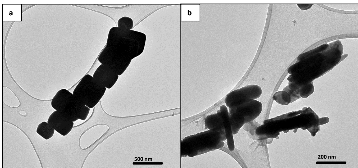
Figure 5.4: TEM micrographs of (a) \text{CuInTe}_2 and (b) \text{CuIn}_{0.8}\text{Ga}_{0.2}\text{Te}_2 semiconductor materials synthesized at 250 °C.
