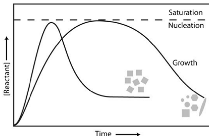
Figure 2.2: The La Mer model of nucleation, where a critical reactant concentration is required for particle nucleation. Homogenous nanoparticle dispersions are favored by a single, rapid nucleation event [25] .
