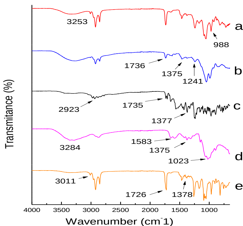
Figure 3.3. FTIR spectra of a) SL-CT-RFP, b) SL-CT, c) RFP, d) CT and e) SL.
