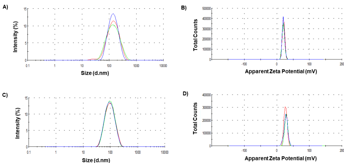
Figure 4.2. Graphical illustration of the Size distribution by intensity of CT-SL-RFP-ISON (A) and Mn-CT-SL-RFP-ISON (C) Nanoparticles, using Dynamic Light Scattering, and their Apparent zeta potentials (B and D, respectively). The nanoparticles expressed a positive surface charge, which prevents flocculation/coalescence of the nanoparticles in suspension, and this may contribute to their stability. In both formulations n=3 and SD < 0.3 .
