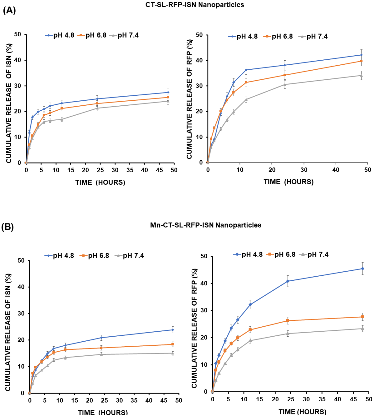
Figure 4.10. In vitro RFP and ISN release profile from CT-SL-RFP-ISN (A) and Mn-CT-SL-RFP-ISN (B) nanoparticles in pH 4.8, 6.8 and 7.4, and at 37°C (n = 3, mean \pm SD).
