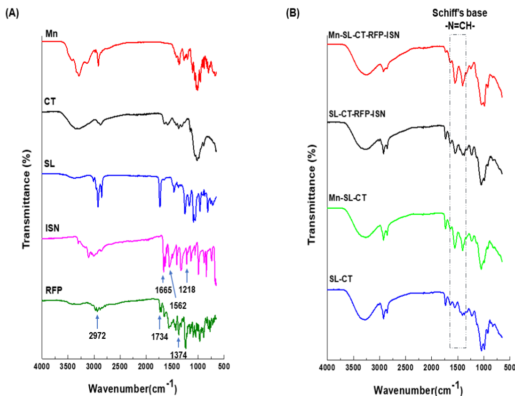
Figure 4.6. FTIR spectra of pure drugs, pristine polymers, mannosylated and unmannosylated nanoparticles showing the various molecular compositions and transitions upon polymer hybridization, drug incorporation and mannose-functionalization. (A) Mn, CT, SL, ISN, and RFP; (B) Mn-CT-SL-RFP-ISN, CT-SL-RFP-ISN, Mn-CT-SL, and CT-SL. CT-SL = unmannosylated chitosan-lecithin nanoparticles; CT-SL-RFP-ISN = unmannosylated rifampicin-isoniazid-loaded chitosan-lecithin nanoparticles; Mn-CT-SL = mannosylated chitosan-lecithin nanoparticles; Mn-CT-SL-RFP-ISN = mannosylated rifampicin-isoniazid-loaded chitosan-lecithin nanoparticles; CT = Chitosan; SL = L- \alpha -Lecithin soybean; RFP = rifampicin; ISN = isoniazid.
