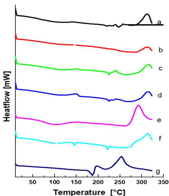
Figure 3.4. DSC thermograms of a) SL-CT-RFP 3:1, b) SL-CT-RFP 1:1, c) SL-CT 3:1, d) SL-CT 1:1, e) CT, f) SL and g) RFP
