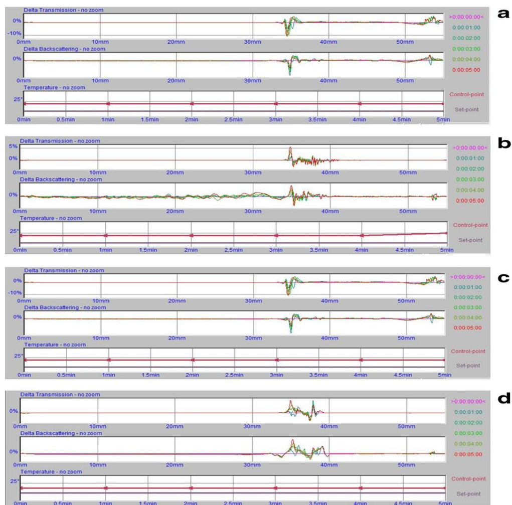
Figure 3.7. Representation of the destabilization kinetics of a) SL-CT 1:1, b) SL-CT 3:1, c) SL-CT-RFP 1:1 and d) SL-CT-RFP 3:1 suspension, indicating \Delta BS and T measured at 25 \pm 0.5 °C for 5-minutes duration.
