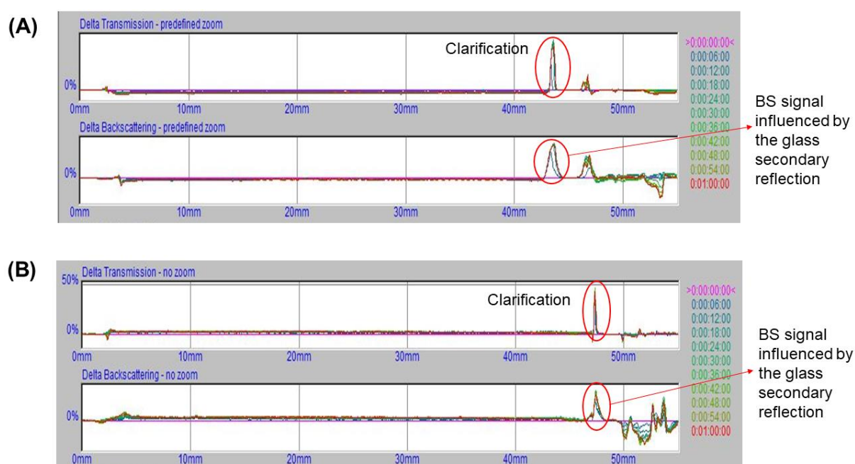
Figure 4.9. Delta transmission (top) and delta backscattering (bottom) for CT-SL-RFP-ISN nanoformulation (A) and Mn-CT-SL-RFP-ISN nanoformulation (B) measured at 25°C for 60-minutes duration. BS = Backscattering.
