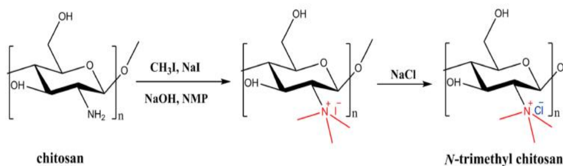
Figure 2.2. Reaction scheme of N-trimethyl chitosan (TMC).
