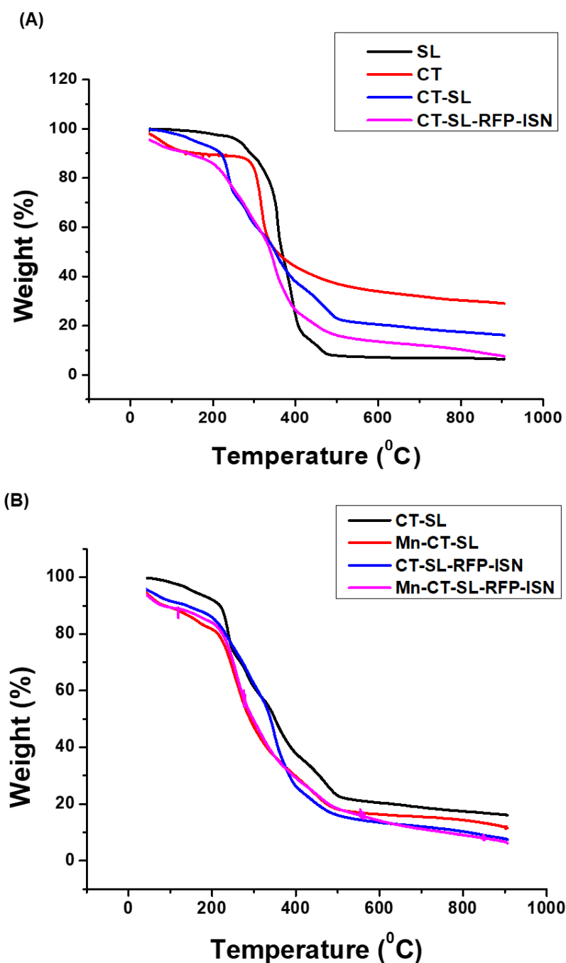
Figure 4.8. Percentage weight versus temperature thermograms depicting the transitions in thermal degradation properties of (A) CT, SL, CT-SL and CT-SL-RFP-ISN, and (B) CT-SL, Mn-CT-SL, CT-SL-RFP-ISN, and Mn-CT-SL-RFP-ISN.
