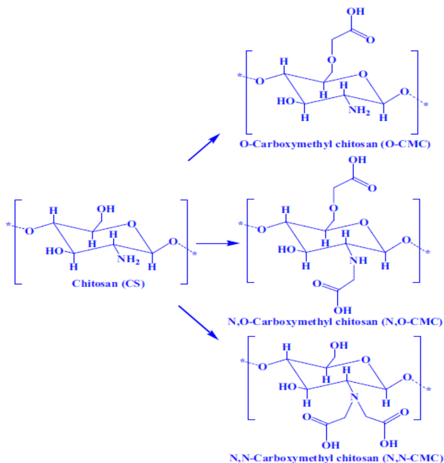
Figure 2.3. The chemical structures of chitosan and the various derivatives of carboxymethyl chitosan (CMC).
