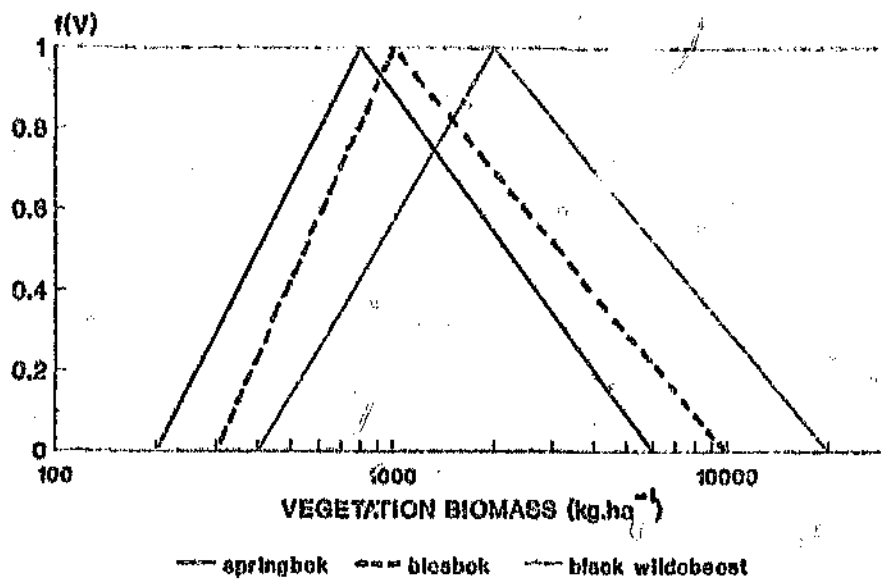
Appendix Figure 2.2 Herbivore functional response f(V) .
