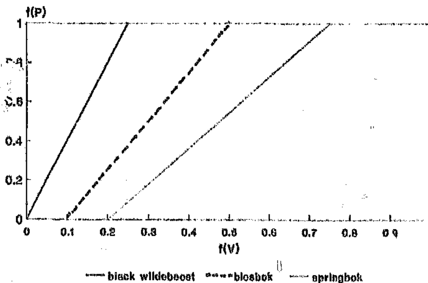
Appendix Figure 2.3 Herbivore population functional response f(P) .
