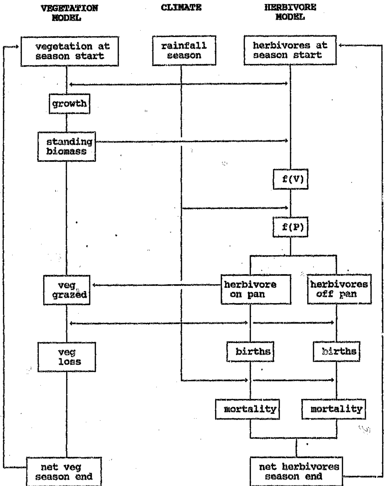
Figure 7.1 Algorithm of plant-herbivore model.
