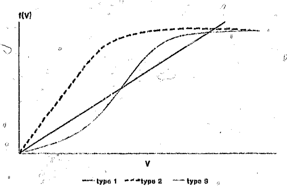
Appendix Figure 2.1 Types of herbivore functional response.
