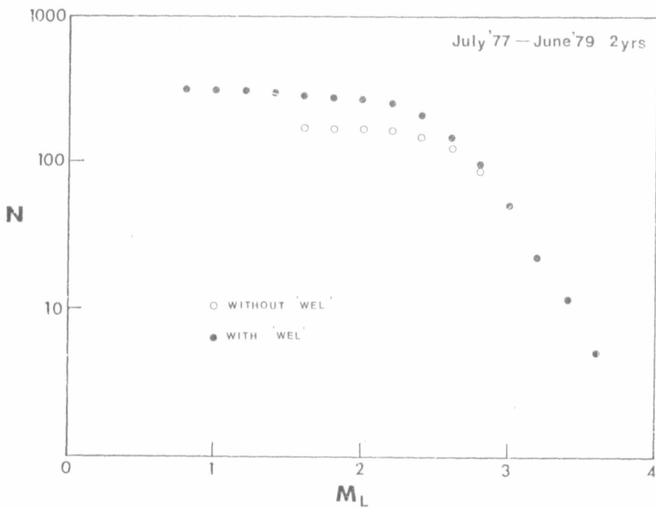
Figure 6.3 Log frequency of events greater than a particular magnitude for the G.S.S.A. records of events originating at Welkom. The data was obtained from the G.S.S.A. monthly seismic bulletins.
