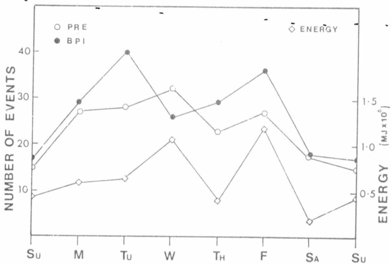
Figure 6.5 Daily variation of Welkom seismic levels expressed in terms of energy, open squares and number of events circles. BPI data represents a magnitude range of -0.5 to 2.7 Pretoria data (GSSA) represents a range of 2.0 up to 5.4.
