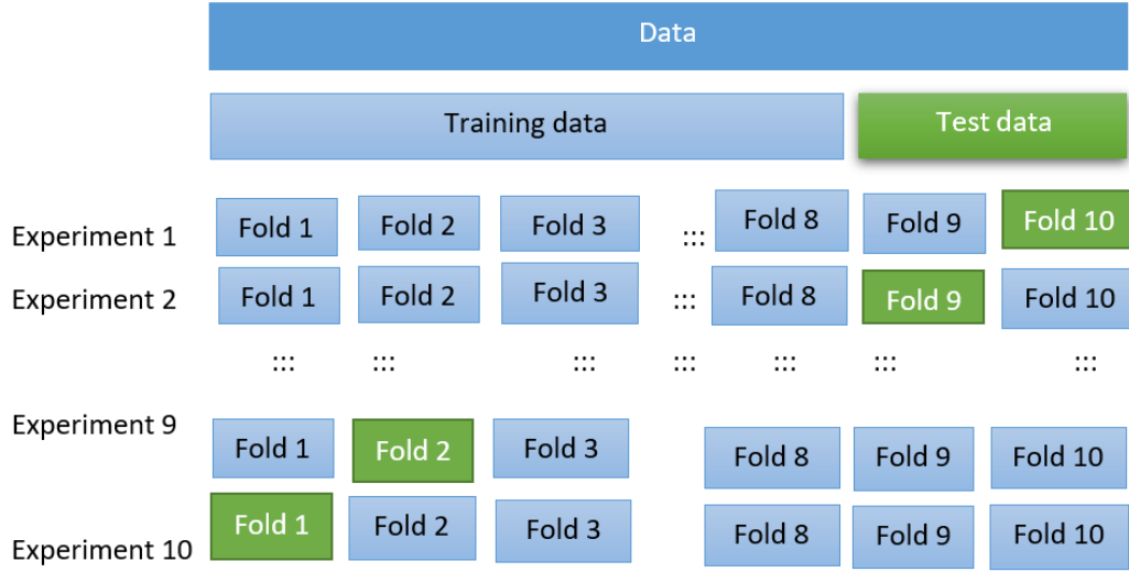
FIGURE 3.5: A 10-fold cross-validation
