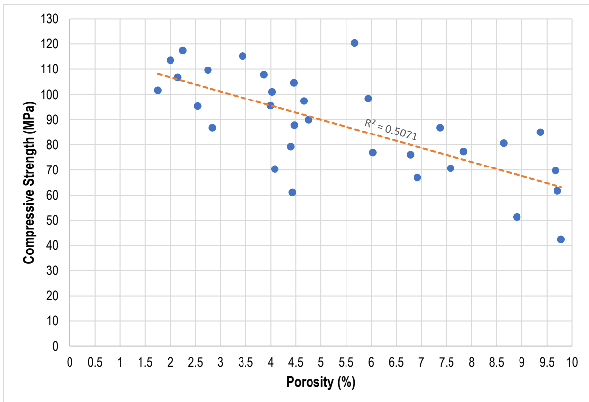
Figure 4.60: Relationship between Compressive Strength and Porosity Determined Using Water Sorptivity Index Test
