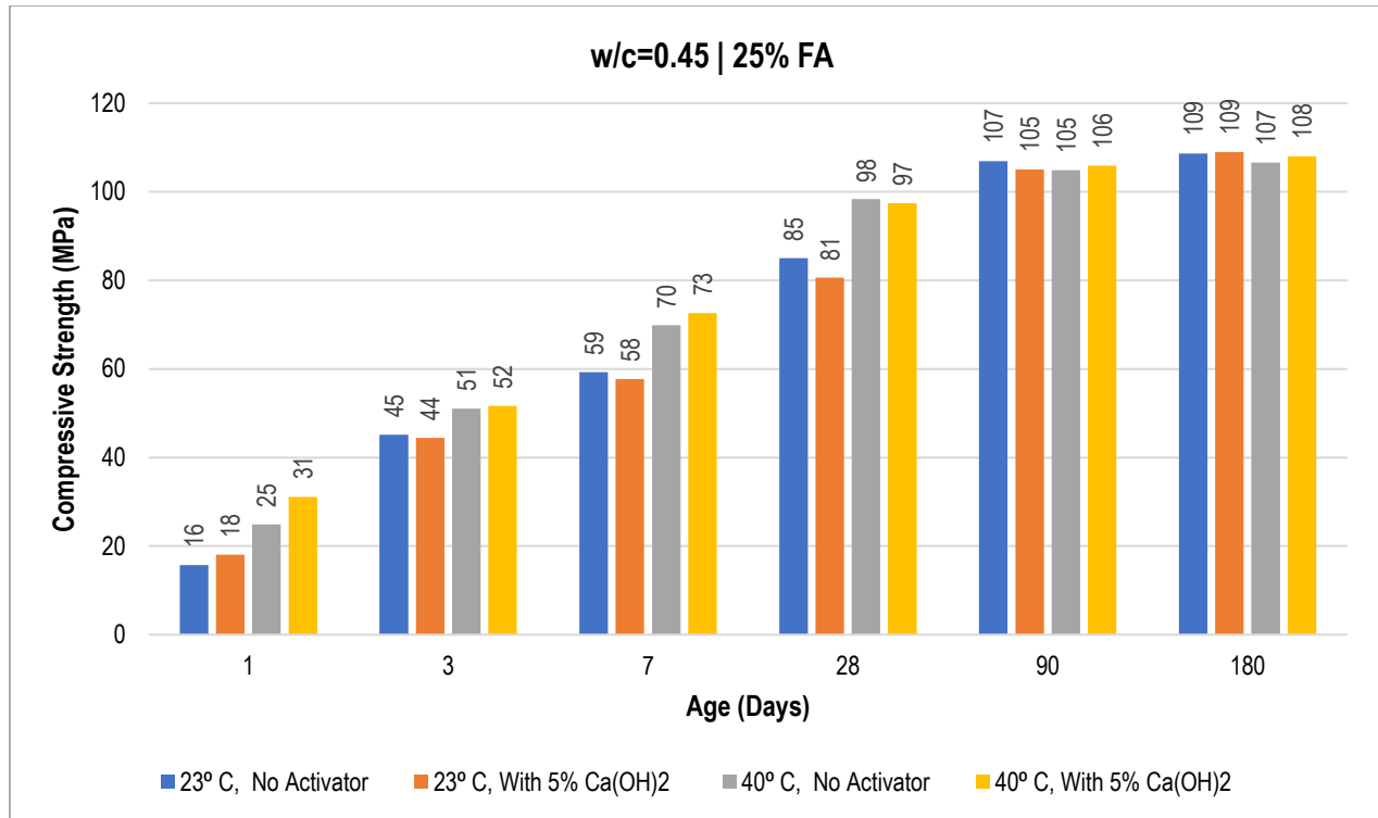
Figure 4.23: Compressive Strength Results for 25%FA Concrete with w/c ratio of 0.45
