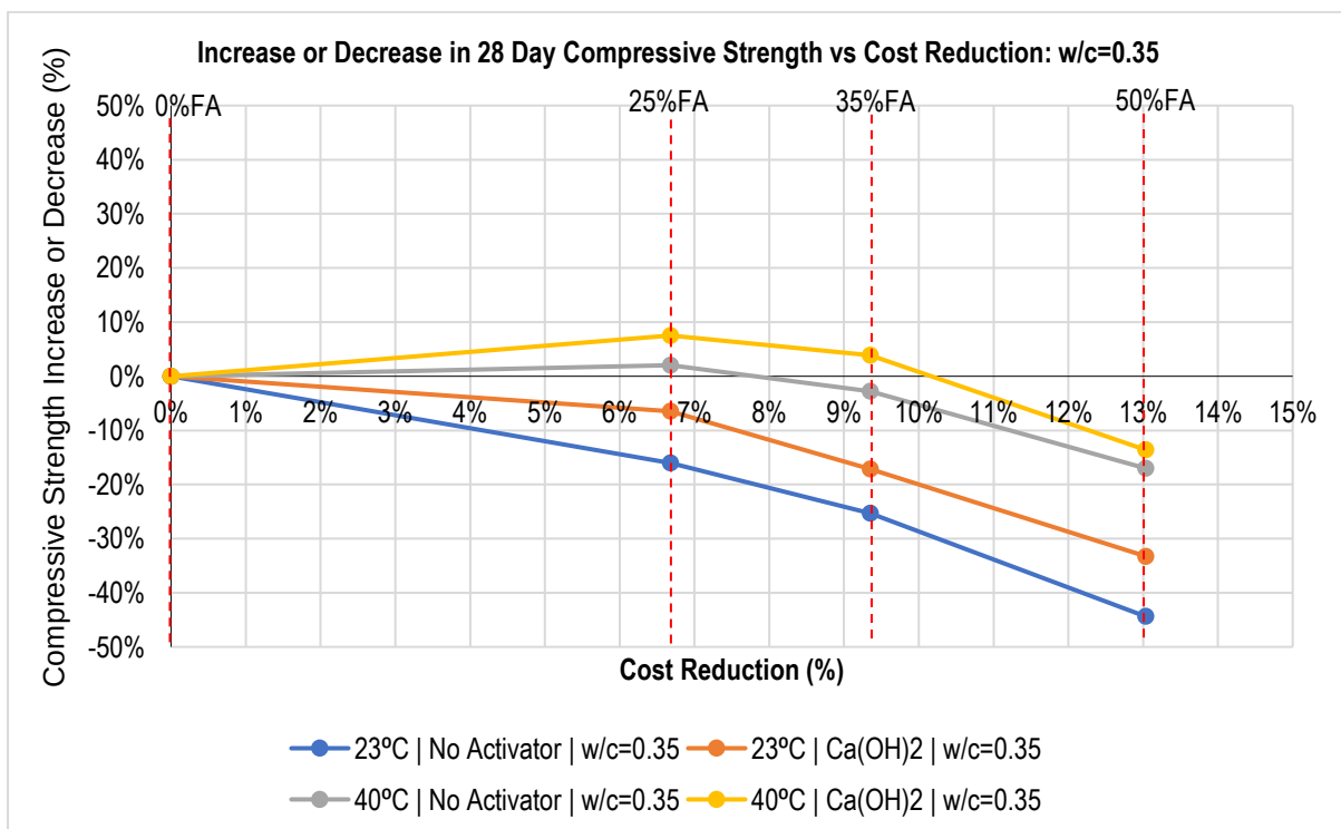
Figure 5.4: Increase or Decrease in 28 Day Compressive Strength vs Cost Reduction (w/c=0.35)
