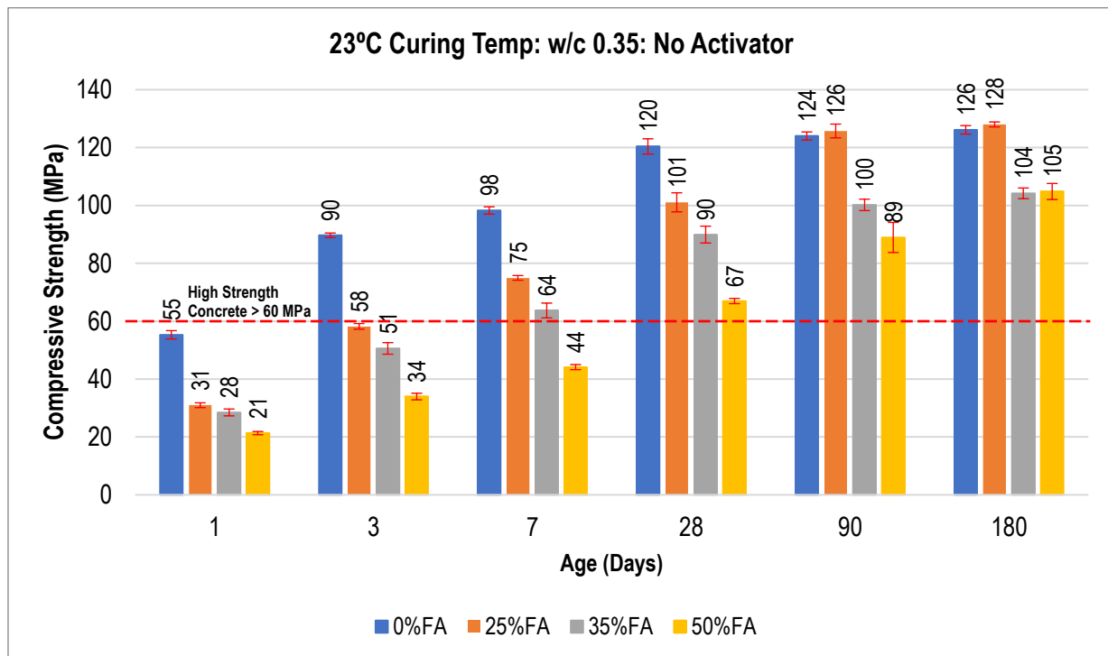
Figure 4.9: Compressive Strength for Concrete Cured at 23°C without \text{Ca(OH)}_2 Activator (w/c = 0.35)
