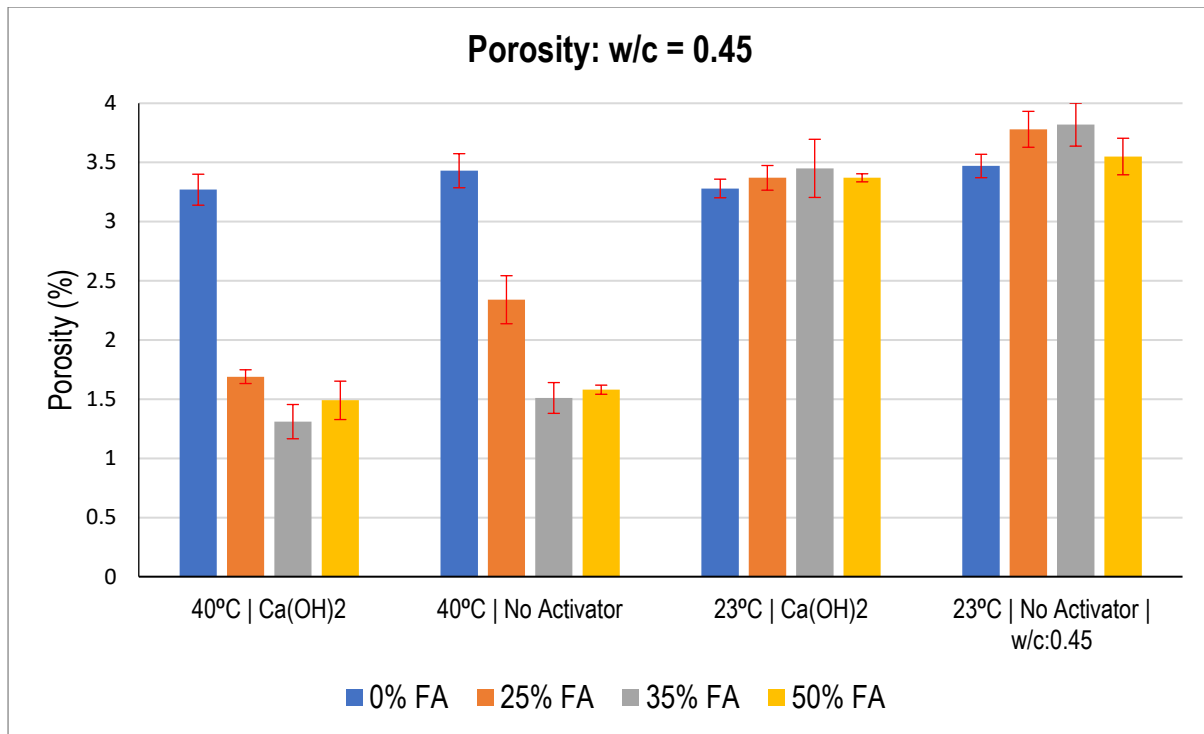
Figure 4.47: Porosity Results from CCI Tests (w/c = 0.45)
