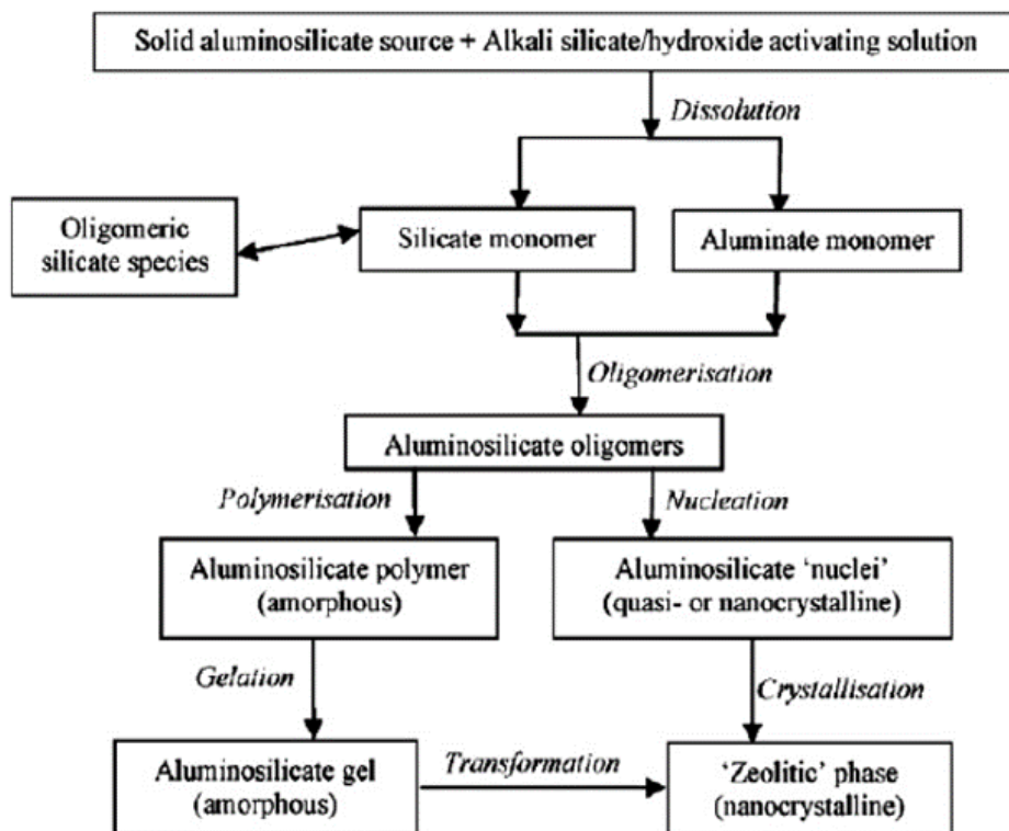
Figure 2.2: Proposed reaction sequence of geopolymerization (Provis et al., 2005)
