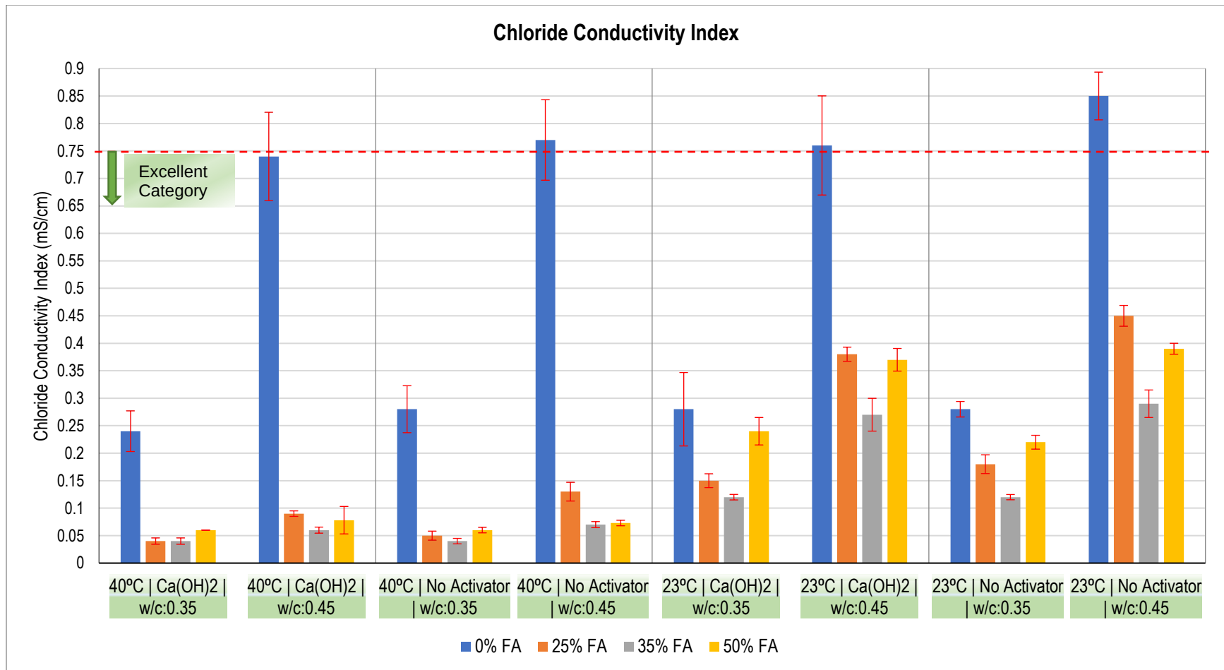
Figure 4.45: Chloride Conductivity Index Results for Specimens with w/c of 0.35 and 0.45
