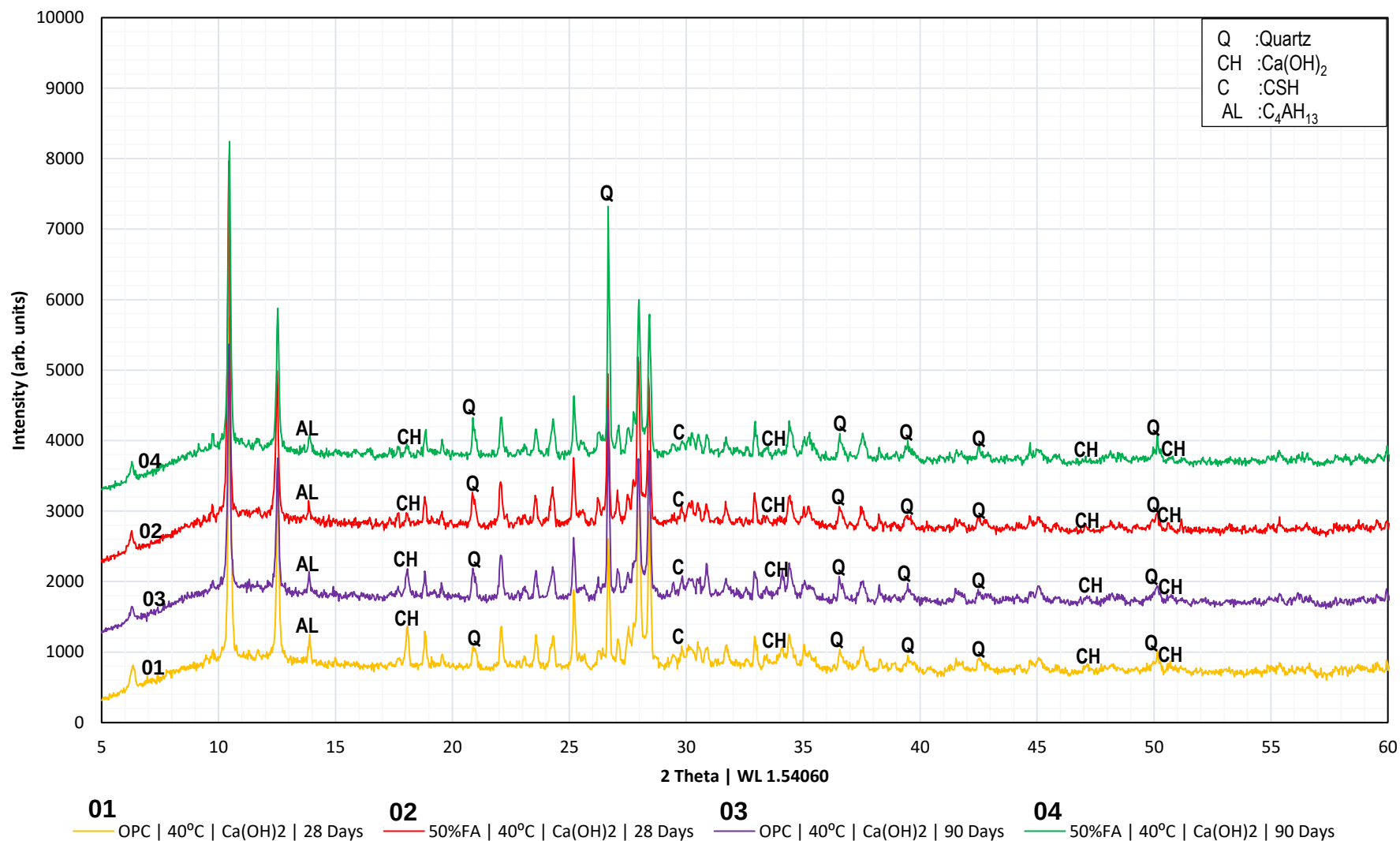
Figure 4.39: XRD Patterns for OPC and 50%FA Concrete cured at 40°C with Ca(OH) 2 Activator
