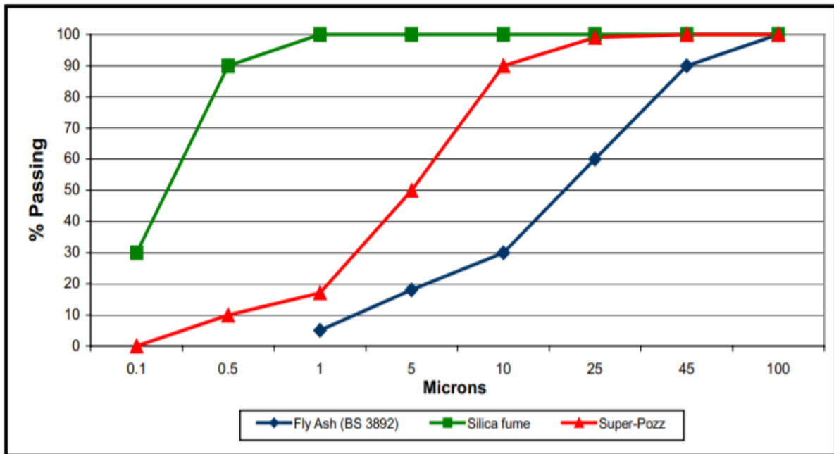
Figure 9.17: Particle Size Distribution for Ultra Fine Fly Ash, Silica Fume and Standard Fly Ash (Source: Seedat, 2003)
