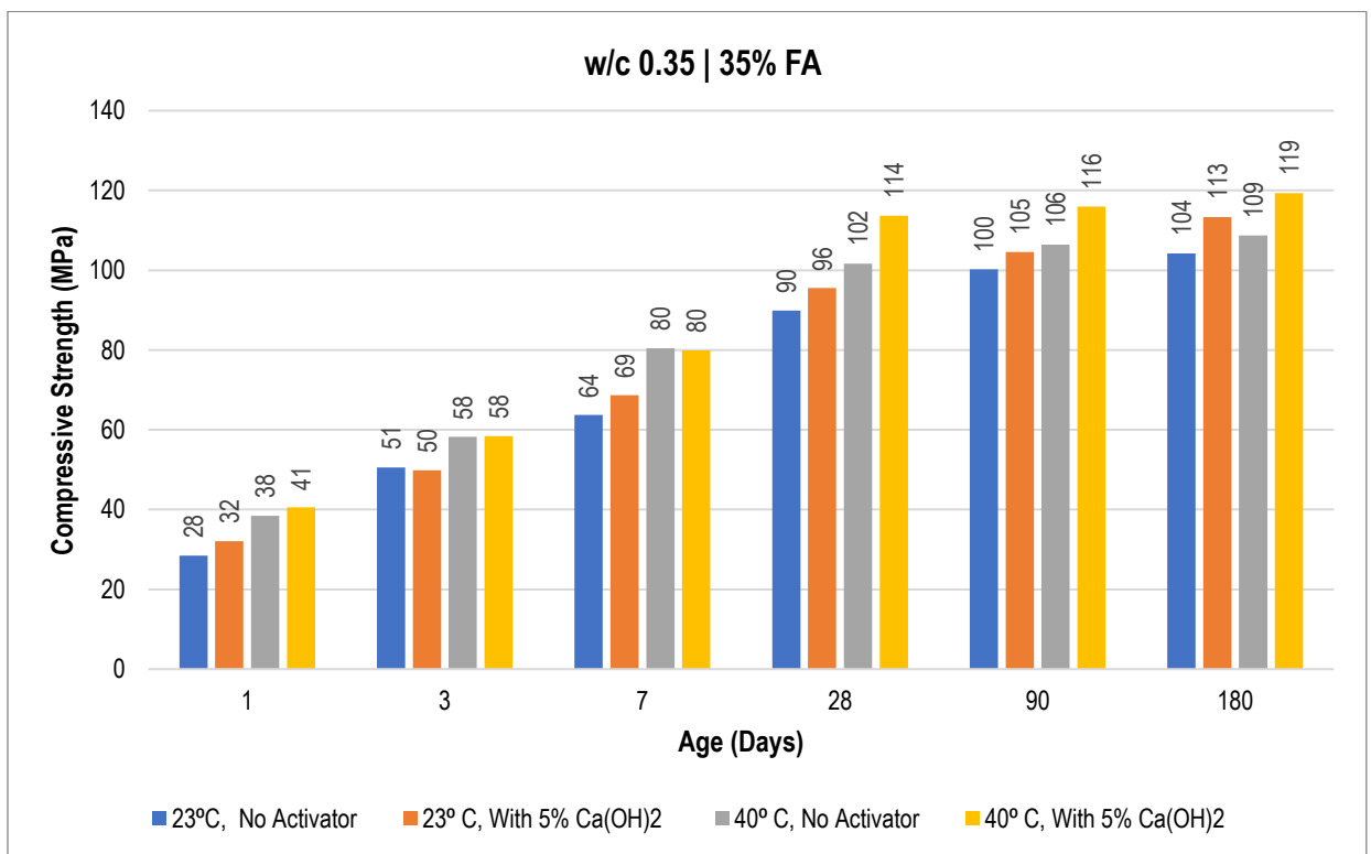
Figure 4.29: Compressive Strength Results for 35%FA Concrete with w/c ratio of 0.35
