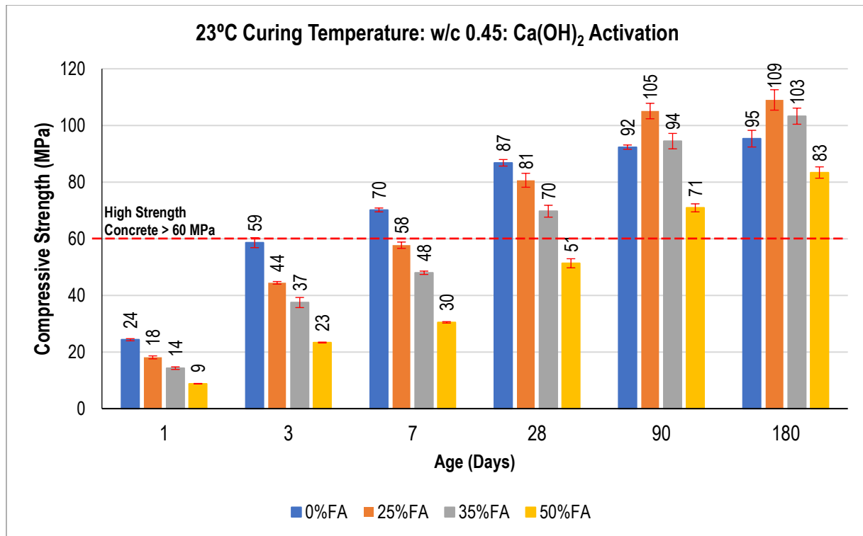
Figure 4.3: Compressive Strength for Cubes Cured at 23°C with Ca(OH) 2 Activation (w/c = 0.45)
