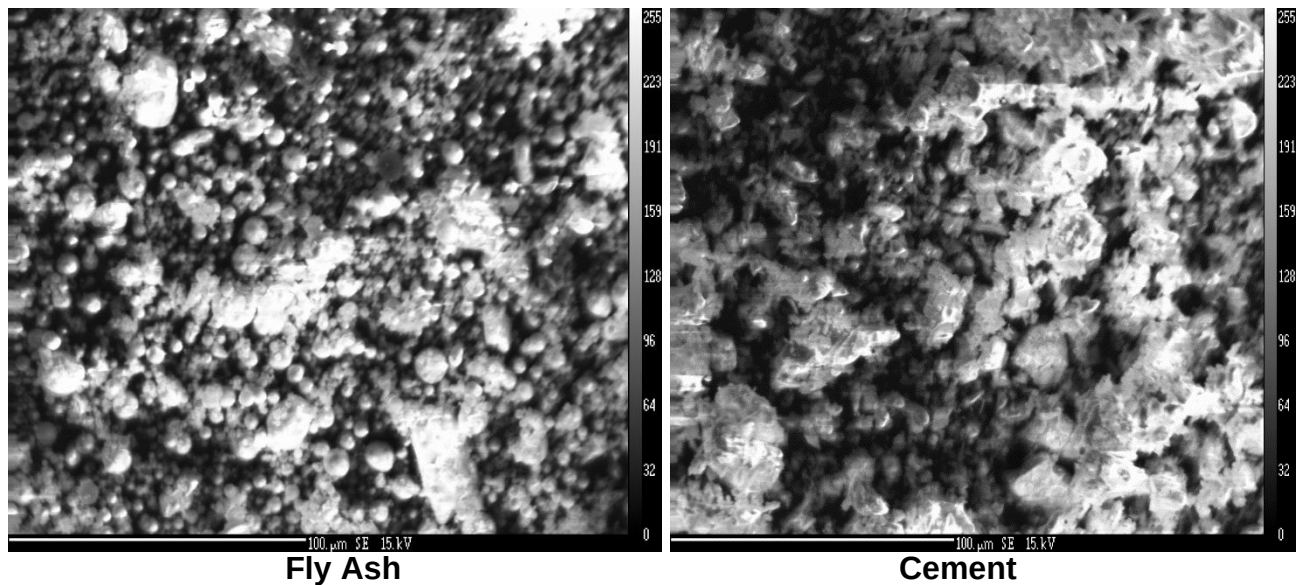
Figure 3.5: Cement and Fly Ash SEM Images
