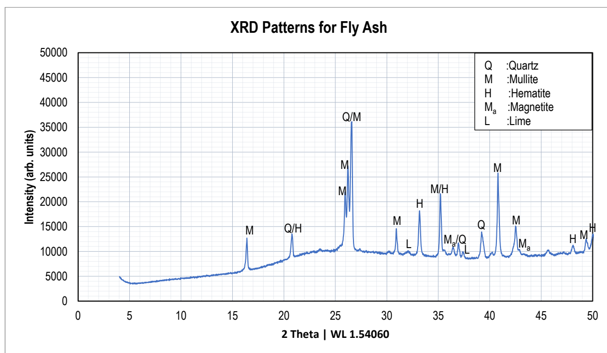
Figure 3.4: XRD Pattern for Fly Ash
