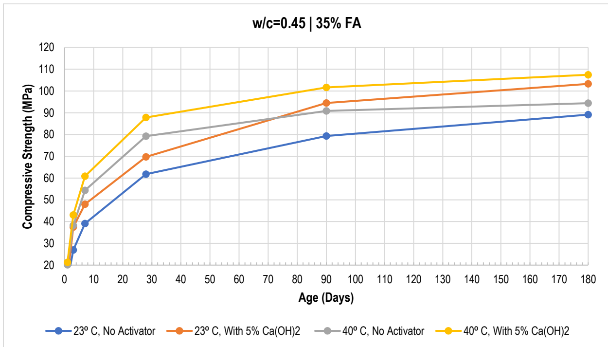
Figure 4.26: Compressive Strength Results for 35%FA Concrete with w/c ratio of 0.45
