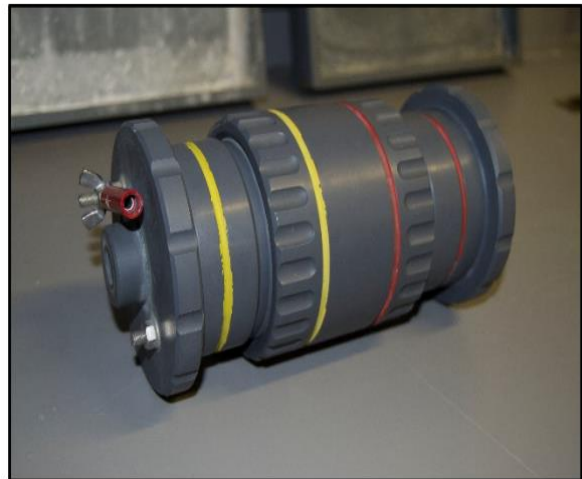
Figure 3.21: Chloride Conductivity Cell (Durability Index Testing Procedure Manual, 2018)
