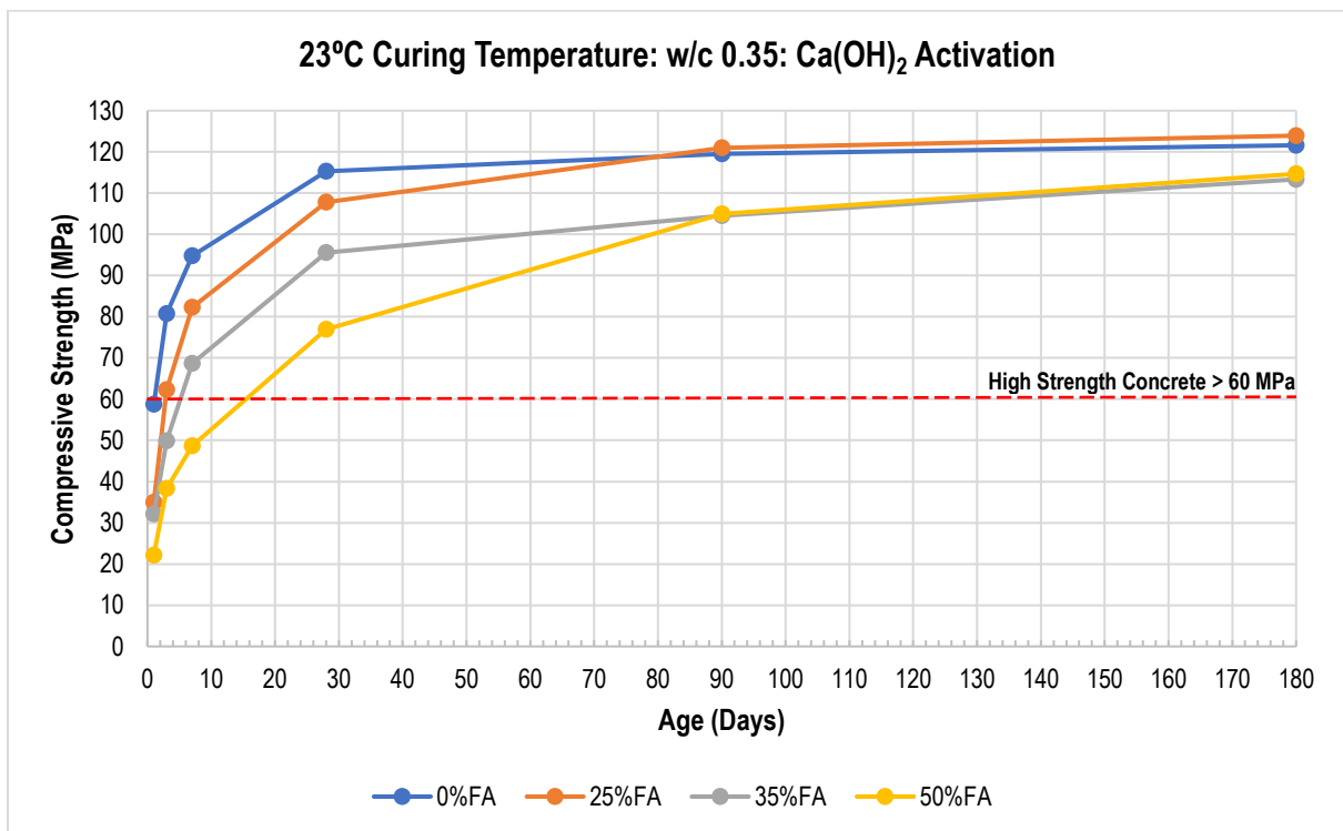
Figure 9.6: Compressive Strength for Concrete Cured at 23°C with \text{Ca(OH)}_2 Activation (w/c = 0.35)
