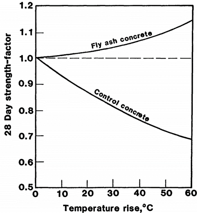
Figure 4.36: Effect of curing temperature rise on compressive strength development (Berry and Malhotra, 1987)
