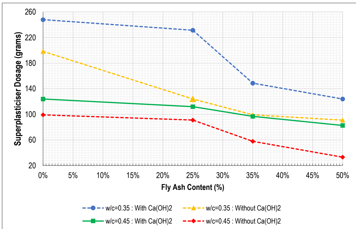
Figure 3.16: Comparison of superplasticiser dosages
