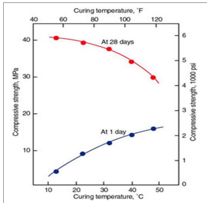
Figure 4.19: Effect of Curing Temperature on Compressive Strength (Zemajtis, 2014)
