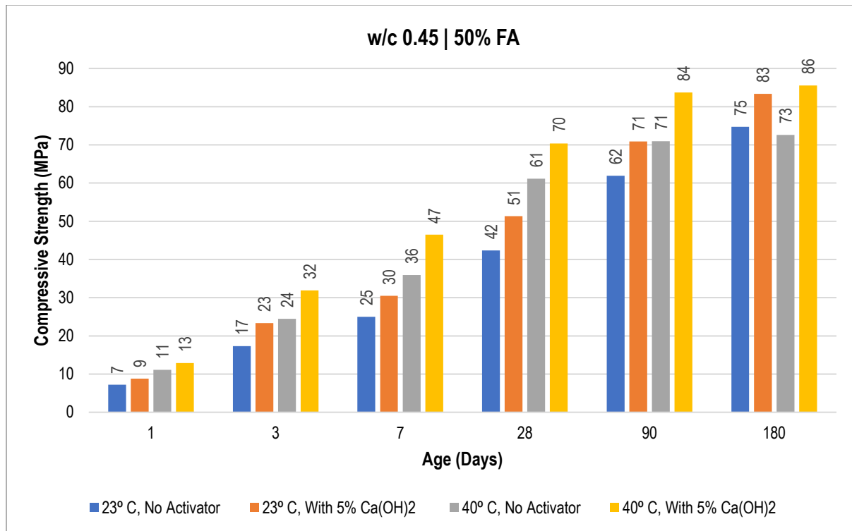
Figure 4.31: Compressive Strength Results for 50%FA Concrete with w/c ratio of 0.45
