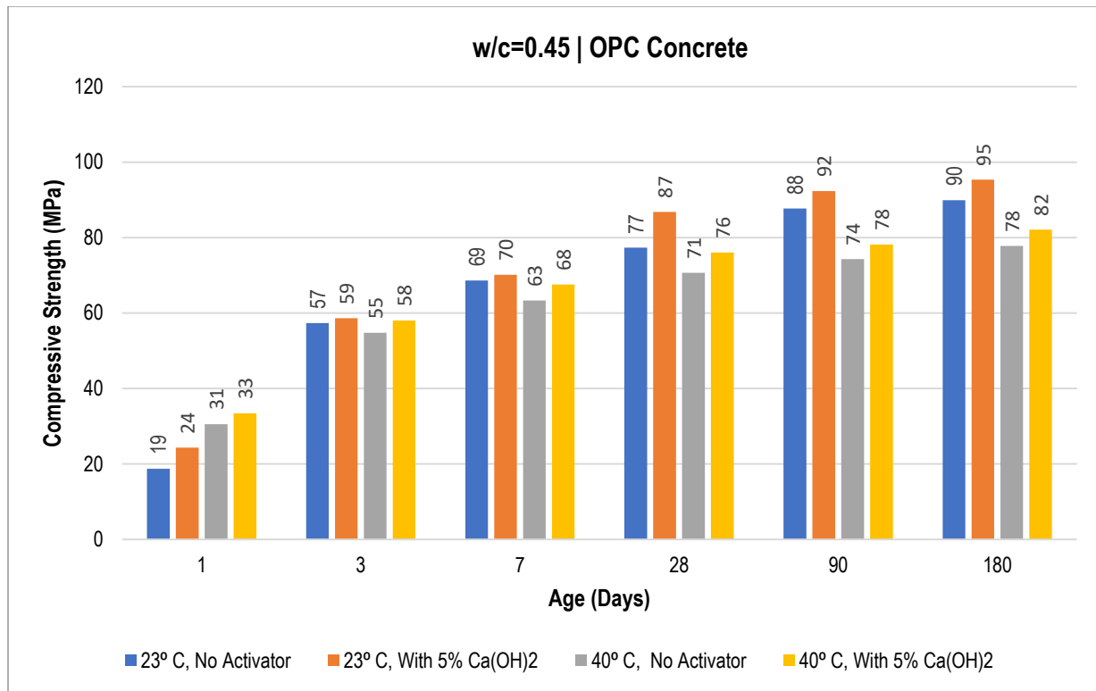
Figure 4.18: Compressive Strength Results of OPC Concrete with w/c ratio of 0.45
