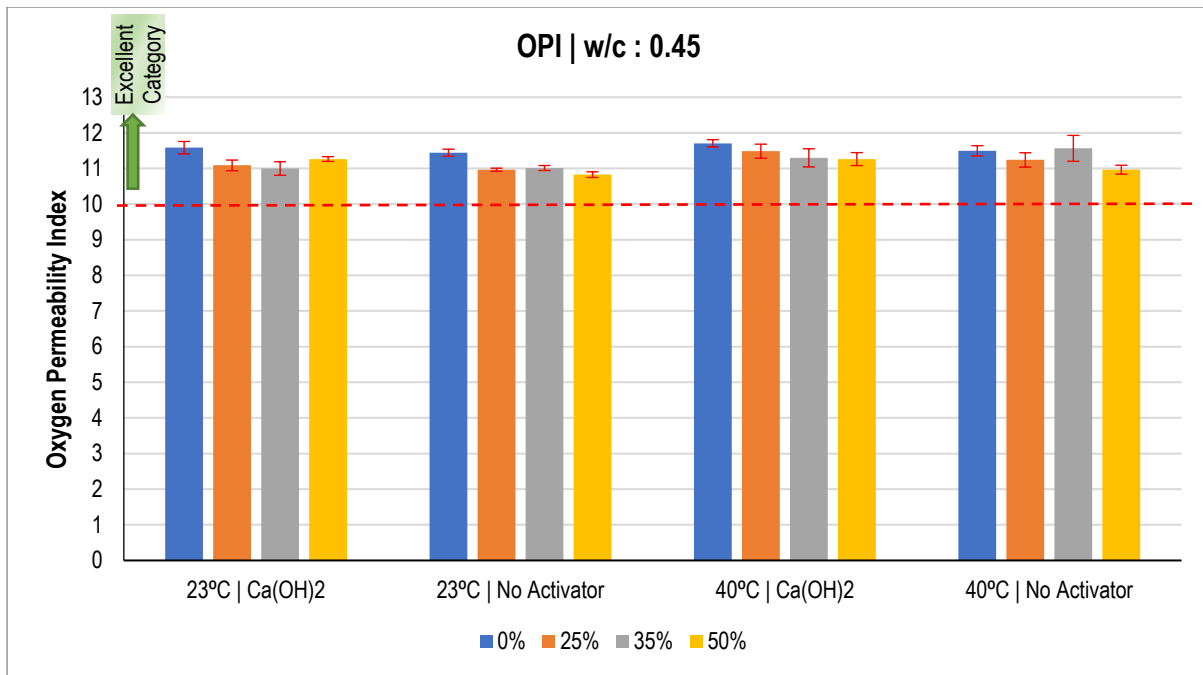
Figure 4.55: Oxygen Permeability Index Results for Specimens with w/c ratio of 0.45
