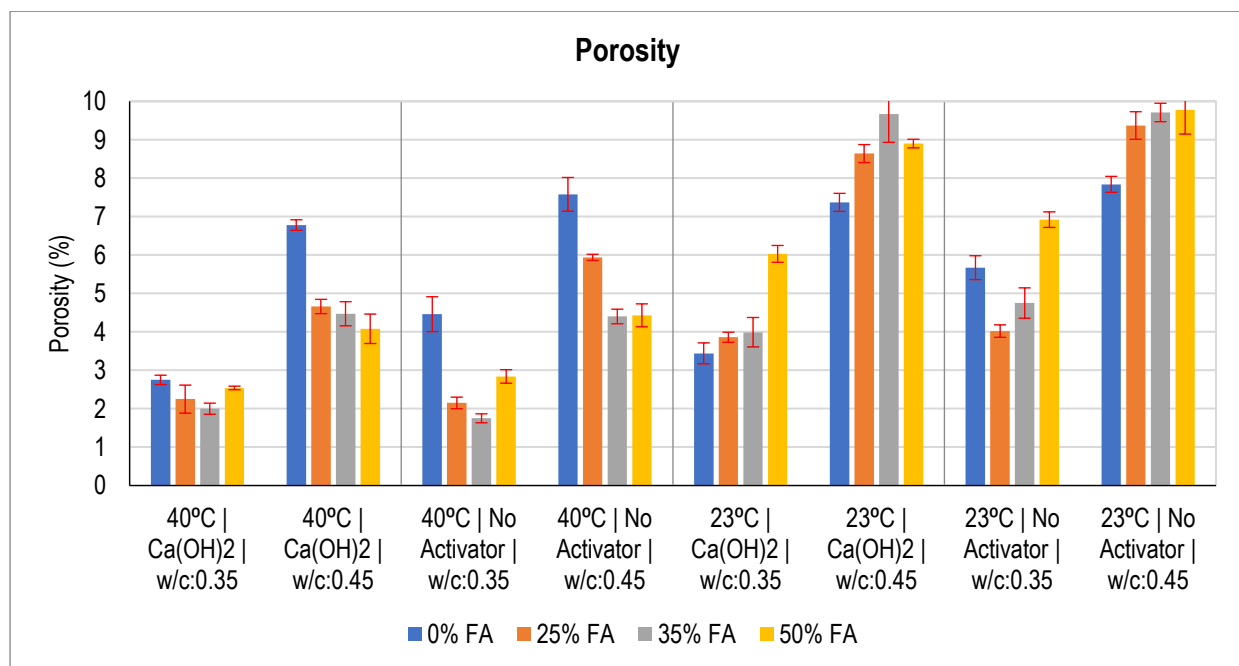
Figure 4.54: Porosity Results for Specimens with w/c of 0.35 and 0.45
