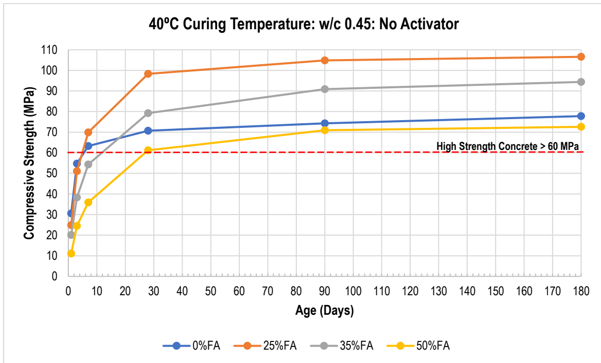
Figure 9.3: Compressive Strength for Concrete Cured at 40°C without \text{Ca(OH)}_2 Activation (w/c = 0.45)
