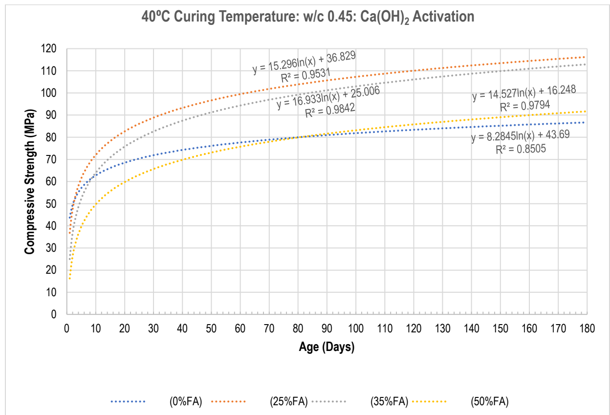
Figure 4.37: Typical Regression Lines for The Relationship Between Compressive Strength and Concrete Age
