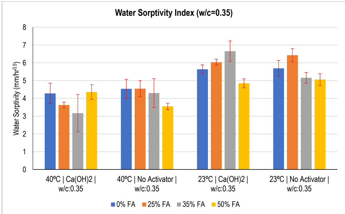
Figure 4.50: Water Sorptivity Index Results for Specimens with w/c of 0.35
