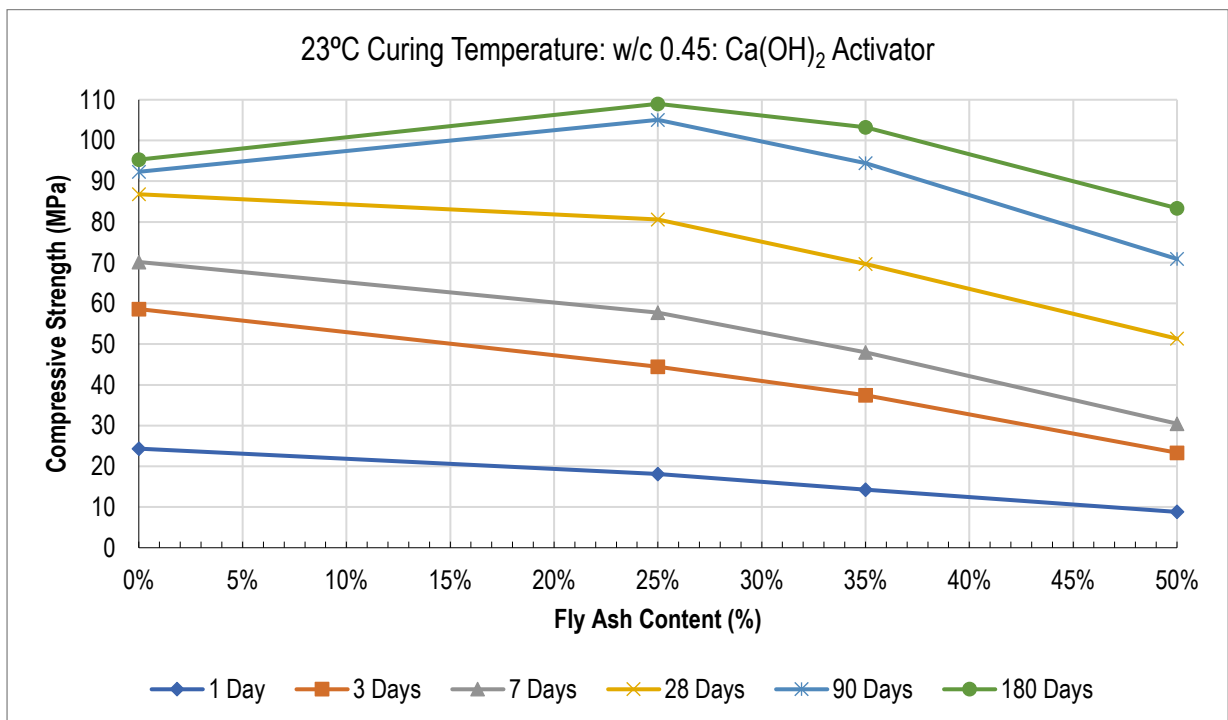
Figure 9.10: Relationship between Compressive strength and FA Content (23°C: w/c 0.45: \text{Ca(OH)}_2 Activator)
