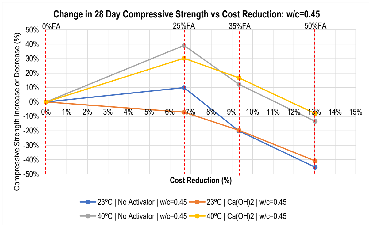
Figure 5.3: Increase or Decrease in 28 Day Compressive Strength vs Cost Reduction (w/c=0.45)
