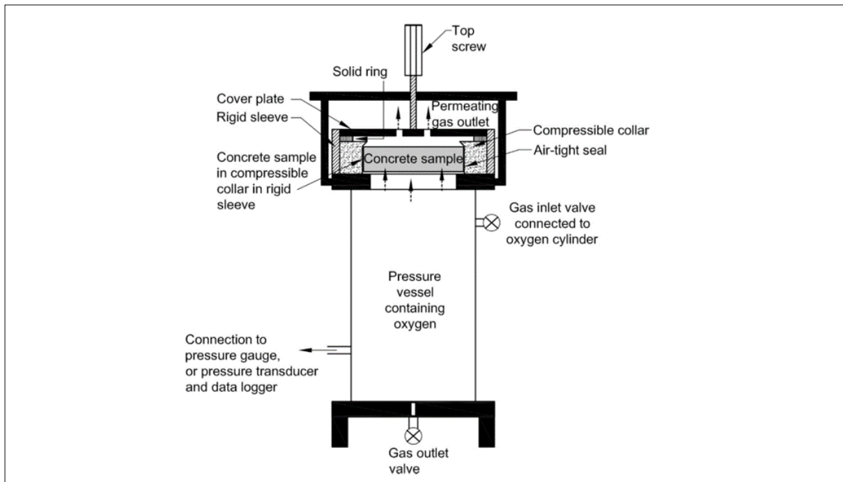
Figure 3.25: Oxygen Permeability Test Setup (Durability Index Testing Procedure Manual, 2018)
