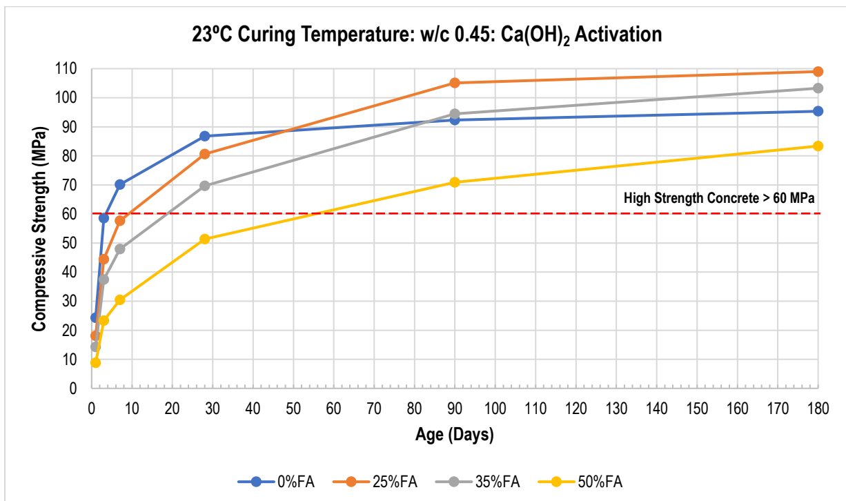
Figure 9.2: Compressive Strength for Concrete Cured at 23°C with \text{Ca}(\text{OH})_2 Activator (w/c = 0.45)
