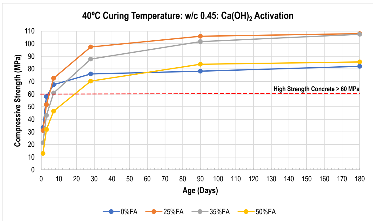
Figure 9.4: Compressive Strength for Concrete at 40°C with \text{Ca(OH)}_2 Activator (w/c = 0.45)
