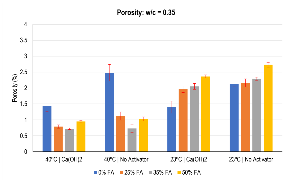
Figure 4.46: Porosity Results from CCI Tests (w/c = 0.35)
