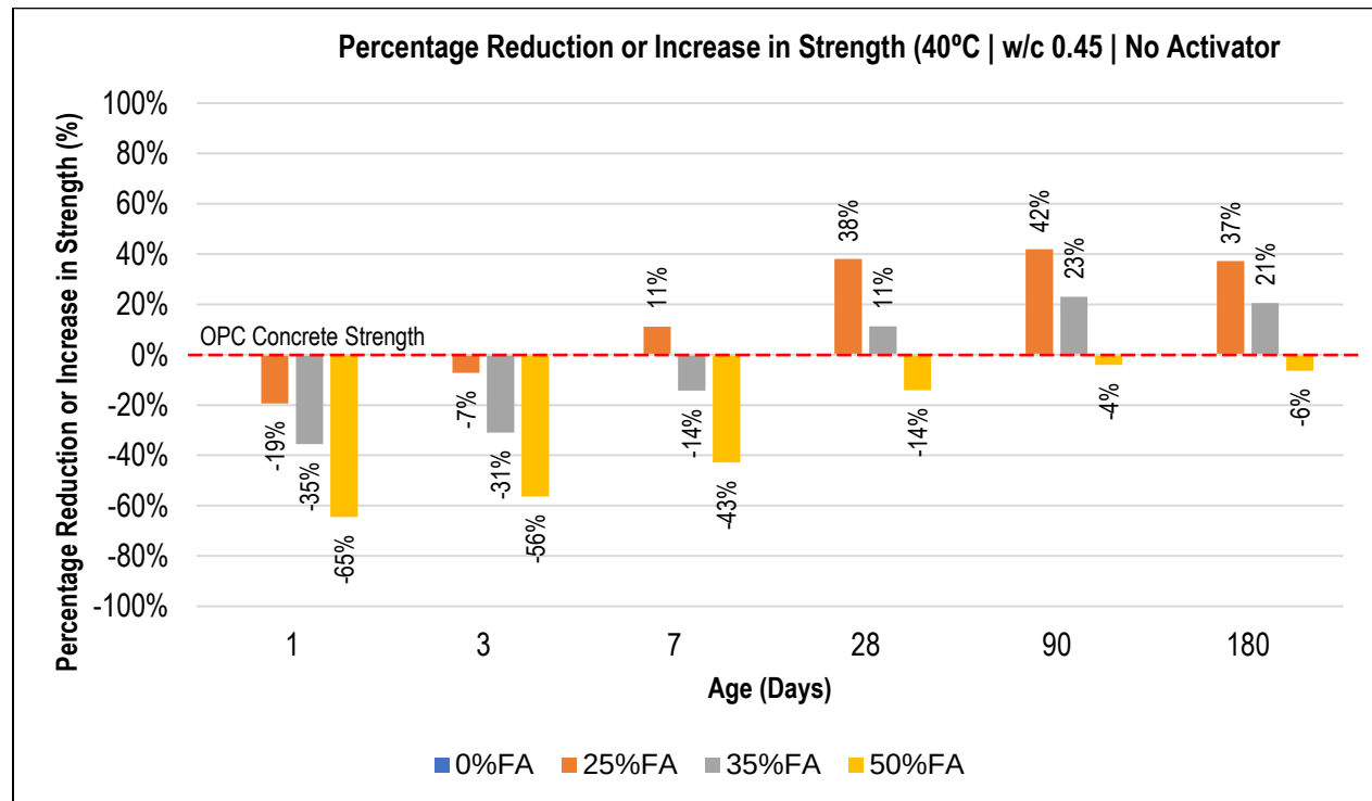
Figure 4.6: Reduction or Increase in Strength as a Percentage of OPC Concrete Strength (40°C:Without Ca(OH) 2 :w/c = 0.45)
