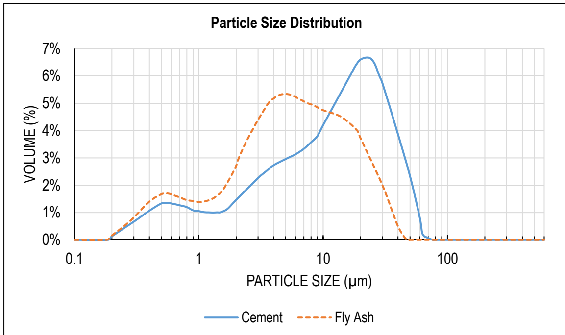
Figure 3.3: Cement and Fly Ash Particle Size Distribution Graph
