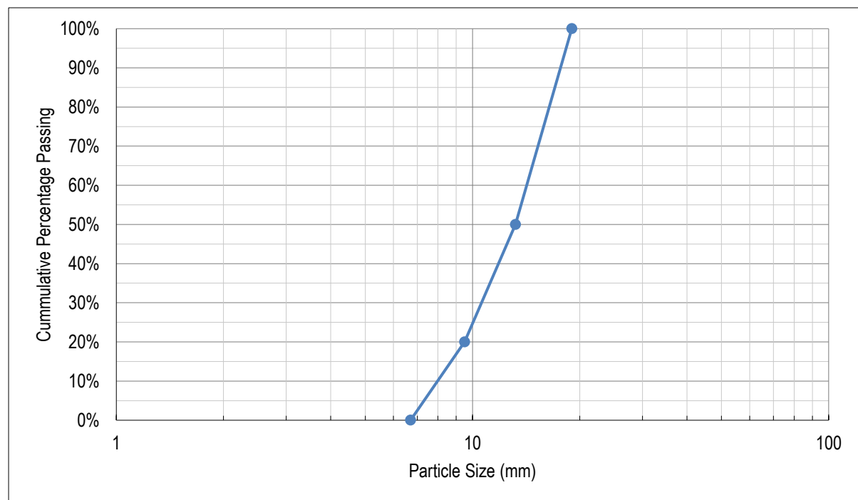
Figure 3.8: Coarse Aggregate Particle Size Distribution
