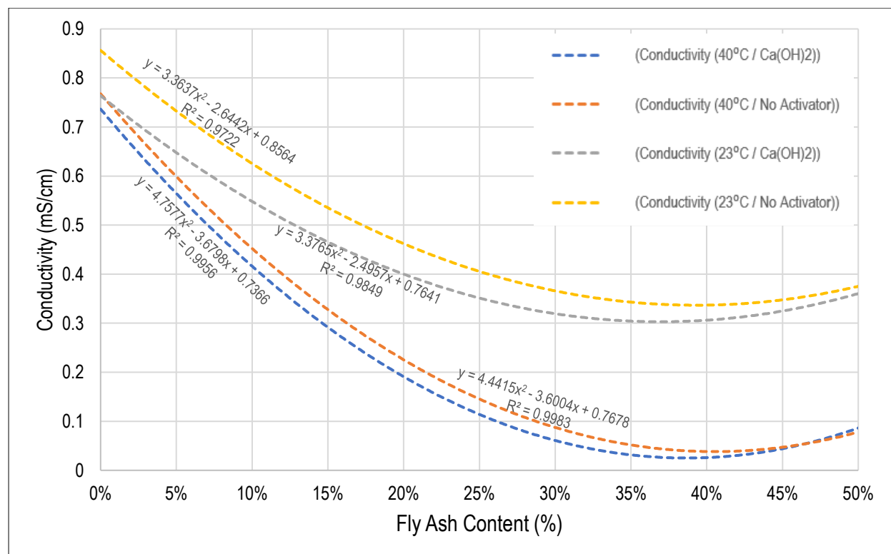
Figure 4.57: Typical Regression Trendlines for the Relationship between FA content and Chloride Conductivity Index
