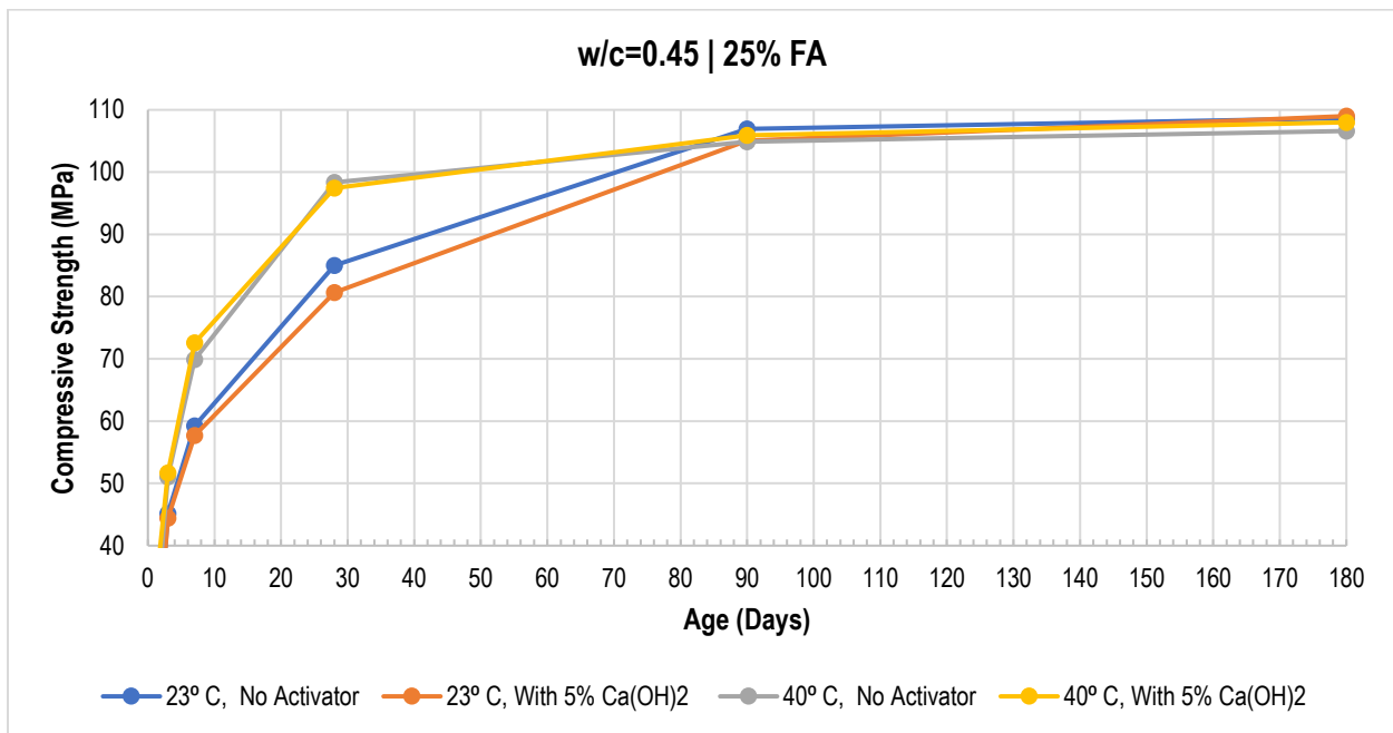
Figure 4.22: Compressive Strength Results for 25%FA Concrete with w/c ratio of 0.45
