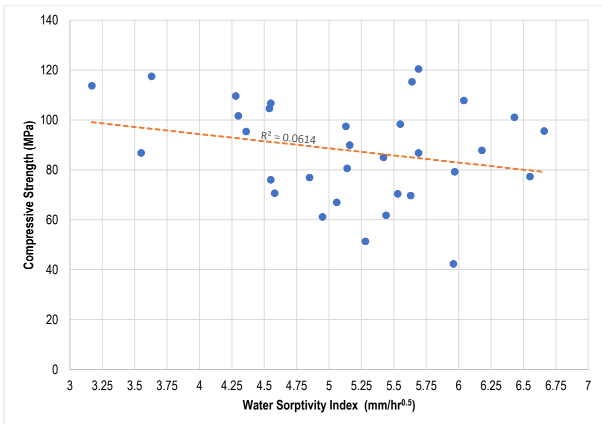
Figure 4.61: Relationship between Compressive Strength and Water Sorptivity Index
