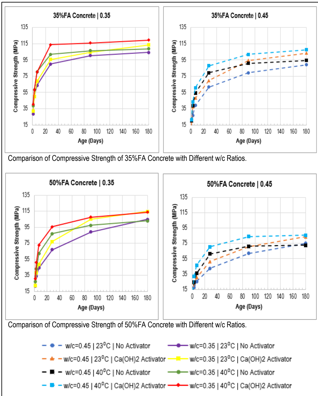
Figure 4.35: Comparison of Compressive Strength of Concrete with Different w/c Ratios
