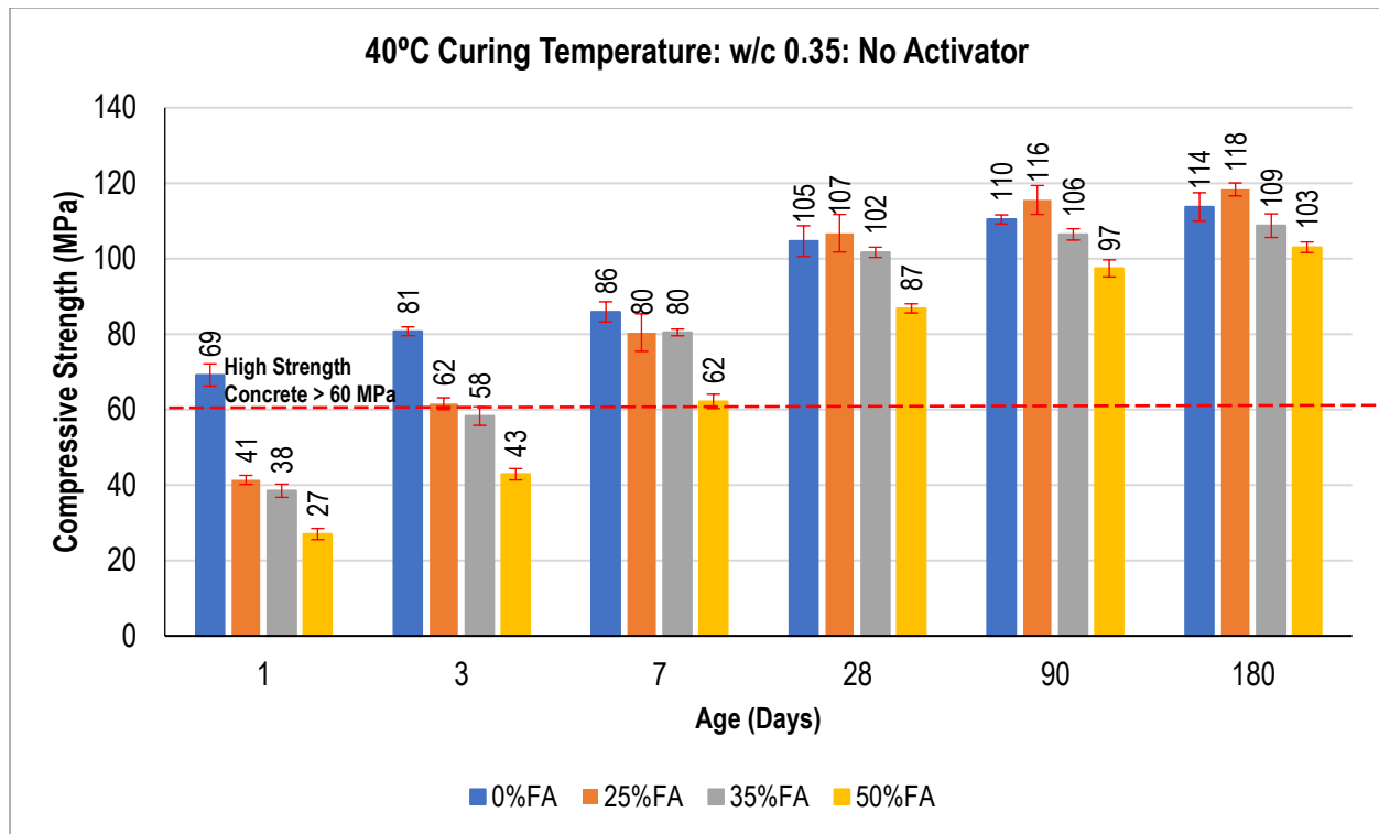
Figure 4.13: Compressive Strength for Concrete Cured at 40°C without Activator (w/c = 0.35)
