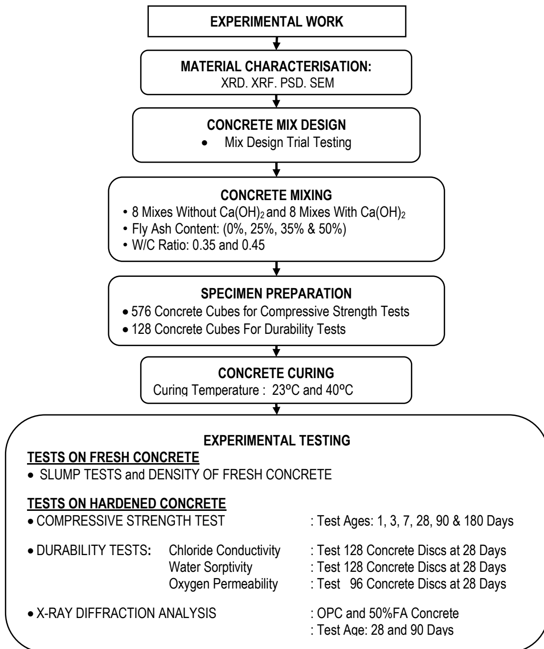
Figure 3.1: Experimental Work Flow Chart
