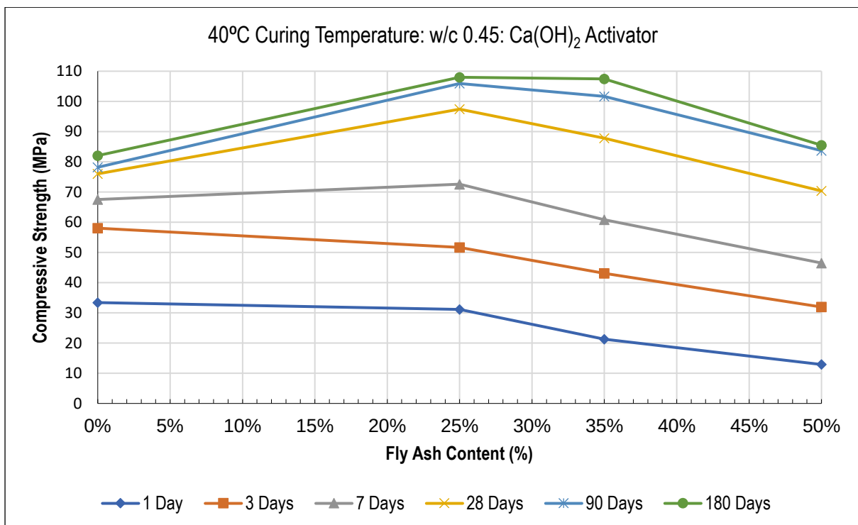
Figure 9.12: Relationship Between Compressive strength and FA Content (40°C: w/c 0.45: Ca(OH) 2 Activator)
