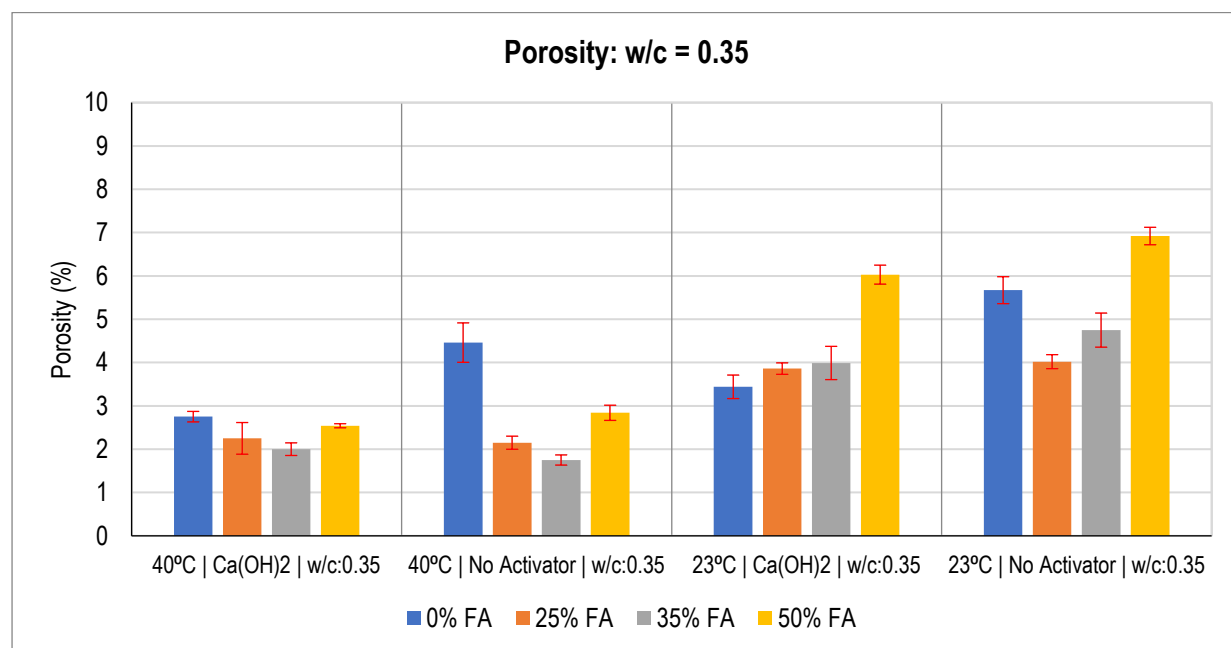
Figure 4.53: Porosity Results for Specimens with w/c of 0.35
