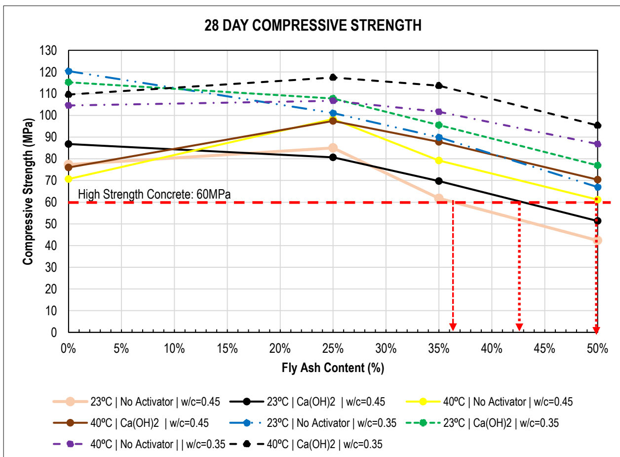
Figure 5.1: Relationship between 28 Day Compressive Strength and Fly Ash Content
