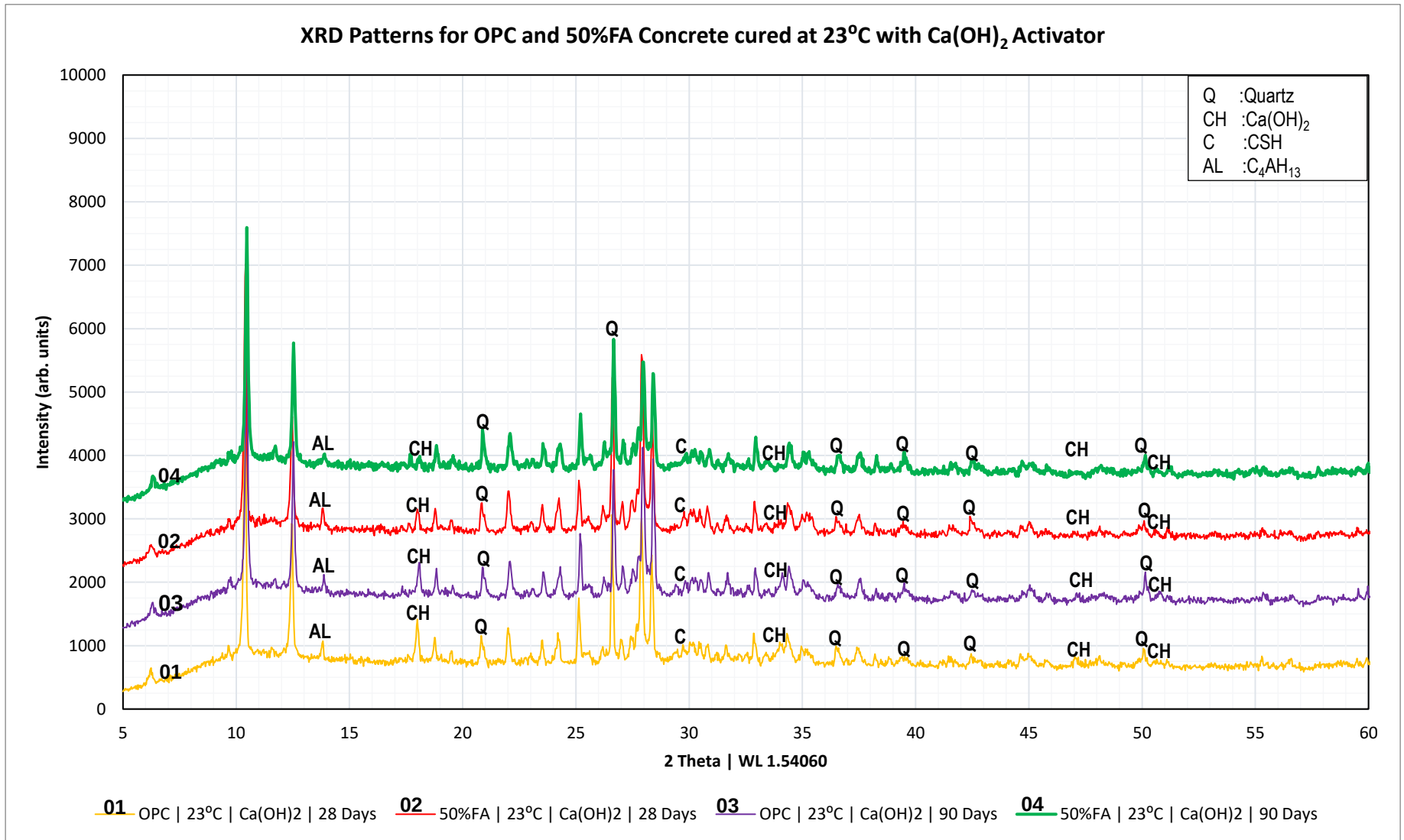
Figure 4.41: XRD Patterns for OPC and 50%FA Concrete cured at 23°C with Ca(OH) 2 Activator
