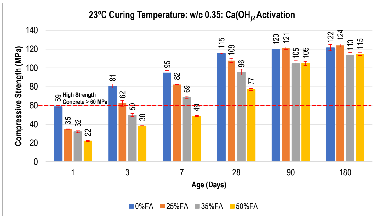
Figure 4.11: Compressive Strength for Concrete Cured at 23°C with Ca(OH) 2 Activation (w/c = 0.35)
