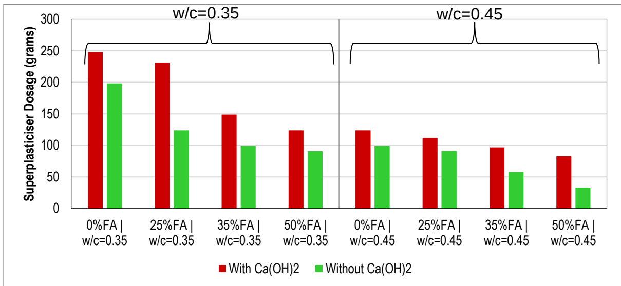
Figure 3.15: Superplasticiser Dosage
