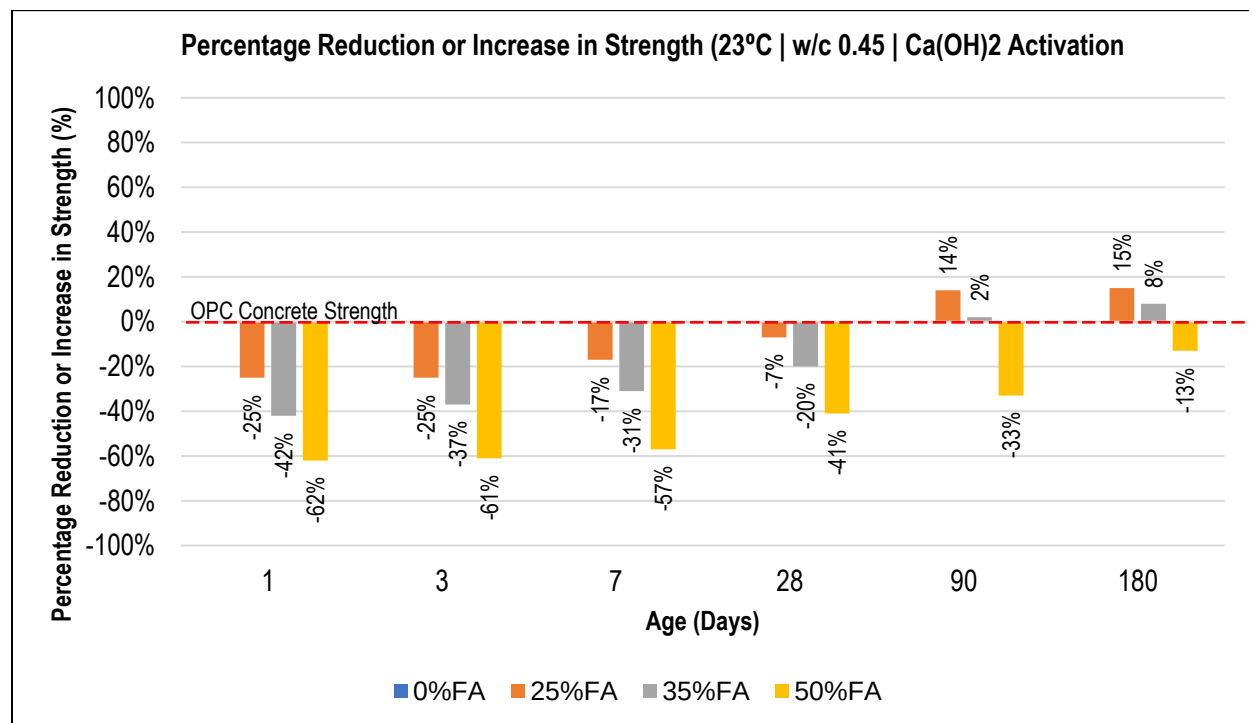
Figure 4.4: Reduction or Increase in Strength as a Percentage of OPC Concrete Strength ( 23^\circ\text{C} : With \text{Ca(OH)}_2 : w/c = 0.45)
