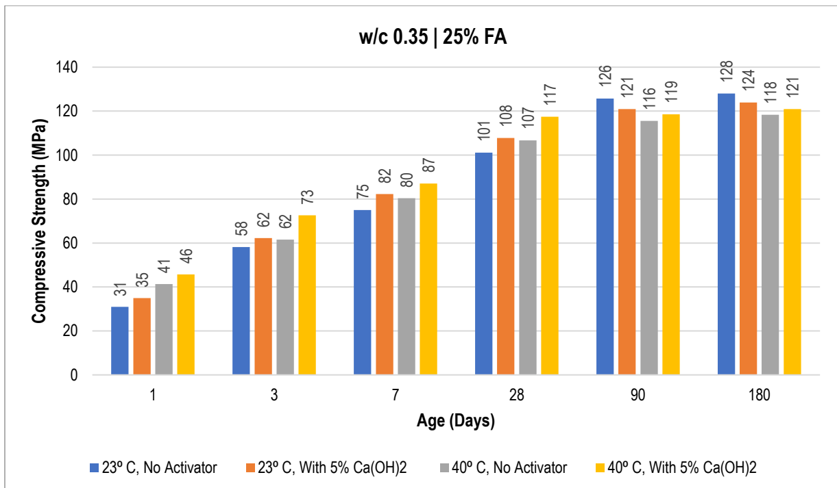
Figure 4.25: Compressive Strength Results for 25%FA Concrete with w/c ratio of 0.35
