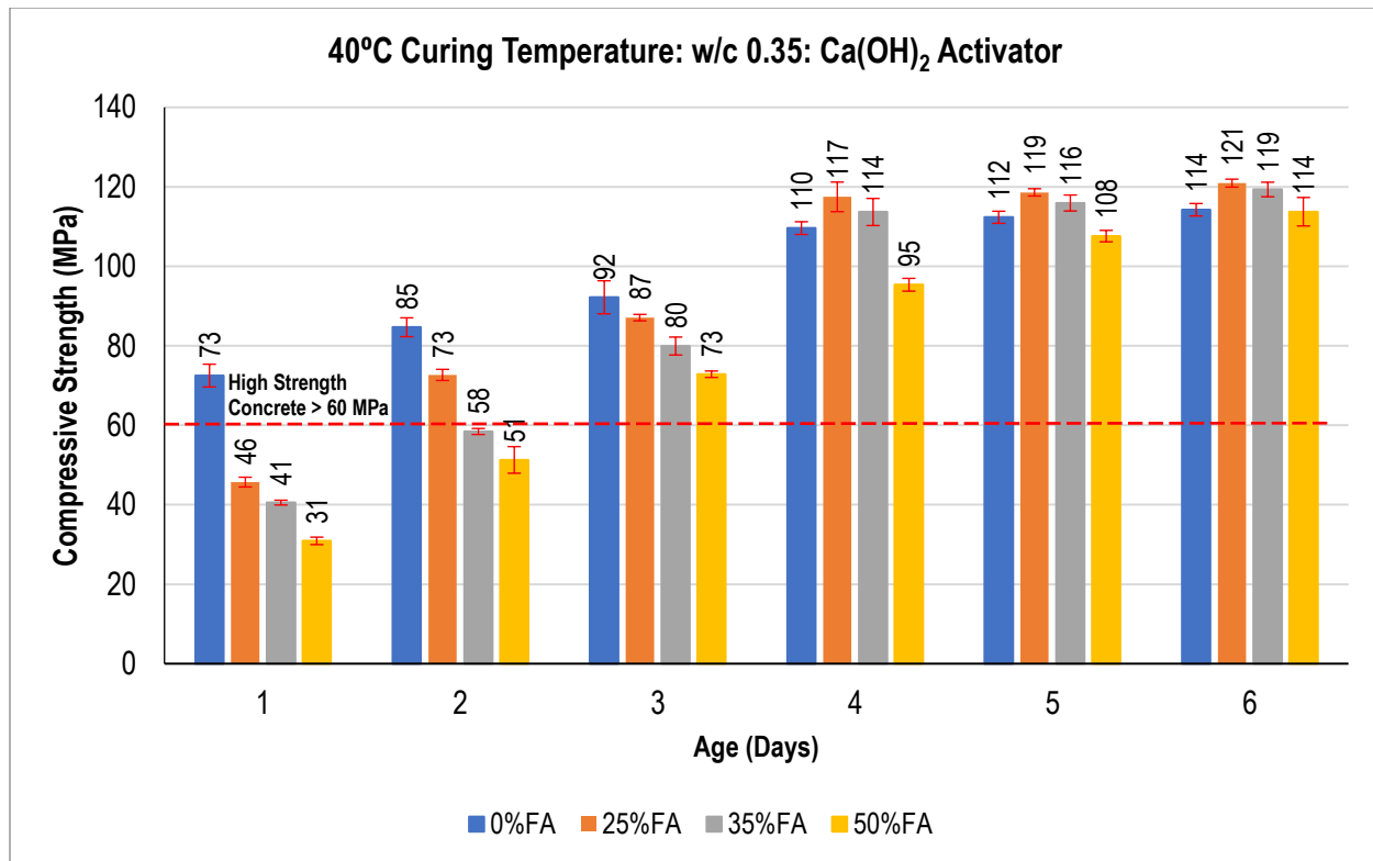
Figure 4.15: Compressive Strength for Concrete Cured at 40°C with Ca(OH) 2 Activator (w/c = 0.35)
