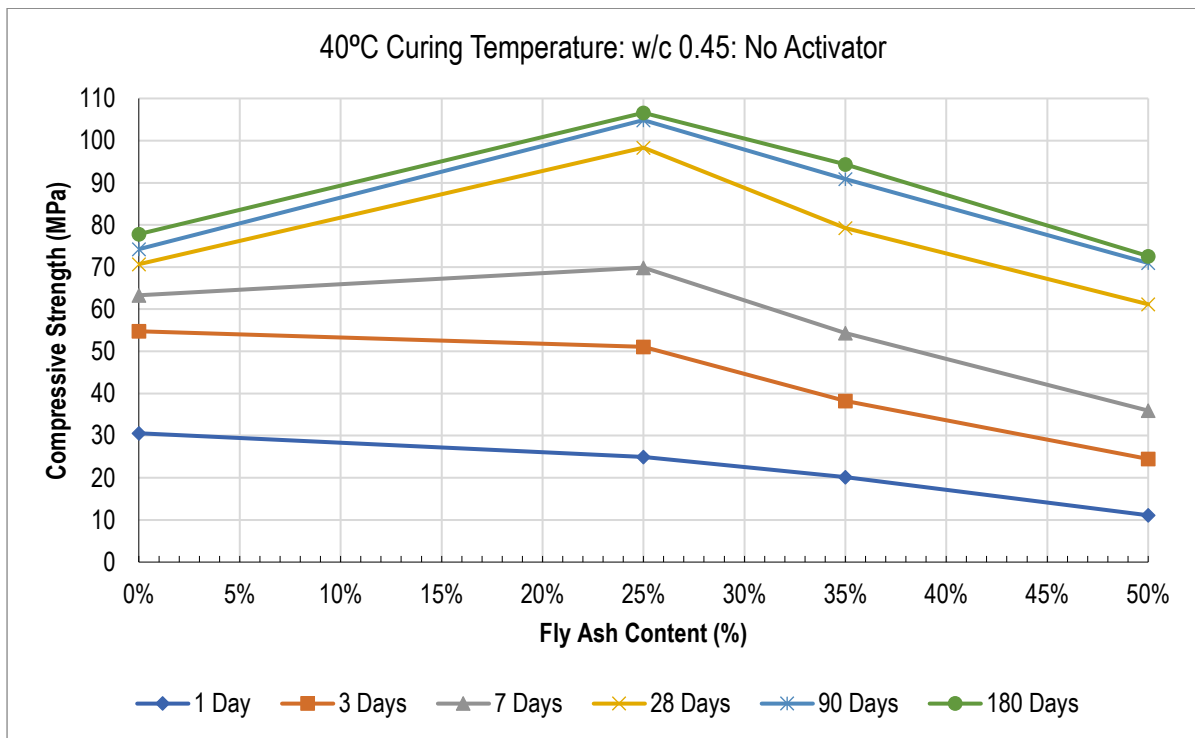
Figure 9.11: Relationship Between Compressive strength and FA Content (40°C: w/c 0.45: No Activator)
