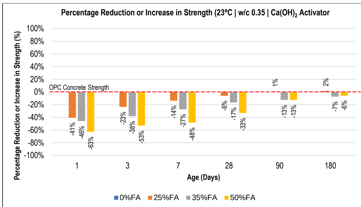
Figure 4.12: Reduction or Increase in Strength as a Percentage of OPC Concrete Strength (23°C : Ca(OH) 2 : w/c= 0.35)
