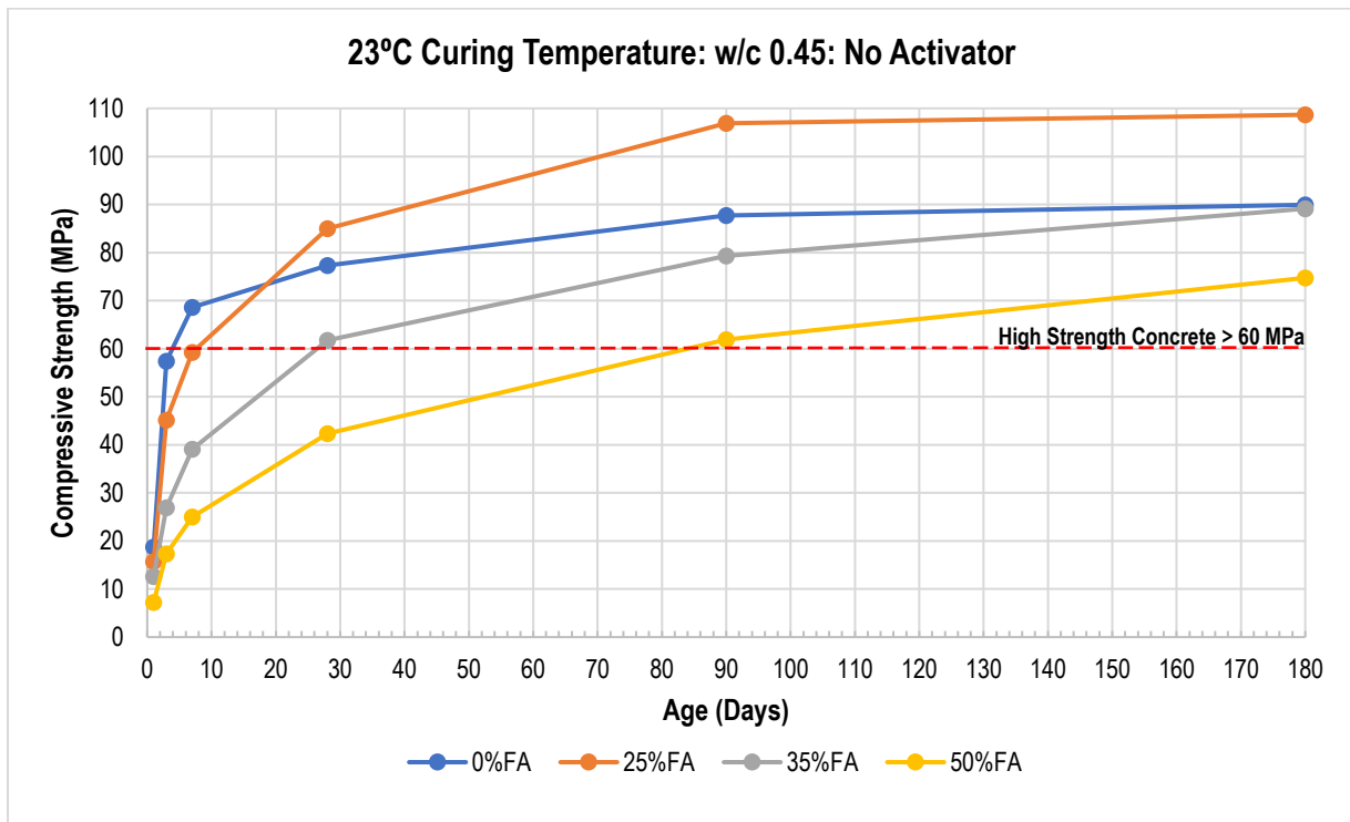
Figure 9.1: Compressive Strength for Concrete Cured at 23°C without \text{Ca}(\text{OH})_2 Activator (w/c = 0.45)
