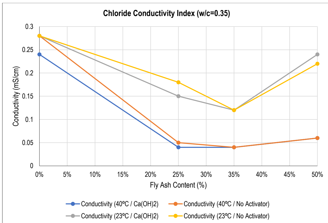
Figure 4.43: Relationship between FA content and Chloride Conductivity Index for Samples with w/c = 0.35
