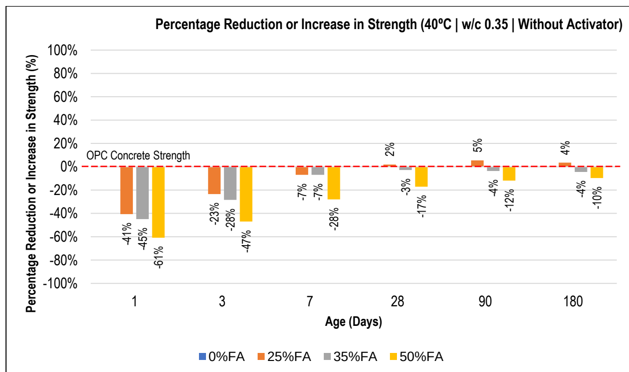
Figure 4.14: Reduction or Increase in Strength as a Percentage of OPC Concrete Strength (40°C : No Activator : w/c = 0.35)
