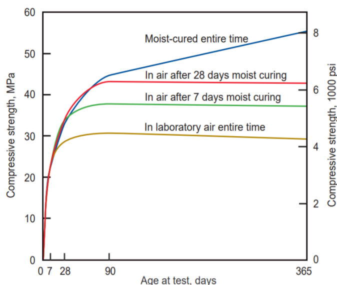
Figure 2.3: Effect of moist curing time on strength gain of concrete (Kosmatka and Wilson, 2011)
