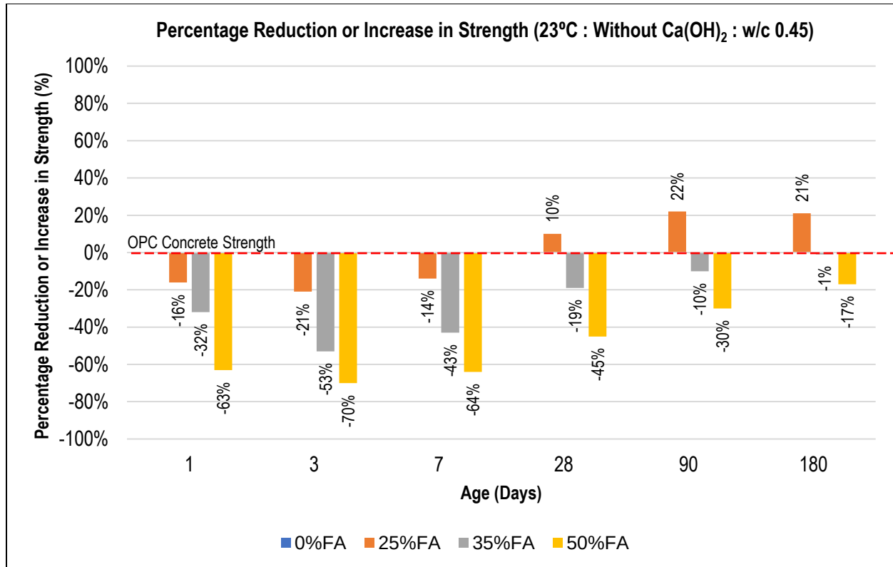
Figure 4.2: Reduction or Increase in Strength as a Percentage of OPC Concrete Strength (23°C : No Activator: w/c = 0.45)
