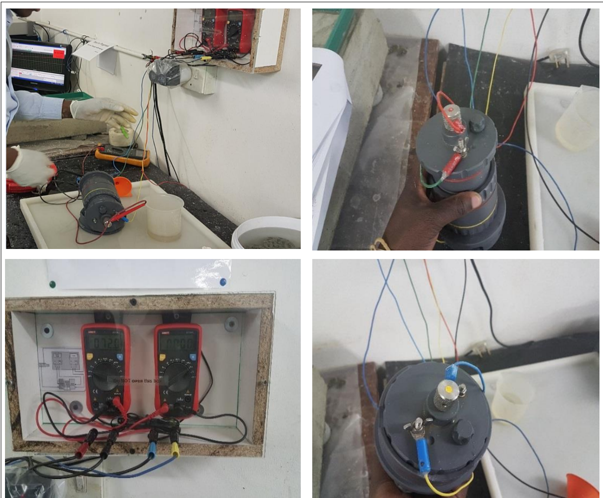
Figure 3.23: Chloride Conductivity Test Apparatus
