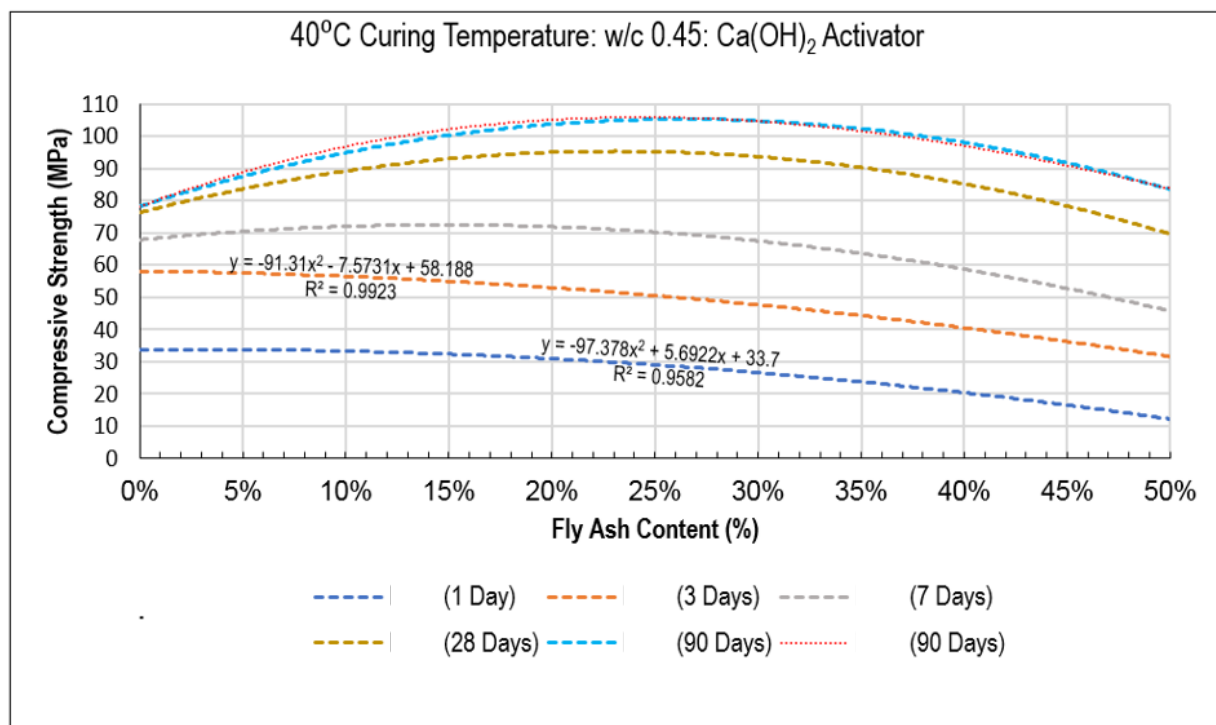
Figure 4.38: Typical Regression Lines for Relationship Between Compressive Strength and FA Content
