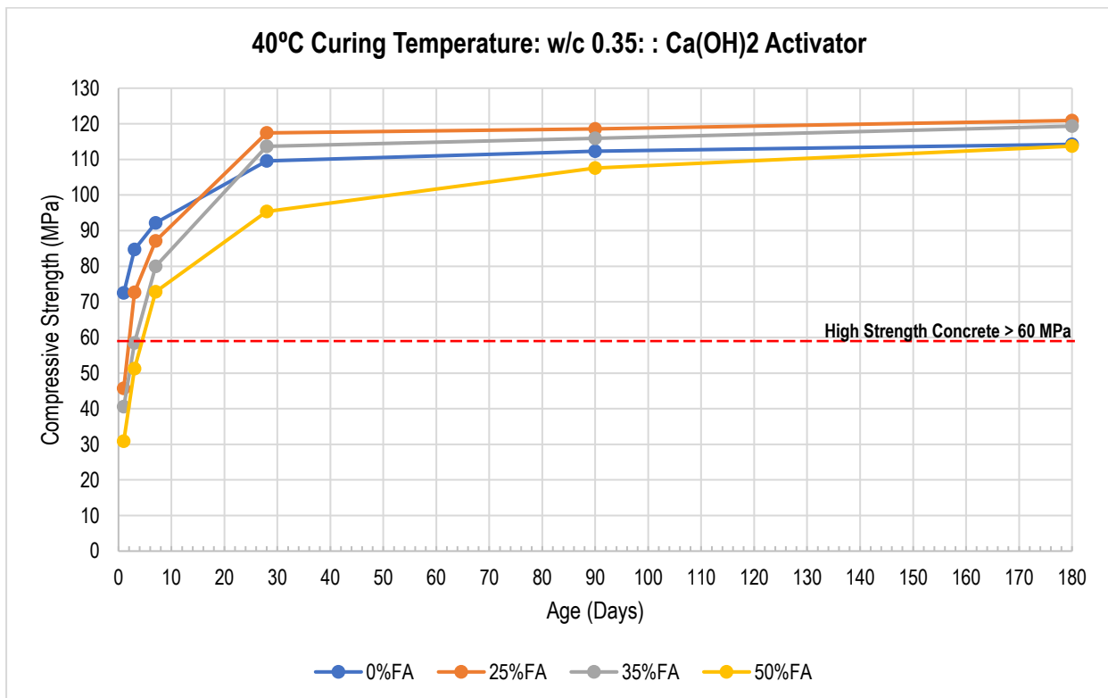
Figure 9.8: Compressive Strength for Concrete Cured at 40°C with Ca(OH) 2 Activator (w/c = 0.35)
