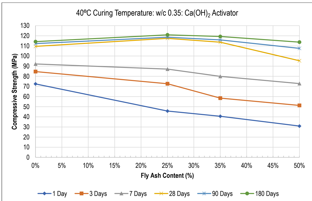
Figure 9.16: Relationship Between Compressive strength and FA Content (40°C: w/c 0.35: Ca(OH) 2 Activator)
