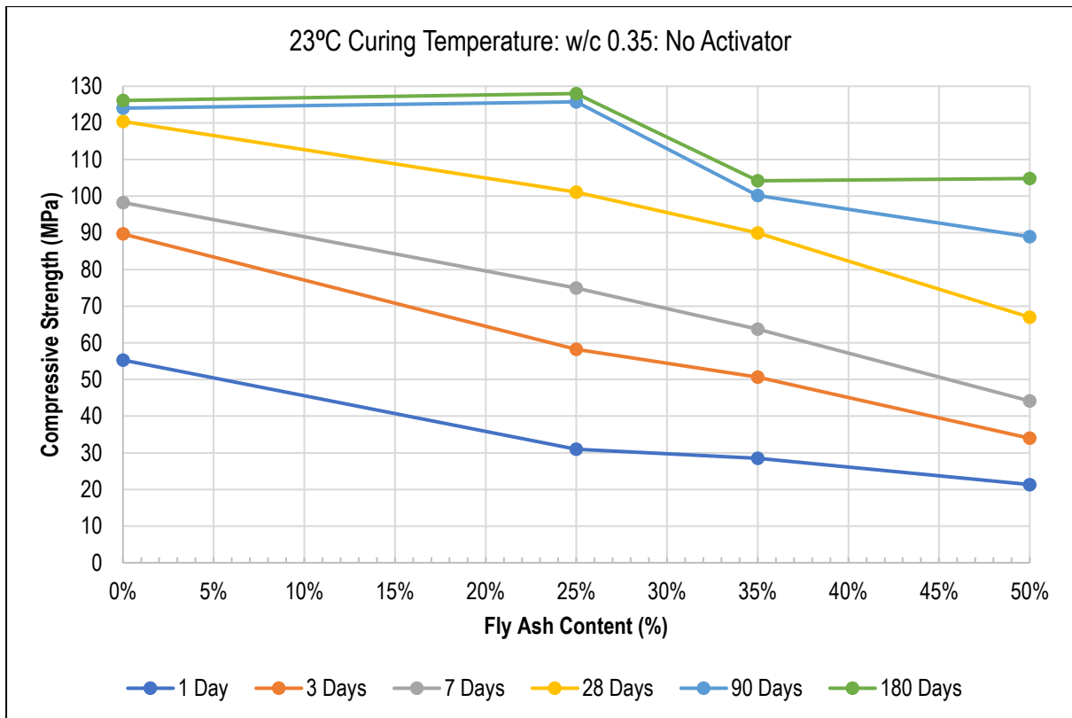
Figure 9.13: Relationship Between Compressive strength and FA Content (23°C: w/c 0.35: No Activator)
