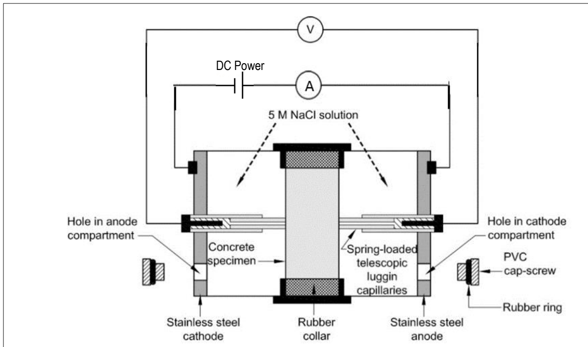
Figure 3.22: Chloride Conductivity Test Circuit Arrangement (SANS 3001-CO3-3:2015)
