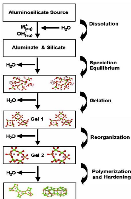
Figure 2.1: Conceptual model for geopolymerization (Duxson et al., 2007)
