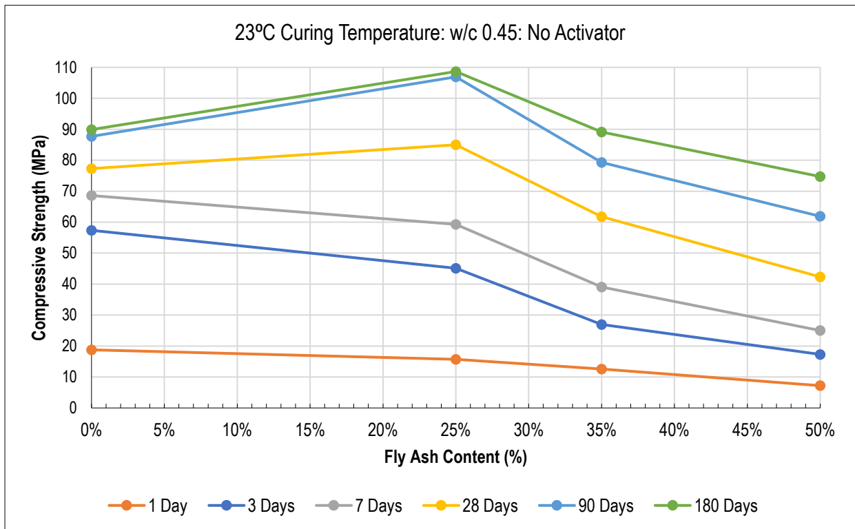
Figure 9.9: Relationship Between Compressive strength and FA Content (23°C: w/c 0.45: No Activator)
