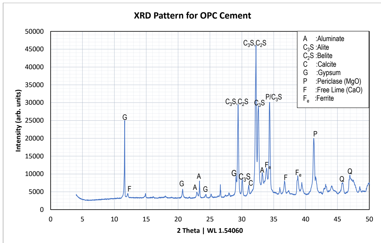
Figure 3.2: XRD Pattern for OPC Cement
