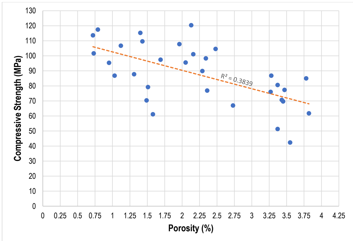
Figure 4.59: Relationship between Compressive Strength and Porosity Determined Using Chloride Conductivity Index Test
