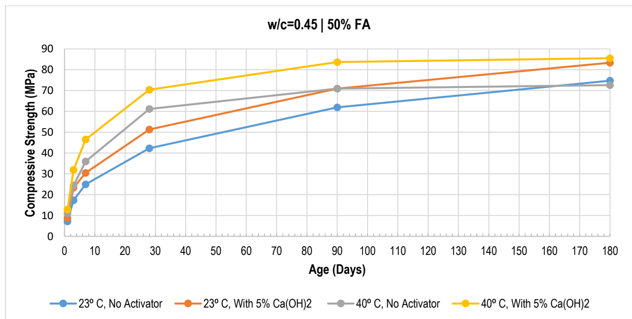
Figure 4.30: Compressive Strength Results for 50%FA Concrete with w/c ratio of 0.45
