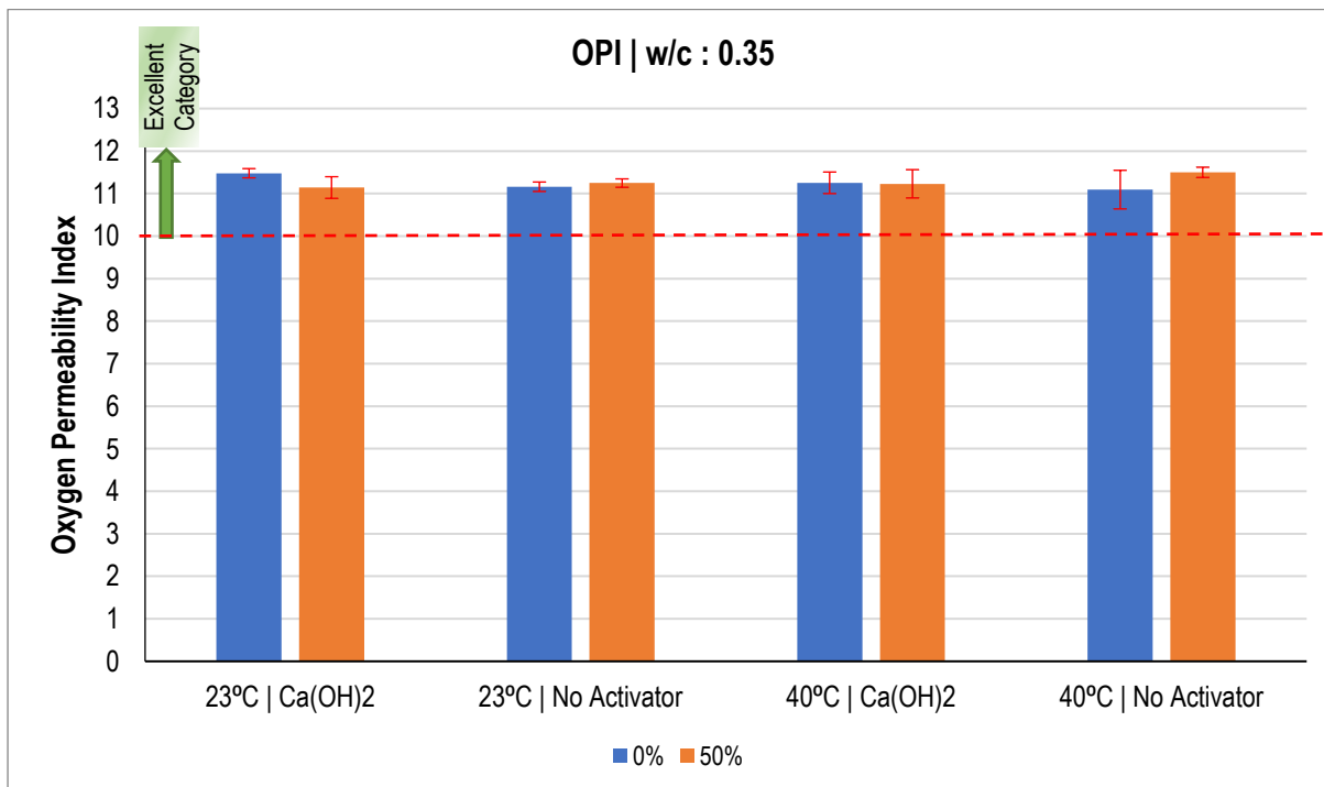
Figure 4.56: Oxygen Permeability Index Results for Specimens with w/c ratio of 0.35
