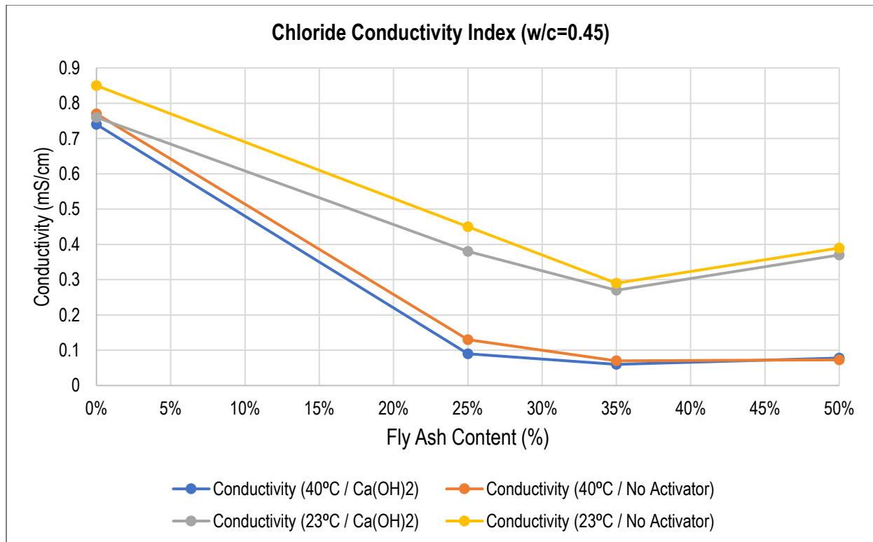
Figure 4.44: Relationship between FA content and Chloride Conductivity Index for Samples with w/c = 0.45
