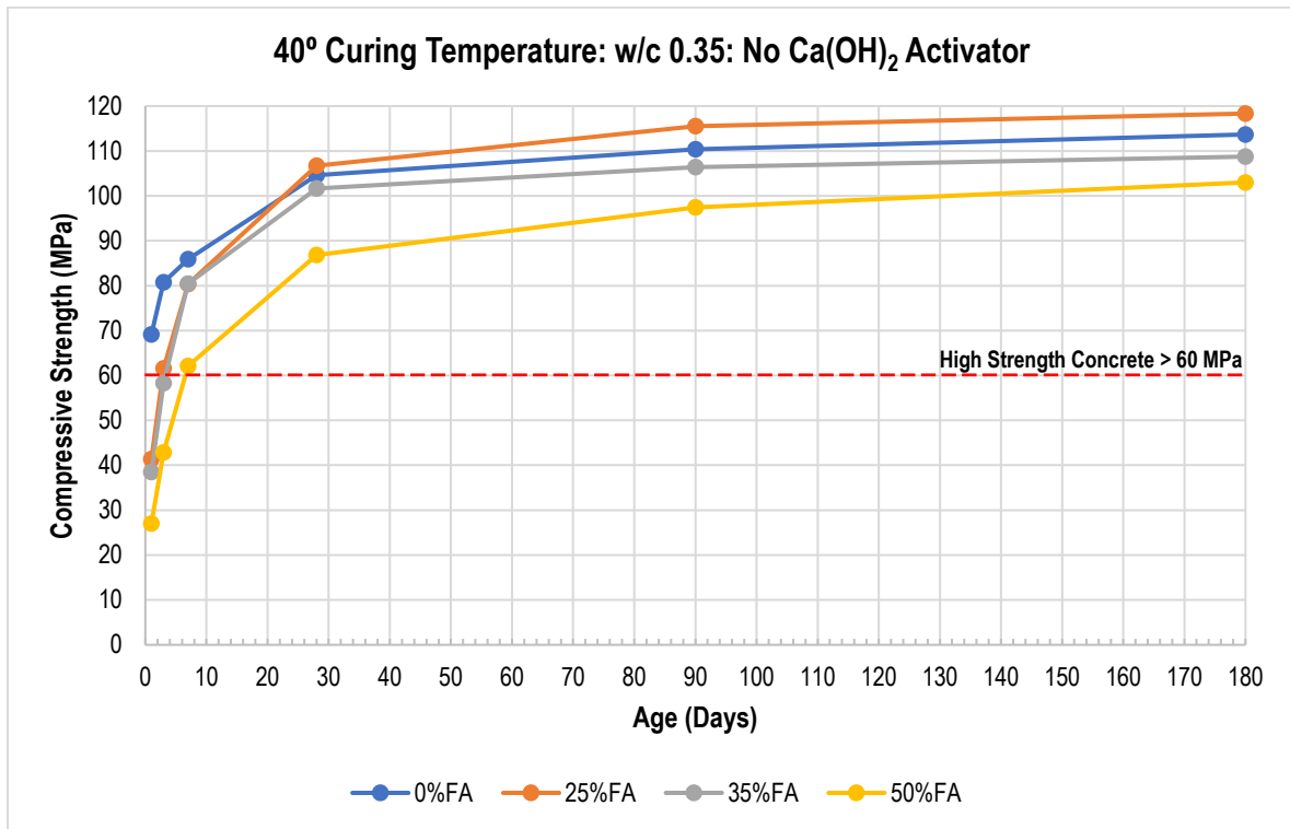
Figure 9.7: Compressive Strength for Concrete Cured at 40°C without Ca(OH) 2 Activator (w/c = 0.35)
