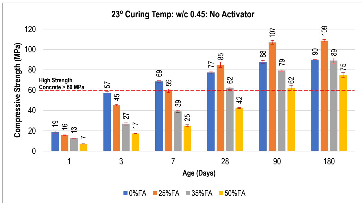
Figure 4.1: Compressive Strength for Concrete Cured at 23°C without Ca(OH) 2 Activator (w/c = 0.45)
