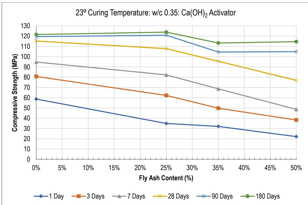
Figure 9.14: Relationship Between Compressive strength and FA Content (23°C: w/c 0.35: Ca(OH) 2 Activator)
