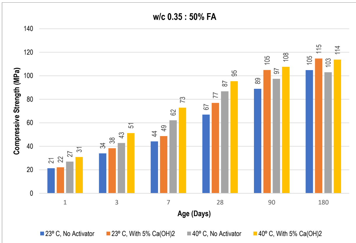
Figure 4.33: Compressive Strength Results for 50%FA Concrete with w/c ratio of 0.35
