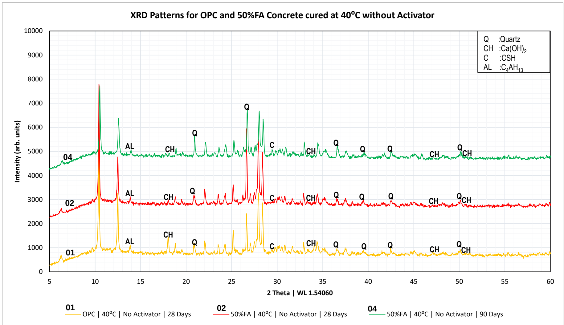
Figure 4.40: XRD Patterns for OPC and 50%FA Concrete cured at 40°C without Activator
