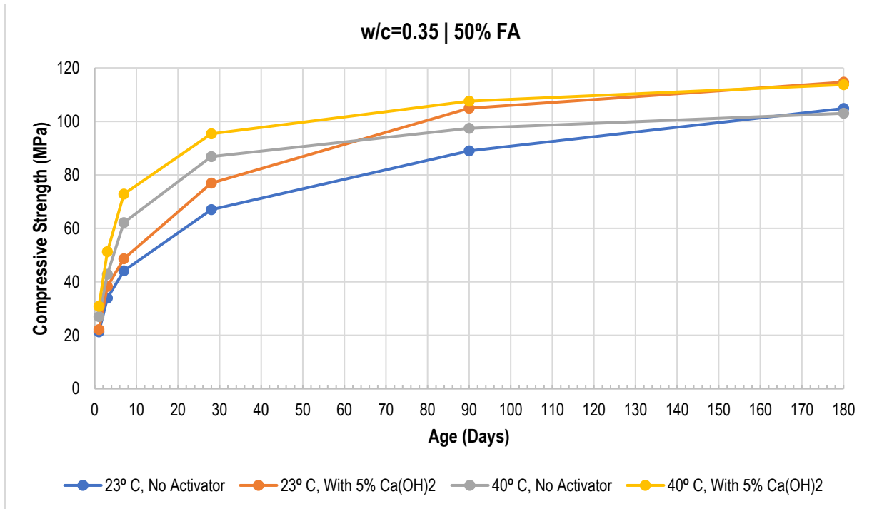
Figure 4.32: Compressive Strength Results for 50%FA Concrete with w/c ratio of 0.35
