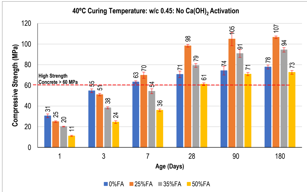
Figure 4.5: Compressive Strength for Concrete Cured at 40°C without Ca(OH) 2 Activator (w/c = 0.45)
