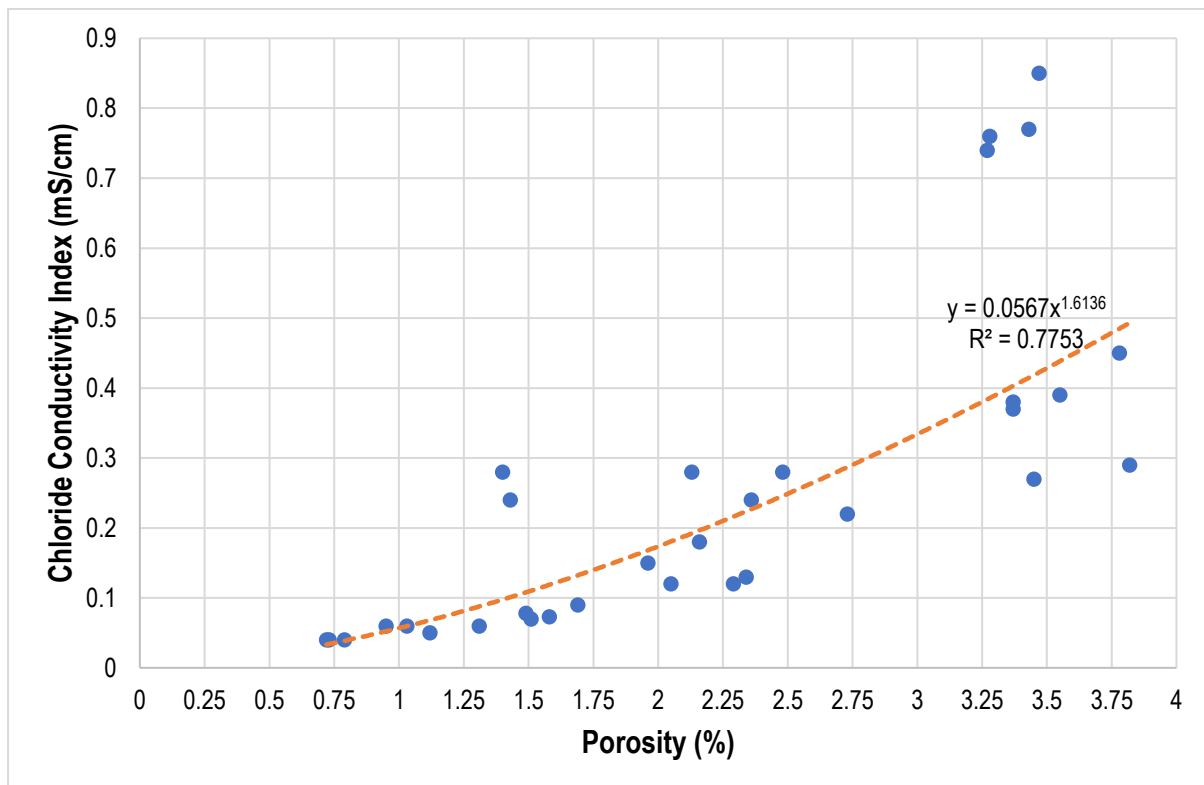
Figure 4.58: Relationship between Chloride Conductivity Index and Porosity Determined Using CCI Test
