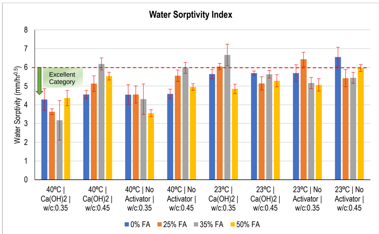
Figure 4.51: Water Sorptivity Index Results for Specimens with w/c of 0.35 and 0.45
