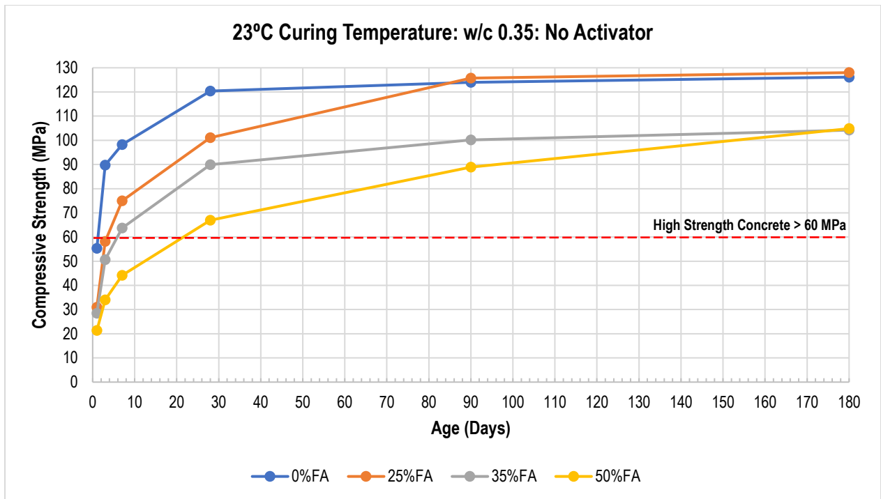
Figure 9.5: Compressive Strength for Concrete Cured at 23°C without \text{Ca(OH)}_2 Activator (w/c = 0.35)
