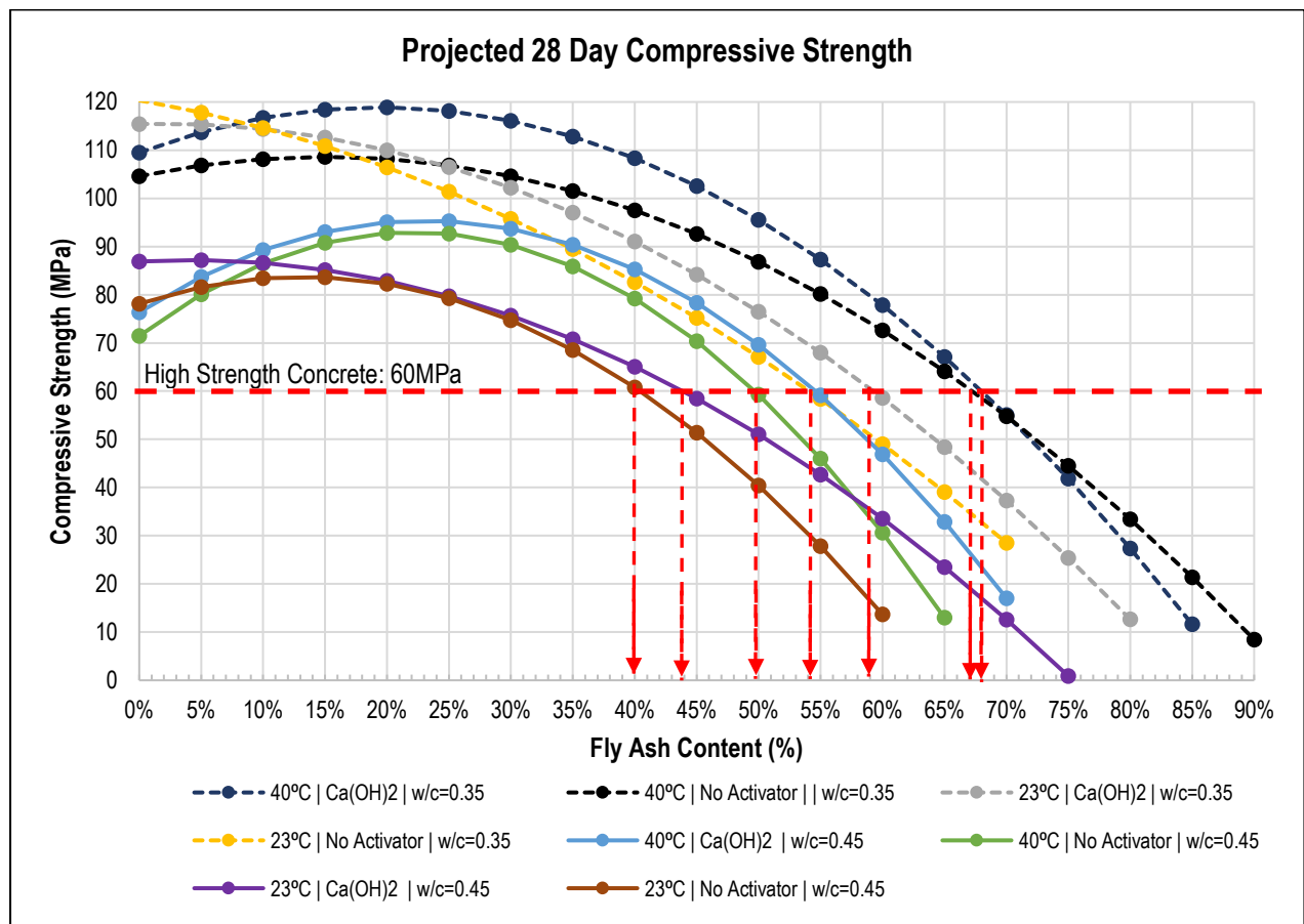
Figure 5.2: Trendlines for the Relationship Between 28 Day Compressive Strength and Fly Ash Content based on Regression Functions Presented in Table 5-1.
