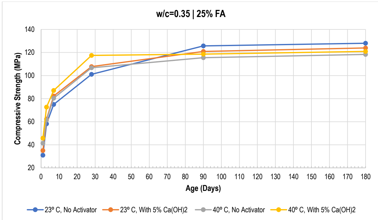
Figure 4.24: Compressive Strength Results for 25%FA Concrete with w/c ratio of 0.35
