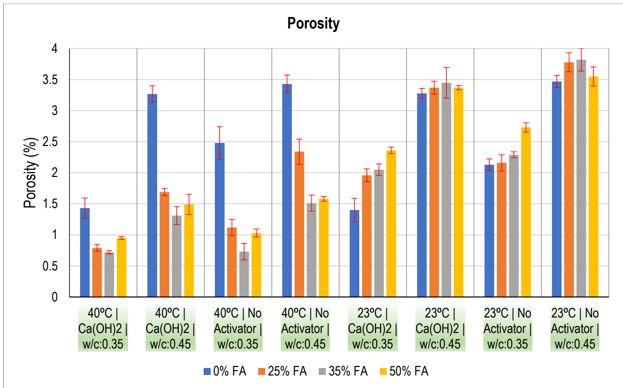
Figure 4.48: Porosity Results for Specimens with w/c of 0.35 and 0.45 based on CCI Test.
