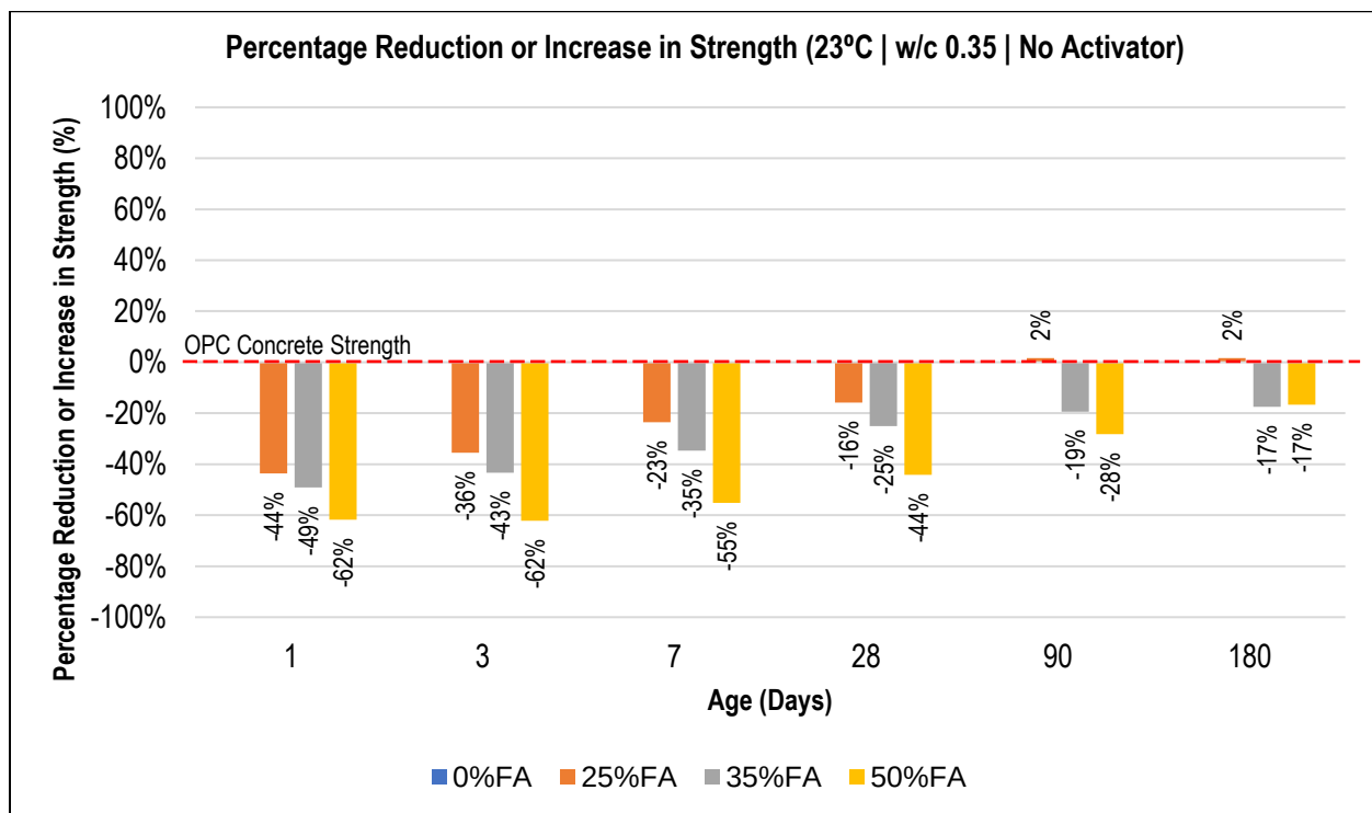
Figure 4.10: Reduction or Increase in Strength as a Percentage of OPC Concrete Strength (23°C : No Activator : w/c = 0.35)
