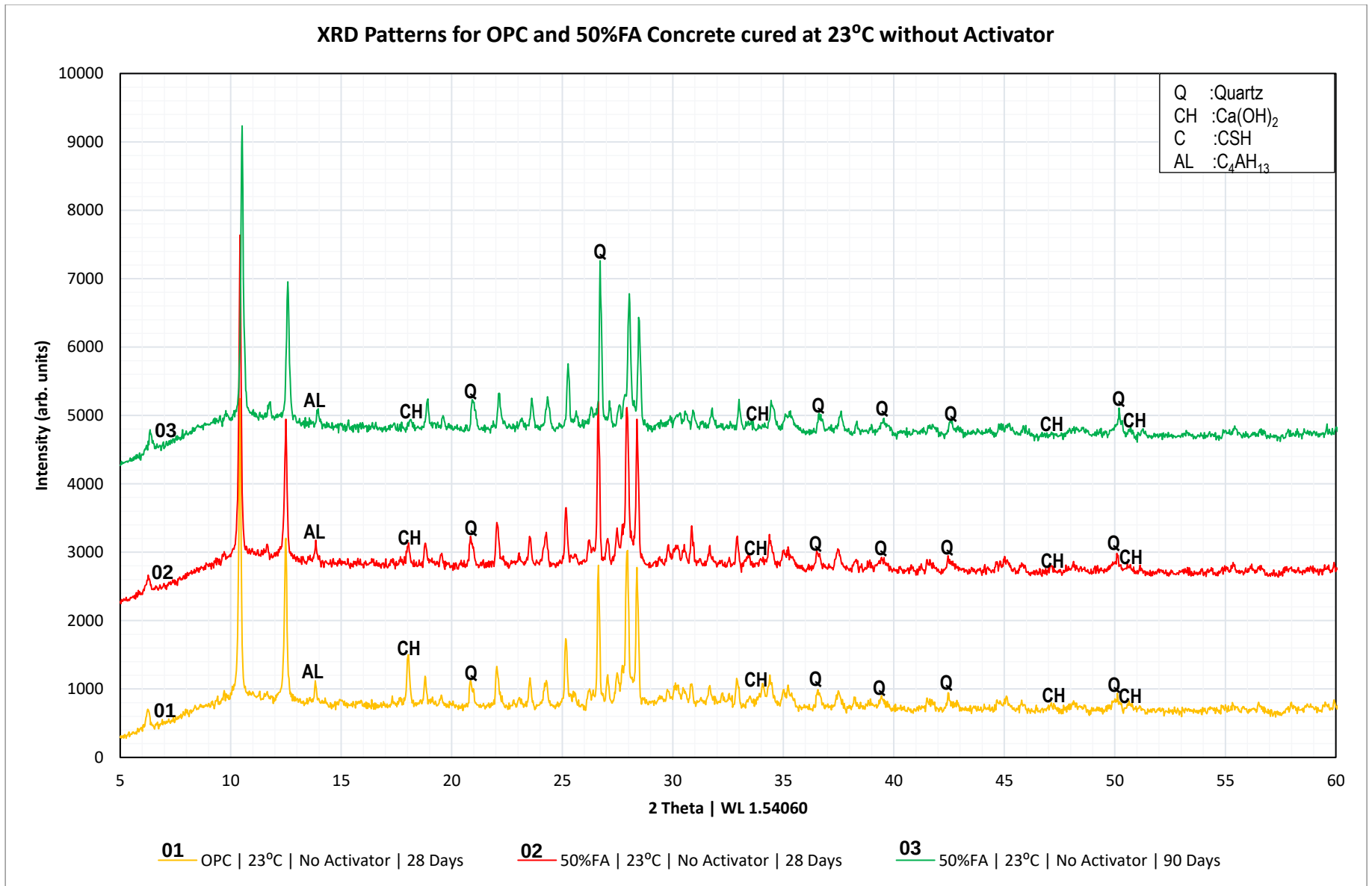
Figure 4.42: XRD Patterns for OPC and 50%FA Concrete cured at 23°C without Activator
