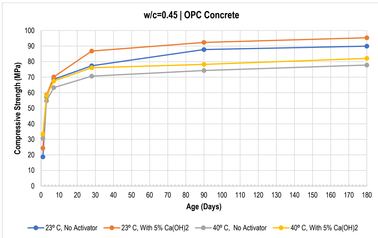
Figure 4.17: Compressive Strength Results of OPC Concrete with w/c ratio of 0.45
