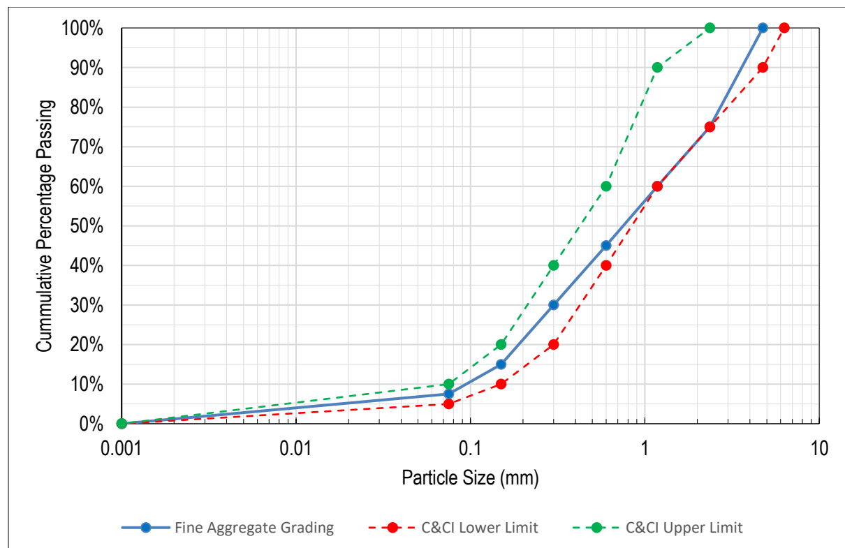
Figure 3.7: Fine Aggregate Particle Size Distribution
