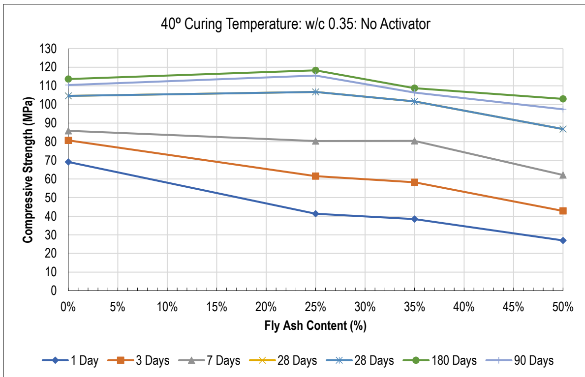
Figure 9.15: Relationship Between Compressive strength and FA Content (40°C: w/c 0.35: No Activator)
