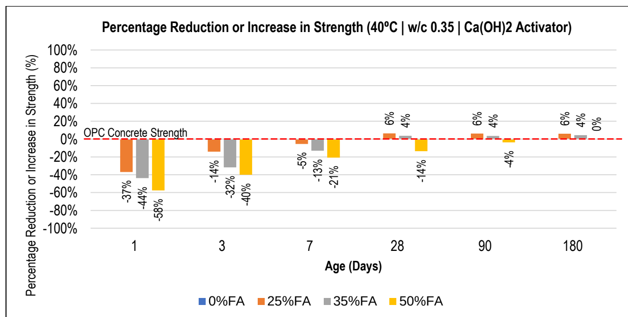
Figure 4.16: Reduction or Increase in Strength as a Percentage of OPC Concrete Strength ( 40^\circ\text{C} : \text{Ca(OH)}_2 : w/c = 0.35)
