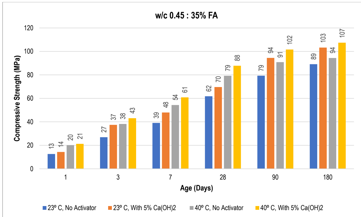
Figure 4.27: Compressive Strength Results for 35% FA Concrete with w/c ratio of 0.45
