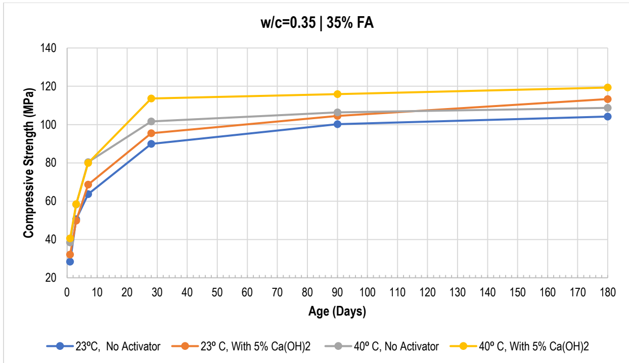
Figure 4.28: Compressive Strength Results for 35%FA Concrete with w/c ratio of 0.35
