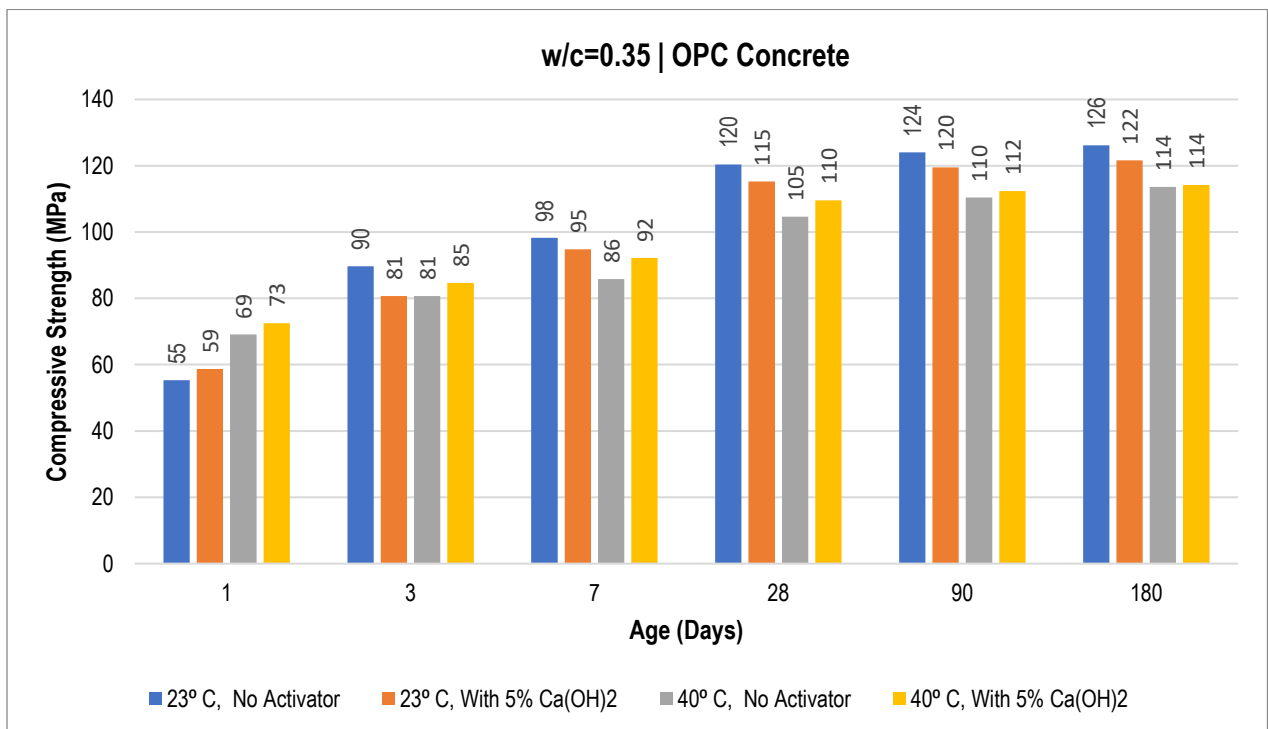
Figure 4.21: Compressive Strength Results for OPC Concrete with w/c of 0.35
