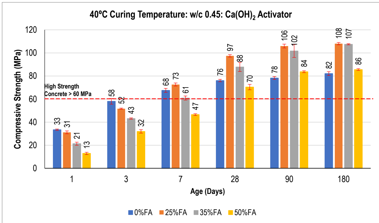
Figure 4.7: Compressive Strength for Concrete Cured at 40°C with Ca(OH) 2 Activator (w/c = 0.45)
