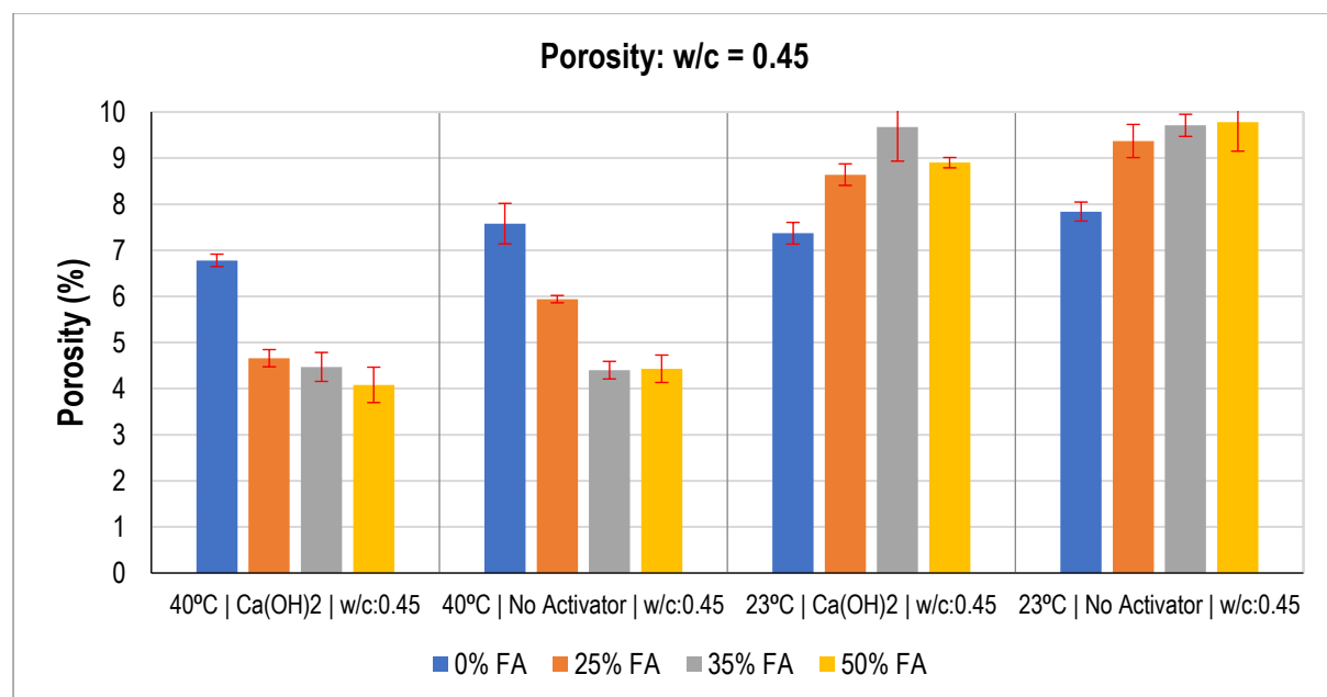
Figure 4.52: Porosity Results for Specimens with w/c of 0.45
