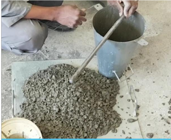
Figure 3.13: Slump for Concrete Mix 1 With Superplasticiser
