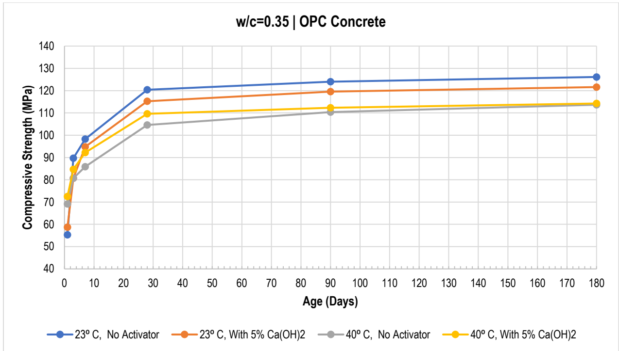
Figure 4.20: Compressive Strength Results for OPC Concrete with w/c ratio of 0.35
