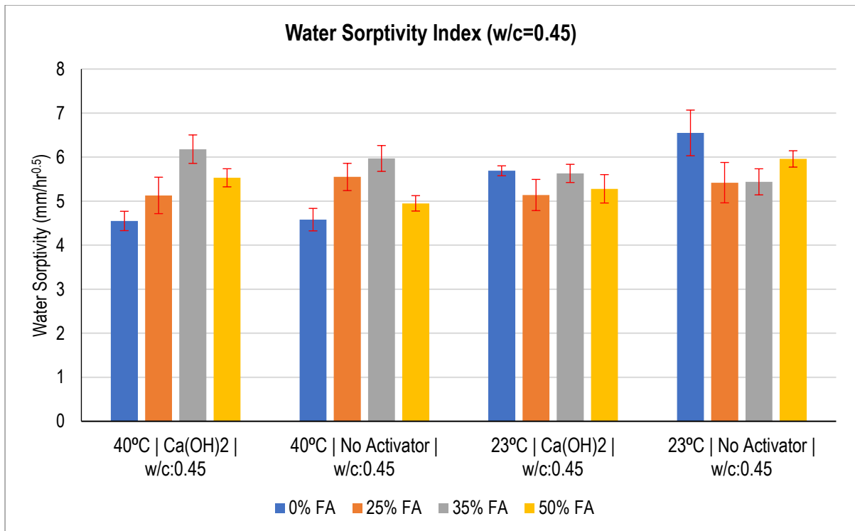
Figure 4.49: Water Sorptivity Index Results for Specimens with w/c of 0.45
