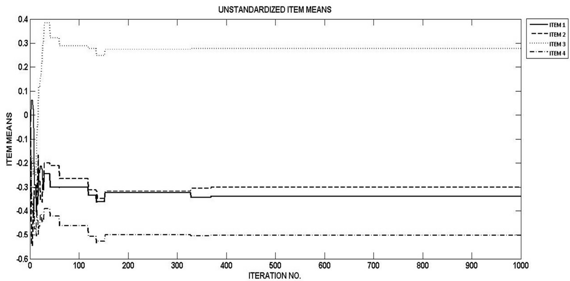
Figure 4.15: Estimates of the item means for Case 1 of table 4.8
