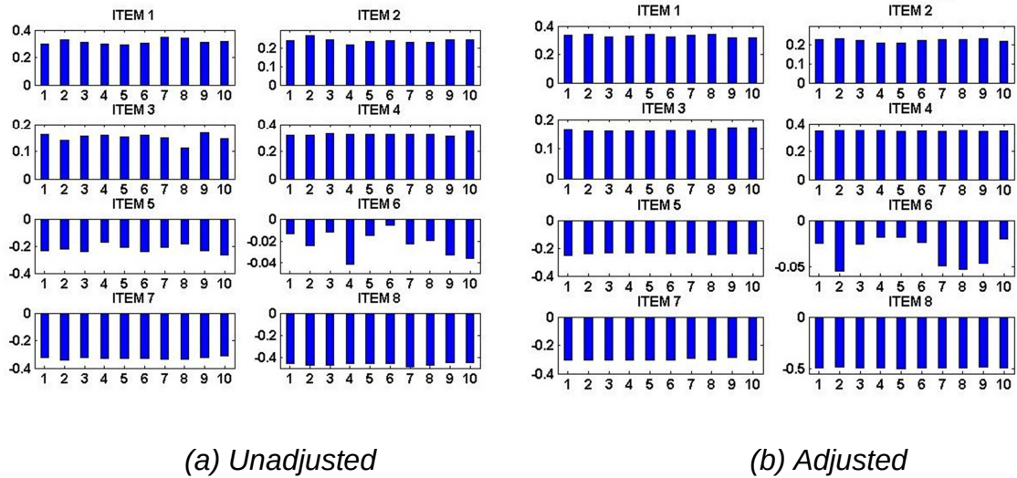
Figure 5.1: Eight item data adjusted for zero entries
