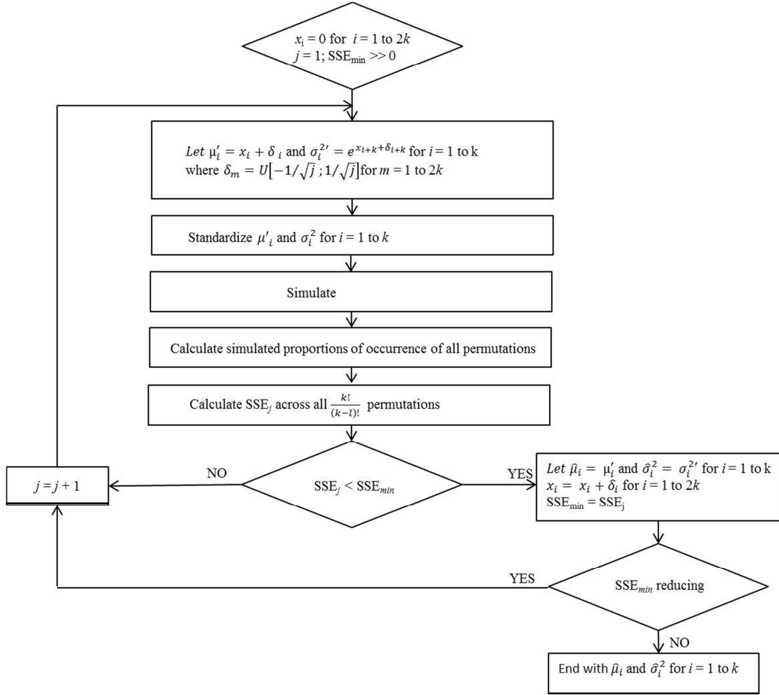
Figure 2.1: Algorithmic flow of the SSPEA
