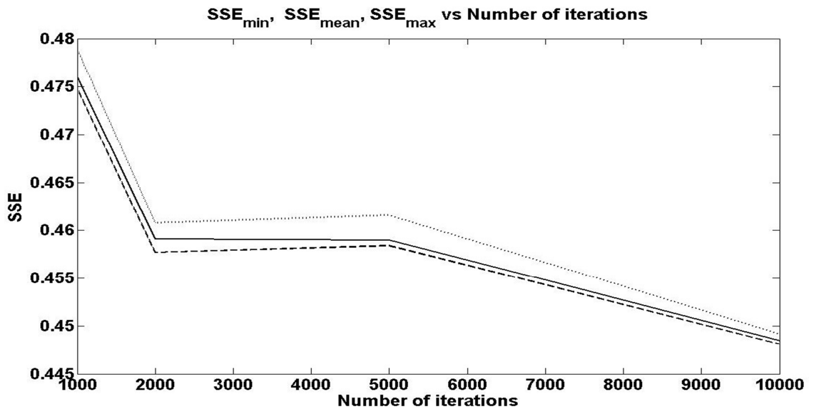
Figure 4.4: SSE plotted against number of iterations
