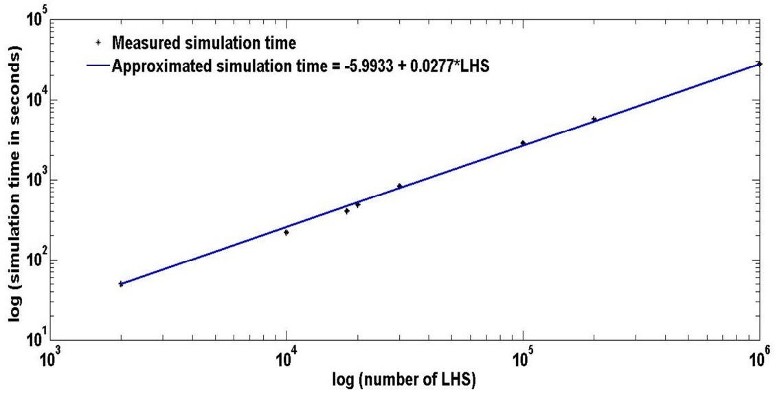
Figure 4.2: log (simulation time) plotted against log (no. of LHS)
