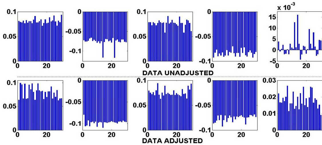
Figure 4.8: Plot of standardized mean of responses for 'unadjusted' and 'adjusted' data
