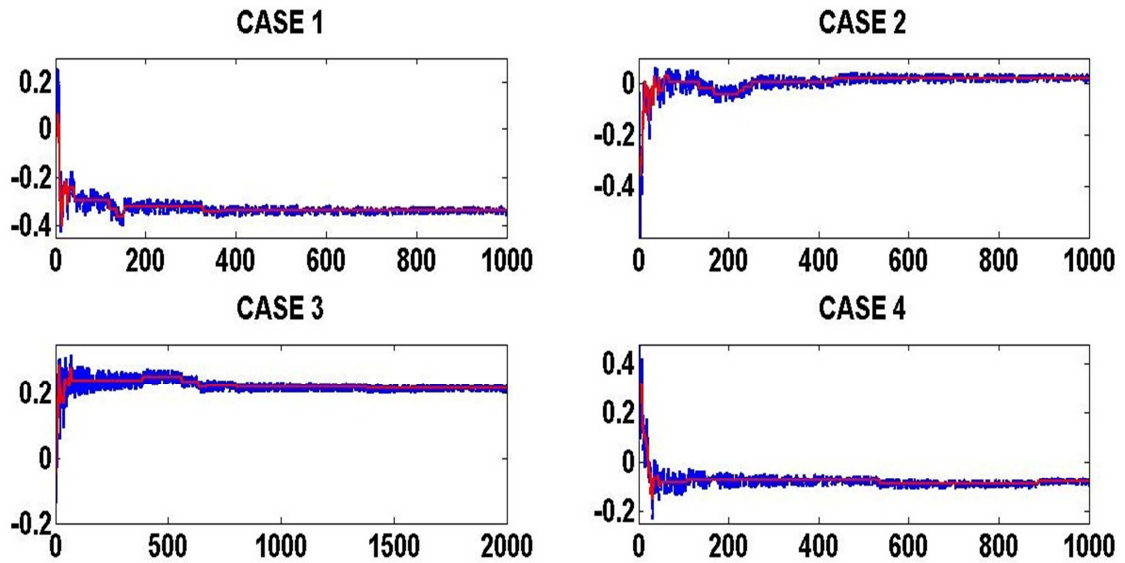
Figure 5.2: Best guesses plotted against all guesses of item 1 for cases in table 4.8
