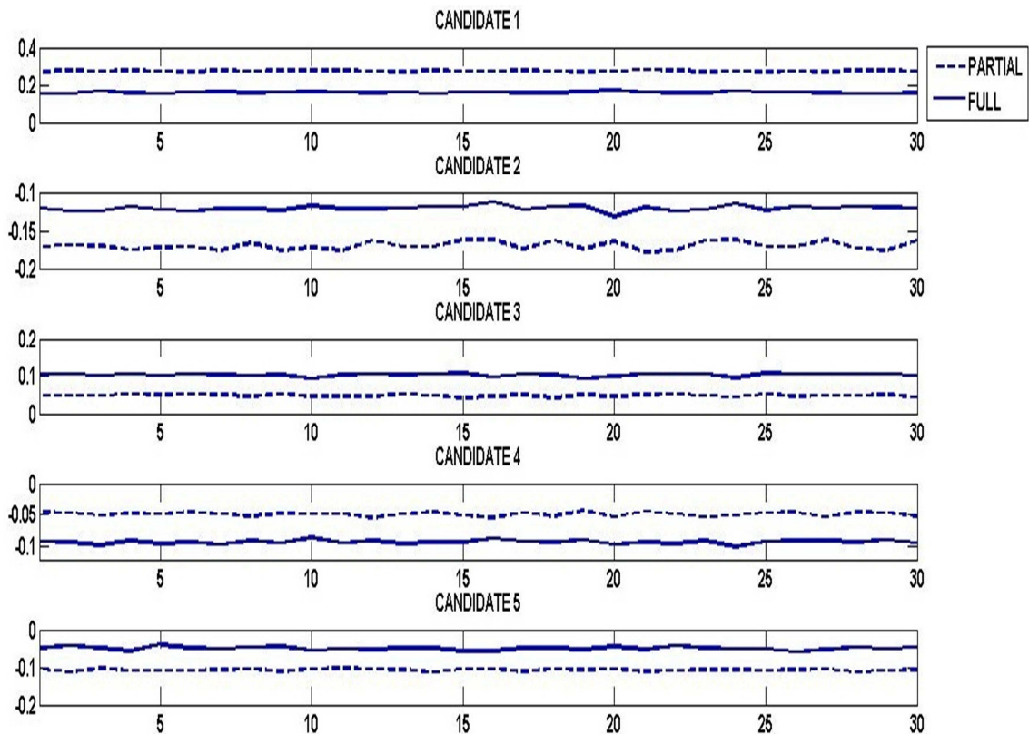
Figure 4.12: Standardized means for a full and partially ranked data set
