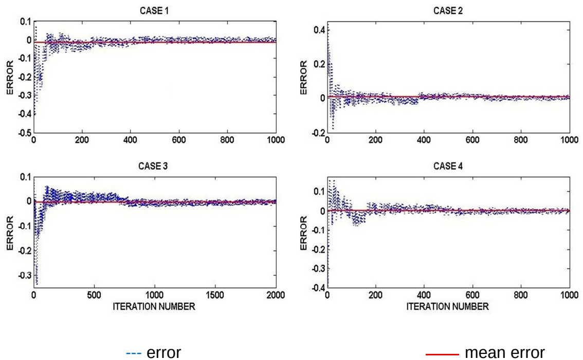
Figure 4.14: Error in mean estimate and mean error
