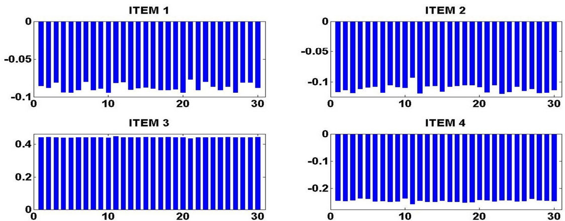
(b) ‘modified’ data
