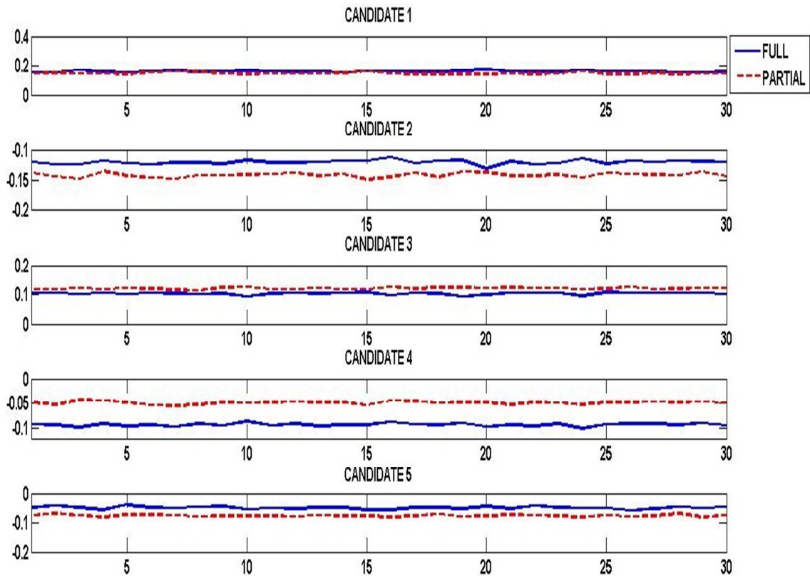
Figure 4.13: Standardized means for a full and modified partially ranked data set
