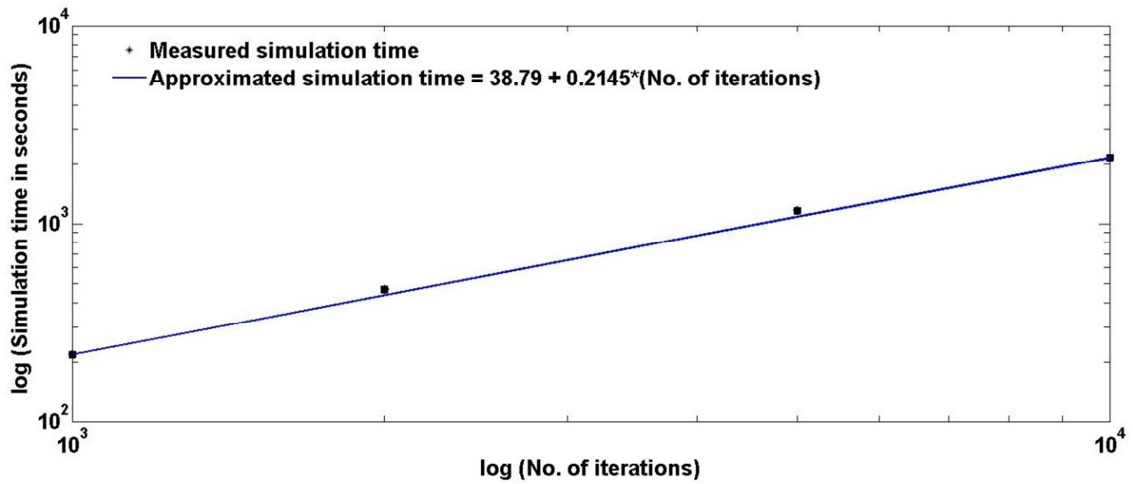
Figure 4.5: log (simulation time) plotted against logarithm no. of iterations
