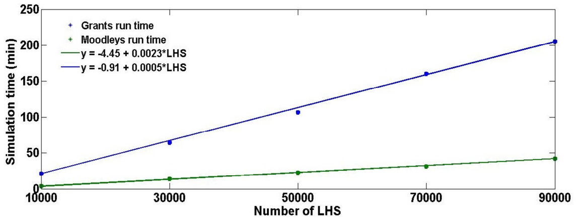
Figure 4.10: Run time vs Number of LHS
