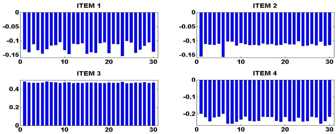
(a) original data
