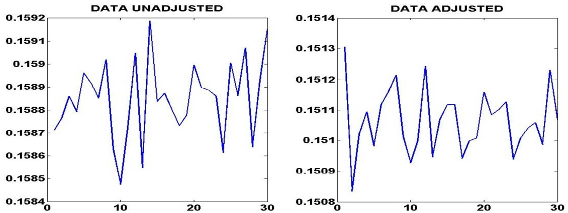
Figure 4.9: Plot of SSE for 'unadjusted' and 'adjusted' data
