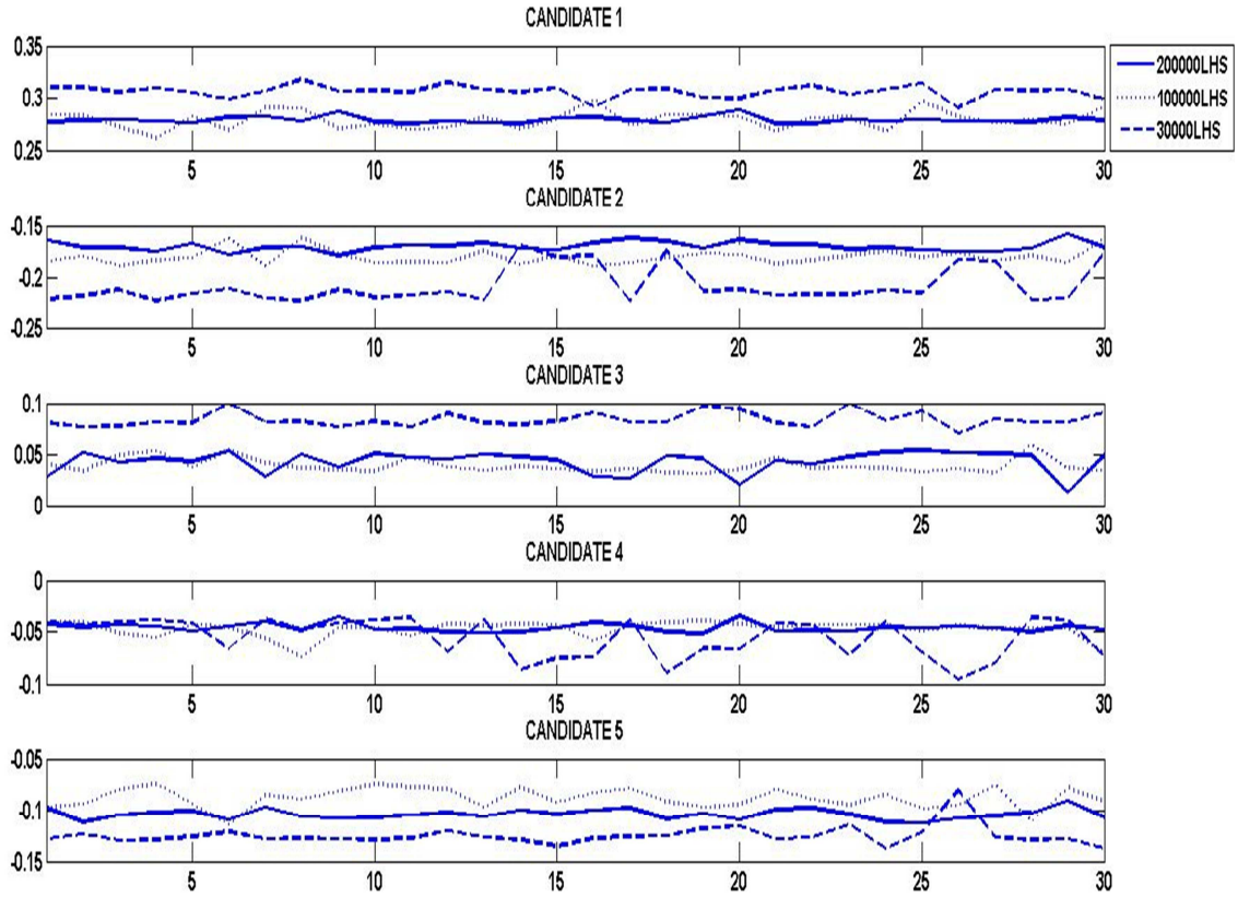
Figure 4.11: Standardized means over the 30 simulation runs
