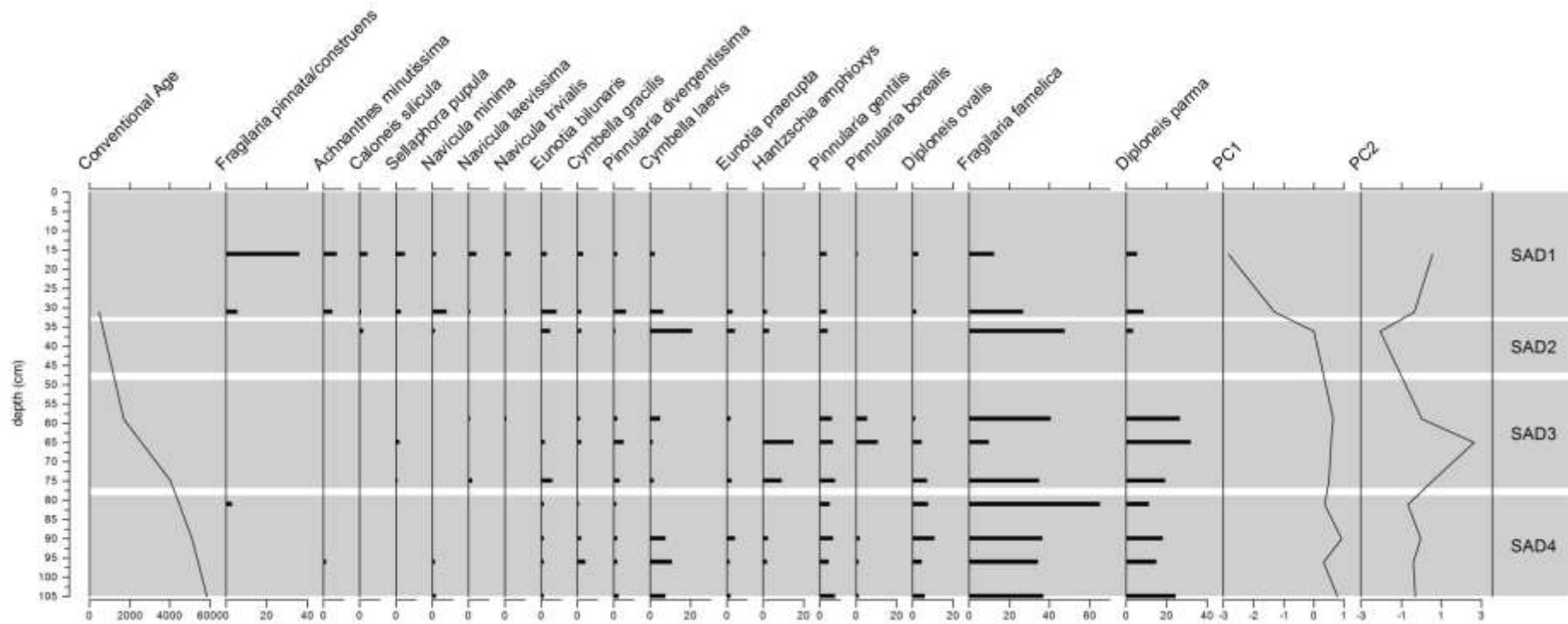
Figure 5.10: Stratigraphic diagram of the relative abundance of diatoms throughout the Sani Valley profile, arranged by PC1 species score, with curves demonstrating PC1 and PC2 sample scores.
