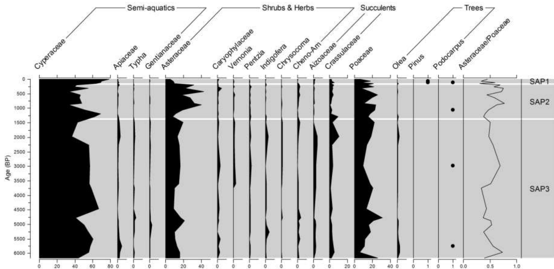
Figure 6.1: Pollen sequence from ~6,000 cal. BP - present at Sani Valley, plotted against age, grouped according to ecology, and zoned according to the CONISS output for pollen. Black circles represent the appearance of 1-5 pollen grains from the particular species.
