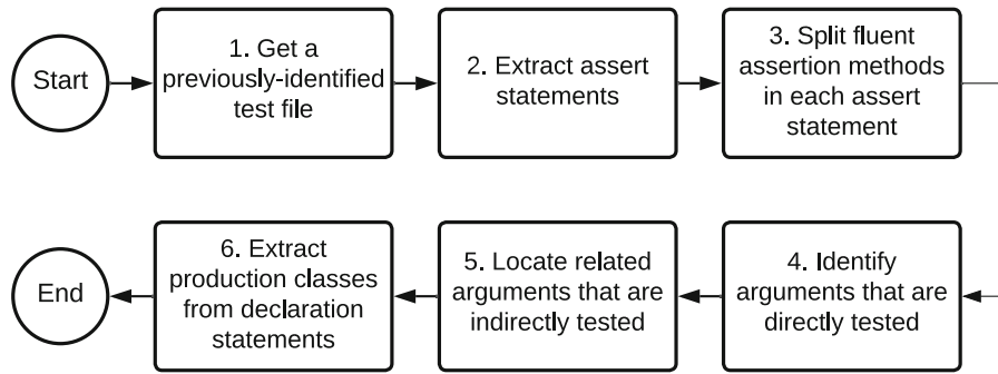
Fig. 2. Flow diagram of the statement-based matching algorithm.
