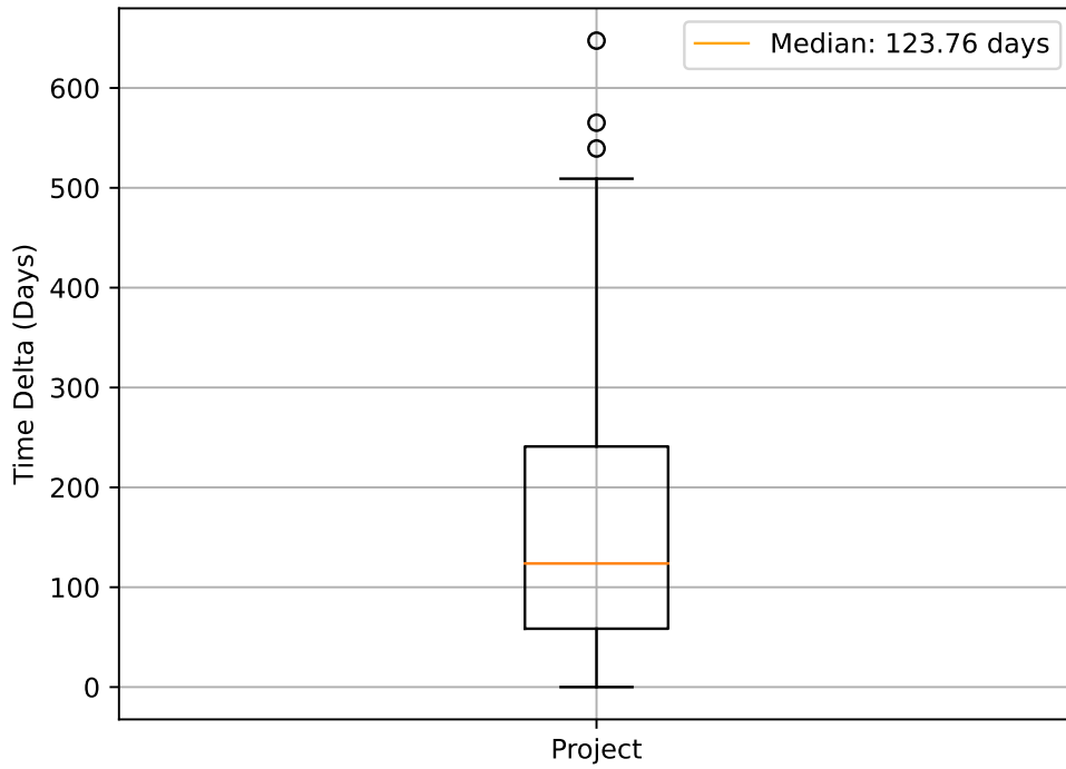
Figure 5.8: The distribution of median time deltas in 100 Java projects
