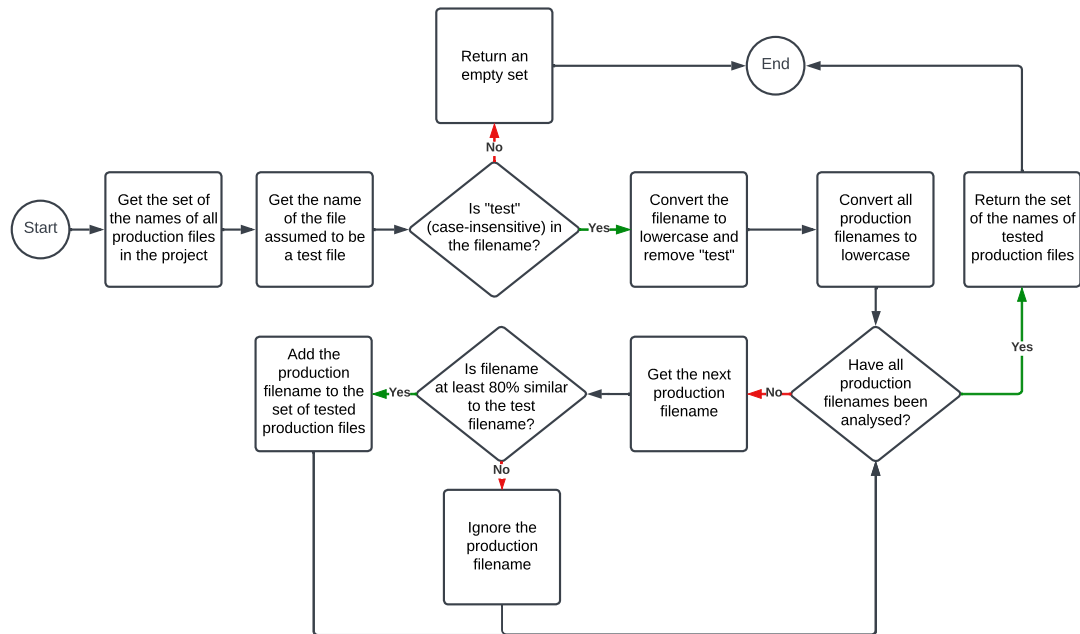
Figure 4.2: Flow diagram of the filename-based matching algorithm.
