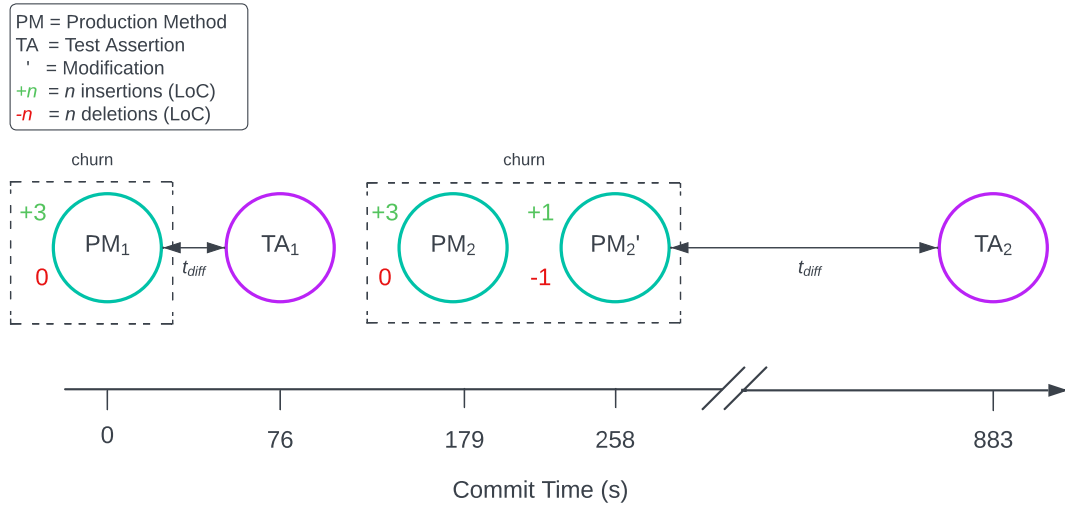
Figure 5.9: A representation of the time deltas and method churn of the Shapes project.
