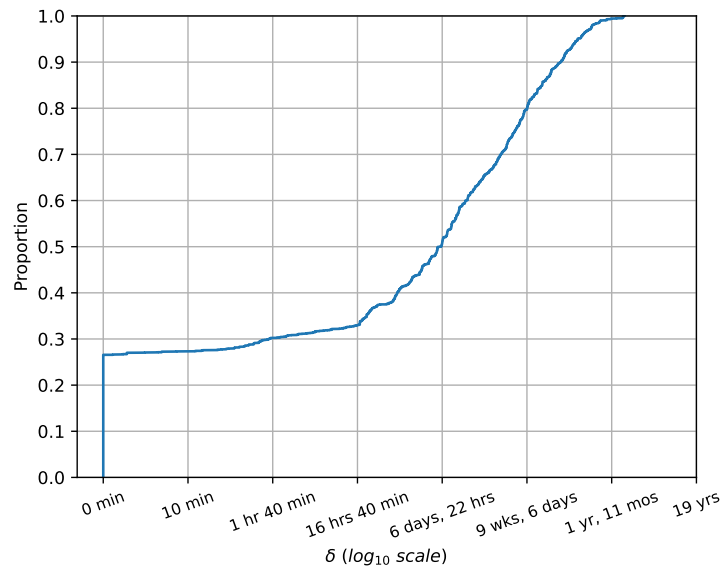
Figure 6.5: A CDF plot of the time deltas between assertions and production methods in SIG-Fasten.
