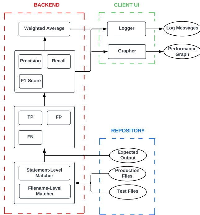
Figure 4.5: Architecture diagram of the performance assessing system.
