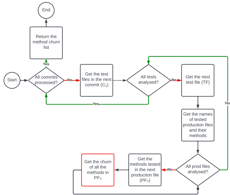
Figure 5.10: Calculating the churn for all the tested production methods of a project.
