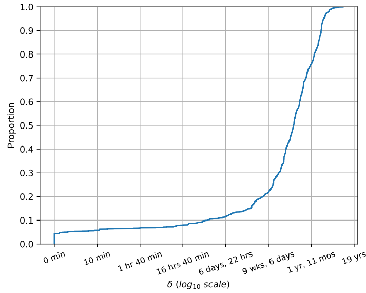
Figure 6.6: A CDF plot of the time deltas between assertions and production methods in ArgoUML.
