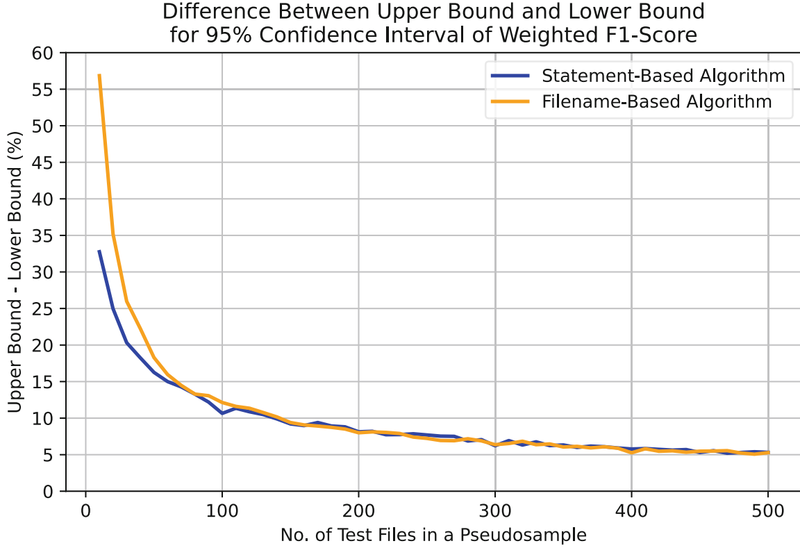
Fig. 4. Difference between the upper bound and lower bound for the 95% confidence interval of the weighted F1-score for the matching algorithms
