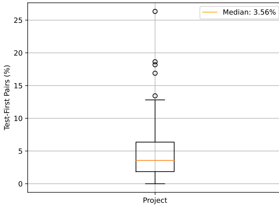
Figure 5.7: The distribution of the percentage of test-first pairs in 100 Java projects.
