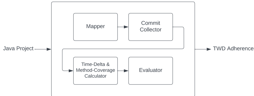
Figure 5.1: The core components of the TWD adherence evaluation system.
