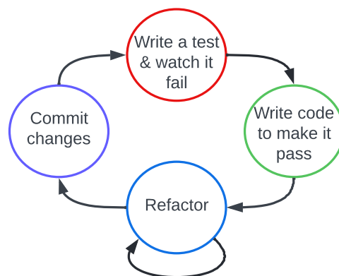
Figure 2.1: A flow diagram of the basic steps of TDD.
