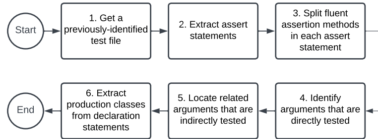
Figure 4.3: Flow diagram of the statement-based matching algorithm.
