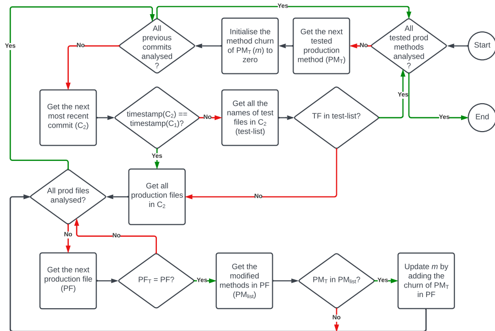
Figure 5.11: Getting the churn for a single production file's tested methods.
