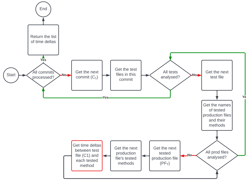
Figure 5.5: Calculating time deltas between all modified tests and each method they test.
