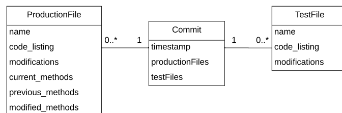
Figure 5.3: A UML diagram of the commit and file data structure.
