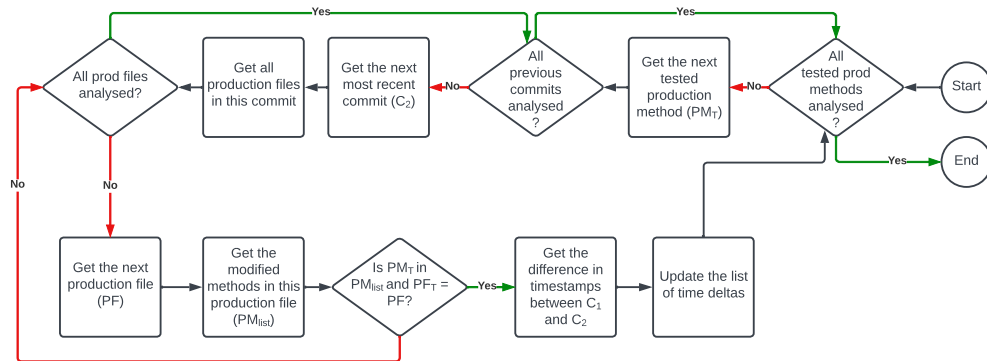
Figure 5.5: Calculating time deltas between all modified tests and each method they test.
