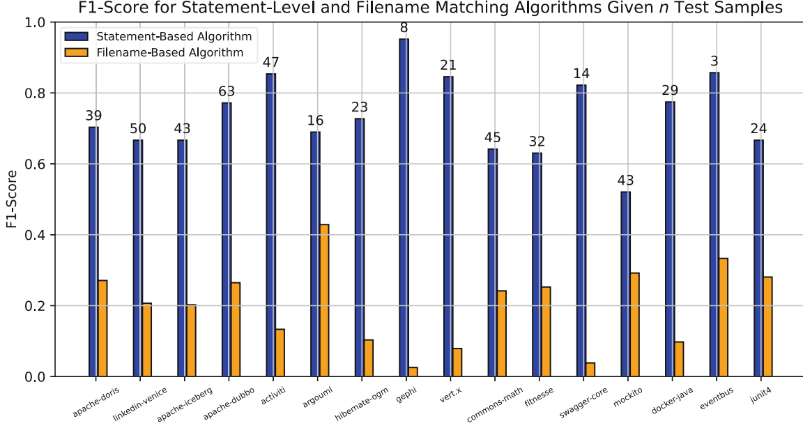
Fig. 3. F1-scores for the statement-based and filename-based matching algorithms given n test samples from different Java projects.
