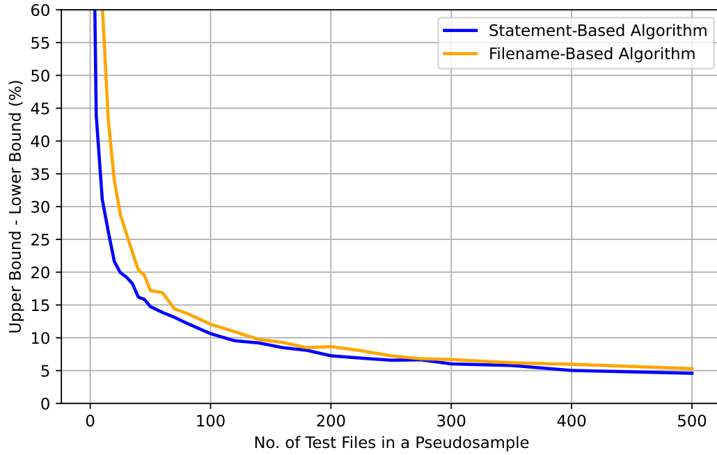
Figure 6.2: Difference between the upper bound and lower bound for the 95% confidence interval of the weighted F1-score for the matching algorithms
