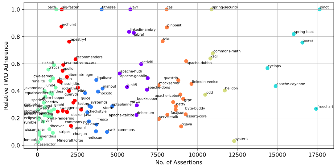
Figure 6.4: The scatter plot of relative TWD adherence for 100 Java projects.
