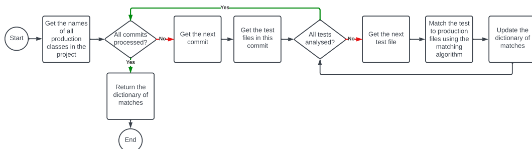
Figure 5.2: The mapping technique between tests and production files.
