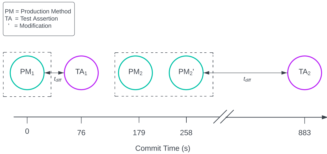
Figure 5.4: A representation of the time deltas of the Shapes project.
