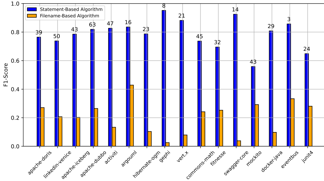
Figure 6.1: F1-scores for the statement-based and filename-based matching algorithms given n test samples from different Java projects.
