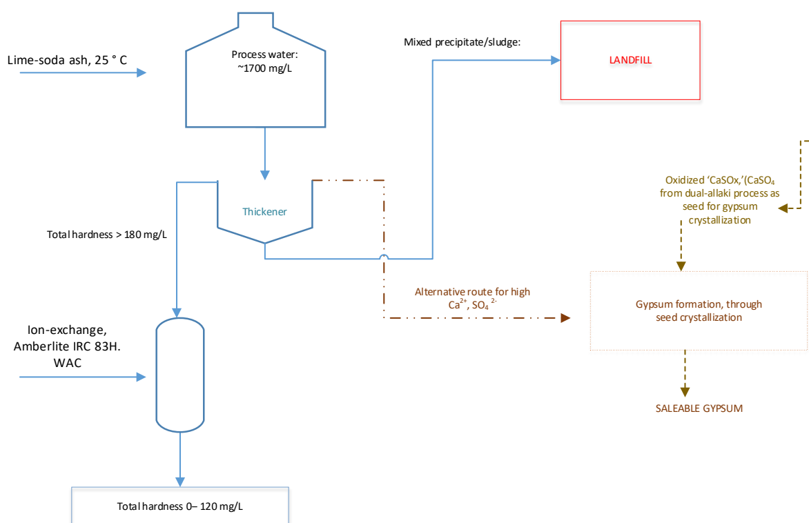
Figure 8. 1 Proposed flowsheet for the water softening process
