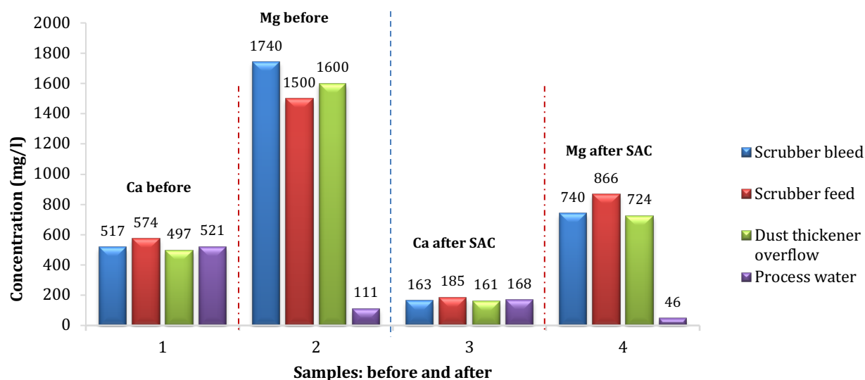
Figure 6. 13 Removal of calcium and magnesium by SAC resin. (Contact time = 60 minutes; Temperature = 25°C; Shaking speed 150 rpm; Resin mass = 10 g; Solution pH 4–10).
