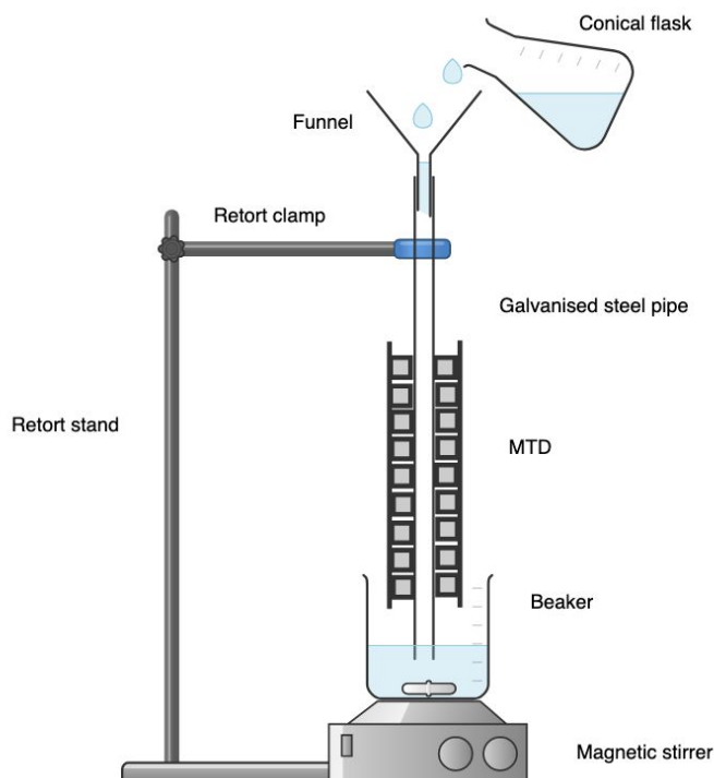
Figure 3. 5 Preliminary MWT setup for effect on pH and DO
