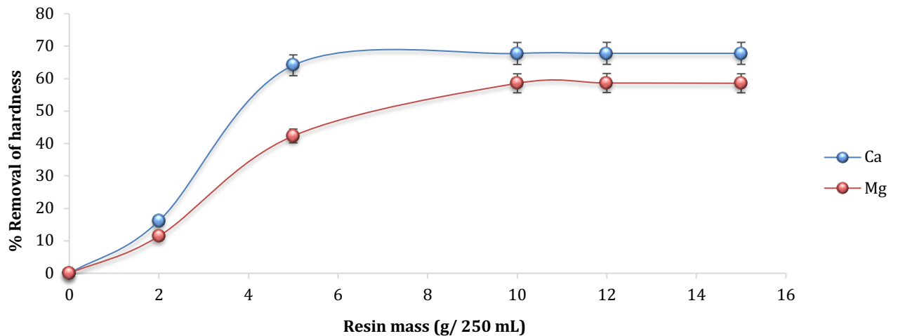
Figure 6. 7 Removal of calcium and magnesium by SAC resin as a function of resin mass. (Initial [Ca^{2+}] = 521 mg/L; initial [Mg^{2+}] = 111 mg/L; stirring speed = 150 rpm, contact time = 60 minutes s; Temperature = 25°C; initial natural pH = 4.85).
