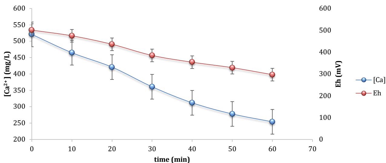
Figure 7. 19 [Ca 2+ ] and E h as a function of time
