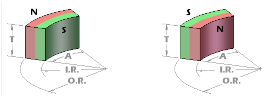
Figure 2. 20 Radially magnetized ( kjmagnets.com, 2022 )
