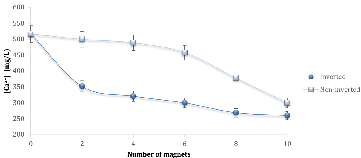
Figure 7. 14 Variation of [Ca^{2+}] against the number of magnets and orientation of magnetic poles for the scrubber bleed sample
