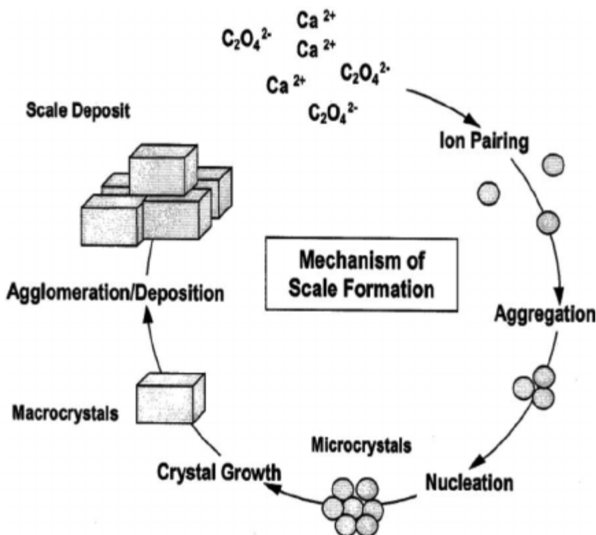
Figure 2. 9 Mechanism of scale formation (Safari et al., 2014)
