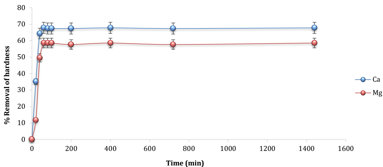
Figure 6. 11 Removal of calcium and magnesium by SAC resin as a function of contact time. (Initial [Ca^{2+}] = 521 \text{ mg/L} ; initial [Mg^{2+}] = 111 \text{ mg/L} ; Contact time = 24hrs; Temperature = 25^{\circ}\text{C} ; Initial natural pH = 4.85).
