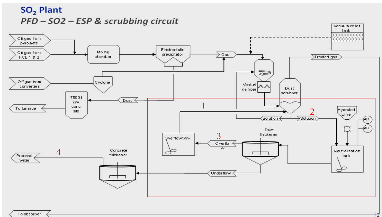
Figure 2. 13 Scrubbing circuit for A PGM smelter (Sibanye-Stillwater, 2019)
