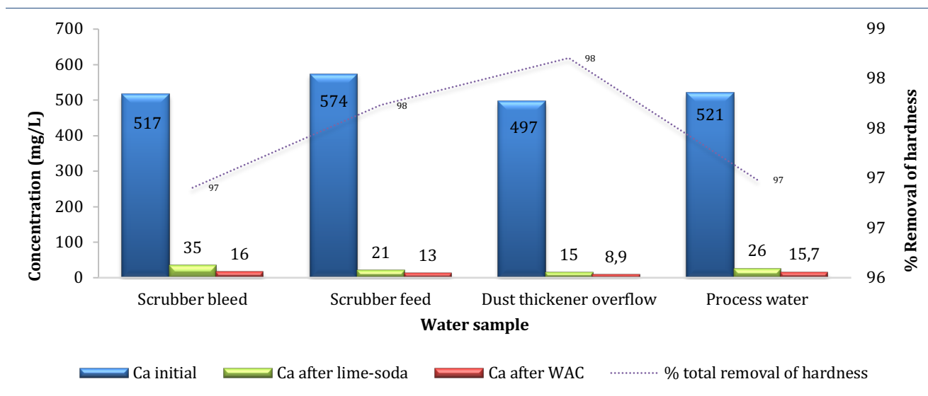
Figure 6. 14 Final Ca concentration after dual softening of water samples with lime-soda ash and WAC resin
