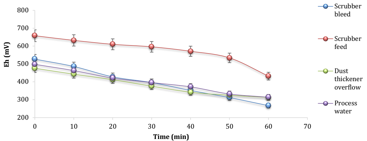
Figure 7. 8 Effect of MTD on E_h for all four water samples
