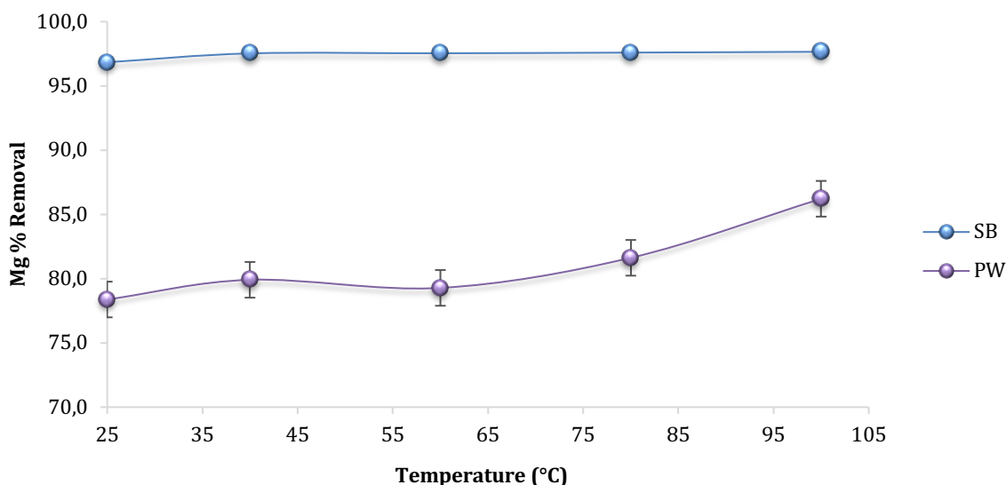
Figure 5. 12 Magnesium removal efficiency with increasing temperature for lime-soda softening
