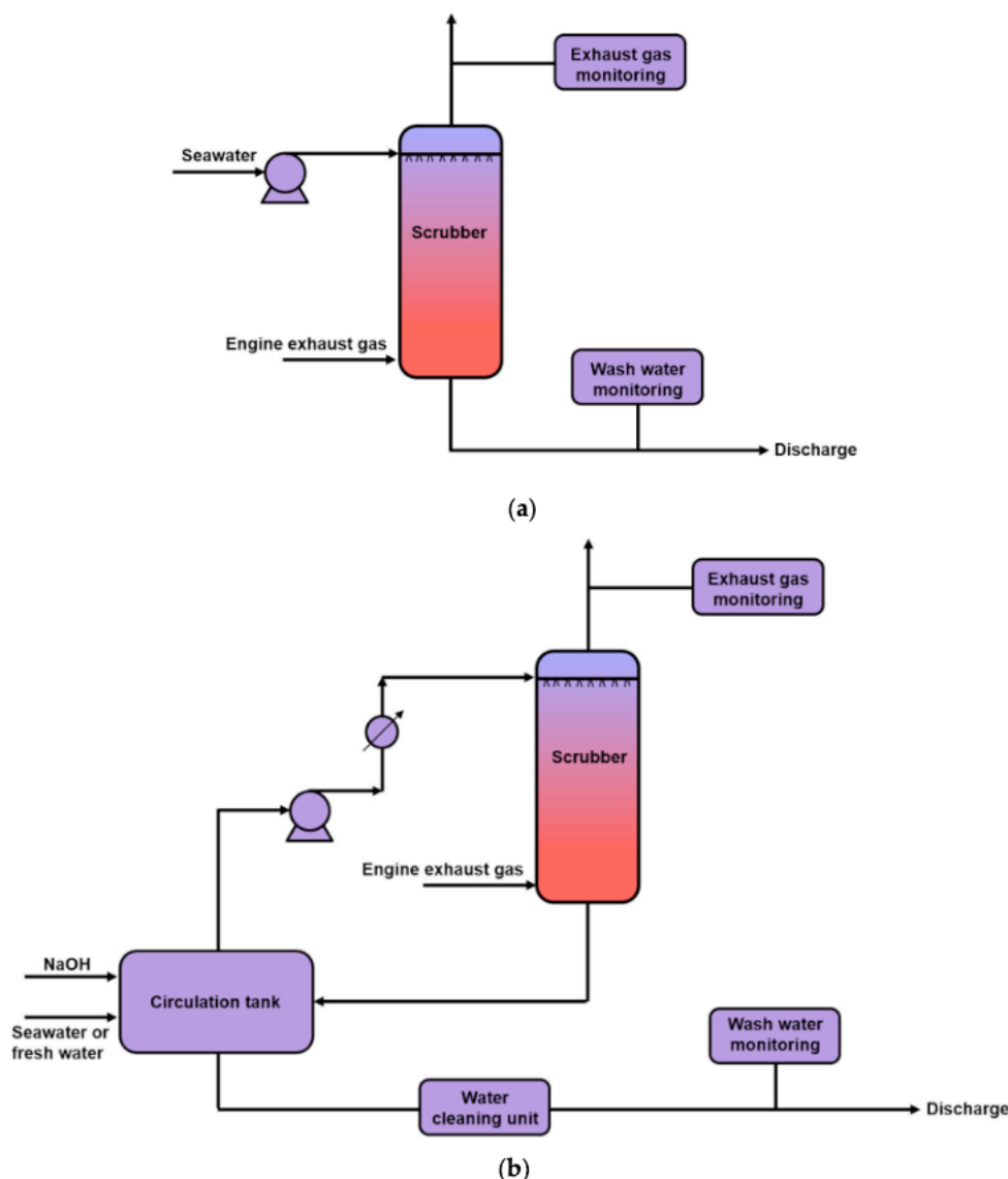
Figure 2. 5 Schematic diagram of the (a) open-loop FGD process, (b) closed-loop FGD process (Long et al., 2020).
