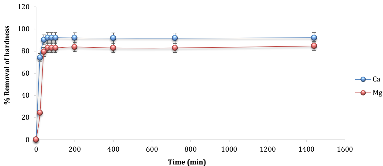
Figure 6. 10 Removal of calcium and magnesium by WAC resin as a function of contact time. (Initial [Ca^{2+}] = 521 \text{ mg/L} ; initial [Mg^{2+}] = 111 \text{ mg/L} ; Contact time = 24hrs; Temperature = 25^{\circ}\text{C} ; Initial natural pH = 4.85).
