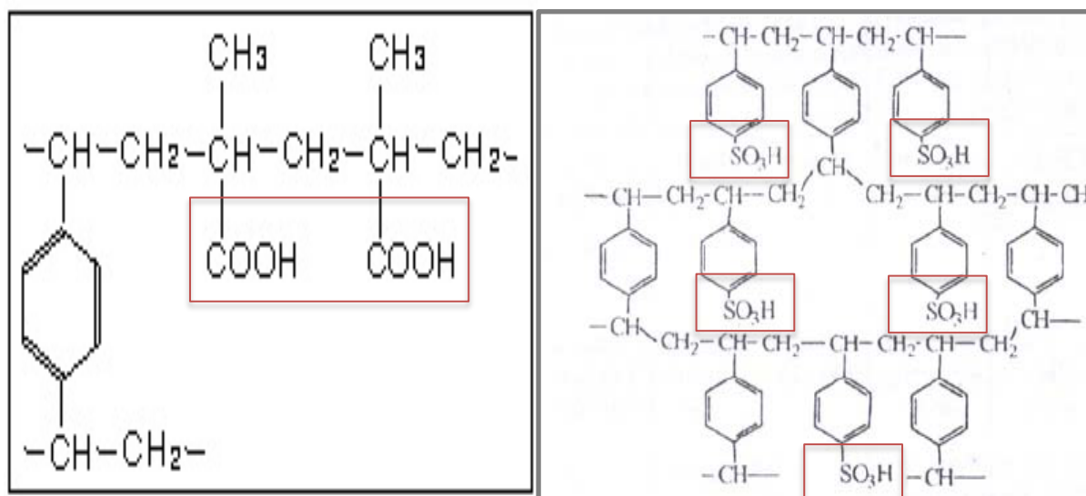
Figure 2. 15 Structure of a weak acid cation resin (left) and a strong acid cation resin (right)
