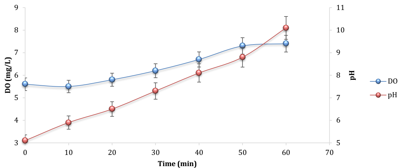
Figure 7.20 DO and pH as a function of time
