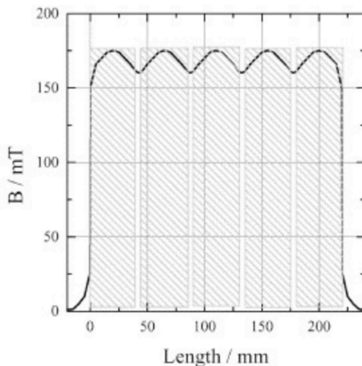
Figure 2. 24 Variation of the magnetic induction in the gap for non-inverted pairs of permanent magnets (Gabrielli et al., 2001).
