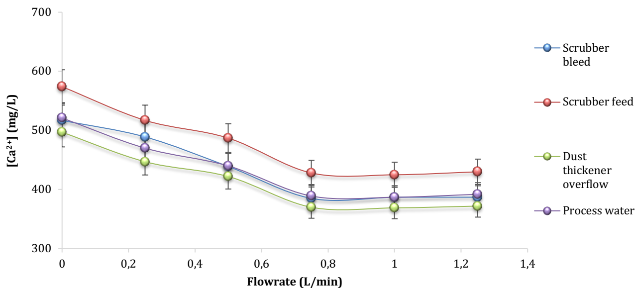
Figure 7. 17 Effect of flowrate on the MTD removal efficiency
