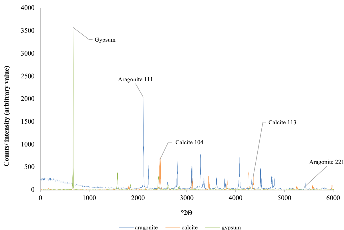
Figure 7. 22 XRD analysis for crystals formed after 60 minutes exposure to MTD
