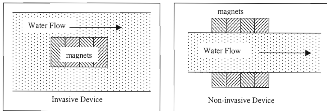
Figure 2. 26 Variations in Installation of Magnets (Rathilal, 2004).
