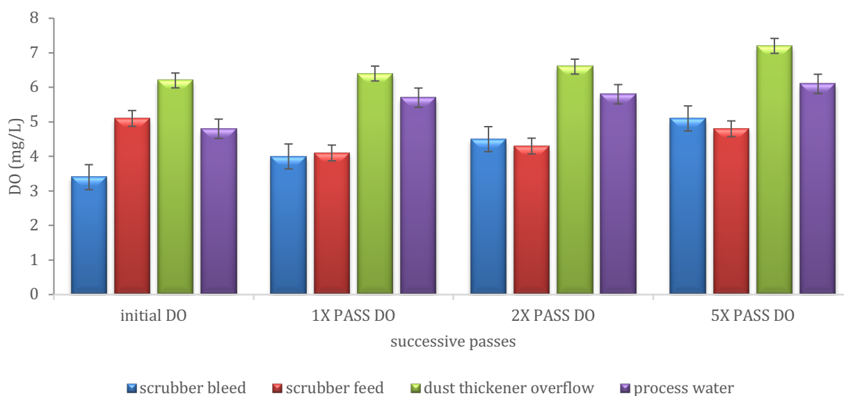
Figure 7. 2 MWT effect on solution DO
