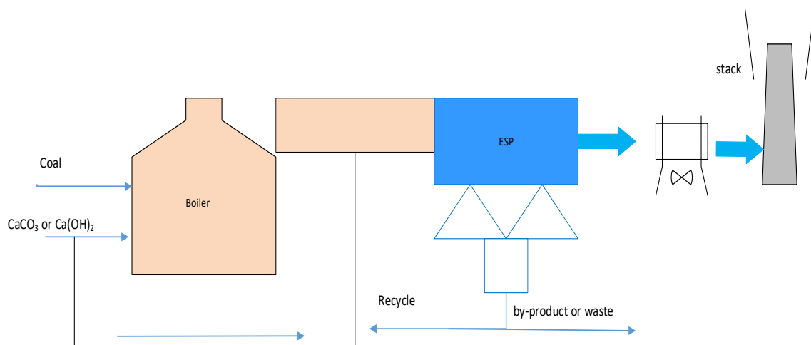
Figure 2. 8 Typical dry sorbent injection process (adapted from Lisnic and Jinga, 2018)
