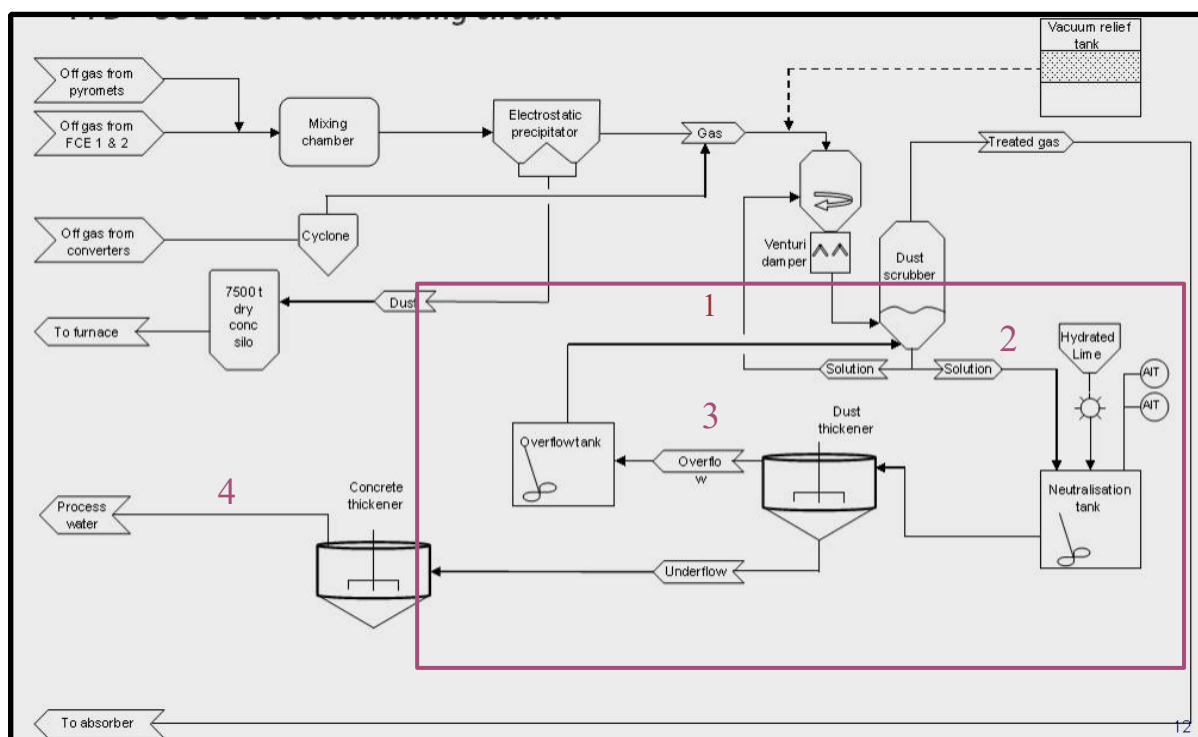
Figure 4. 2 Liquid sample points from the scrubbing circuit
