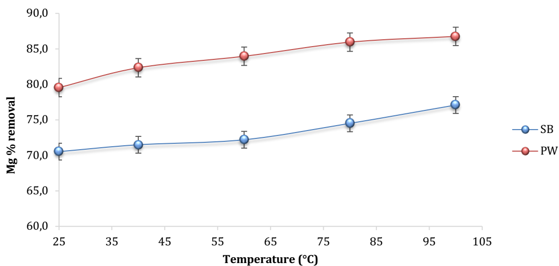
Figure 5. 8 Magnesium removal with increasing temperature for lime softening procedure
