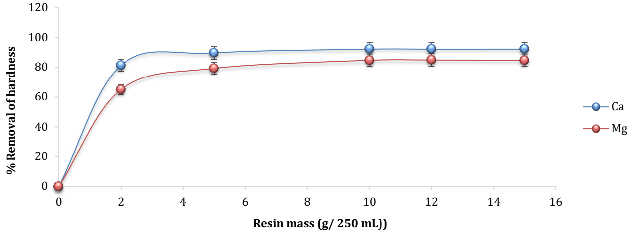
Figure 6. 6 Removal of calcium and magnesium by WAC resin as a function of resin mass. (Initial [Ca^{2+}] = 521 mg/L; initial [Mg^{2+}] = 111 mg/L; stirring speed = 150 rpm, contact time = 60 minutes; Temperature = 25°C; initial natural pH = 4.85).
