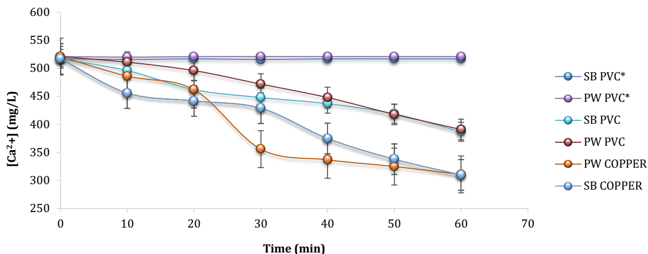
Figure 7. 18 Variation of [Ca^{2+}] against the pipe material of the MTD
