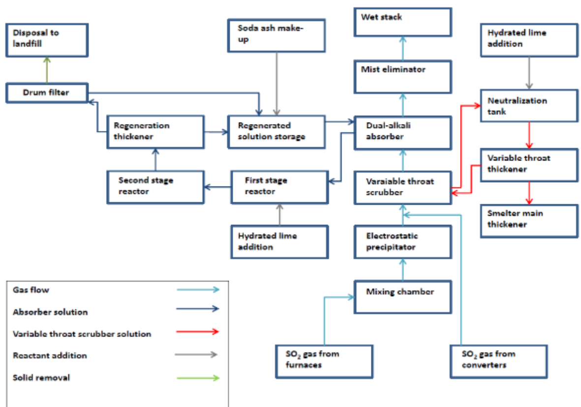
Figure 1. 2 Simplified flow diagram of the dual-alkali system. Figure adapted from Bezuidenhout et al. (2012, pg. 2)
