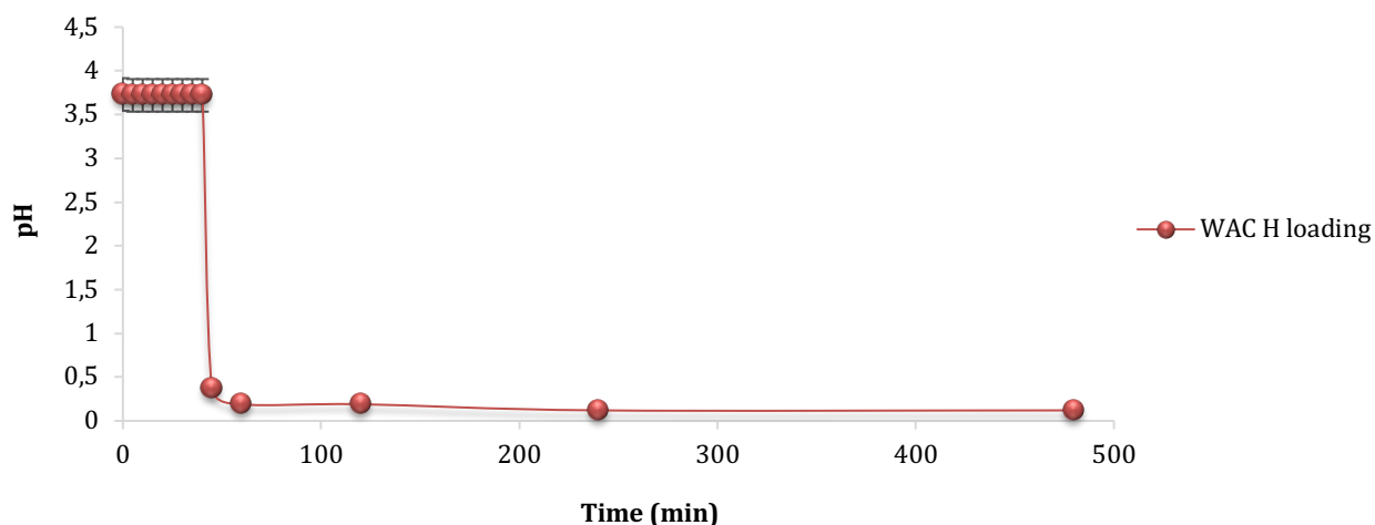
Figure 6. 1 Proton ( H^+ ) loading on WAC resin ( Amberlite IRC83H )
