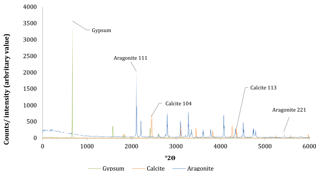
Figure 7. 23 XRD analysis for crystals formed after 3 hours exposure to MTD
