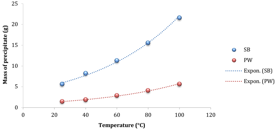
Figure 5. 6 Relationship between temperature and mass of precipitate formed for lime treatment
