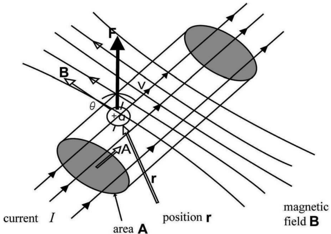
Figure 2. 31 An electric wire with cross-section A flown by a current I is submitted to a force F when placed into a magnetic field B (Sawaftah, 2017)
