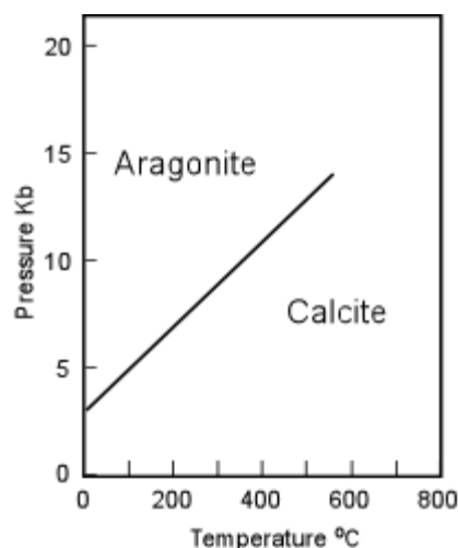
Figure 2. 11 Stability of aragonite and calcite with respect to pressure and temperature (Nelson, 2014).
