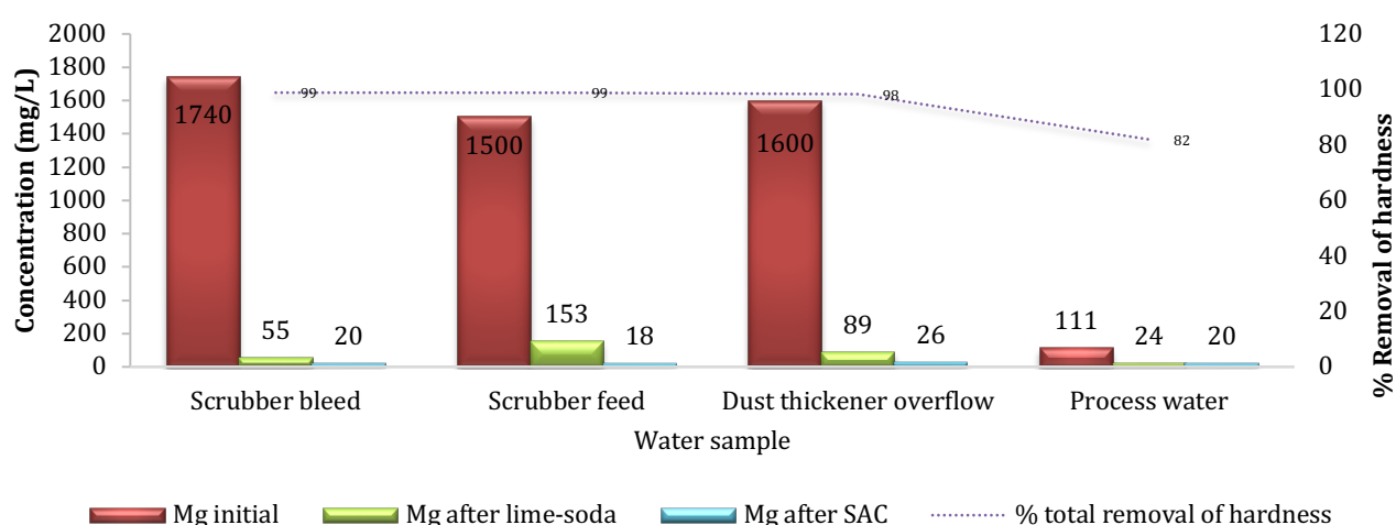
Figure 6. 17 Final Mg concentration after dual softening of water samples with lime-soda ash and SAC resin
