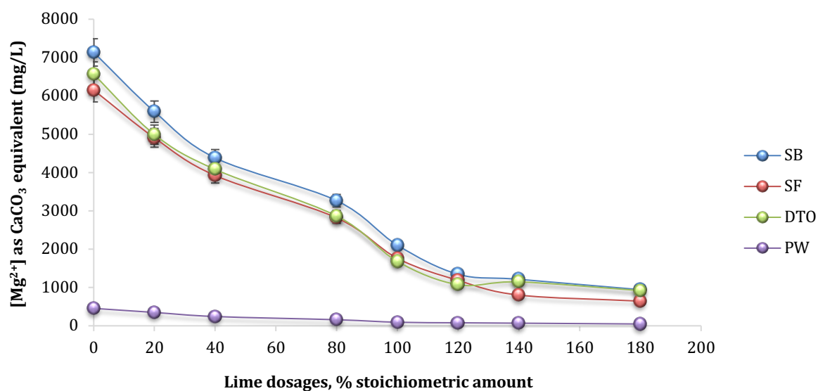
Figure 5. 3 Variation of magnesium for varying lime dosages
