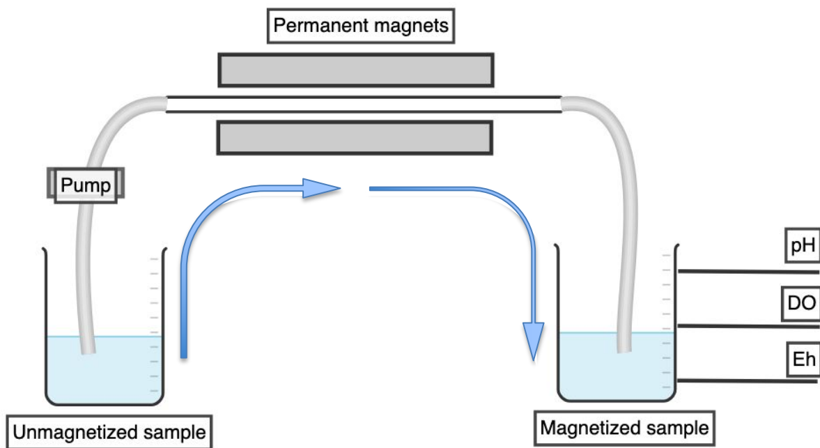
Figure 3. 7 Adjusted MTD for further tests
