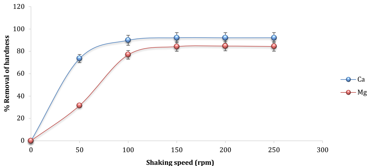
Figure 6.8 Removal of calcium and magnesium by WAC resin as a function of shaking speed. (Initial [Ca^{2+}] = 521 mg/L; initial [Mg^{2+}] = 111 mg/L; contact time = 24hrs; Temperature = 25°C; initial natural pH = 4.85).
