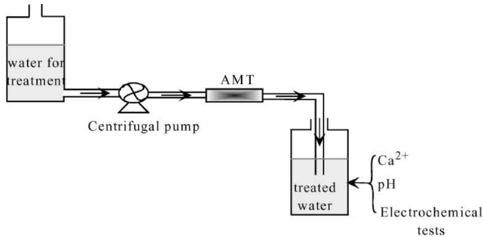
Figure 2. 25 Typical MTD setup for water treatment (Gabrielli et al., 2001).
