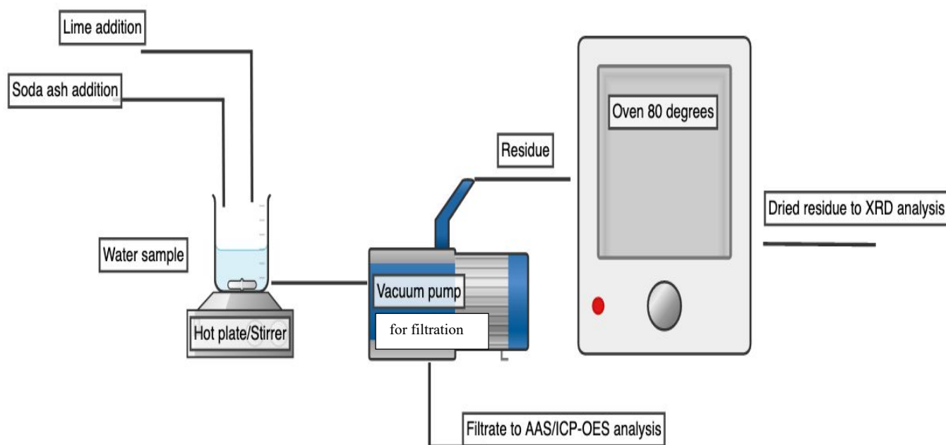
Figure 3. 4 Diagrammatic representation of the lime-soda ash process
