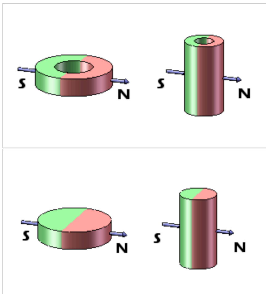
Figure 2. 21 Diametrically magnetized ( kjmagnets.com , 2022)
