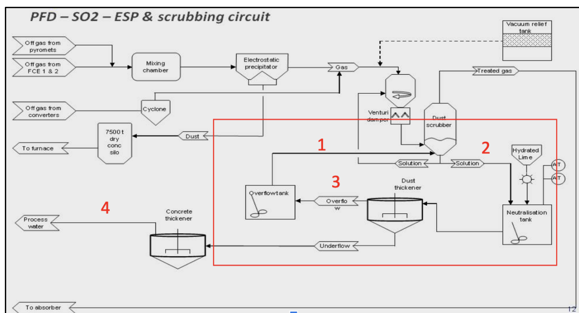
Figure 3. 2 Scrubber circuit at Sibanye-Stillwater indicating sampling points (1. Scrubber feed, 2. Scrubber bleed, 3. Dust-thickener overflow and 4. Process water).
