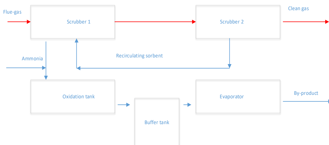
Figure 2. 7 Flow diagram of the Walther method (adapted from Poullikkas, 2015).
