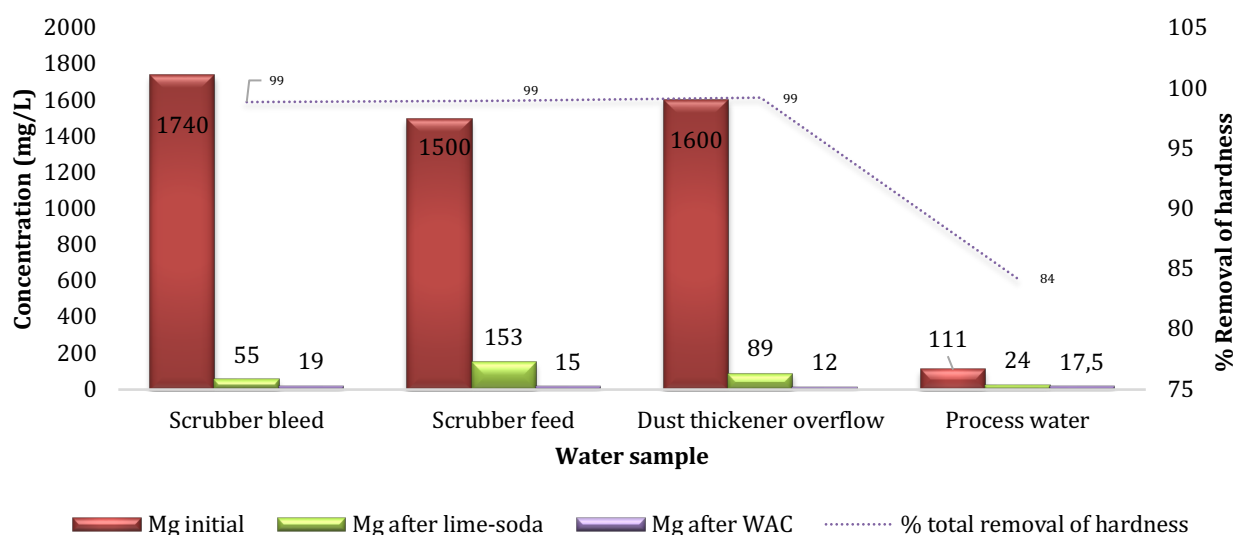
Figure 6. 15 Final Mg concentration after dual softening of water samples with lime-soda ash and WAC resin
