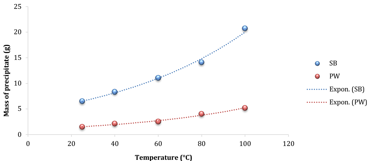
Figure 5. 10 Relationship between temperature and mass of precipitate formed for lime-soda ash treatment
