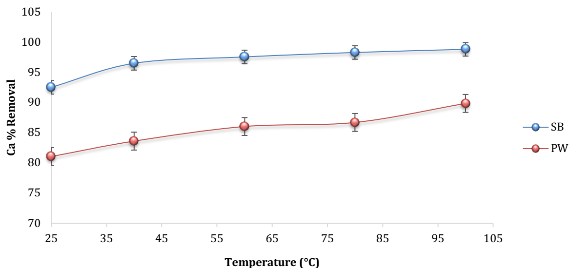
Figure 5. 7 Calcium removal with increasing temperature for lime softening procedure
