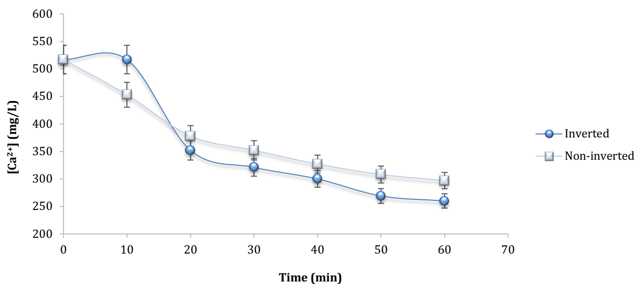
Figure 7. 11 Inverted vs non-inverted magnetic poles and the effect on [Ca^{2+}] of the scrubber bleed sample
