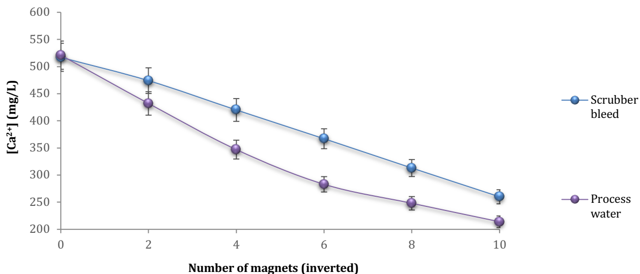
Figure 7. 10 Relationship between number of magnets/ effective magnetic strength and [\text{Ca}^{2+}]
