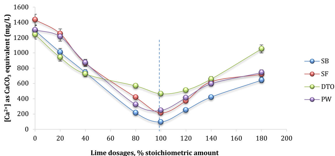
Figure 5. 2 Variation of calcium for varying lime dosages
