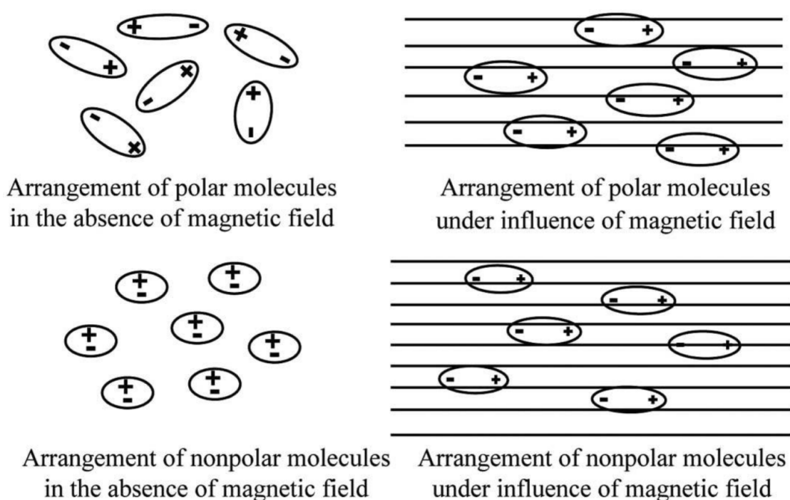
Figure 2. 27 Effect of a magnetic field on polar (top) and nonpolar (bottom) molecules (Sawaftah, 2017)
