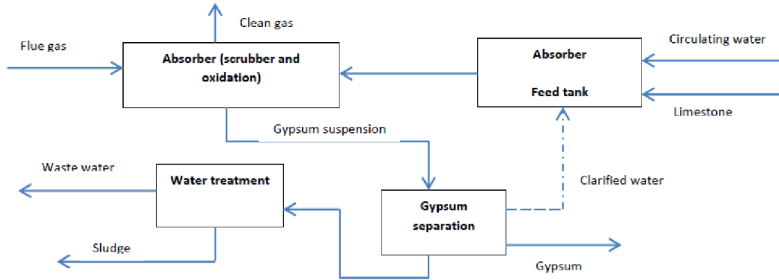
Figure 2. 3 Flow diagram of the limestone scrubbing method (adapted from Poullikkas, 2015)
