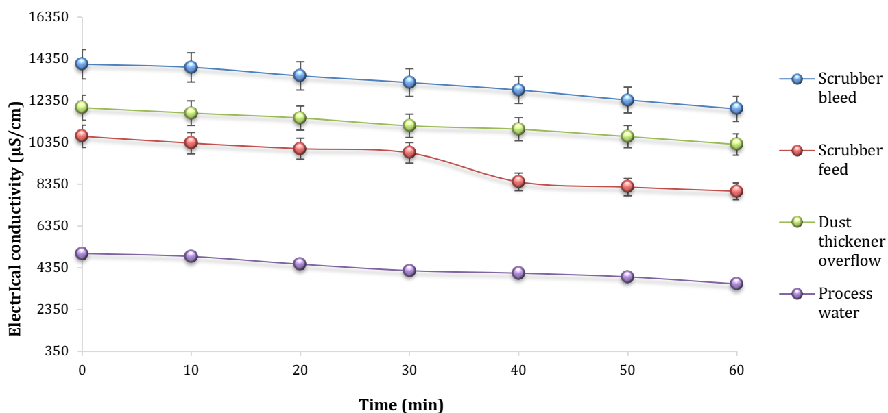
Figure 7. 4 Effect of MTD on EC for all four water samples
