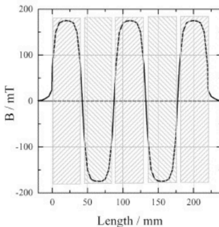
Figure 2. 23 Variation of the magnetic induction for inverted pairs of permanent magnets (Gabrielli et al., 2001).
