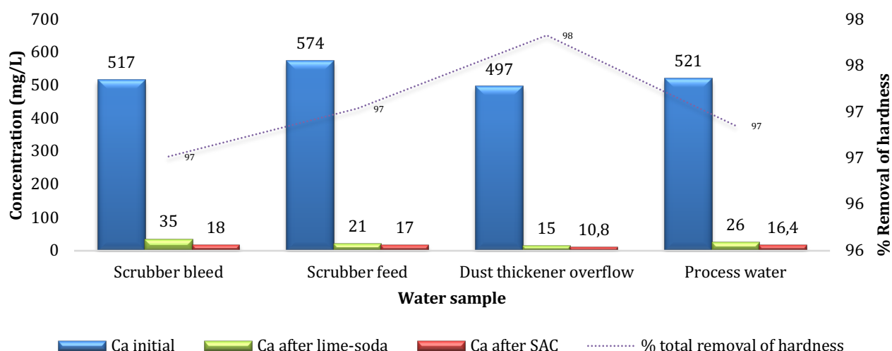
Figure 6. 16 Final Ca concentration after dual softening of water samples with lime-soda ash and SAC resin
