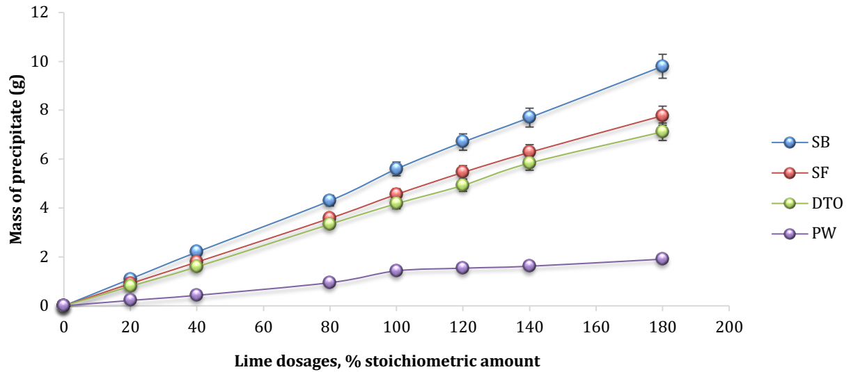
Figure 5. 5 Effect of varying lime dosage on precipitate mass
