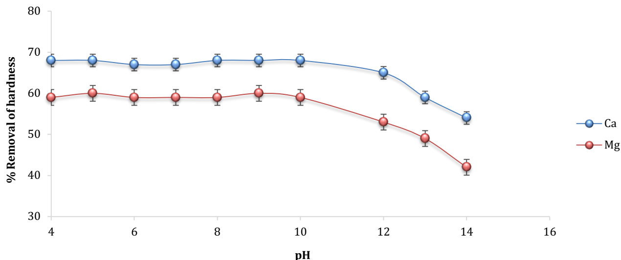
Figure 6. 4 Removal of calcium and magnesium by SAC resin as a function of initial pH of the solution (Initial [Ca^{2+}] = 521 mg/L; initial [Mg^{2+}] = 111 mg/L; stirring speed = 150 rpm, contact time = 60 minutes; Temperature = 25°C)
