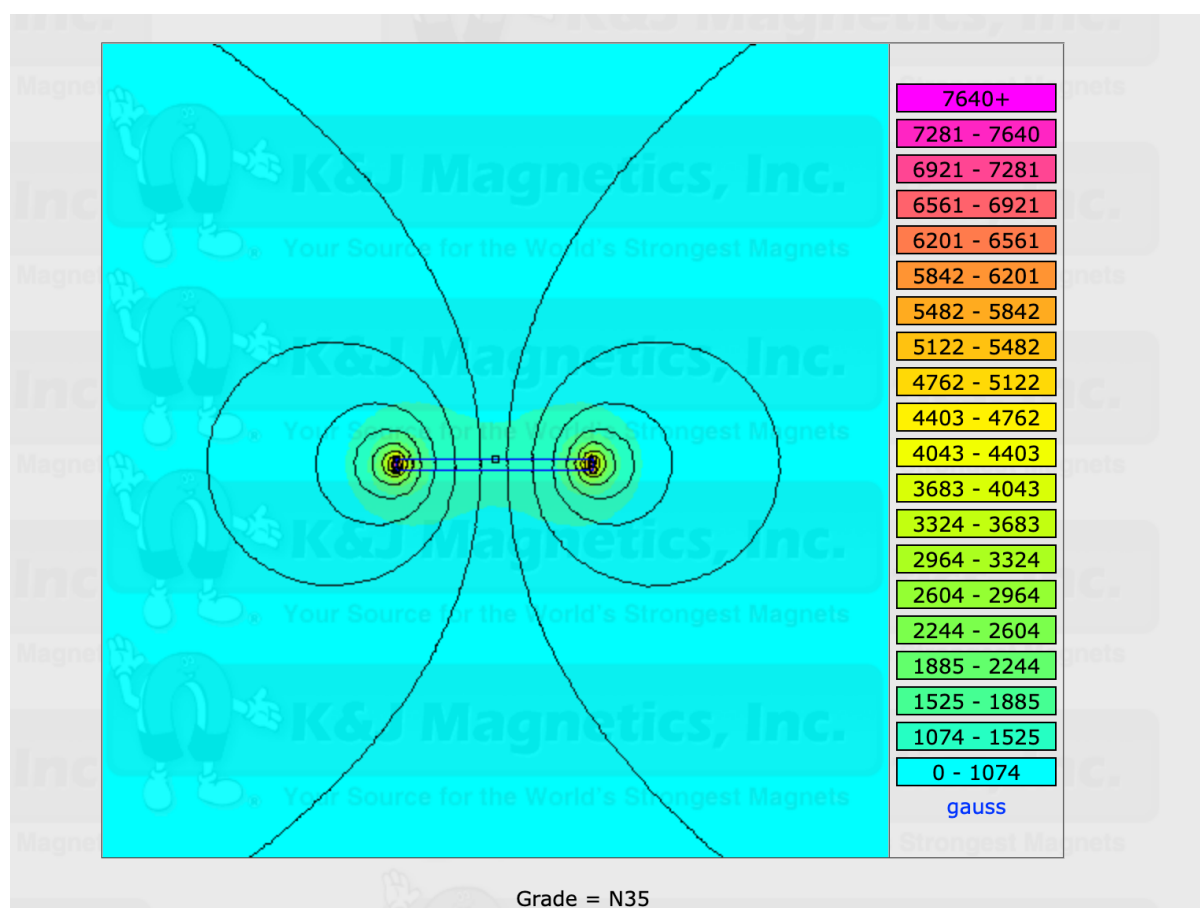
Figure 3. 9 Direction of magnetic field for the neodymium magnets used, axially magnetized ( kjmagnets.com , 2022)
