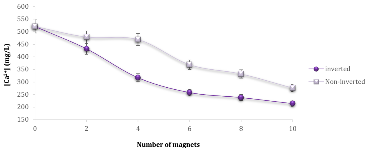
Figure 7. 15 Variation of [Ca^{2+}] against the number of magnets and orientation of magnetic poles for the process water sample
