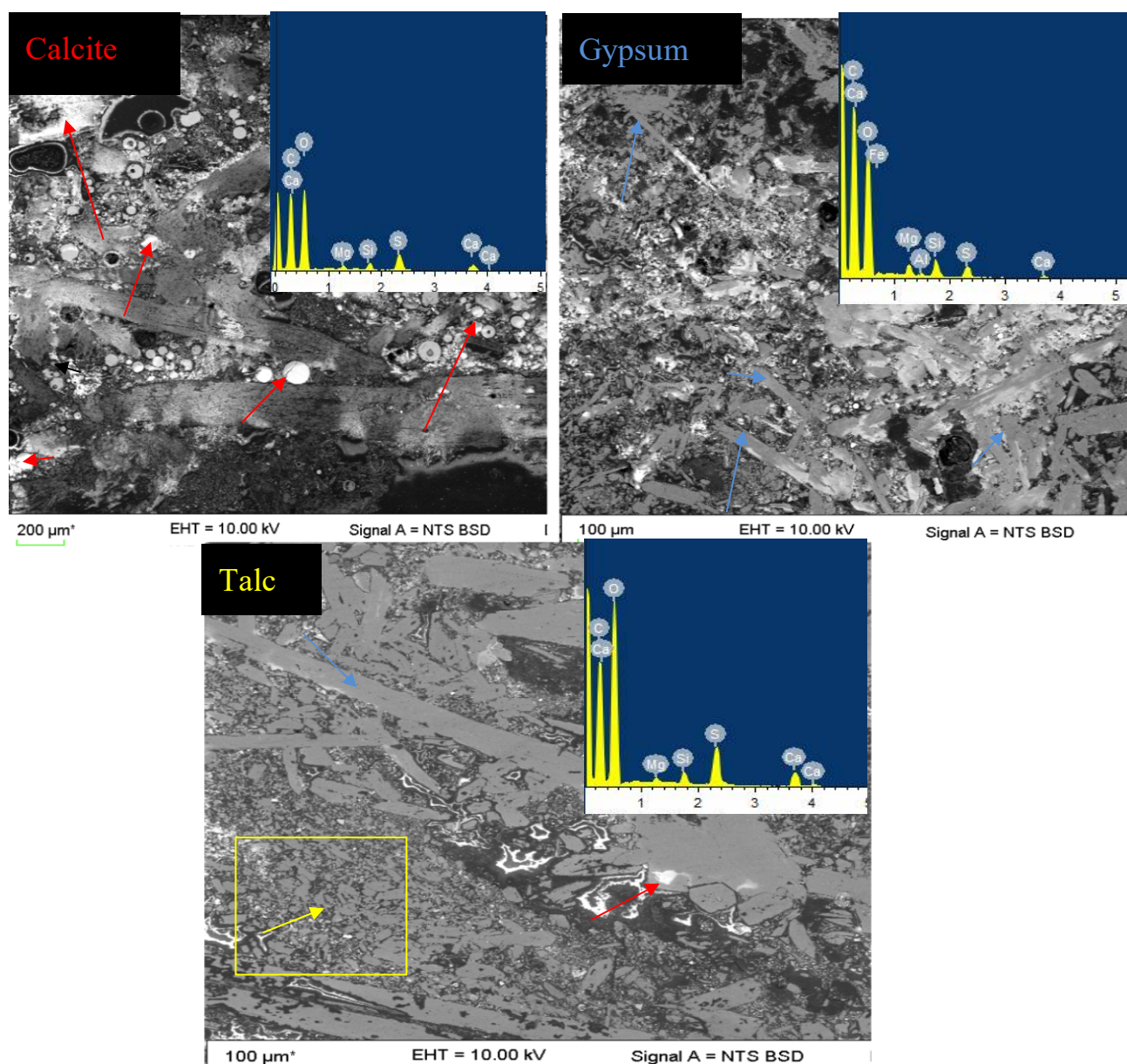
Figure 4. 1 SEM photomicrographs of three of the samples collected presenting major crystal phases
