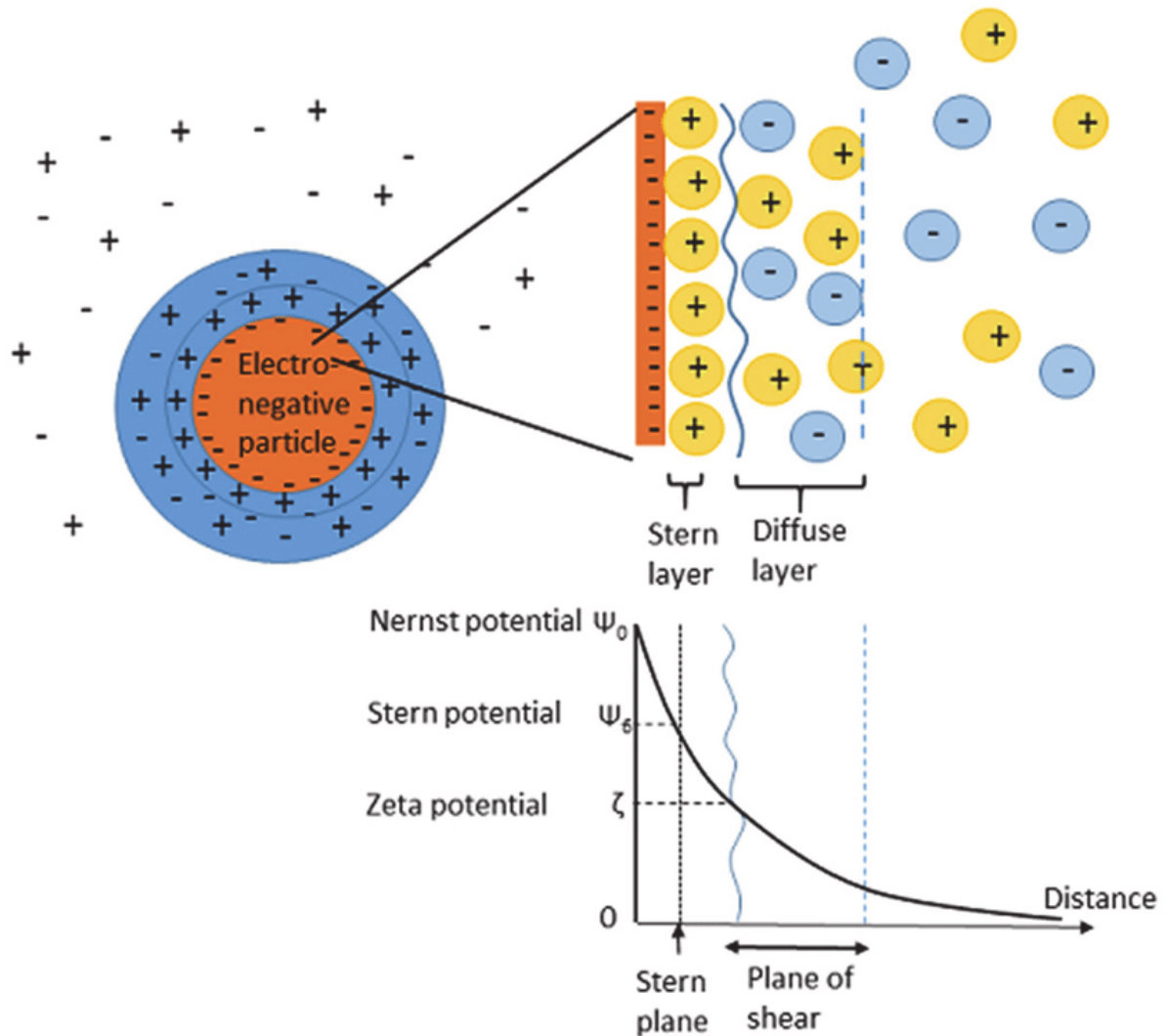
Figure 2. 29 Representation of the electrical double layer (Stern and diffuse layer) (Suopajarvi, 2015).
