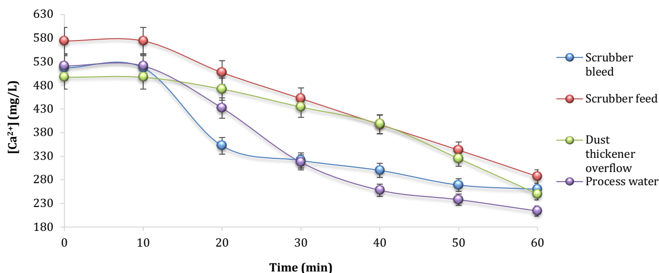
Figure 7. 3 Effect of MTD on [Ca^{2+}] for all four water samples
