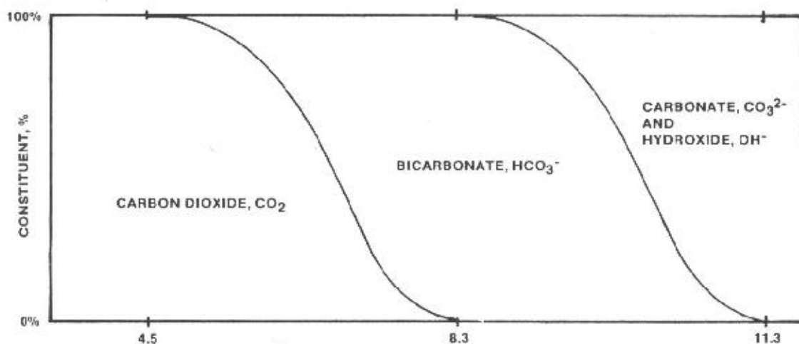
Figure 2. 14 Relationship between pH and alkalinity ( \text{HCO}_3^- , \text{CO}_3^{2-} and \text{OH}^- ) (Minnesota Rural Water Association, 2009, page 5).
