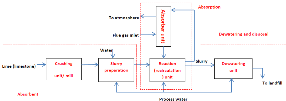
Figure 2. 2 General flow diagram for a wet FDG process (adapted from Živković et al., 2014)
