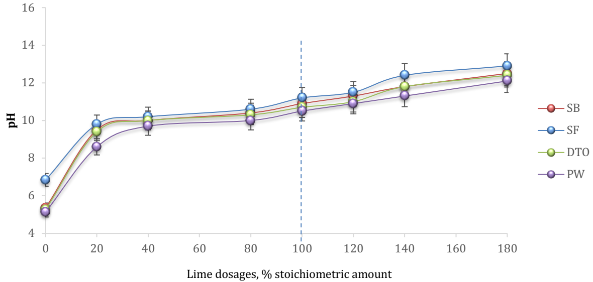
Figure 5. 1 Effect of varying lime dosage on pH
