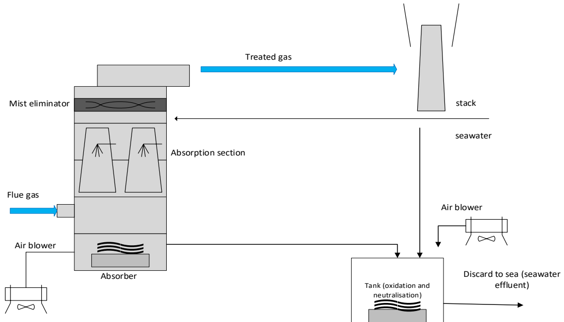
Figure 2. 4 Seawater FGD process (adapted from Lisnic and Jinga, 2018)
