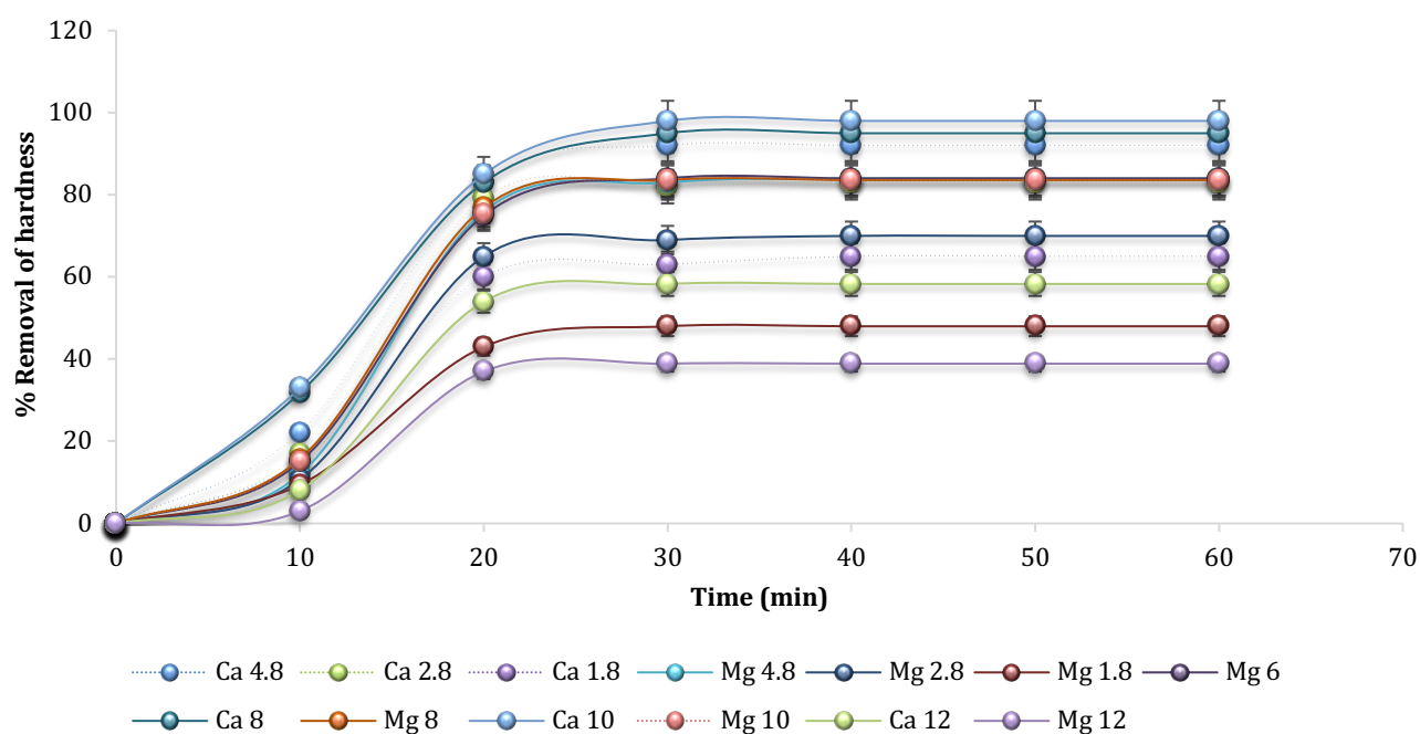
Figure 6. 3 Removal of calcium and magnesium by WAC resin as a function of initial pH of the solution (Initial [\text{Ca}^{2+}] = 521 mg/L; initial [\text{Mg}^{2+}] = 111 mg/L; stirring speed = 150 rpm, contact time = 60 minutes; Temperature = 25°C)
