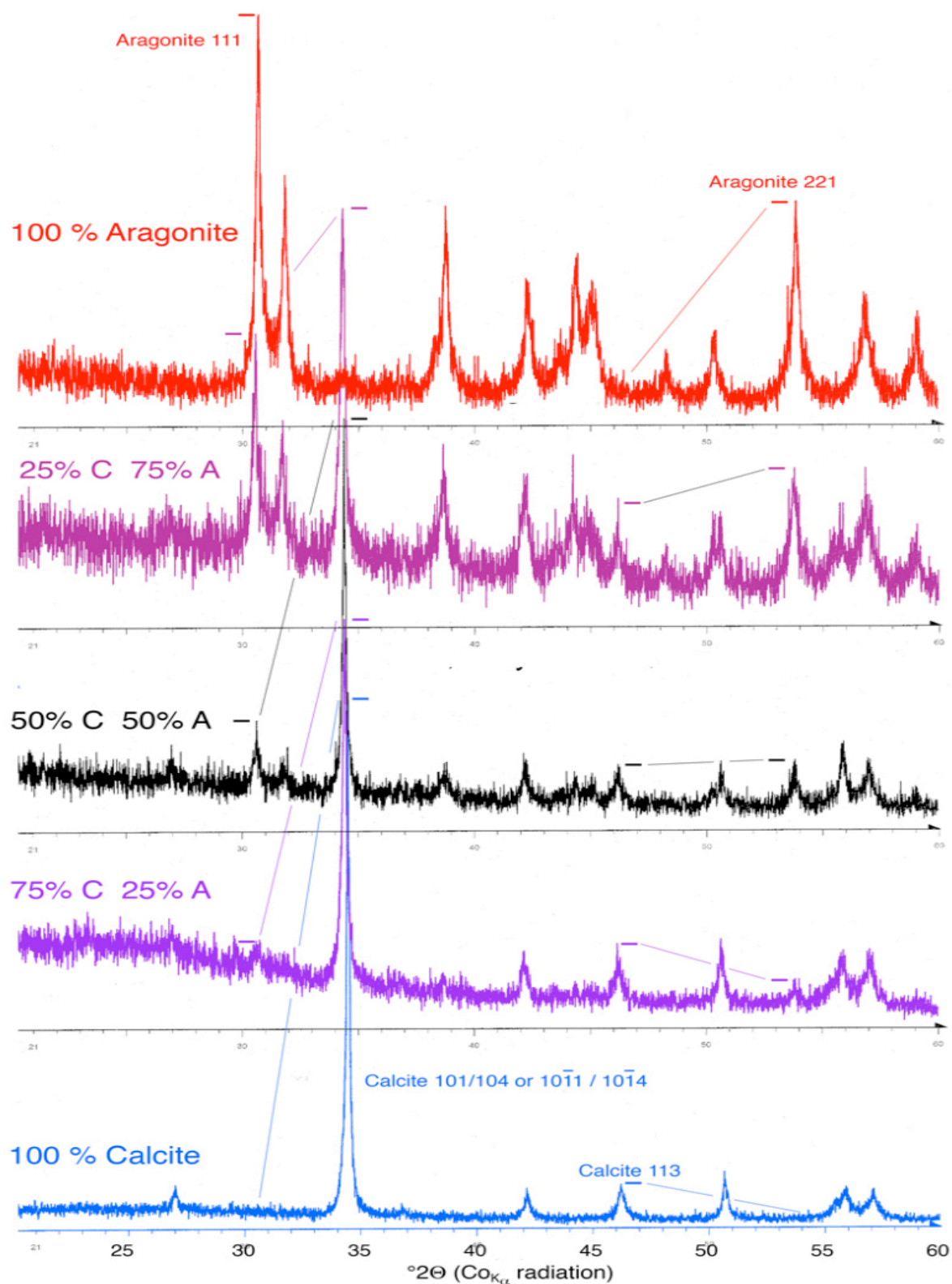
Figure 2. 12 X-ray diffraction (XRD) pattern for a mixture of aragonite and calcite, highlighting significant peaks for the purpose of identification (Railsback, 2006).
