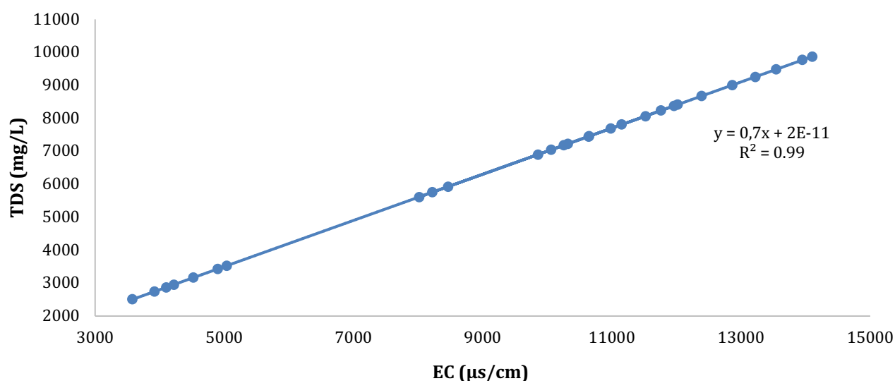
Figure 7. 5 Relationship between TDS and EC for all water samples.
