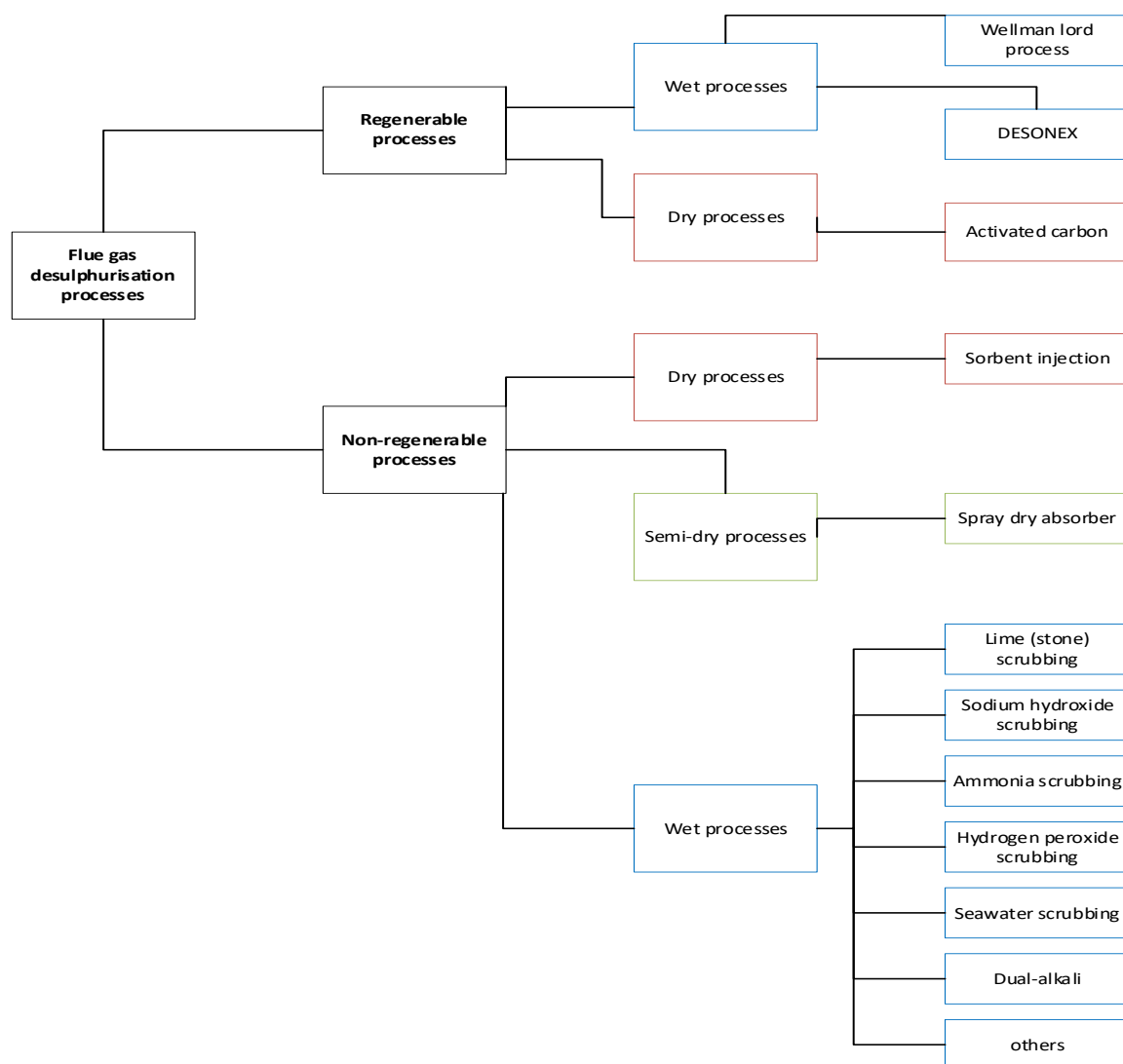
Figure 2. 1 FGD process classification (adapted from Lisnic and Jinga, 2018)
