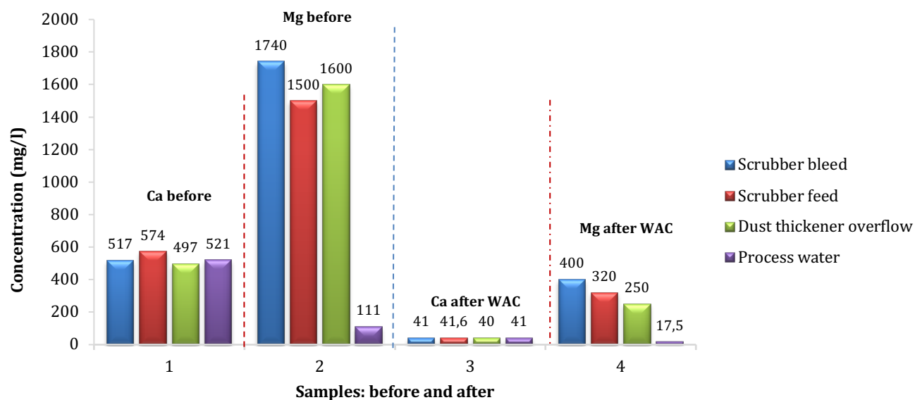
Figure 6. 12 Removal of calcium and magnesium by WAC resin. (Contact time = 60 minutes; Temperature = 25°C; Shaking speed 150 rpm; Resin mass = 10 g; Solution pH 4 –10).
