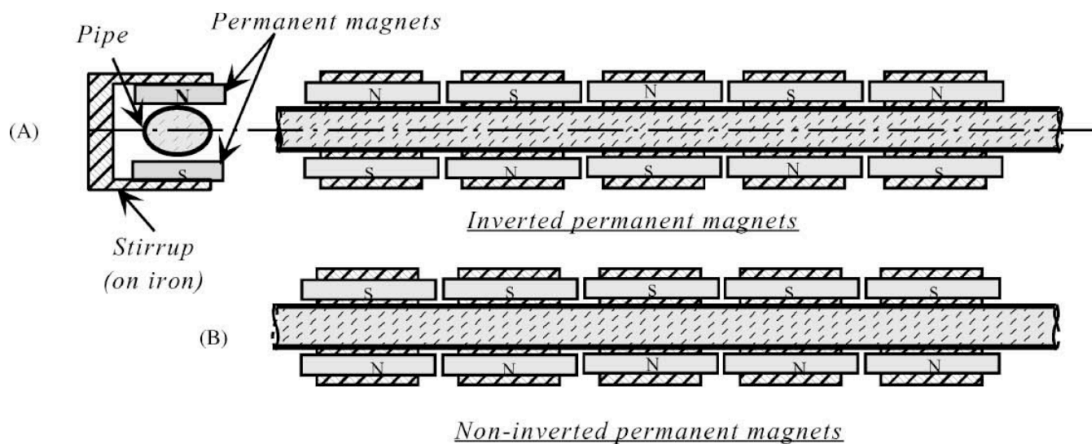
Figure 2. 22 Scheme of the MTD with alternated magnetic poles (inverted), (B) scheme of the MTD without inversion of the magnetic poles (non-inverted) (Gabrielli et al., 2001).
