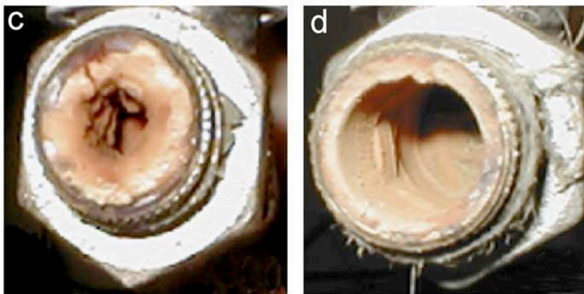
Figure 2. 17 MWT effect: Left (c) is the steel pipe without MWT. Right (d) shows a similar pipe treated with a magnetic field (Lipusa and Dobersek, 2007)
