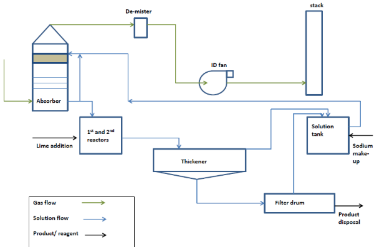
Figure 1. 1 Block flow diagram of the off-gas handling equipment. Figure adapted from Bezuidenhout et al. (2012, pg. 2)
