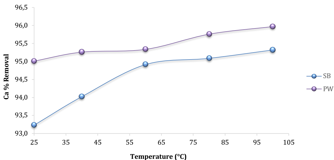
Figure 5. 11 Calcium removal efficiency with increasing temperature for lime-soda softening
