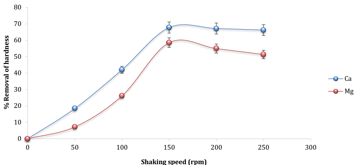
Figure 6. 9 Removal of calcium and magnesium by SAC resin as a function of shaking speed. (Initial [Ca^{2+}] = 521 mg/L; initial [Mg^{2+}] = 111 mg/L; contact time = 24hrs; Temperature = 25°C; initial natural pH = 4.85).
