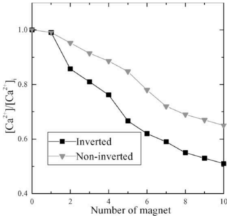
Figure 7. 16 Variation of the concentration of the ionic calcium against the length of the magnetic device obtained by varying the number of inverted or non-inverted pairs of permanent magnets (Gabrielli et al., 2001).
