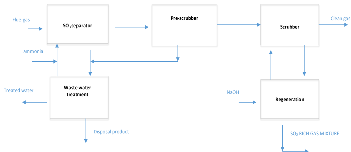
Figure 2. 6 Flow diagram of the Wellman-Lord process (adapted from Poullikkas, 2015)
