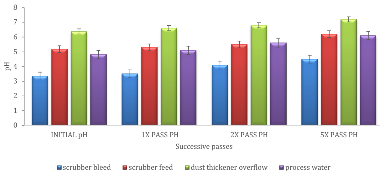
Figure 7. 1 MWT effect on solution pH
