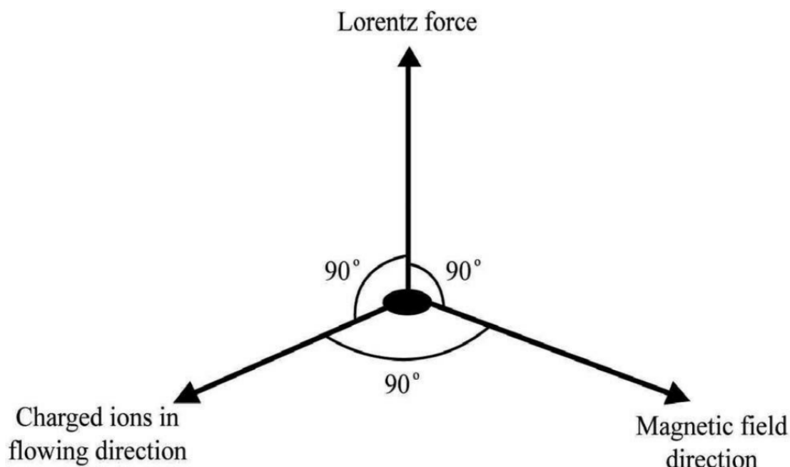
Figure 2. 30 The Laplace-Lorentz force on a moving charged ion is at a right angle of both the ion flowing direction and the magnetic field direction (Sawaftah, 2017)
