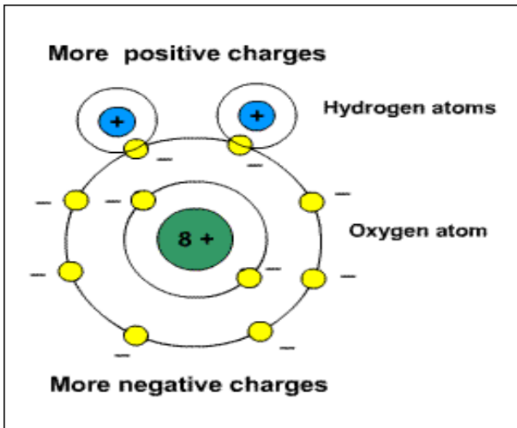
Figure 2. 28 Dipole moment of a water molecule (McMahon, 2009)
