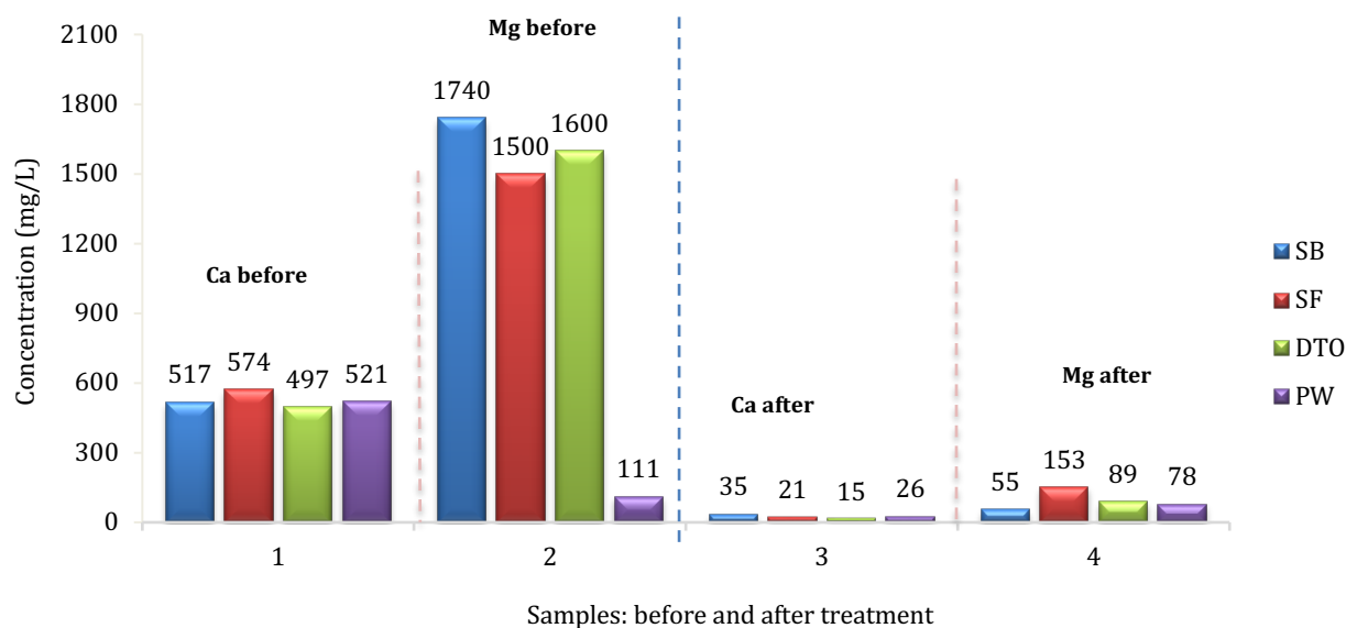
Figure 5. 9 Lime-soda ash treatment for Ca and Mg removal
