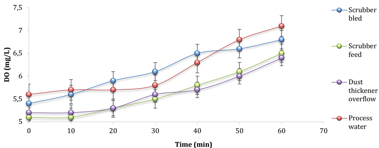
Figure 7. 7 Effect of MTD on DO for all four water samples
