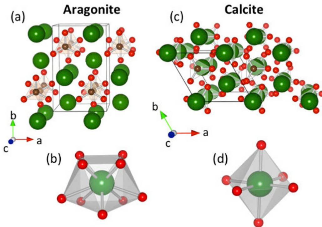
Figure 2. 10 Crystal structure of aragonite (a, b) and calcite (c, d) (Soldati et al., 2016).
