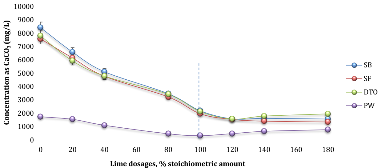
Figure 5. 4 Variation of total hardness for varying lime dosages
