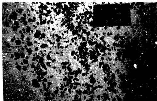
Figure 6.27 : 85 Iron Grit After 11 Cuts (magnified 10 times)
