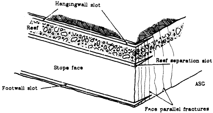
Figure 1.6 : Configuration of Slots for Cutting and Breaking Method
