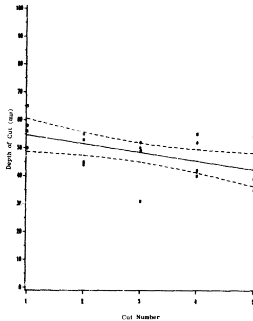
Figure 6.24 : Effect of Cut Number (number of times the abrasive is re-used) on Depth of Cut in Norite Using Quartzite Abrasive
