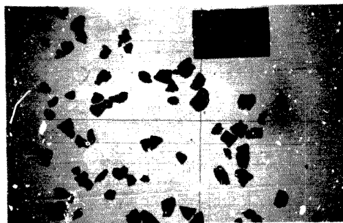
Figure 6.26 : 85 Iron Grit Before Cutting (magnified 10 times)
