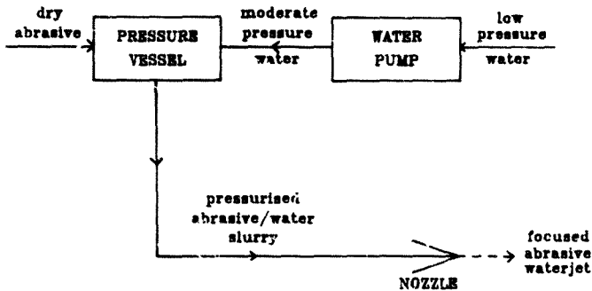
Figure 1.9 : Schematic Illustration of Abrasive Waterjet Cutting Systems
