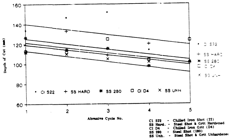
Figure 6.14 : Effect of Cut Number (number of times abrasive has been re-used) on Depth of Cut in Norite
