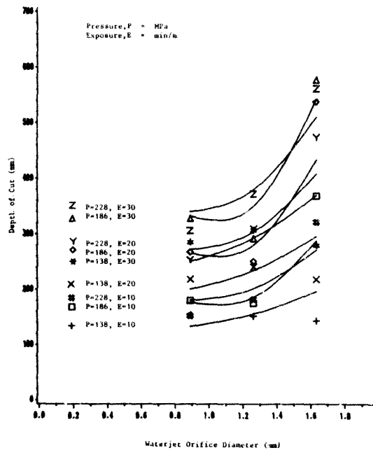
Figure 6.8 : The Effect of Orifice Size on Depth of Cut in Quartzite (High MPF Model)
