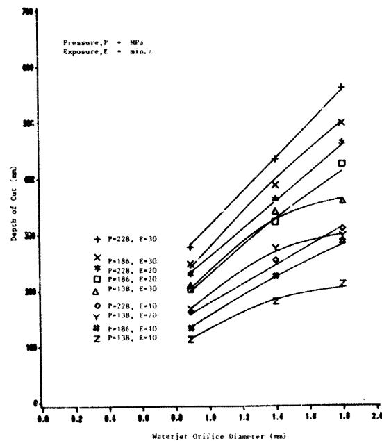
Figure 6.2 : The Effect of Orifice Size on Depth of Cut in Norite
