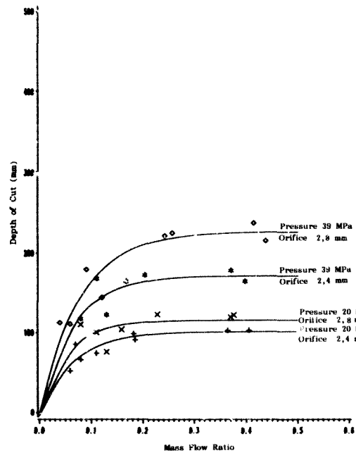
Figure 6.18 : Effect of MFR on Depth of Cut in Norite (first exposure)
