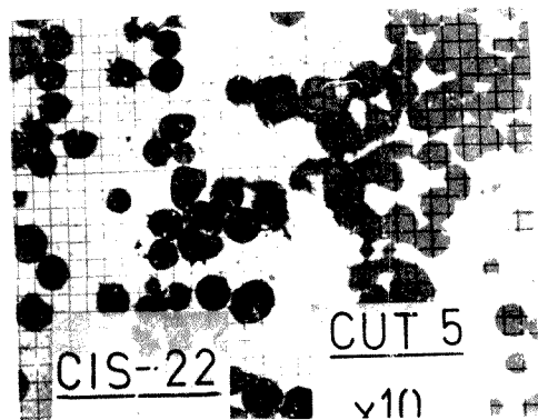
Figure 6.15 : Photographic Analysis of the Degradation of Chilled Iron Shot
