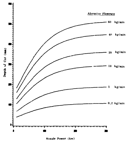
Figure 6.29 : Depth of Cut, for Slurry Cutting, Modelled in Terms of Nozzle Power and Abrasive Flowrate
