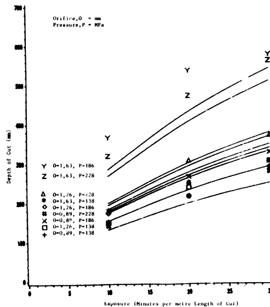
Figure 6.12 : The Effect of Exposure Time on Depth of Cut in Quartzite (High MFR Model)
