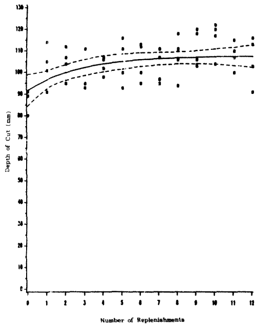
Figure 6.28 : Effect of Abrasive Replenishment with Abrasive Recycling on Depth of Cut in Nozzle
