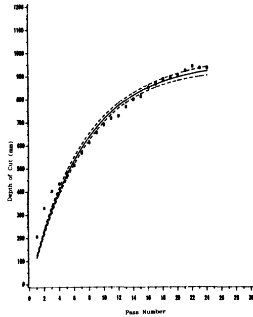
Figure 6.19 : Effect of Pass Number (Exposure) on Depth of Cut in Noctis
