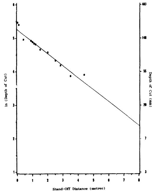
Figure 6.20 : Effect of Stand-off Distance on Depth of Cut in Noctis
