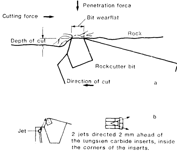
Figure 2.1 : Diagram of a Drag Bit Cutting the Rock illustrating the Components of the Bit Force and the Optimum Jet Position (after Riemann [11], Hood [12])
