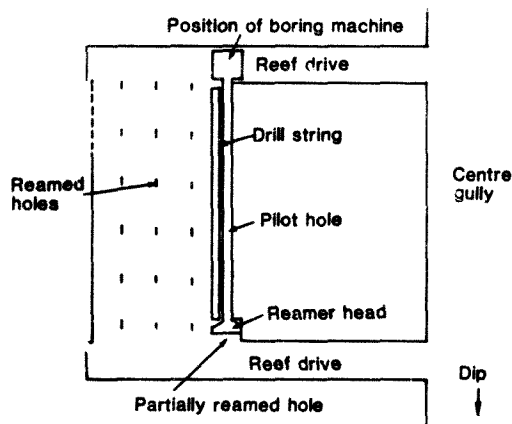
Figure 2.8 : Typical Position of Reef Borer
