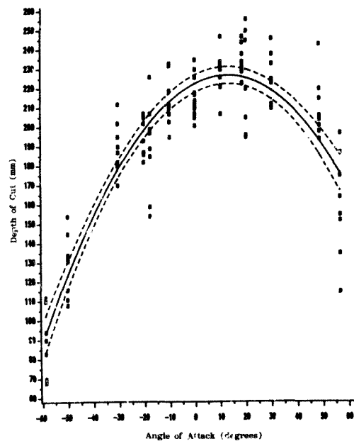
Figure 6.21 : Effect of Angle of Attack on Depth of Cut in Norite
