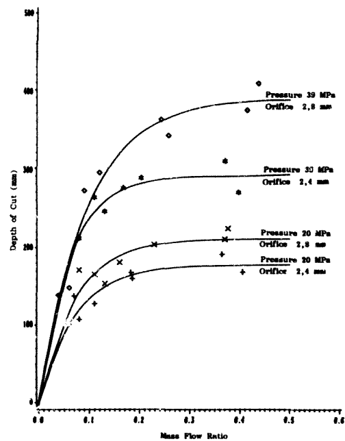
Figure 6.17 : Effect of MFR on Depth of Cut in Norite (second exposure)
