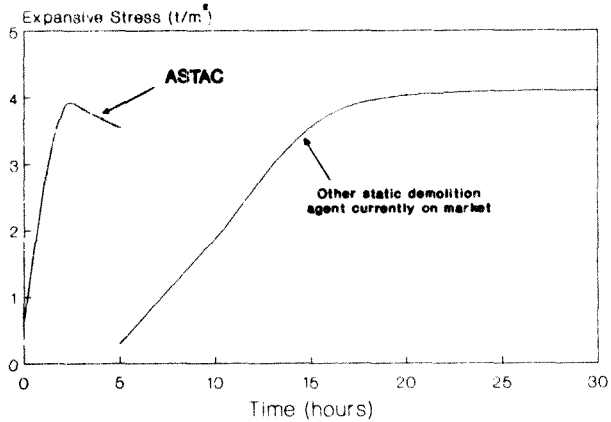
Figure 2.18 : Setting Behaviour of Expanding Cements
