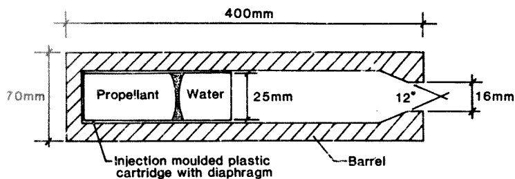
Figure 2.16 : CSIR Water Gun (Cannon)
