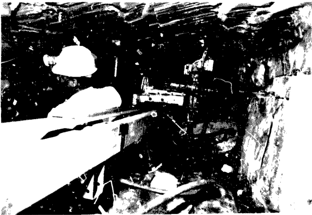
Figure 3.8 : Bullwedging Operation Underground (200 J Blow Energy at 1 490 Blows per Min.)
