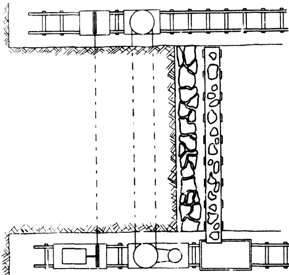
Figure 2.5 : Diamond Wire Saw (after Hatch [18])
