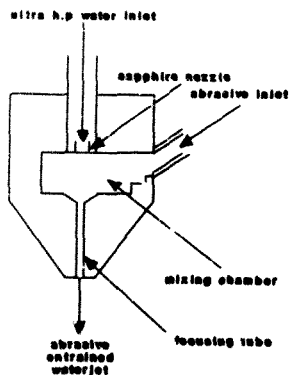
Dry Abrasive Waterjet Nozzle
