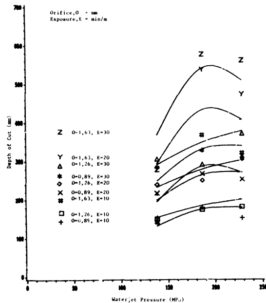
Figure 6.6 : The Effect of Water Pressure on Depth of Cut in Quartzite (High MPR Model)
