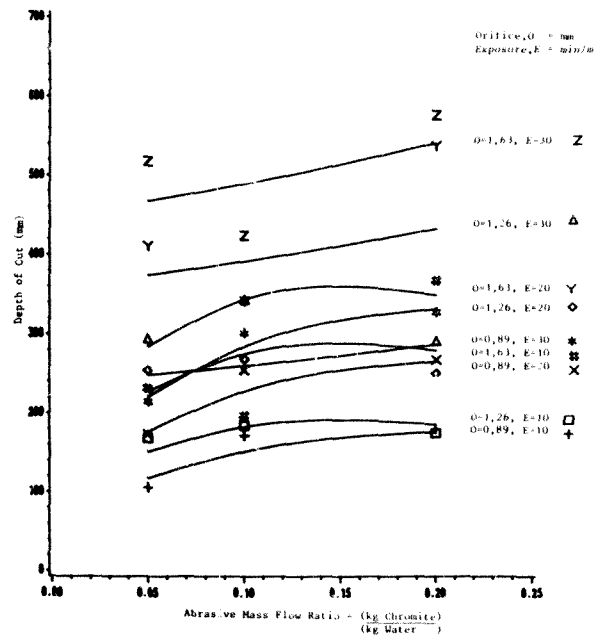
Figure 6.10 : The Effect of MPR on Depth of Cut in Quartzite (High MPR Range, Pressure = 100 MPa)
