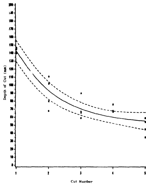
Figure 6.23 : Effect of Cut Number (number of times the abrasive is re-used) on Depth of Cut in Norite Using Chromite Abrasive
