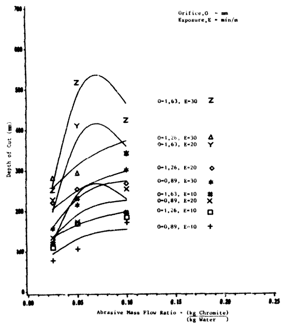
Figure 6.9 : The Effect of MPR on Depth of Cut in Quartzite (Low MPR Range, Pressure = 100 MPa)
