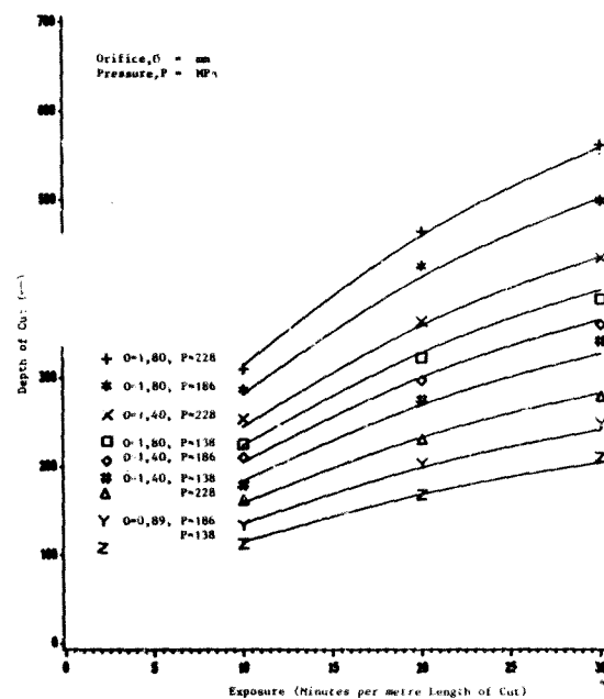
Figure 6.4 : The Effect of Exposure Time on Depth of Cut in Norite
