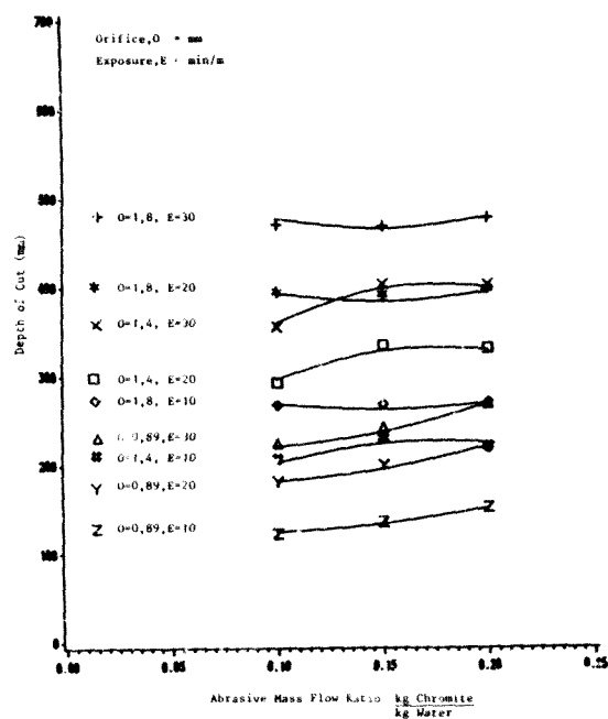
Figure 6.3 : The Effect of MFR on Depth of Cut in Norite
