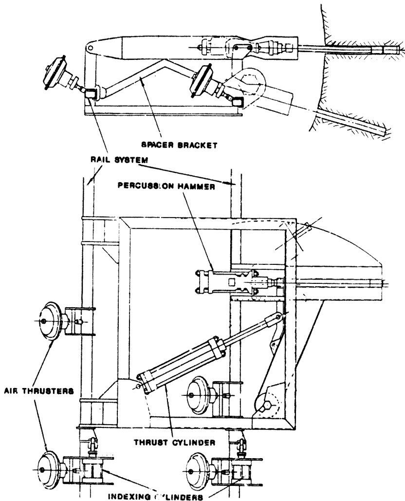
Figure 2.3 : The Board Radial Rockslotter
