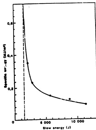
Figure 2.10 : Laboratory Drop Test Rig Results (after Haase et al [4])
