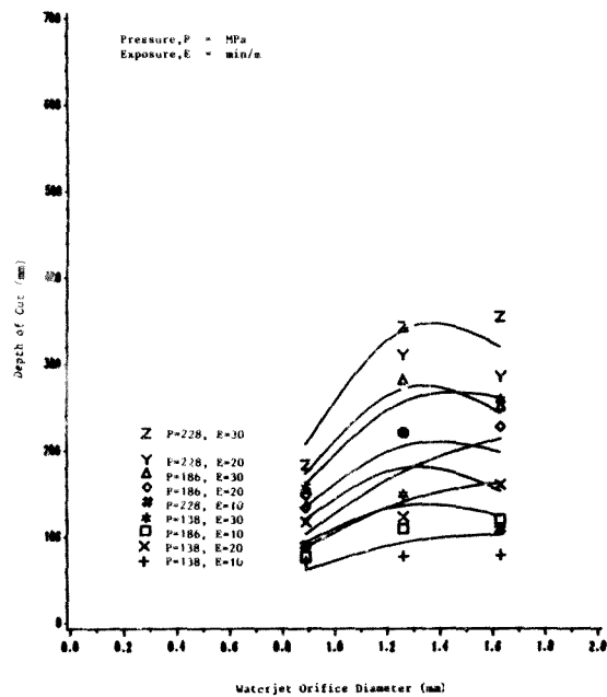
Figure 6.7 : The Effect of Orifice Size on Depth of Cut in Quartzite (Low MPF Model)
