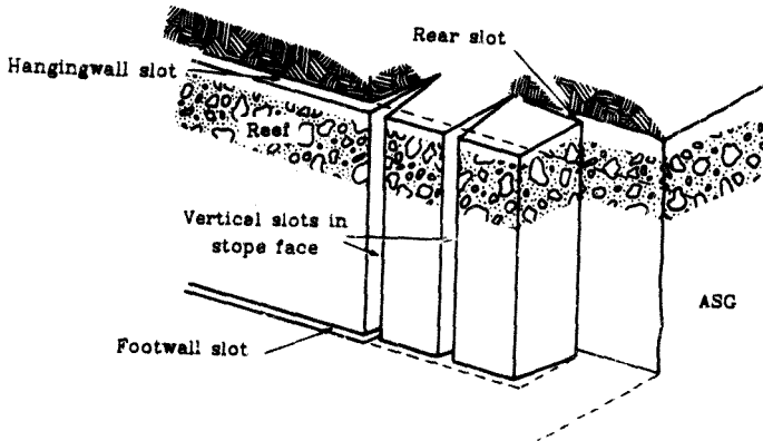
Figure 1.7 : Configuration of Slots for Block-Cutting Method
