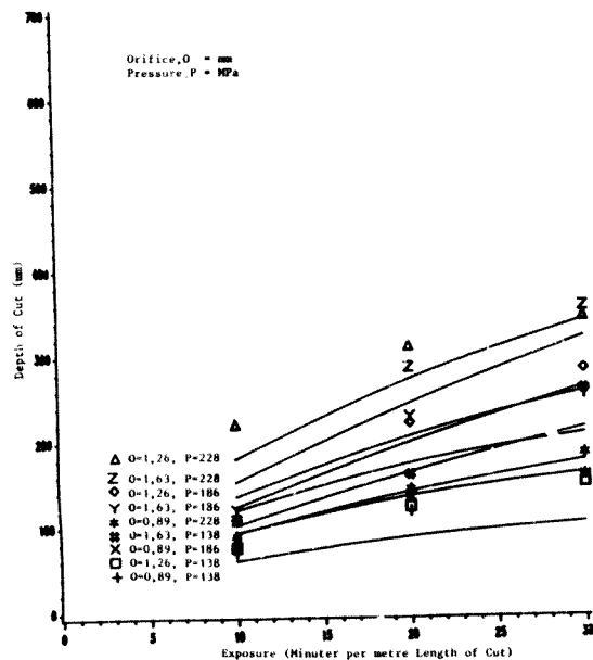
Figure 6.11 : The Effect of Exposure Time on Depth of Cut in Quartzite (Low MFR Model)
