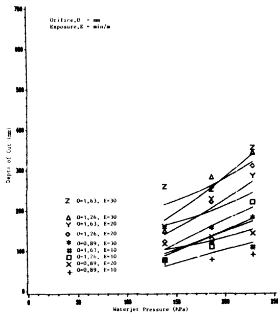
Figure 6.5 : The Effect of Water Pressure on Depth of Cut in Quartzite (Low MPR Model)
