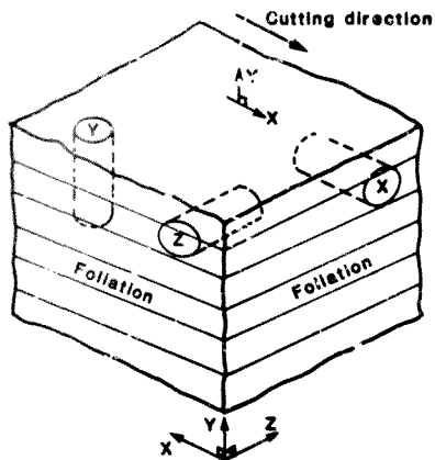
Figure 5.2 : Foliation and Weakness Planes of Norite
