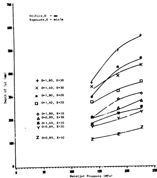
Figure 6.1 : The Effect of Water Pressure on Depth of Cut in Norite
