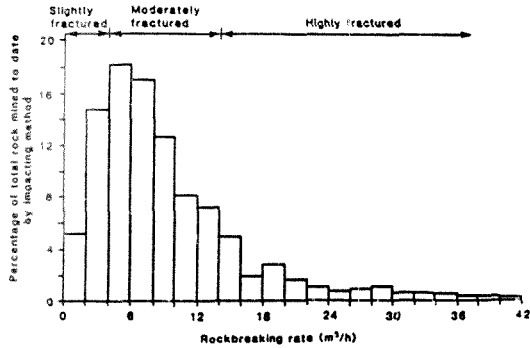
Figure 2.13 : Results Achieved with the Impact Ripper (after Spies [52])
