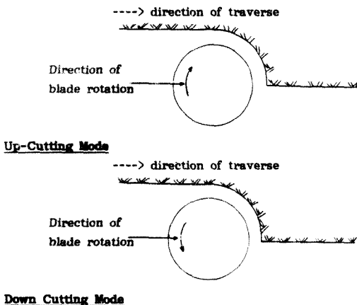
Figure 6.30: Schematic Illustration of Diamond Circular Saw Cutting Modes
