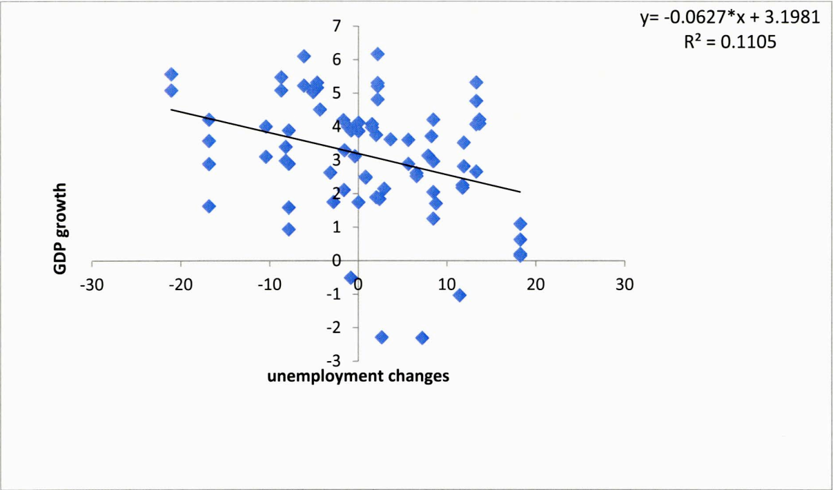
Chart 6.2: The difference version of Okun's law, age group 15-24
