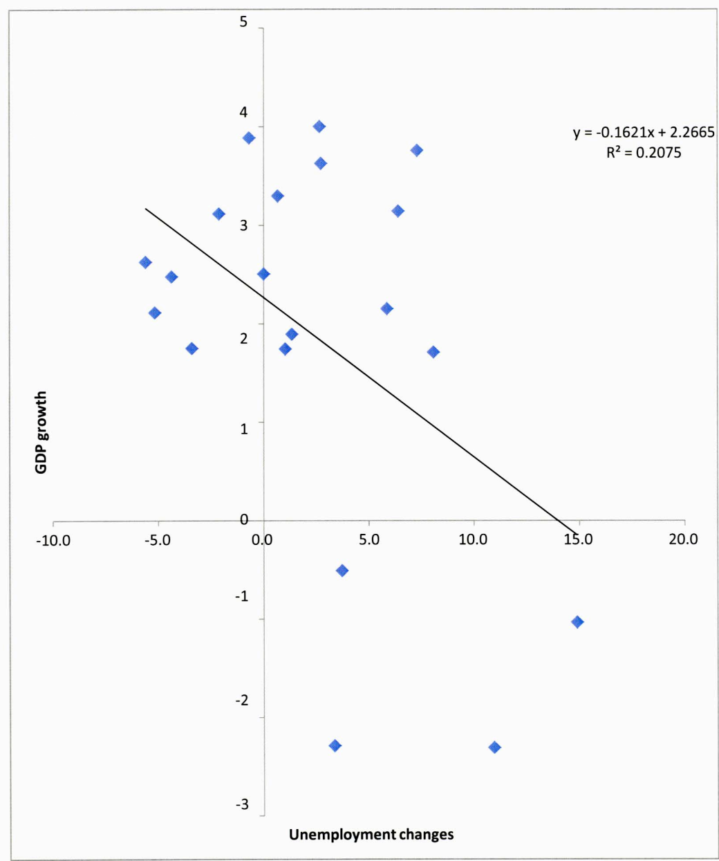
Chart 3: The difference version of Okun's law, age group 25-34
