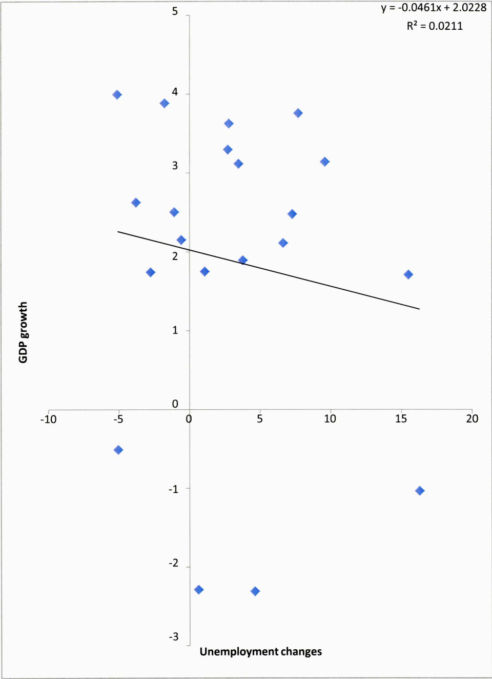
Chart 4: The difference version of Okun's law, age group 35-44
