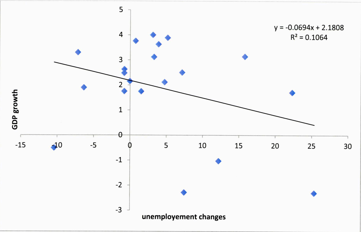
Chart 6.5: The difference version of Okun’s law, age group 45-54
