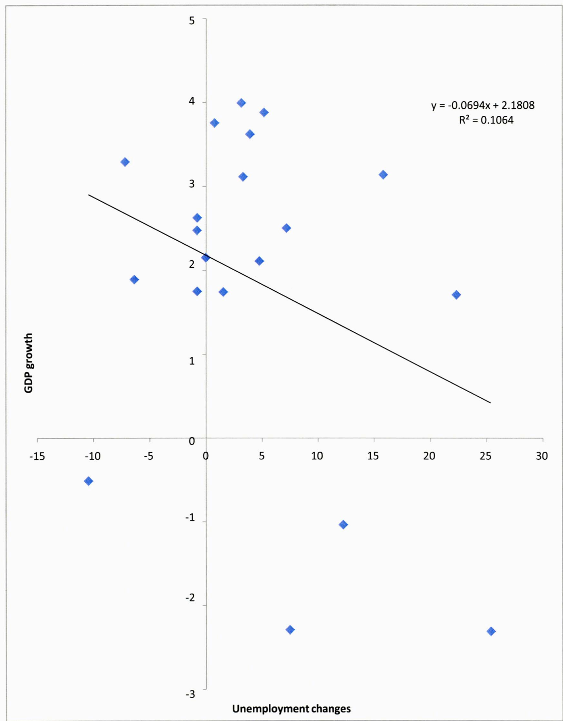
Chart 5: The difference version of Okun's law, age group 45-54
