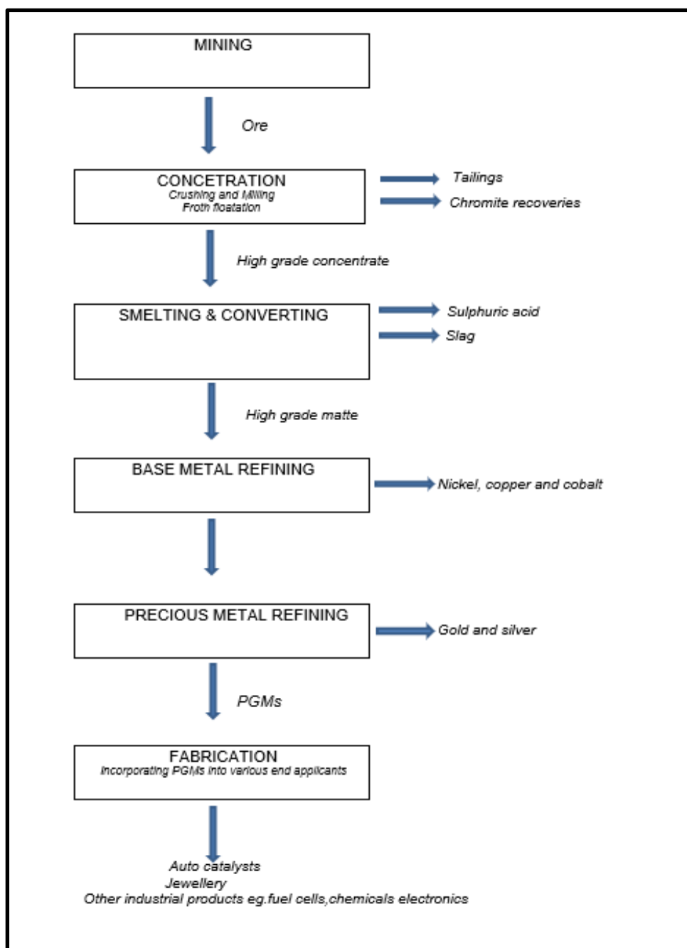
Figure 5.5: PGMs beneficiation flow diagram. (Source: Dube, 2016)
