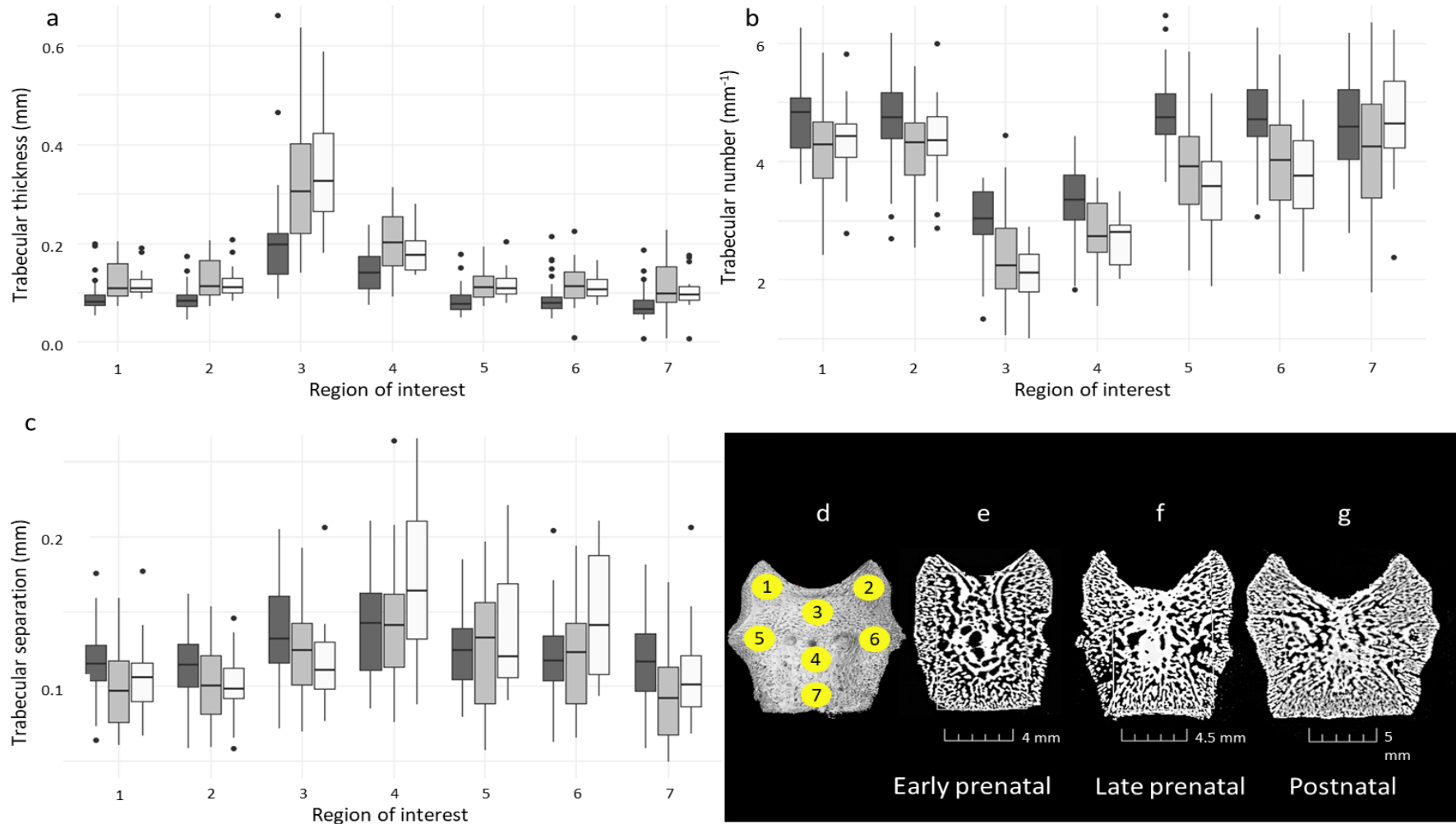
Figure 6: Regional variations of (a) trabecular thickness (TbTh), (b) trabecular number (TbN) and (c) trabecular separation (TbSp) in the pars basilaris. Dark grey: early prenatal (20–30 gestational weeks, n=28 ). Light grey: late prenatal (30–40 gestational weeks, n=31 ). White: postnatal (birth–7.5 months, n=25 ). Dots represent outliers. Regions of interest (ROI) are illustrated on (d) 3D reconstruction of the intracranial late prenatal pars basilaris. Yellow circles represent ROIs: (ROI 1): right anterolateral maxima of the foramen magnum. (ROI 2): left anterolateral maxima of the foramen magnum. (ROI 3): anterior foramen magnum border. (ROI 4): primary ossification site. (ROI 5): right lateral angle. (ROI 6): left lateral angle. (ROI 7): spheno-occipital synchondrosis. Differences in TbTh, TbN, TbSp are illustrated on the (e) early prenatal, (f) late prenatal, and (g) postnatal pars basilaris. Contrast and brightness have been adjusted to highlight trabeculae; therefore, the colour intensity is not representative of density. Graphs were created in RStudio using ggplot2 (Wickham, 2016). Images were generated using VGStudio Max V2.2 software (Volume Graphics GmbH, Heidelberg, Germany).
