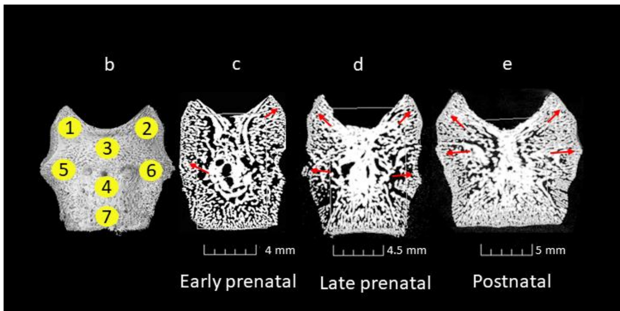
Figure 8: Regional variations of the degree of anisotropy (DA) in the pars basilaris. (a) Dark grey: early prenatal (20–30 gestational weeks, n=28). Light grey: late prenatal (30–40 gestational weeks, n=31). White: postnatal (birth–7.5 months, n=25). Dots represent outliers. Regions of interest (ROI) are illustrated (b) 3D reconstruction of the intracranial late prenatal pars basilaris. Yellow circles represent regions of interest (ROI): (ROI 1): right anterolateral maxima of the foramen magnum. (ROI 2): left anterolateral maxima of the foramen magnum. (ROI 3): anterior foramen magnum border. (ROI 4): primary ossification site. (ROI 5): right lateral angle. (ROI 6): left lateral angle. (ROI 7): spheno-occipital synchondrosis. Differences in DA are illustrated on the (c) early prenatal, (d) late prenatal and (e) postnatal pars basilaris. Red arrows represent the direction of the trabeculae in the anterolateral maxima (ROI 1 and ROI 2) and lateral angles (ROI 5 and ROI 6). Contrast and brightness have been adjusted to highlight trabeculae; therefore, the colour intensity is not representative of density. Graphs were created in RStudio using ggplot2 (Wickham, 2016). Images were generated using VGStudio Max V2.2 software (Volume Graphics GmbH, Heidelberg, Germany).
