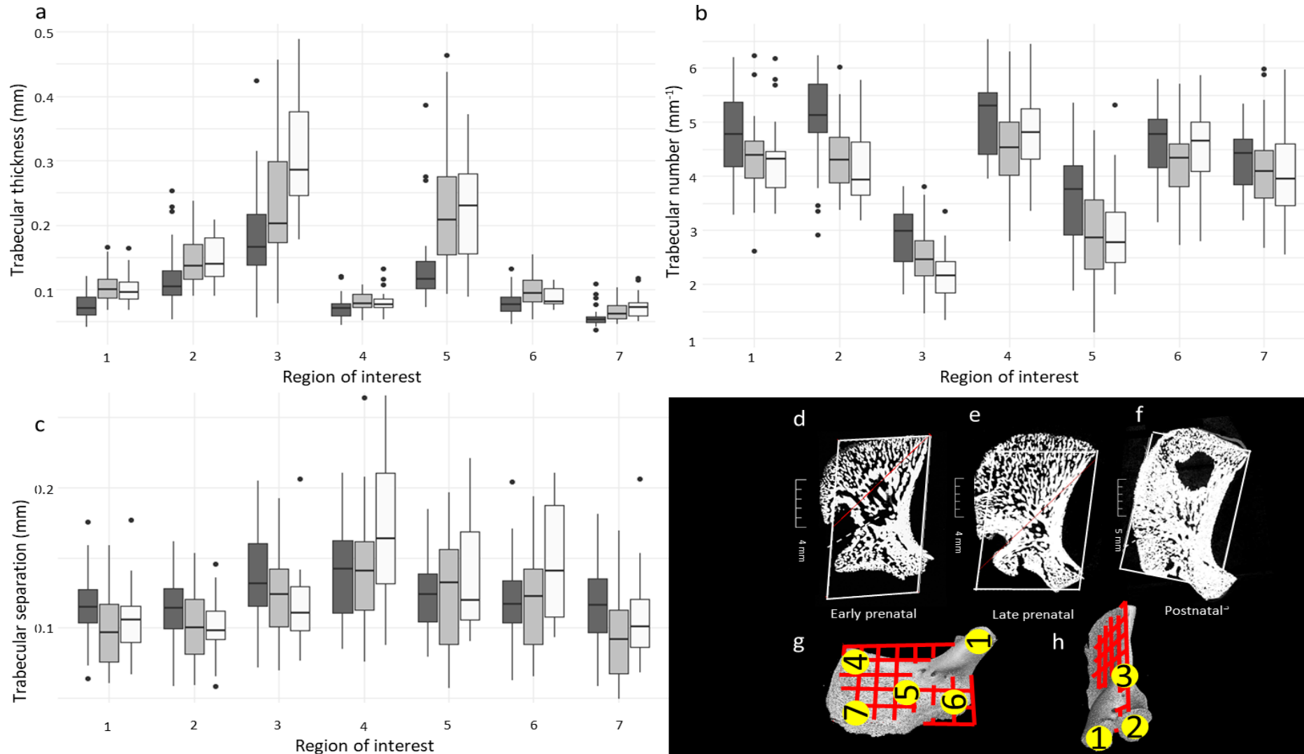
Figure 7: Regional variations of (a) trabecular thickness (TbTh), (b) trabecular number (TbN) and (c) trabecular separation (TbSp) in the pars lateralis. Dark grey: early prenatal (20–30 gestational weeks, n=30 ). Light grey: late prenatal (30–40 gestational weeks, n=37 ). White: postnatal (birth–7.5 months, n=29 ). Dots represent outliers. Differences in TbTh, TbN, TbSp are illustrated on the (d) early prenatal, (e) late prenatal and (f) postnatal pars lateralis. Contrast and brightness have been adjusted to highlight trabeculae; therefore, the colour intensity is not representative of density. Regions of interest (ROI) are illustrated on (g) 3D reconstruction of the intracranial late prenatal pars lateralis and (h) 3D reconstruction of the hypoglossal region of the late prenatal pars lateralis. Yellow circles represent ROIs: (ROI 1): jugular limb. (ROI 2): condylar limb. (ROI 3): lateral foramen magnum border. (ROI 4): posteromedial corner. (ROI 5): primary ossification site. (ROI 6): jugular process. (ROI 7): mastoid temporal border. Graphs were created in RStudio using ggplot2 (Wickham, 2016). Images were generated using VGStudio Max V2.2 software (Volume Graphics GmbH, Heidelberg, Germany).
