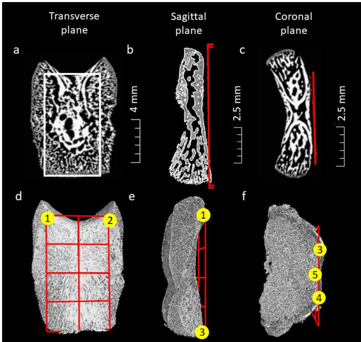
Figure 1: Reference planes for the pars basilaris: (a) Transverse view: white border represents reference plane. (b) Sagittal view: red line represents reference plane. (c) Coronal view: red line represents reference plane. (d) 3D reconstruction of the extracranial aspect of the early prenatal pars basilaris. (e) 3D reconstruction of lateral aspects of early prenatal pars basilaris. (f) 3D reconstruction of the spheno-occipital region of the early prenatal pars basilaris. Yellow circles represent landmarks: (landmarks 1 and 2): horns for the occipital condyle on the extracranial surfaces of the left and right posterior most projections of the pars basilaris. (landmarks 3 and 4): left and right anterior most projections on the extracranial surface of the spheno-occipital synchondrosis. (landmark 5): midline point on the extracranial spheno-occipital border. Images were generated using VGStudio Max V2.2 software (Volume Graphics GmbH, Heidelberg, Germany).
