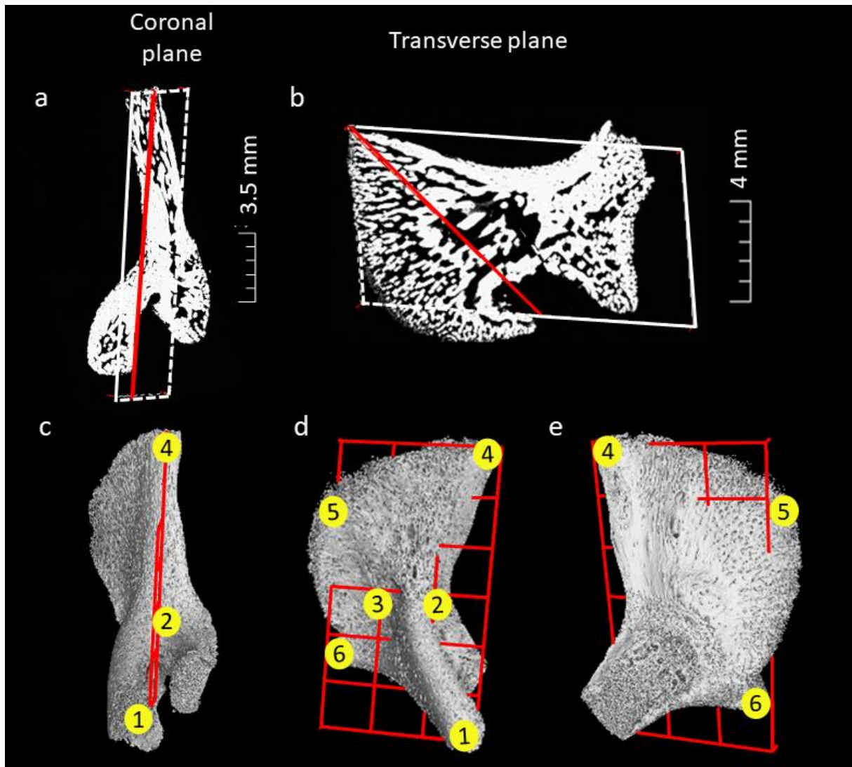
Figure 2: Reference planes for the pars lateralis: (a) Coronal view: white border and red line represent reference plane. (b) Transverse view: white border and red line represent reference plane. (c) 3D reconstruction of the hypoglossal region of the early prenatal pars lateralis. (d) 3D reconstruction of the intracranial aspect of the early prenatal pars lateralis. (e) 3D reconstruction of the extracranial aspect of the early prenatal pars lateralis. Yellow circles represent landmarks: (landmark 1): posterior border of the jugular limb. (landmark 2): angle on the medial border of the pars lateralis corresponding with the lateral borders of the foramen magnum. (landmark 3): primary ossification site on the intracranial surface. (landmark 4): posterior most corner on the medial border of the pars lateralis. (landmark 5): midline point on the mastoid temporal border. (landmark 6): immature jugular process. Images were generated using VGStudio Max V2.2 software (Volume Graphics GmbH, Heidelberg, Germany).
