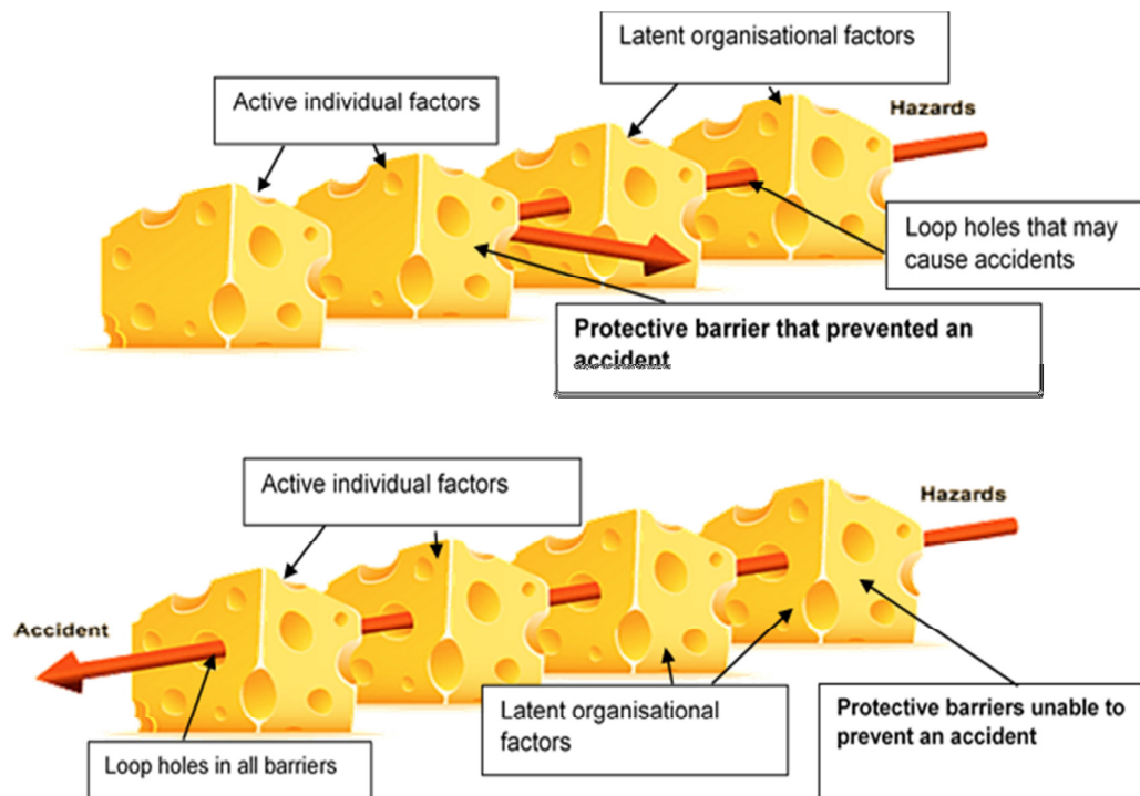
Figure 2: Swiss cheese model
