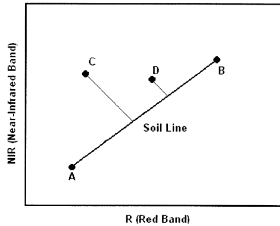
Figure 5: Soil line concept demonstrating the observed linear relationship between red (R) and near-infra-red (NIR) reflectance or image intensity of bare soil. The soil line extends from darker soils with low R and NIR image intensity (Point A) to an upper region of bright soils with high R and NIR image intensity (Point B). Point C represents a pure vegetation pixel and Point D represents a partially vegetated pixel (Fox and Sabbagh, 2002).
