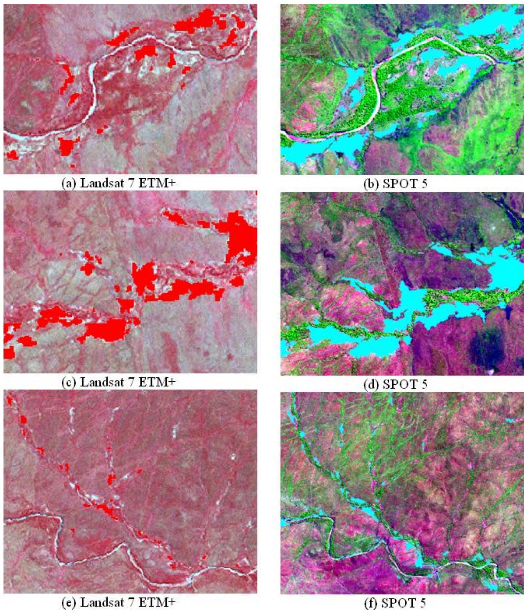
Figure 65: Spatial resolution comparison between the Landsat 7 ETM+ 30m multi-spectral (21 May 2001) and SPOT 5 10m multi-spectral (12 April 2008) late wet season to early dry season object-based classification of sodic sites.
