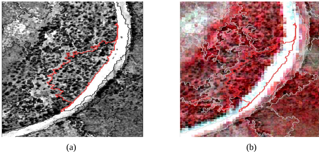
Figure 45: SPOT 5 panchromatic imagery segmentation (a) overlaid on ASTER multi-spectral imagery for the same river bed showing the pixel misalignment due to a georeferencing shift of approximately 40m.
