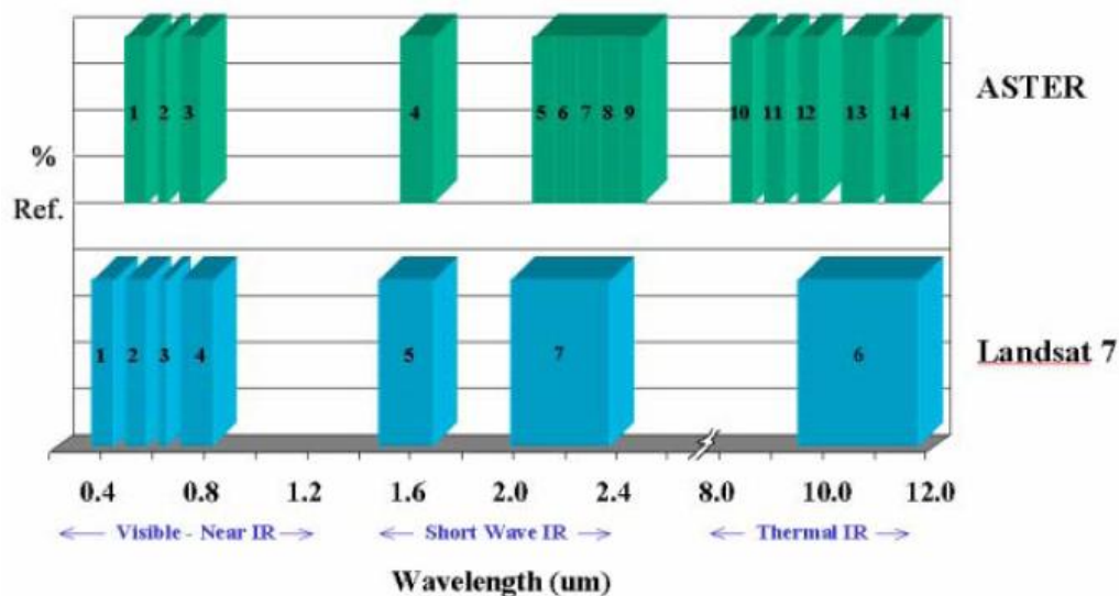
Figure 71: Comparison of Spectral Bands between ASTER and Landsat 7 ETM+ showing percentage reflectance per wavelength. 10
