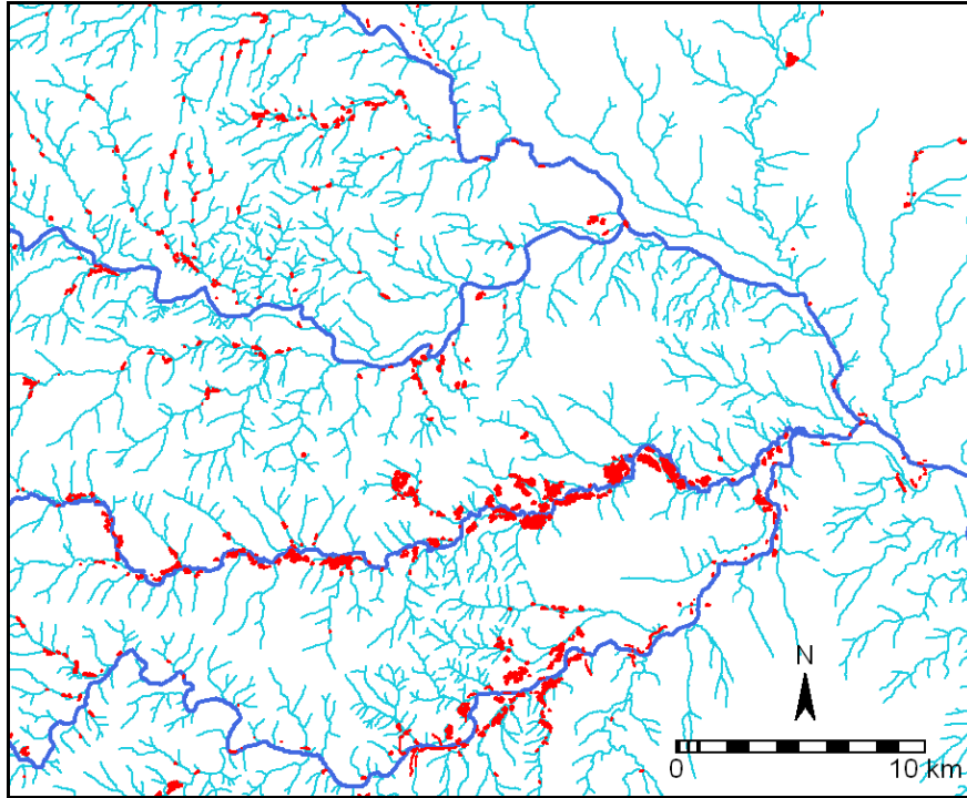
Figure 51: SPOT 5 (5 October 2005) classified sodic sites (red) showing the main Shingwedzi catchment rivers (blue) and tributaries (light blue). Area of sodic sites = 9.28 km 2 out of 1202.86 km 2 total area = 0.77 % cover.
