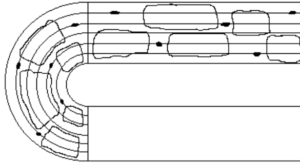
Figure 17: An outline illustrating lamellate tunnels in transverse (semi-circular image) and longitudinal section (horizontal image) (Redrawn from Hackett (1981)).
