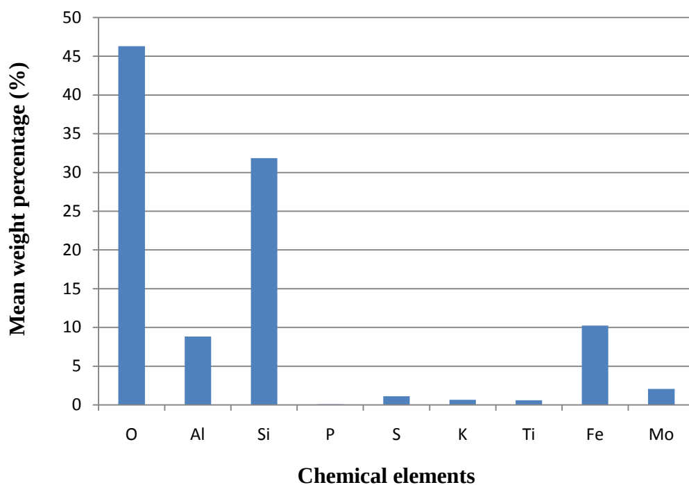
Figure 39: Bar graph illustrating the chemical composition of the soil from the Crown Mines.
