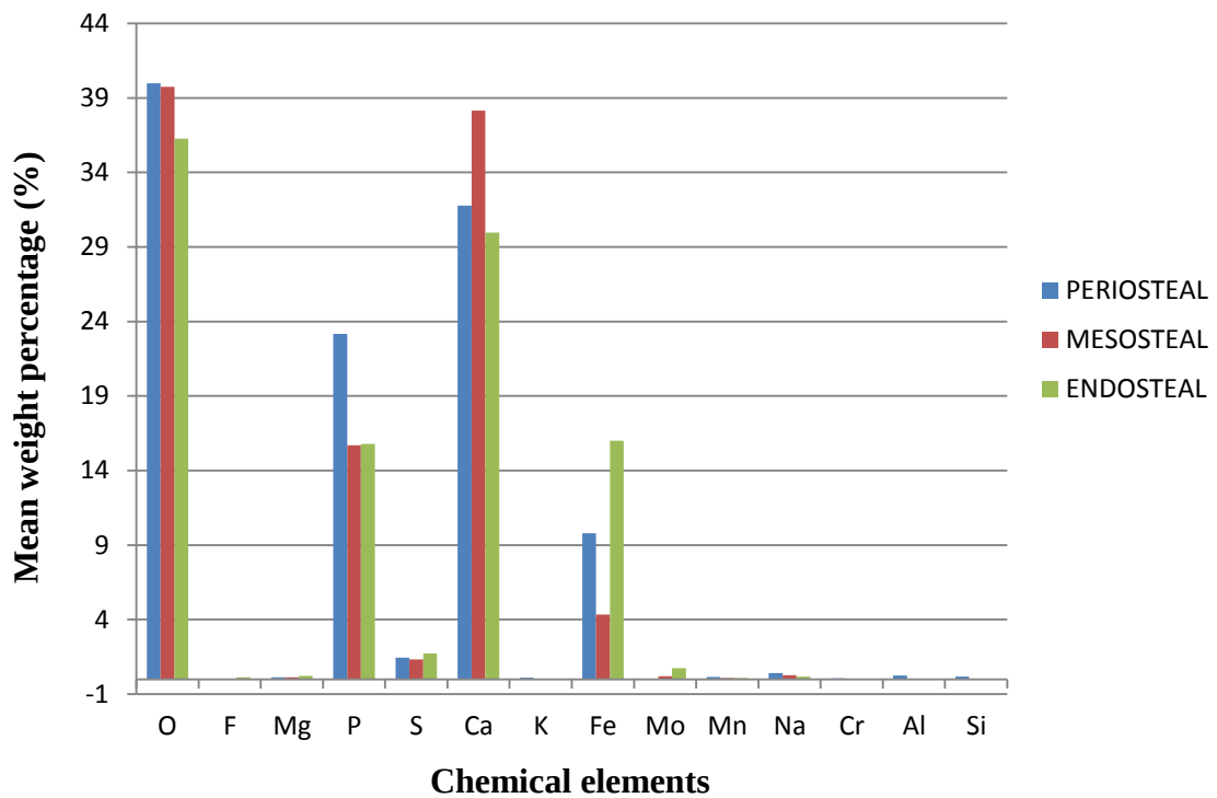
Figure 37: Bar graph displaying the chemical composition of the periosteal, mesosteal and endosteal zones of the bone samples acquired from the Crown Mines.
