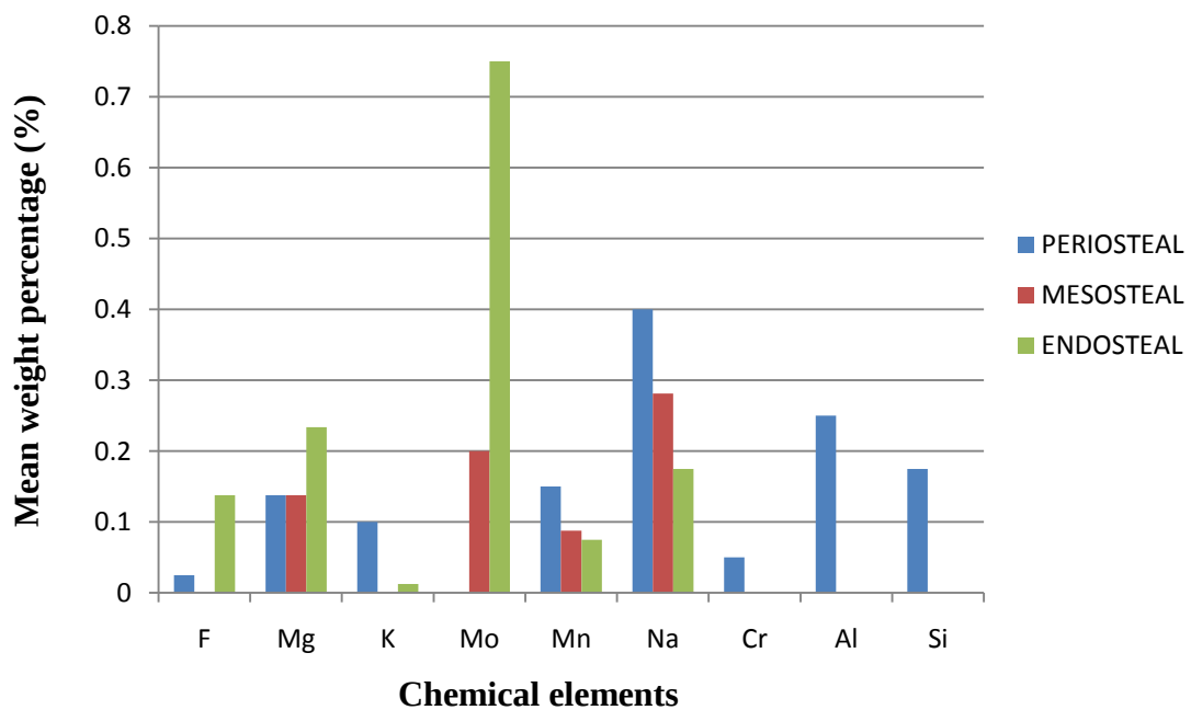
Figure 38: Bar graph displaying the trace elements contributing to the chemical composition of the Crown Mines bone samples.
