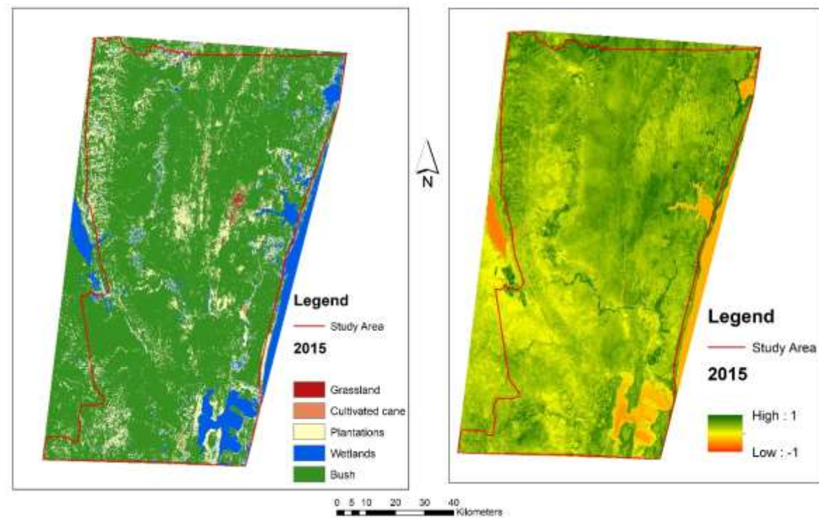
Landsat imagery and NDVI for winter 2015
