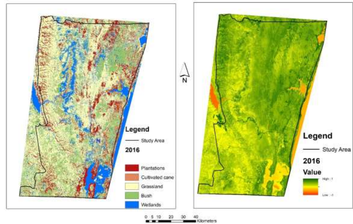
Landsat imagery and NDVI for winter 2016
