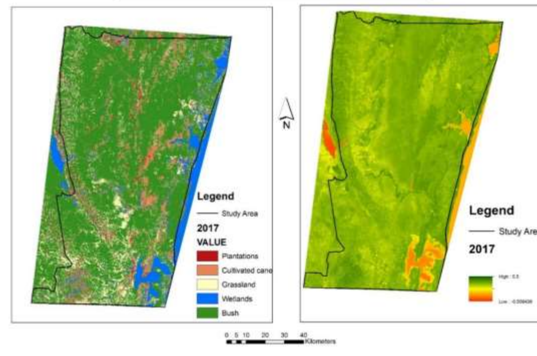
Landsat imagery and NDVI for winter 2017
