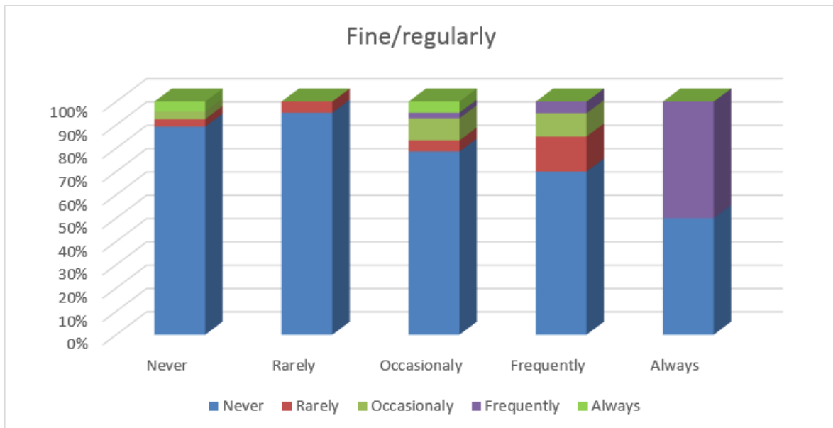
Histogram 11: Fine/regularly
