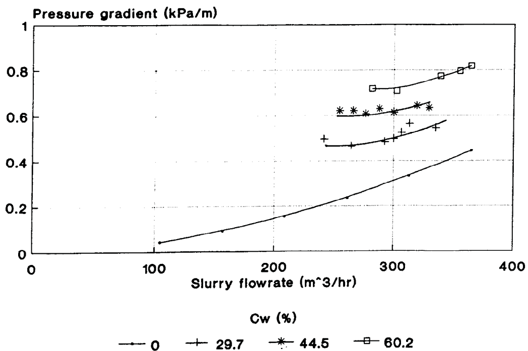
Fig 9.12 Tails 15 Friction Gradients (Rubber)
