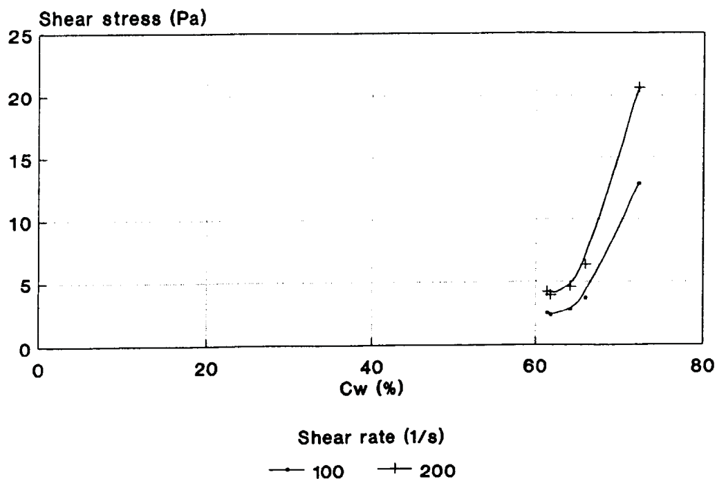
Figure 9.9 Constant shear rate diagram
