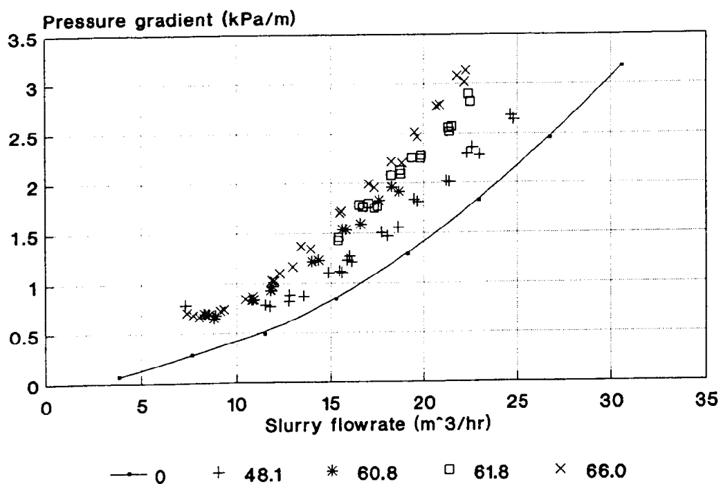
Figure 9.3 Slurry friction gradients ( D = 52\text{mm} )
