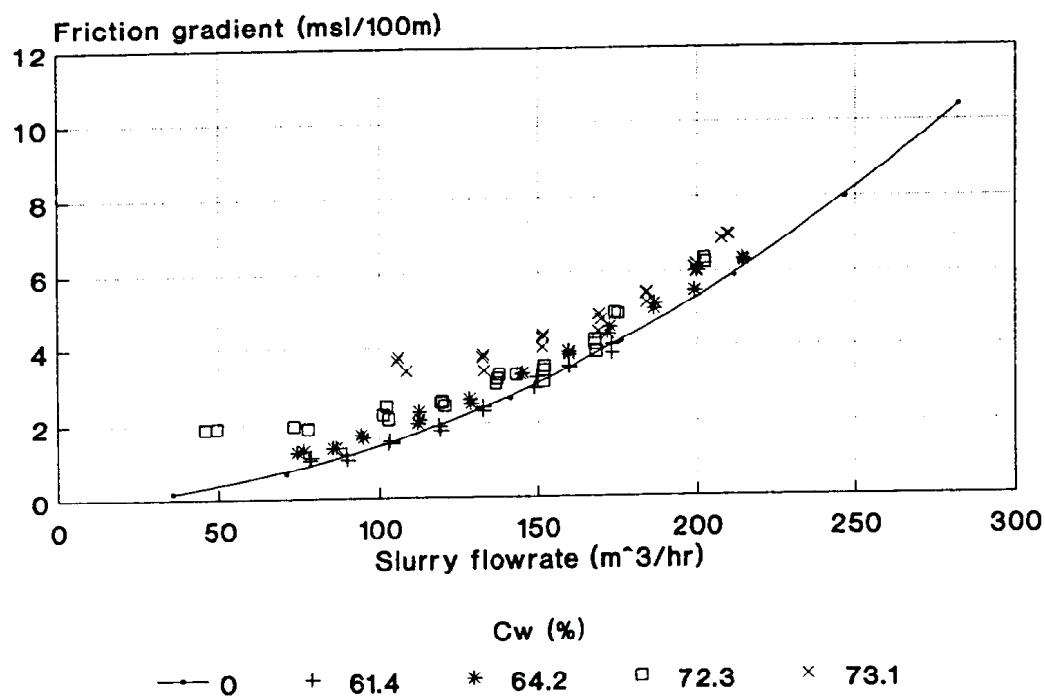
Figure 9.6 Slurry friction gradients (D = 158mm)
