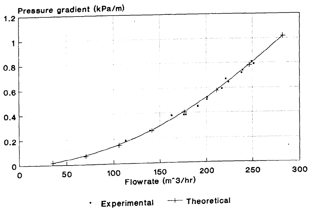
Figure 9.2 Clean water friction gradients ( D = 158\text{mm} )
