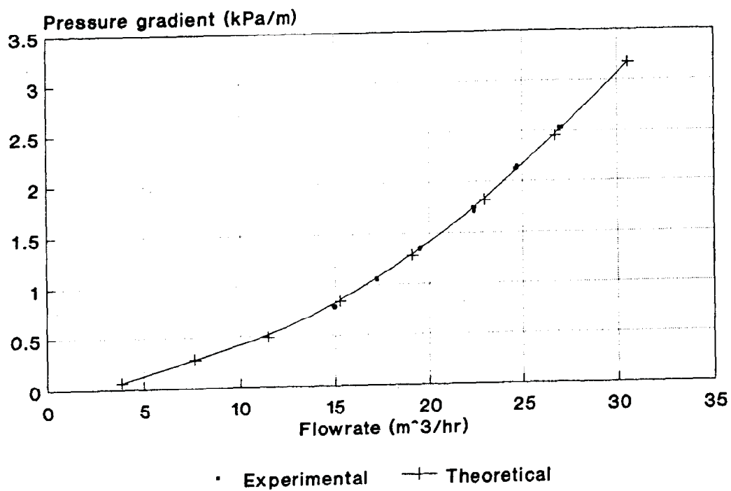
Figure 9.1 Clean water friction gradients ( D = 52\text{mm} )
