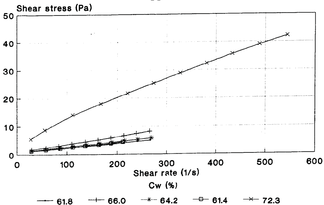
Figure 9.8 Comparative tailings 14 slurry rheogram
