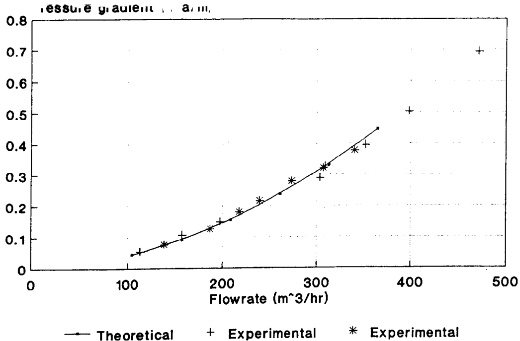
Fig. 9.10 Clean water friction gradients for the rubber lined pipeline (ID = 192mm)
