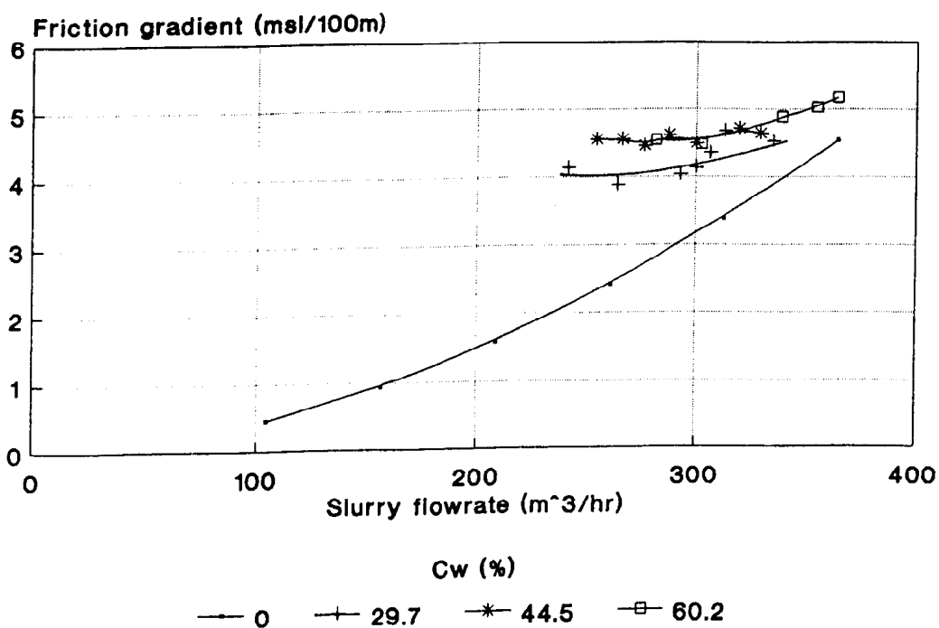
Fig. 9.13 Tails 15 Friction Gradients (Rubber)
