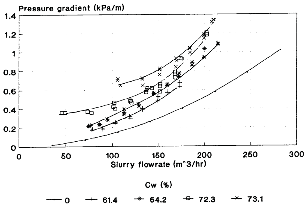
Figure 9.5 Slurry friction gradients (D = 158mm)
