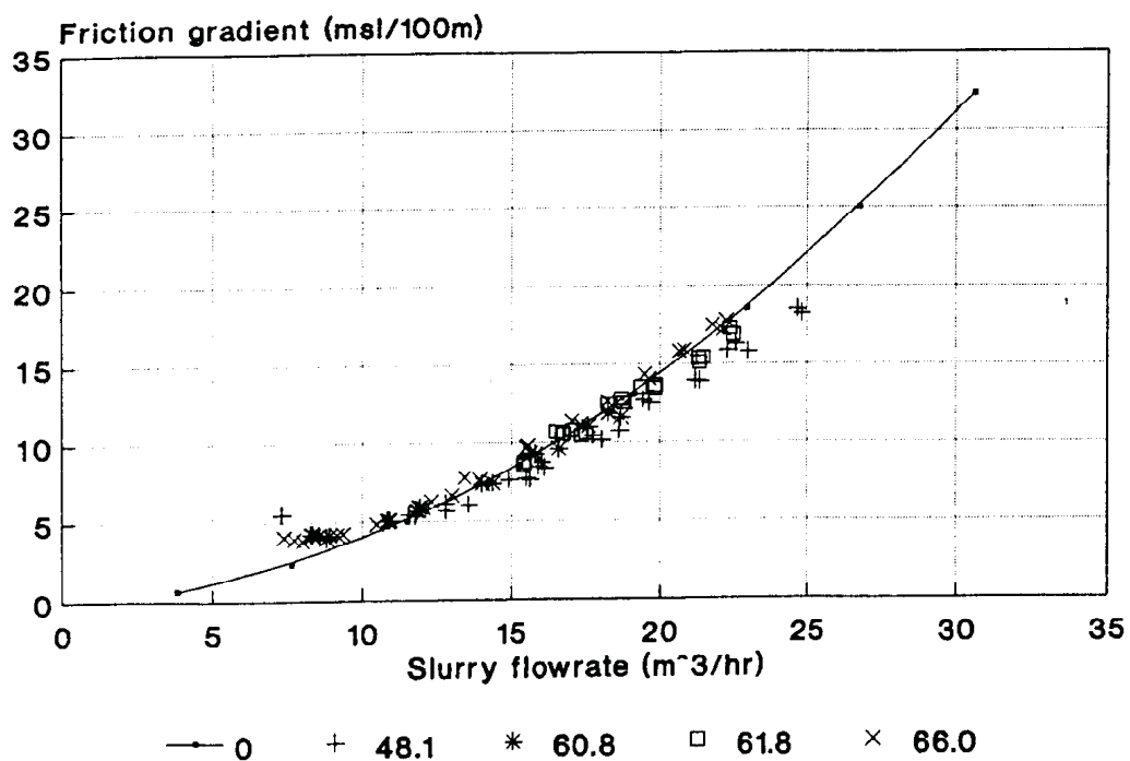
Figure 9.4 Slurry friction gradients ( D = 52\text{mm} )
