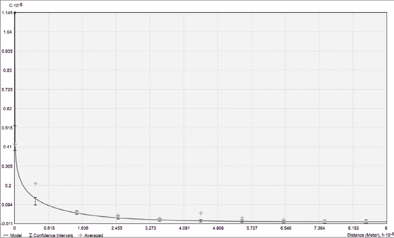
Figure 4: Variogram of the 1996 unemployment data.
