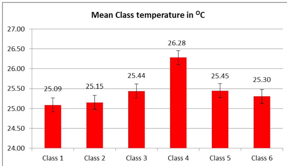
Figure 4.7 - Mean temperature in °C per patch class, with Std. error bars
