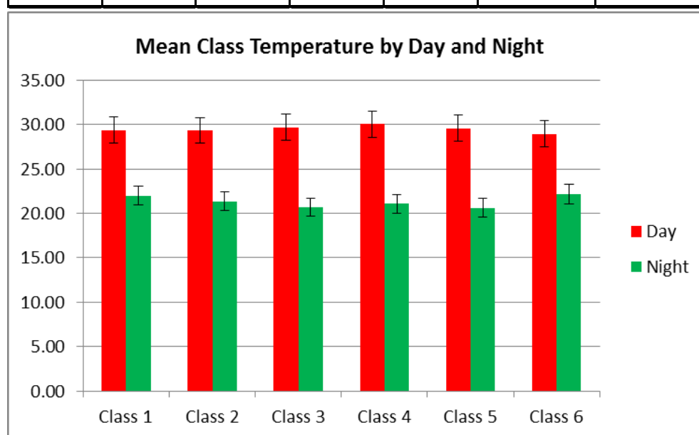
Figure 4.8 - Mean class temperature, by Day and by Night, with Std. error bars
