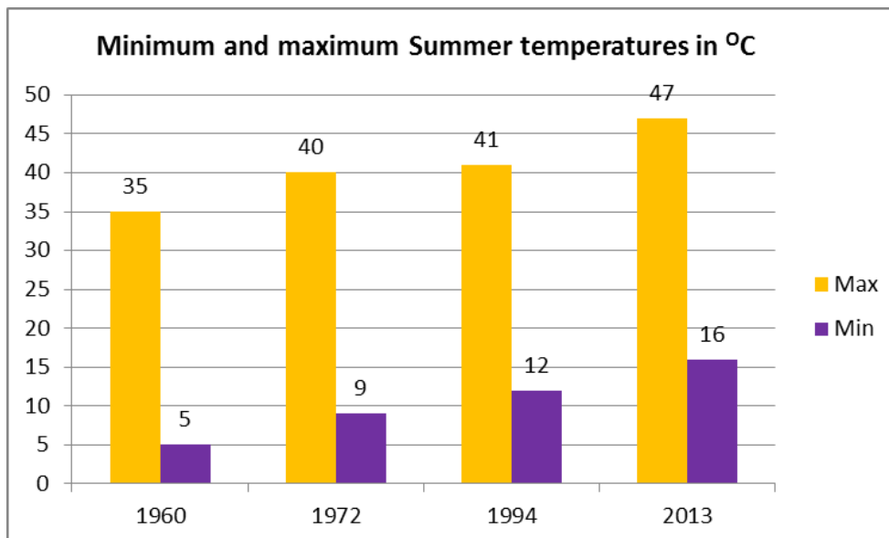
Figure 4.10 - Illustration of the trend in minimum and maximum summer temperatures in the Central Kalahari in °C, as reported in the literature from 1960 to 1994, and the current study
