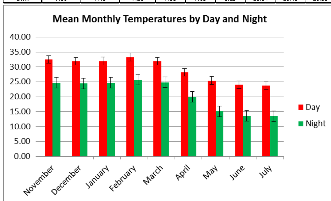
Figure 4.9 - Mean monthly temperature in °C, by Day and by Night, with Std. error bars
