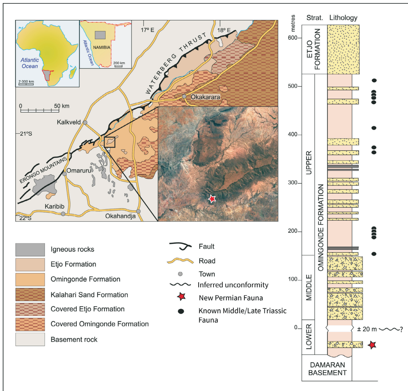
Figure 1. A, Geological map of outcrop and sub-outcrop of Omingonde and Etjo formations in the study area with satellite image of Mount Etjo showing the locality of the new Permian fauna (starred). B, Generalized stratigraphy and known tetrapod fossil localities from the exposures at the southern end of Mount Etjo. Section from Smith & Swart (2002) was measured close to the new Permian fossil locality (starred).
