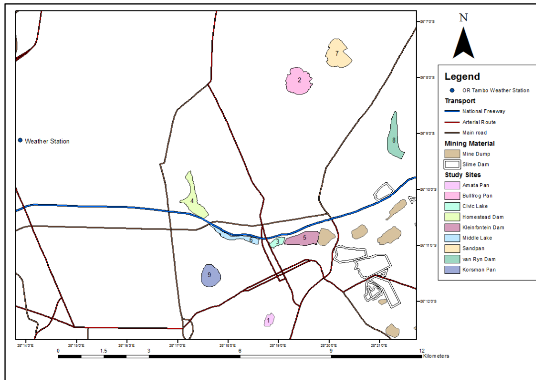
Figure 3.27: Map showing the relation of the O.R. Tambo Weather Station to the study sites
