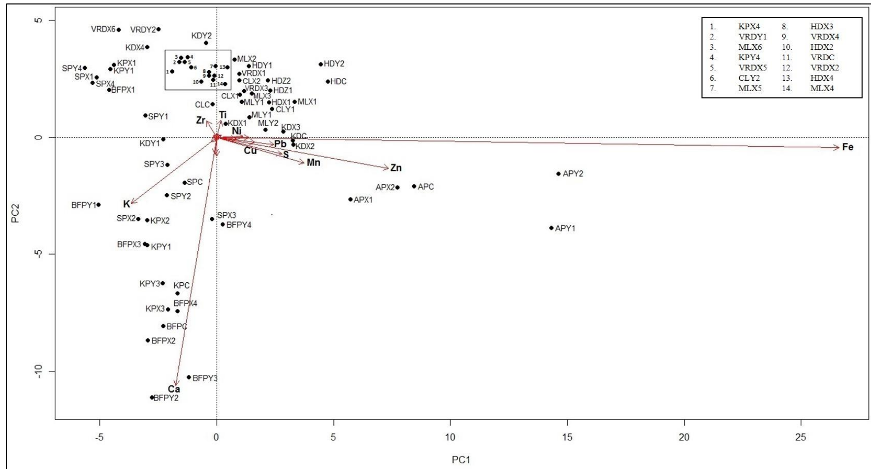
Figure 4.13: The PCA expressing the relationship of individual samples across the entire research area
