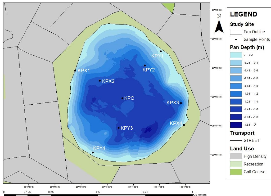
Figure 4.4: Bathymetric Map of Korsman Pan
