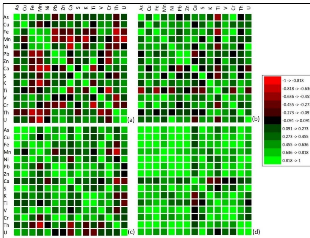
Figure 4.37: Image representation of the correlation matrix done for the relationship between trace elements analysed from various sediment samples for the four dams that fall along the same river gradient (a. Homestead Dam; b. Middle Lake; c. Civic Lake; d. Kleinfontein Dam)
