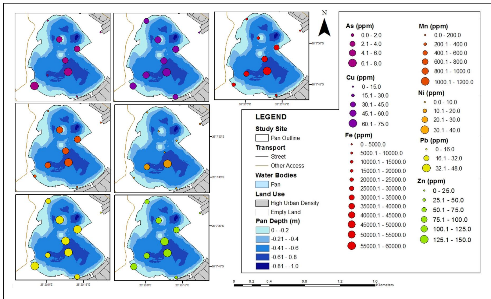
Figure 4.19: Spatial distribution of 7 trace metal concentrations across Sandpan
