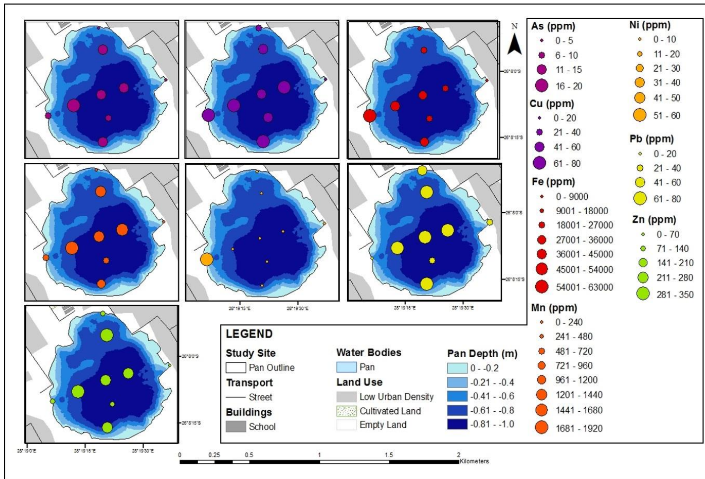
Figure 4.18: Spatial distribution of 7 trace metal concentrations across Bullfrog Pan
