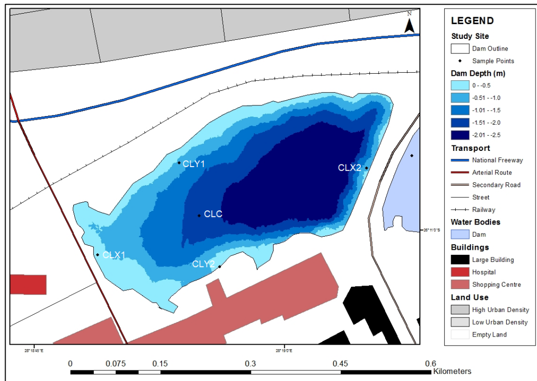
Figure 4.5: Bathymetric Map of Civic Lake
