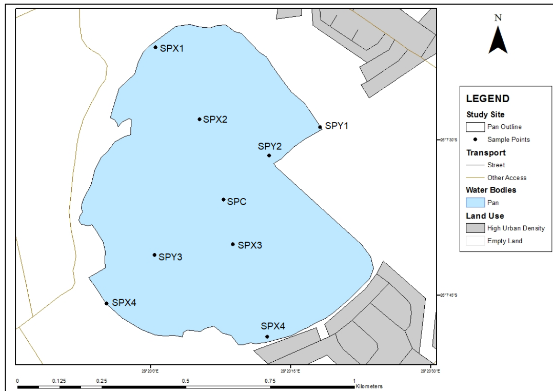
Figure 3.8: Map showing Sandpan and relative sample points within the site
