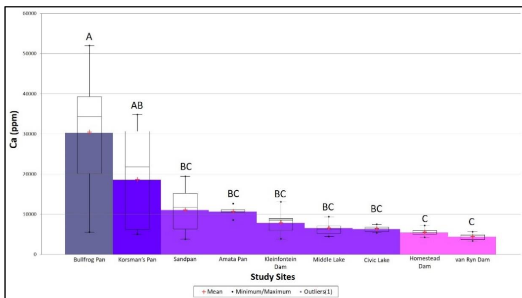
Figure 4.26: The ANOVA plot comparing each site to each other based on mean Ca concentrations.
