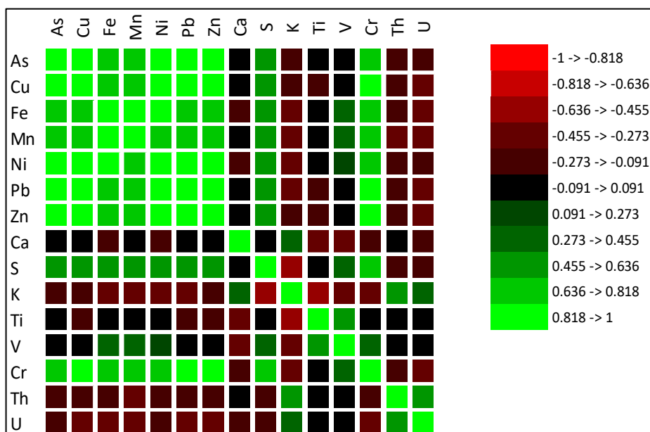
Figure 4.35: An image representation of the correlations matrix for trace element concentrations from sediment samples across the entire region
