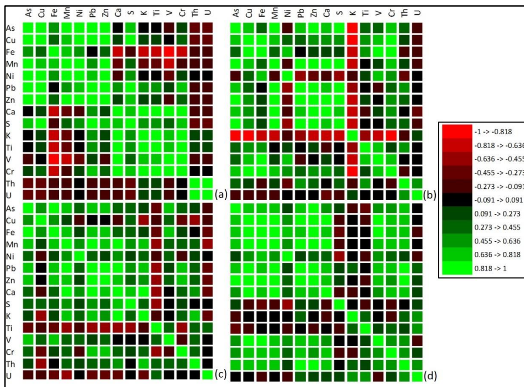
Figure 4.36: An image representation of multiple correlation matrices for trace element concentrations from across the four pans (a. Amata Pan; b. Bullfrog Pan; c. Korsman Pan; d. Sandpan)
