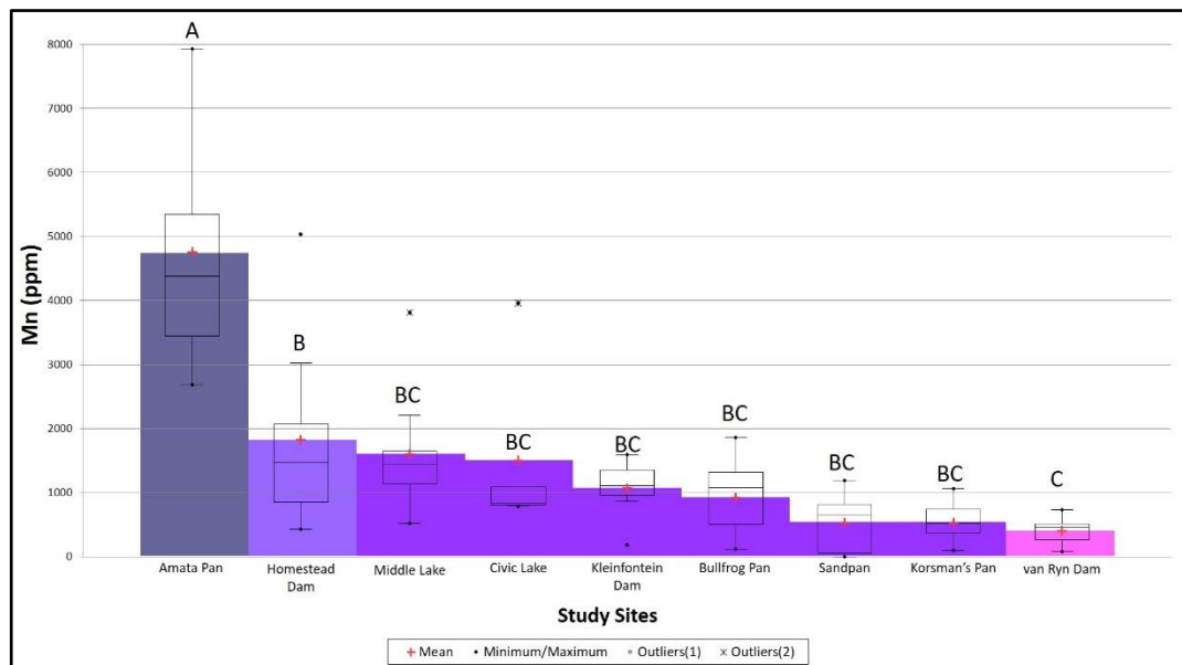
Figure 4.30: The ANOVA plot comparing each site to each other based on mean Mn concentrations.
