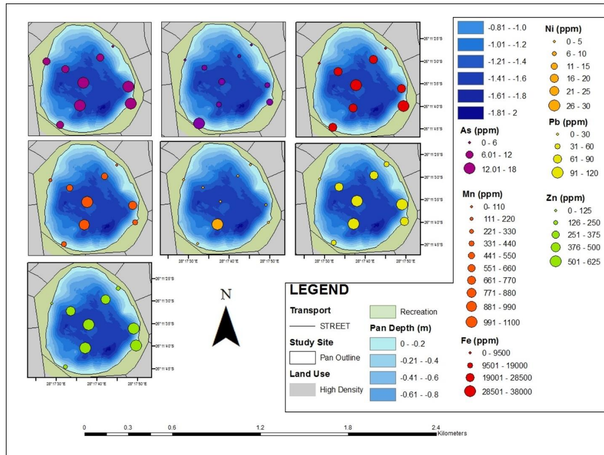
Figure 4.17: Spatial distribution of 7 trace metal concentrations across Korsman Pan
