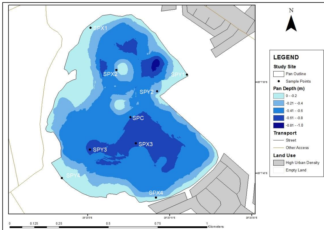
Figure 4.3: Bathymetric Map of Sandpan
