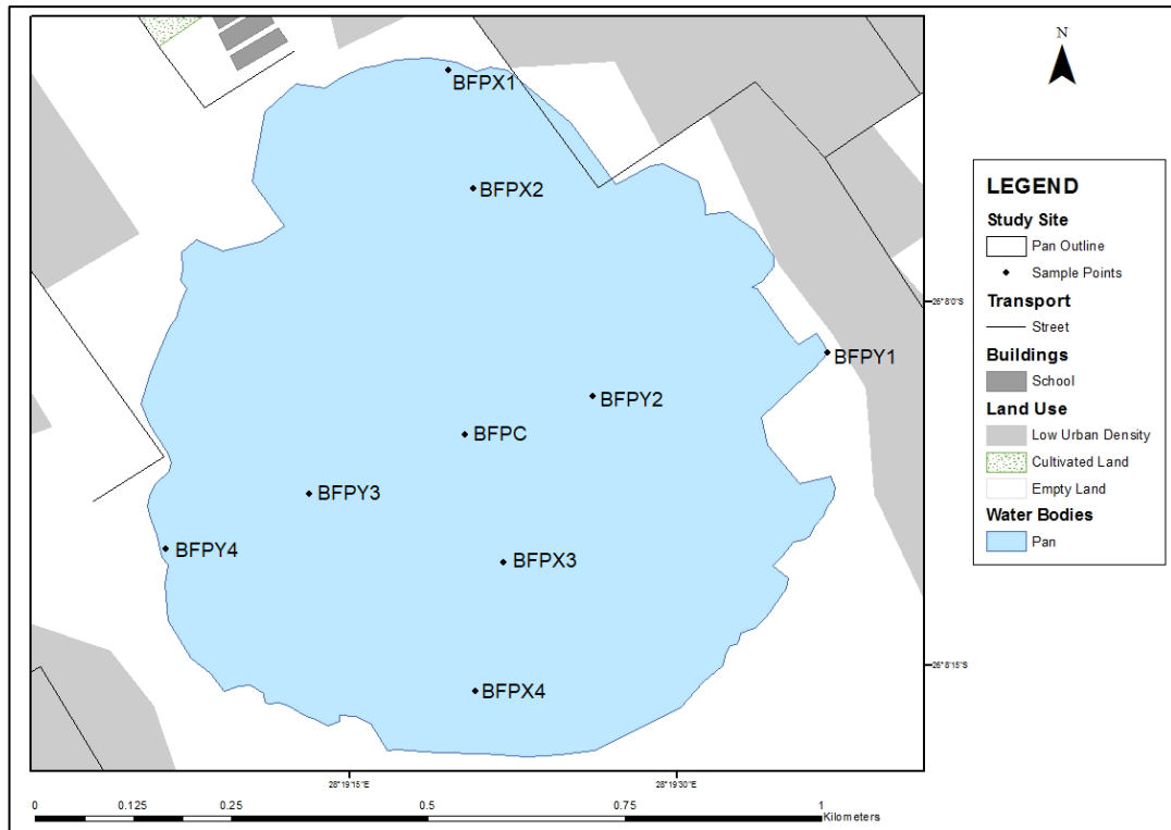
Figure 3.5: Map showing Bullfrog Pan and relative sample points within the site
