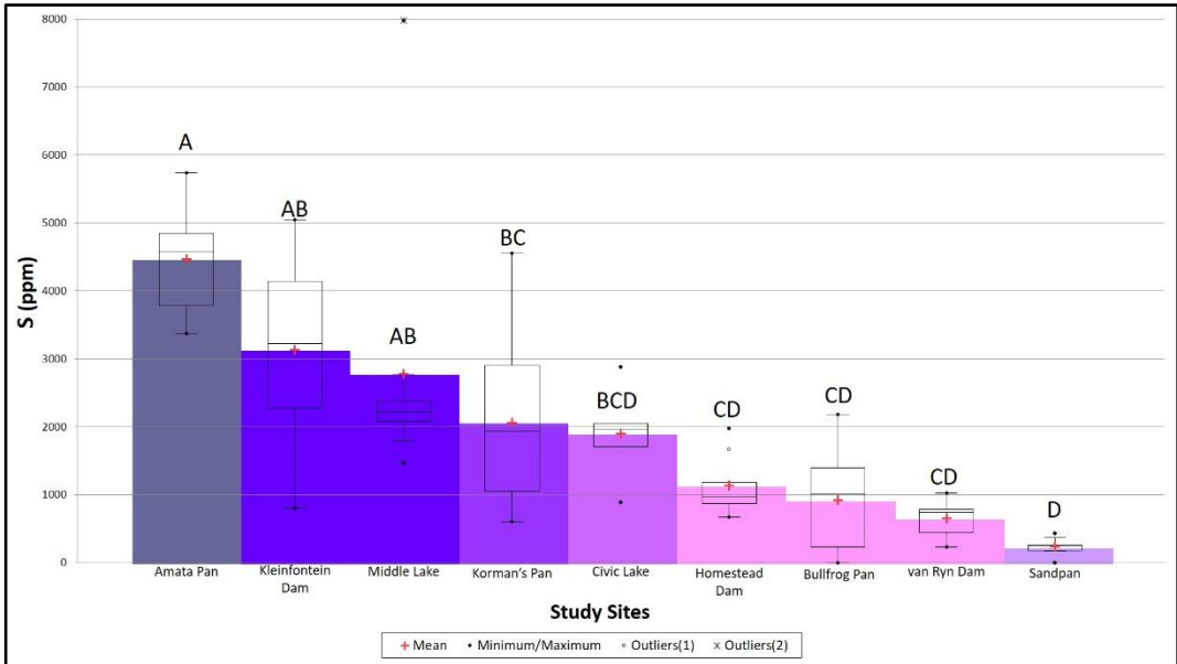
Figure 4.32: The ANOVA plot comparing each site to each other based on mean S concentrations.
