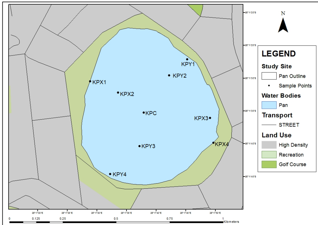
Figure 3.2: Map showing Korsman's Pan and relative sample points within the site
