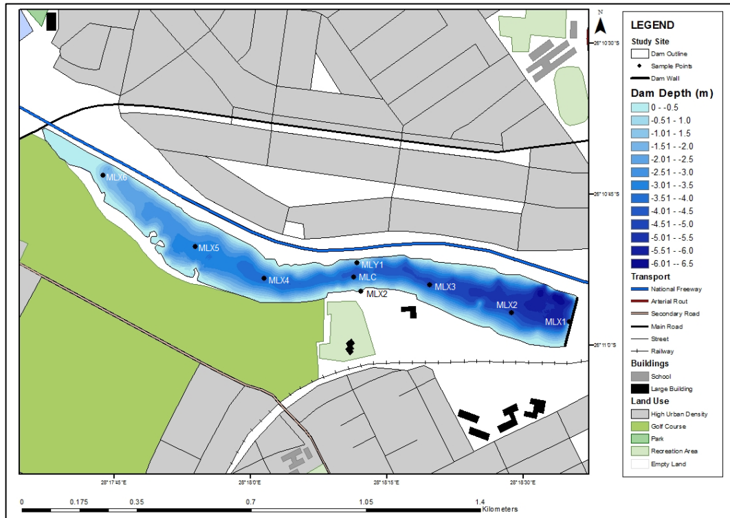
Figure 4.8: Bathymetric Map of Middle Lake
