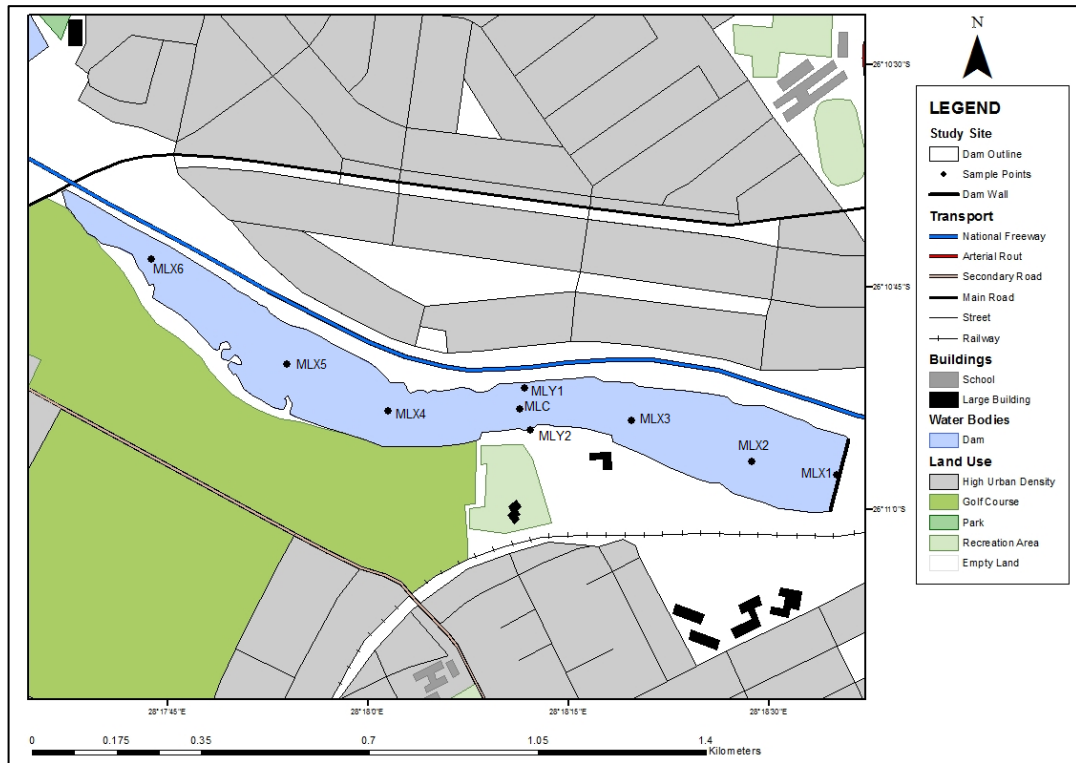
Figure 3.12: Map showing Middle Lake and relative sample points within the site
