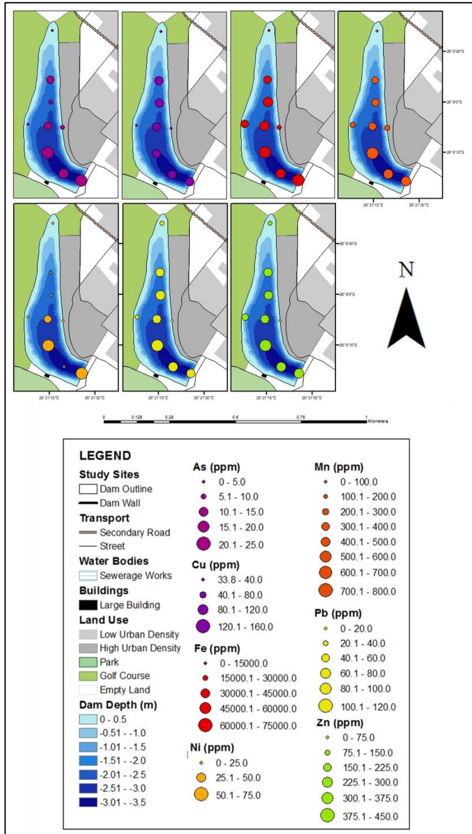
Figure 4.24: Spatial distribution of 7 trace metal concentrations across van Ryn Dam
