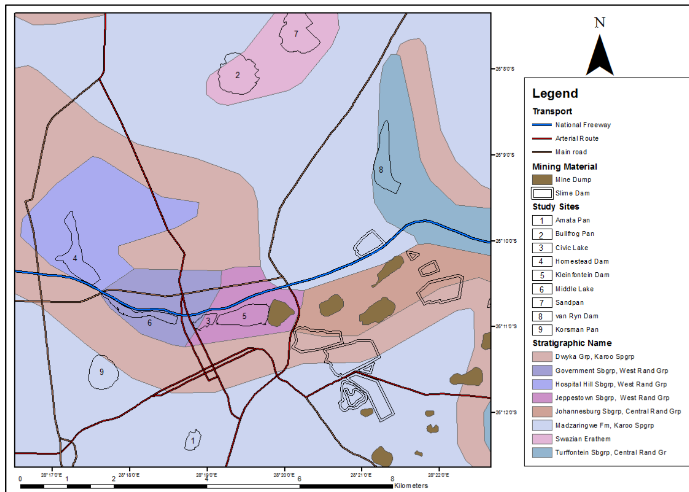
Figure 1.4: Geologic Map of the Benoni Area, and subsequent study sites
