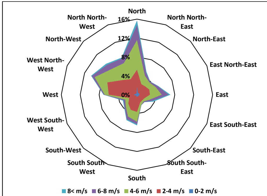
Figure 4.11: Wind rose diagram comparing the average wind speed and direction for 2017
