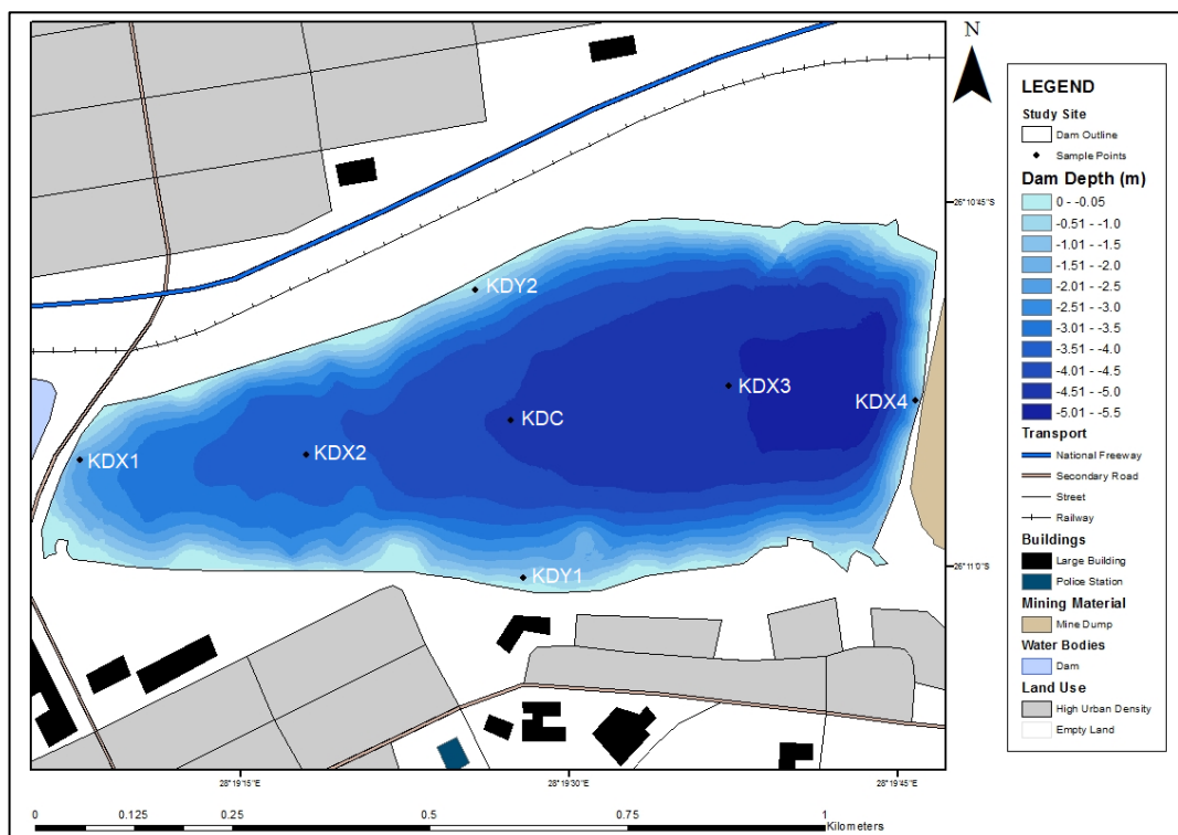
Figure 4.7: Bathymetric Map of Kleinfontein Dam
