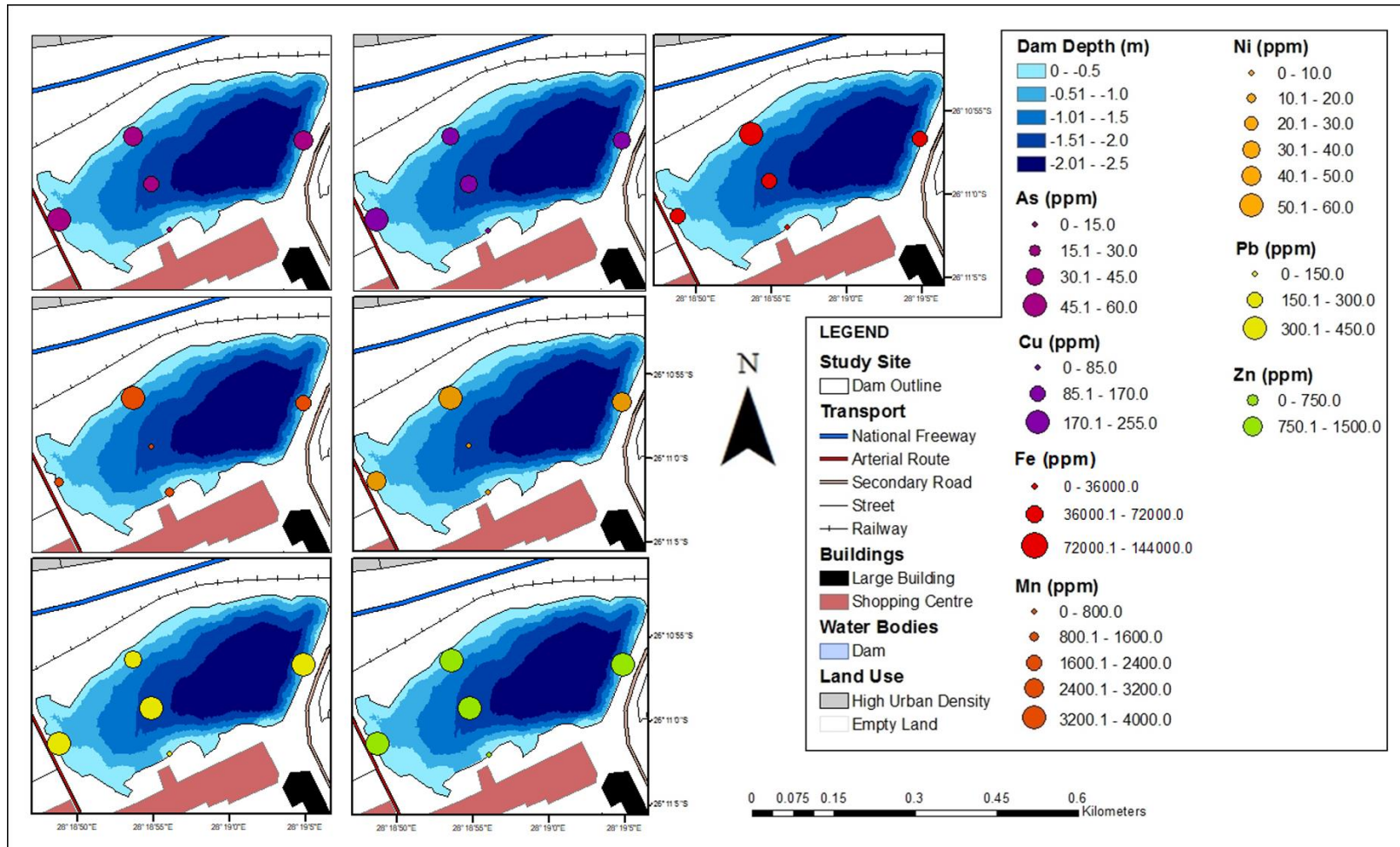
Figure 4.22: Spatial distribution of 7 trace metal concentrations across Civic Lake
