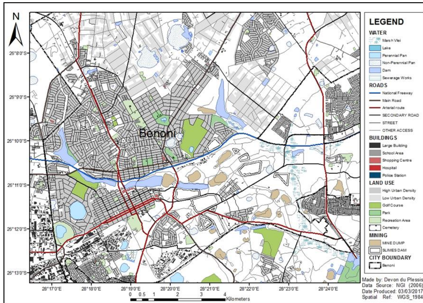
Figure 1.2: Detailed base map of the City of Benoni, Ekurhuleni
