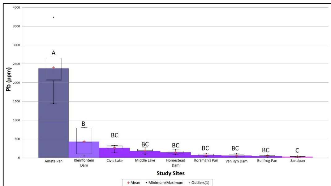
Figure 4.31: The ANOVA plot comparing each site to each other based on mean Pb concentrations.
