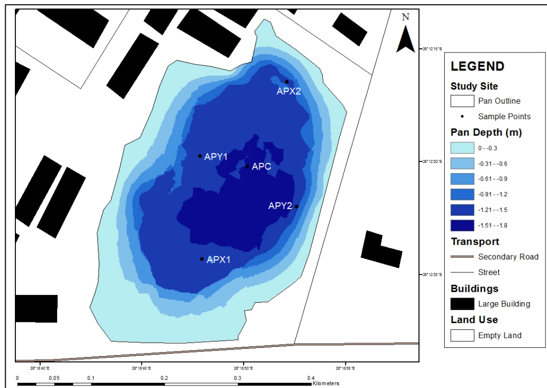
Figure 4.1: Bathymetric Map of Amata Pan
