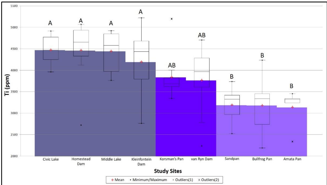
Figure 4.33: The ANOVA plot comparing each site to each other based on mean Ti concentrations
