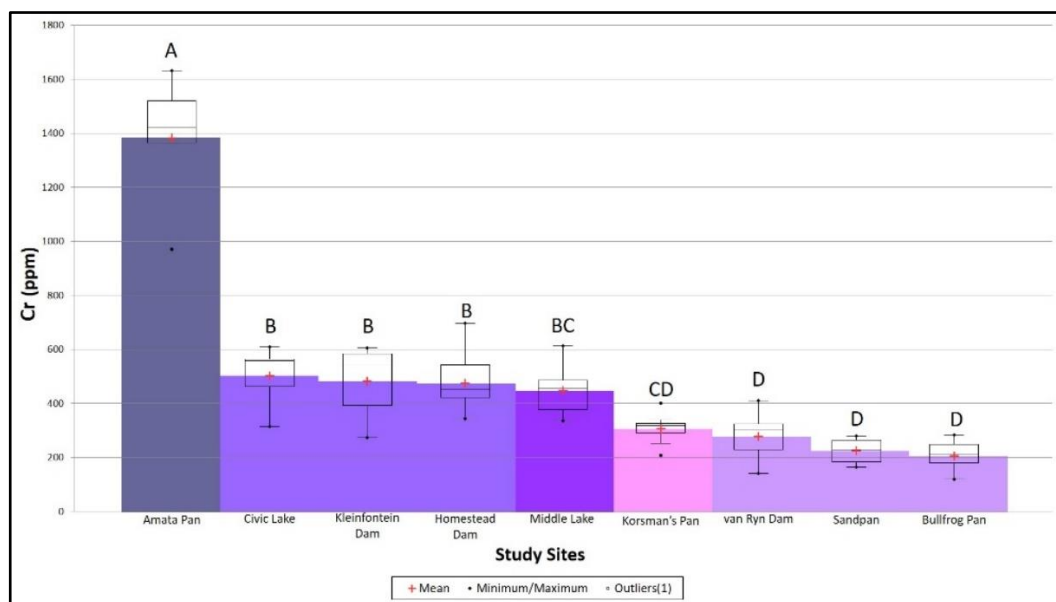
Figure 4.27: The ANOVA plot comparing each site to each other based on mean Cr concentrations.
