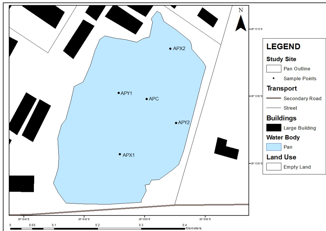
Figure 3.2: Map showing Amata Pan and relative sample points within the site
