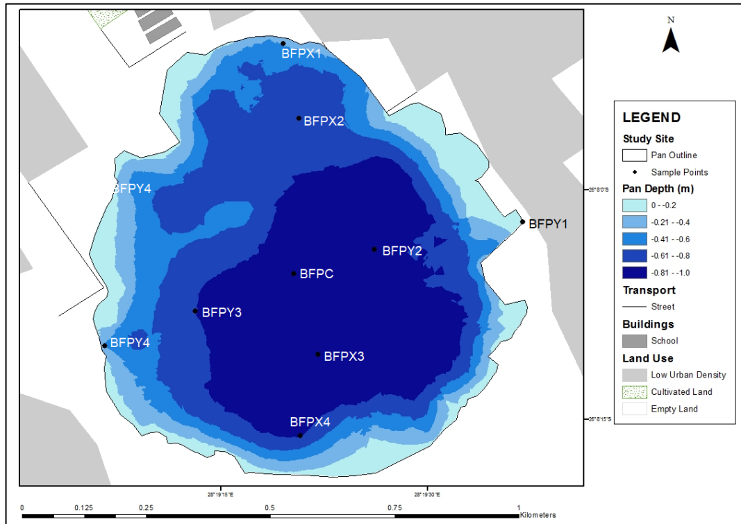
Figure 4.2: Bathymetric Map of Bullfrog Pan
