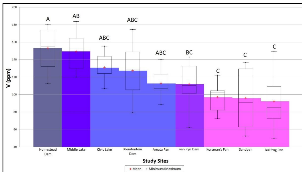
Figure 4.34: The ANOVA plot comparing each site to each other based on mean V concentrations
