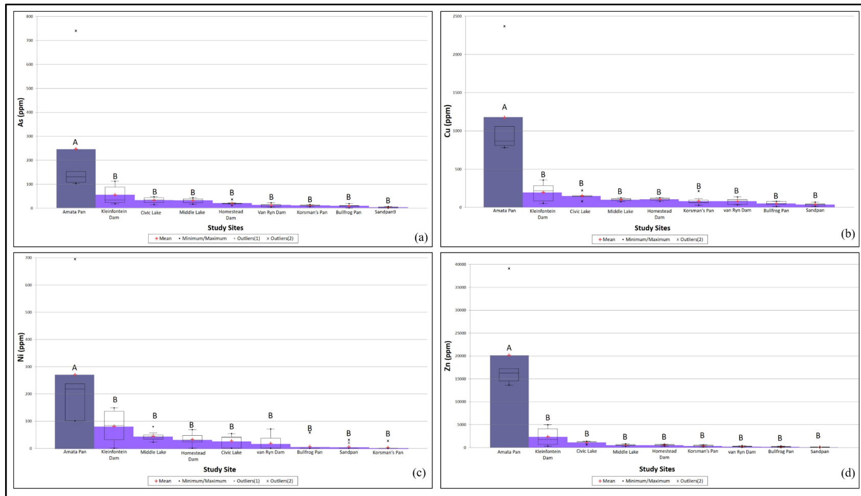
Figure 4.25: The ANOVA plot comparing each site to each other based on mean As (a), Cu (b), Ni (c), and Zn (d) concentrations.
