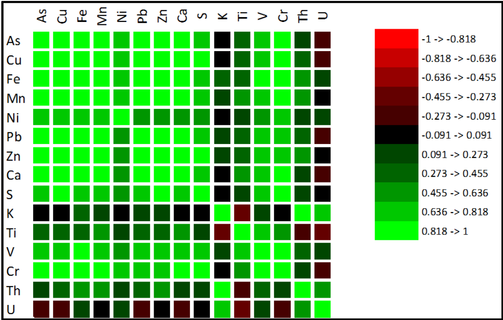
Figure 4.38: Image representation of the correlation matrix for the relationship between trace elements identified in sediments at van Ryn Dam
