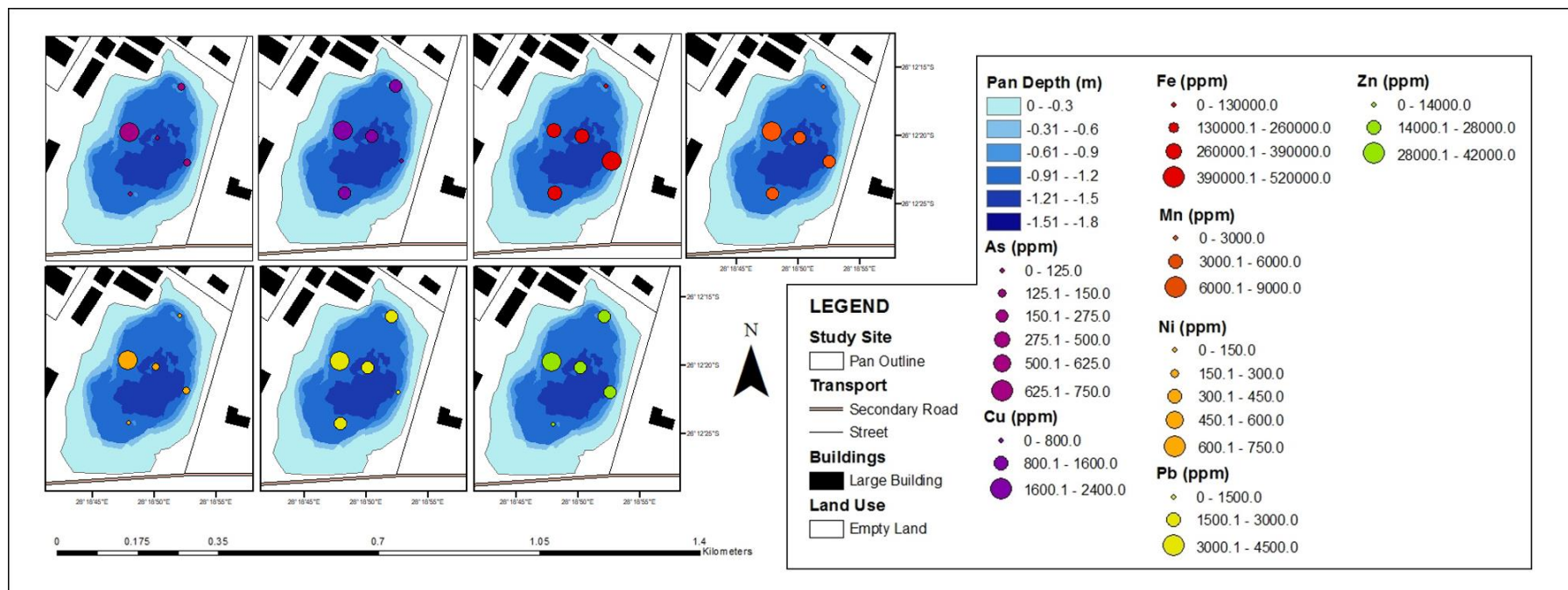
Figure 4.16: Spatial distribution of 7 trace metal concentrations across Amata Pan
