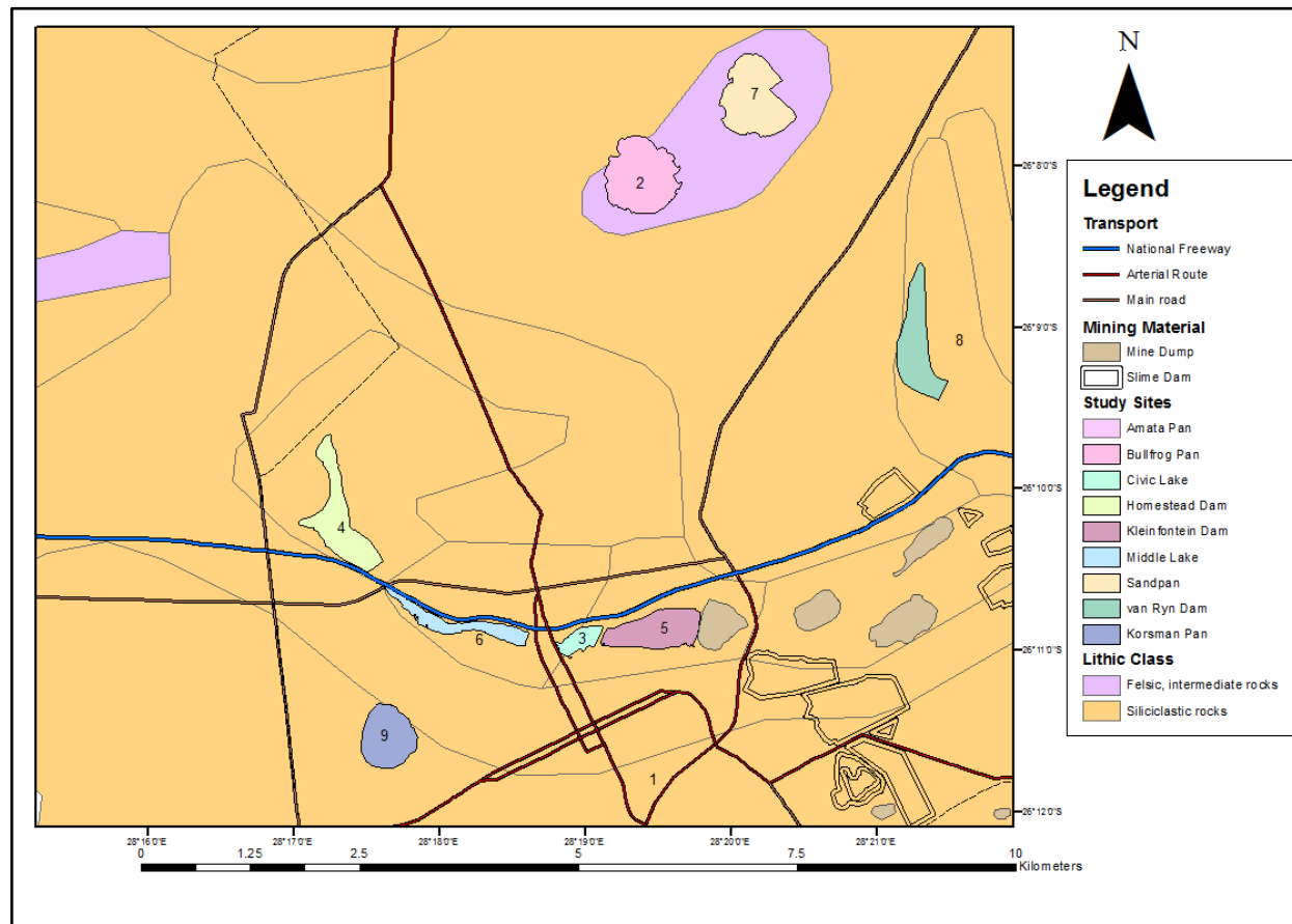
Figure 1.3: The lithic classification of the Benoni Area, and subsequent study sites
