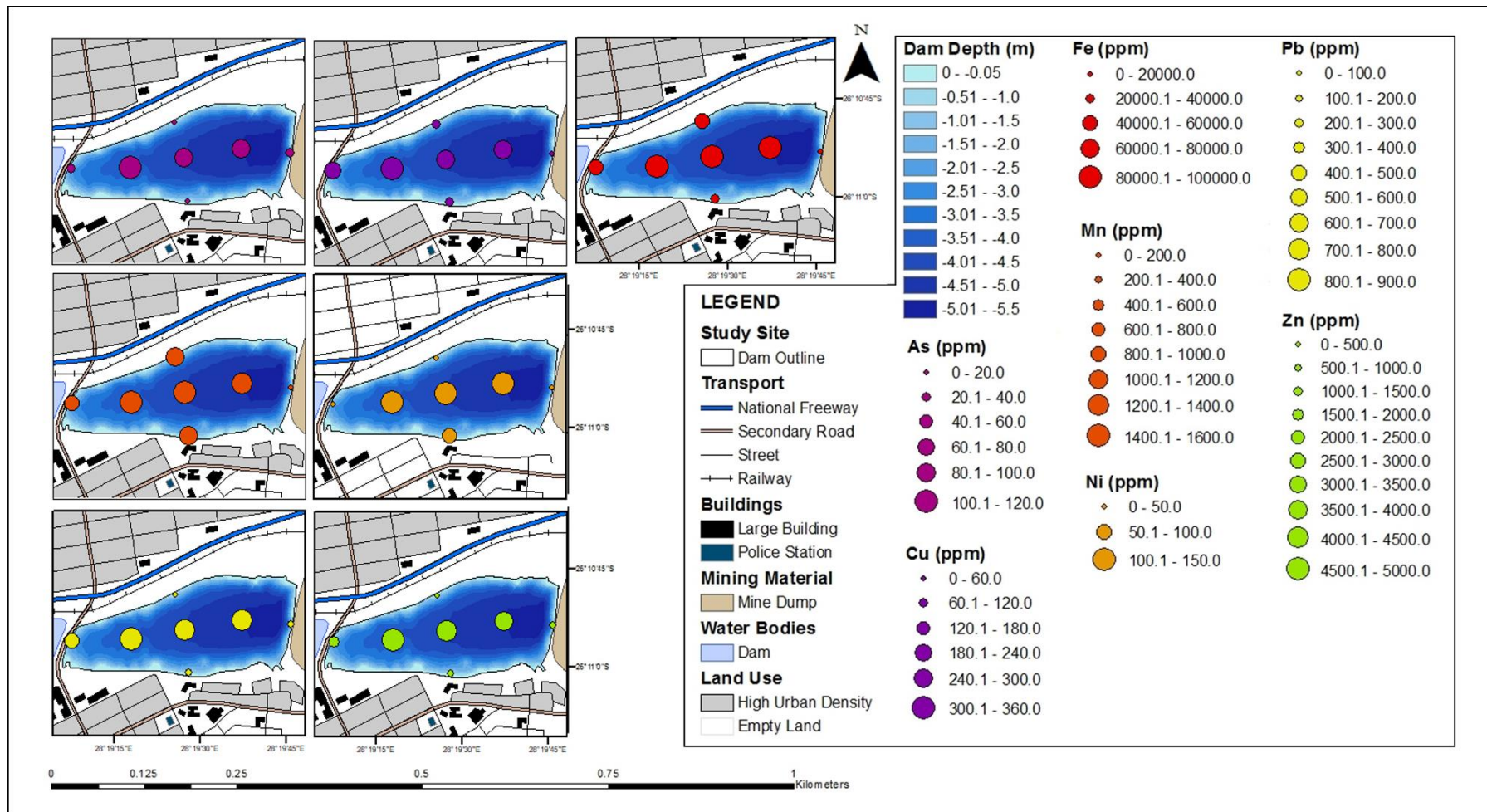
Figure 4.23: Spatial distribution of 7 trace metal concentrations across Kleinfontein Dam
