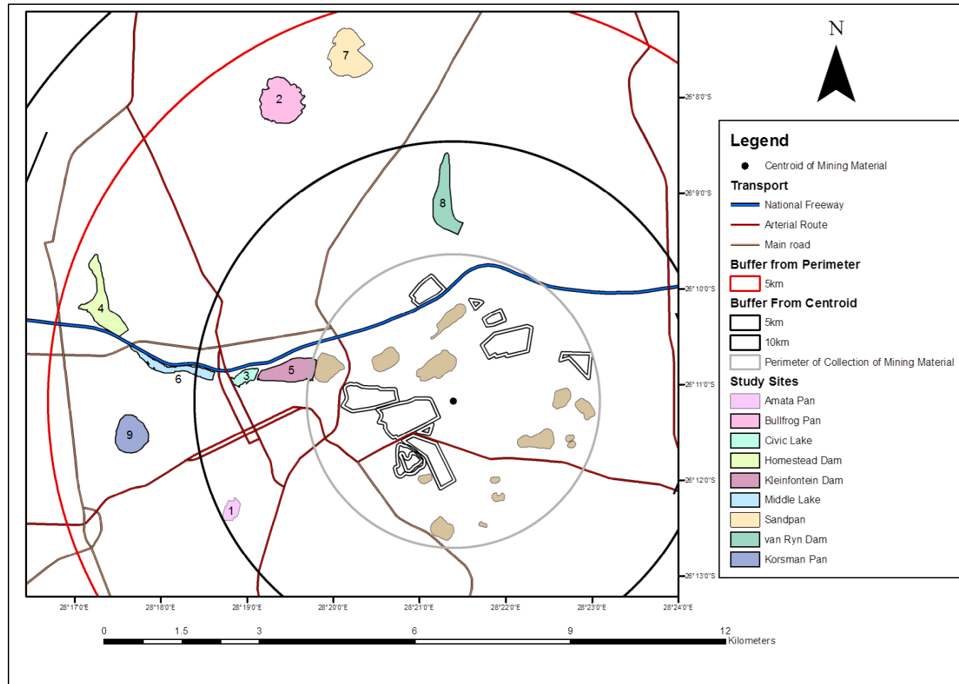
Figure 3.1: The study sites (dams and pans) that were used to conduct the research study. The site number corresponds to Table 3.1
