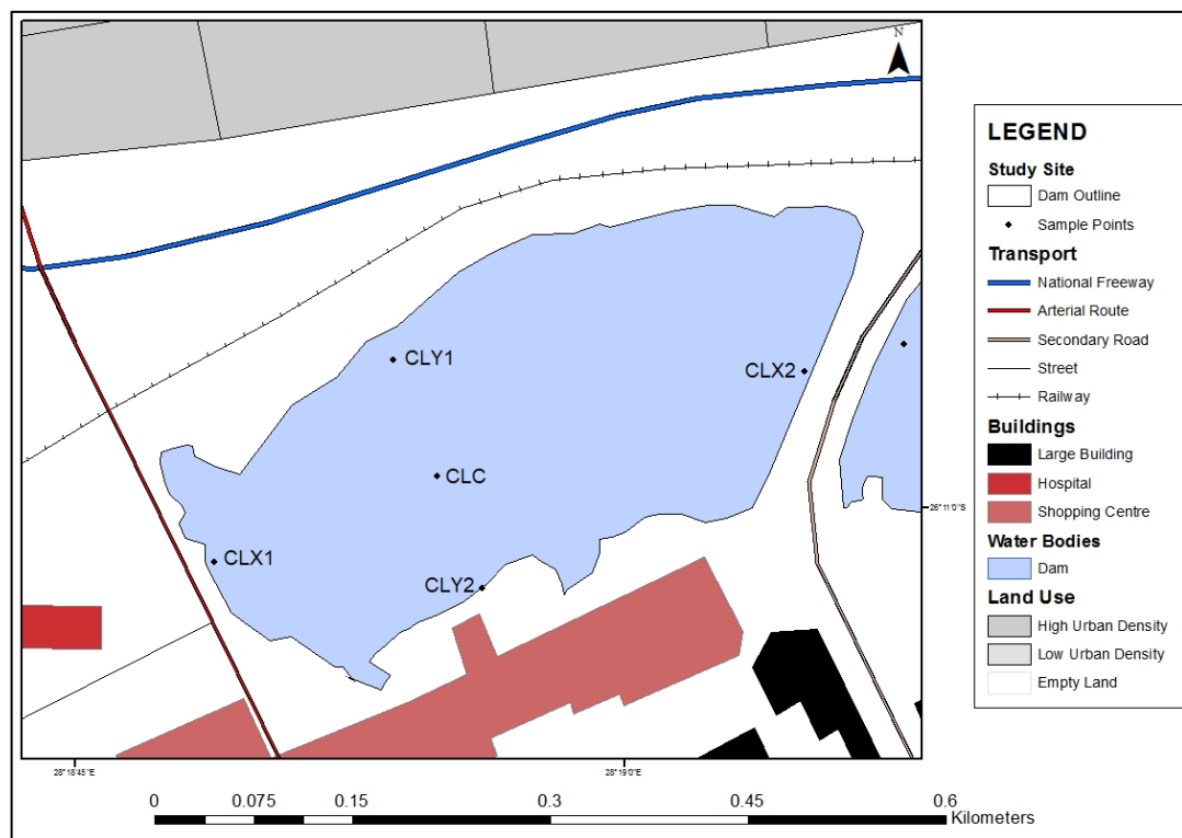
Figure 3.14: Map showing Civic Lake and relative sample points within the site
