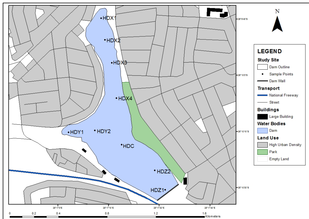
Figure 3.10: Map showing Homestead Dam and relative sample points within the site
