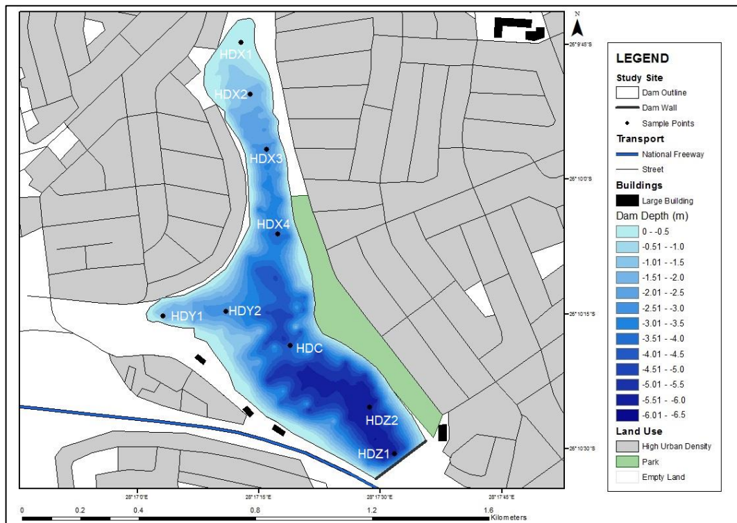
Figure 4.9: Bathymetric Map of Homestead Dam
