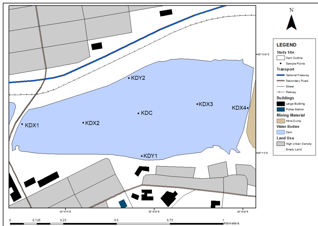
Figure 3.17: Map showing Kleinfontein Dam and relative sample points within the site
