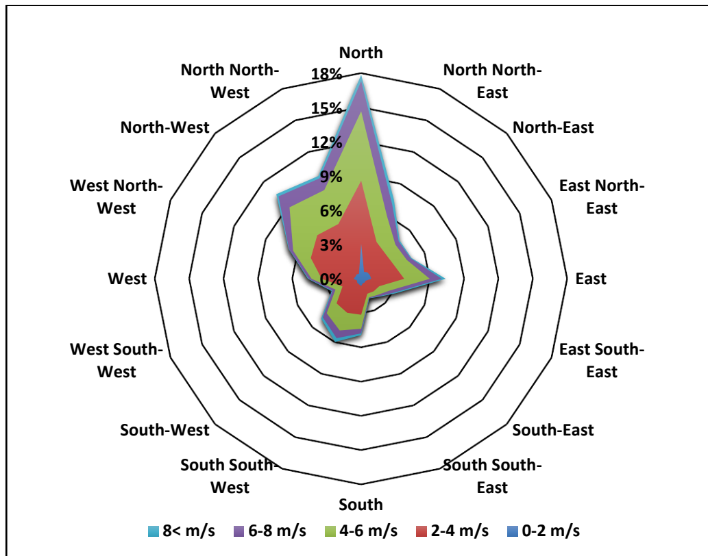
Figure 4.10: Wind rose diagram comparing the average wind speed to the average direction for a 20-year period (1997 - 2017)
