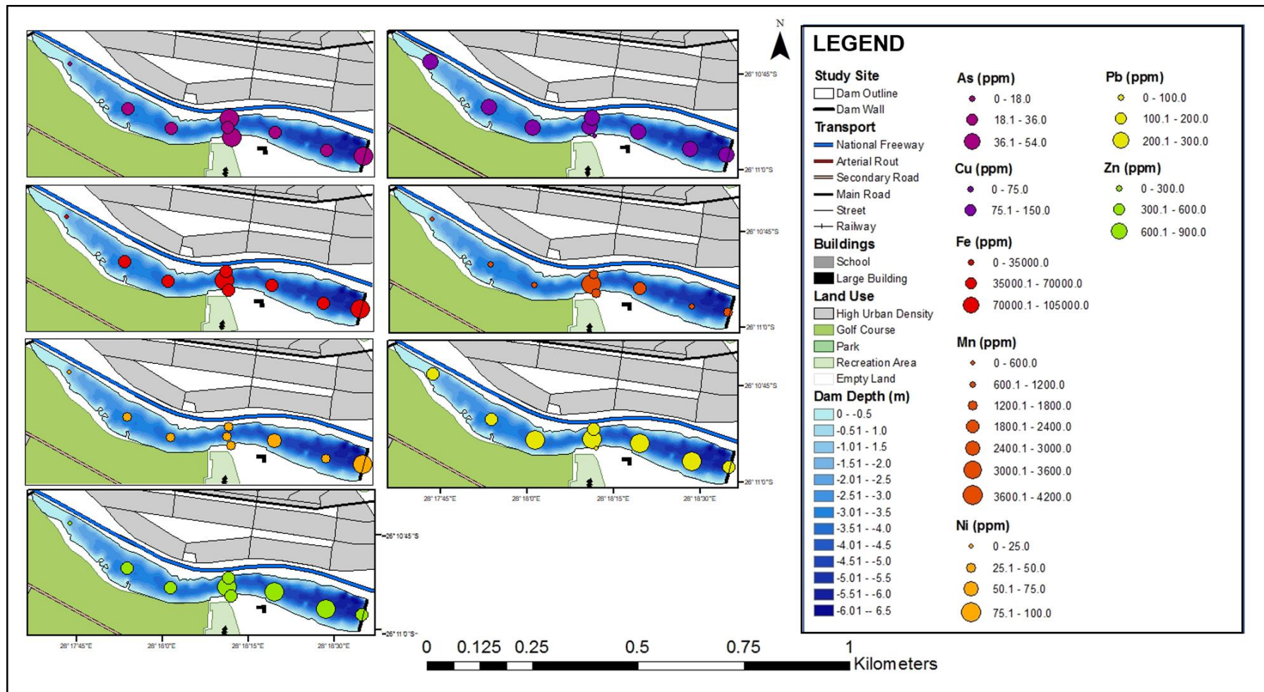
Figure 4.21: Spatial distribution of 7 trace metal concentrations across Middle Lake
