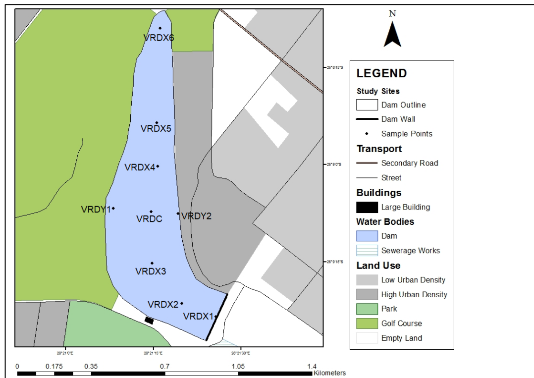
Figure 3.20: Map showing van Ryn Dam and relative sample points within the site
