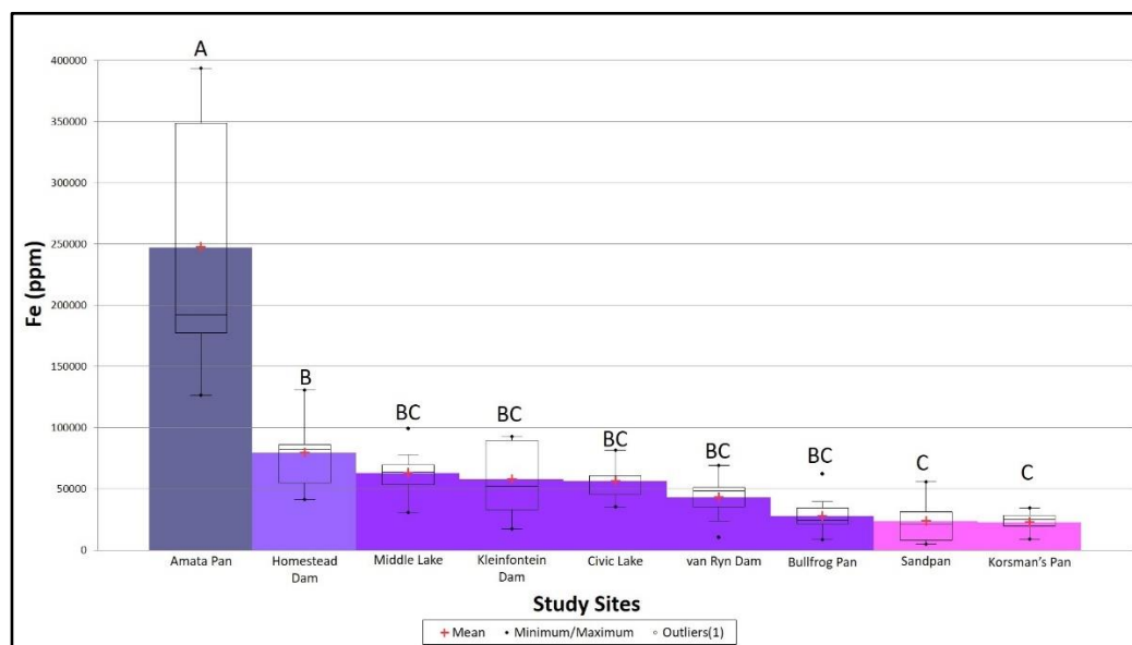
Figure 4.28: The ANOVA plot comparing each site to each other based on mean Fe concentrations.
