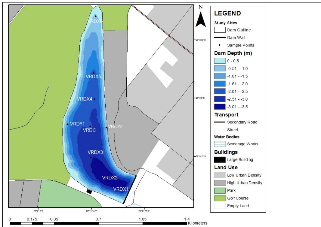
Figure 4.6: Bathymetric Map of van Ryn Dam
