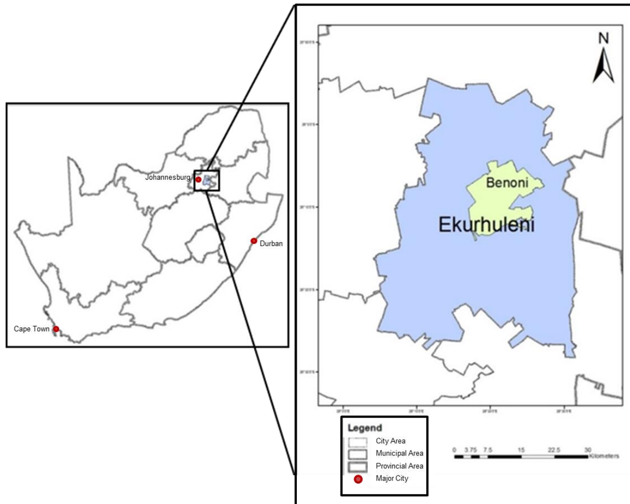
Figure 1.1: A reference map to show the relation of the City of Benoni to the rest of South Africa
