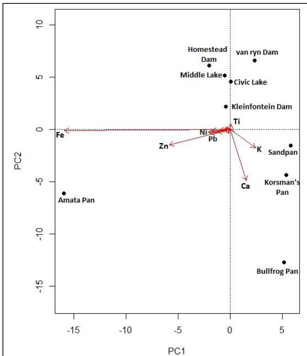
Figure 4.12: The relationship between the individual sites and the main trace elements (site mean values) found within them
