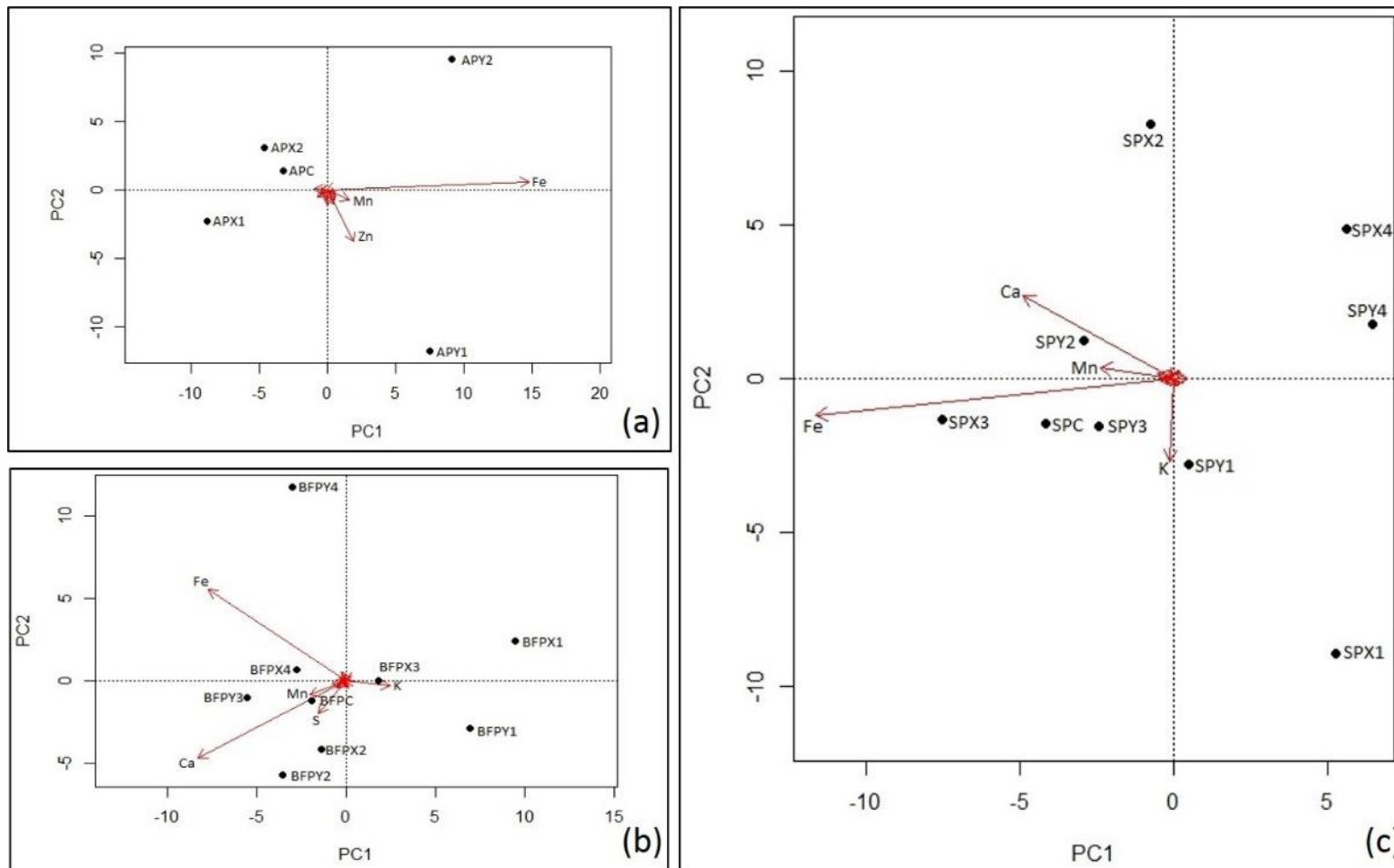
Figure 4.14: PCA expressing the relationship of samples and trace elements within selected sites (a. Amata Pan; b. Bullfrog Pan; c. Sandpan)
