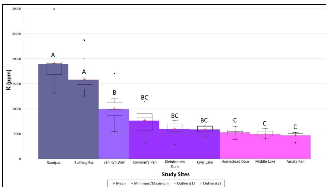
Figure 4.29: The ANOVA plot comparing each site to each other based on mean K concentrations.
