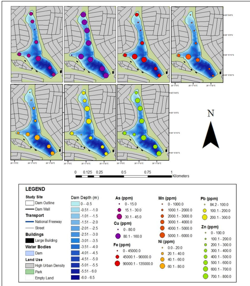
Figure 4.20: Spatial distribution of 7 trace metal concentrations across Homestead Dam
