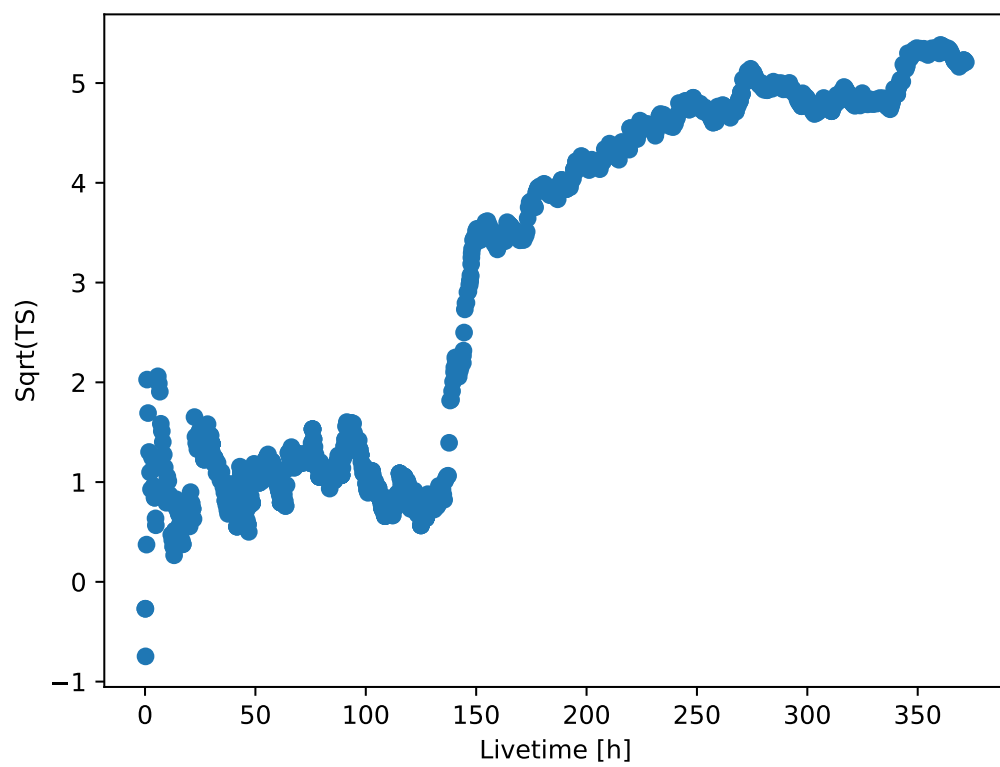
FIGURE 3.7: Plot of the cumulative significance of the full dataset of LMC P3 plotted over the livetime.
