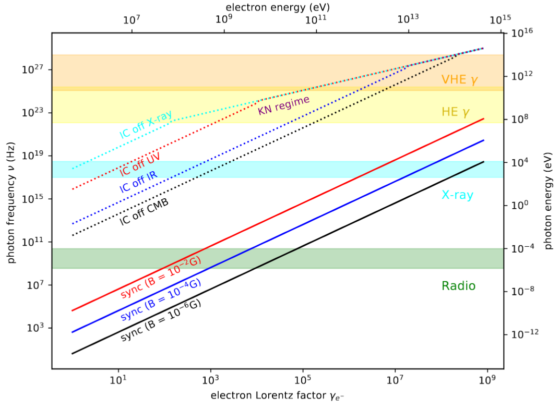
FIGURE 2.4: This plot shows the photon energy produced in the non-thermal processes (Synchrotron radiation and Inverse Compton radiation) for different seed photon energies and electron energies (or Lorentz factors). To produce TeV gamma-rays, an electron energy of at least \approx 10^{11} eV is required for an X-ray seed photon. It can also be seen from the figure that in the Klein-Nishina regime, The energy of the IC photon depends less on the seed photon and more on the electron's initial energy. Source: Paredes & Bordas (2019)
