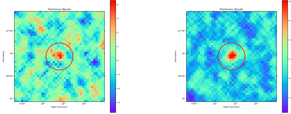
(e) Inferior Conjunction (0.207-0.268) (f) Post-Inferior Conjunction (0.268-0.366)
