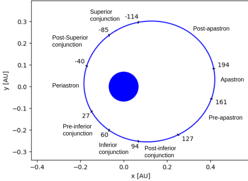
FIGURE 3.9: Orbital binning
