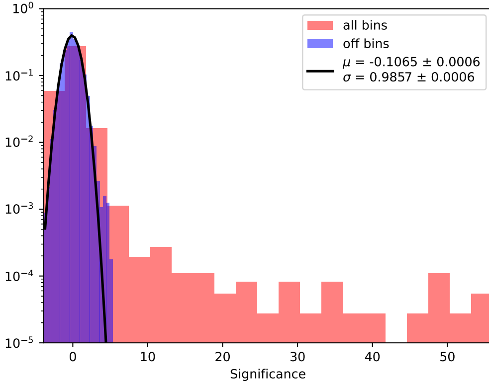
FIGURE 4.3: Gaussian fit of the off-regions. This is the plot for all 1344 runs. Fit result: \mu = -0.1065 \pm 0.0006 , \sigma = 0.9857 \pm 0.0006 .
