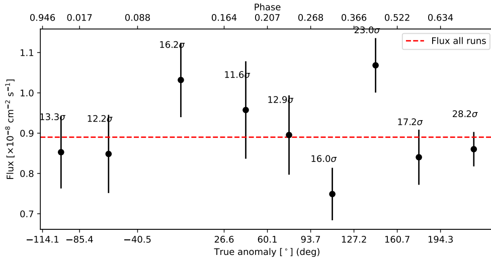
FIGURE 4.10: The runs for N 157B folded on the period of LMC P3 to check if the flux is constant.
