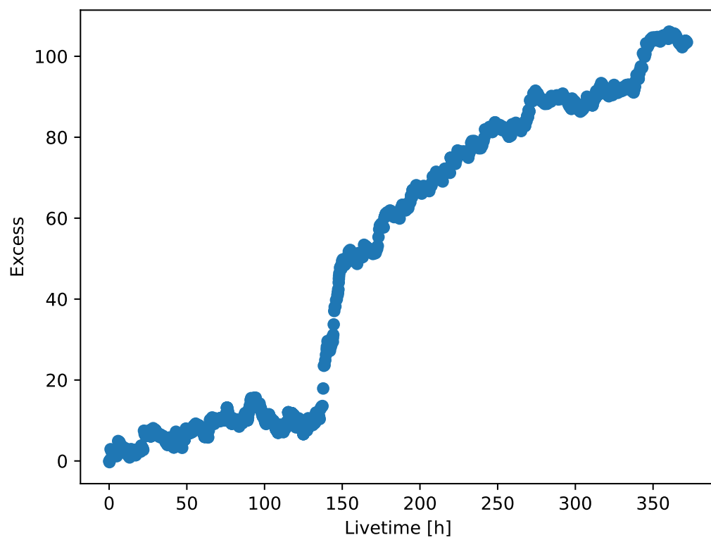
FIGURE 3.6: Plot of the cumulative excess of the full dataset of LMC P3 plotted over the livetime.
