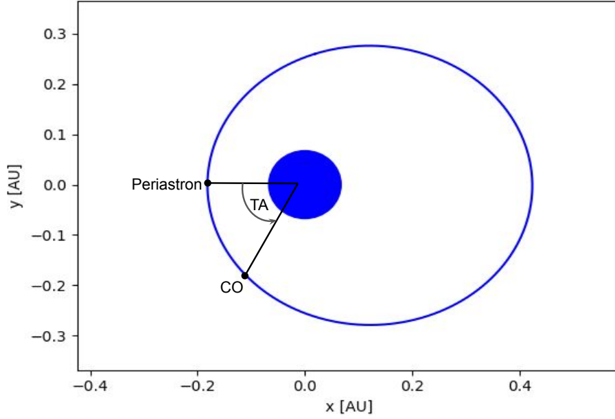
FIGURE 3.8: The true anomaly is the angle, TA, drawn from periastron, through the star and to the current position of the orbiting body, CO.
