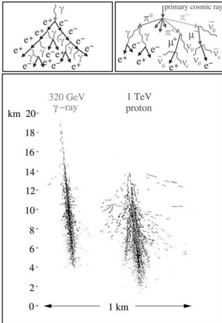
FIGURE 3.3: Top panels: Schematic development of a gamma-ray shower (left) and a proton shower(right). Main panel: Monte Carlo simulations of gamma-ray and cosmic proton showers. The tracks of some of the particles that emit Cherenkov light are shown. Source: Weekes (2003)
