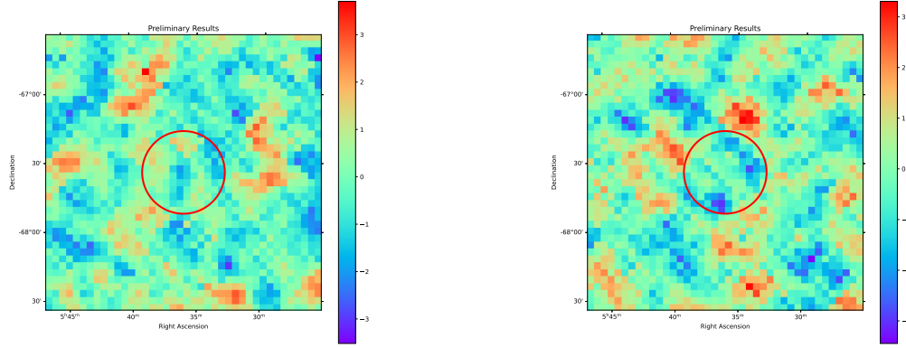
(a) Superior Conjunction (0.946-0.017) (b) Post-superior Conjunction (0.017-0.088)
