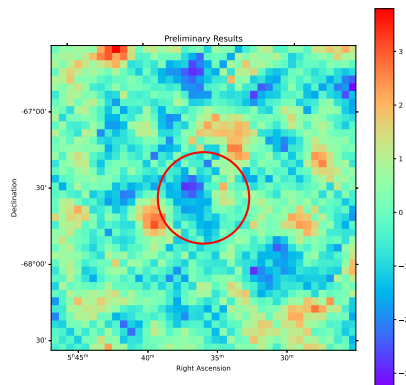
(i) Post-apastron (0.634-0.946)
