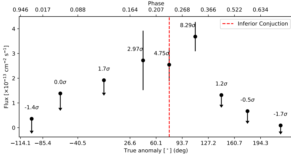
FIGURE 4.15: Lightcurve for LMC P3. The peak flux is observed after inferior conjunction (0.268-0.366) with a significance of 8.29 \sigma . Upper limits are calculated at the 95 % confidence range.
