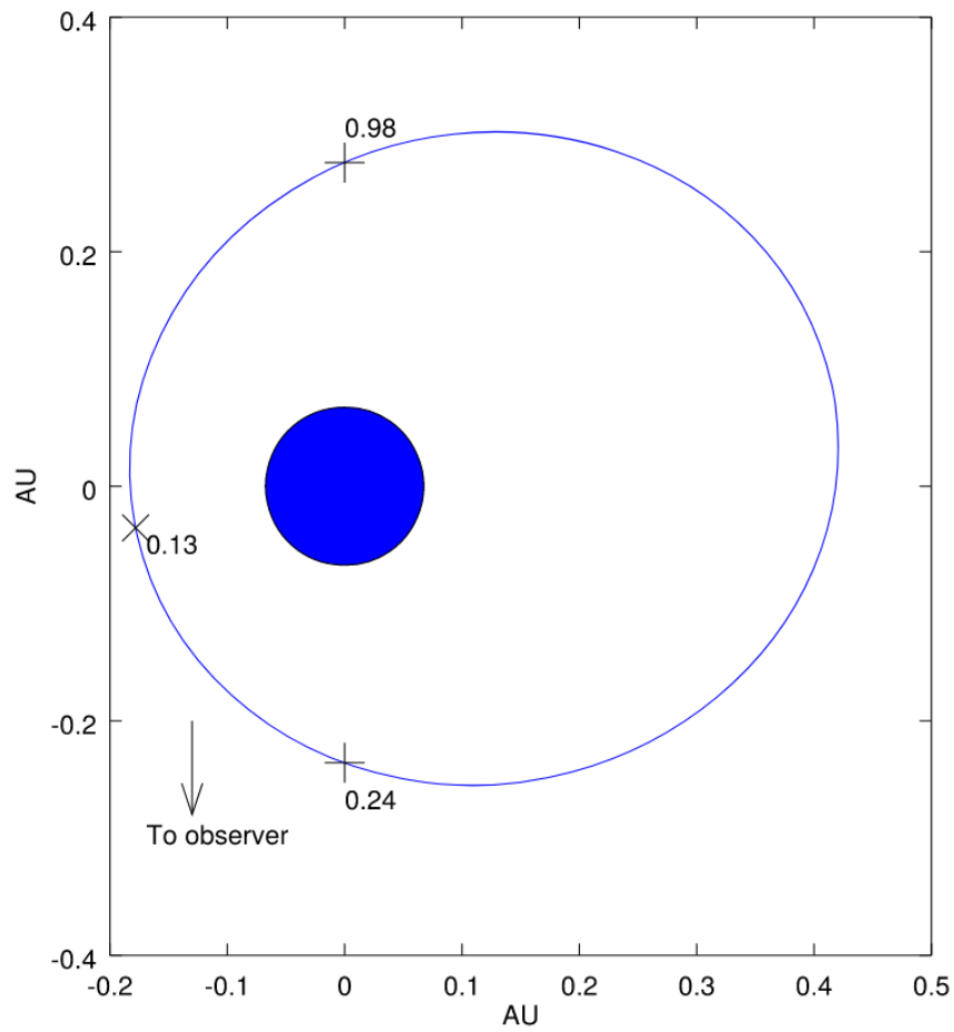
FIGURE 3.5: The binary orientation of LMC P3 showing the star (blue circle), positions of inferior and superior conjunction marked with a + and periastron \times . Source: van Soelen et al. (2019)
