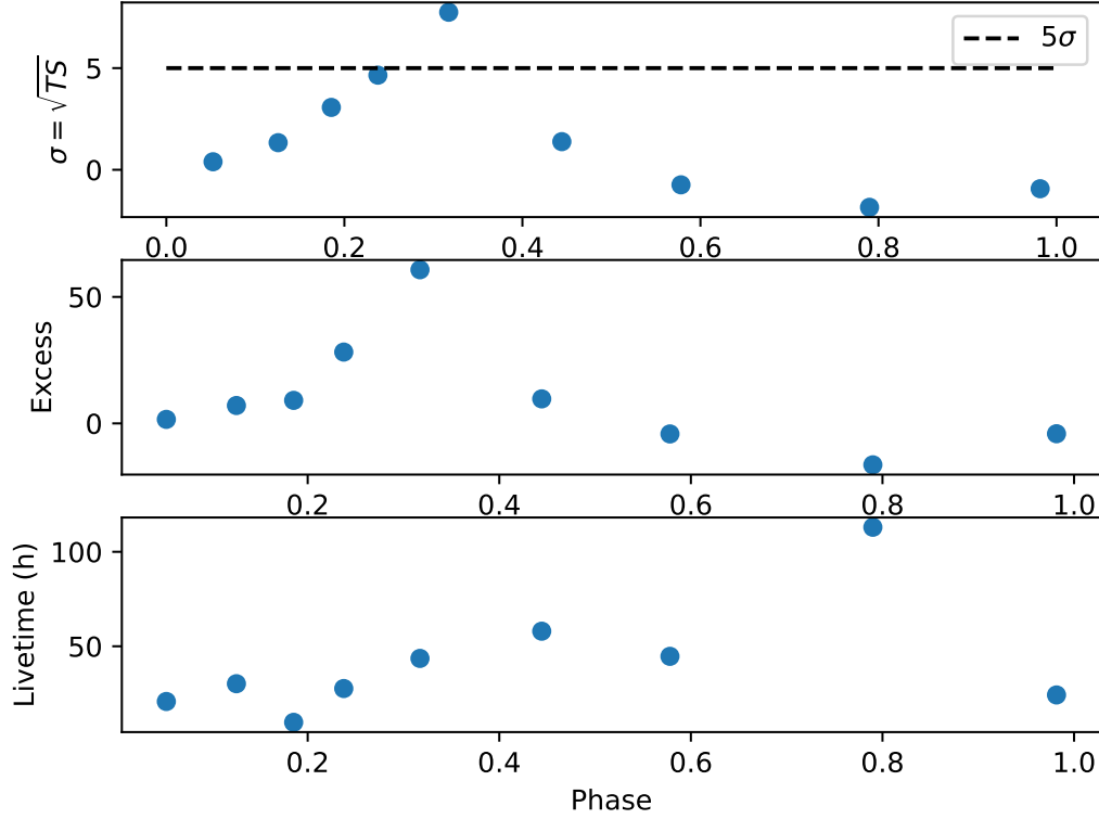
FIGURE 4.11: Significance evolution for LMC P3. The total significance (Top Panel) for different orbital phases of LMC P3 as well as the excess (Middle Panel) and live-time (Bottom Panel), are plotted for LMC P3. A black dashed line in the top panel indicates the 5\sigma significance level.
