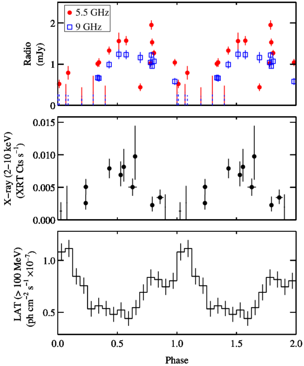
FIGURE 2.2: This plot shows the Radio (Top panel), X-ray (Middle panel) and HE gamma-ray light curves. Source: Corbet et al. (2016)
