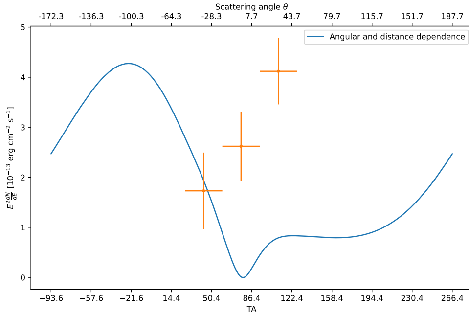
FIGURE 4.16: Inverse Compton Scattering Model for LMC P3 (blue line) and the spectral energy points found from the analysis (orange line). These points consider photons of energy 1 to 10 TeV. The top axis shows the scattering angle between the stellar photons and the electrons/positrons from the compact object.
