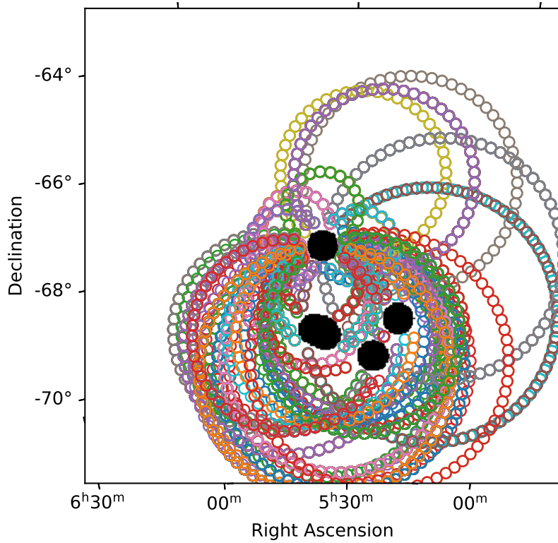
FIGURE 4.6: Background determination of LMC P3. The coloured circles show the background regions selected. The blacked out regions show the areas on the map which have not been used to determine the background, to prevent the background estimation from being contaminated by source emission.
