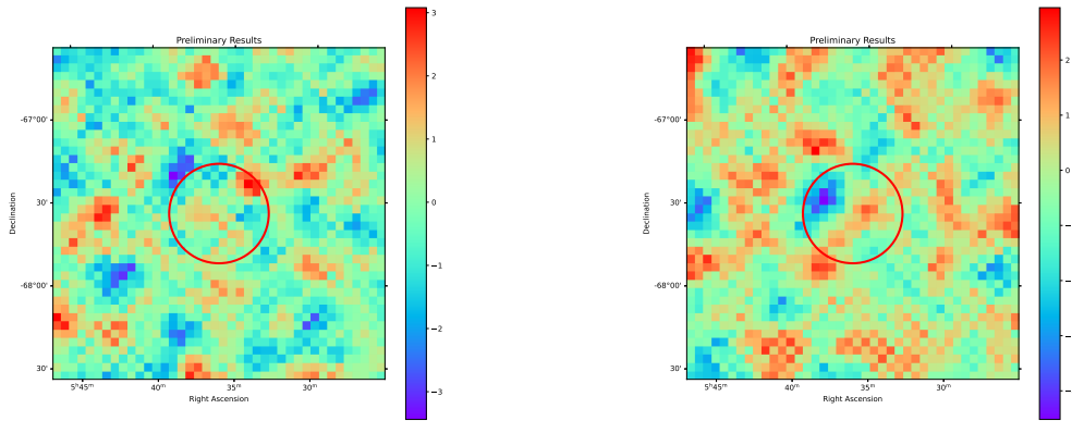
(g) Pre-apastron (0.366-0.522)
