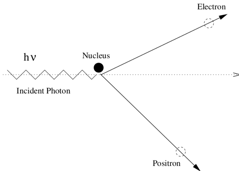
FIGURE 3.1: This plot shows the incident gamma ray interacting with a target atmospheric nucleus to annihilate and form an electron-positron pair. Source: Weekes (2003)
