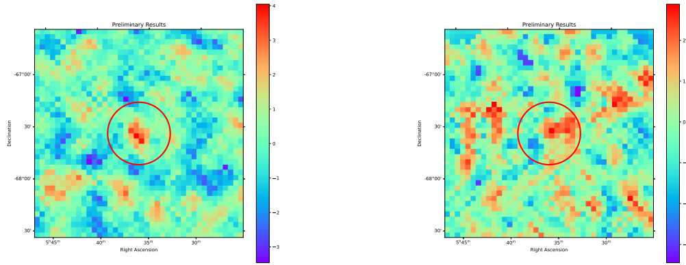
(c) Periastron (0.088-0.164) (d) Pre-Inferior Conjunction (0.164-0.207)
