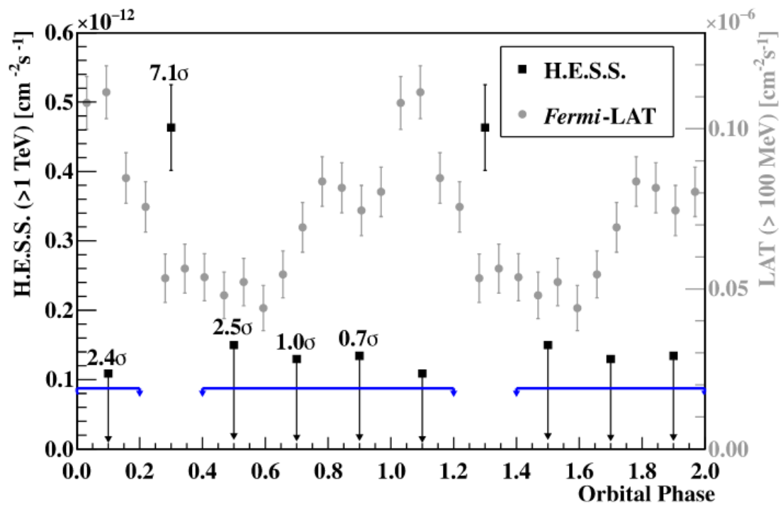
FIGURE 2.3: This plot shows the VHE phase folded light curve (black) imposed on the Fermi-LAT curve. Source: Abdalla et al. (2018)
