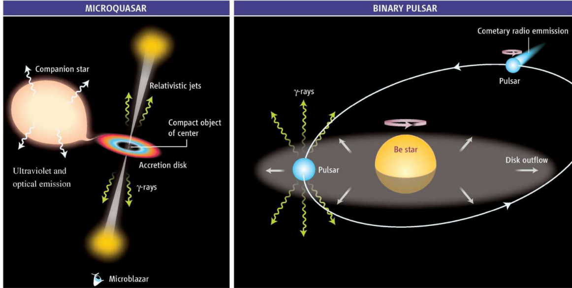
FIGURE 2.1: Left: The microquasar-jet model. Matter from the companion star is accreted onto the neutron star or black hole, producing relativistic jets which produce gamma rays. Right: The pulsar scenario where the wind from the pulsar interacts with the stellar environment from the companion to produce the gamma rays. Source: Mirabel (2007)
