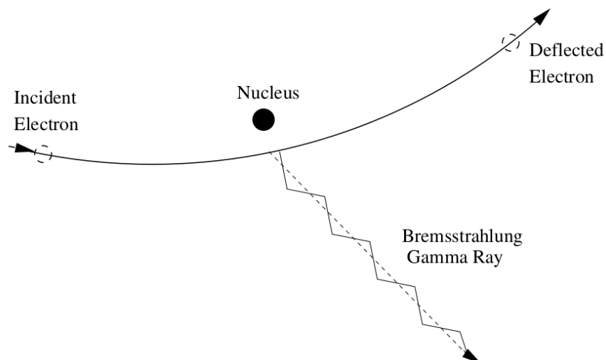
FIGURE 3.2: This plot shows the deflection of an electron interacting with a target atmospheric nucleus to produce a photon. Source: Weekes (2003)
