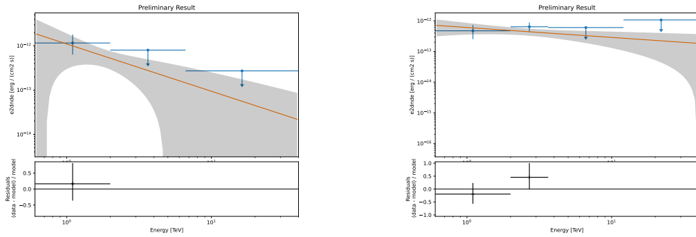
(a) Pre-Inferior Conjunction (0.164-0.207) (b) Inferior Conjunction (0.207-0.268)
