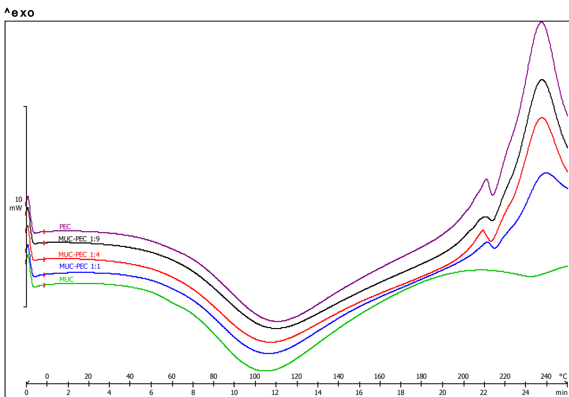
Figure 3.13: DSC thermogram of; MUC, MUC-PEC USP (ratio 1:1, 1:4 and 1:9) and PEC evaluated from -10°C to 250°C.
