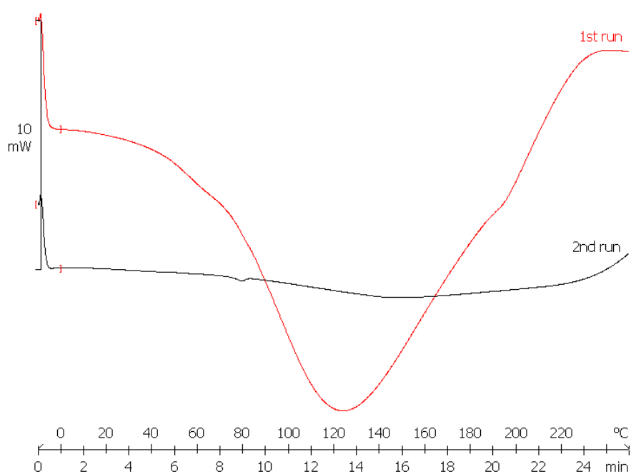
Figure 3.12: First and second run DSC thermograms of BP36 measured from -10^{\circ}\text{C} to 250^{\circ}\text{C}
