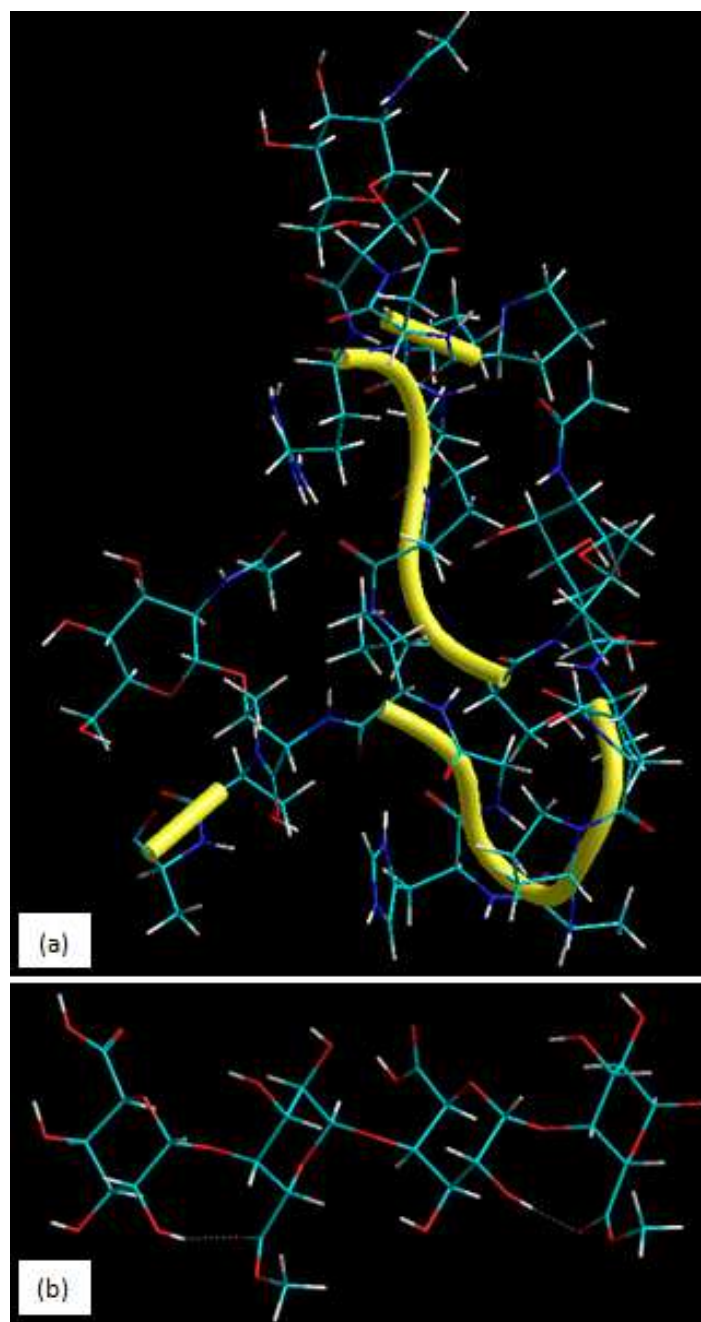
Figure 3.17: Energy minimized molecular structures of, (a) glycosylated MUC and (b) PEC generated by HyperChem™ 8.0.8 Molecular Modeling System (Hypercube Inc., Gainesville, Florida, USA). Colour codes: C (cyan), O (red), N (blue) and H (white).
