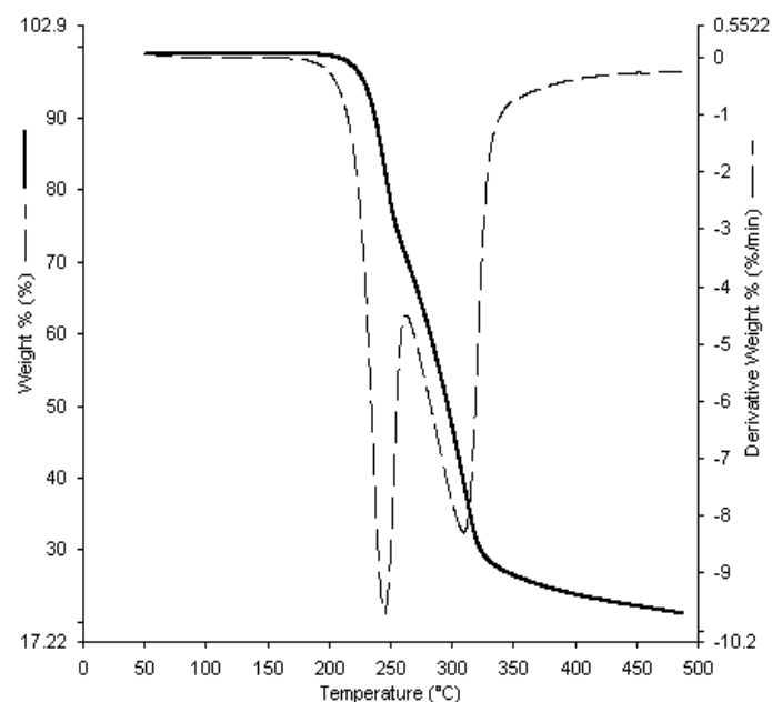
Figure 3.7: TGA (solid) and DTGA (dotted) thermogram of AZT obtained when AZT was analyzed from 50°C to 500°C
