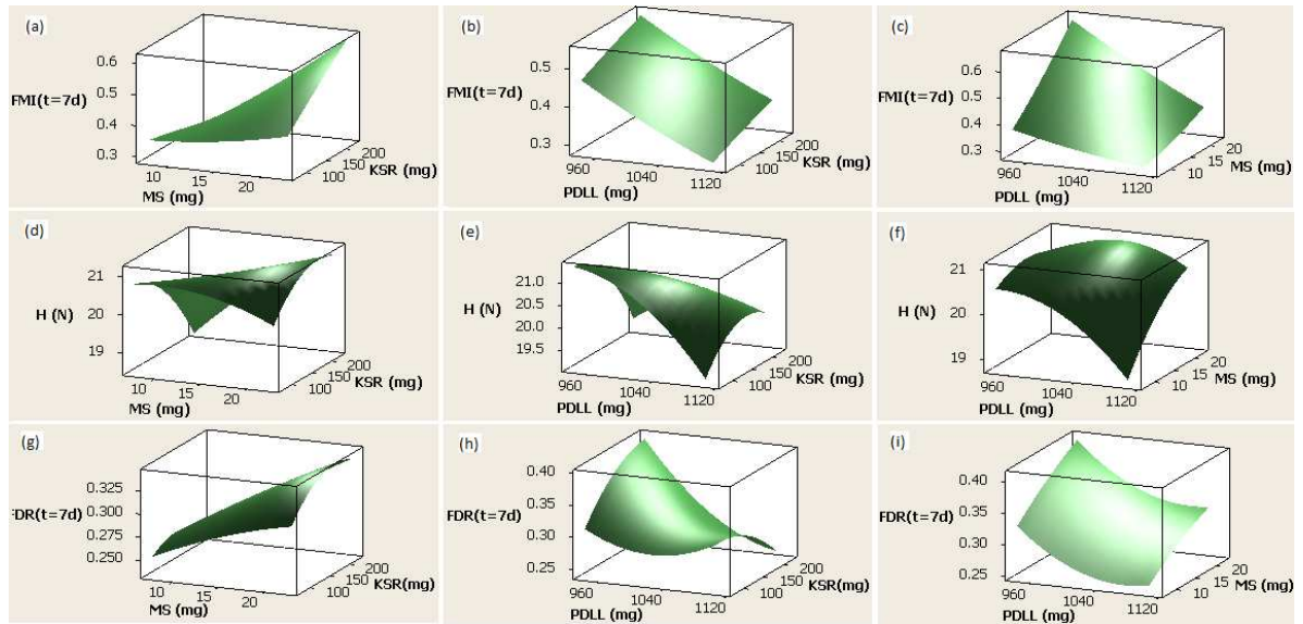
Figure 5.2: Response surface plots correlating responses; fractional of mass increase (FMI), matrix hardness (H) and fractional drug release (FDR) to independent parameters; masses of magnesium stearate (MS), polyvinyl acetate/polyvinylpyrrolidone (KSR) and poly(D,L-lactide) (PDLL) used in fabricating the polymeric caplet.
