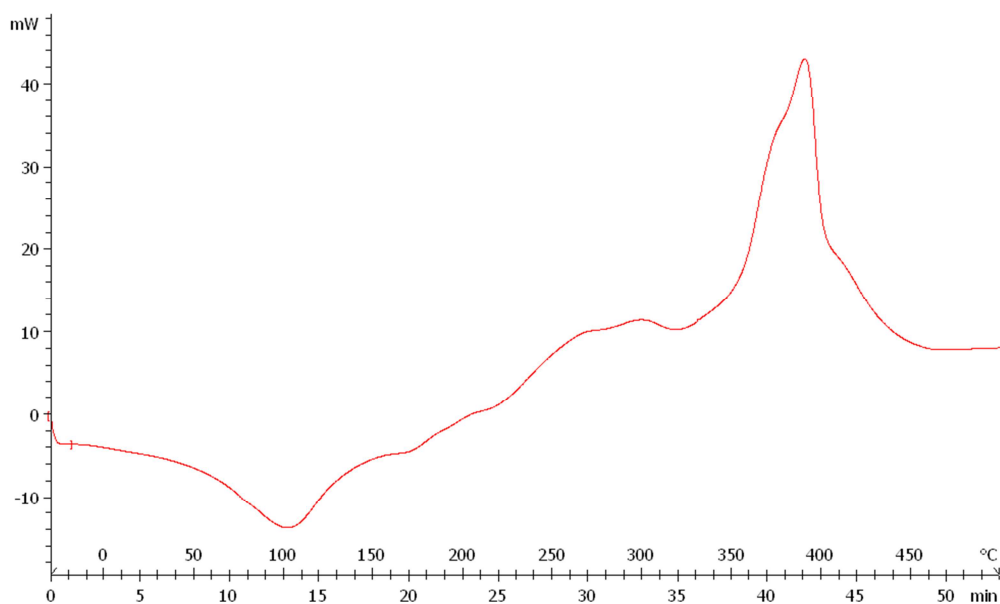
Figure 3.11: First run DSC thermogram of BP36 measured from -10^{\circ}\text{C} to 500^{\circ}\text{C}
