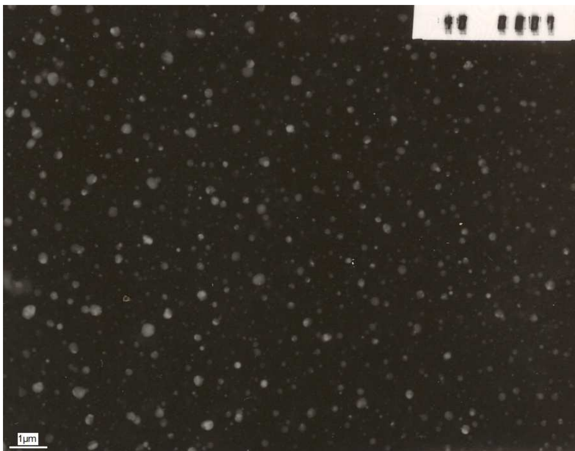
Figure 4.3: Transmission electron micrograph of AZT-loaded MUC-PEC-PEG SMs observed at 40 000X magnification using a JEOL S100 transmission electron microscope
