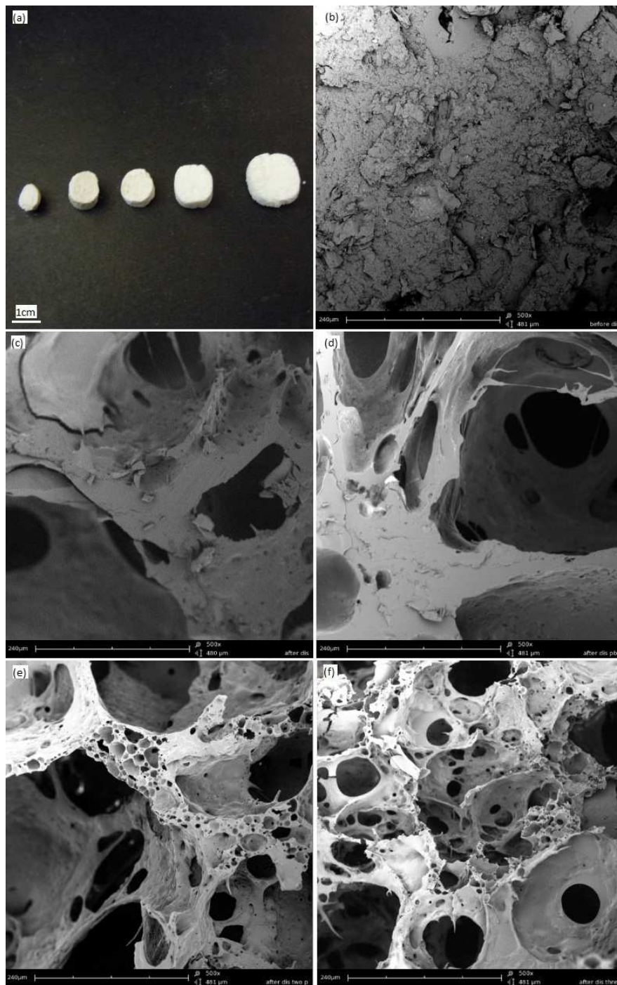
Figure 5.4: Depicts; (a) digital photograph of the caplet's cross-section (from left to right); before dissolution and after 1% poly(acrylic acid) containing caplet's dissolution in SVF and PBS then 2% and 3% poly(acrylic acid) containing caplet's dissolution in SVF respectively (b) SEM micrograph acquired at 500X magnification of the caplet's cross-section before dissolution and (c-f ) SEM micrograph of the caplet cross-section after a 30 day dissolution of the caplet containing, (c) 1% poly(acrylic acid) in SVF (d) 1% poly(acrylic acid) in PBS (e) 2% poly(acrylic acid) in SVF and (f) 3% poly(acrylic acid) in SVF.
