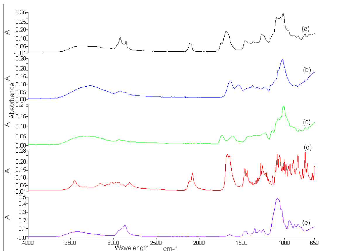
Figure 4.7: ATR-FTIR spectra of; (a) AZT-loaded PEC-MUC-PEG SMs, (b) MUC, (c) PEC, (d) AZT and (e) PEG
