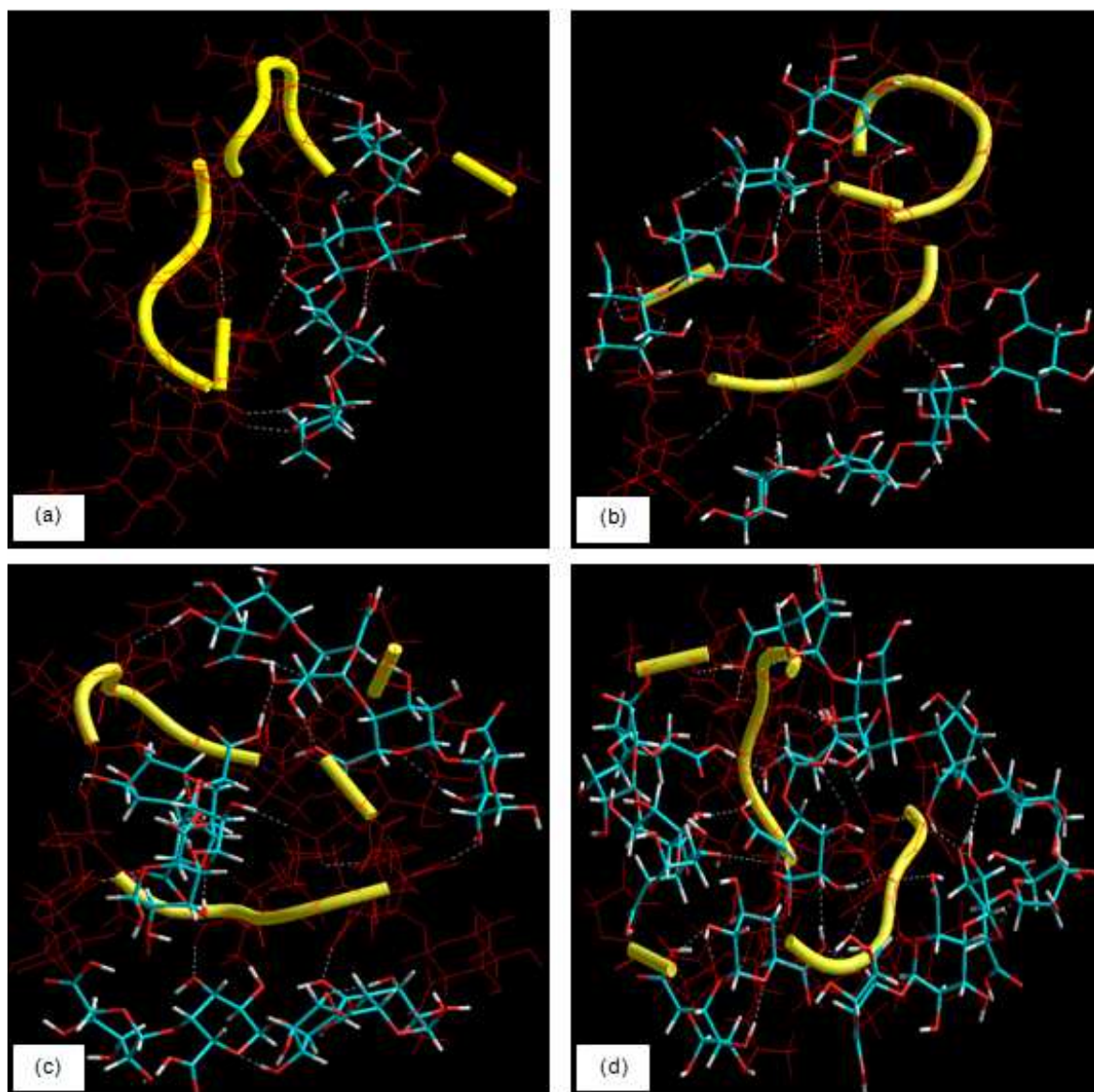
Figure 3.18: Visualization of geometrical preferences of; (a) MUC:PEC::1:1, (b) MUC:PEC::1:2, (c) MUC:PEC::1:3 and (d) MUC:PEC::1:4 along with H-bonds after molecular simulation in vacuum. MUC is rendered as stick model (red) with coiled (yellow) secondary structure. Colour codes: C (cyan), O (red), N (blue) and H (white).
