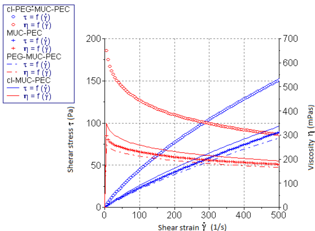
Figure 3.15: Rheological pseudoplastic flow and viscosity profiles of MUC, PEC_{USP} and MUC-PEC_{USP} 9:1 illustrating the effect of addition of PEG 400 and crosslinking with calcium ions on viscosity.
