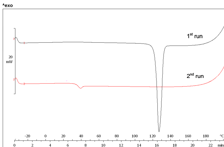
Figure 3.10: First and second run DSC thermograms of AZT measured from -10°C to 200°C
