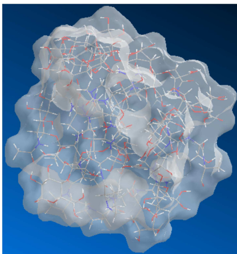
Figure 3.19: Connolly molecular electrostatic potential surfaces of a simulated submicrosphere in wire mesh display mode
