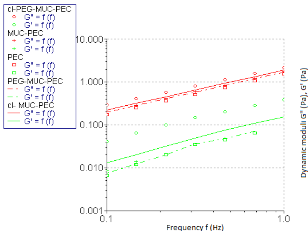
Figure 3.16: Effect on dynamic moduli of PEG 400 and crosslinking with calcium ions as measured by dynamic oscillatory rheology
