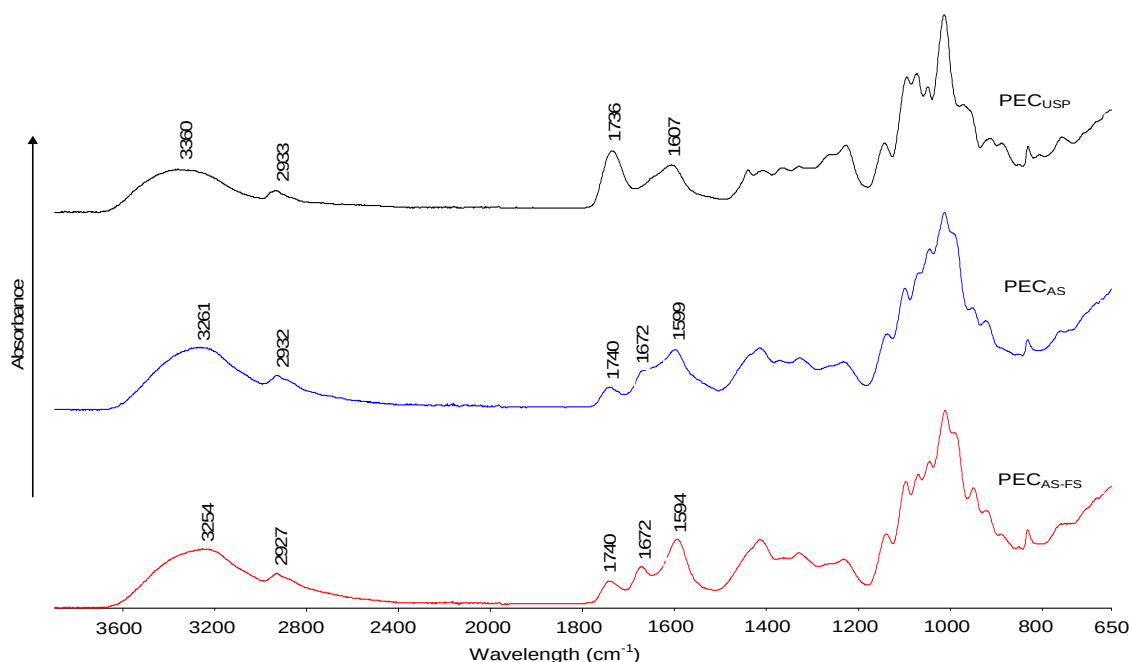
Figure 3.3: Split ATR-FTIR absorbance spectra of lyophilized aqueous dispersions of different types of pectin; \text{PEC}_{\text{AS-FS}} , \text{PEC}_{\text{AS}} and \text{PEC}_{\text{USP}}
