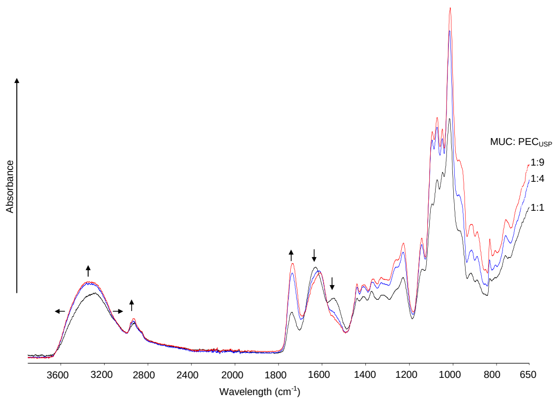
Figure 3.5: Overlay ATR-FTIR absorbance spectra of lyophilized aqueous dispersions of porcine gastric mucin (MUC) and pectin (PEC USP ) that compares the different MUC:PEC USP ratios in MUC-PEC USP lyophilized aqueous dispersions, thus depicting the type and extent of macromolecular interactions between MUC and PEC USP .
