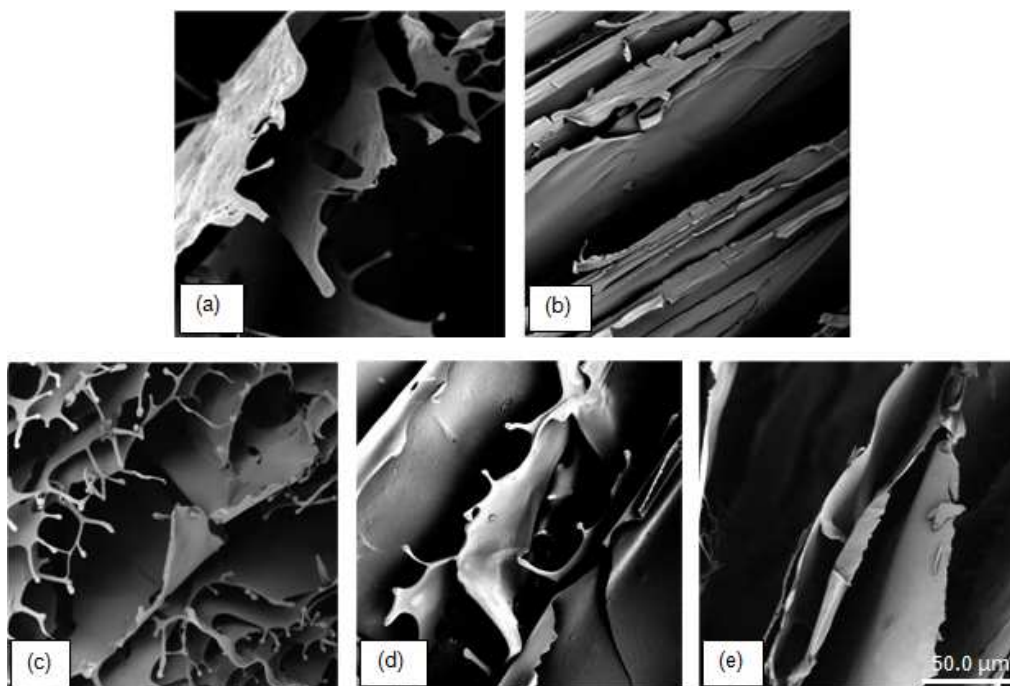
Figure 3.6: SEM images, taken at 510X magnification, depicting membranous scaffolds of lyophilized MUC-PEC USP combinations; (a) MUC, (b) PEC USP , (c) MUC-PEC USP 1:1, (d) MUC-PEC USP 1:4 and (e) MUC-PEC USP 1:9. Bar =50.0μm
