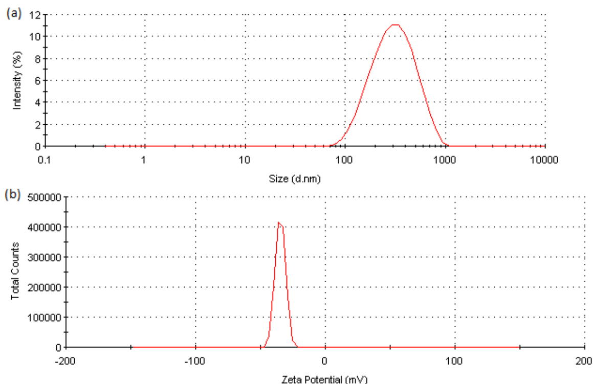
Figure 4.4: Showing, (a) particle size distribution with intensity and (b) zeta potential distribution profile of the optimized SMs obtained using a zetasizer
