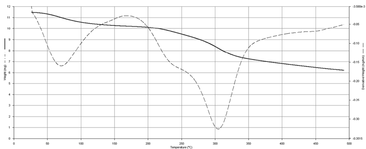
Figure 3.8: TGA (solid) and DTGA (dotted) thermogram for BP36 obtained when BP36 was analyzed from 25°C to 500°C
