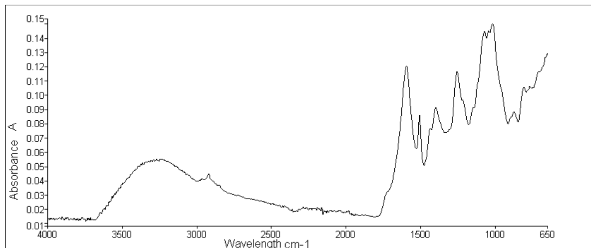
Figure 3.2: ATR-FTIR absorbance spectrum of BP36
