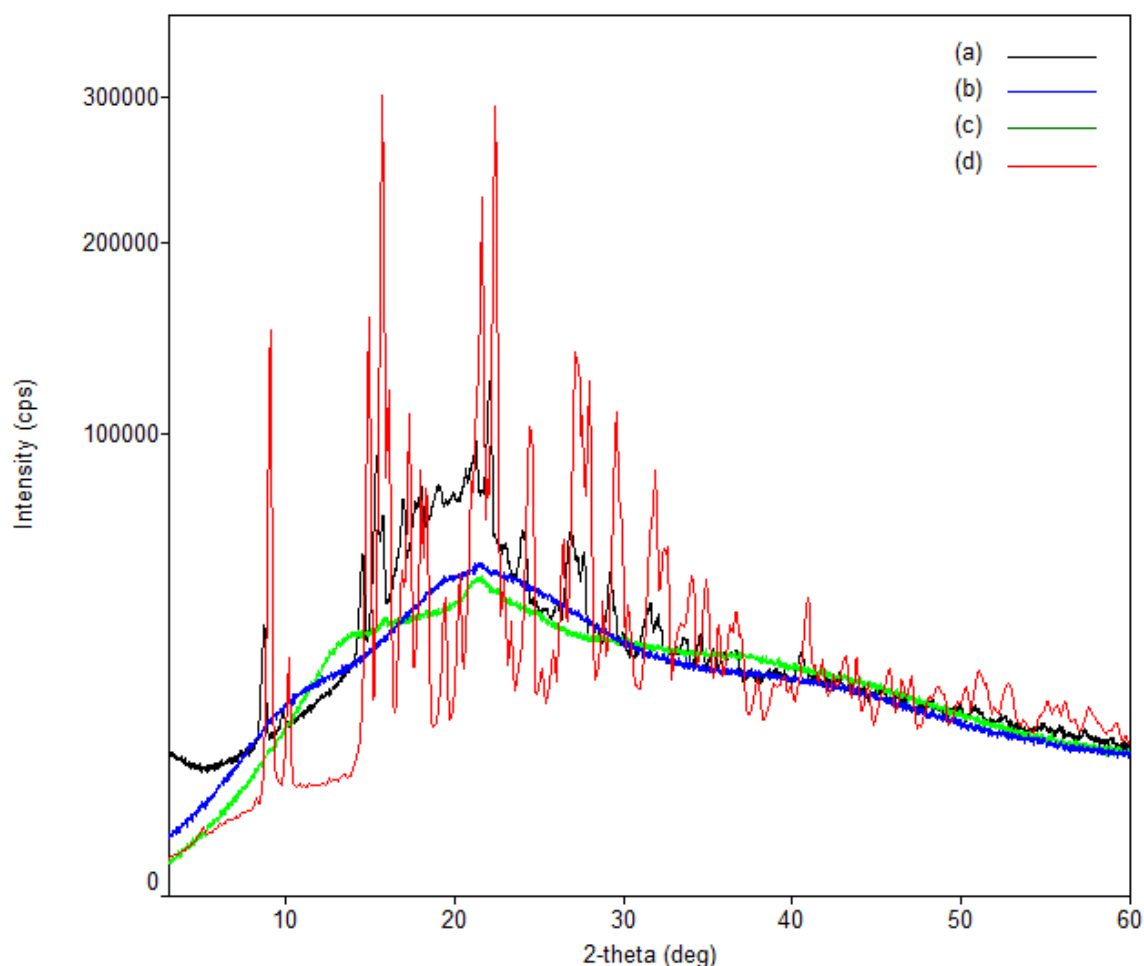
Figure 4.10: Three dimensional X-ray diffractograms of; (a) AZT-loaded PEC-MUC-PEG SMS (black), PEC (green), MUC (blue) and AZT (red)
