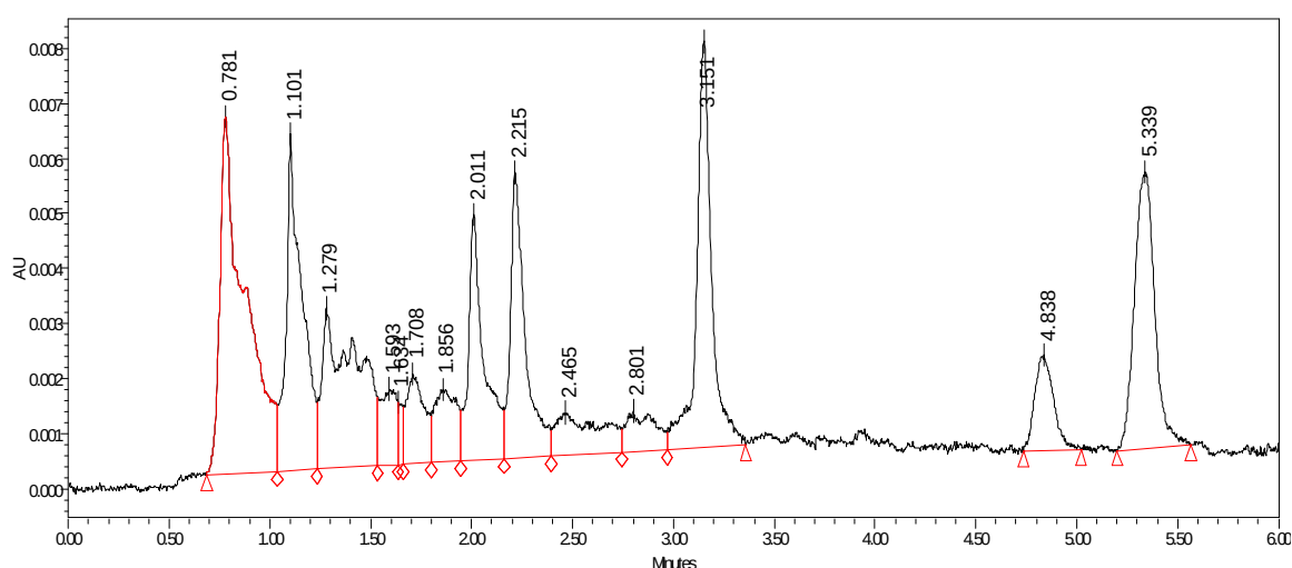
Figure 6.12: UPLC-PDA chromatogram of BP36
