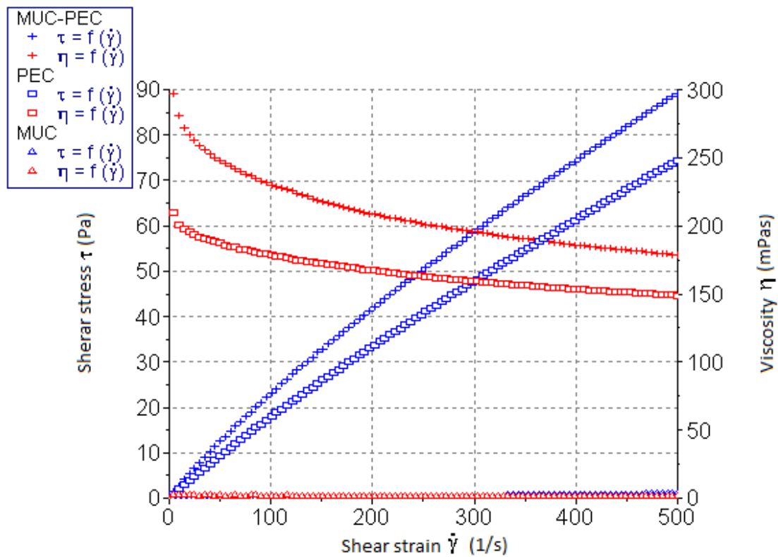
Figure 3.14: Rheology profile properties of MUC, PEC USP and MUC-PEC USP 9:1 illustrating non-Newtonian shear thinning (pseudoplastic) flow and rheological synergism.
