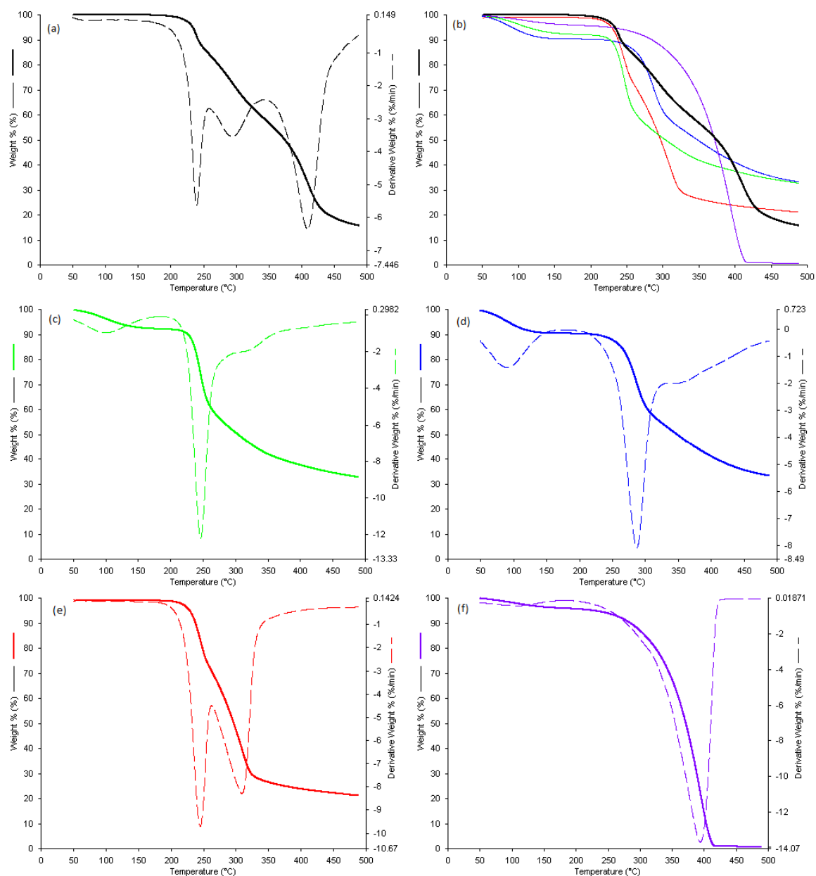
Figure 4.9: The TGA (solid) and DTGA (dotted) thermograms of: (a) PEC-MUC-PEG+AZT SMs; (b) (i) MUC, (ii) PEC, (iii) AZT, (iv) PEC-MUC-PEG+AZT MS and (v) PEG; (c) PEC; (d) MUC; (e) AZT and (f) PEG
