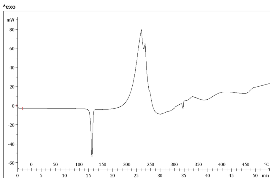
Figure 3.9: First run DSC thermogram of AZT measured from -10°C to 500°C
