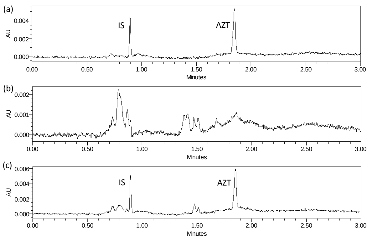
Figure 6.7: Chromatograms obtained for; (a) IS and AZT spiked in diluent, (b) typical blank plasma sample and (c) IS and AZT spiked in plasma sample
