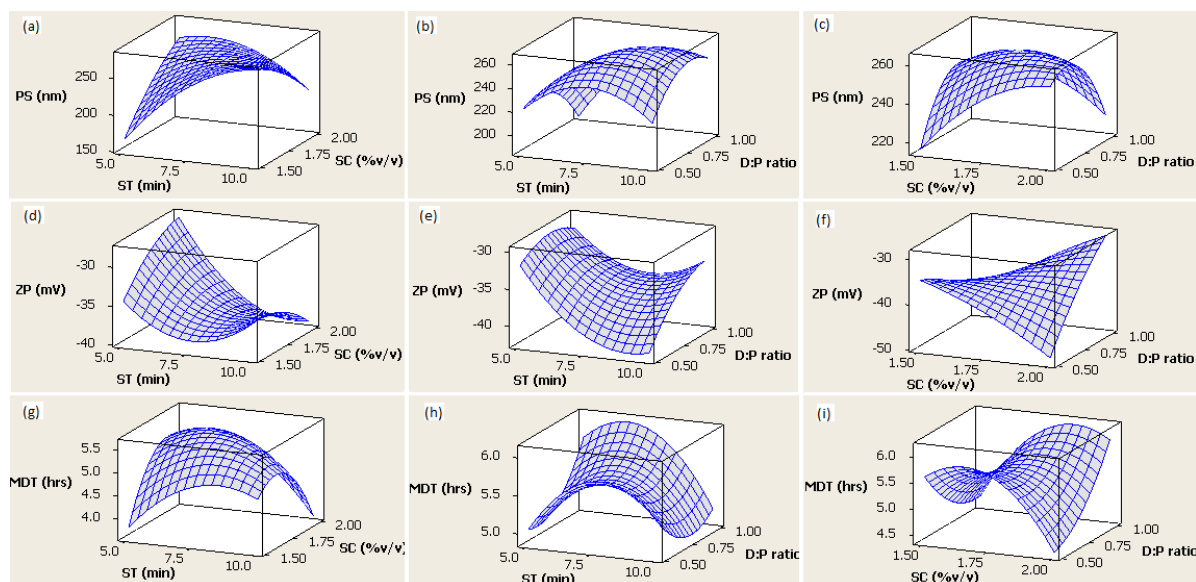
Figure 4.1: Response mesh plots correlating dependent formulation parameters/responses; PS, ZP and MDT to their independent parameters; ST, SC and D:P ratio
