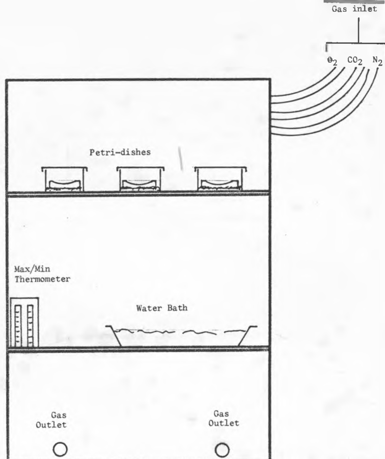
Text figure 3 : Drawing of the Incubator
