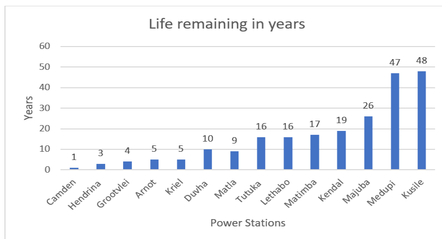
Figure 21: South Africa's fossil fuel power stations economical life (Juodaityte, 2011).
