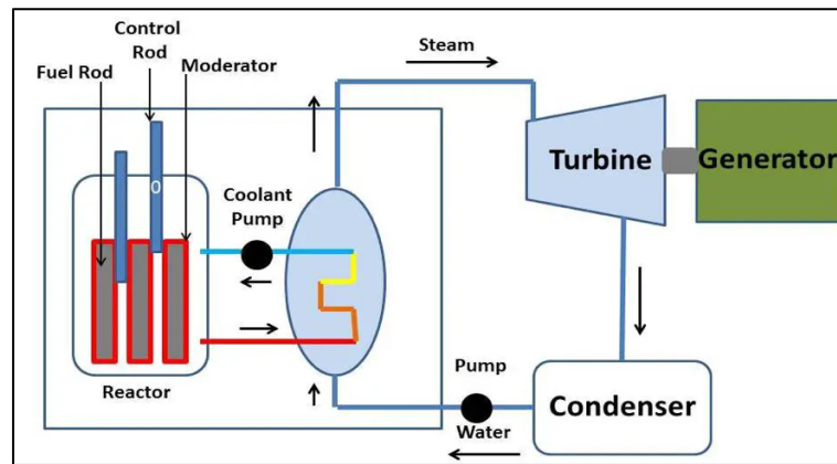
Figure 39: Nuclear Power plant (IRENA, 2020).
