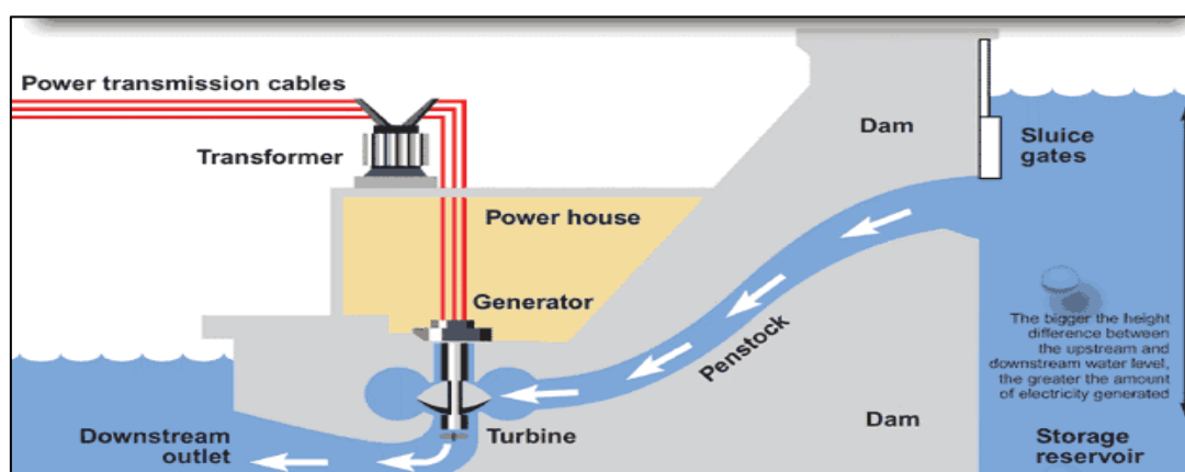
Figure 40: Typical Hydroelectric Power Plant (IRENA, 2022).
