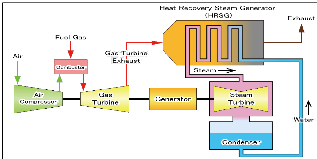
Figure 24: Schematic diagram of a CCGT plant.
