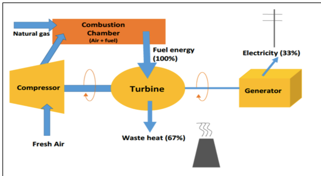
Figure 23: Schematic diagram of an OCGT plant.
