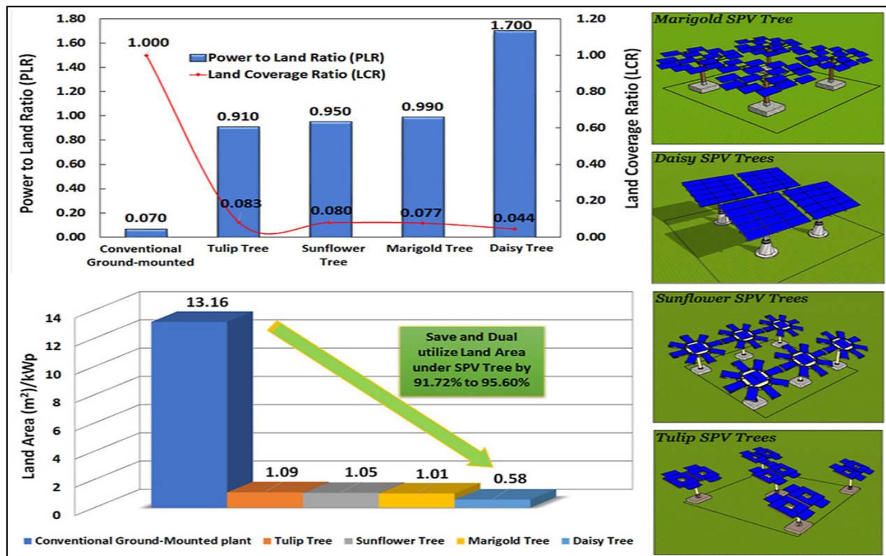
Figure 31: Power to Land Ratio of Solar PV designs.
