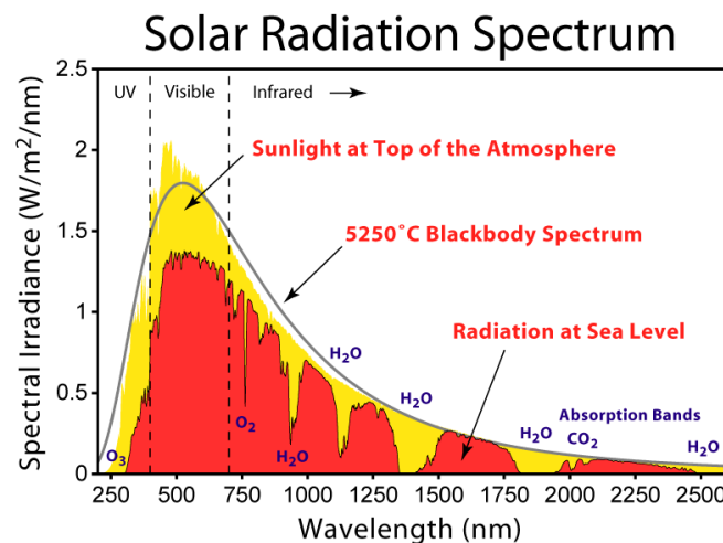
Figure 27: Solar radiation spectrum.
