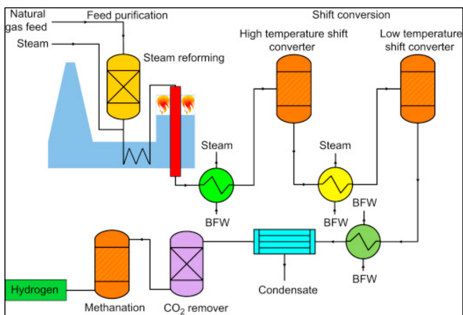
Figure 35: Typical Steam Reforming process to produce Hydrogen.
