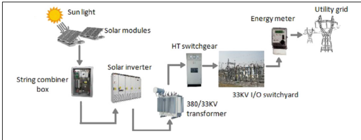
Figure 28: Typical Solar PV Schematic diagram (Kumar et al., 2015).
