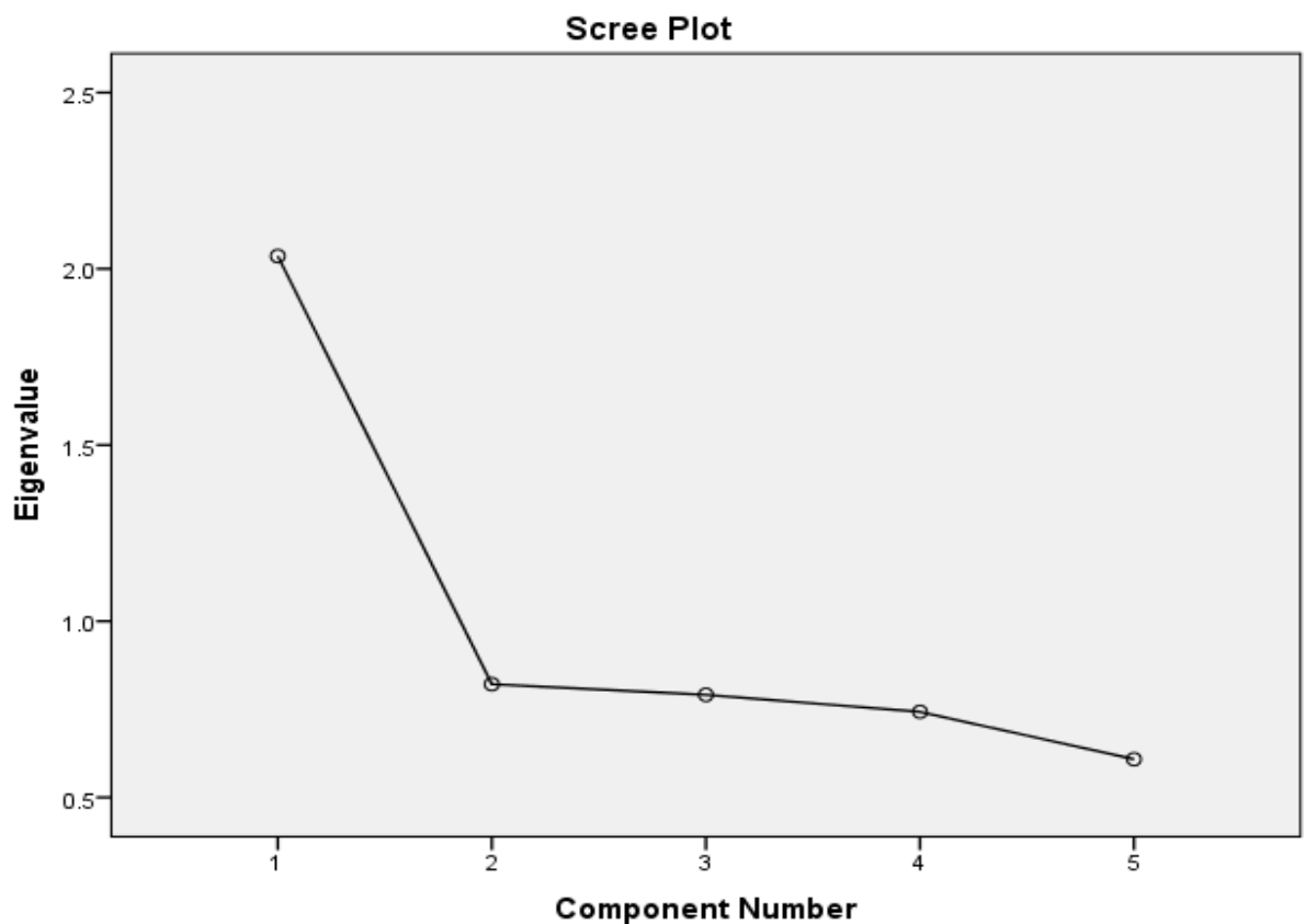
Figure 9: Scree Plot
