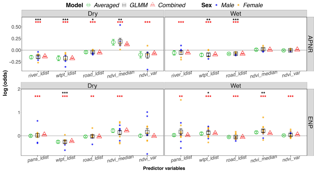
Fig. 5. The population-level RSF coefficient estimates calculated by taking the average of the individual-specific model results ('averaged' model; green circles), mixed effect model with individual elephants as random effect ('glmm'; black squares) and 'combined' model (red triangles) of the APNR and ENP elephants. Asterisks indicate the significant P -value of the 'glmm' and 'combined' model predictor variables ( P -value < 0.001 '***'; < 0.01 '**'; < 0.05 '*'). Blue and orange dots represent the random coefficient estimates of individual elephants for each predictor variable in the 'glmm' model (blue = males; orange = females). For further details, see Table S4 and S5 in Supplementary material available online.
