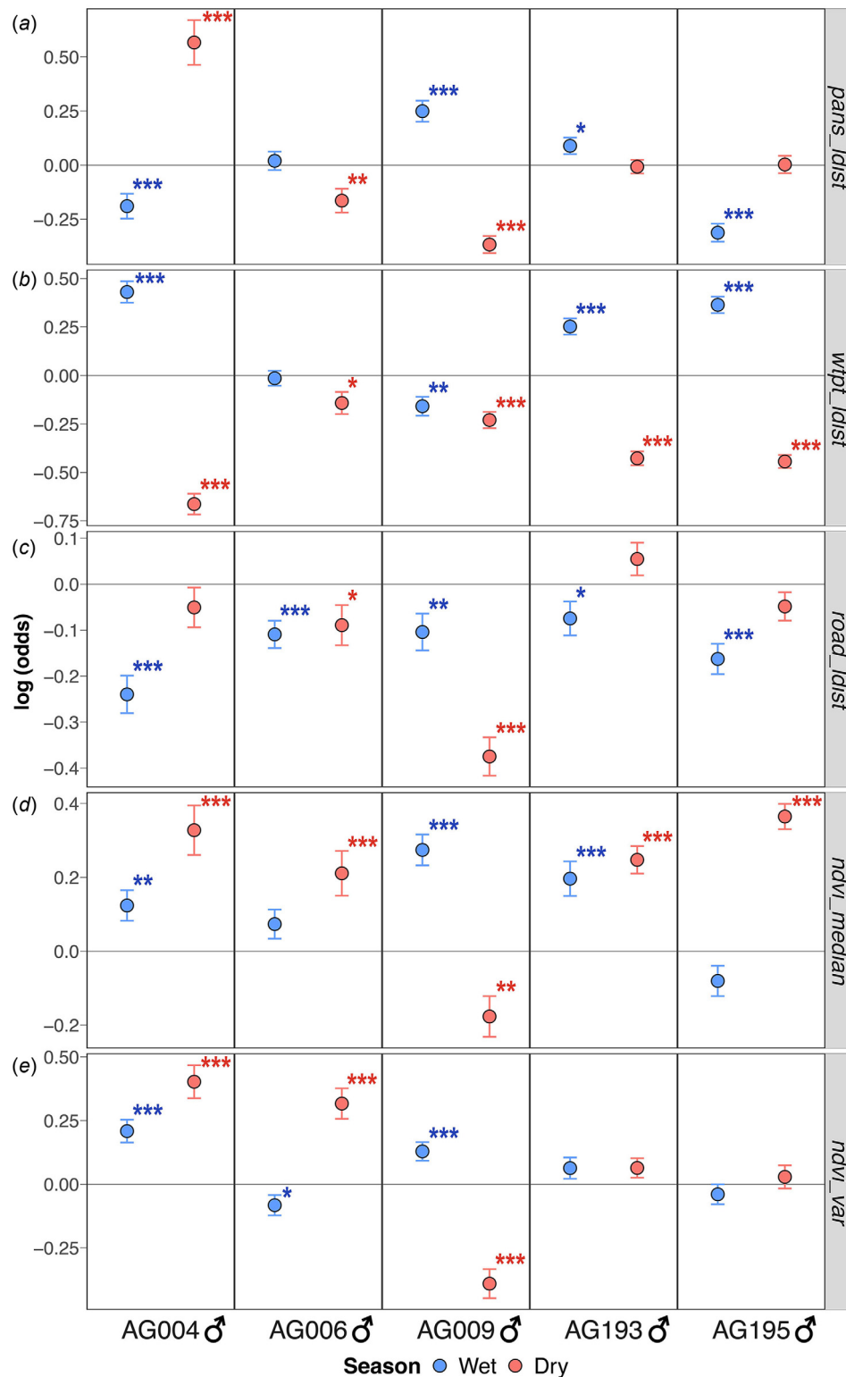
Fig. 3. The coefficient estimates and standard error bars of the environmental variables in individual-specific RSFs of the ENP male elephants. Variables include (a) log distance to pans ( pans_ldist ), (b) log distance to water points ( wtpt_ldist ), (c) log distance to roads ( road_ldist ), (d) seasonal vegetation productivity ( ndvi_median ) and (e) within-season variability of productivity ( ndvi_var ). Asterisks indicate the significant P -value of the predictor variables ( P -value < 0.001 '***'; < 0.01 '**'; < 0.05 '*').
