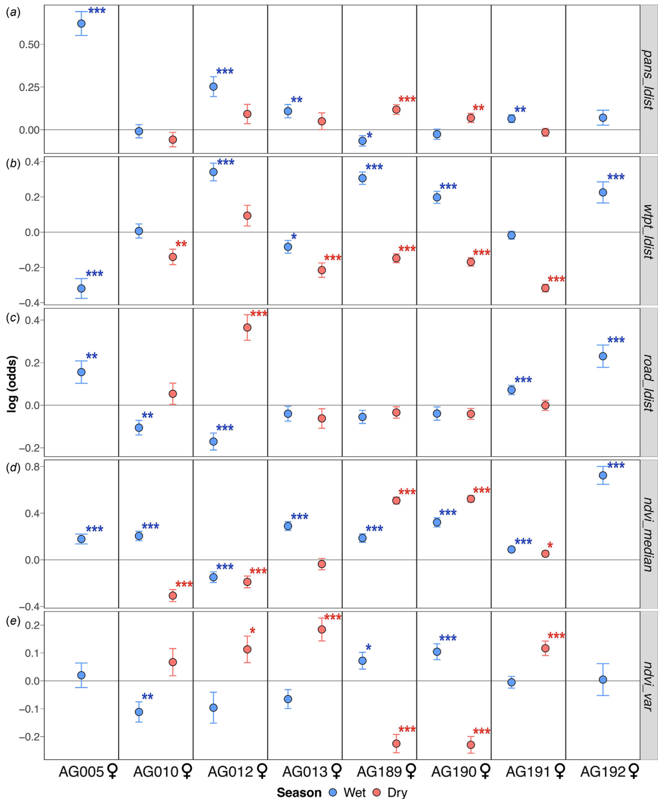
Fig. 4. The coefficient estimates and standard error bars of the environmental variables in individual-specific RSFs of the ENP female elephants. Variables include (a) log distance to pans ( pans_ldist ), (b) log distance to water points ( wtpt_ldist ), (c) log distance to roads ( road_ldist ), (d) seasonal vegetation productivity ( ndvi_median ) and (e) within-season variability of productivity ( ndvi_var ). Asterisks indicate the significant P -value of the predictor variables ( P -value < 0.001 '***'; < 0.01 '**'; < 0.05 '*').
