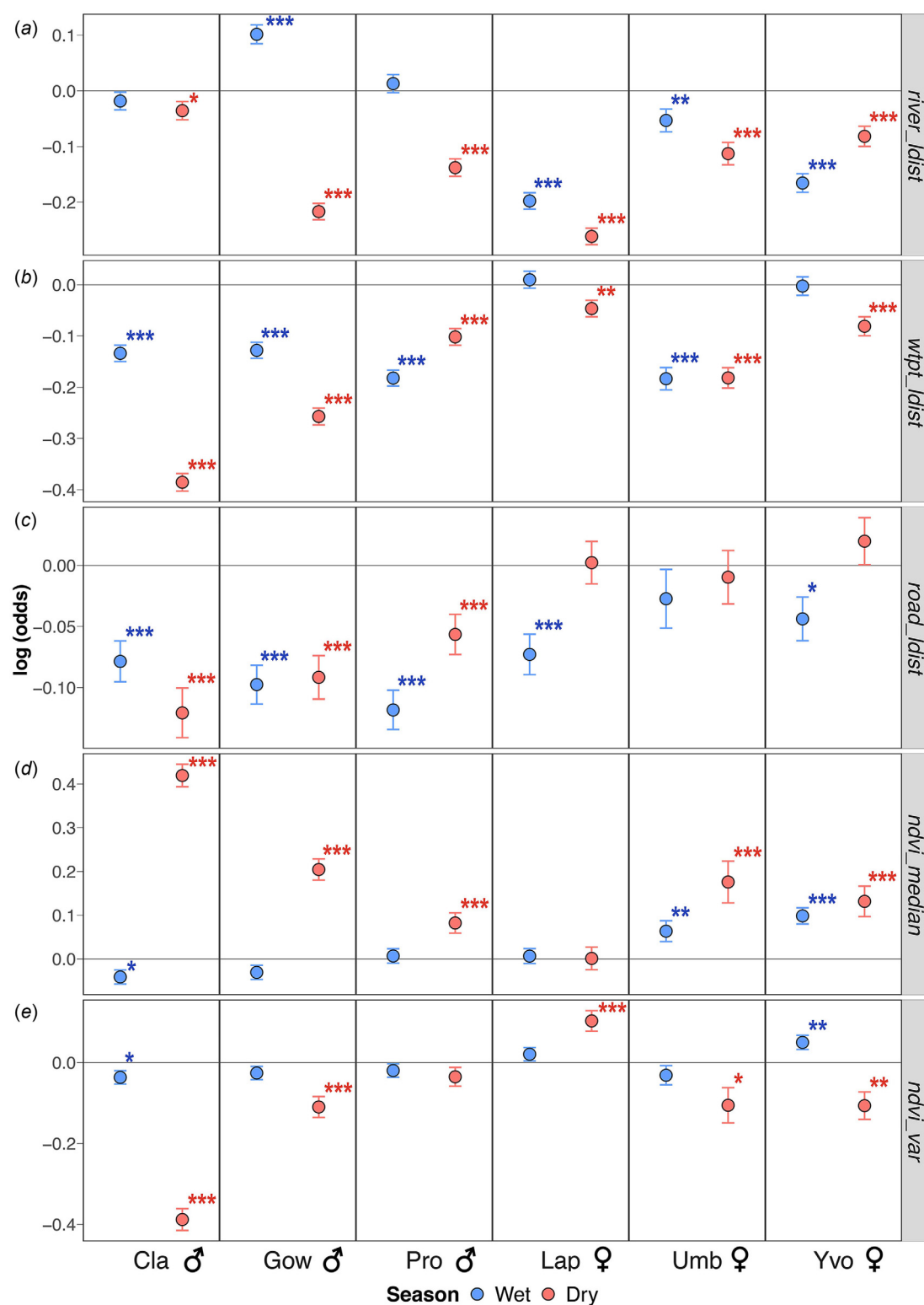
Fig. 2. The coefficient estimates and standard error bars of the environmental variables in individual-specific RSFs of the APNR elephants (male: Cla, Gow, Pro; female: Lap, Umb, Yvo). Variables include (a) log distance to rivers ( river_ldist ), (b) log distance to water points ( wtpt_ldist ), (c) log distance to roads ( road_ldist ), (d) seasonal vegetation productivity ( ndvi_median ) and (e) within-season variability of productivity ( ndvi_var ). Asterisks indicate the significant P -value of the predictor variables ( P -value < 0.001 '***'; < 0.01 '**'; < 0.05 '*').
