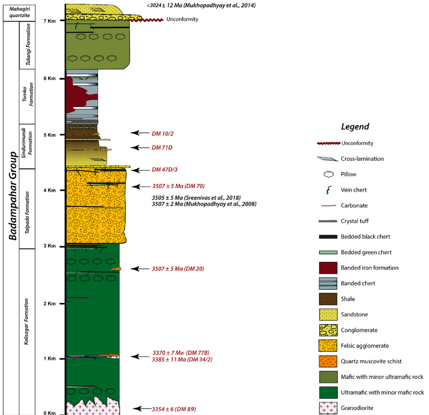
Fig. 3. Stratigraphic column of the Badampahar Group of the Daitari belt (modified from Jodder, 2021) and geochronological information for igneous samples.
