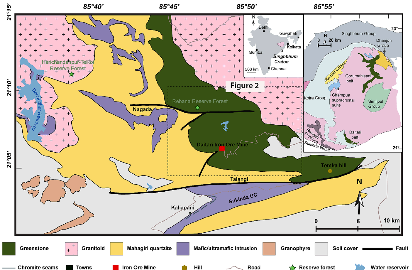
Fig. 1. Geological map of the Daitari Greenstone Belt, Singhbhum Craton, India. Modified after Prasada Rao et al. (1964).
