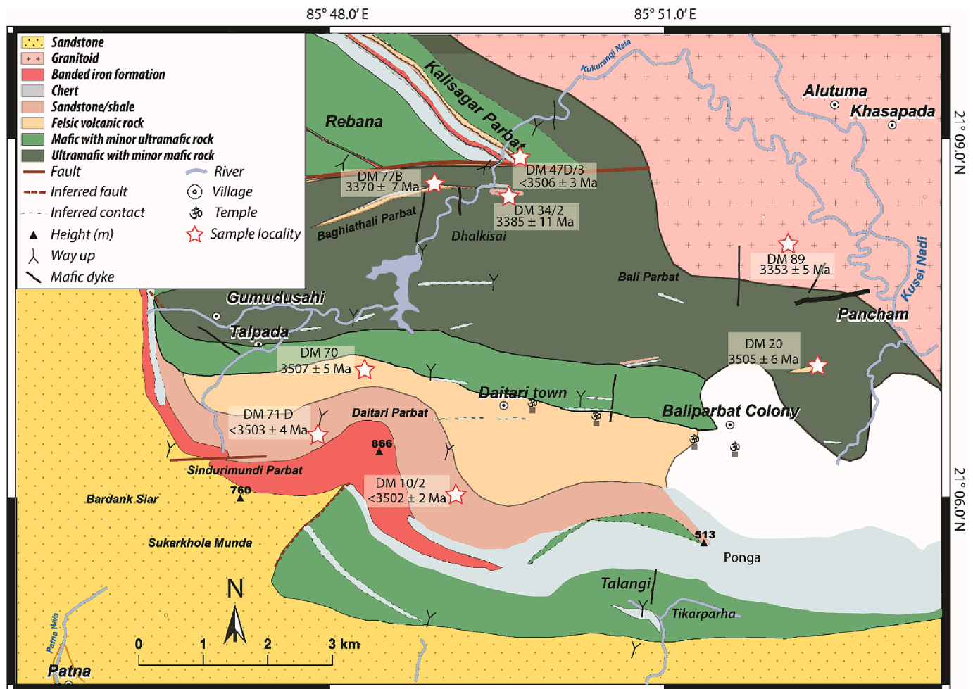
Fig. 2. Geological map of the central portion of Daitari Greenstone Belt (modified after Jodder, 2021). Note star symbols in the map represent sample localities with U-Pb zircon age data.
