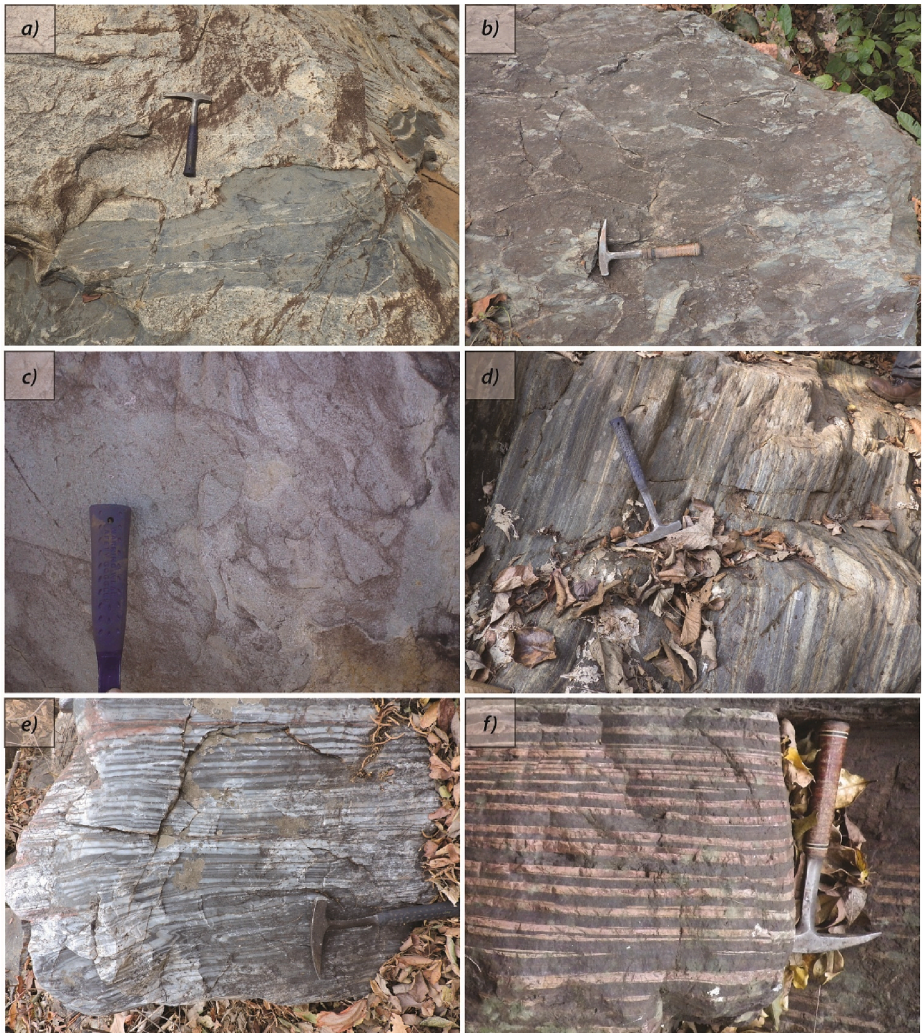
Fig. 4. a) Granodiorite with greenstone xenoliths intrusive into the Kalisagar Formation. b) Pillow basalt, Kalisagar Formation. c) Clast-supported blocks and bombs embedded in a tuffaceous matrix, Talpada Formation. d) Thin, normally graded beds within the turbidite sequence of the Sindurimundi Formation. e) Banded chert, Tomka Formation. f) Banded Iron Formation, Tomka Formation.
