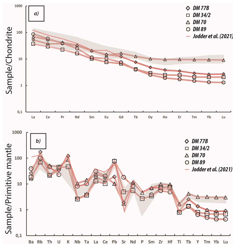
Fig. 5. a) Chondrite-normalized trace element plot of felsic igneous rocks from the Daitari belt (Sun and McDonough, 1985). b) Primitive mantle-normalized trace element plot of felsic igneous rocks from the Daitari belt (McDonough and Sun, 1995). Note trace element data of dacite samples described by Mukhopadhyay et al. (2012) is shown in grey shaded area and trace element data of felsic volcanoclastic sample GUD-3 from the Gorumahisani belt (Jodder et al., 2021) represented by a thin red line. (For interpretation of the references to color in this figure legend, the reader is referred to the web version of this article.)
