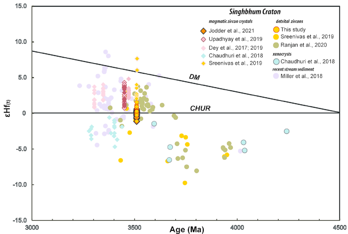
Fig. 9. Plot showing the \epsilon\text{Hf}(t) values vs U-Pb ages of magmatic zircon crystals and sedimentary zircon grains of the Singhbhum Craton.
