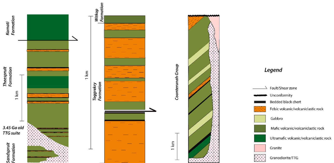
Fig. 10. Stratigraphic columns of the lowermost Onverwacht Group, Nondweni and Coonterunah groups of the Kaapvaal and Pilbara cratons respectively (Figure modified after Viljoen and Viljoen, 1969a; Wilson and Versfeld, 1994a, and Green et al., 2000). (For interpretation of the references to color in this figure legend, the reader is referred to the web version of this article.)
