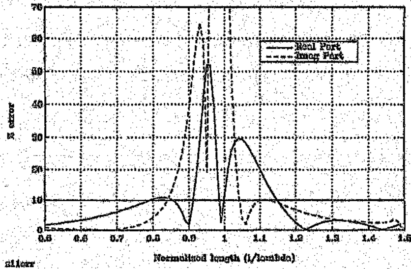
Figure 3.4: Percentage error in the use of Z_{11Free} instead of Z_{11}
