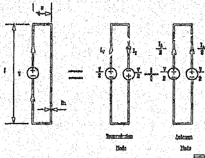
Figure 2.3: The decomposition of the folded dipole current into an antenna mode and a transmission line mode
