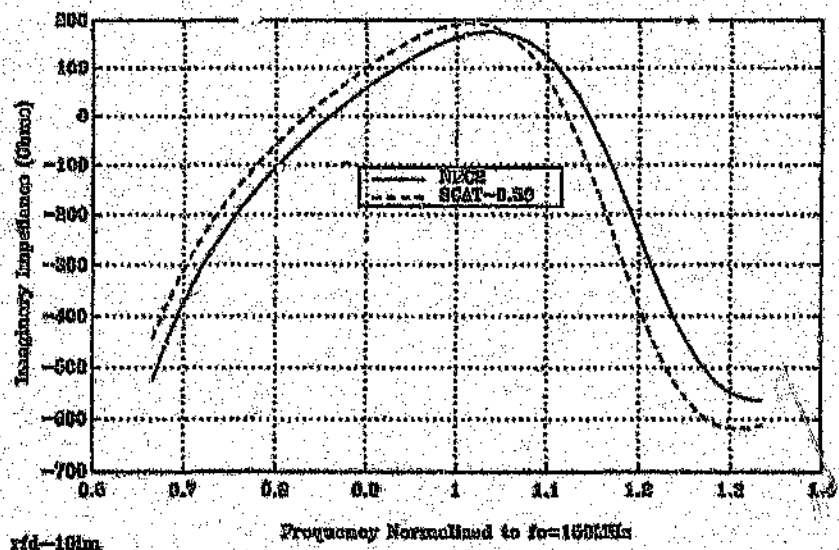
Figure 4.5: Compared folded dipoles input impedance for r = 2\lambda_c/400 ( \epsilon=53.5\Omega )
