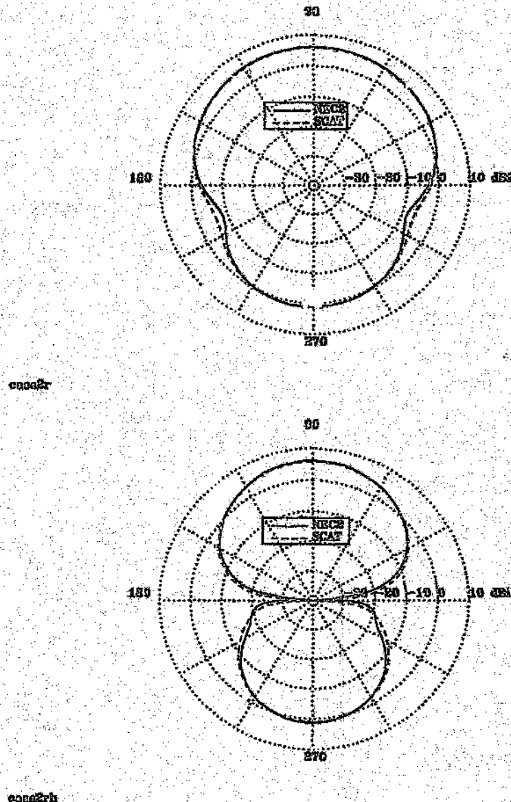
Figure 4.22: NEC vs SCAT radiation pattern – 2 element Yagi-Uda, folded dipole feed
