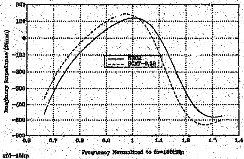
Figure 4.6: Compared folded dipole input impedance for s = 3\lambda_c/400 ( \epsilon=56\Omega )
