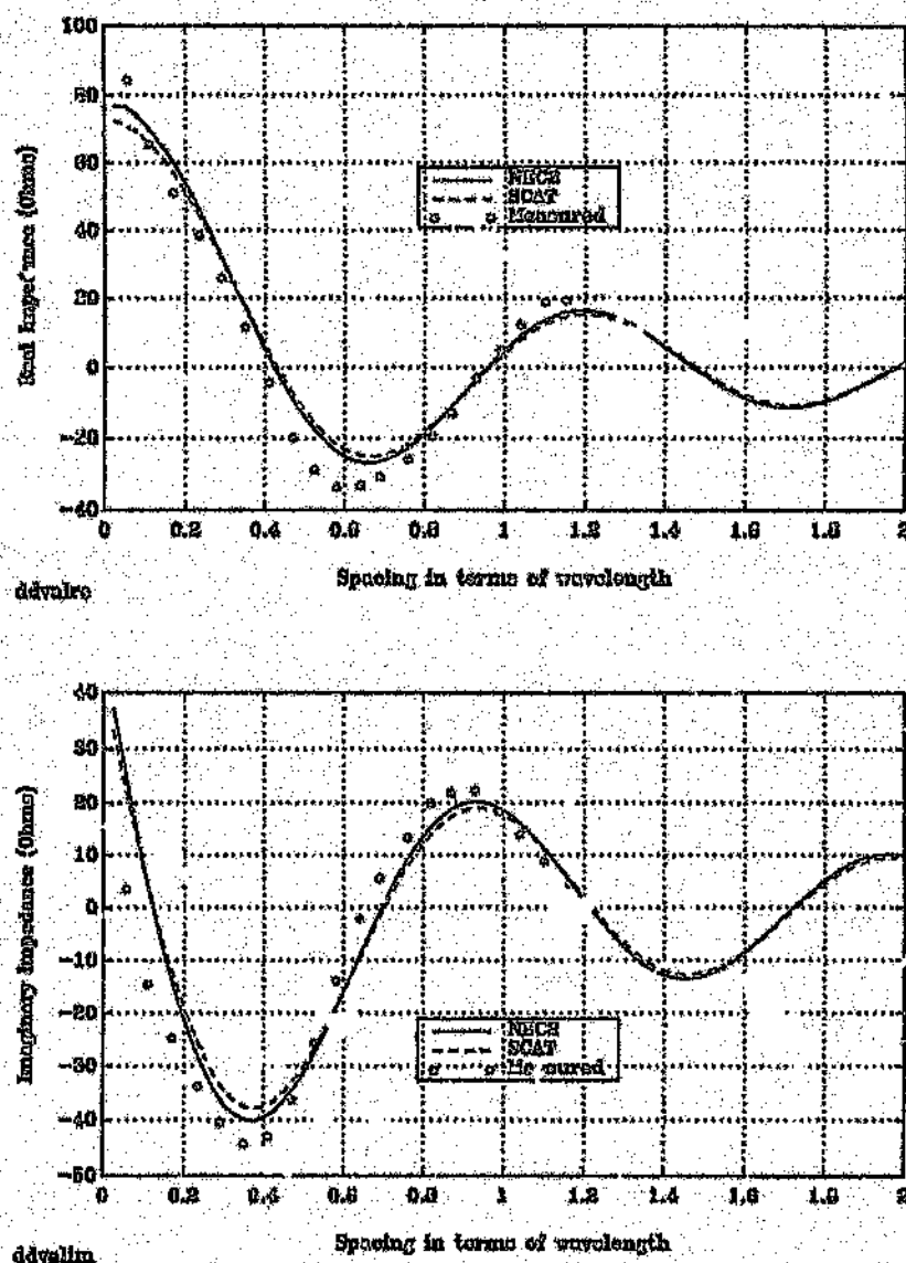
Figure 4.12: Comparison of mutual impedances obtained from NEC2, theoretical (labelled SCAT) and measurement.
