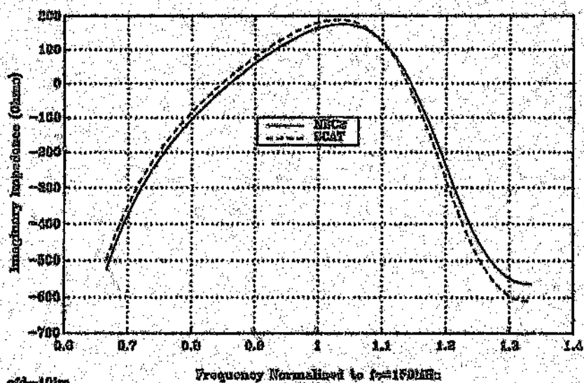
Figure 4.8: Compared FDZin using the full correction. r = 2\lambda_0/400 ( \epsilon=33.05 )
