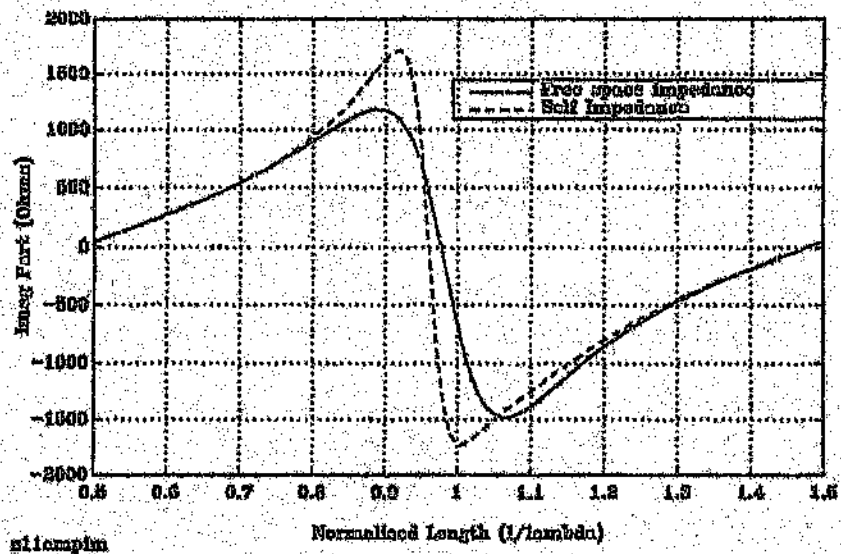
Figure 3.3: Comparison of Free space vs Self impedance of a dipole
