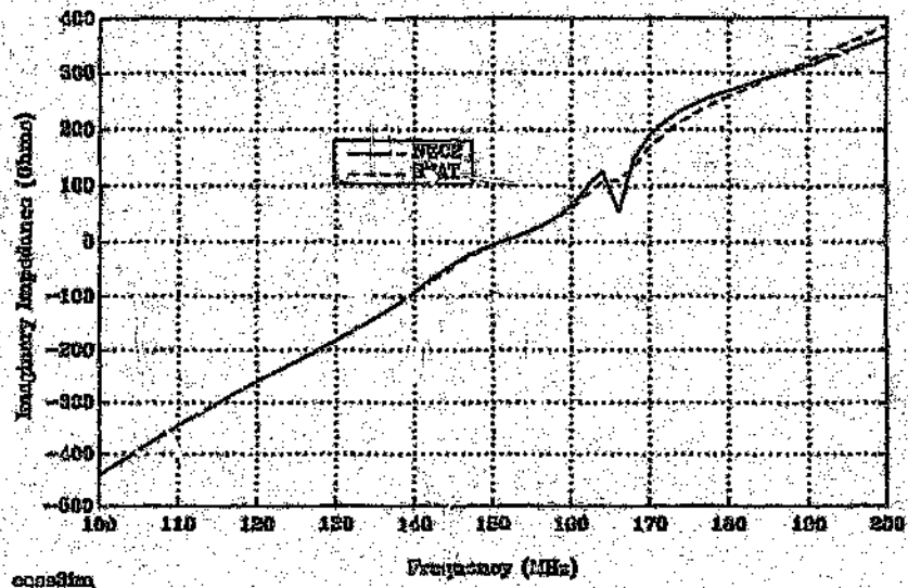
Figure 4.24: NEC vs SCAT impedance -- 5 element Yagi-Uda, dipole feed replacing the folded dipole; (error norm = 6.12Ω)
