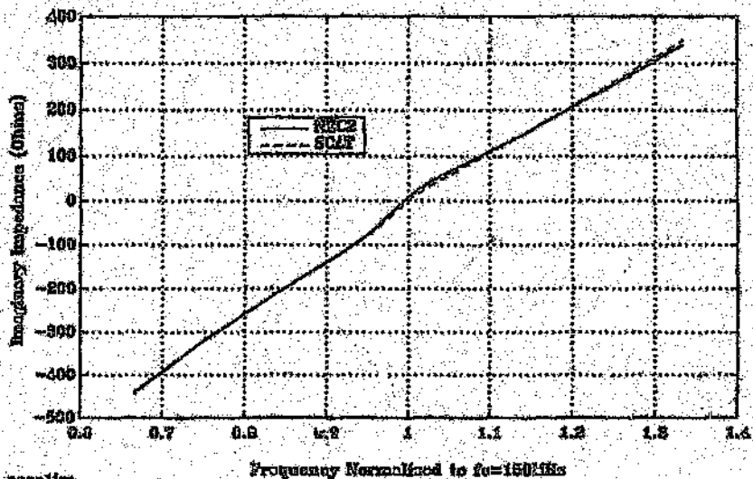
Figure 4.19: NEC vs SCAT input impedance - 2 element Yagi-Uda, dipole feed replacing the folded dipole; (error norm = 2.43 \Omega )
