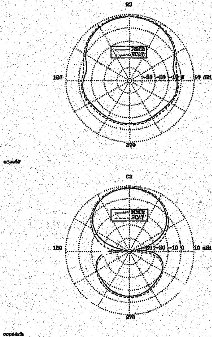
Figure 4.27: NEC vs SCAT radiation pattern - 5 element Yagi-Uda, folded dipole feed
