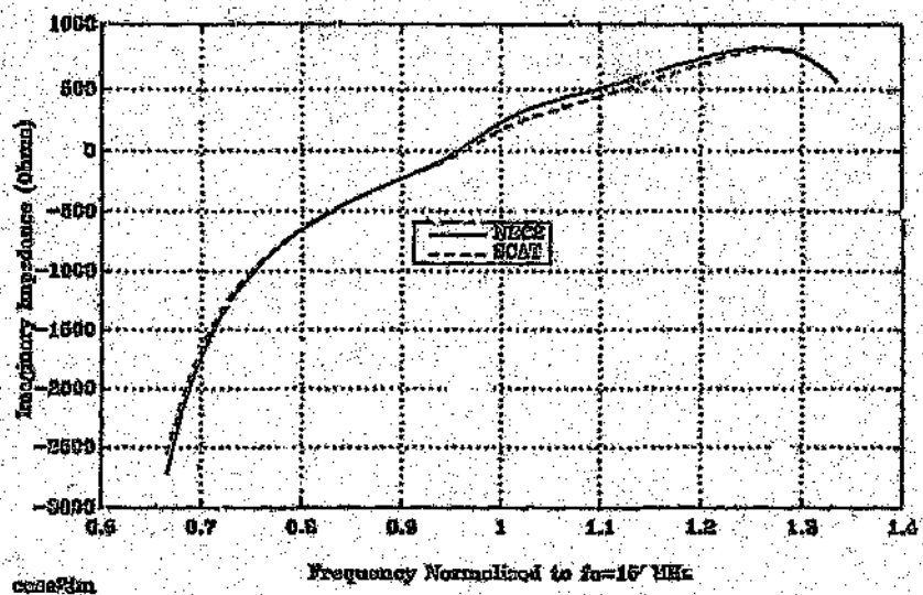
Figure 4.21: NEC vs SCAT input impedance - 2 element Yagi-Uda with a folded dipole feed; (error norm = 36.37\Omega )
