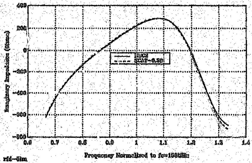
Figure 4.4: Compared folded dipole input impedance for r = \lambda_c/400 ( \epsilon=22.4\Omega )
