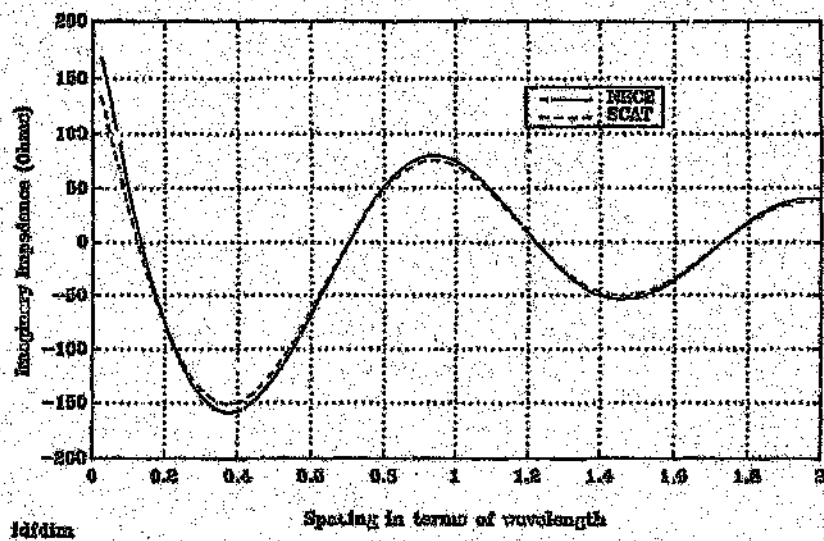
Figure 4.16: Folded dipole to folded dipole mutual impedance
