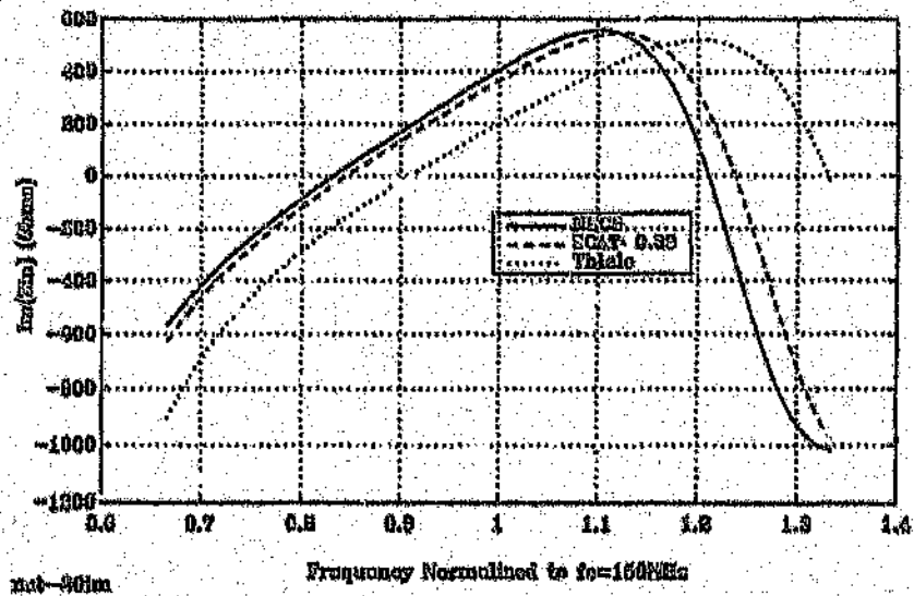
Figure 4.3: Compared folded dipole input impedance for s = \lambda_0/10 . Thiele vs. NEC2 vs. SCAT \alpha = 0.30
