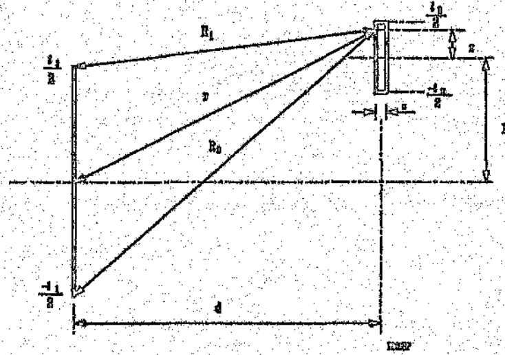
Figure 3.6: Coupling geometry with a folded dipole as the second antenna.
