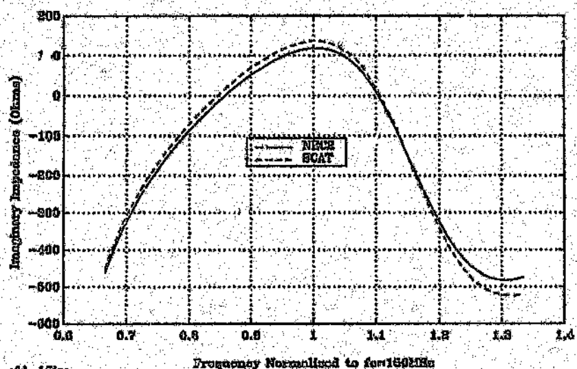
Figure 4.9: Compared FDZin using the full correction. r = 3\lambda_c/400 ( \epsilon=28.68\Omega )
