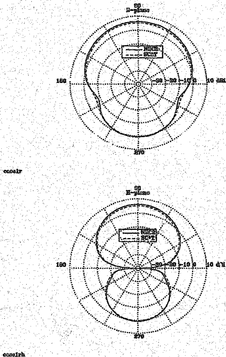
Figure 4.20: NEC vs SCAT radiation pattern – 2 element Yagi-Uda, dipole feed replacing the folded dipole
