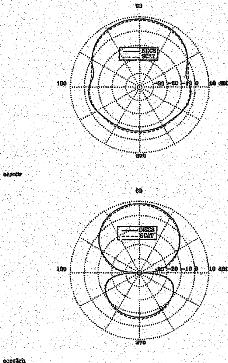
Figure 4.25: NEC vs SCAT radiation pattern - 5 element Yagi-Uda, dipole feed replacing the folded dipole
