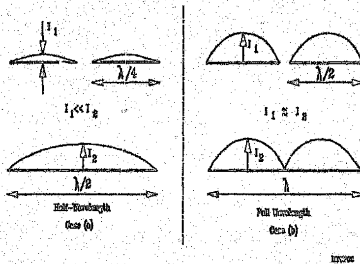
Figure 3.1: The current distribution on half and full wavelength dipoles
