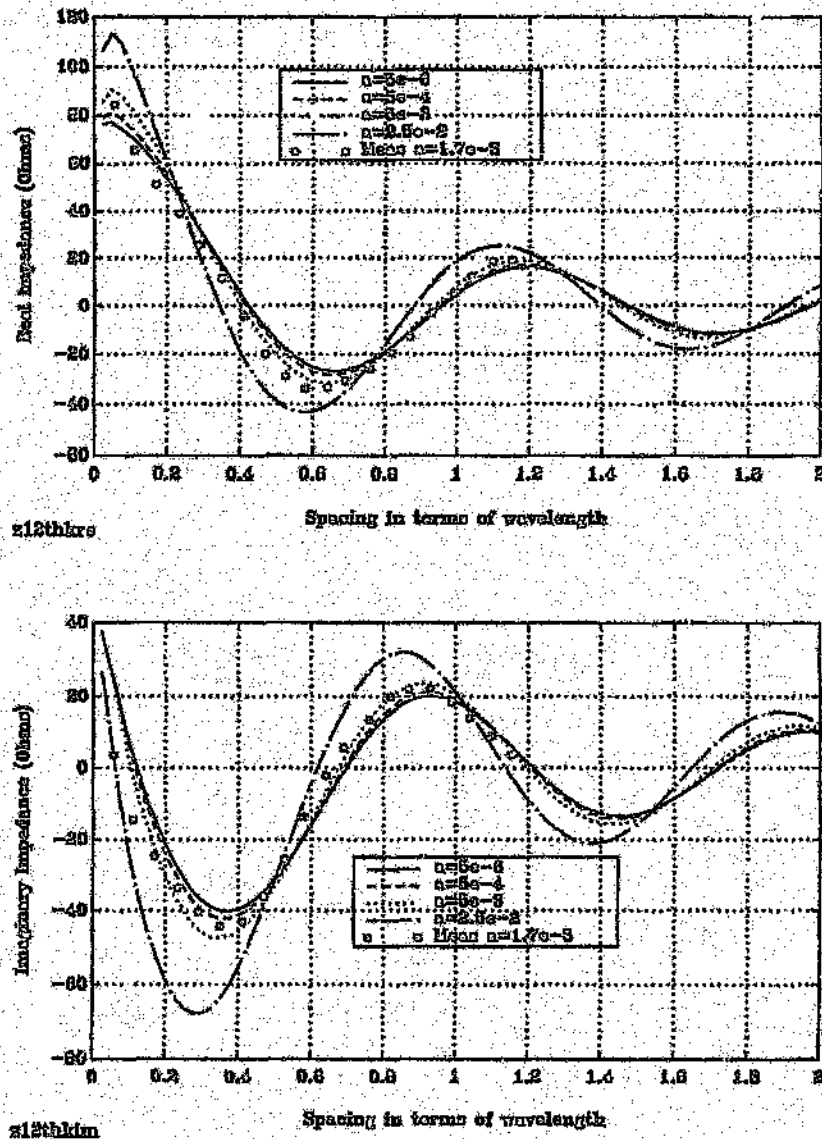
Figure 4.17: The effect of dipole thickness on mutual impedance – curves are obtained from NEC2 and measurement.
