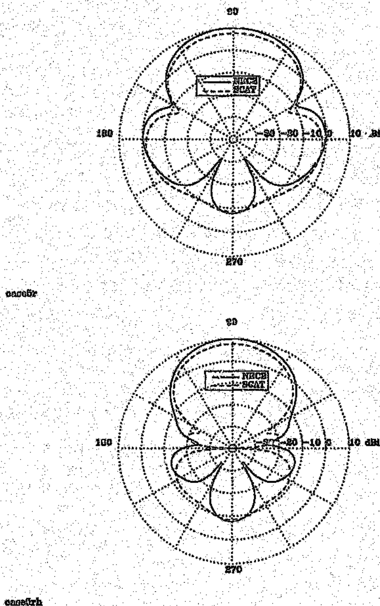
Figure 4.29: NEC vs SCAT radiation pattern - 5 element Yagi-Uda, folded dipole feed, 19mm diameter tubing.
