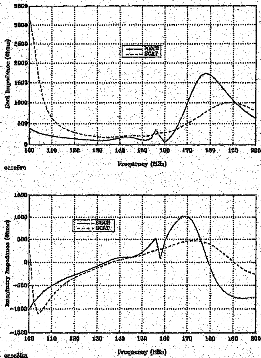
Figure 4.28: NEC vs SCAT impedance -- 5 element Yagi-Uda folded dipole feed, 19mm diameter tubing. (error norm = 382.53Ω)
