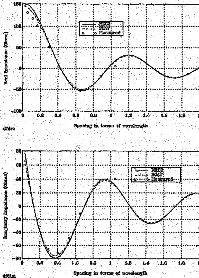
Figure 4.14: Folded dipole to dipole mutual impedance
