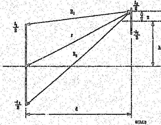
Figure 2.4: Geometry of two parallel dipoles in echelon
