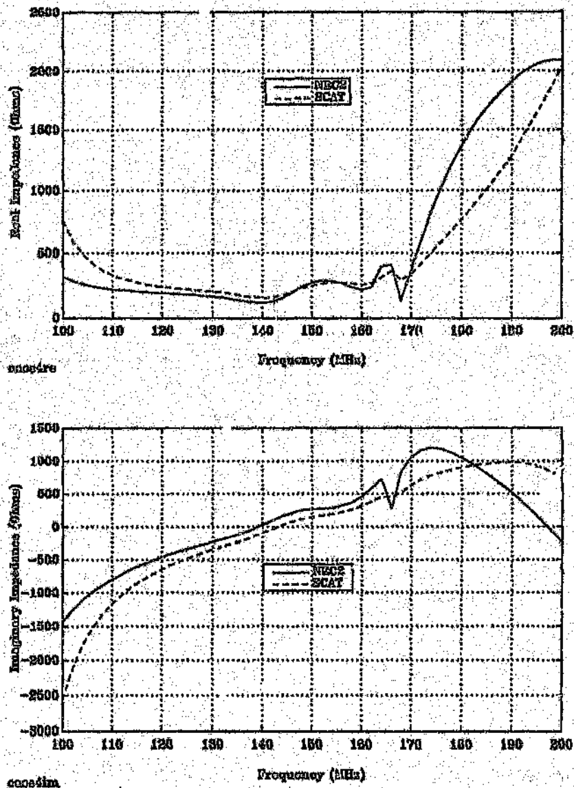
Figure 4.26: NEC vs SCAT impedance -- 5 element Yagi-Uda folded dipole feed; (error norm = 278.85 \Omega )
