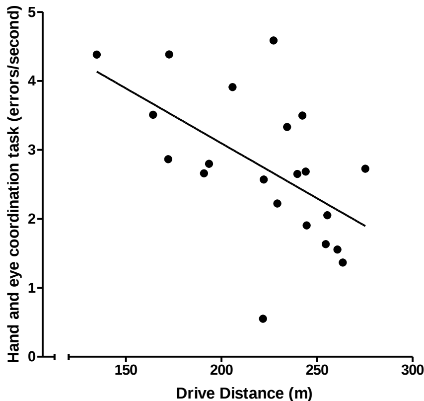
Figure 3.1: The correlation between drive distance (m) and the hand-eye coordination task (errors/second). ( r = -0.563 , p = 0.008 ).
