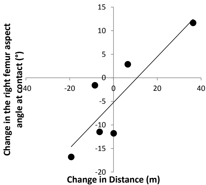
Figure 3.5: The correlation between the change in right femur aspect angle at contact (°) and the change in drive distance (m) in a sub-group of 6 golfers. R^2 = 0.751 r = 0.867 p = 0.025 .
