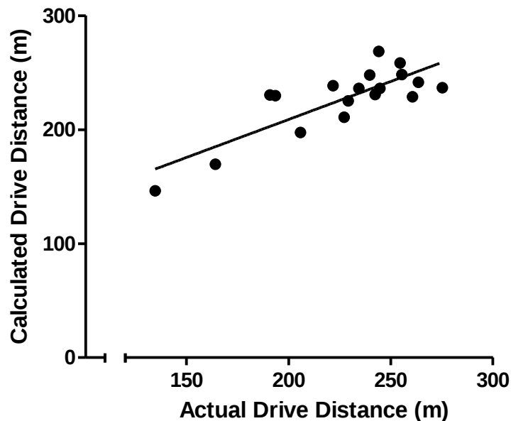
Figure 3.2: The physiological model for achieving drive distances. R^2 value is 0.667 (Adjusted R^2 0.595) p=0.001 . Beta values: Age (years) 1.228* Lean Mass percentage 1.899* Left Leg Balance (seconds) 1.542†. * p < 0.05 † p < 0.01 .
