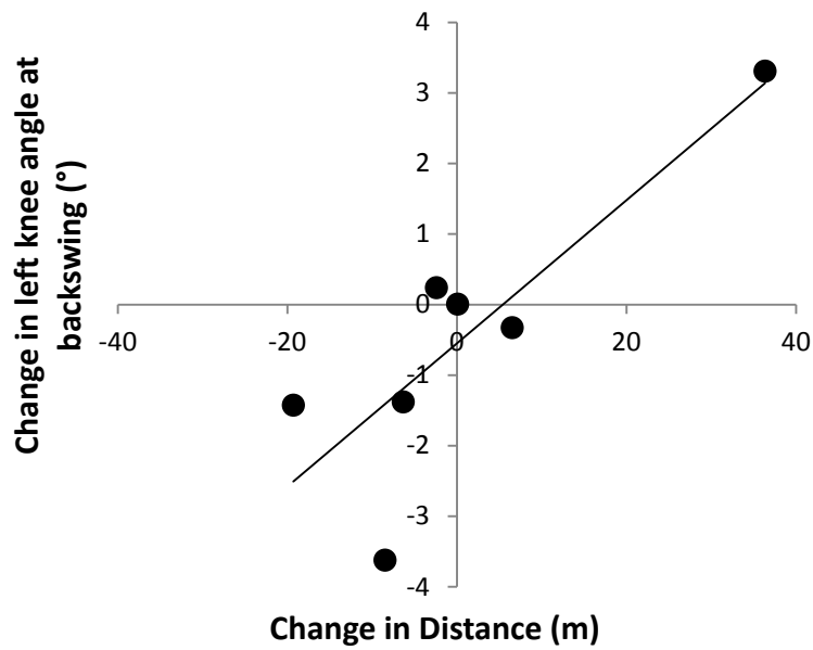
Figure 3.4: The correlation between the change in left knee angle at backswing (°) and the change in drive distance (m) in a sub-group of 7 golfers. R^2 = 0.712 r = 0.844 p = 0.017 .
