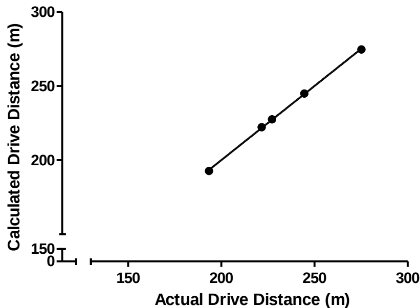
Figure 3.3: The Biomechanical model for achieving drive distances (n=5). Significant contributors include leading arm angle 16.51, left elbow angle -0.265, lateral bend - 1,297. Intercept constant =207.05, R^2=0.9996 , (Adjusted R^2 = 0.9985 ) Overall p value = 0.025
