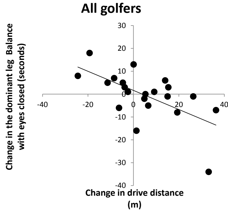
Figure 3.6 A and B: (A) The correlation between the change in balance in the dominant leg with eyes closed (seconds) and the change in drive distance (m) in a group of 21 golfers. R^2 = 0.383 r=-0.619 p=0.003 , and (B) in a group of 8 golfers with scores greater than 89 strokes. R^2 = 0.650 r=-0.807 p=0.016 .
