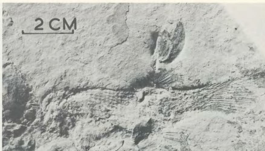
Figure 1 Semionotus cf. capensis from Farm Denwood, Bird's River, E. Cape. C—Dt. II 355. B.P.I.
