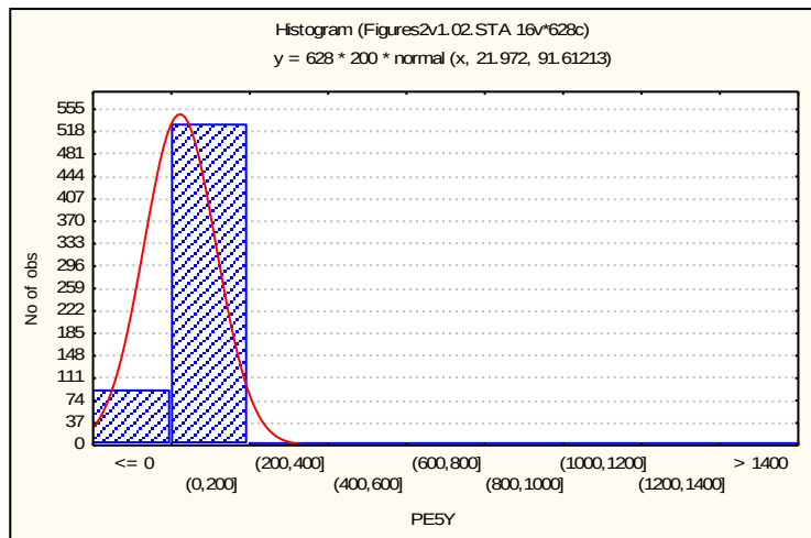
Figure B15: Histogram of P-E Ratio Data for Five-Year Average
