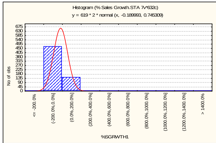
Figure B2: Histogram of Sales Growth Data for Two-Year Average
