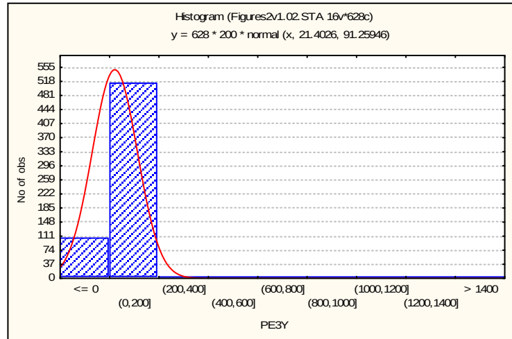
Figure B13: Histogram of P-E Ratio Data for Three-Year Average
