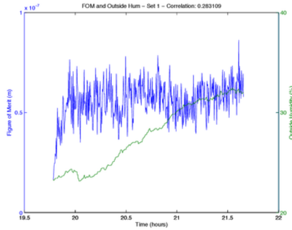
Figure 3.20: FoM and humidity after [weighted moving average] filtering corrections (01 March 2011): humidity increases almost linearly but remains relatively low while figure of merit rapidly increases from 20 nm to about 60 nm and tends to stabilise at that level for the remaining time; this indicates improvement over simple moving average previously used
