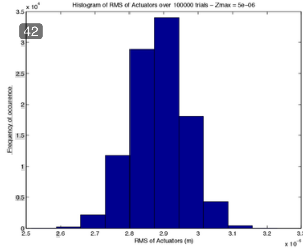
Figure 3.10: Histogram of acceptable RMS actuator displacements using SVD: with z_{\max} = 5 \times 10^{-6} metre, acceptable controllability (less than 0.1 arcsecond RMS tip/tilt errors) is achieved via SVD with a 99.5% probability
