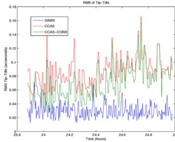
Figure 3.24: RMS of tip/tilts after [exponential moving average] filtering corrections (01 March 2011): according to SAMS (our approach using QR/SVD and exponential moving average, in blue) the system is under control; this is also the case with the output from CCAS before (red) and after GRoC corrections (green); this confirms an improvement over previous methods
