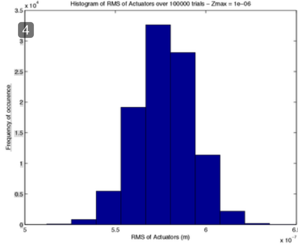
Figure 4.1: Histogram of RMS actuators for z_{\max} = 10^{-6} metre: RMS actuator displacements varies between 0.5 and 0.65 microns with a distribution close to normal, and the primary mirror can be controlled with QR or SVD
