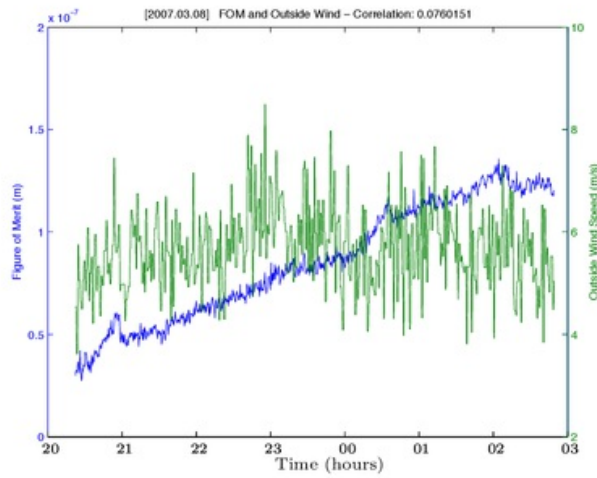
Figure 2.5: FoM and outside wind speed vs time (08 March 2007): wind speed is relatively stable and not highly correlated to FoM, and they don't have similar behavior
