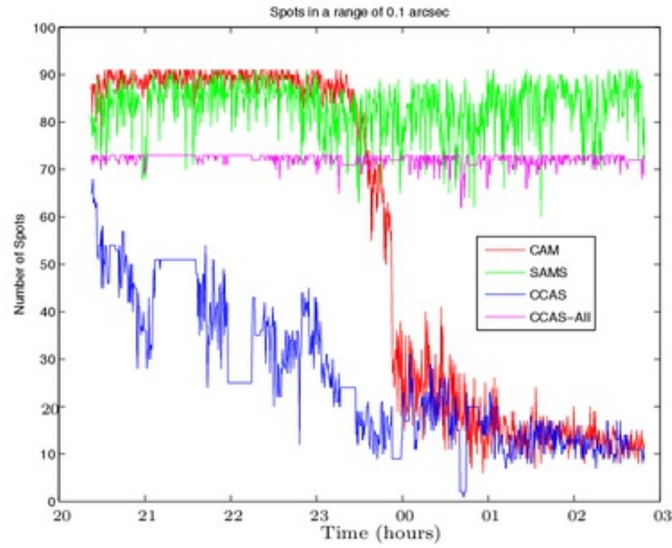
Figure 3.15: Spots in acceptable range before corrections (08 March 2007): SAMS (green) believes that almost all the time, at least 80 segments are in acceptable range (0.1 arcsecond) while CCAS indicates that out of 73 segments in general (purple), at most 60 and decreasing (blue), are in acceptable range; our approach (red) agrees with SAMS, then switches to CCAS around 11pm, indicating a possible disturbance
