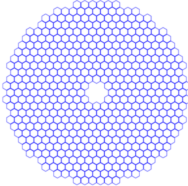
Figure 1.4: Layout of the TMT primary mirror
