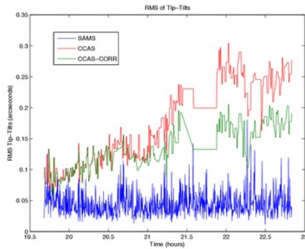
Figure 3.17: RMS of tip/tilts after least squares corrections (13 July 2010): from our approach (QR/SVD), SAMS believes the primary mirror is under control (blue), which is in disagreement with CCAS (red before GRoC corrections and green after GRoC corrections); this suggests further improvements should follow
