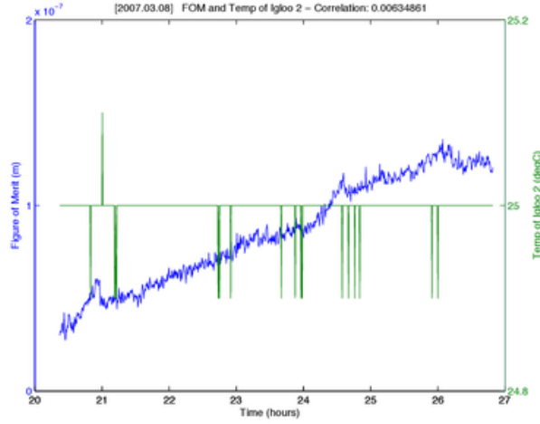
Figure 2.9: FoM and temp of igloo 2 vs time (08 March 2007): temperature is relatively low, stable and not highly correlated to FoM, and they don't have similar behavior
