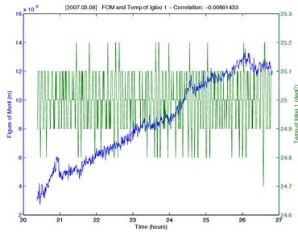
Figure 2.8: FoM and temp of igloo 1 vs time (08 March 2007): temperature is relatively low, stable and not highly correlated to FoM, and they don't have similar behavior
