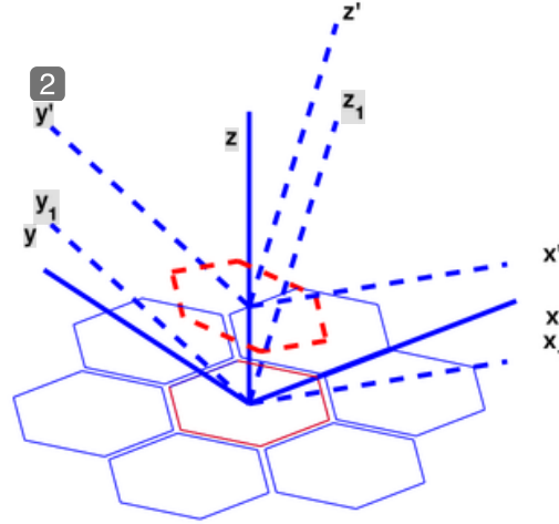
Figure 3.1: Different axes types for the SALT primary mirror
