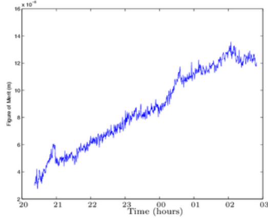
Figure 2.1: Figure of merit in one night (08 March 2007). Figure of merit increasing with time and going beyond 60\text{nm} = 6 \times 10^{-8}\text{m} indicates failure of primary mirror control with time
