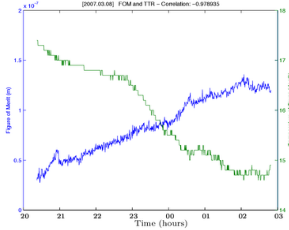
Figure 2.6: FoM and temp of truss vs time (08 March 2007): temperature is relatively low and highly correlated to FoM, and FoM increases as temperature decreases
