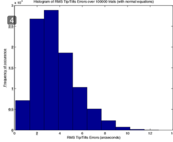
Figure 3.7: Histogram of RMS tip/tilt errors using normal equations: the probability is very high that the mirror is out of acceptable alignment (probability is about 10^{-4} for the mirror to be in the 0.1 arcsecond range) while SAMS believes the mirror is under control
