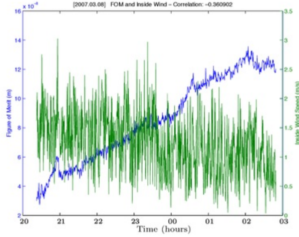
Figure 2.4: FoM and inside wind speed vs time (08 March 2007): wind speed is relatively stable and not highly correlated to FoM, and they don't have similar behavior
