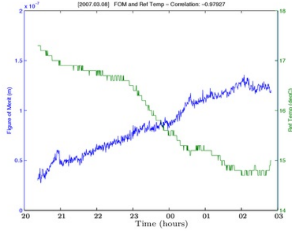
Figure 2.7: FoM and reference temp vs time (08 March 2007): temperature is relatively low and highly correlated to FoM, and FoM increases as temperature decreases
