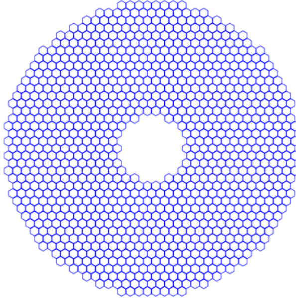
Figure 1.5: Layout of the E-ELT primary mirror
