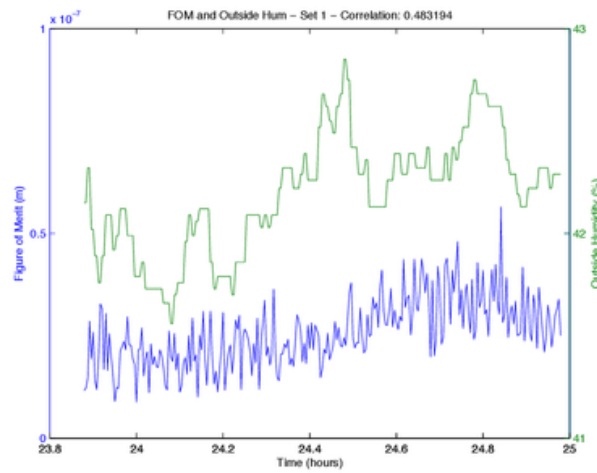
Figure 3.23: FoM and humidity after [exponential moving average] filtering corrections (01 March 2011): figure of merit is stable and below 50 nm, and not highly correlated to humidity which is relatively low and follows a pattern similar to that of figure of merit; this suggests exponential moving average is an improvement over weighted moving average
