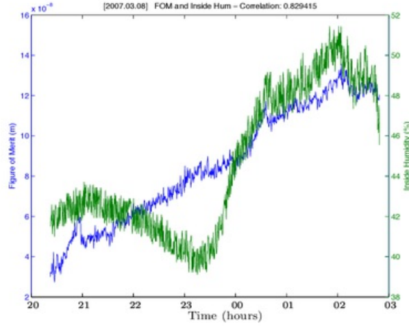
Figure 2.2: FoM and inside humidity vs time (08 March 2007): humidity is relatively low and highly correlated to FoM, but they don't have similar behavior
