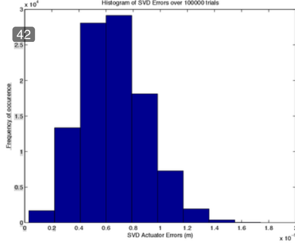
Figure 3.6: Histogram of RMS actuator errors using SVD: algorithmic accuracy is not ideal but much better than that of normal equations and QR
