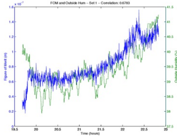
Figure 3.16: FoM and humidity after least squares corrections (13 July 2010): figure of merit increases rapidly at start, then stabilises, but still gets out of range; its curve follows that of humidity, but with reduced correlation compared to the case before corrections
