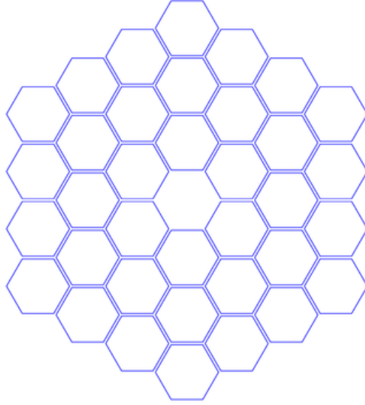
Figure 1.3: Layout of one KECK primary mirror
