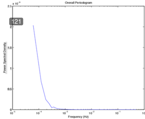
Figure 2.12: Spectrum of relative heights (30 July 2010): this indicates a low pass process
