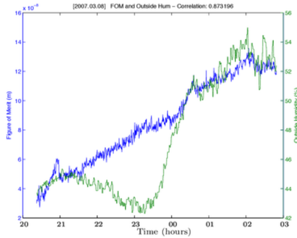
Figure 3.13: FoM and humidity before corrections (08 March 2007): the behavior of figure of merit shows concern about mirror controllability while humidity, although strongly correlated to figure of merit, displays a different pattern
