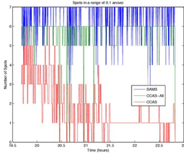
Figure 3.18: Spots in acceptable range after least squares corrections (13 July 2010): according to SAMS (blue), at least 5 of 7 segments are in the 0.1 arcsecond range almost all the time, while from CCAS, out of 5 or 6 segments, at most 5 (and decreasing) are in the 0.1 arcsecond range; this confirms need of further improvements
