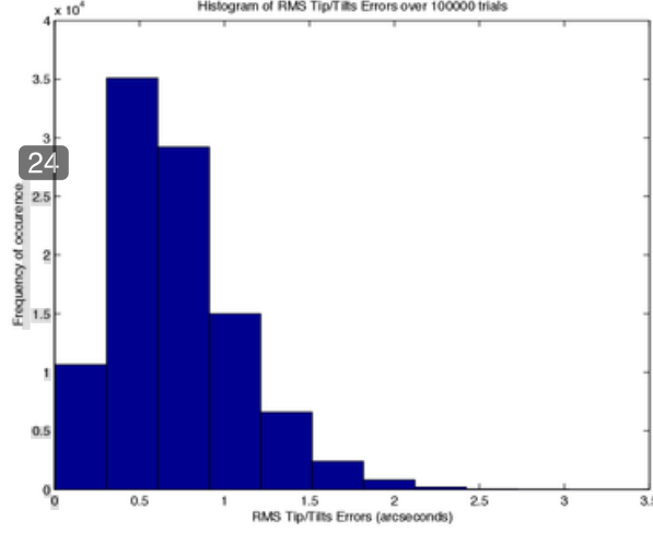
Figure 3.9: Histogram of RMS tip/tilt errors using SVD: the probability is high (but not as in normal equations and QR) that the mirror is out of acceptable alignment (probability is about 5 \times 10^{-3} for the mirror to be in the 0.1 arcsecond range) while SAMS believes the mirror is under control
