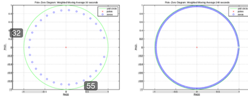
Figure 3.12: Pole-zero diagram of the weighted moving average filter using the last 30 measurements (left) and 240 measurements (right)
