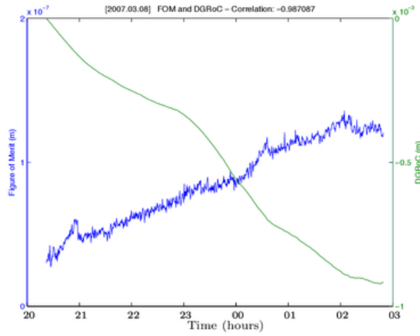
Figure 2.10: FoM and DGRoC vs time (08 March 2007): DGRoC is relatively low, highly correlated to FoM, and decreases as FoM increases
