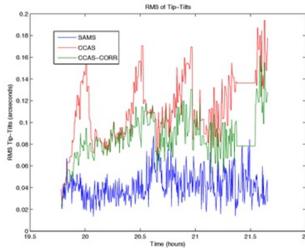
Figure 3.21: RMS of tip/tilts after [weighted moving average] filtering corrections (01 March 2011): according to SAMS (blue) the system is under control, which is to some extent in agreement with CCAS after GRoC corrections (green); output from CCAS before GRoC corrections goes out of range from time to time but attempts to recover; this confirms weighted moving average as an improvement over simple moving average
