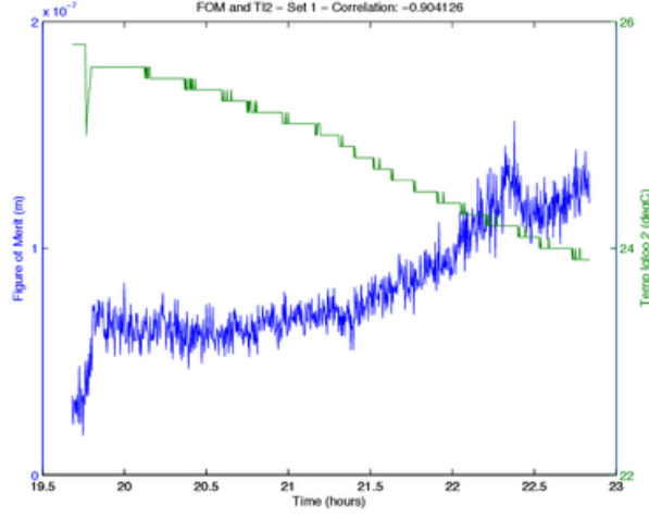
Figure 3.19: Figure of Merit and Temperature of Igloo 2 after least squares corrections (13 July 2010): temperature of igloo 2 decreases while FoM increases and they are strongly correlated; lack of stability of temperature of igloo can have a serious impact on the outcome of the electronics
