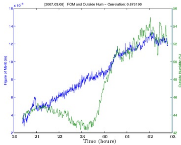
Figure 2.3: FoM and outside humidity vs time (08 March 2007): humidity is relatively low and highly correlated to FoM, but they don't have similar behavior
