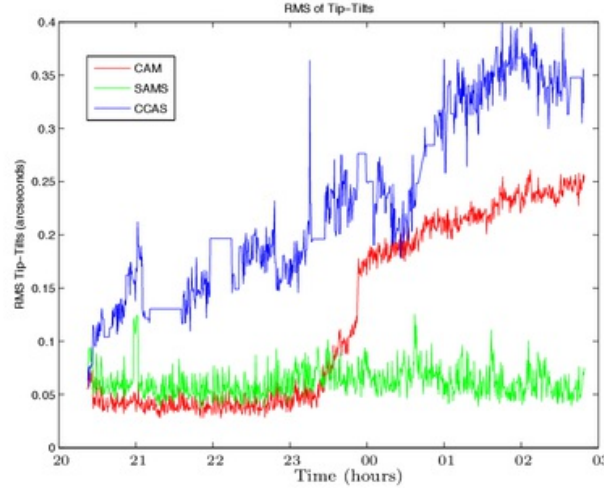
Figure 3.14: RMS of tip/tilts before corrections (08 March 2007): SAMS believes the mirror is under control (green), which is in disagreement with CCAS (blue); our calculations (red) confirms that there might be a problem with SAMS; the system seems to undergo a sudden disturbance around 11pm, which is not captured by SAMS
