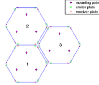
Figure 1.2: SALT segments with sensors and mounting points
