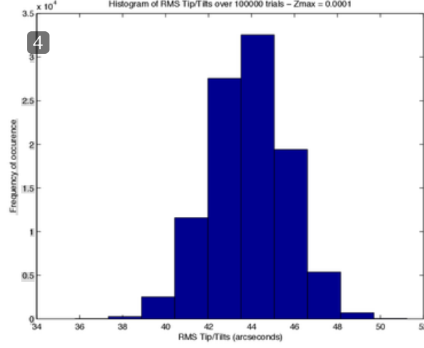
Figure 4.3: Histogram of RMS tip/tilt for z_{\max} = 10^{-4} metre: this clearly shows that the primary mirror is far out of acceptable alignment since RMS tip/tilts is far greater than 0.1 arcsecond; this corresponds to an uncontrollable primary mirror configuration
