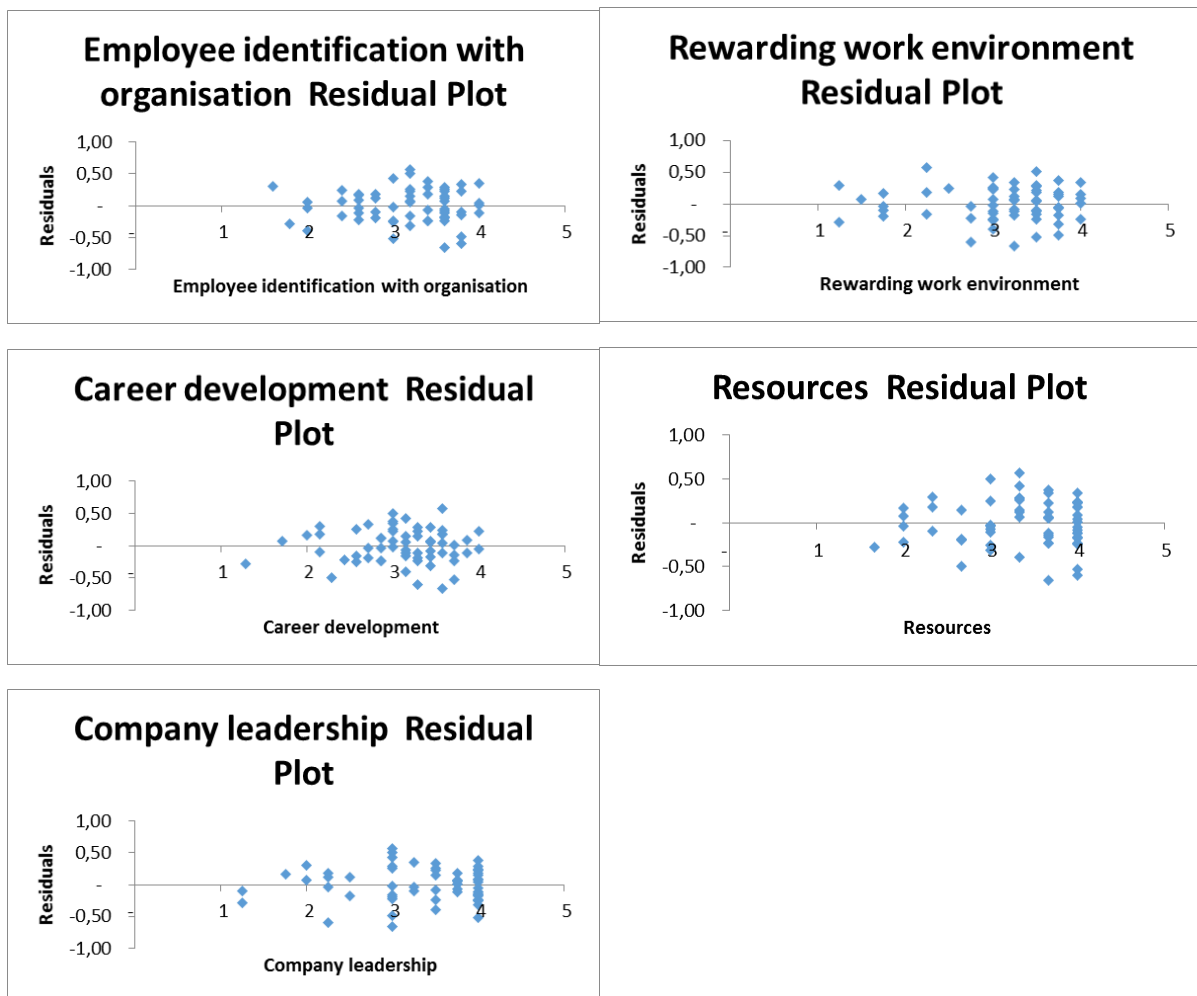
Fig 7: Graphs showing residual plots
