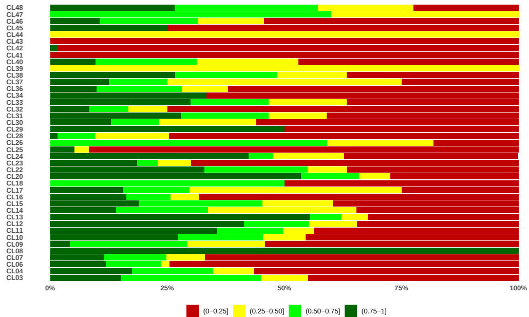
Figure 4.14: Coveralls: distribution of Delta Maintainability (DMM). Each colour represent the range and the size of the bar is the percentage of the patches whose impact lies within the range.
