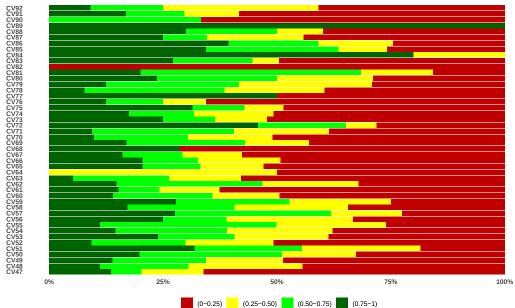
Figure 4.17: Codecov Cont: distribution of maintainability (DMM) across revisions. Each colour represent the range and the size of the bar is the percentage of the patches whose impact lies within the range.
