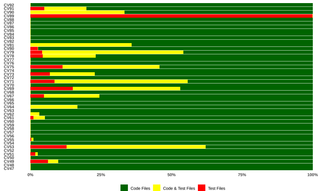
Figure A.3: Exploratory Question 1: Codecov Cont - Coevolution of Production and Test code. Size of bar represents the proportion of builds over the total number of builds in each category.
