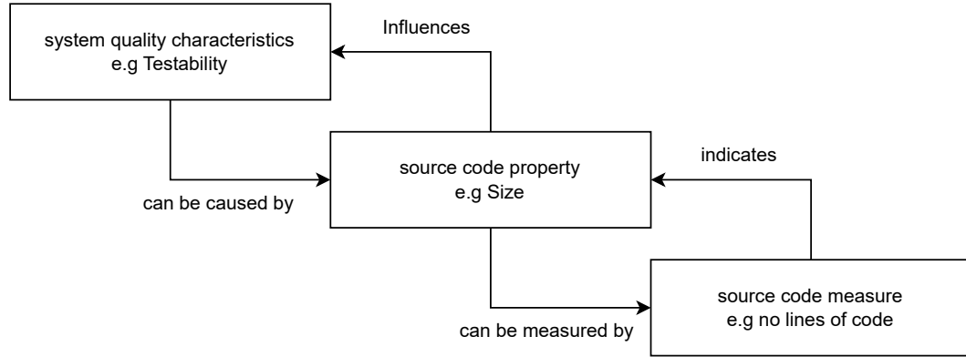
Figure 2.3: ISO/IEC 25010 - SIG Metrics - Measure Mapping Flow
