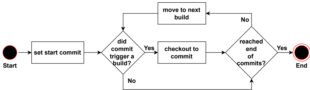
Figure 3.4: Build and Commit Hash Relation
