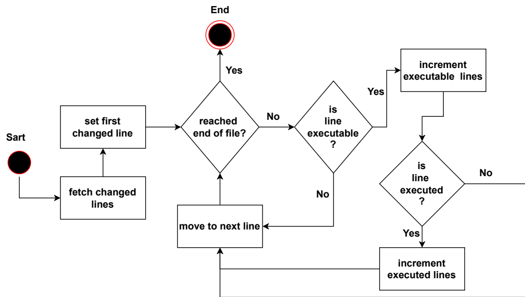
Figure 3.7: Covered Lines Block: LineMapper function
