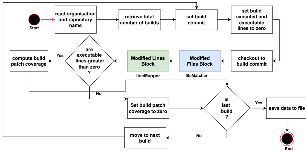
Figure 3.5: Algorithm pipeline-flow
