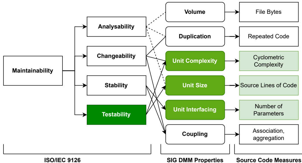
Figure 2.2: Relation between SIG Maintainability Model and source code measures and ISO/IEC 25010 quality characteristics
