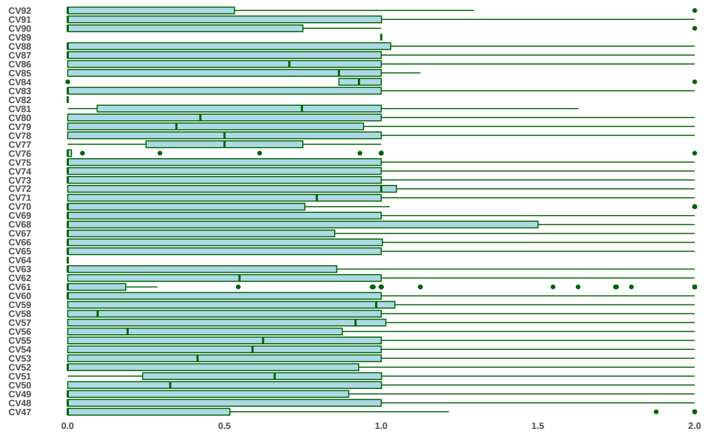
Figure 4.19: Codecov CRAP Metric Cont: distribution of the delta CRAP metric across revisions.
