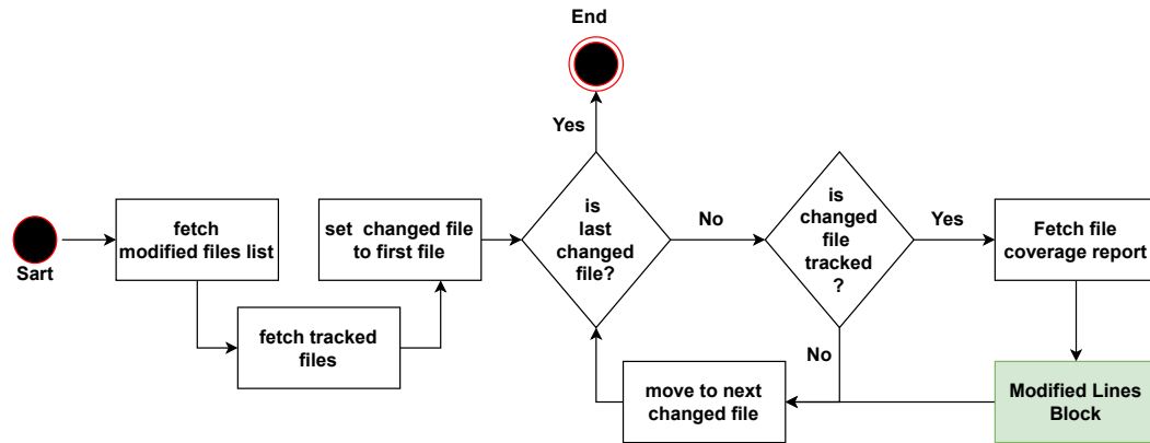
Figure 3.6: Modified Files Block: FileMatcher function
