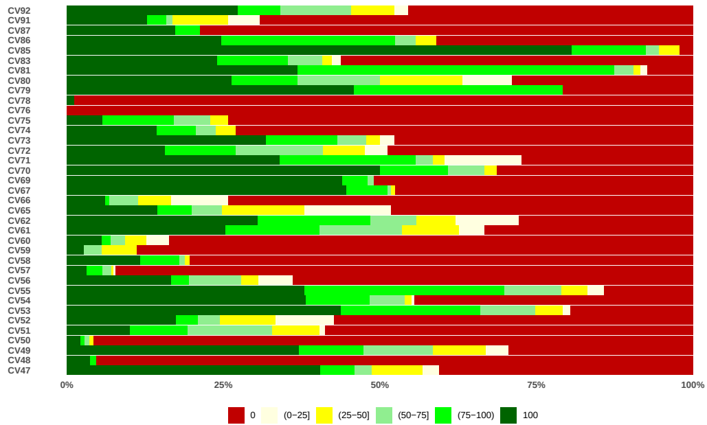
Figure 4.9: Native Rest API Patch Coverage From Codecov: Distribution of patch coverage across revisions. Each colour represent the range and the size of the bar is the percentage of the patches whose coverage lies within the range.
