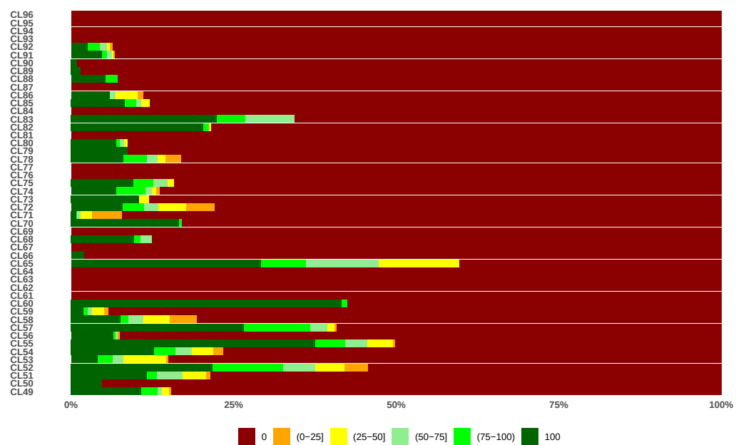
Figure H.4: Coveralls Patch Coverage distribution Cont: The bar chart illustrates the distribution of Patch Coverage in patches affecting Code and Non-Code files, with each bar representing the percentage of patches falling within a specific coverage range.
