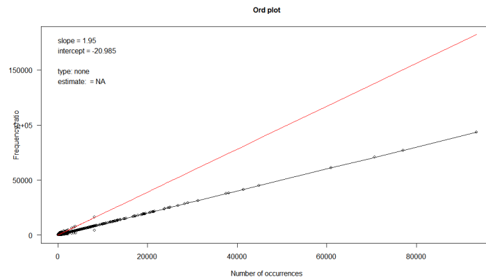
Figure 4.23: Ord plot
