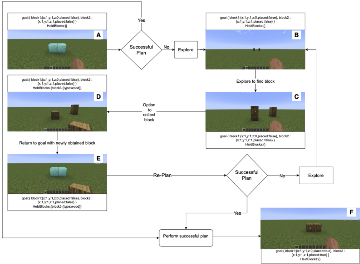
Figure 5.1: The procedure followed to create a structure of two blocks. The goal is to collect and place two wood blocks in the locations of the diamond signifier blocks.
