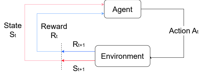
Figure 2.1: Reinforcement learning training loop displaying the agent-environment interaction [Sutton and Barto 2018]
