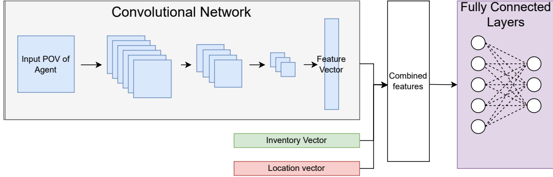
Figure 5.2: Feature combination used in the DQN Algorithm
