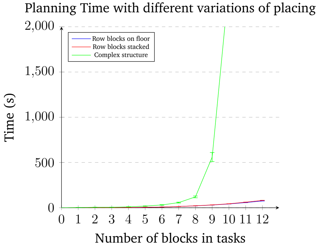
Figure 6.2: A time comparison between different variants of structure shape for Plan-Explore, being a line of blocks that increase horizontally, a wall structure of vertical size two and a complex shape, with these results being an average over 3 runs. These structures can be viewed in Appendix A .
