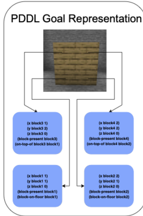
Figure 5.4: A direct comparison between the PDDL representation and the world state, showing how blocks in Minecraft are represented in a symbolic manner. This image represent a structure of four blocks where each block is translated into a symbolic object. Each block represented symbolically is comprised of the x , y , z coordinates of the block location relative to the Minecraft world coordinate system, as well as predicates expressing whether the block is present within the world and if the block is on the floor or on top of another block.
