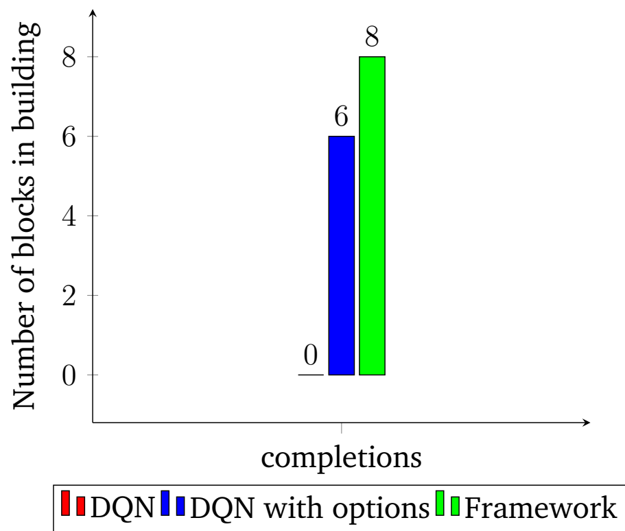
Figure 6.3: A difference in the maximum number of blocks each framework can place.
