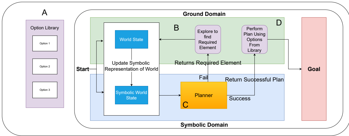
Figure 4.1: Plan, then Explore Framework to complete a given goal. The initialisation wherein the symbol state reflects the information extracted from the world state. The planner attempts to find a plan that is successful, if not, an element required to complete the goal is returned where we explore and find the required element using the options selected from the options library.
