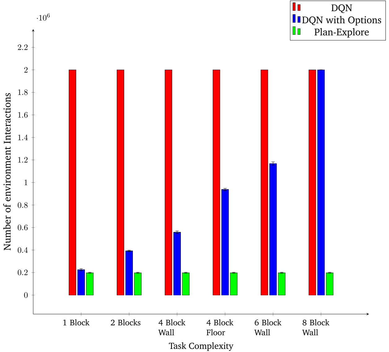
Figure 6.1: A direct comparison between the DQN, DQN with options and Plan-Explore, comparing the total number of environment interactions in tasks of varying complexity in a partially observable environment. The mean and standard deviation are calculated over 3 runs for each algorithm. A maximum of two million interactions depicts that the algorithm failed to complete the task.
