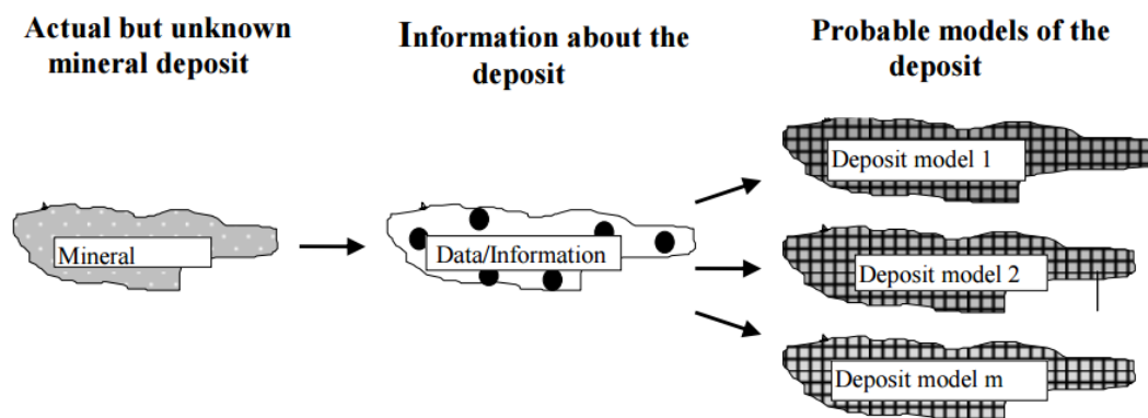
Figure 2-1: Reality in the ore deposit is partially accessible through drilling information; uncertainty associated with in-situ grade and geological variability is captured in multiple realisations (Dimitrakopoulos, 1998, pp 174).
