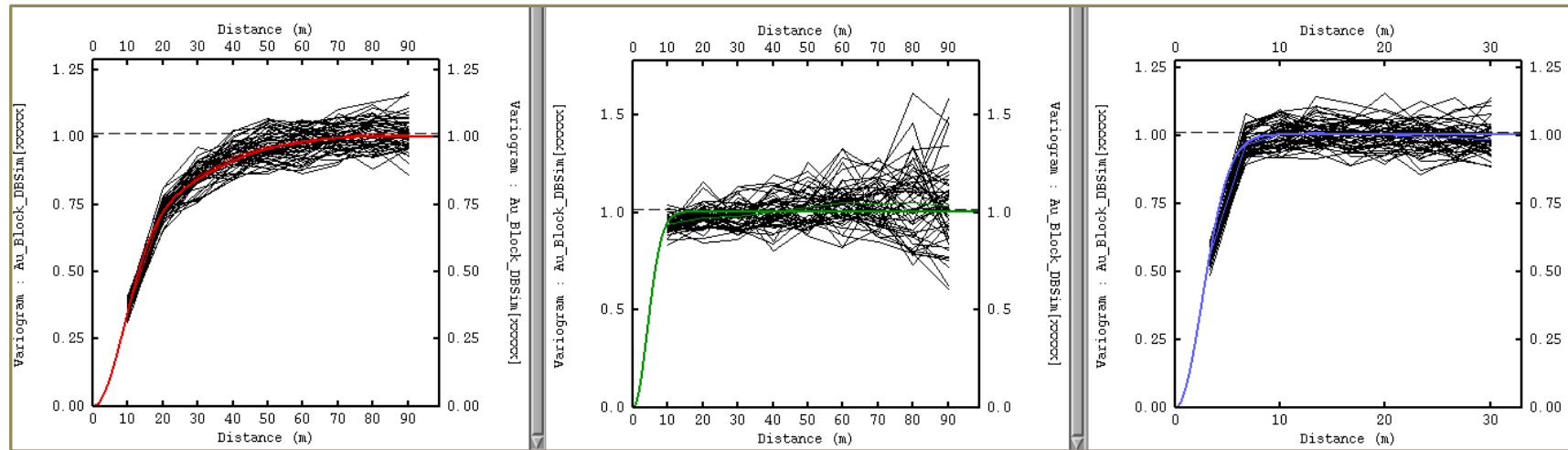
Figure 3-32: GHEW high grade data variogram model (red, green and blue lines) against variograms for simulated realisations (black lines)
