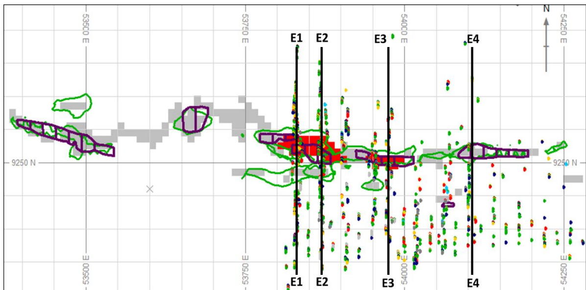
Figure 4-16: Plan view showing the location of cross sections (E1-E4) through GHEE to compare upside and downside scenarios for the High and Low Grade DBSim realisations on a 10m x 10m x 3,333m simulation grid.
