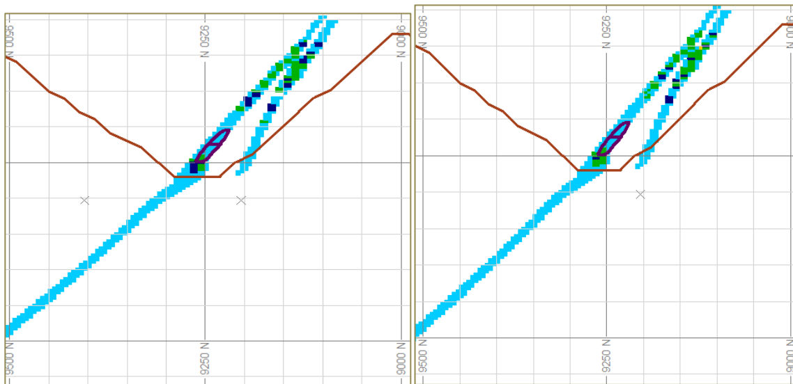
Figure 4-43: Section view (S12) showing the potential grade downside scenario (left) and upside scenario (right) for the joint uncertainty model (10m x 10m x 3,333m grid). Proposed location of stope designs are depicted by purple outlines. Resource pit surface is indicated by the brown line.
