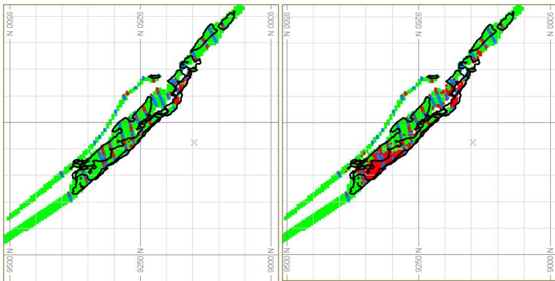
Figure 4-4: Section view (E2) showing the potential downside scenario (left) and upside scenario (right) based on ranked SIS realisations for GHEE using a 5m x 5m x 3,333m simulation grid. IK high grade wireframe for the deposit is depicted by black outlines.
