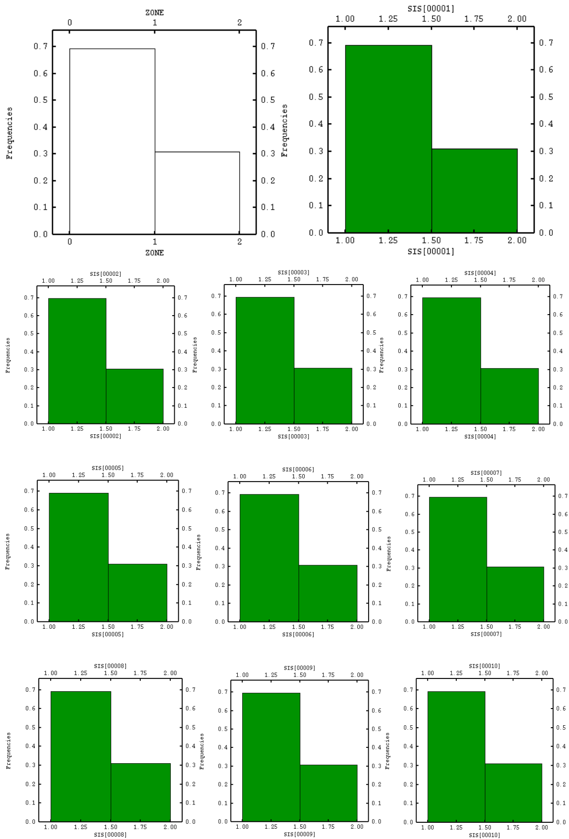
Figure A-2: West SIS histogram reproduction
