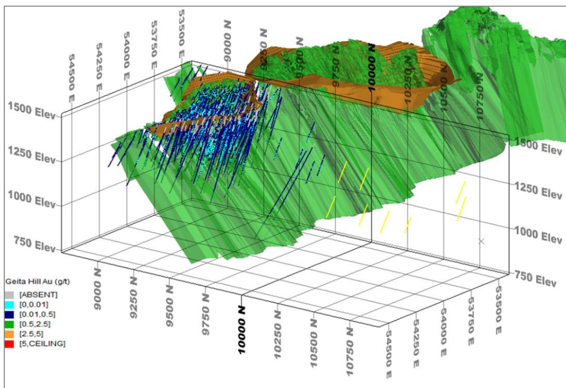
Figure 3-7: View of the entire study area in relation to the pit and low grade ore wireframe. The drill holes are displayed according to grade values. Holes highlighted in yellow were excluded from the study.
