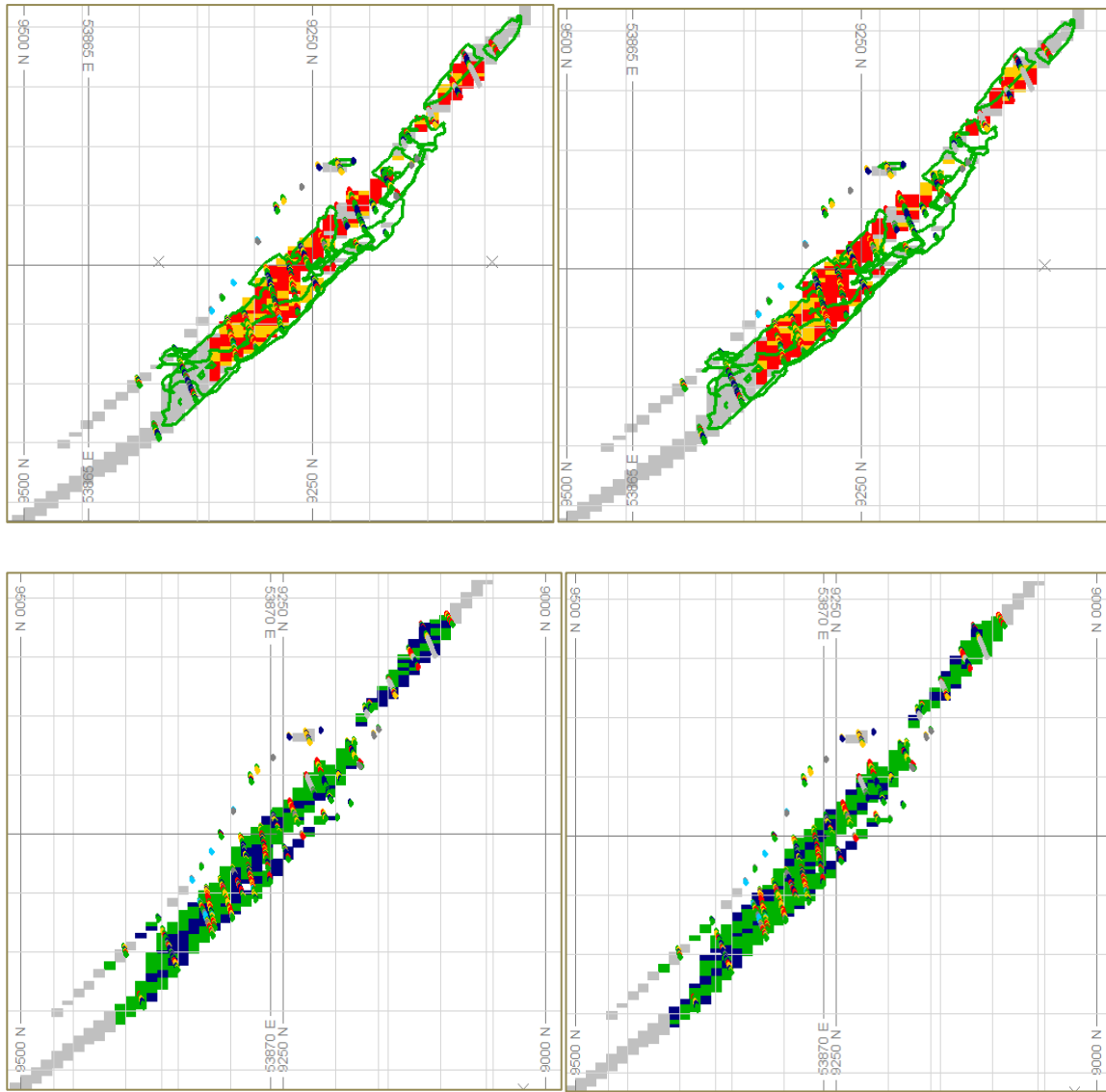
Figure 4-18: Section view (E2) showing the HG potential downside scenario (top left) and upside scenario (top right) and LG potential downside scenario (bottom left) and upside scenario (bottom right) based on ranked DBSim realisations for GHEE using a 10m x 10m x 3,333m simulation grid. IK high grade wireframe for the deposit is depicted by green outlines for the HG simulations
