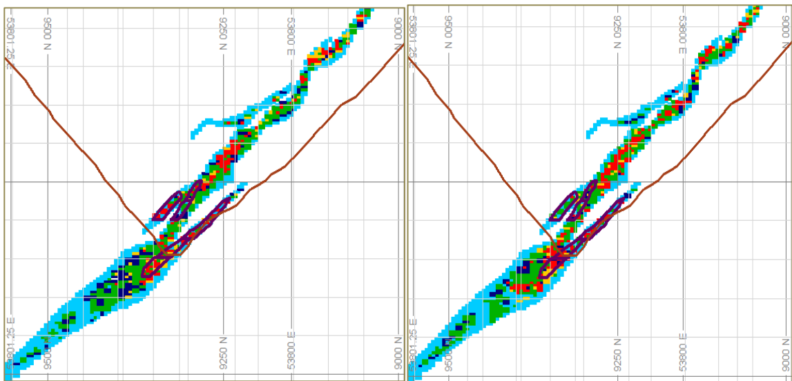
Figure 4-35: Section view (S4) showing the potential grade downside scenario (left) and upside scenario (right) for the joint uncertainty model (10m x 10m x 3,333m grid). Proposed location of stope designs are depicted by purple outlines. Resource pit surface is indicated by the brown line.
