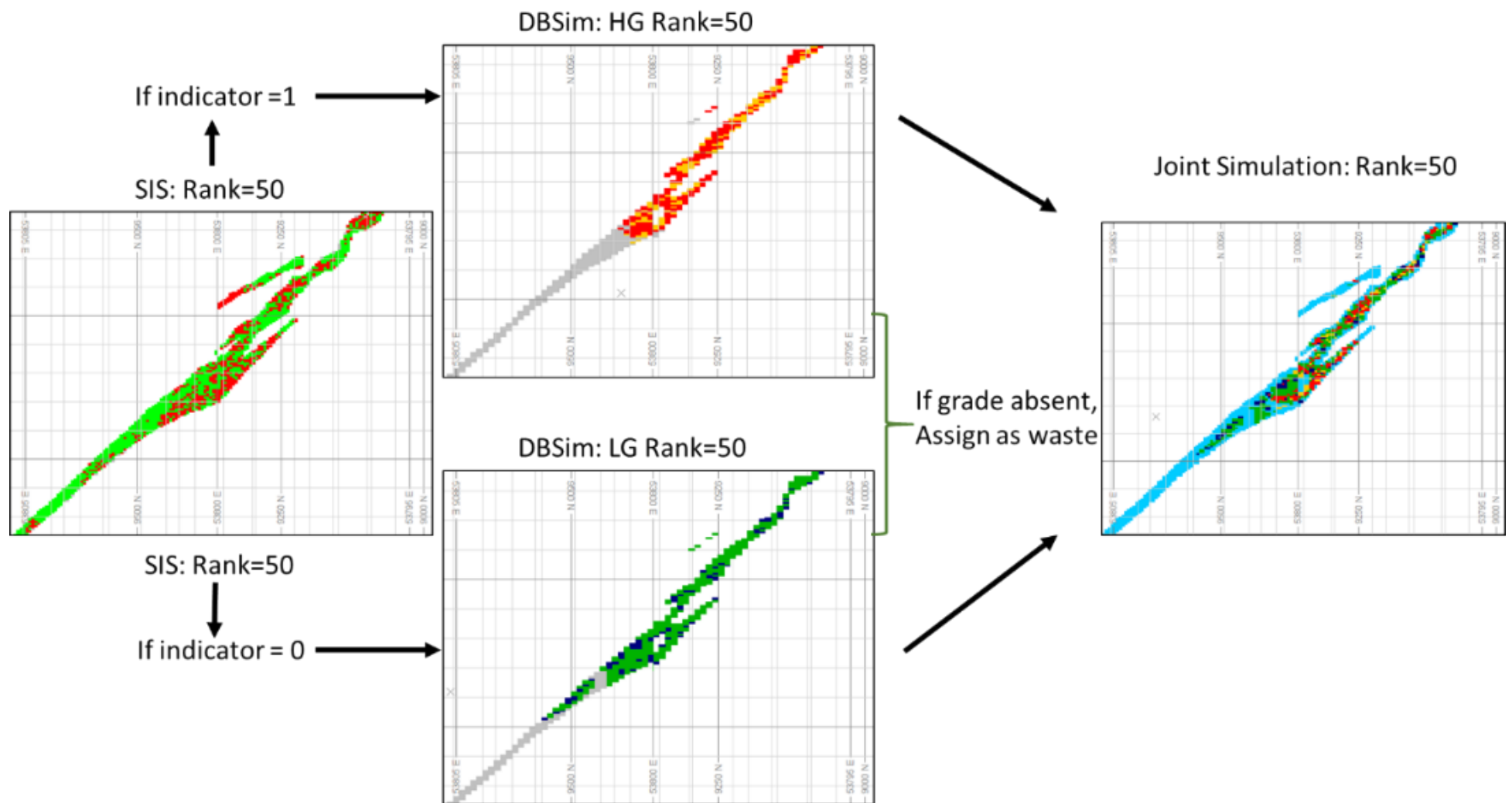
Figure 3-35: Schematic showing the logic behind combining SIS and DBSim realisations to give an indication of potential joint uncertainty
