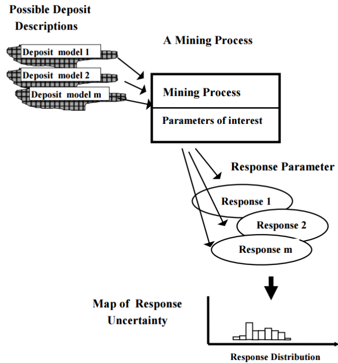
Figure 2-2: Mapping the space of response uncertainty (Dimitrakopoulos, 1998, pp 175)
