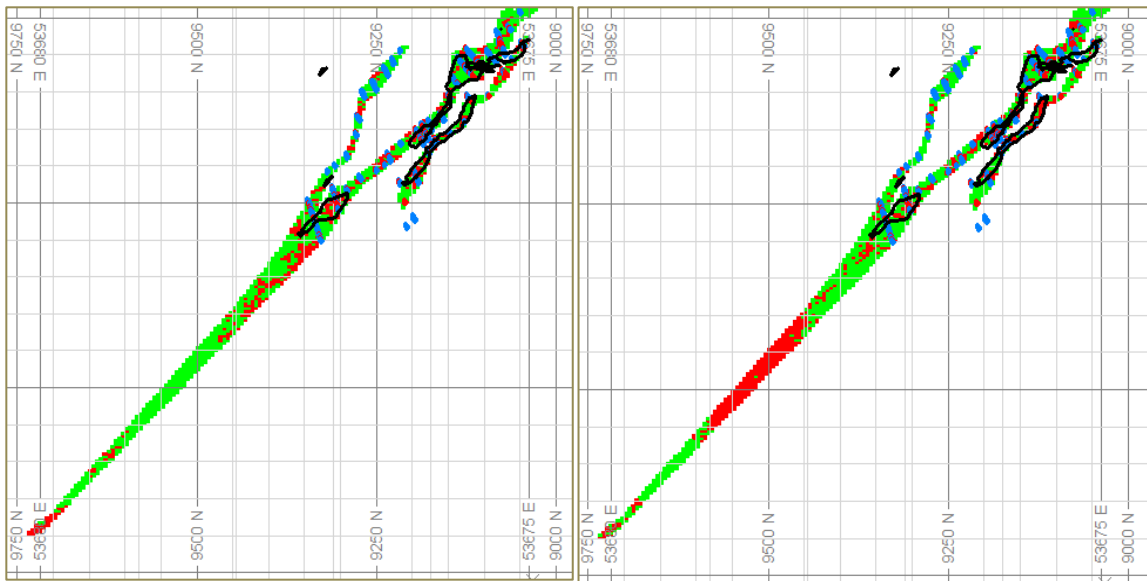
Figure 4-12: Section view (W4) showing the potential downside scenario (left) and upside scenario (right) based on ranked SIS realisations for GHEW using a 5m x 5m x 3,333m simulation grid. IK high grade wireframe for the deposit is depicted by black outlines.
