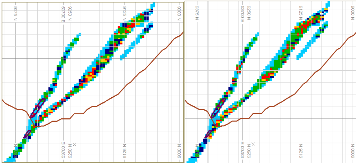
Figure 4-36: Section view (S5) showing the potential grade downside scenario (left) and upside scenario (right) for the joint uncertainty model (10m x 10m x 3,333m grid). Proposed location of stope designs are depicted by purple outlines. Resource pit surface is indicated by the brown line.
