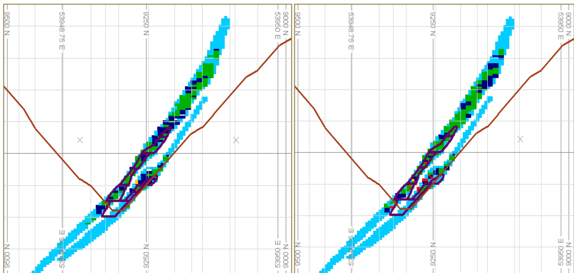
Figure 4-41: Section view (S10) showing the potential grade downside scenario (left) and upside scenario (right) for the joint uncertainty model (10m x 10m x 3,333m grid). Proposed location of stope designs are depicted by purple outlines. Resource pit surface is indicated by the brown line.
