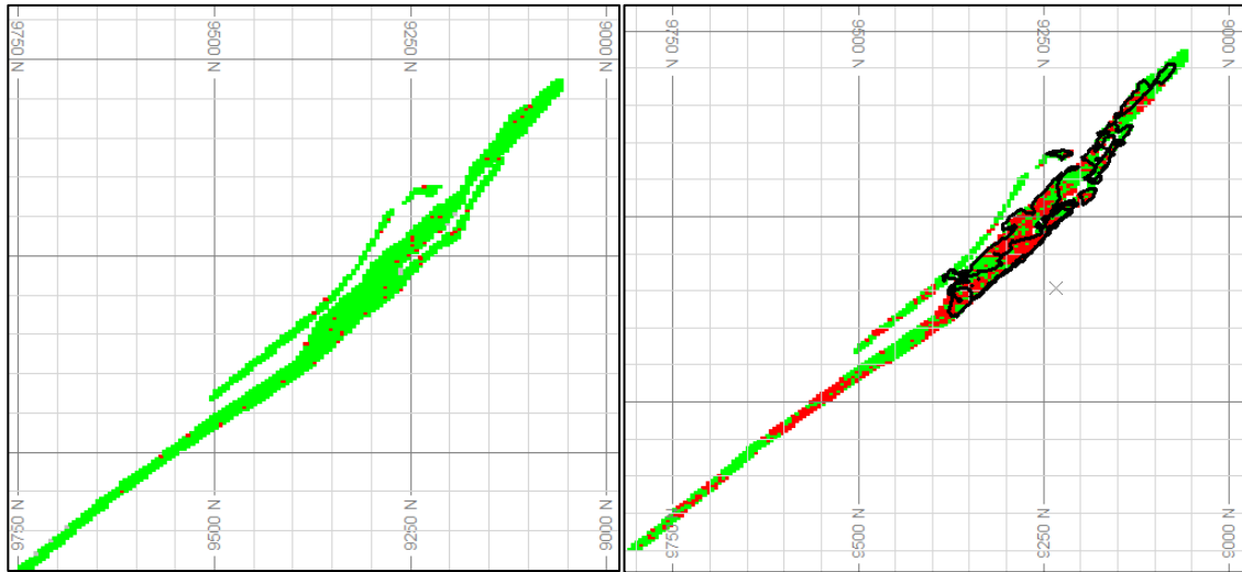
Figure 3-16: Section view through SIS realisations for GHEW run using conditioning data composited to 1m (left) and 3m (right), using the same variogram model parameters
