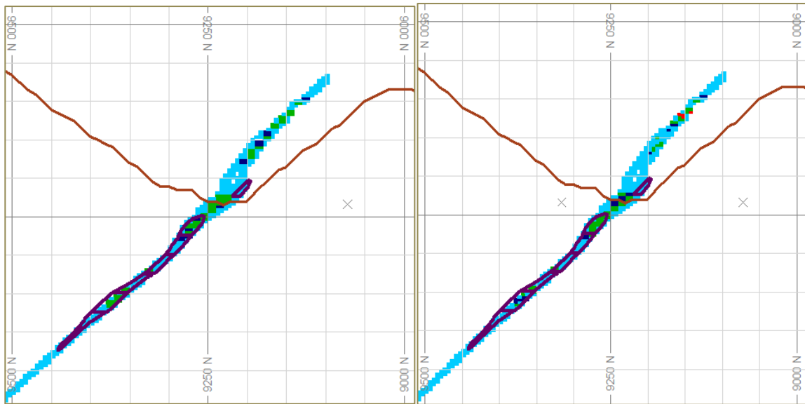
Figure 4-44: Section view (S13) showing the potential grade downside scenario (left) and upside scenario (right) for the joint uncertainty model (10m x 10m x 3,333m grid). Proposed location of stope designs are depicted by purple outlines. Resource pit surface is indicated by the brown line.
