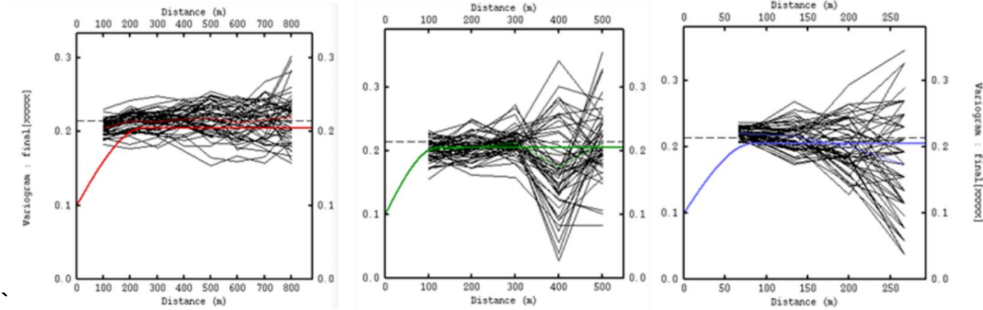
Figure 3-17: East SIS variogram validation. Variograms for data is indicated as solid lines (red, green and blue) for each anisotropic direction. Variogram models for each realisation is indicated by black lines.
