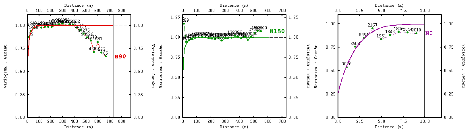
Figure 3-25: Variogram model fitting for GHEW Low Grade Gaussian Gold variables in 3 anisotropic directions. Experimental pairs of data are indicated as green points in each figure. The solid coloured lines represent the variogram models.
