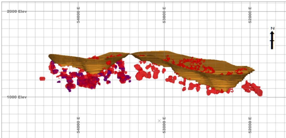
Figure 3-2: East-West section through the Geita Hill pits showing the preliminary mining stope layouts (purple wireframe) targeting higher grade lenses below the pit.
