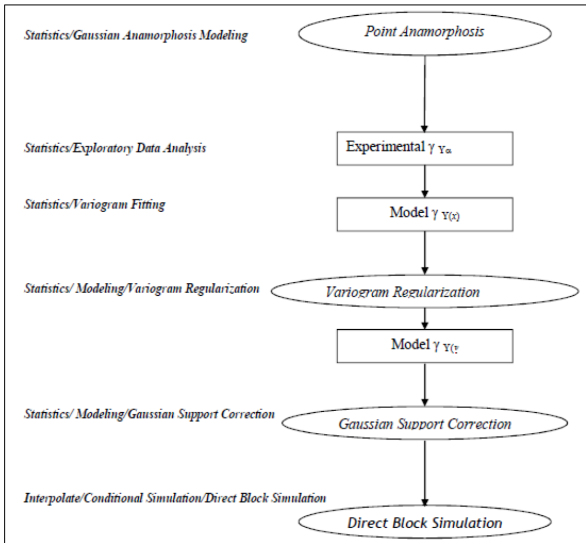
Figure 3-19: Recommended workflow for simulating grades using DBSim in ISATIS (ISATIS user manual, 2016)
