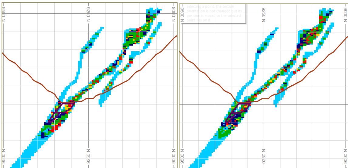
Figure 4-39: Section view (S8) showing the potential grade downside scenario (left) and upside scenario (right) for the joint uncertainty model (10m x 10m x 3,333m grid). Proposed location of stope designs are depicted by purple outlines. Resource pit surface is indicated by the brown line.
