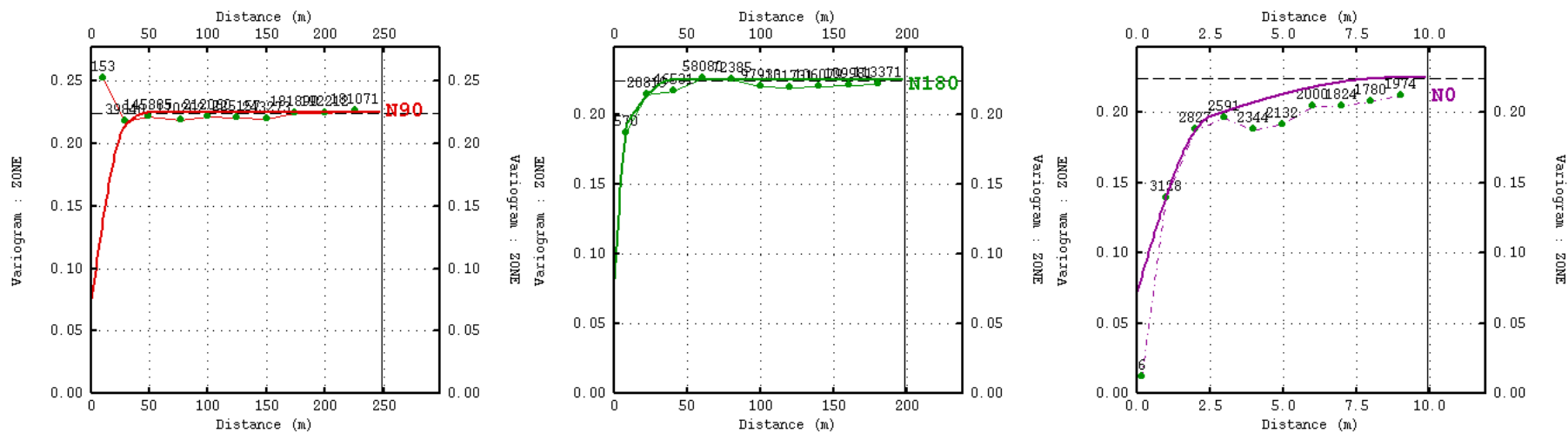
Figure 3-10: East SIS directional variogram models
