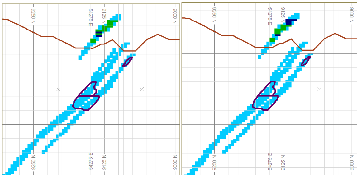
Figure 4-47: Section view (S16) showing the potential grade downside scenario (left) and upside scenario (right) for the joint uncertainty model (10m x 10m x 3,333m grid). Proposed location of stope designs are depicted by purple outlines. Resource pit surface is indicated by the brown line.
