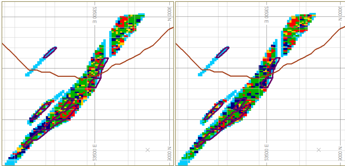
Figure 4-32: Section view (S1) showing the potential grade downside scenario (left) and upside scenario (right) for the joint uncertainty model (10m x 10m x 3,333m grid). Proposed location of stope designs are depicted by purple outlines. Resource pit surface is indicated by the brown line.
