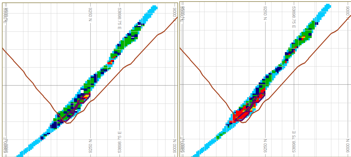
Figure 4-40: Section view (S9) showing the potential grade downside scenario (left) and upside scenario (right) for the joint uncertainty model (10m x 10m x 3,333m grid). Proposed location of stope designs are depicted by purple outlines. Resource pit surface is indicated by the brown line.
