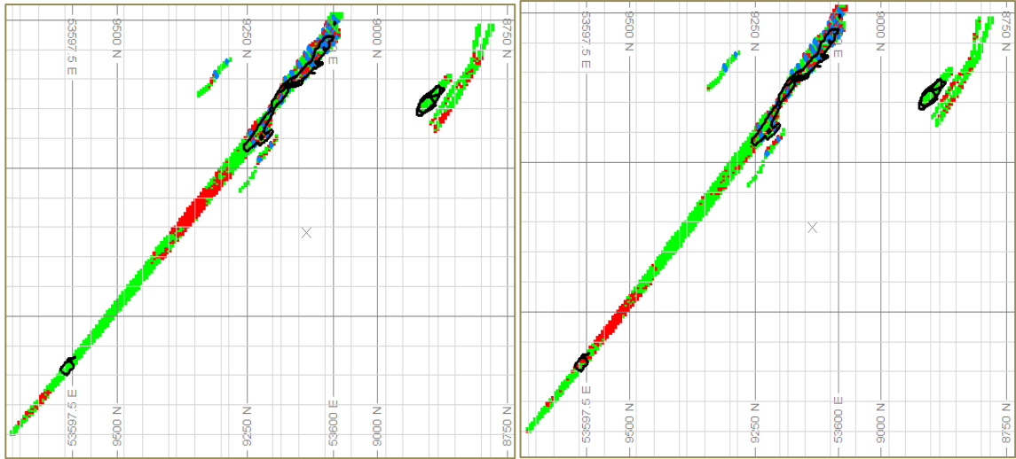
Figure 4-11: Section view (W3) showing the potential downside scenario (left) and upside scenario (right) based on ranked SIS realisations for GHEW using a 5m x 5m x 3,333m simulation grid. IK high grade wireframe for the deposit is depicted by black outlines.
