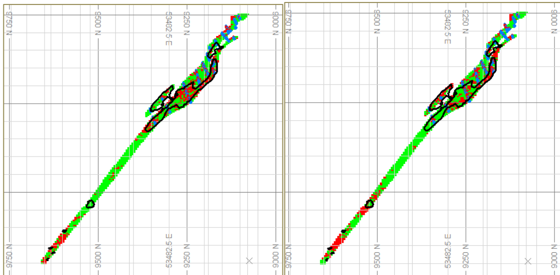
Figure 4-9: Section view (W1) showing the potential downside scenario (left) and upside scenario (right) based on ranked SIS realisations for GHEW using a 5m x 5m x 3,333m simulation grid. IK high grade wireframe for the deposit is depicted by black outlines.
