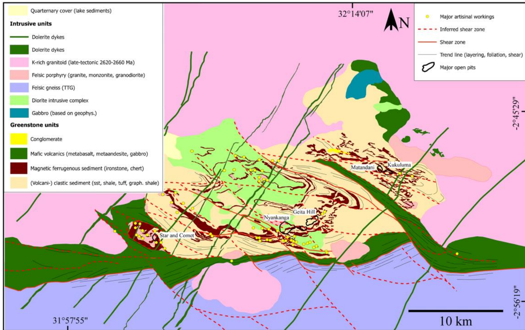
Figure 3-4: Geological map of the Geita Greenstone Belt (Sanislav, Brayshaw, Kolling, Dirks, Cook, & Blenkinsop, 2016, pp 3)
