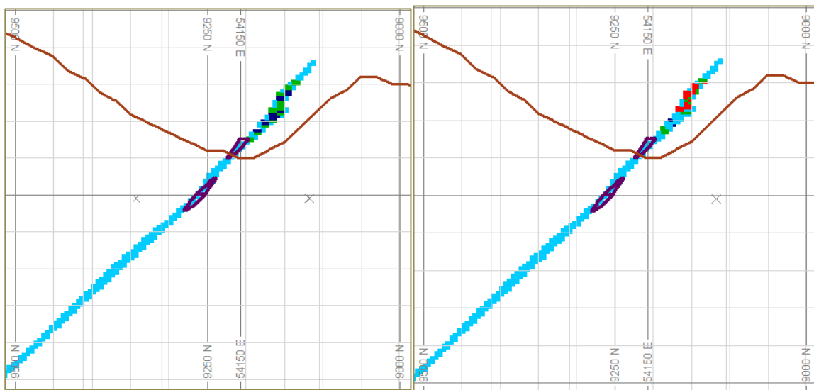
Figure 4-45: Section view (S14) showing the potential grade downside scenario (left) and upside scenario (right) for the joint uncertainty model (10m x 10m x 3,333m grid). Proposed location of stope designs are depicted by purple outlines. Resource pit surface is indicated by the brown line.
