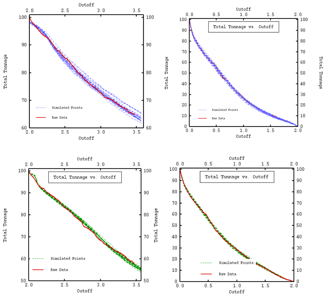
Figure 3-34: Grade tonnage curve comparison for raw data and DBSim point realisations: GHEE HG (top left), GHEE LG (top right), GHEW HG (bottom left) and GHEW LG (bottom right).
