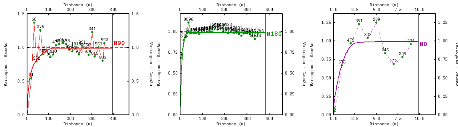
Figure 3-22: Variogram model fitting for GHEE High Grade Gaussian Gold variables in 3 anisotropic directions. Experimental pairs of data are indicated as green points in each figure. The solid coloured lines represent the variogram models.
