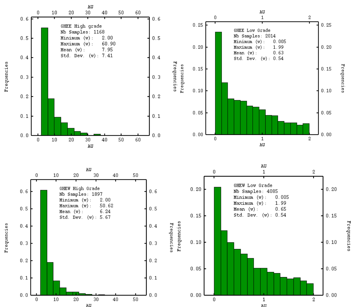
Figure 3-20: Raw Gold Grade distributions for conditioning data
