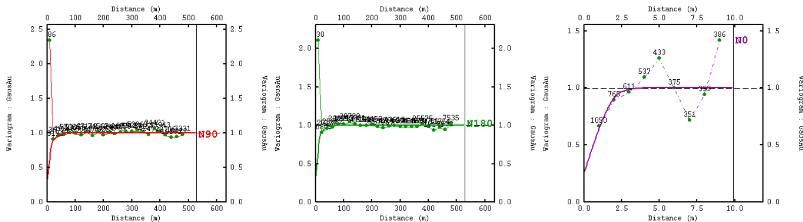
Figure 3-24: Variogram model fitting for GHEW High Grade Gaussian Gold variables in 3 anisotropic directions. Experimental pairs of data are indicated as green points in each figure. The solid coloured lines represent the variogram models.
