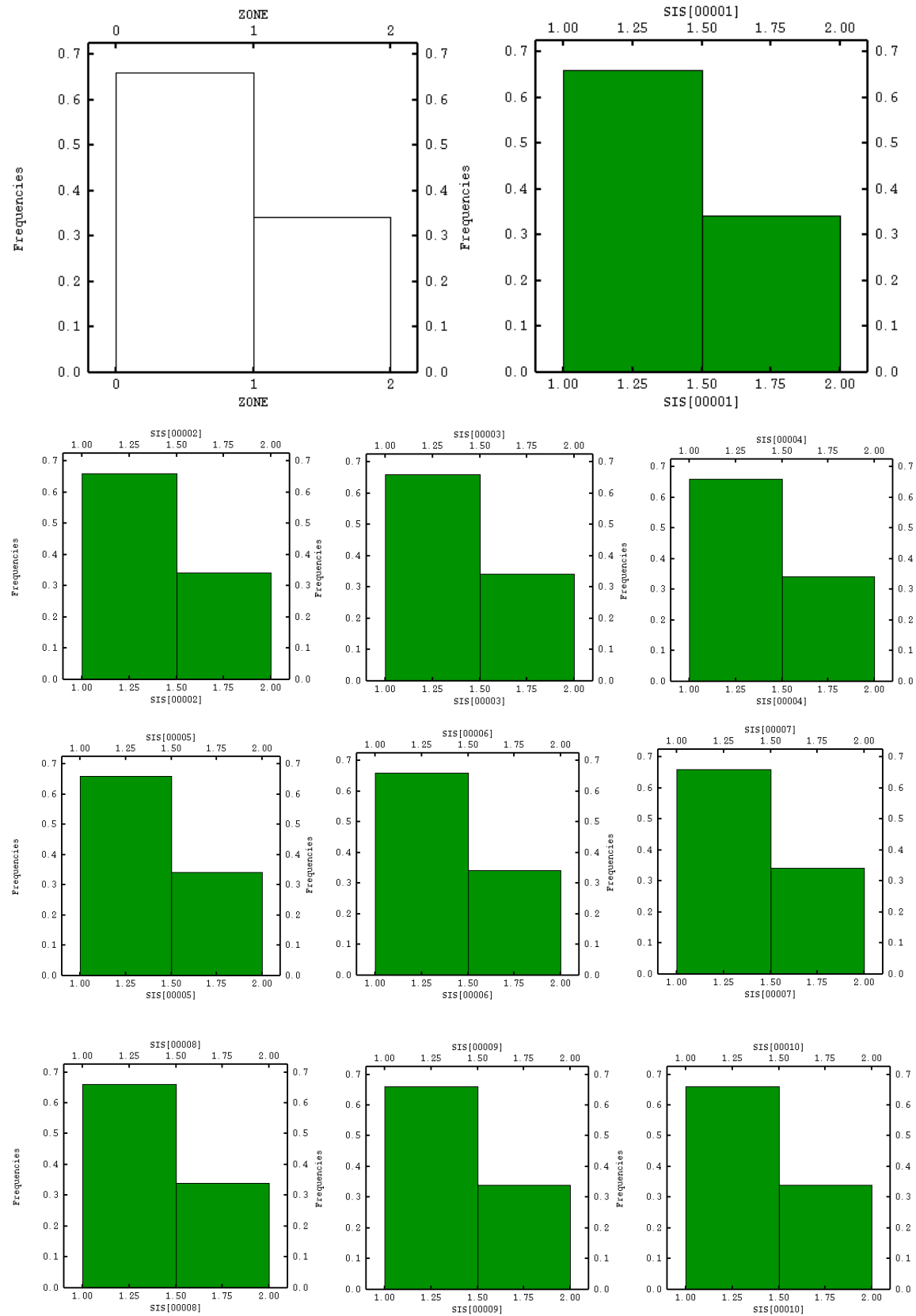
Figure A-1: East SIS histogram reproduction
