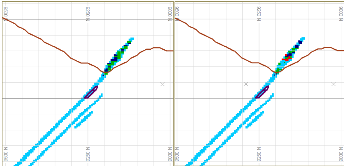
Figure 4-46: Section view (S15) showing the potential grade downside scenario (left) and upside scenario (right) for the joint uncertainty model (10m x 10m x 3,333m grid). Proposed location of stope designs are depicted by purple outlines. Resource pit surface is indicated by the brown line.
