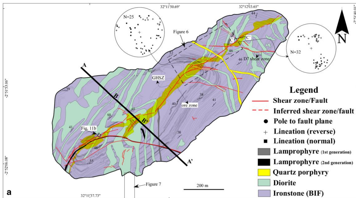
Figure 3-5: Geological map of the Geita Hill West gold deposit. The background of the map (thin grey lines) represents the pit wireframe. (Sanislav, Brayshaw, Kolling, Dirks, Cook, & Blenkinsop, 2016, pp. 6)
