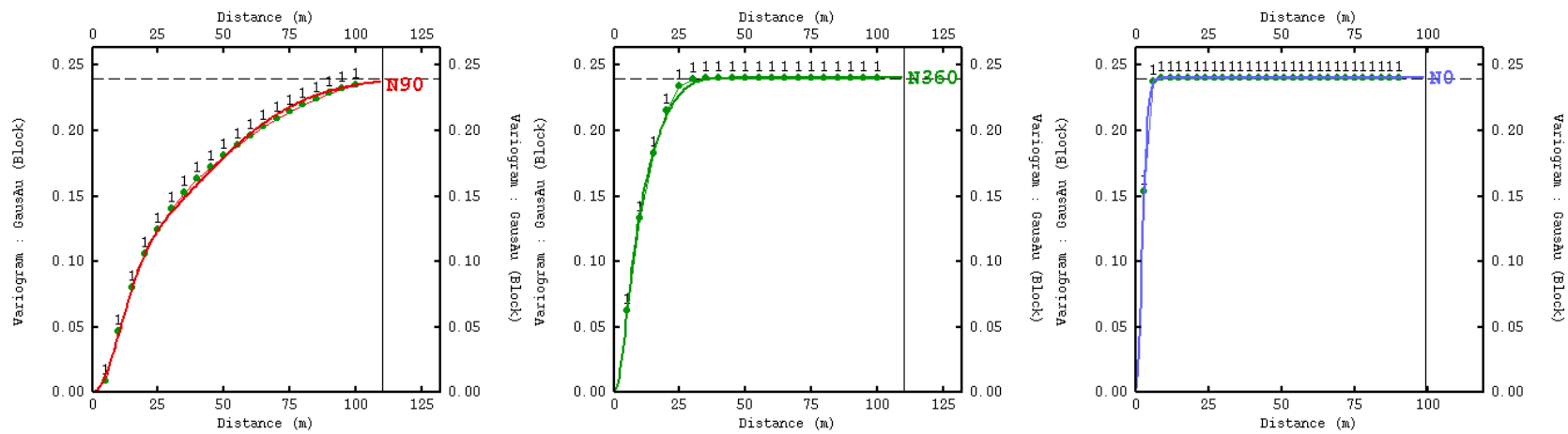
Figure 3-26: Regularised Block Variogram model fit on Gaussian point variables for GHEE High Grade.
