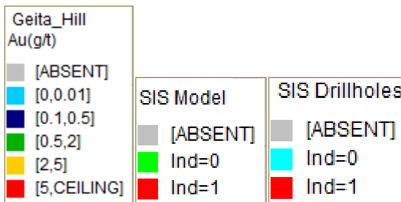
Figure 4-1: Legends used to display gold grades and simulated indicators
