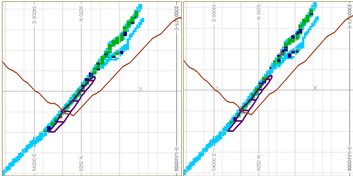
Figure 4-42: Section view (S11) showing the potential grade downside scenario (left) and upside scenario (right) for the joint uncertainty model (10m x 10m x 3,333m grid). Proposed location of stope designs are depicted by purple outlines. Resource pit surface is indicated by the brown line.
