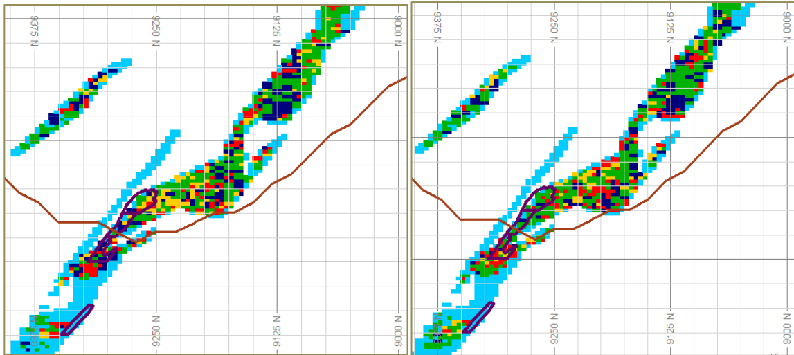
Figure 4-38: Section view (S7) showing the potential grade downside scenario (left) and upside scenario (right) for the joint uncertainty model (10m x 10m x 3,333m grid). Proposed location of stope designs are depicted by purple outlines. Resource pit surface is indicated by the brown line.
