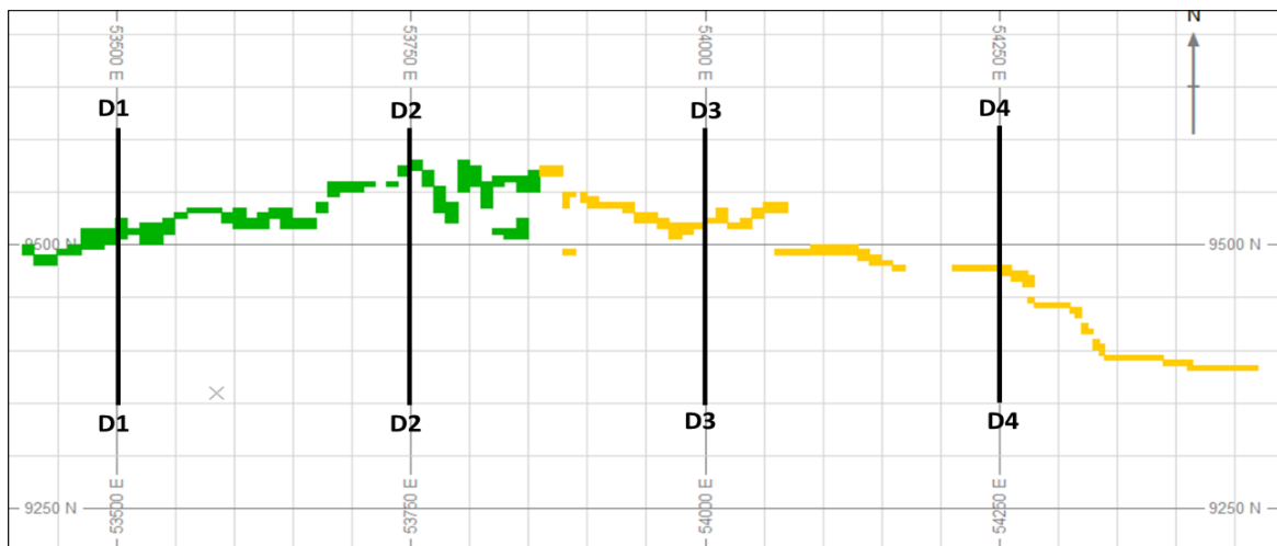
Figure 4-26: Plan view showing the location of cross sections (D1-D4) through GHEW and GHEE to compare upside and downside scenarios for the High Grade DBSim realisations on a 10m x 10m x 3,333m simulation grid against the deterministic estimated model for the study areas.
