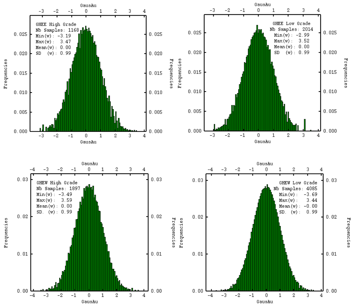
Figure 3-21: Transformed Grade distributions for conditioning data
