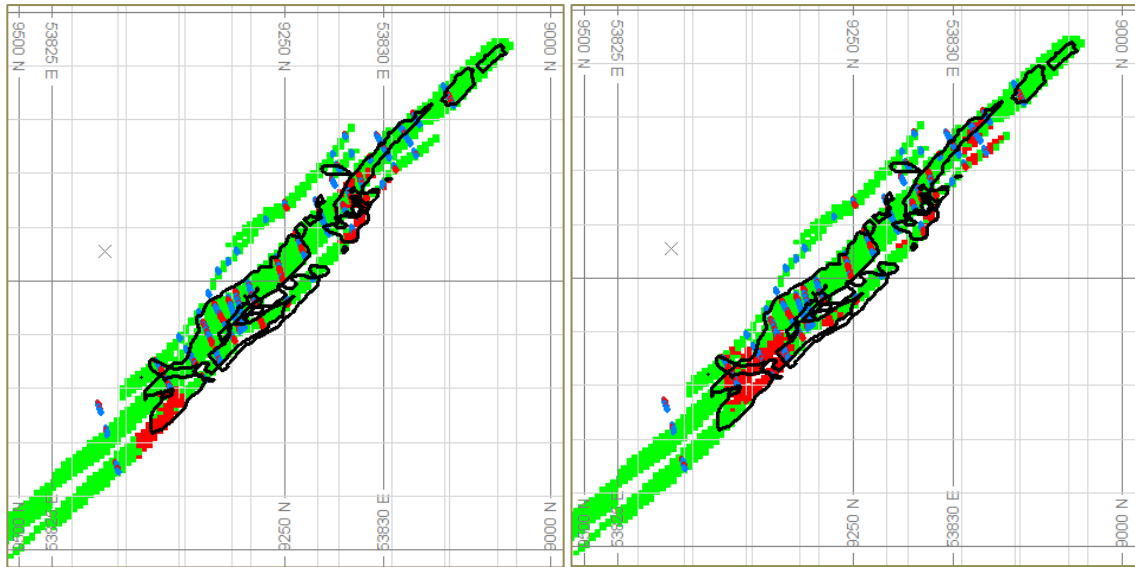
Figure 4-3: Section view (E1) showing the potential downside scenario (left) and upside scenario (right) based on ranked SIS realisations for GHEE using a 5m x 5m x 3,333m simulation grid. IK high grade wireframe for the deposit is depicted by black outlines.
