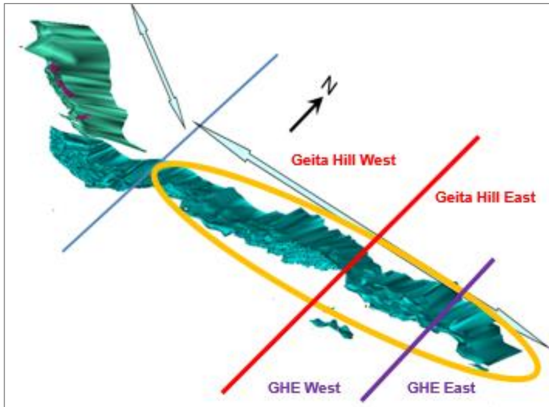
Figure 3-6: Reef Thrust Geometry. The portion of the reef forming the Geita Hill deposit is highlighted in yellow. The deposit is divided into Geita Hill East and Geita Hill West. Geita Hill East is further differentiated into GHE West and GHE East.
