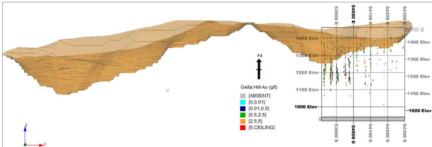
Figure 3-8: W-E section through Geita Hill pits showing the sample information available in the GHEE sub area.
