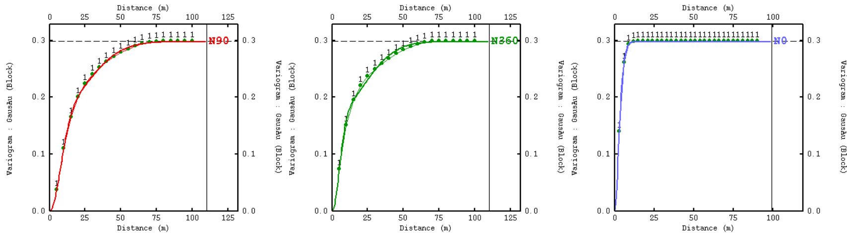
Figure 3-29: Regularised Block Variogram model fit on Gaussian point variables for GHEW Low Grade
