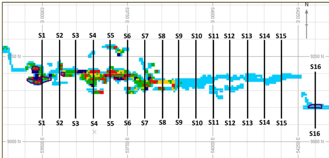
Figure 4-31: Plan view showing the location of cross sections (S1-S16) through GHEW and GHEE to compare upside and downside scenarios for the joint uncertainty models on a 10m x 10m x 3,333m simulation grid.
