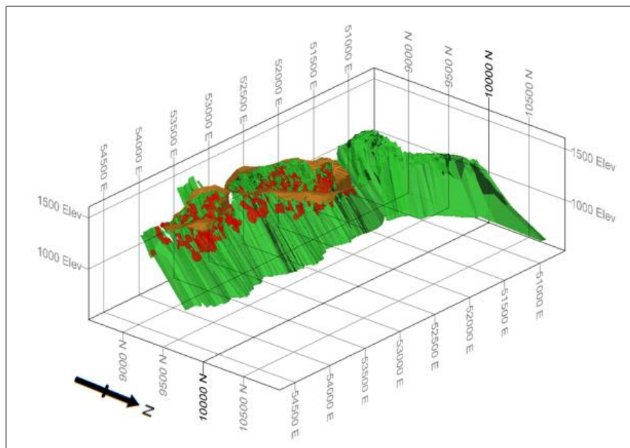
Figure 3-1: View of the Geita Hill pits showing the existing interpretation for the location and extent of higher grade lenses (red wireframe) within the known low grade mineralisation (green wireframe).
