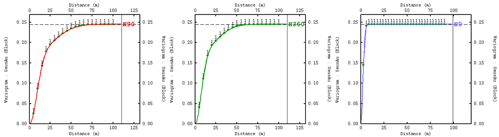
Figure 3-28: Regularised Block Variogram model fit on Gaussian point variables for GHEW High Grade.
