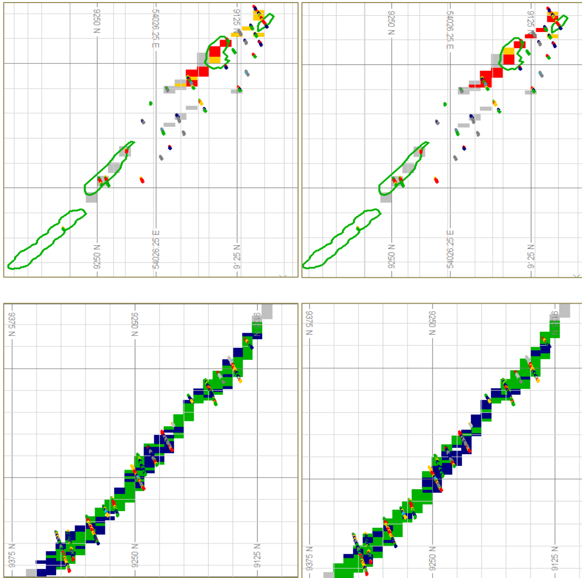
Figure 4-19: Section view (E3) showing the HG potential downside scenario (top left) and upside scenario (top right) and LG potential downside scenario (bottom left) and upside scenario (bottom right) based on ranked DBSim realisations for GHEE using a 10m x 10m x 3,333m simulation grid. IK high grade wireframe for the deposit is depicted by green outlines for the HG simulations
