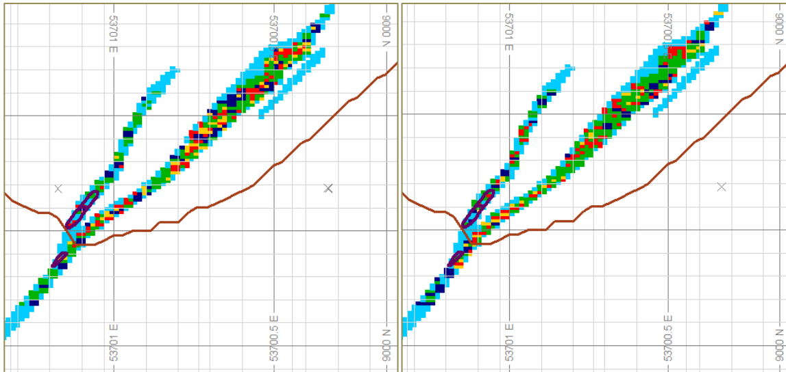
Figure 4-34: Section view (S3) showing the potential grade downside scenario (left) and upside scenario (right) for the joint uncertainty model (10m x 10m x 3,333m grid). Proposed location of stope designs are depicted by purple outlines. Resource pit surface is indicated by the brown line.
