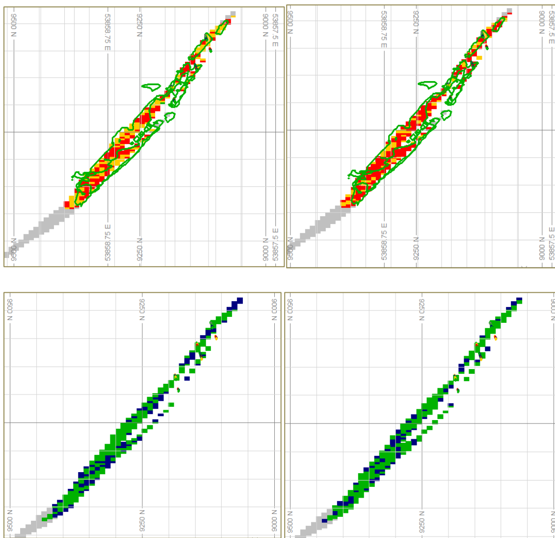
Figure 4-22: Section view (W1) showing the HG potential downside scenario (top left) and upside scenario (top right) and LG potential downside scenario (bottom left) and upside scenario (bottom right) based on ranked DBSim realisations for GHEW using a 10m x 10m x 3,333m simulation grid. IK high grade wireframe for the deposit is depicted by green outlines for the HG simulations
