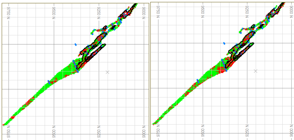
Figure 4-14: Section view (W6) showing the potential downside scenario (left) and upside scenario (right) based on ranked SIS realisations for GHEW using a 5m x 5m x 3,333m simulation grid. IK high grade wireframe for the deposit is depicted by black outlines.
