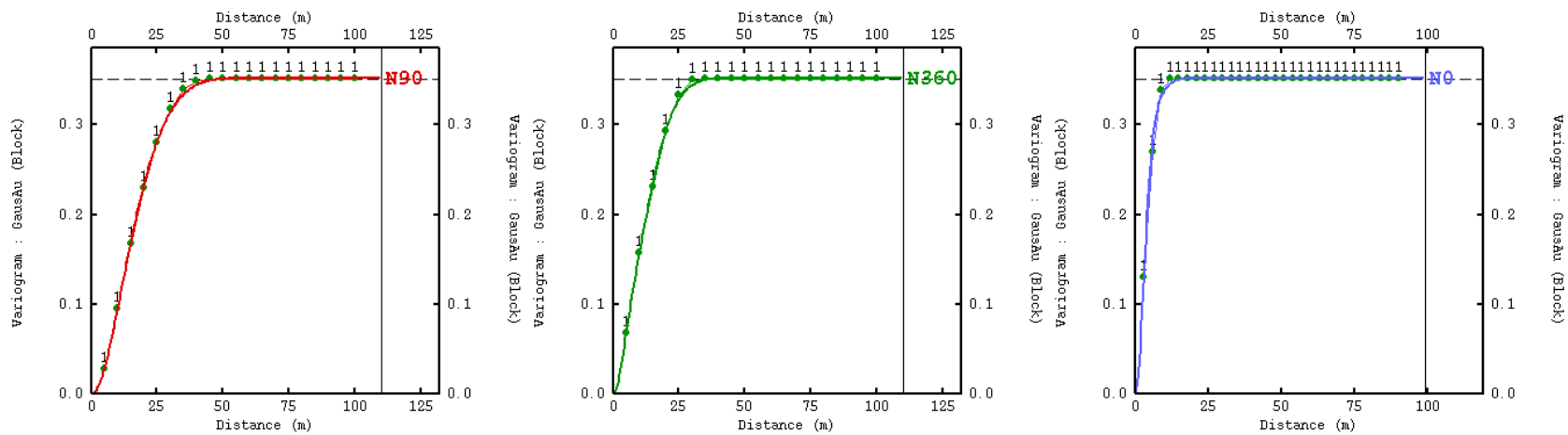
Figure 3-27: Regularised Block Variogram model fit on Gaussian point variables for GHEE Low Grade.
