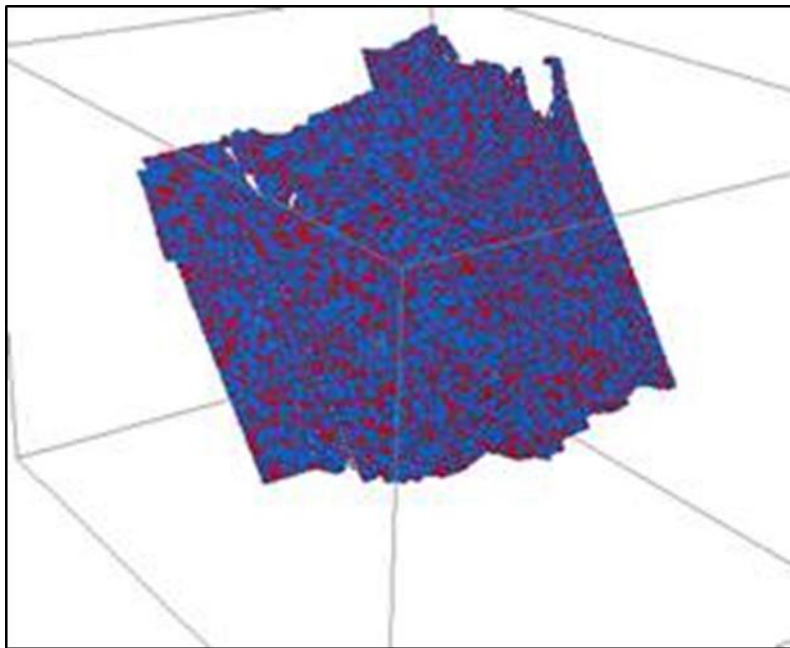
Figure 3-14: 3D view of resultant noisy simulation
