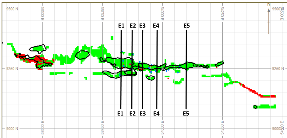
Figure 4-2: Plan view showing the location of cross sections (E1-E5) through GHEE to compare upside and downside scenarios for the SIS realisations on the 5m x 5m x 3,333m simulation grid.
