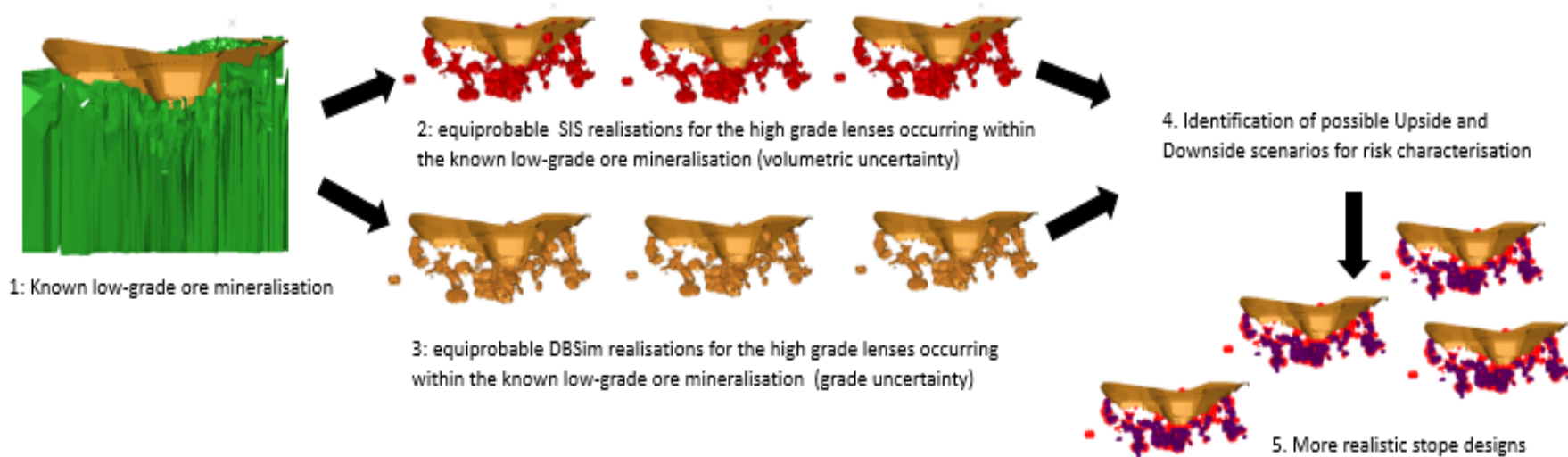
Figure 3-37: Description of the stochastic workflow followed for the study area
