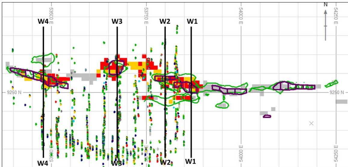
Figure 4-21: Plan view showing the location of cross sections (W1-W4) through GHEW to compare upside and downside scenarios for the High and Low Grade DBSim realisations on a 10m x 10m x 3,333m simulation grid.
