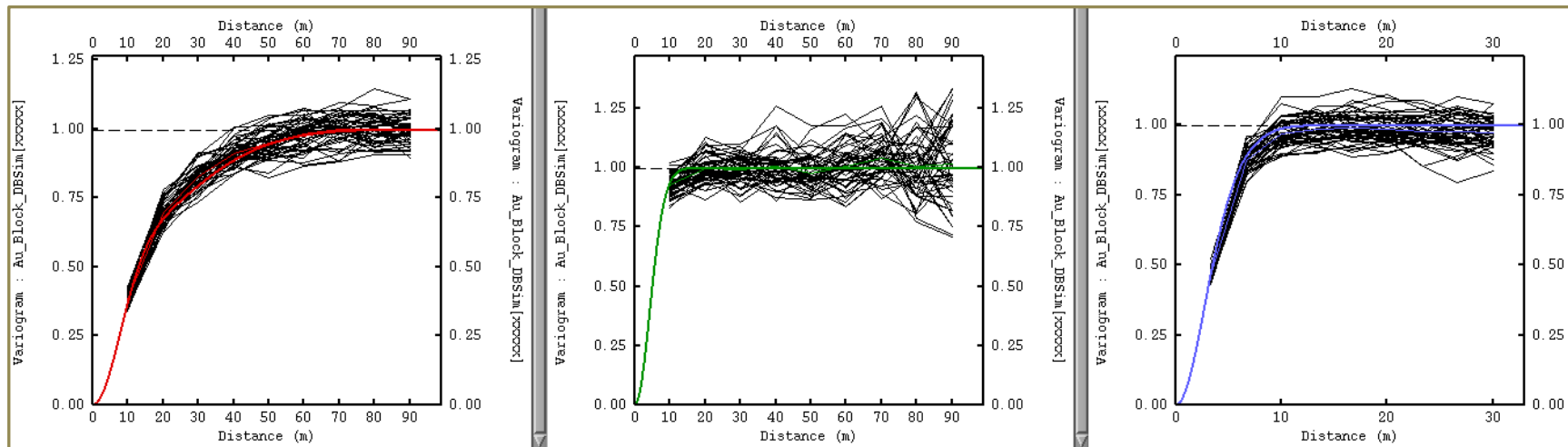
Figure 3-33: GHEW low grade data variogram models (red, green and blue lines) against variograms for simulated realisations (black lines)
