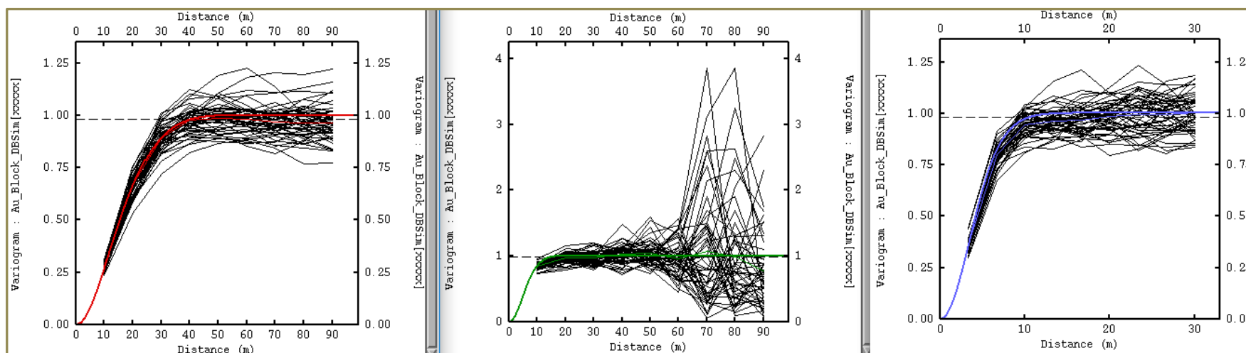
Figure 3-31: GHEE low grade data variogram models (red, green and blue lines) against variograms for simulated realisations (black lines)
