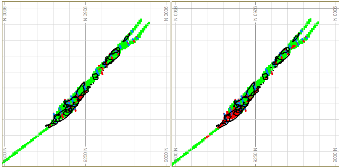
Figure 4-5: Section view (E3) showing the potential downside scenario (left) and upside scenario (right) based on ranked SIS realisations for GHEE using a 5m x 5m x 3,333m simulation grid. IK high grade wireframe for the deposit is depicted by black outlines.
