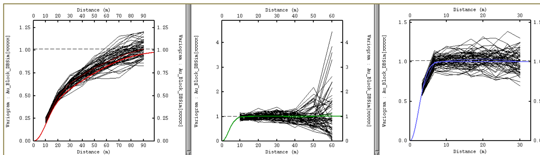
Figure 3-30: GHEE high grade data variogram models (red, green and blue lines) against variograms for simulated realisations (black lines)
