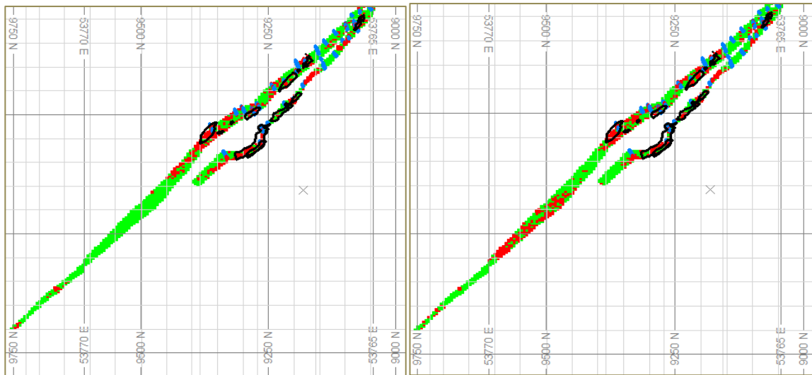
Figure 4-13: Section view (W5) showing the potential downside scenario (left) and upside scenario (right) based on ranked SIS realisations for GHEW using a 5m x 5m x 3,333m simulation grid. IK high grade wireframe for the deposit is depicted by black outlines.
