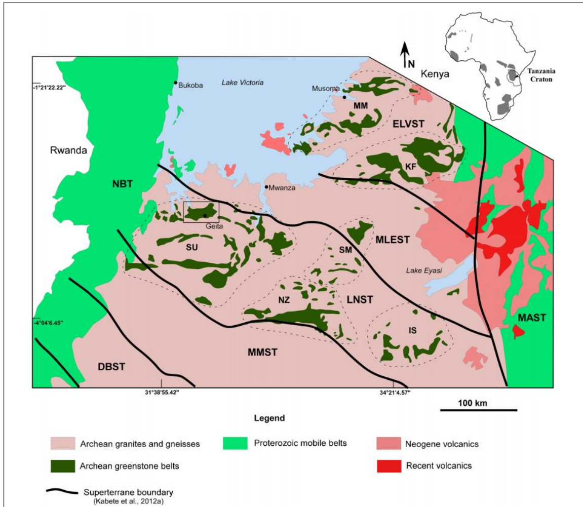
Figure 3-3: A simplified geological map for the Lake Victoria Region showing the main geological units. SU Sukumaland Greenstone Belt, NZ Nzega Greenstone Belt, SM Shynianga-Malita Greenstone Belt, IS Iramba-Sekenke Greenstone Belt, KF Kilimafedha Greenstone Belt, MM Musoma-Mara Greenstone Belt. Super-terrane boundaries include: ELVST East Lake Victoria, MLEST Mwanza Lake Eyasi, LNST Lake Nyanza, MMST Moyowosi-Manyoni, DBST Dodoma Basement, MAST MbuluMasai, NBT Nyakahura-Burigi. Inset map of Africa showing the location of Archean blocks (Sanislav, Brayshaw, Kolling, Dirks, Cook, & Blenkinsop, 2016, pp 2).
