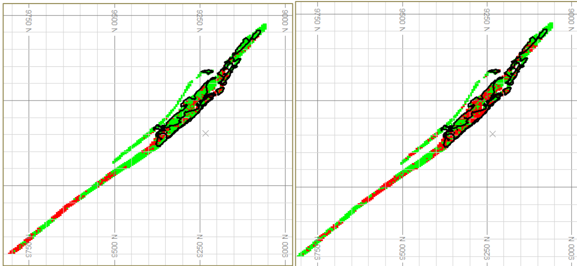
Figure 4-15: Section view (W7) showing the potential downside scenario (left) and upside scenario (right) based on ranked SIS realisations for GHEW using a 5m x 5m x 3,333m simulation grid. IK high grade wireframe for the deposit is depicted by black outlines.
