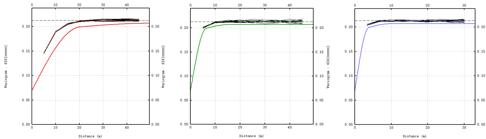
Figure 3-13: West SIS variogram validation. Variograms for data is indicated as solid lines (red, green and blue) for each anisotropic direction. Variogram models for each realisation is indicated by black lines.
