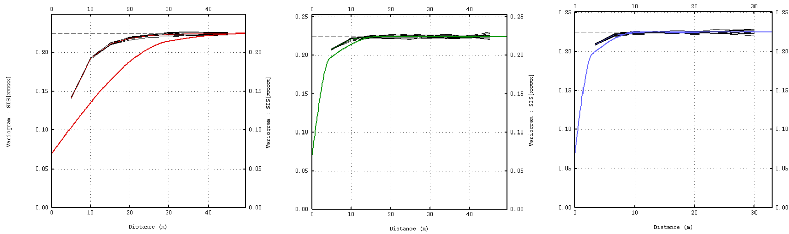
Figure 3-12: East SIS variogram validation. Variograms for data is indicated as solid lines (red, green and blue) for each anisotropic direction. Variogram models for each realisation is indicated by black lines.
