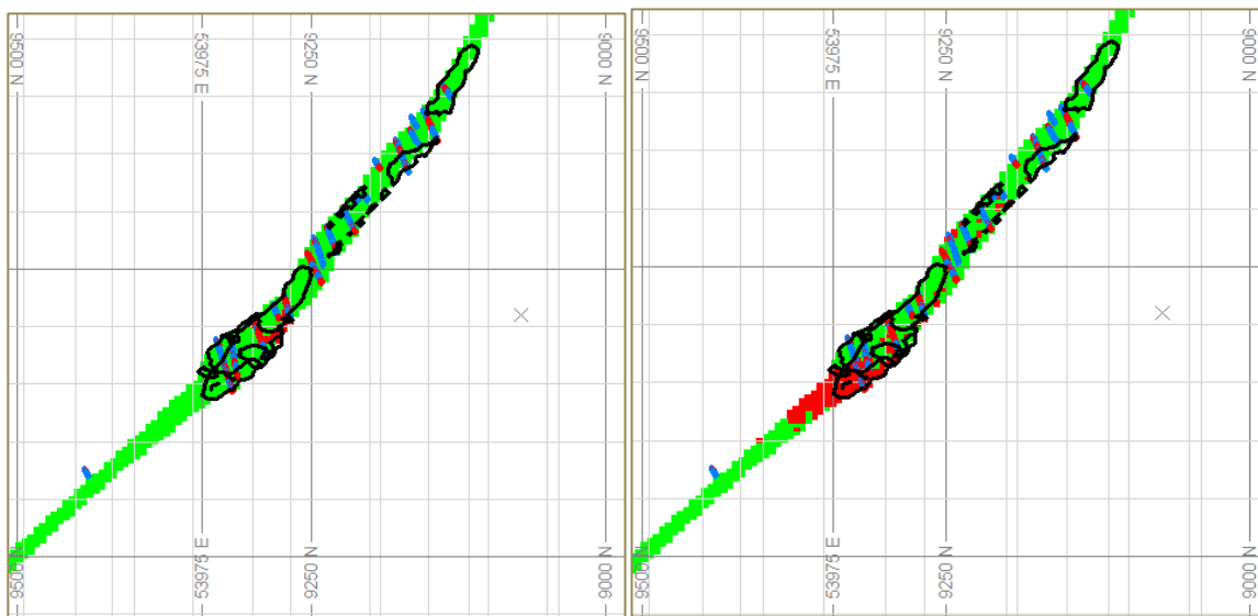
Figure 4-6: Section view (E4) showing the potential downside scenario (left) and upside scenario (right) based on ranked SIS realisations for GHEE using a 5m x 5m x 3,333m simulation grid. IK high grade wireframe for the deposit is depicted by black outlines.
