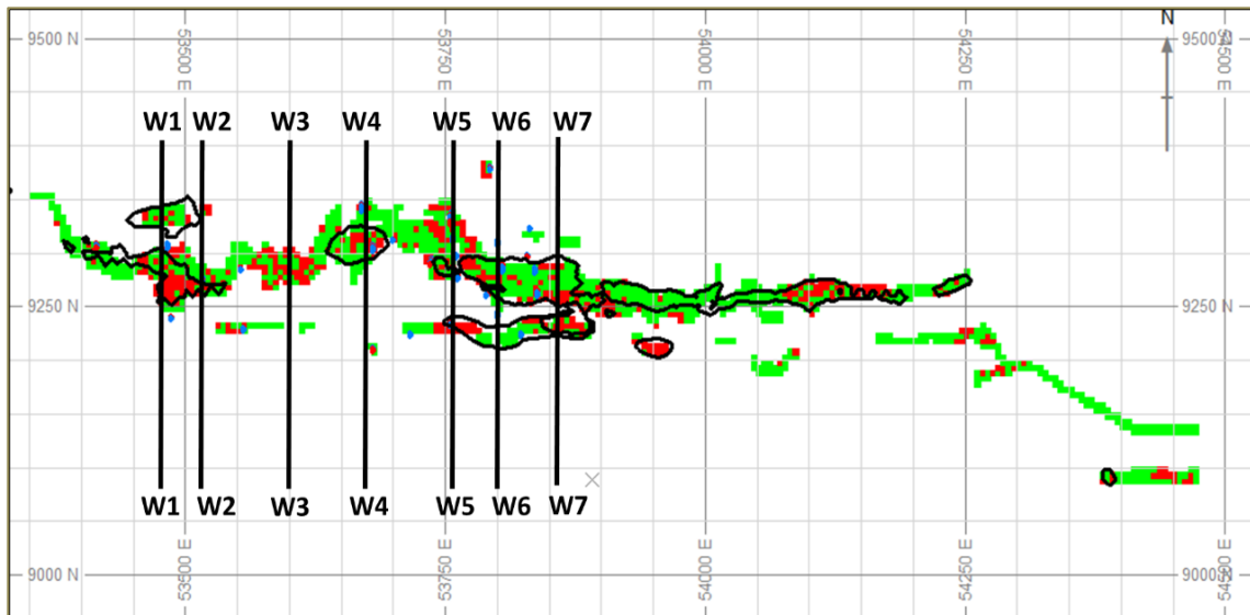
Figure 4-8: Plan view showing the location of cross sections (W1-W7) through GHEW to compare upside and downside scenarios for the SIS realisations on the 5m x 5m x 3,333m simulation grid.
