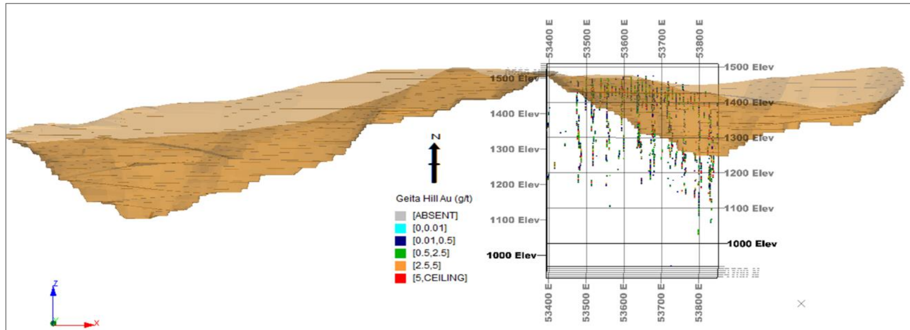
Figure 3-9: W-E section through Geita Hill pits showing the sample information available in the GHEW sub area.
