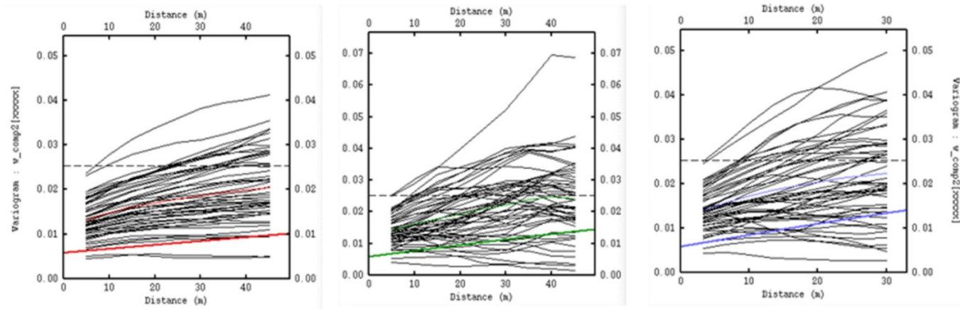
Figure 3-18: West SIS variogram validation. Variograms for data is indicated as solid lines (red, green and blue) for each anisotropic direction. Variogram models for each realisation is indicated by black lines.
