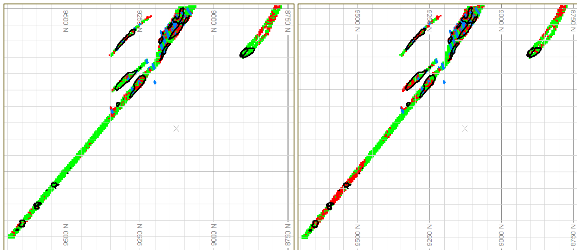
Figure 4-10: Section view (W2) showing the potential downside scenario (left) and upside scenario (right) based on ranked SIS realisations for GHEW using a 5m x 5m x 3,333m simulation grid. IK high grade wireframe for the deposit is depicted by black outlines.
