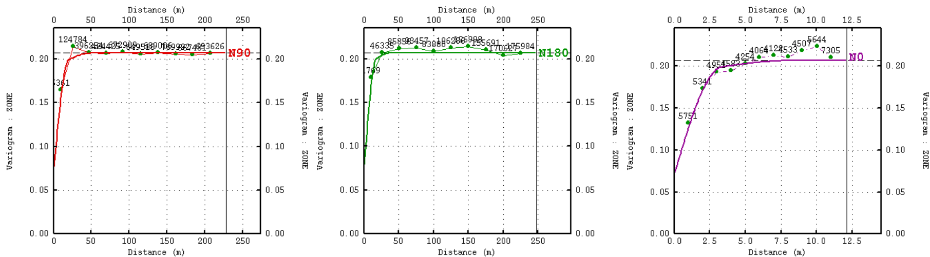
Figure 3-11: West SIS directional variogram models
