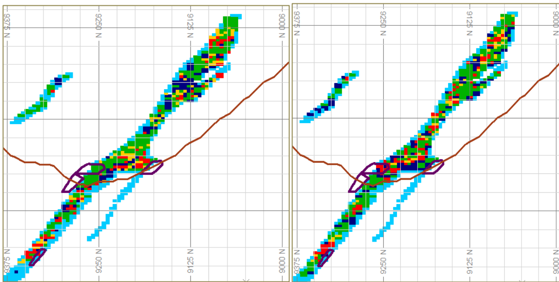
Figure 4-37: Section view (S6) showing the potential grade downside scenario (left) and upside scenario (right) for the joint uncertainty model (10m x 10m x 3,333m grid). Proposed location of stope designs are depicted by purple outlines. Resource pit surface is indicated by the brown line.
