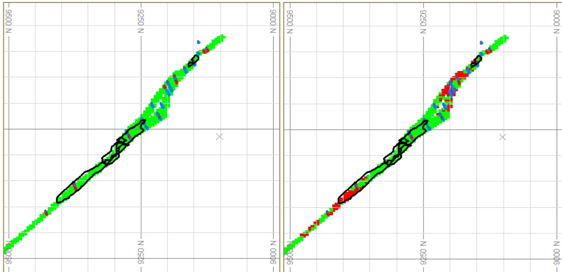
Figure 4-7: Section view (E5) showing the potential downside scenario (left) and upside scenario (right) based on ranked SIS realisations for GHEE using a 5m x 5m x 3,333m simulation grid. 1K high grade wireframe for the deposit is depicted by black outlines.
