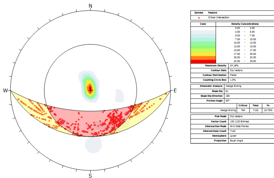
Figure D-23 Wedge failure for PE03 Northern Wall at 61° inter-ramp slope angle (Current design).
