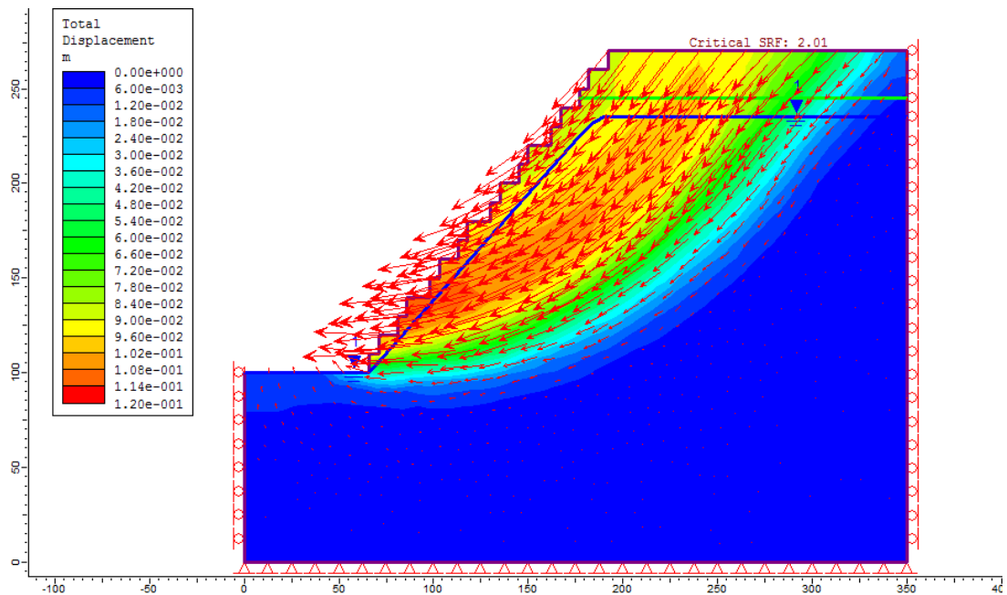
Figure 4-6 Finite element model for a slope with alternating 10 m and 5 m benches at 90 ° bench slope angle and 54 ° overall slope angle (OD1).
