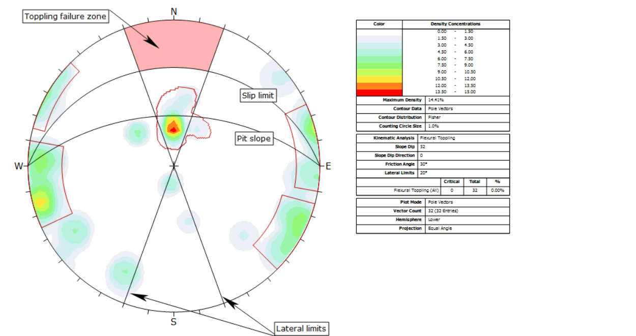
Figure 3-28 Toppling failure for PE03 Southern Wall at 52° final pit slope angle.
