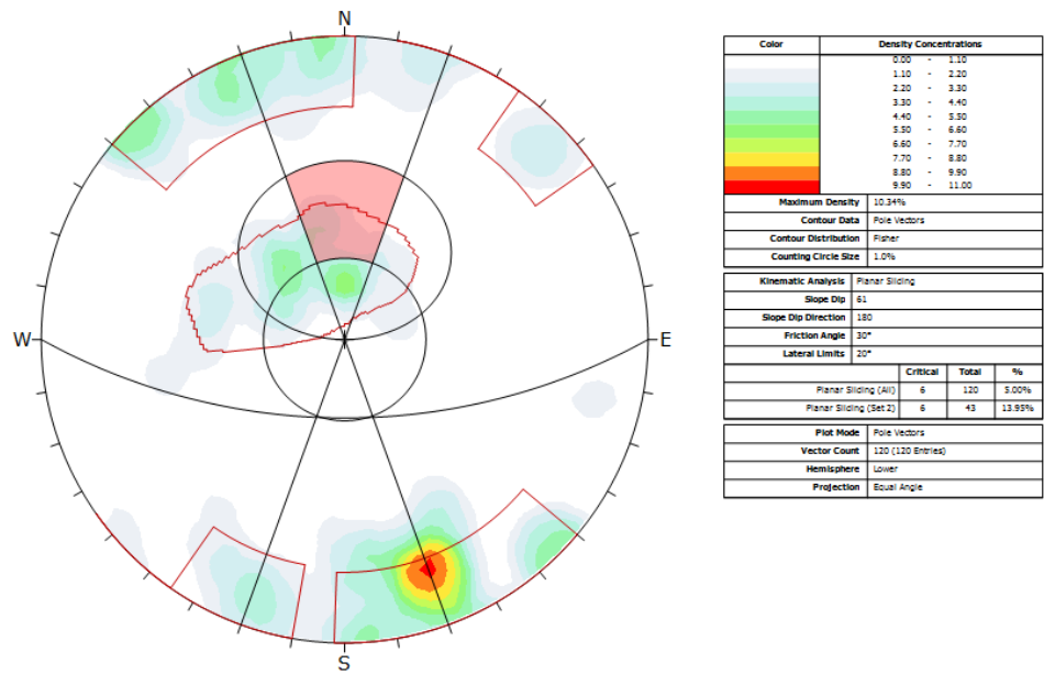
Figure D-22 Planar failure for PE03 Northern Wall at 61° inter-ramp slope angle (Current design).
