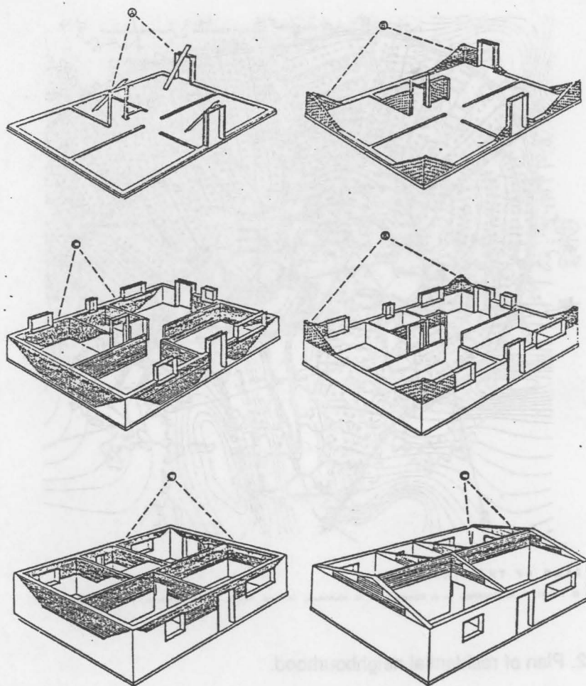
Fig. 24.—NE 51/9 type house showing the six brickwork tasks.
