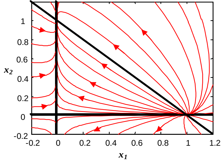
Figure 2.2 : A Residue curve map with curves shown inside the MBT, i.e. \sum x_i=1 and x_i \geq 0 ; as well as outside the MBT where x_i < 0 .
