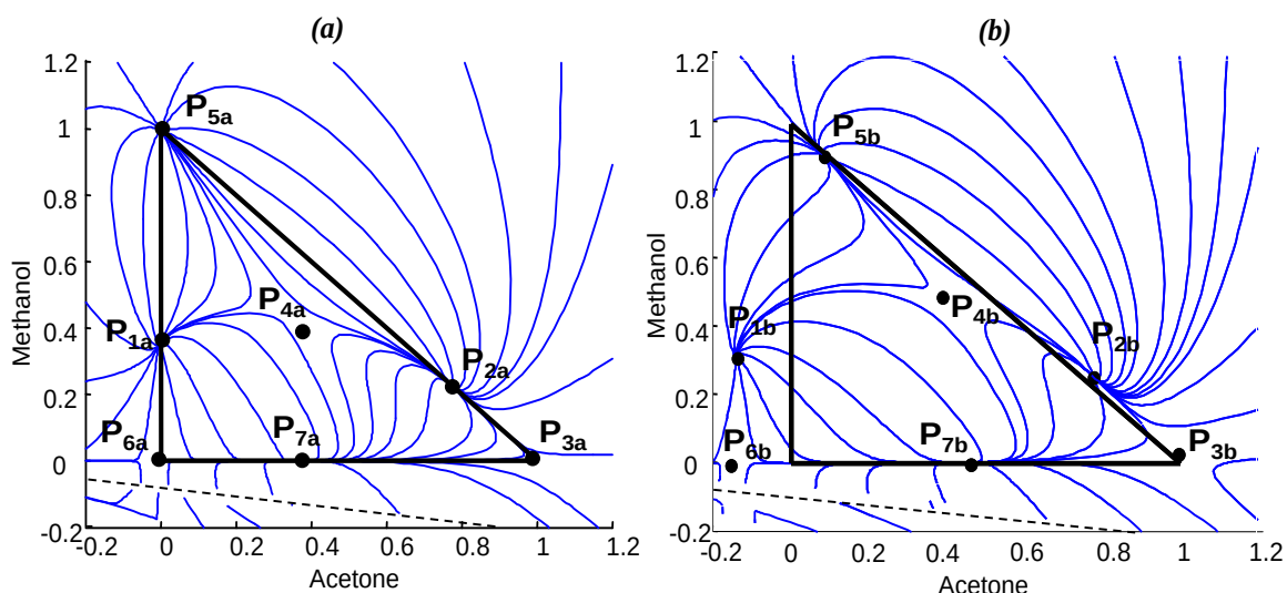
Figure 6.8: Column Profile Maps showing all stationary points for the Acetone/ Methanol/ Chloroform system at (a) infinite reflux and (b) at a finite reflux of R_A=8 and X_A=[0.8, 0.1] . Composition profiles are indicated by blue lines, while pinched compositions are given by black dots. Discontinuous regions are represented by a dashed black line.
