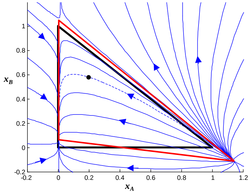
Figure 3.2: A Column Profile Map with a generalized reflux ratio of R_\Delta=9 and a Difference Point of X_\Delta = [0.2, 0.6] (black dot). The dashed blue lines represent principal profiles emanating from the Difference Point which corresponds to a CS with a product cut. Secondary column profiles, drawn in solid blue lines, represent CSs with the same Difference Point as the principal profile but with different entering liquid and vapour compositions. All profiles may be extended beyond the boundaries of the mass balance triangle (in black) for gaining a better understanding of both the topology and pinch points. Each profile approaches the stationary points indicated by the red triangle.
