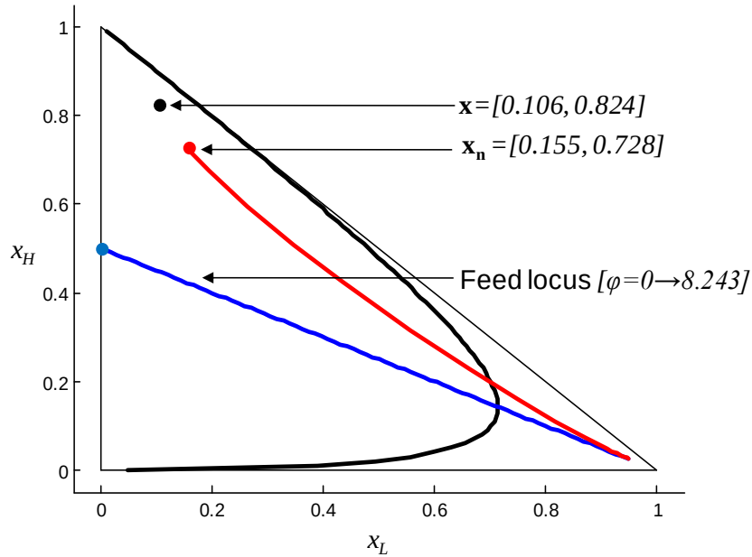
Figure 5.8: A CSTR coupled with a rectifying column section for R_A=3 , n=5 and X_A = [0.950, 0.025] . The red and blue line represent the Column Profile and the Feed locus line, respectively, while the red, black and blue dots represent the bottom liquid composition of the column section, the reactor composition and the feed composition that contains no product, respectively. The black curve represents the reaction equilibrium curve.
