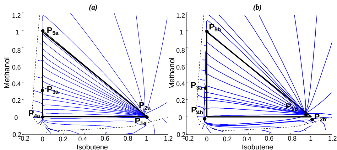
Figure 6.9: Column Profile Maps showing all stationary points for the Isobutene / MTBE / Methanol system at (a) infinite reflux and (b) at a finite reflux of R_A=-5 and X_A=[0.8, 0.1] . Composition profiles are indicated by blue lines, while pinched compositions are given by black dots. Discontinuous regions are represented by a dashed black line.
