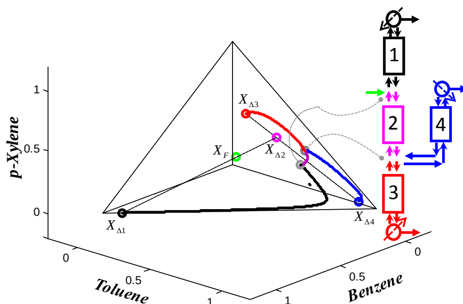
Figure 3.20: A feasible side rectifier design for the Benzene / Toluene / p-Xylene / Phenol system, showing areas of profile intersection and the location of all respective Difference Points.
