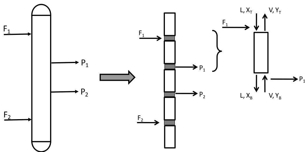
Figure 4.1: An example of a generalised column section
