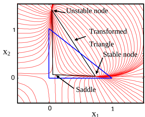
Figure 1: CPM for X_A = [0.3, -0.2] and R_A = 9
