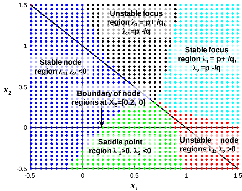
Figure 2.13: Eigenvalue map for x_i = [-0.5...1.5] at R_\Delta = 1.25
