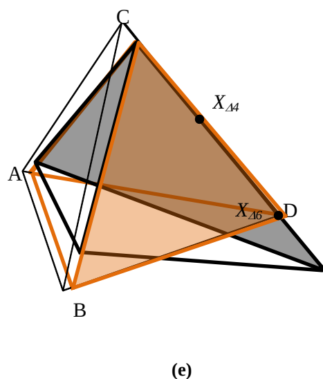
Figure 4.15: Transformed tetrahedrons at minimum reflux for the DSR. (a) Column sections 5 and 6. (b) Column sections 3 and 4. (c) Column sections 1 and 2. (d) Column sections 2 and 4. (e) Column sections 4 and 6.
