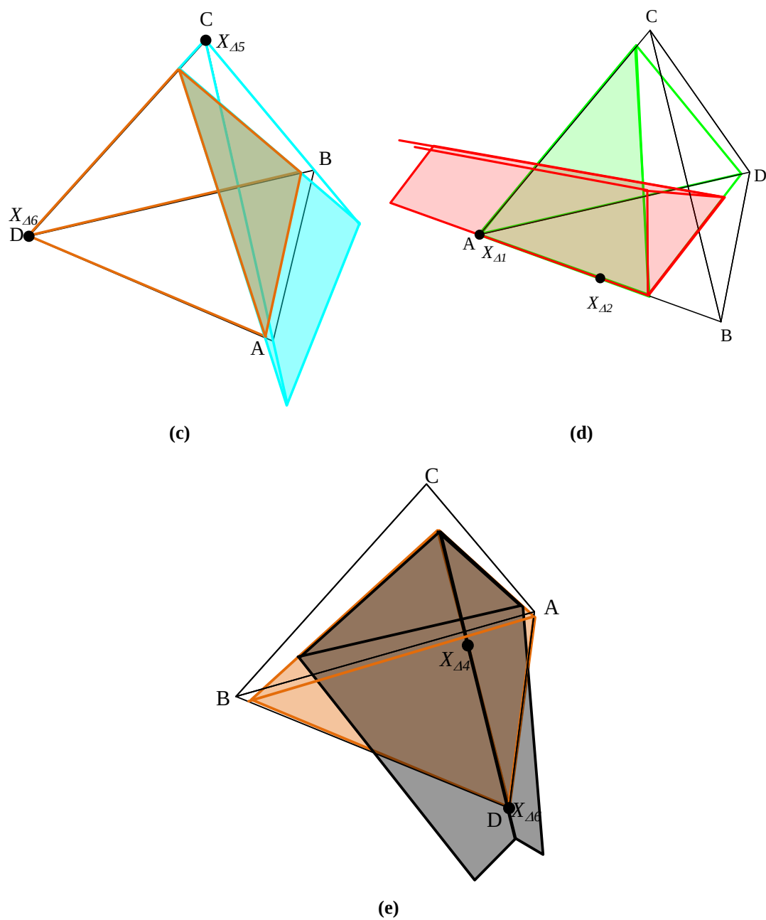
Figure 4.17: Transformed tetrahedrons at minimum reflux for the HSSR and Kaibel columns. (a) Column sections 1 and 3. (b) Column sections 2 and 4. (c) Column sections 5 and 6. (d) Column sections 1 and 2. (e) Column sections 4 and 6.
