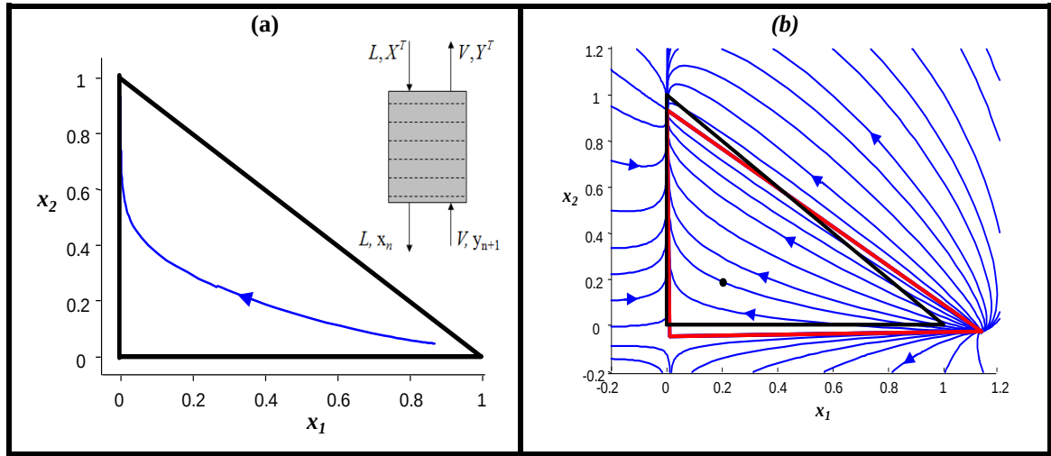
Figure 6.1: (a) A single liquid composition profile with R_\Delta=9 and X_\Delta=[0.2, 0.2] , with the definition of a generalized Column Section, and (b) a Column Profile Map with R_\Delta=9 and X_\Delta=[0.2, 0.2] where the blue lines represent the column profiles, inside and outside the positive composition space, and the red triangle indicates the shifted Pinch Points.
