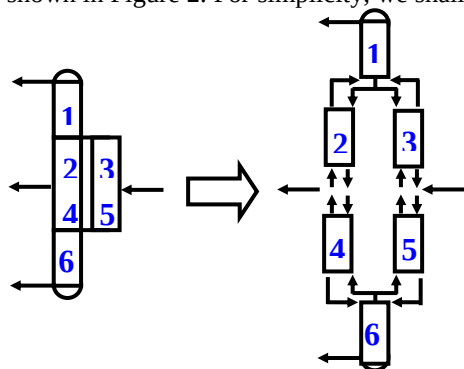
Figure 2: Column section breakdown for the Petlyuk column
