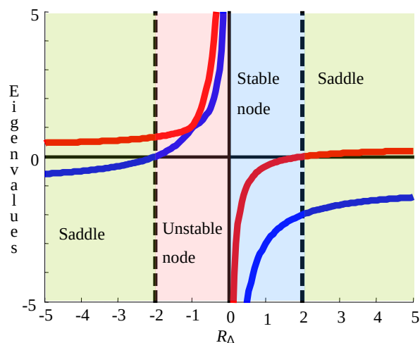
Figure 6: Operating regions for X_A=[0;0;1] Sharp split Kaibel column design
