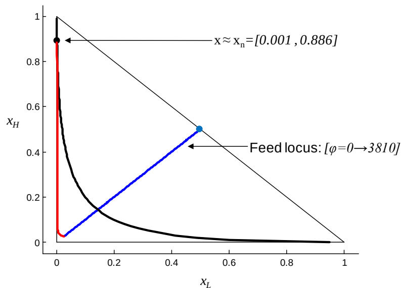
Figure 5.13: A CSTR coupled with a rectifying column section for R_A=10 , n=12 and X_A = [0.025, 0.025] . The red and blue line represent the column profile and the feed locus line, respectively, while the red, black and blue dots represent the bottom liquid composition of the column section, the reactor composition and the feed composition that contains no product, respectively. The black curve represents the reaction equilibrium curve.
