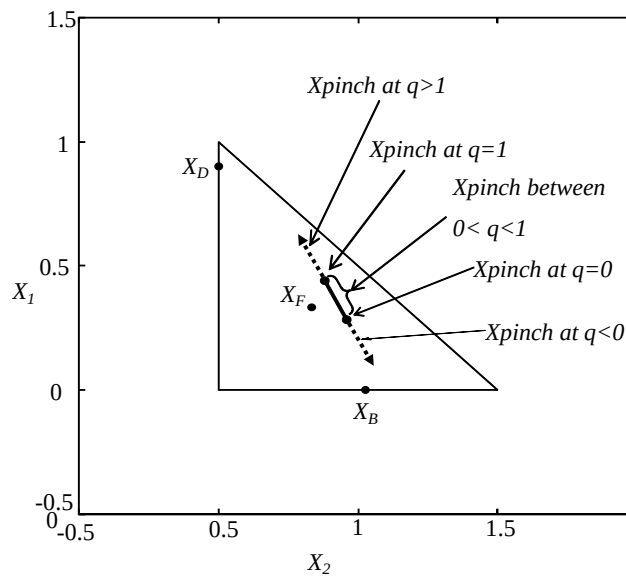
Figure 4.10: Pinch point locations for various feed qualities
