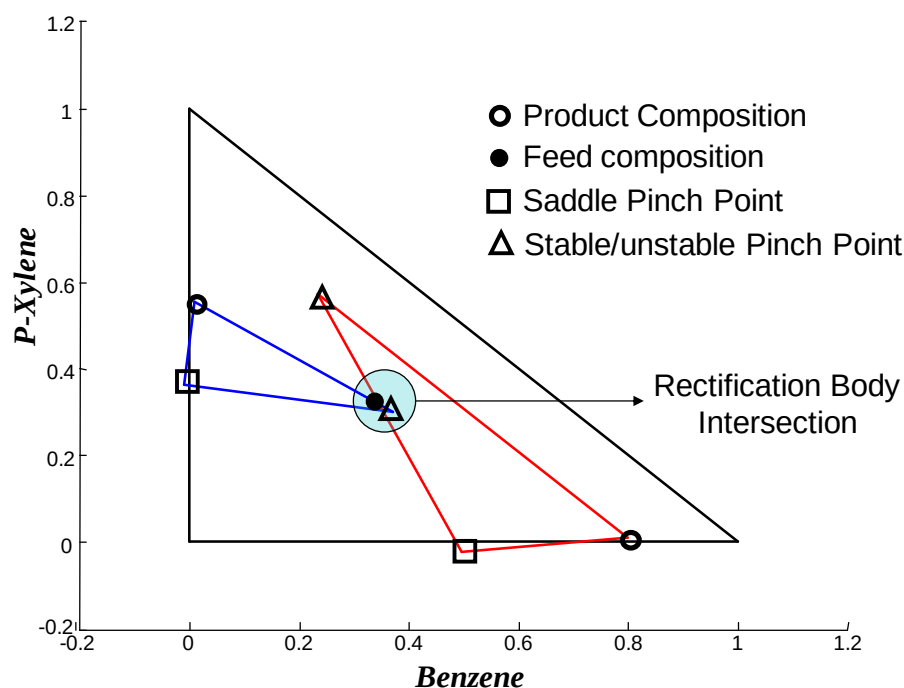
Figure 6.2: Intersecting Rectification Bodies for the Benzene / Xylene / Toluene system
