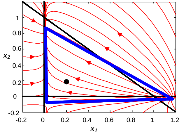
Figure 2.3 : A CPM with R_\Delta = 9 and X_\Delta = [0.2, 0.2] (marked with a dot) with a “shifted triangle” in blue indicating the movement of stationary points.
