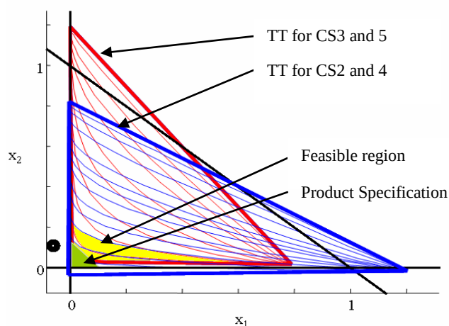
Figure 3: Superimposed transformed triangles for coupled column system
