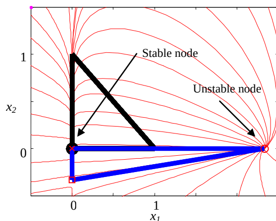
Figure 5: A stable node fixed on the intermediate boiler special case where X_A is placed on one of the 3 pure component vertices, a node is also fixed to the same vertex. So, by knowing the position of a stationary point and X_A , we can trace the nature of the node by varying R_A . For example, Figure 6 shows which values of R_A correspond to a specific node on the intermediate boiler vertex. The nature of the nodes are defined by the eigenvalues of the Jacobian when the DPE=0.
