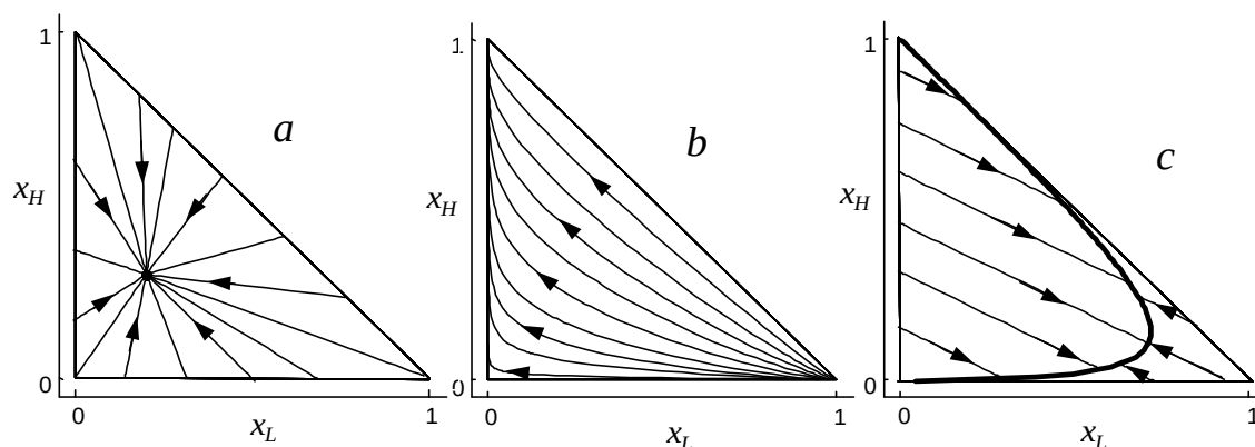
Figure 5.2: Phenomena vector fields for (a) Mixing with x_F = [0.2, 0.3] ; (b) Separation for a constant relative volatility system with \alpha = [5, 1, 2] ; and (c) Reaction for 1I + 1H \leftrightarrow 2L with elementary reaction rate and K_{eq} = 25
