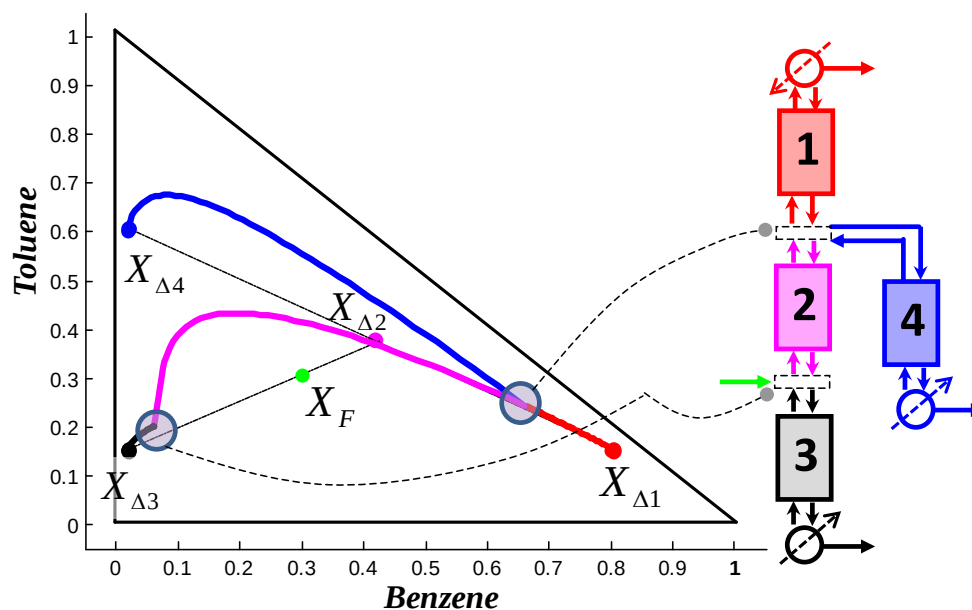
Figure 3.8: Feasibility of a side stripper arrangement for the Benzene / Toluene / p-Xylene system. The Bubble Point Distance between CS 2 and CS 3 , and the triple Bubble Point Distance between CS 1 , CS 2 and CS 4 , needs to be zero for the side stripper column to be feasible. This criterion is indicated by the highlighted areas
