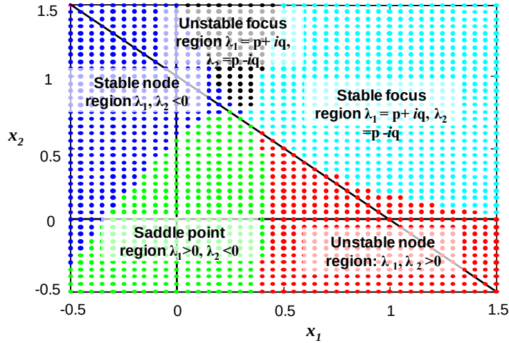
Figure 2.9: Eigenvalue map for x_i = [-0.5....1.5] at R_\Delta = \pm\infty
