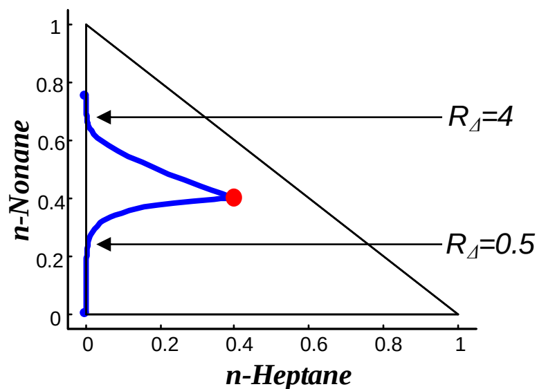
Figure 2.20: Column Profiles for X_\Delta = [0, 0] , with R_\Delta = 4 and R_\Delta = 0.5 respectively
