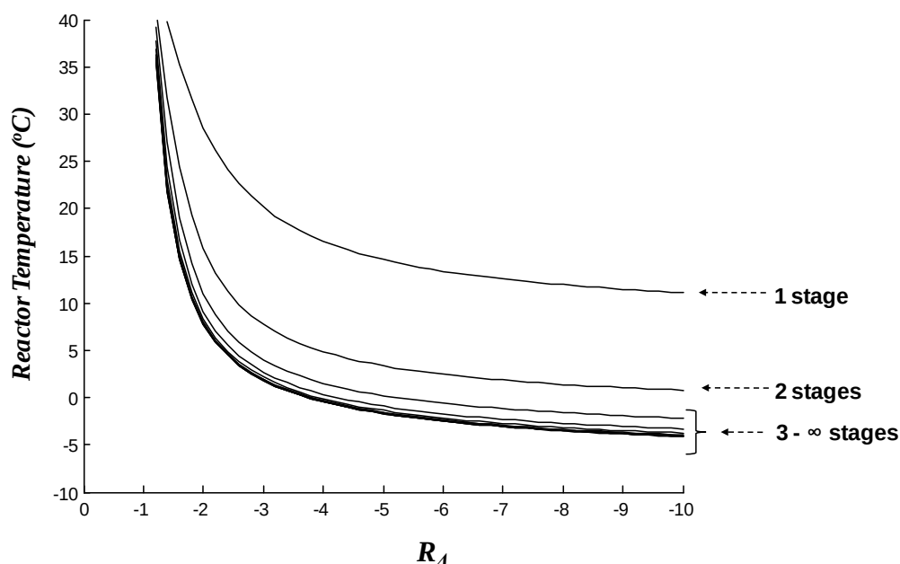
Figure 5.19 The effect of the number of stages and reflux ratio on reactor temperature for the MTBE process at 1 atm, with X_A=[0.950, 0.025] and x_{MTBE}=0 for a CSTR coupled to a stripping, non-reactive column section..
