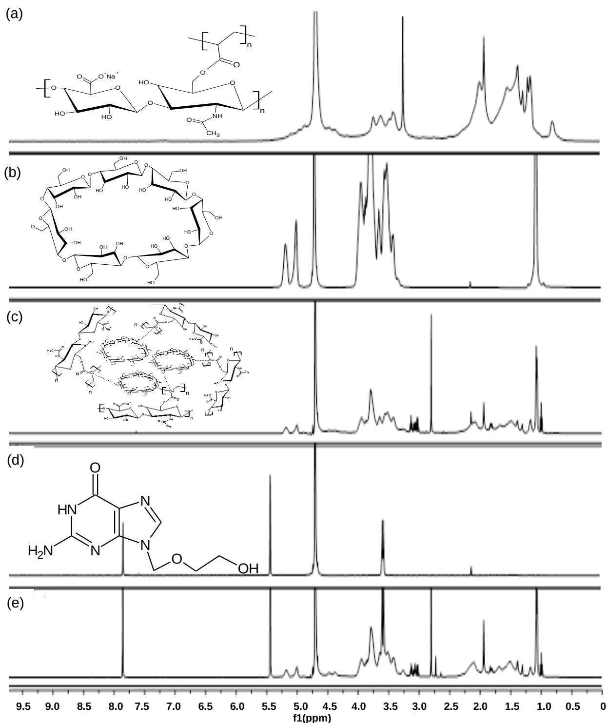
Figure 3.5: ^1\text{H} NMR spectra of (a) HAA-PAA, (b) HP- \beta -CD, (c) HA-PAA-HP- \beta -CD, (d) ACV and (e) ACV-loaded HA-PAA-HP- \beta -CD in \text{D}_2\text{O} .
