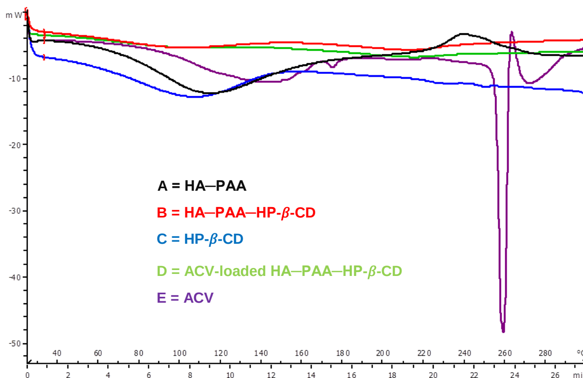
Figure 3.9: DSC thermograms of (a) HA–PAA, (b) HA–PAA–HP- \beta -CD; (c) HP- \beta -CD and d) ACV-loaded HA–PAA–HP- \beta -CD, measured from 25°C to 300°C.
