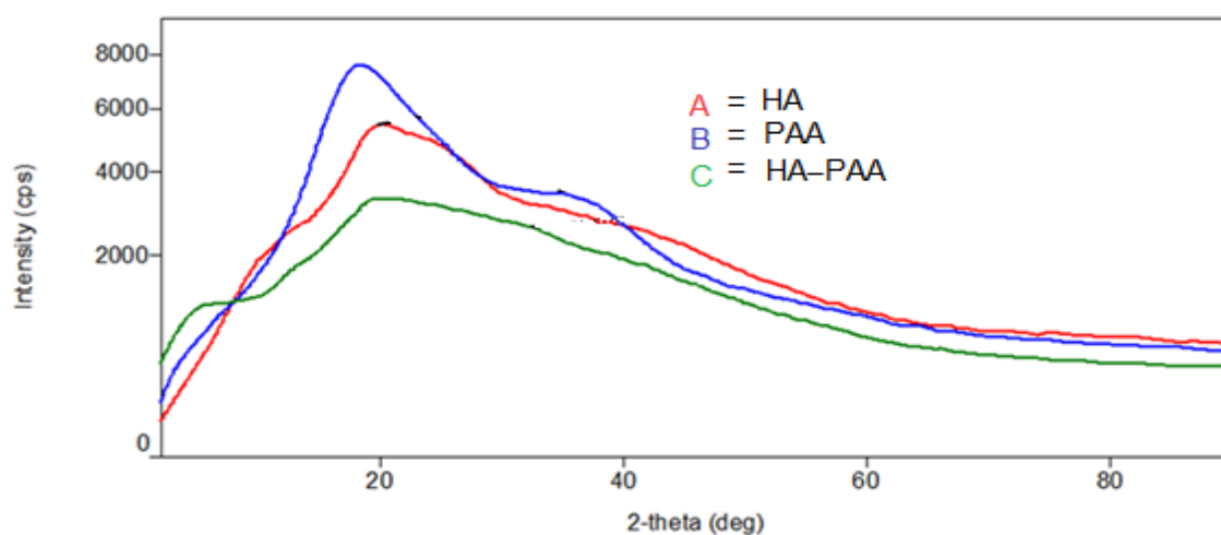
Figure 3.6: The XRD spectra for (a) HA, (b) PAA, and (c) HA–PAA.
