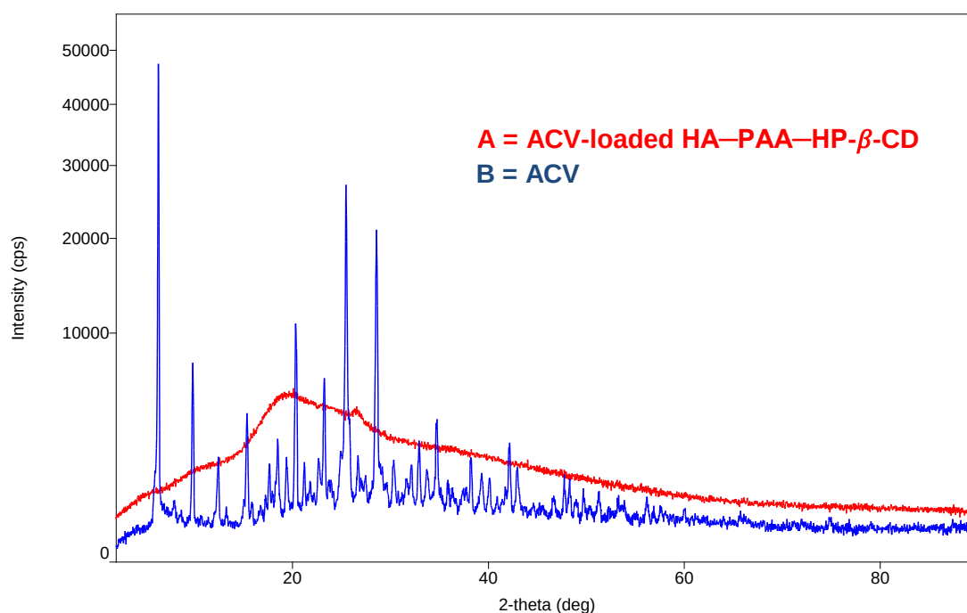
Figure 3.7.1: The XRD spectra for (a) ACV-loaded HA–PAA–HP-β-CD and (b) ACV
