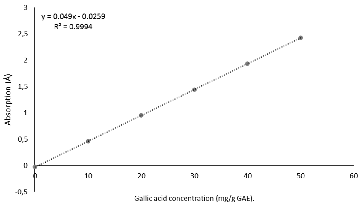
Figure 1. 27 Gallic acid standard curve for the quantification of TPC.
