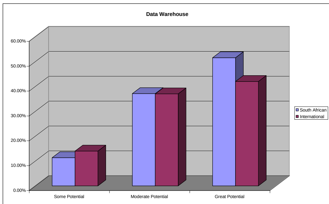
Figure 33: Data warehouse
