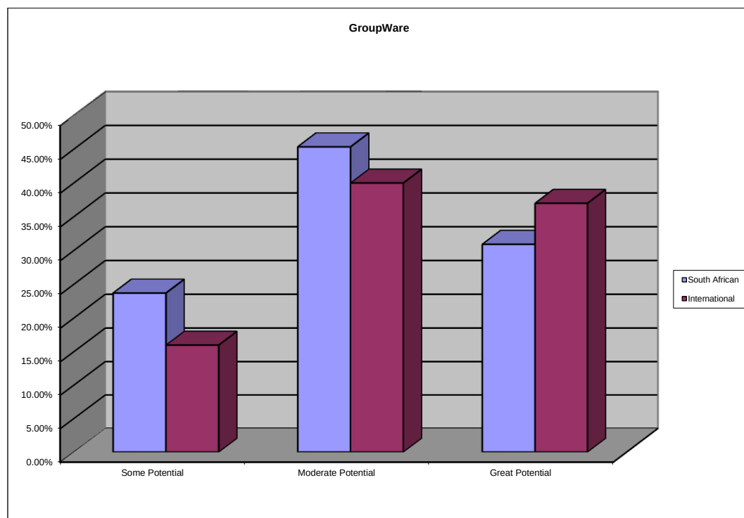
Figure 32: Groupware
