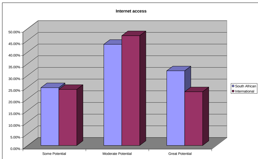
Figure 35: Internet access
