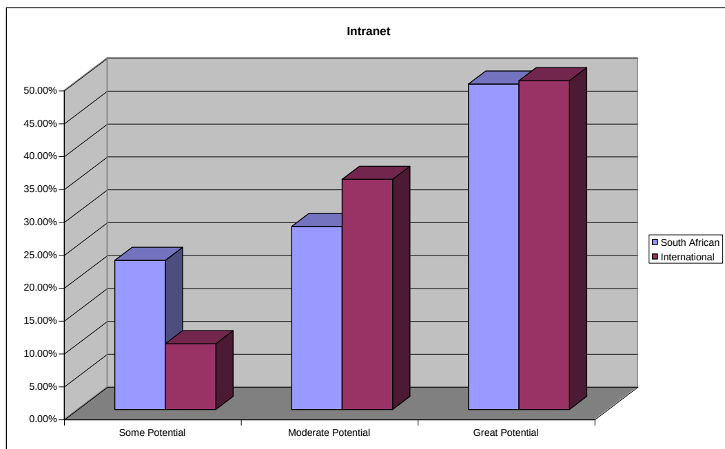
Figure 36: Intranet
