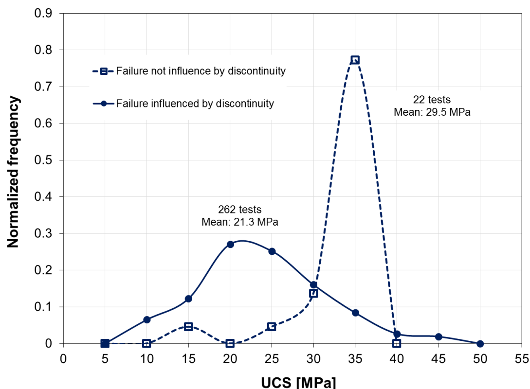
Figure 19. The influence of discontinuities on the strength of coal in uniaxial compression.
