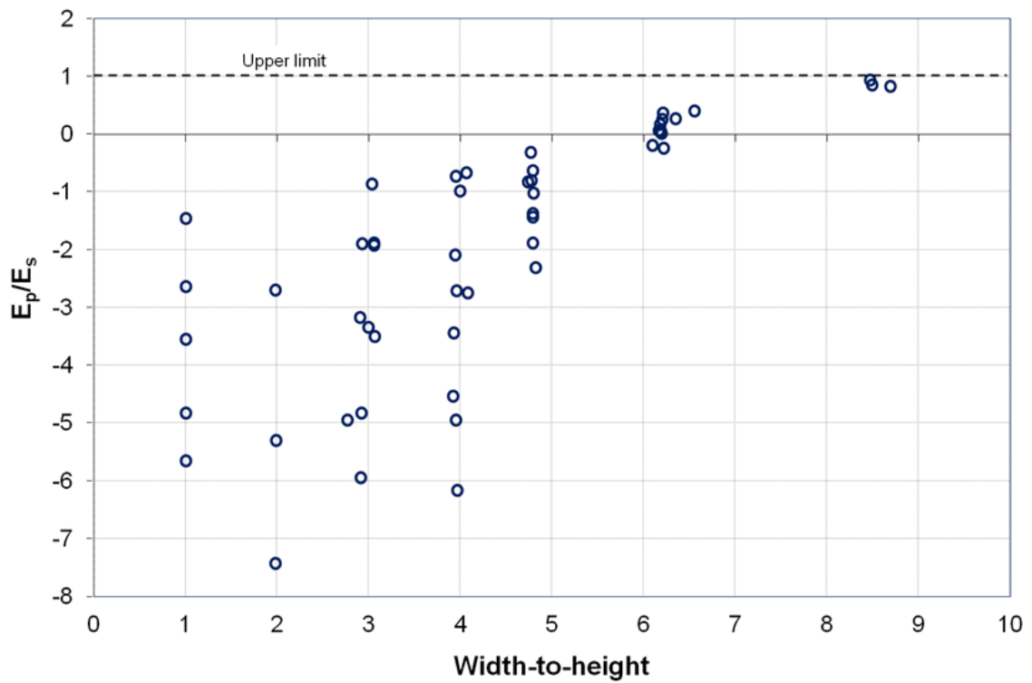
Figure 62. Modulus ratios E_p/E_s for coal-crete specimen of 42 mm diameter and varying w/h -ratios.
