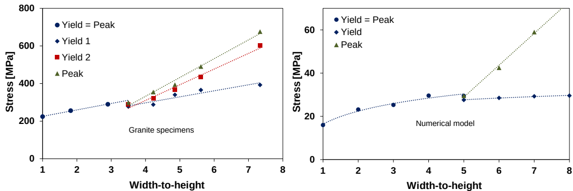
Figure 98. Yield and peak stresses observed in granite specimens (left) and numerical models (right).
