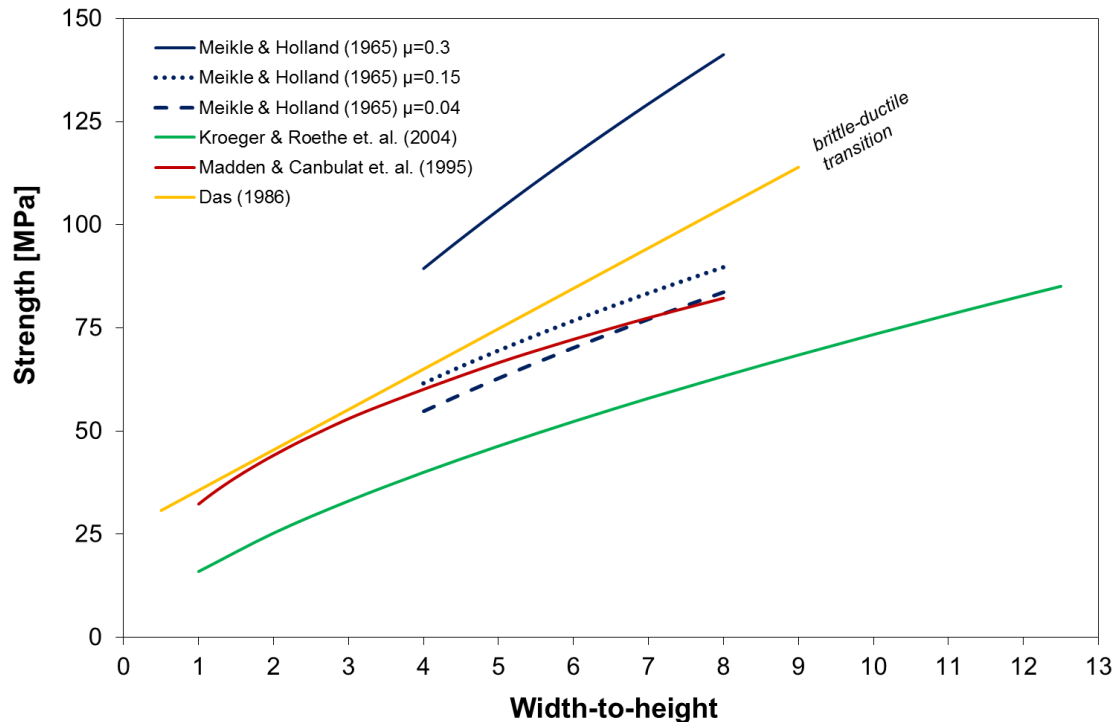
Figure 6. Compression tests on laboratory sized specimens of coal in the squat region by different investigators.
