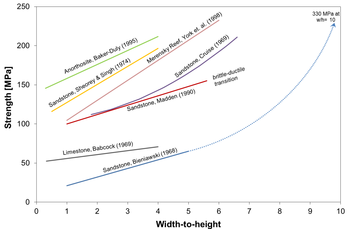
Figure 7. Compression tests on laboratory sized specimens of hard rock in the squat region by different investigators.
