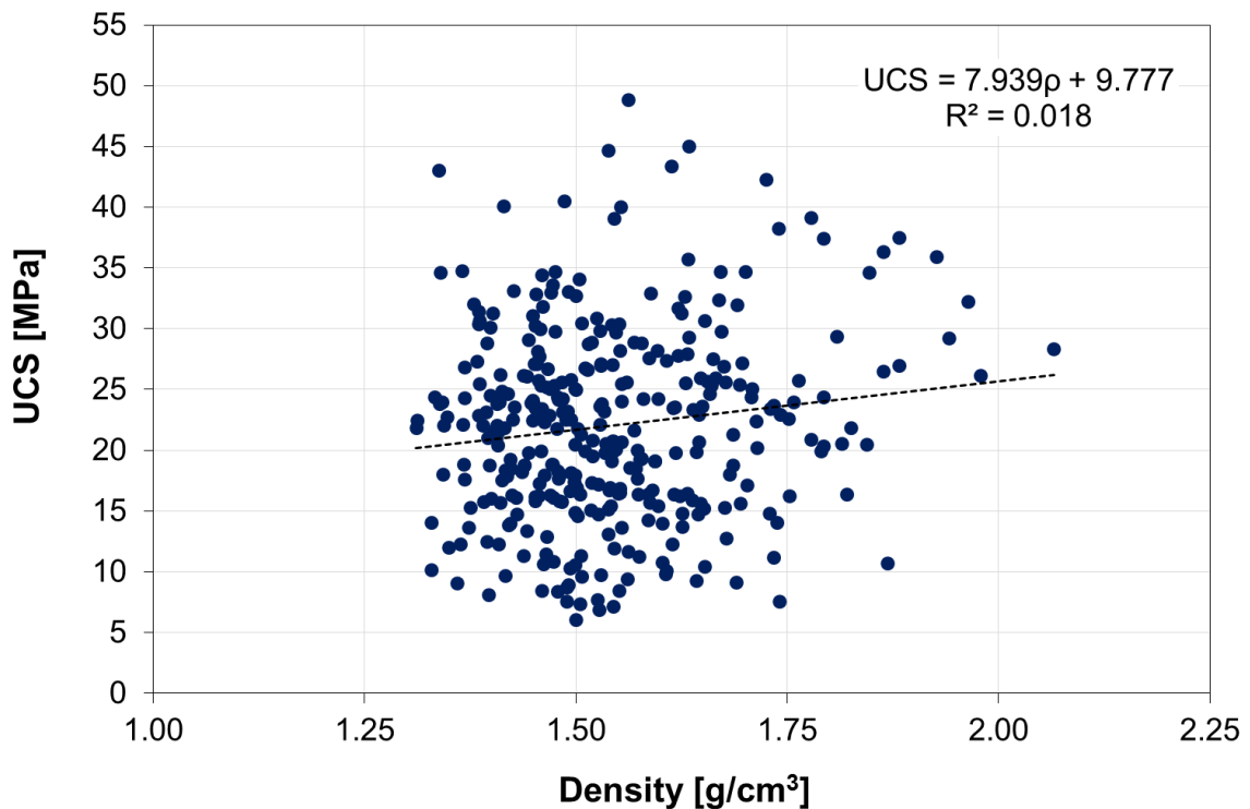
Figure 33. UCS versus density of coal specimens.
