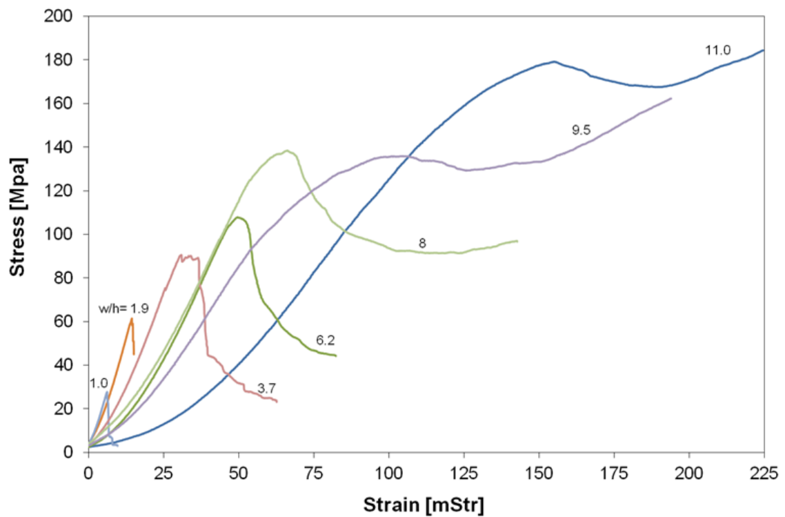
Figure 57. Examples of calculated stress-strain curves for coal specimens of 42 mm diameter at different w/h -ratios.
