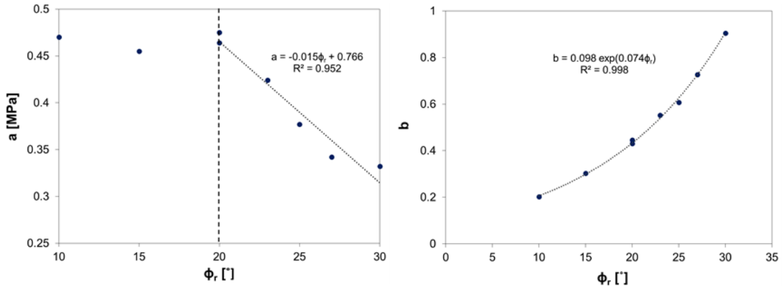
Figure 92. Relationship of the exponential strength parameters a and b with \phi_r in the FLAC models.
