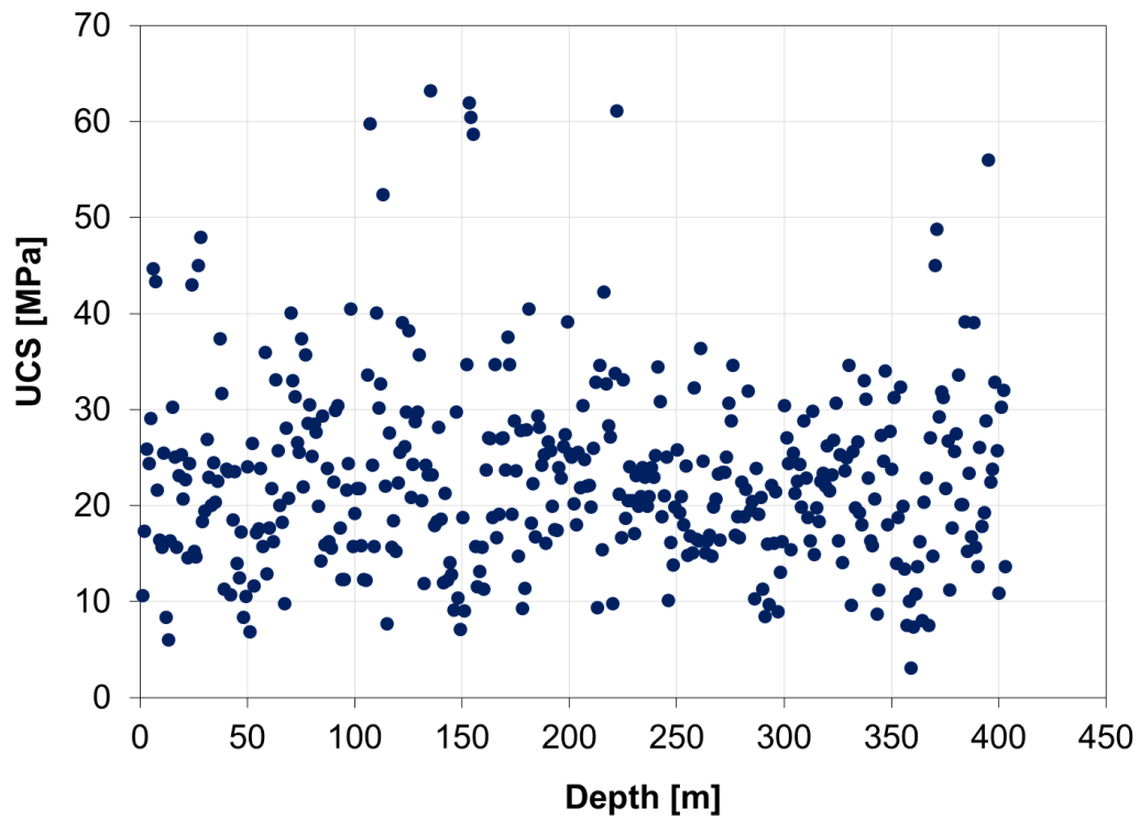
Figure 34. UCS versus depth of all coal specimens.
