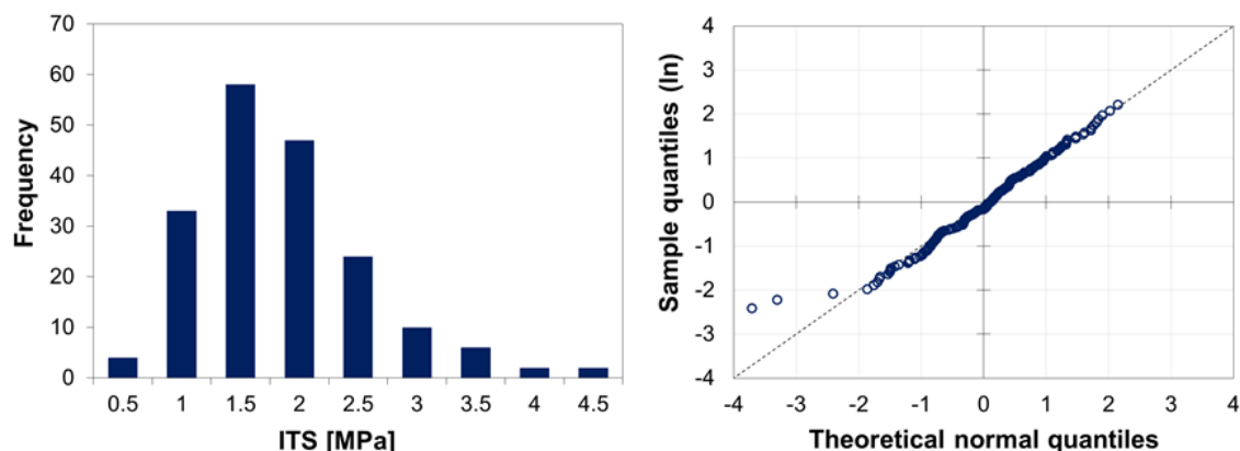
Figure 30. Histogram for the indirect tensile strength of South African coal determined on 186 coal specimens (left) and QQ -plot for a hypothesised lognormal distribution of the sample data (right).
