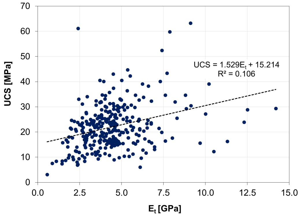
Figure 36. UCS versus tangential elastic modulus E_t for all coal specimens.
