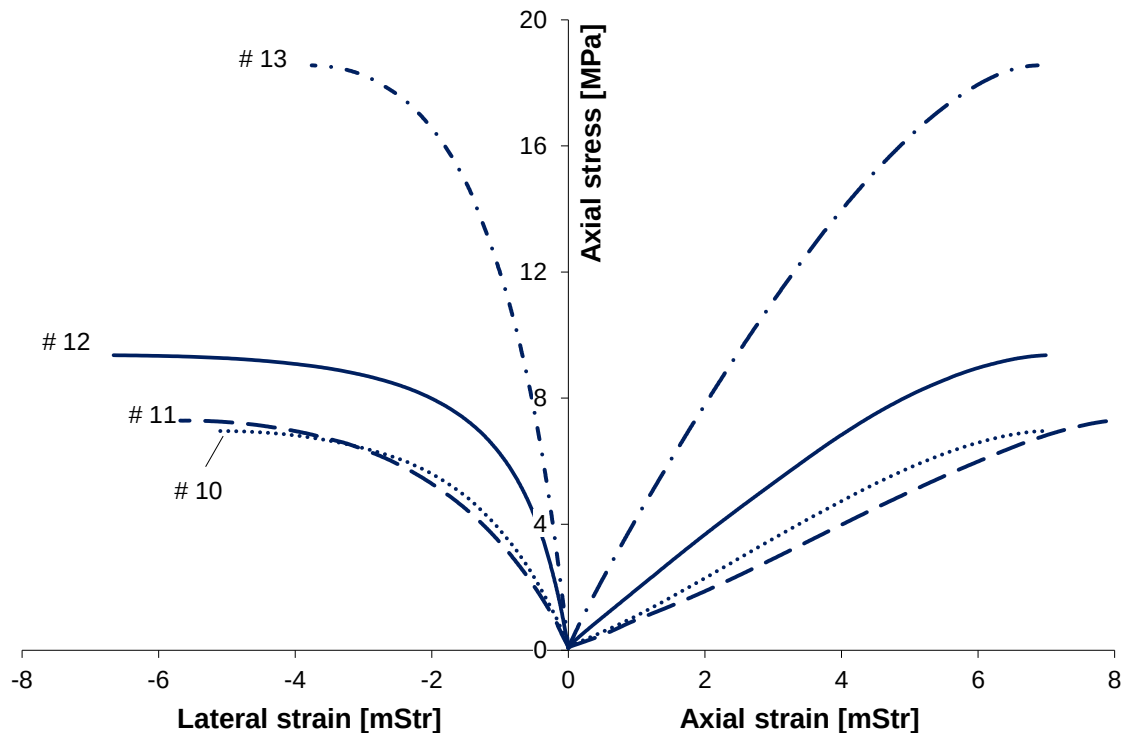
Figure 43. Stress-strain curves for coal-crete samples 10 – 13 with polymer binder.
