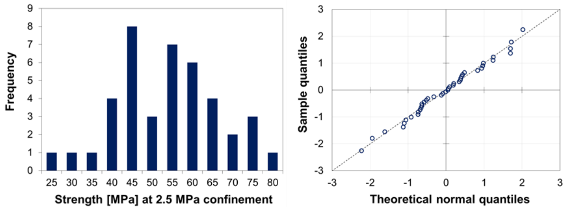
Figure 24. Histogram of the strength of 41 coal specimens at 2.5 MPa confinement (left) and QQ -plot for a hypothesised normal distribution of the data (right).
