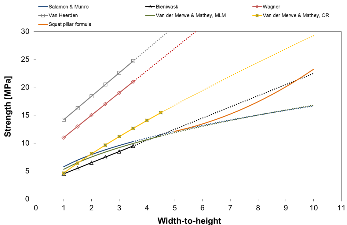
Figure 1. Comparison of South African coal pillar strength formulae for an assumed pillar height of 3 m.
