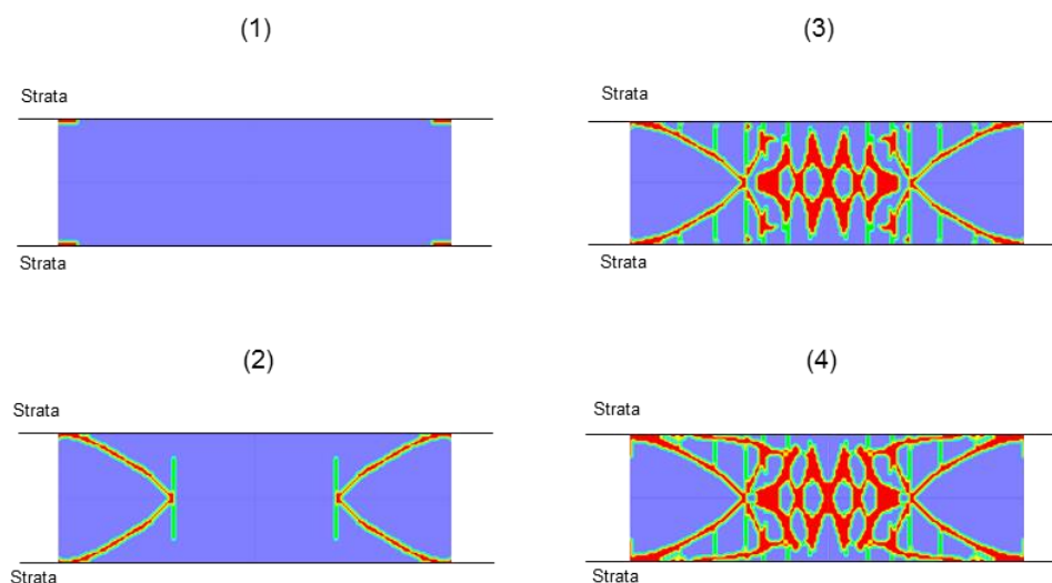
Figure 90. Evolution of failure in a pillar of w/h = 3 with perfectly stiff and rigid interfaces with the surrounding strata, demonstrated as stepwise loss of cohesion (red zones) during pillar loading.
