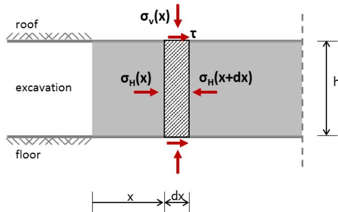
Figure 9. Limit equilibrium conditions around a pillar 'slice' in analytical models.
