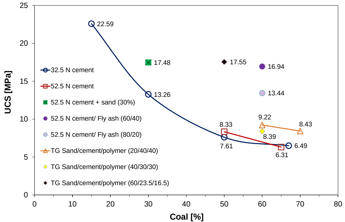
Figure 44. The uniaxial compressive strength of coal-crete.
