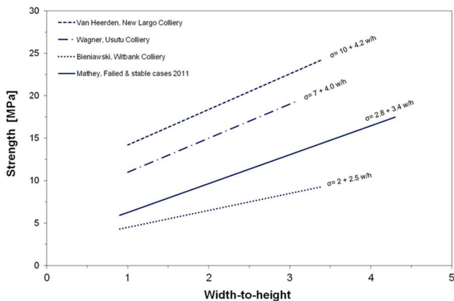
Figure 81. The strength of in-situ coal pillars in linear expression.
