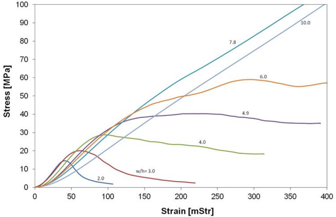
Figure 60. Examples of calculated stress-strain curves for coal-crete specimens of 150 m square width at different w/h -ratios.
