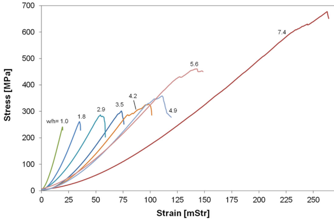
Figure 56. Examples of calculated stress-strain curves for granite specimens of 42 mm diameter at different w/h -ratios.
