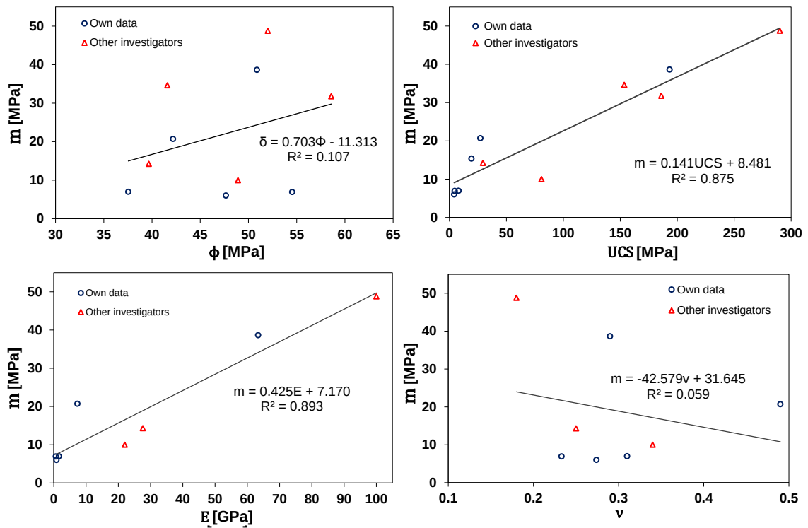
Figure 80. Correlations between the gradient of strength increase m and the mechanical properties of the materials.
