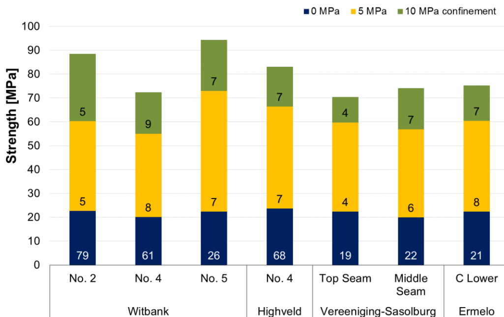
Figure 28. The average compressive strength of coal specimens from different seams at 0 MPa, 5 MPa and 10 MPa confinement. The number of tests evaluated for each confinement level are given at the base of the bars.
