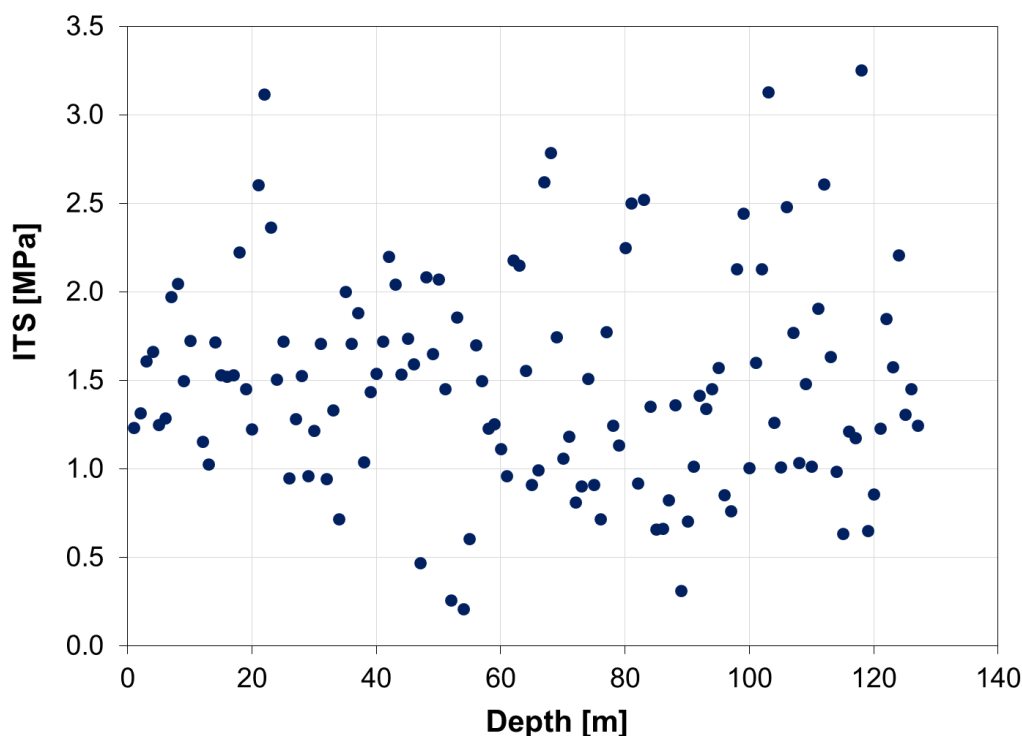
Figure 38. ITS versus depth of all coal specimens.
