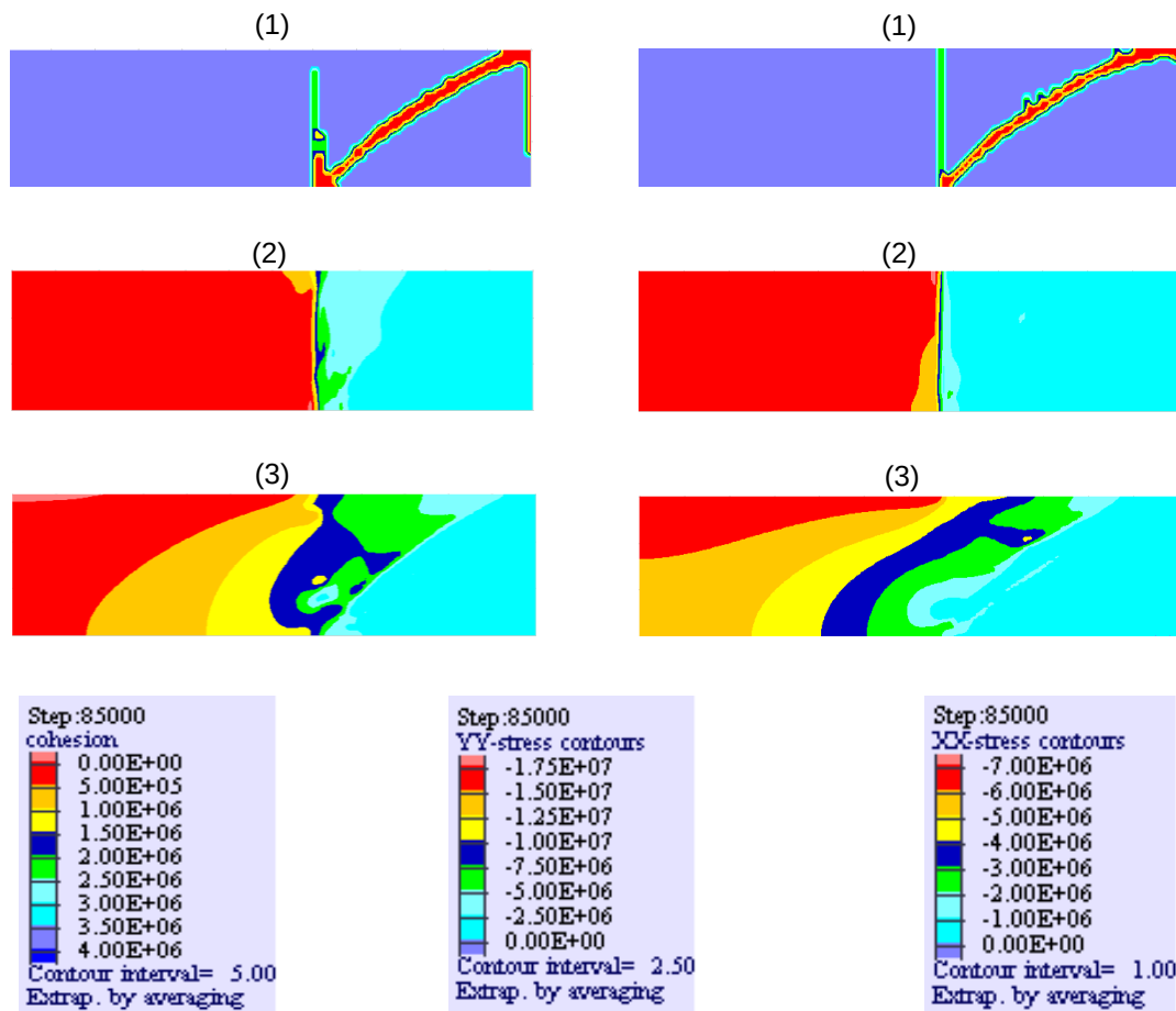
Figure 91. The effect of residual friction on the squat effect in FLAC model pillars.
