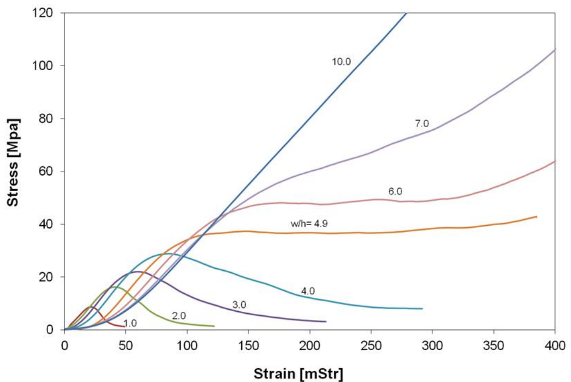
Figure 59. Examples of calculated stress-strain curves for coal-crete specimens of 100 mm square width at different w/h -ratios.
