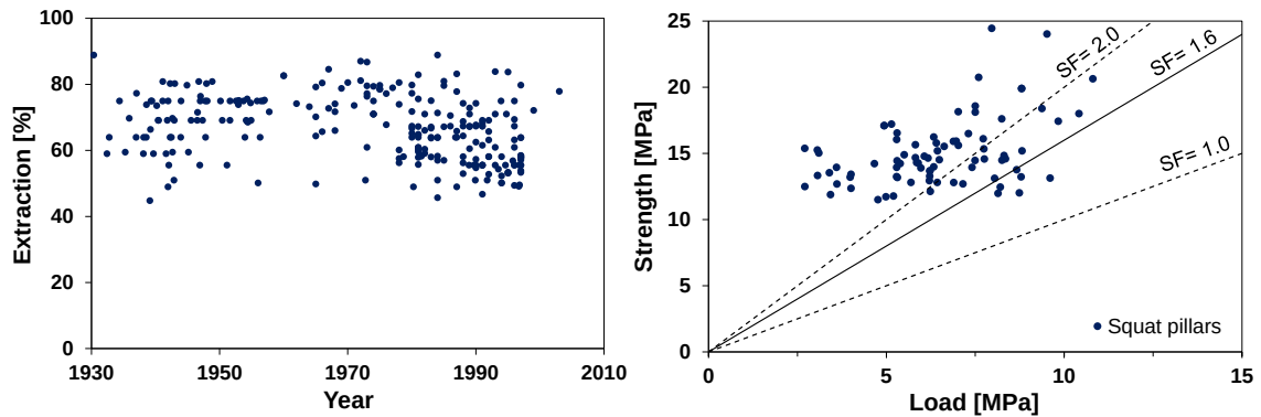
Figure 102. Extraction ratio in slender pillar layouts ( w/h < 5 ) over time (left) and safety factors used in squat pillar layouts calculated after the latest maximum-likelihood updated pillar strength equation (right).
