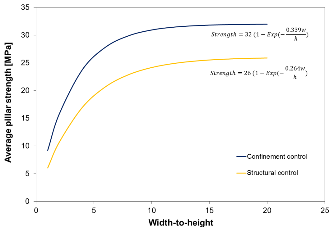
Figure 5. Coal pillar strength after Maleki (1992).
