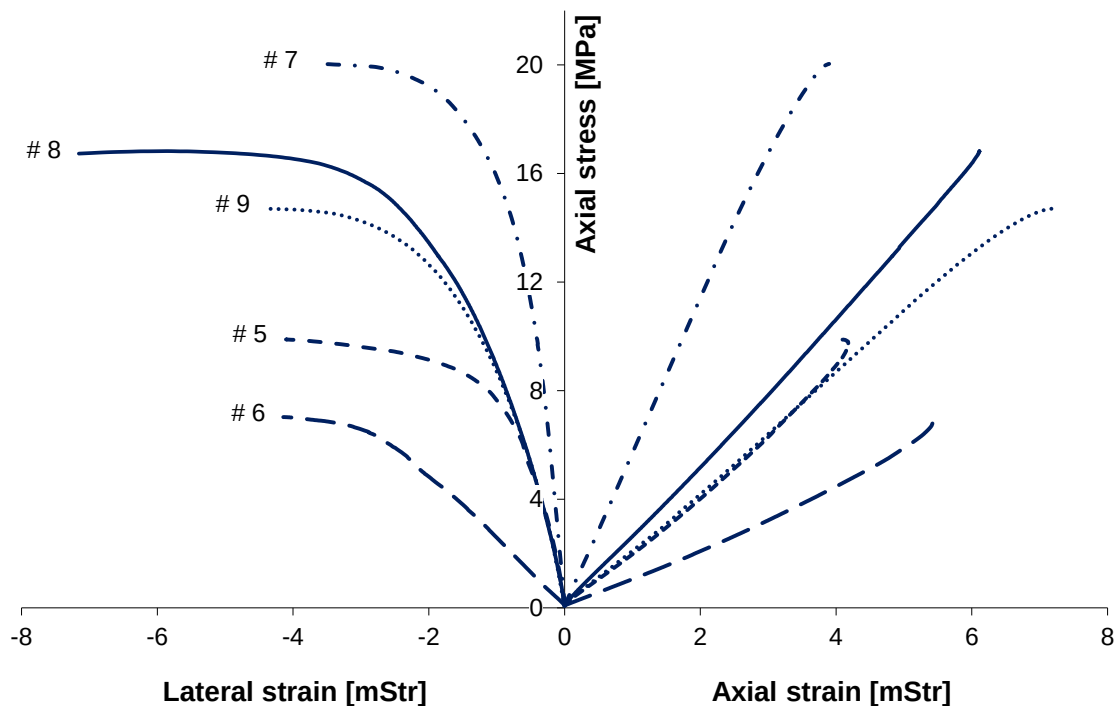
Figure 42. Stress-strain curves for coal-crete samples 5 – 9 without polymer binder.
