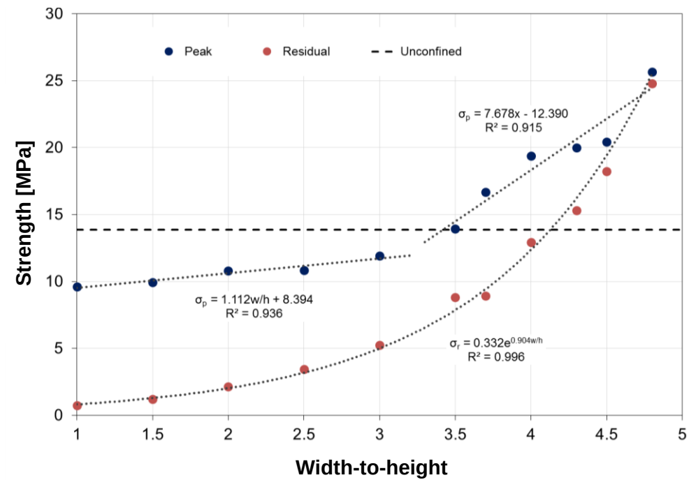
Figure 87. FLAC-computed peak and residual pillar strength versus w/h -ratio for model pillars in scenario S1.
