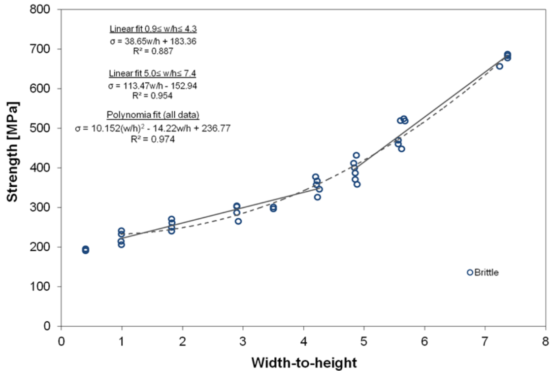
Figure 68. Strength of granite specimen of 42 mm diameter and various w/h -ratios.
