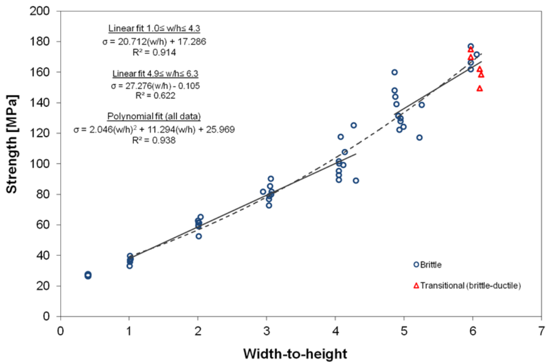
Figure 67. Strength of sandstone specimen of 42 mm diameter and various w/h -ratios.
