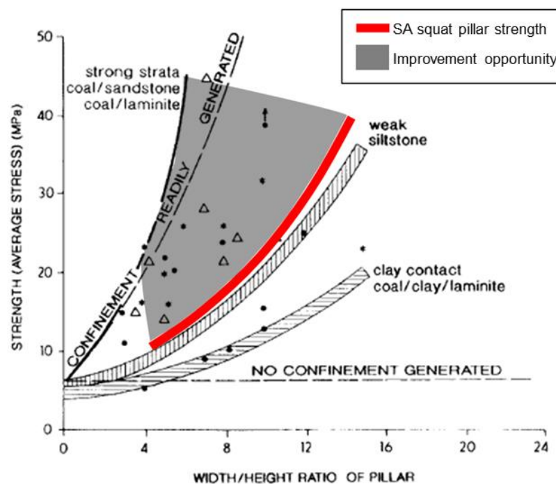
Figure 12. Strength and width-to-height for different geological environments, according to Gale (1999), overlain with current South African squat pillar strength and improvement opportunity.
