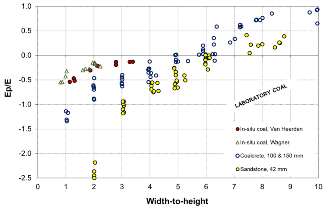
Figure 83. Post-beak behaviour of specimens in the laboratory and in-situ.
