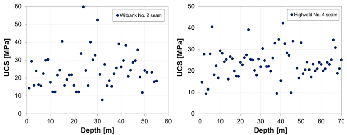
Figure 35. UCS versus depth of coal specimens from the Witbank No. 2 seam (left) and Highveld No. 4 seam (right).
