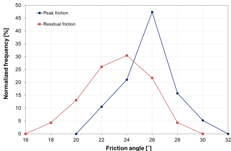
Figure 84. Normalized frequency distribution of coal-rock friction angles, re-analysed after specimen tests provided by York, Canbulat and Jack (2000).
