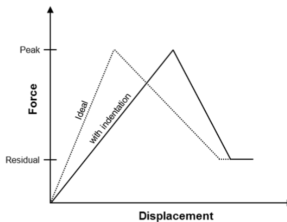
Figure 50. The effect of indentation in the testing setup on the recorded force-displacement curve for specimens.
