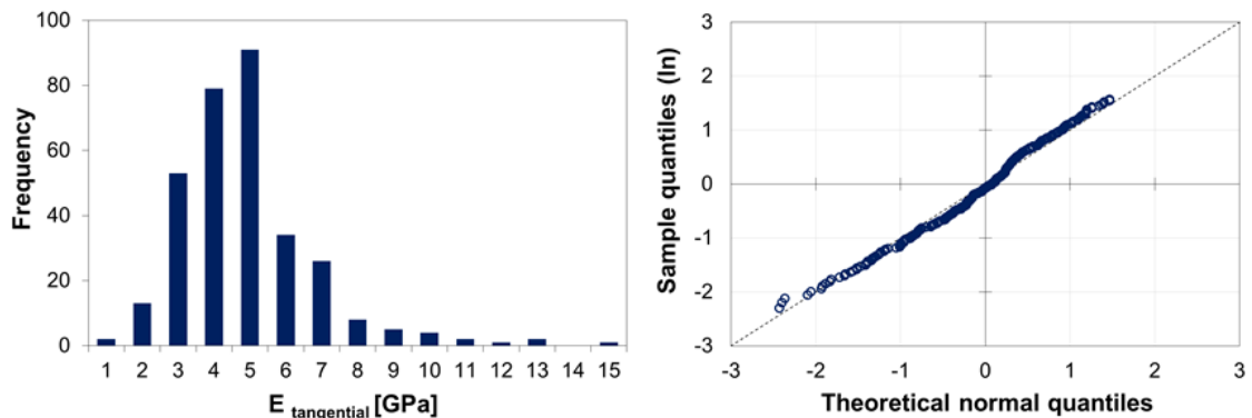
Figure 22. Histogram for the tangential elastic modulus measured on 322 coal specimens (left) and QQ -plot for a hypothesised lognormal distribution of the sample data (right).
