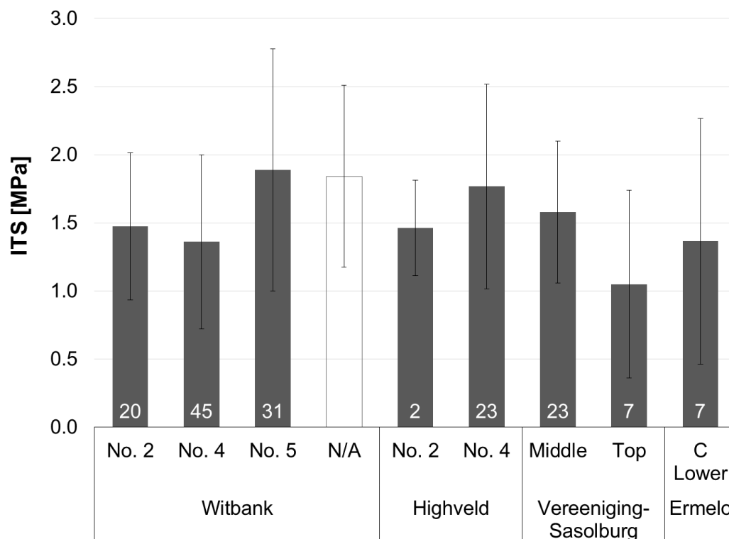
Figure 31. Seam-specific average ITS with accompanying standard deviations of coal in various coalfields in South Africa. The number of tests evaluated per coal seam are given in the base of the columns.
