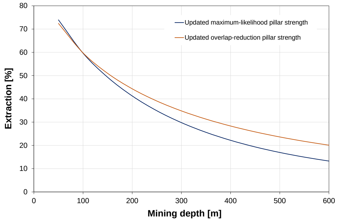
Figure 103. Extraction ratio versus mining depth for pillar design based on the updated empirical pillar strength equations.
