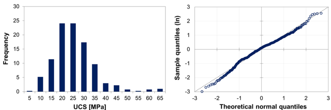
Figure 18. UCS histogram for all 403 specimens (left) and QQ -plot for a hypothesised lognormal distribution of the UCS (right).
