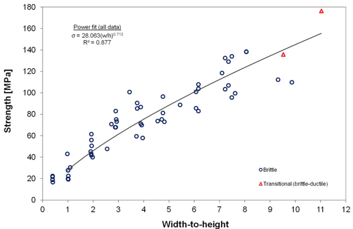
Figure 69. Strength of coal specimen of 42 mm diameter and various w/h -ratios.
