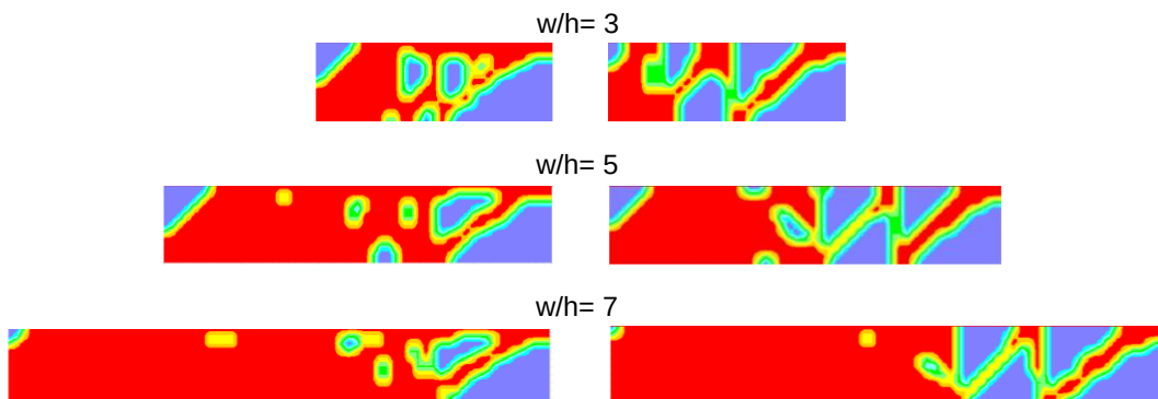
Figure 96. Stress-strain behaviour, strength trends and failure pattern in FLAC model pillars with “coarse” mesh, brittle constitutive law, in-situ boundary conditions and different w/h -ratios.
