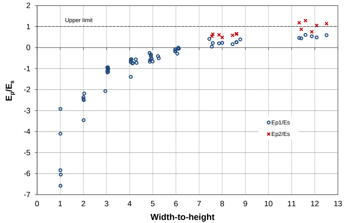
Figure 63. Modulus ratios E_p/E_s for sandstone specimen of 42 mm diameter and varying w/h -ratios.
