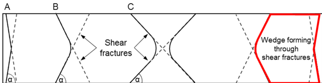
Figure 73. Idealized cross-section of fracture patterns in specimens of w/h = 2 - 6 .
