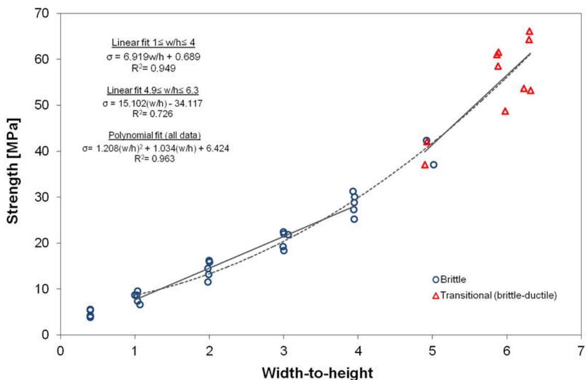
Figure 65. Strength of coal-crete specimen of 100 mm width and various w/h -ratios.
