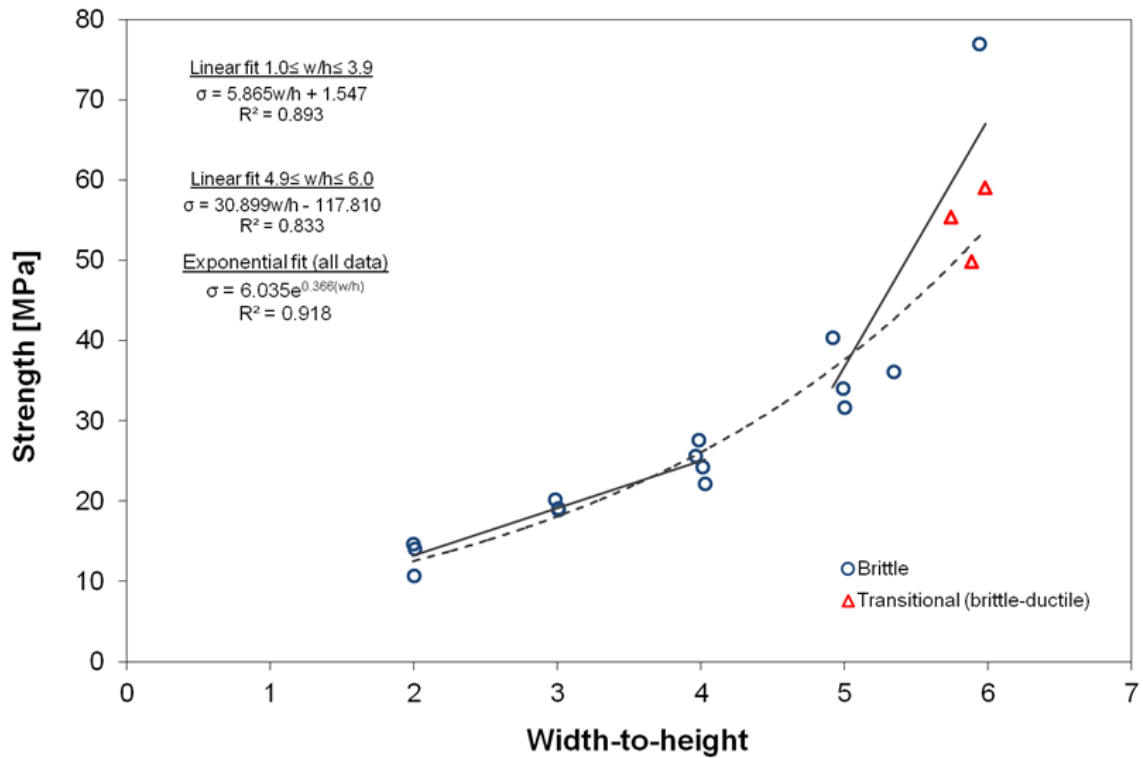
Figure 66. Strength of coal-crete specimen of 150 mm width and various w/h -ratios.
