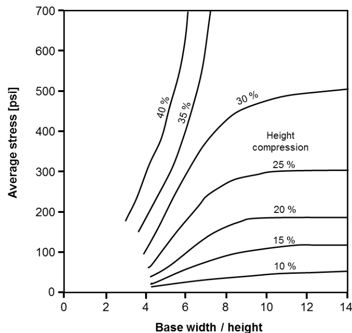
Figure 8. Relationship between specimen width-to-height ratio and average load bearing capacity of crushed granite aggregates at various levels of compression, reproduced after Schümann and Cook (1967).
