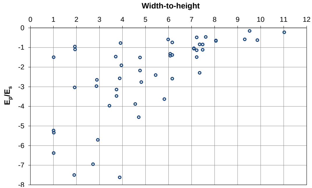
Figure 64. Modulus ratios E_p/E_s for coal specimen of 42 mm diameter and varying w/h -ratios.
