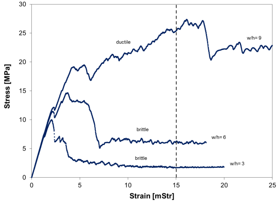
Figure 86. Typical stress-strain behaviour for brittle FLAC pillar models in scenario S2.
