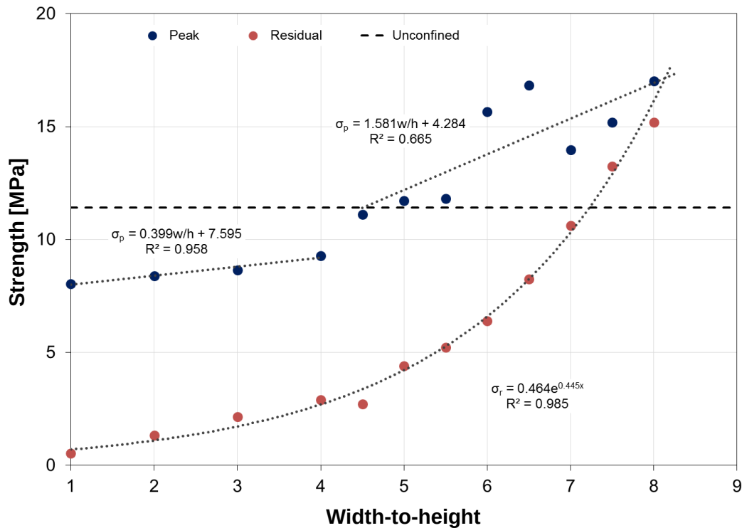
Figure 89. FLAC-computed peak and residual pillar strength versus w/h -ratio for model pillars in scenario S3.
