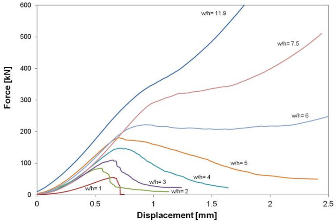
Figure 52. Examples of force-displacement curves for sandstone specimen and varying w/h -ratio.
