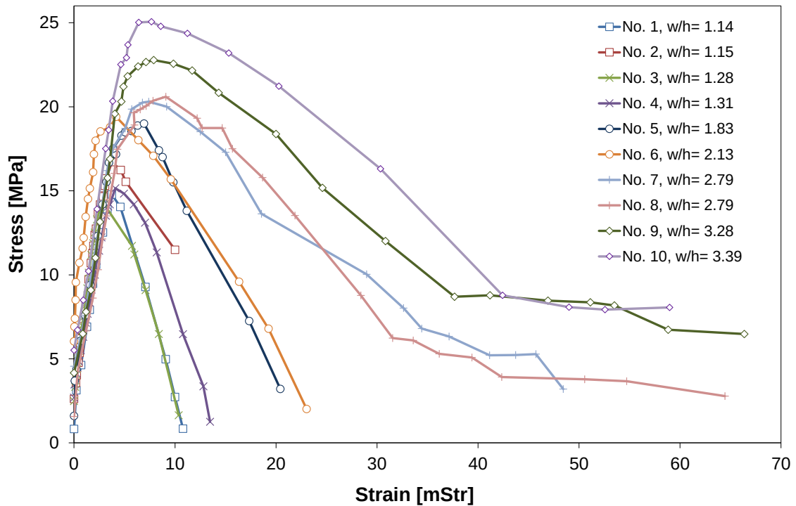
Figure 99. Stress-strain behaviour of coal pillars in Van Heerden's large-scale in-situ tests, reproduced from Van Heerden (1974).
