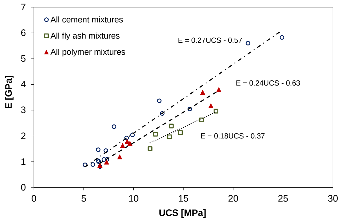
Figure 45. Young's Modulus E versus UCS of coal-crete.
