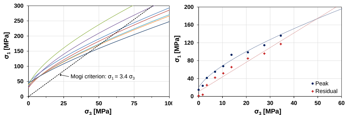
Figure 104. Estimation of brittle-ductile transition in coal specimens through Mogi's criterion in conjunction with extrapolated peak strength trends for South African coals (left) and from triaxial tests conducted by Kripakov (1981) (right).
