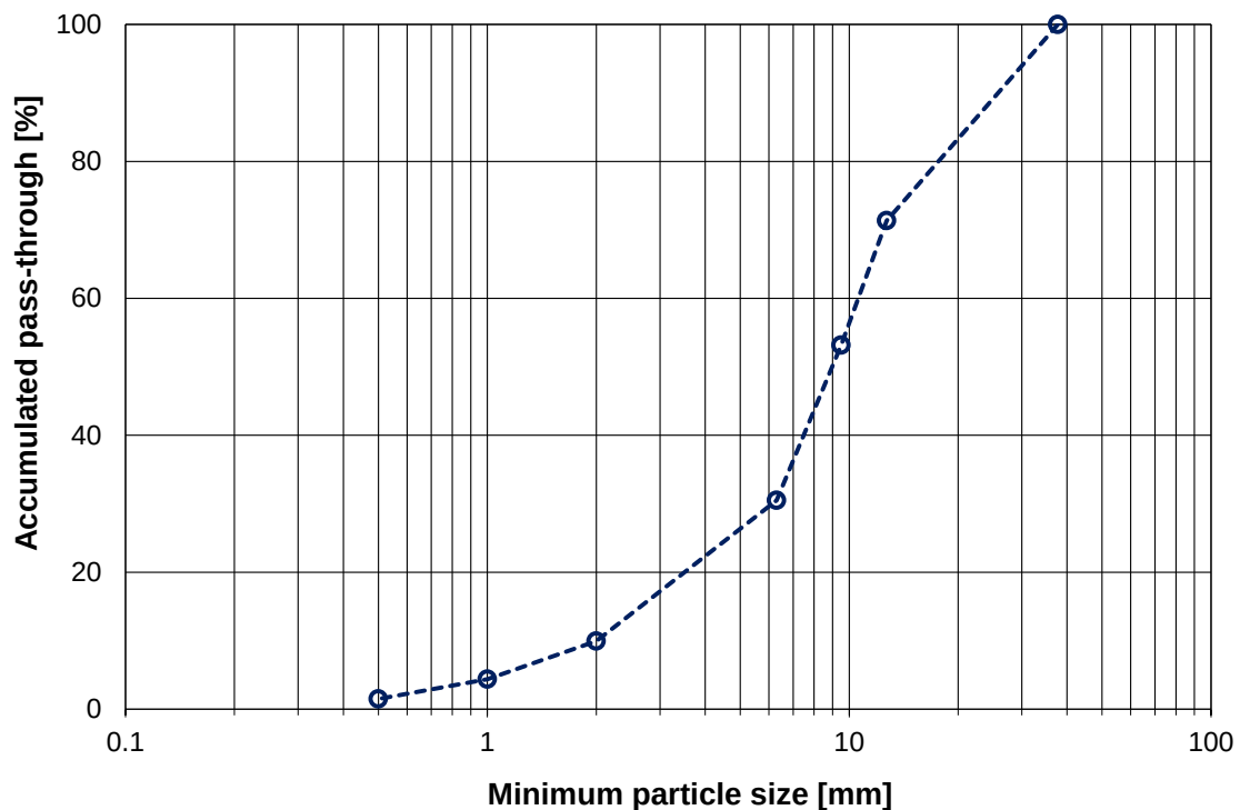
Figure 40. Sieve analysis of coal debris used in the coal-crete development study.
