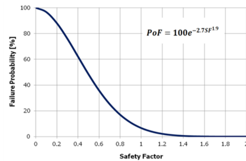
Figure 4. Link between the safety factor and failure probability for coal pillars whose strength is calculated with the updated maximum likelihood strength equation.
