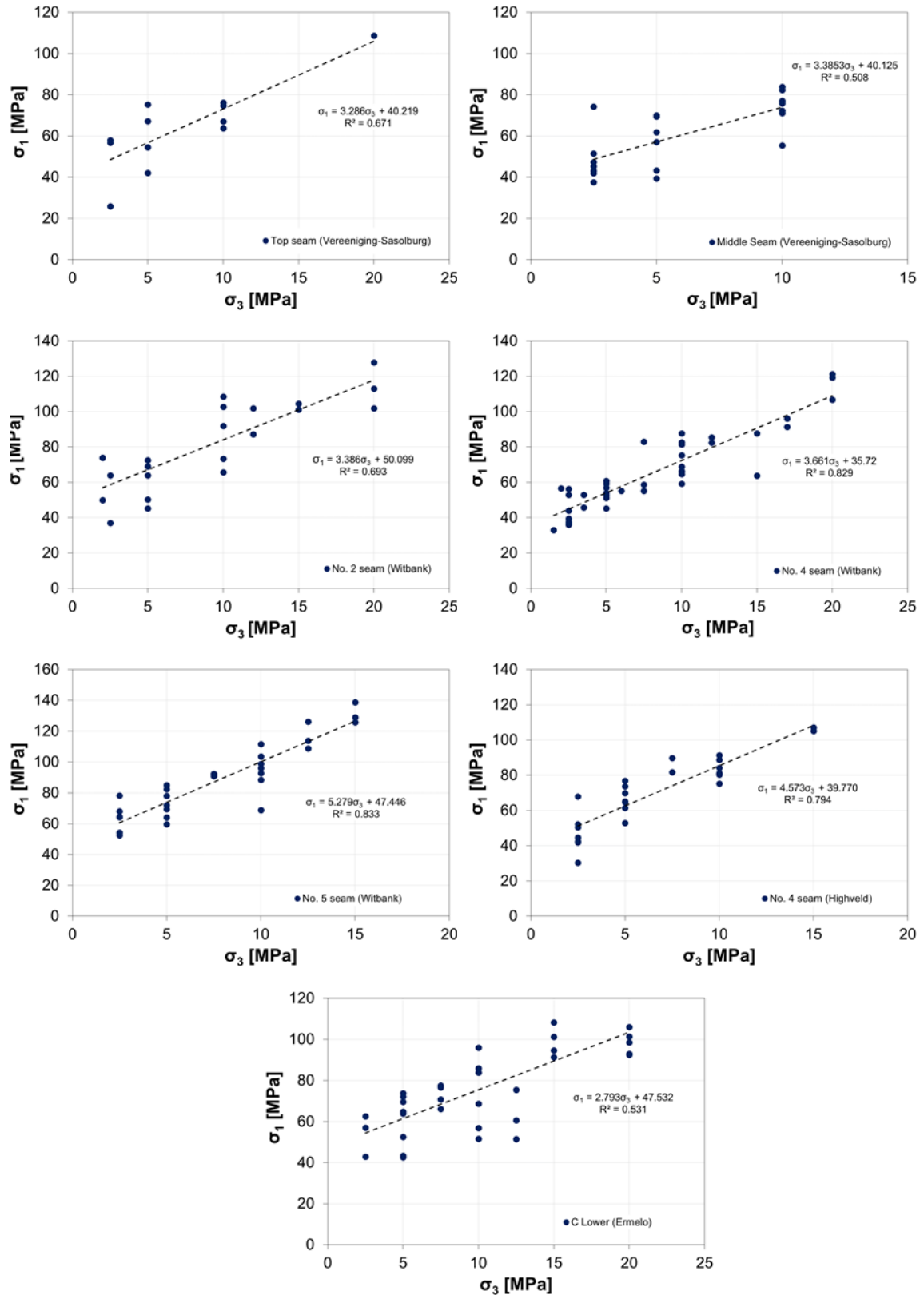
Figure 29. \sigma_1 - \sigma_3 plots of triaxial coal strength in different coal seams.
