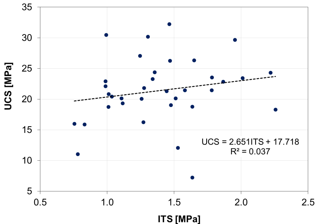
Figure 37. Average sample UCS versus average sample ITS of coal.
