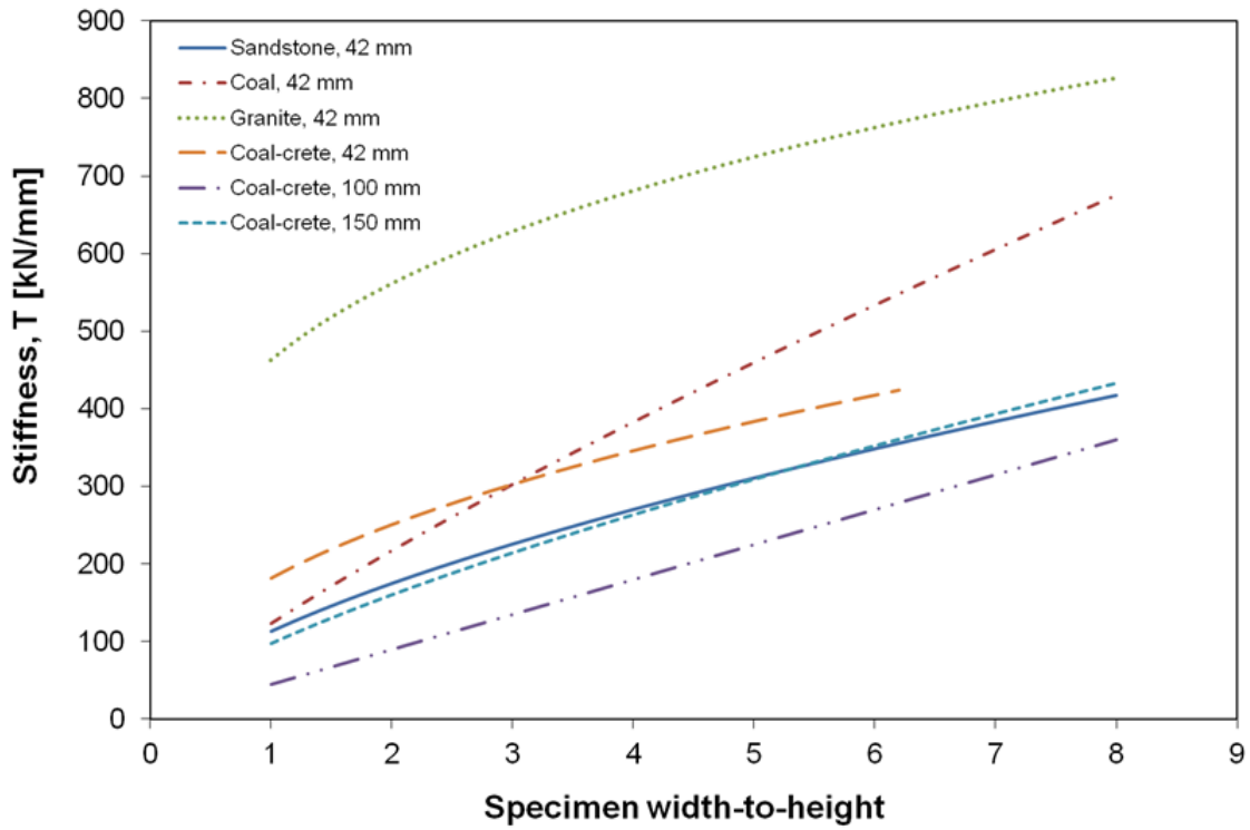
Figure 53. Specimen stiffness over w/h -ratio for different tested materials.
