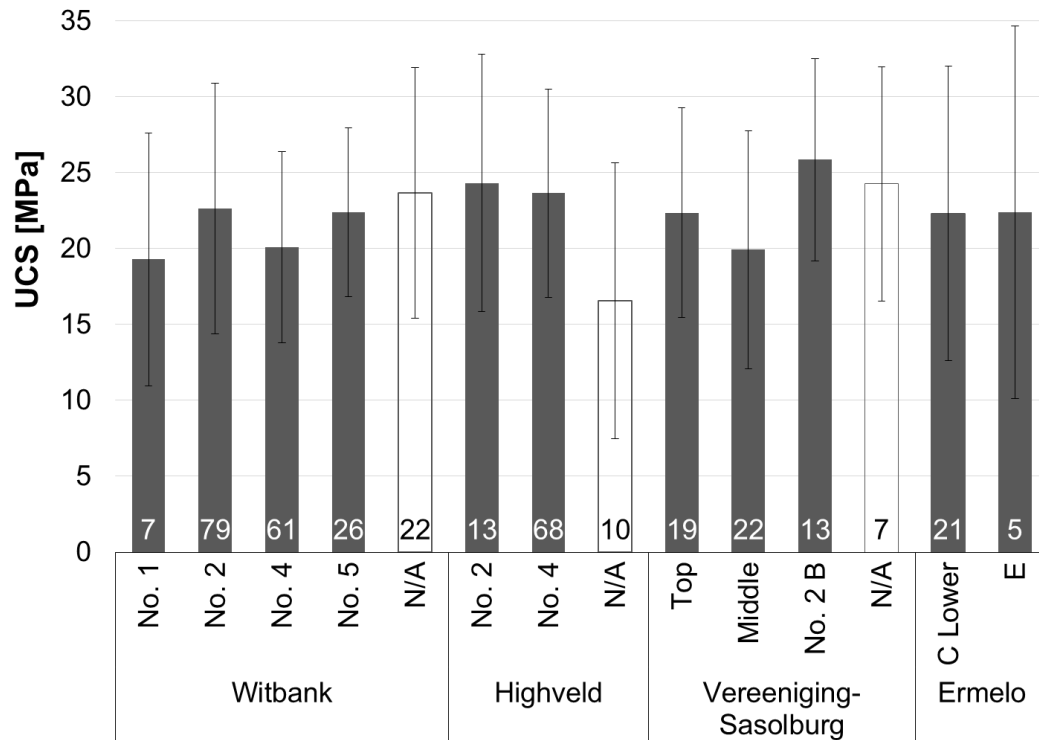
Figure 20. Seam-specific average UCS with accompanying standard deviations of coal in various coalfields in South Africa after removal of outliers in the dataset. The amount of tests evaluated per coal seam are given in the base of the columns.
