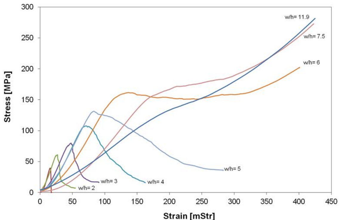
Figure 55. Examples of calculated stress-strain curves for sandstone specimens of 42 mm diameter at different w/h -ratios.
