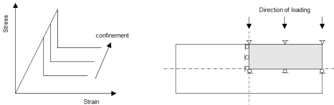
Figure 85. Schematic illustration of constitutive material model (left) and boundary conditions used in the pillar model scenarios S1 – S3 (right).
