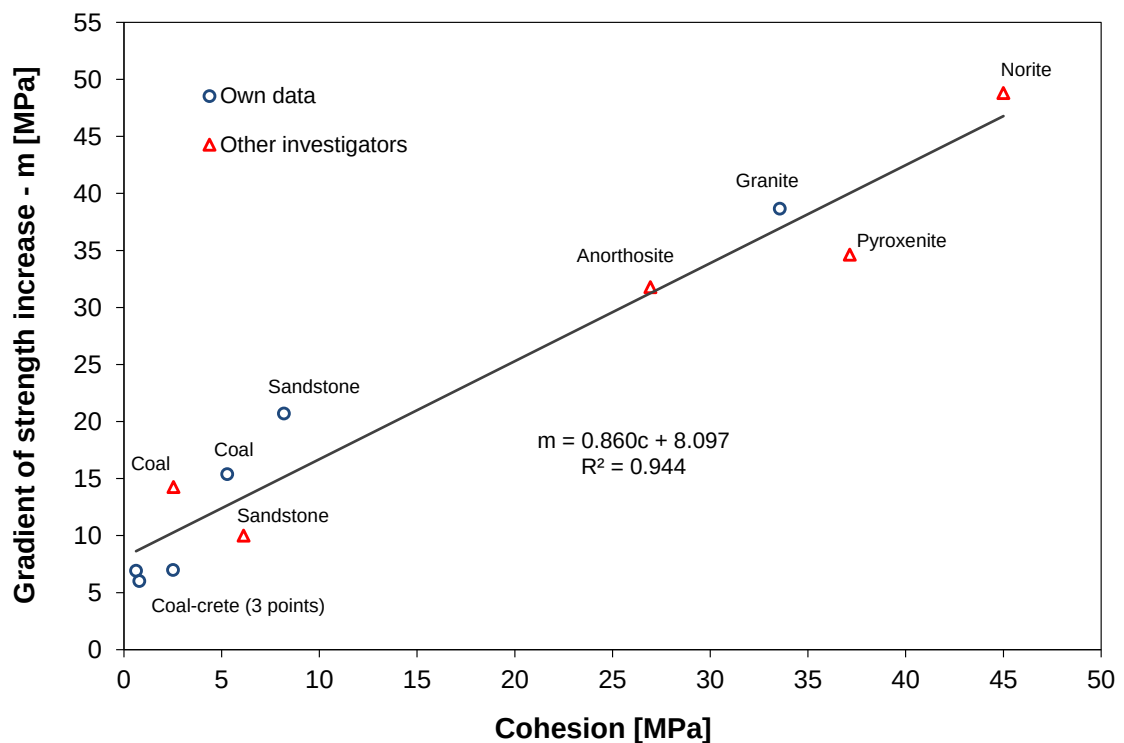
Figure 79. Correlation between the material cohesion ( c ) and the gradient of strength increase ( m ) over 1 \leq w/h \leq 4 .
