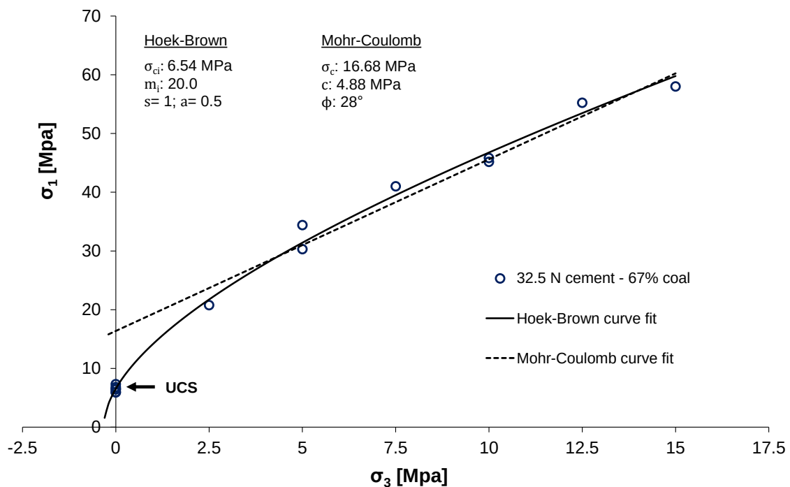
Figure 47. Mohr-Coulomb and Hoek-Brown curve fit for a coal-crete with 32.5 N cement and 67 % coal content.
