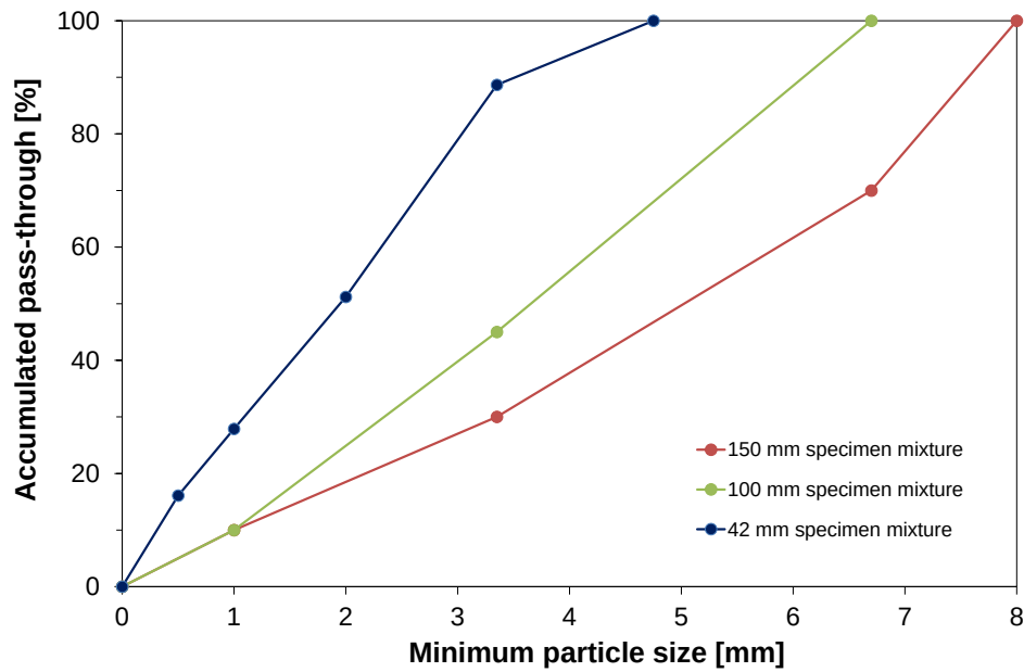
Figure 48. Grain-size distribution for coal debris used in the coal-crete mixtures for 42 mm, 100 mm and 150 mm specimens.
