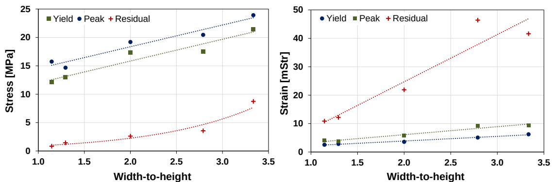
Figure 100. Average yield, peak and residual stress and strains in coal pillars of different w/h -ratios tested by Van Heerden.
