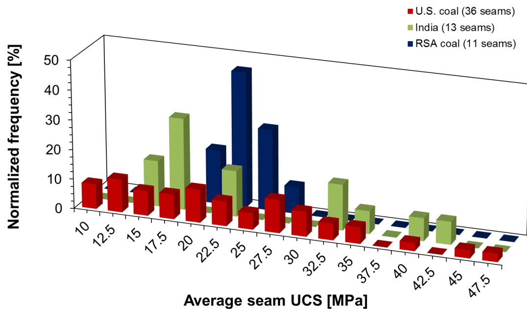
Figure 39. Normalized frequency distribution of average uniaxial compressive strength in 11 South African, 13 Indian and 36 U.S. coal seams.
