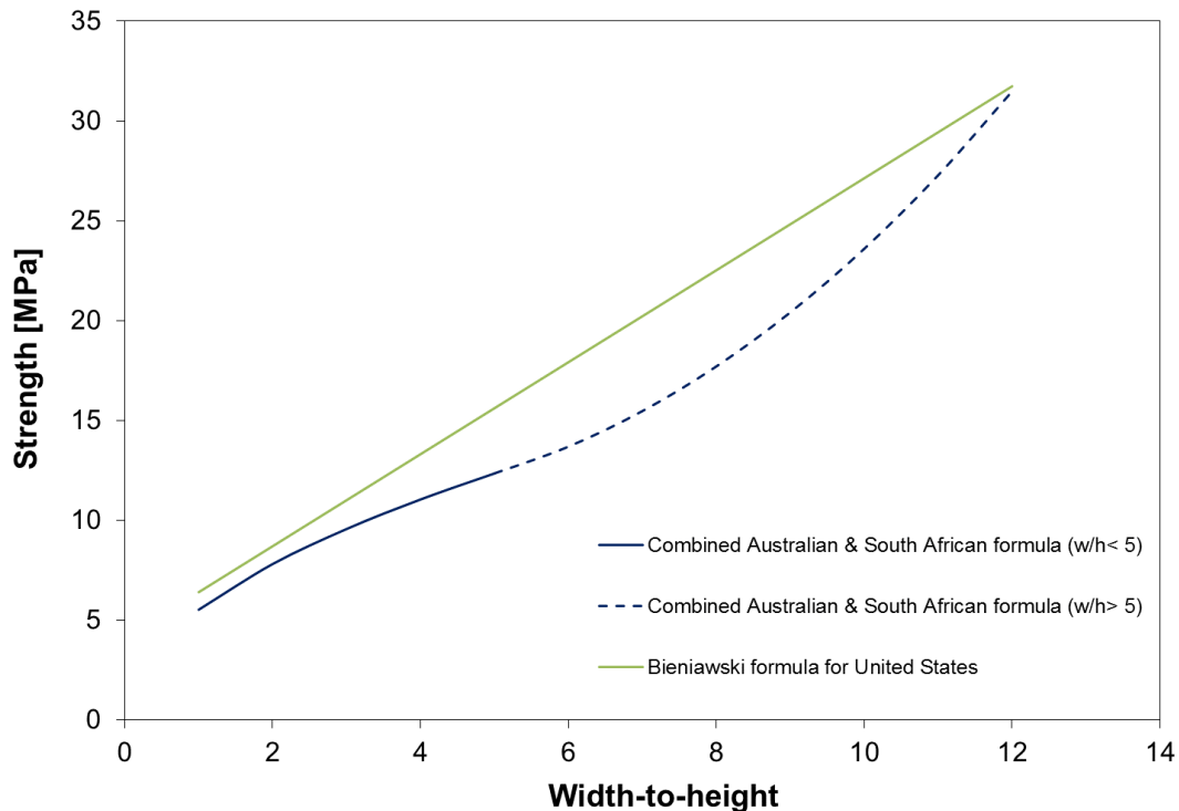
Figure 2. Shape effects in coal pillars as predicted by the Bieniawski formula for the United States and the combined Australian and South African formulae.
