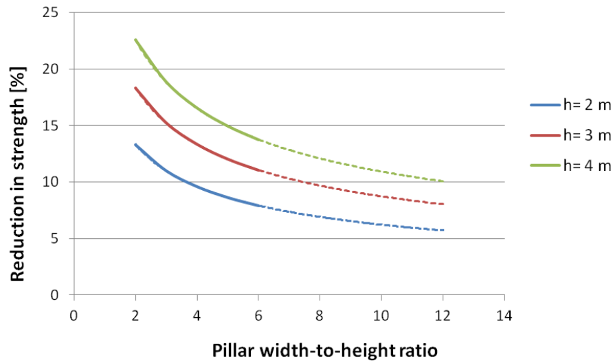
Figure 13. Reduction of strength for pillars of 2 – 4 m height due to a set of 2 m distant joints inclined at an angle of 30^\circ .
