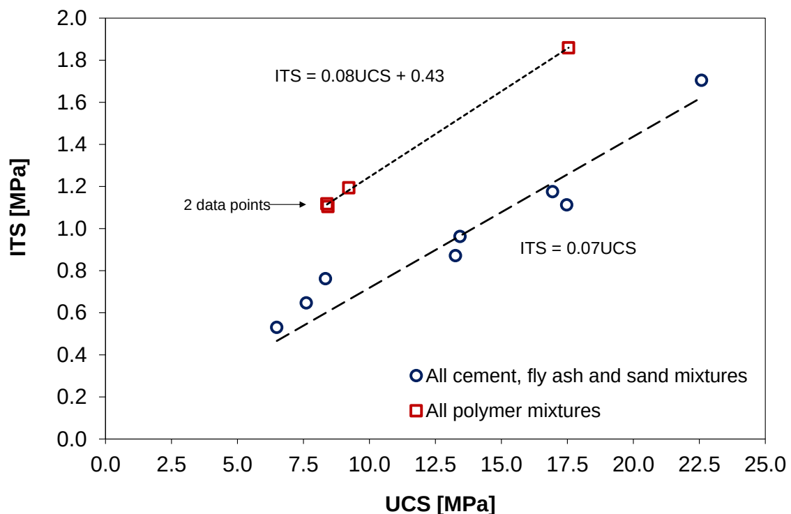
Figure 46. Relationship between ITS and UCS of coal-crete.
