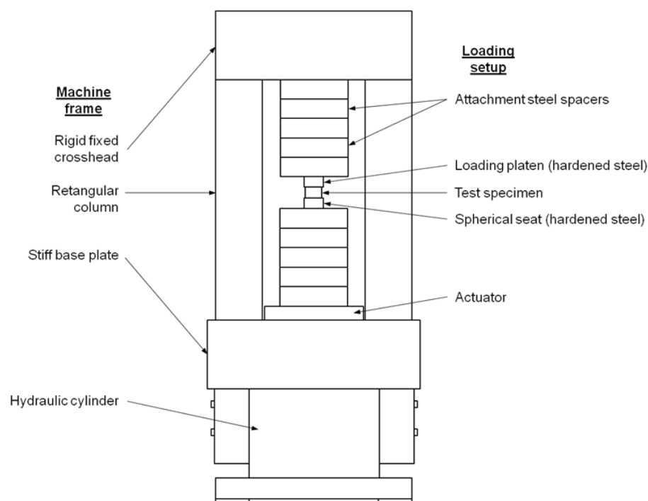
Figure 49. Schematic drawing of the testing apparatus
