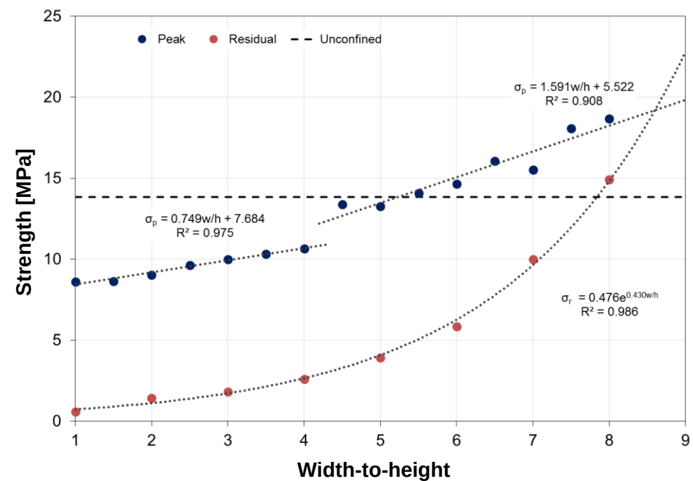
Figure 88. FLAC-computed peak and residual pillar strength versus w/h -ratio for model pillars in scenario S2.
