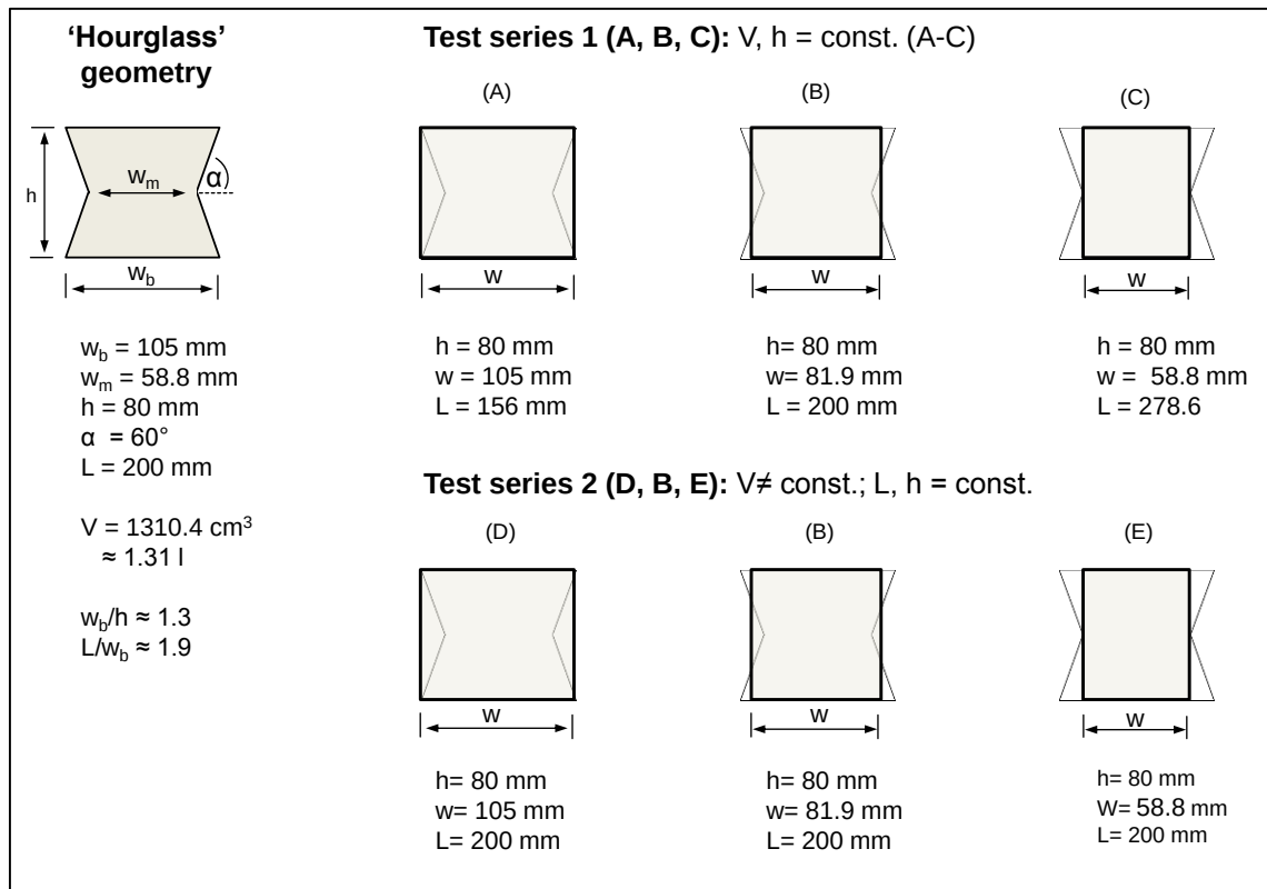
Figure 105. Test specimen design for laboratory investigation into the strength of 'hour-glass' shaped pillars.
