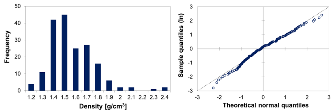
Figure 16. Density histogram for all ITS specimens (left) and QQ -plot for a hypothesised lognormal distribution of the density up to 2.0 \text{ g/cm}^3 (right).
