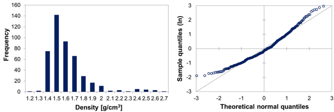
Figure 15. Density histogram for UCS specimens (left) and QQ -plot (right) for a hypothesised lognormal distribution of UCS specimen density up to 2.1 \text{ g/cm}^3 .
