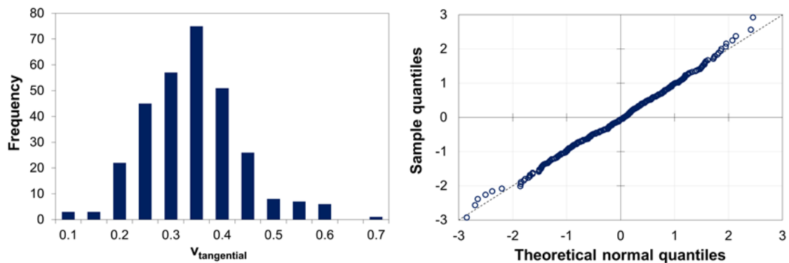
Figure 23. Histogram for the tangential Poisson's Ratio measured on 322 coal specimens (left) and QQ -plot for a hypothesised normal distribution of the sample data (right).
