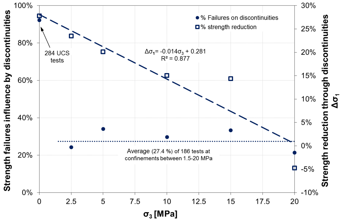
Figure 27. Influence of confinement on the failure mode and average peak strength of coal specimens.
