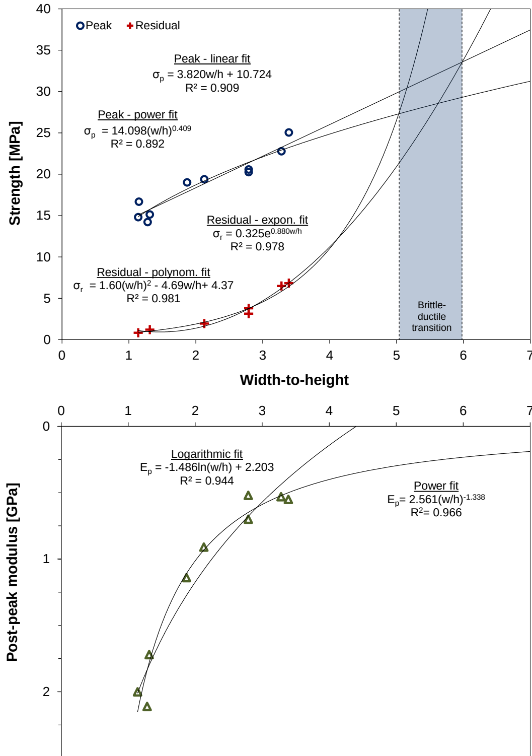
Figure 101. Extrapolated trends for peak and residual strength (top) and post-peak stiffness (below) in Van Heerden's large-scale in-situ tests.
