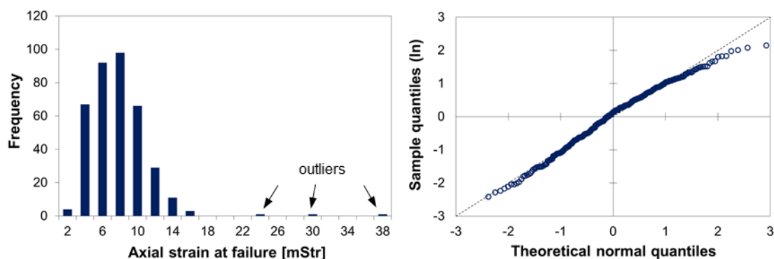
Figure 14. Histogram of the axial strain at strength failure for UCS specimens (left) and QQ -plot (right) for a hypothesised lognormal distribution of the data.
