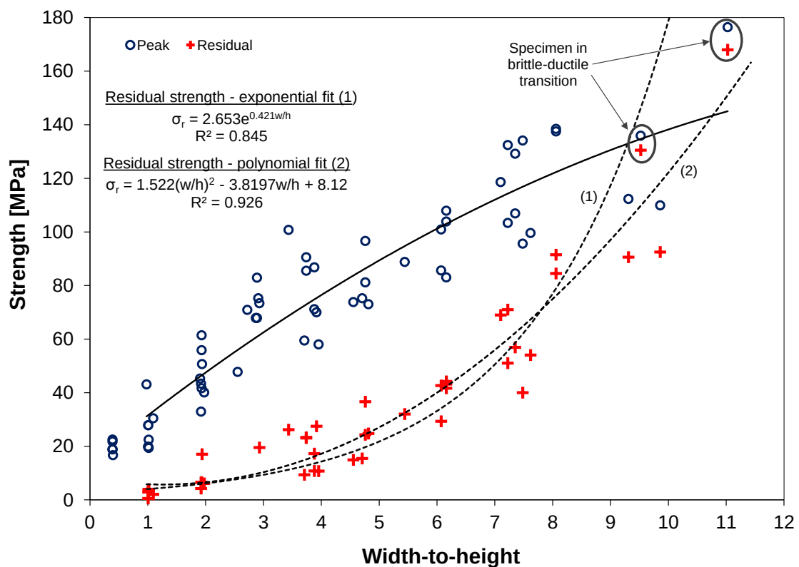
Figure 97. Trends in the residual strength of coal specimens of different w/h -ratio.
