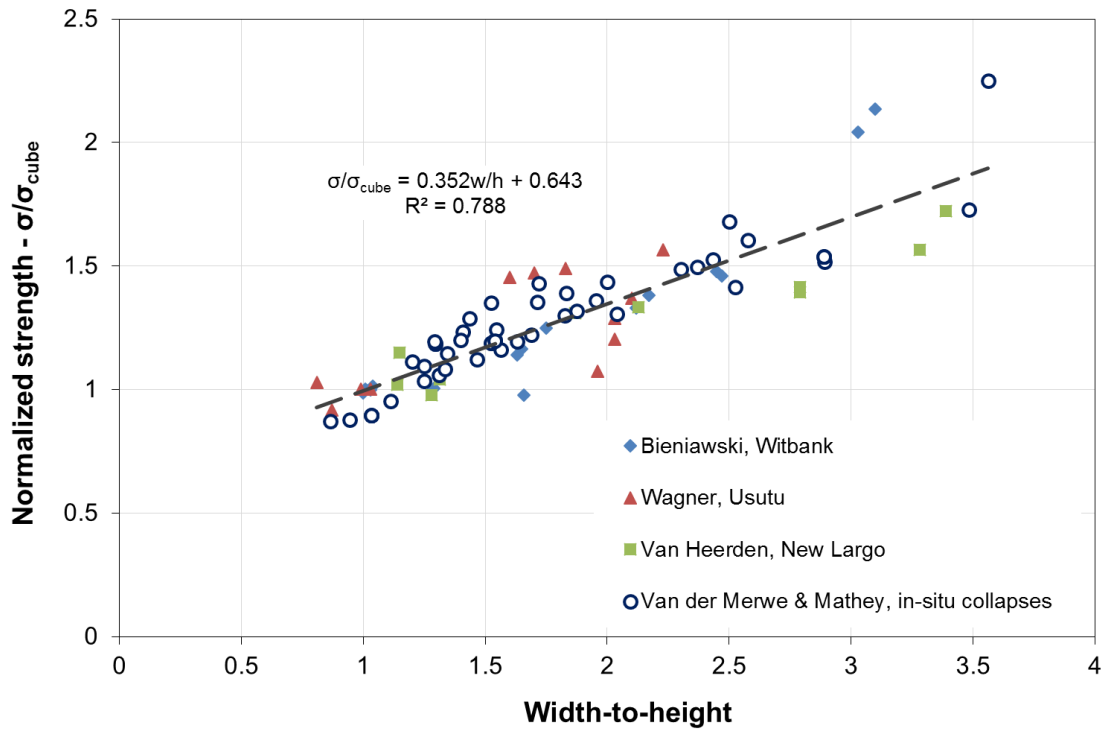
Figure 82. Strength of coal pillars normalized to the strength of a coal cube.
