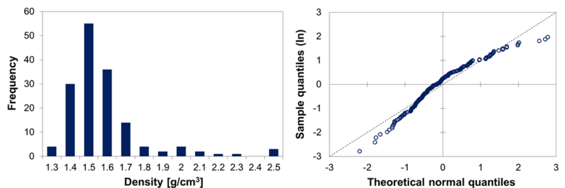
Figure 17. Density histogram for all TCS specimens (left) and QQ -plot for a hypothesised lognormal distribution of the density up to 1.9 \text{ g/cm}^3 (right).
