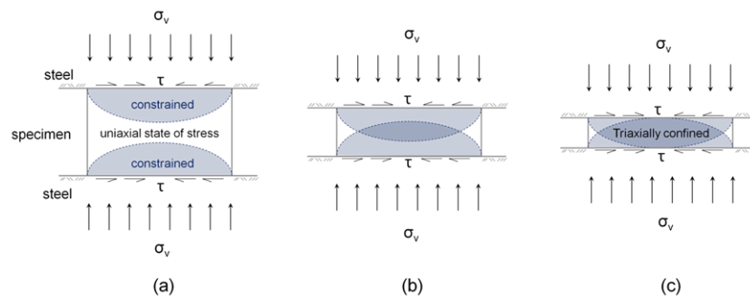
Figure 54. Schematic illustration of end-effects and induced triaxial stress-state in compression tests on flat specimen.
