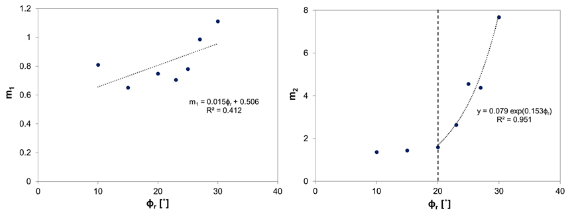
Figure 93. Rates of pillar strength increase m_1 and m_2 prior and subsequent to the squat effect as a function of the assigned residual friction in failed zones of the FLAC models.
