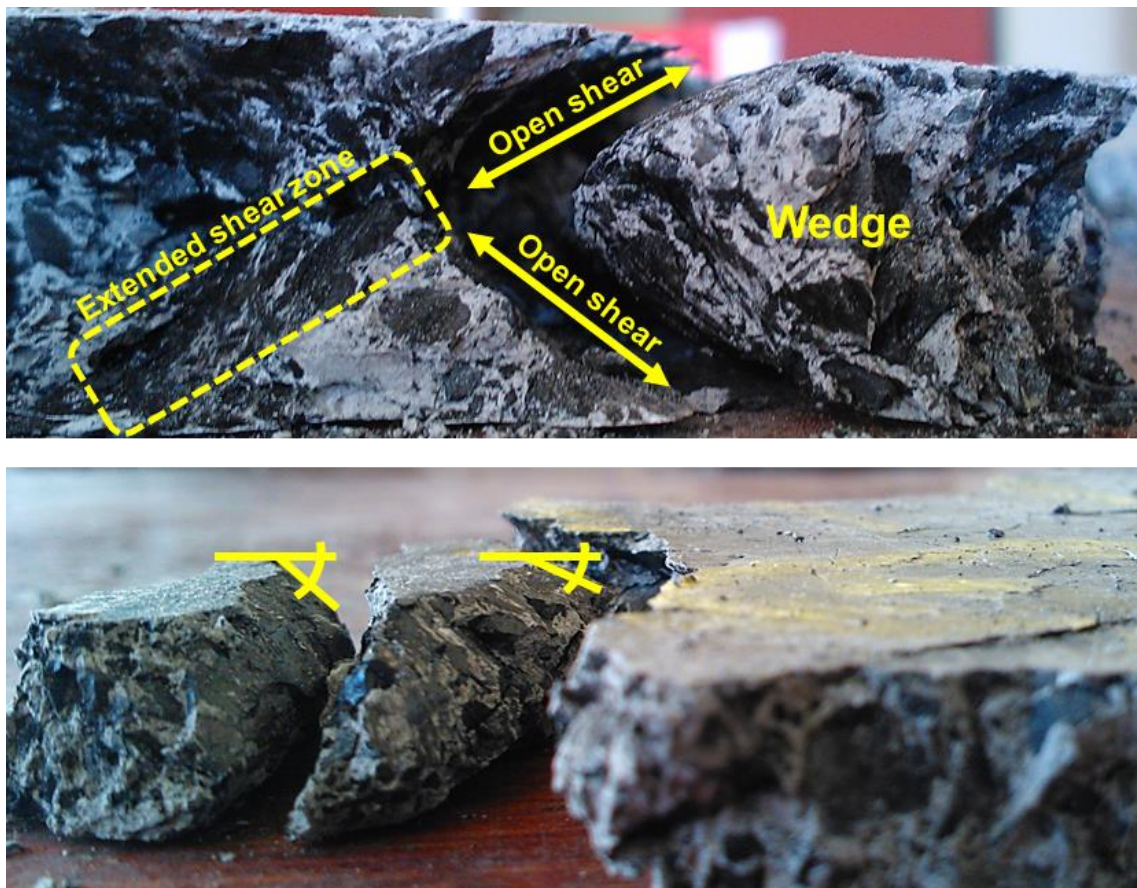
Figure 72. Coal-crete specimens of w/h = 5 in side-view after failure.
