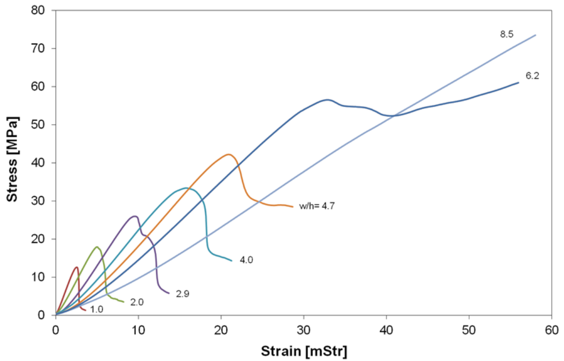
Figure 58. Examples of calculated stress-strain curves for coal-crete specimens of 42 mm diameter at different w/h -ratios.
