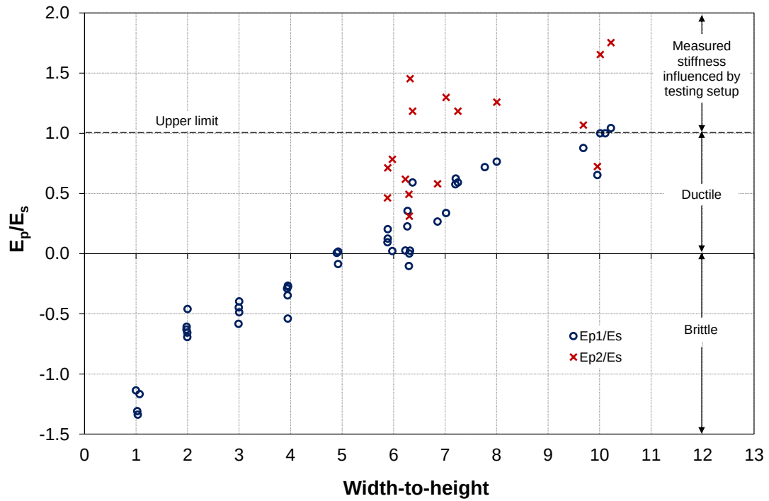
Figure 61. Modulus ratios E_p/E_s for coal-crete specimen of 100 mm square width and varying w/h -ratios. The plotted values correspond very closely with those obtained for 150 mm square specimen.
