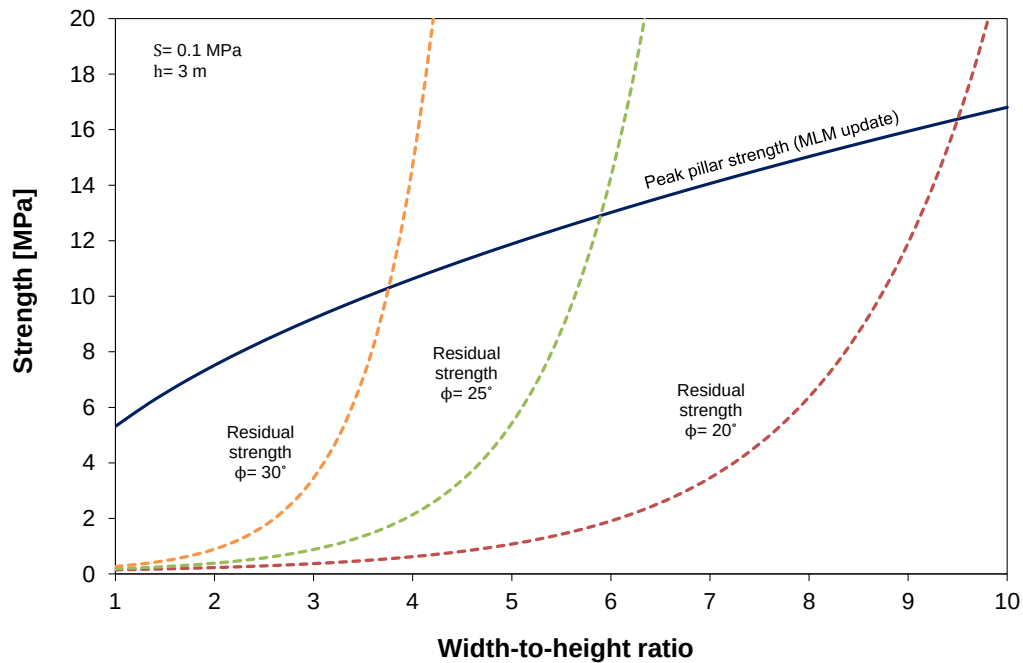
Figure 10. The residual strength of coal pillars for different internal friction angles \phi according to the analytical model of Napier and Malan.
